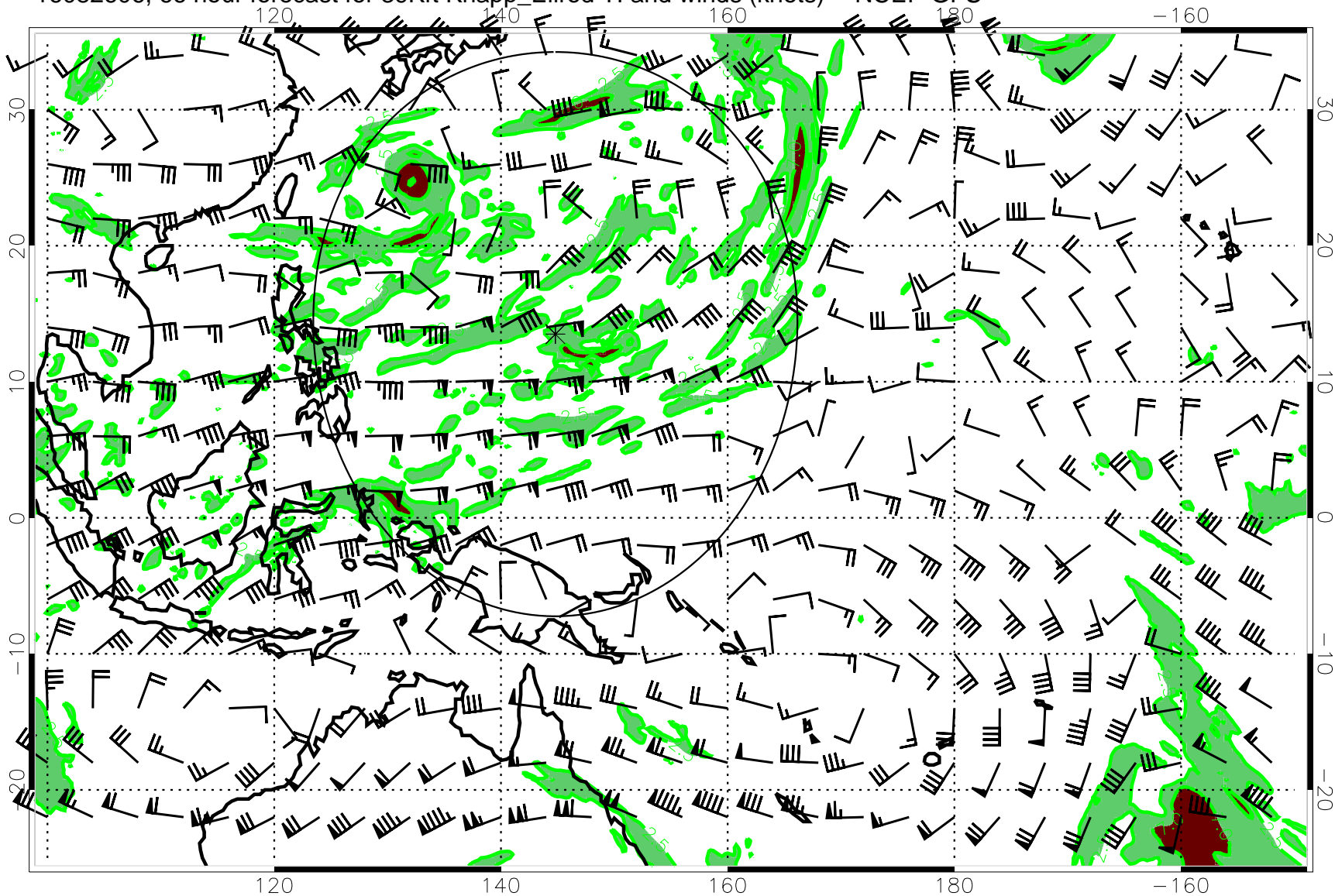
16082606, 66 hour forecast for 39Kft Knapp_Ellrod TI and winds (knots) -- NCEP GFS
