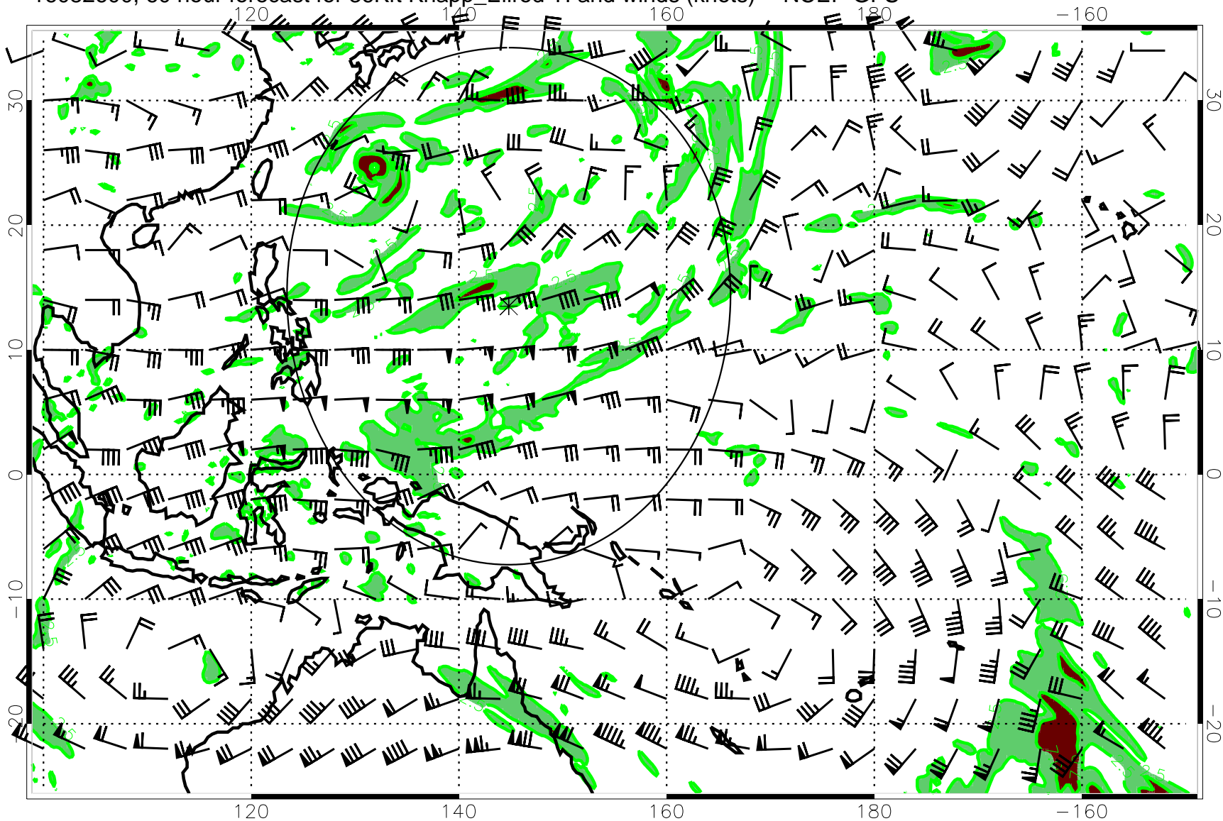
16082600, 60 hour forecast for 36Kft Knapp_Ellrod TI and winds (knots) -- NCEP GFS
