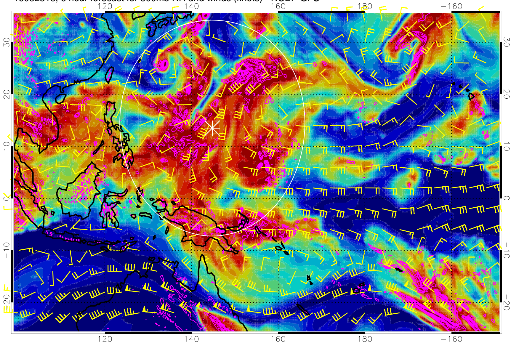
16082318, 6 hour forecast for 500mb RH and winds (knots) - NCEP GFS
