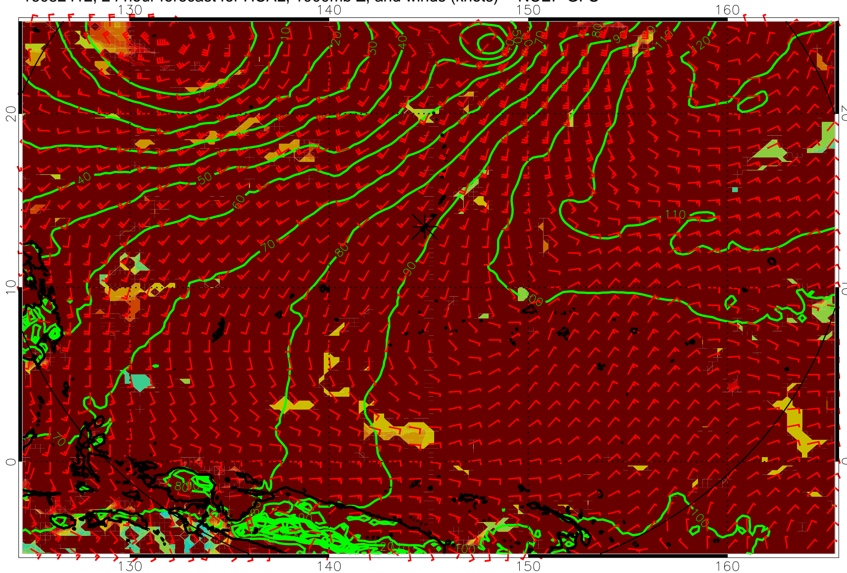
16082412, 24 hour forecast for HCAL, 1000mb Z, and winds (knots) -- NCEP GFS
