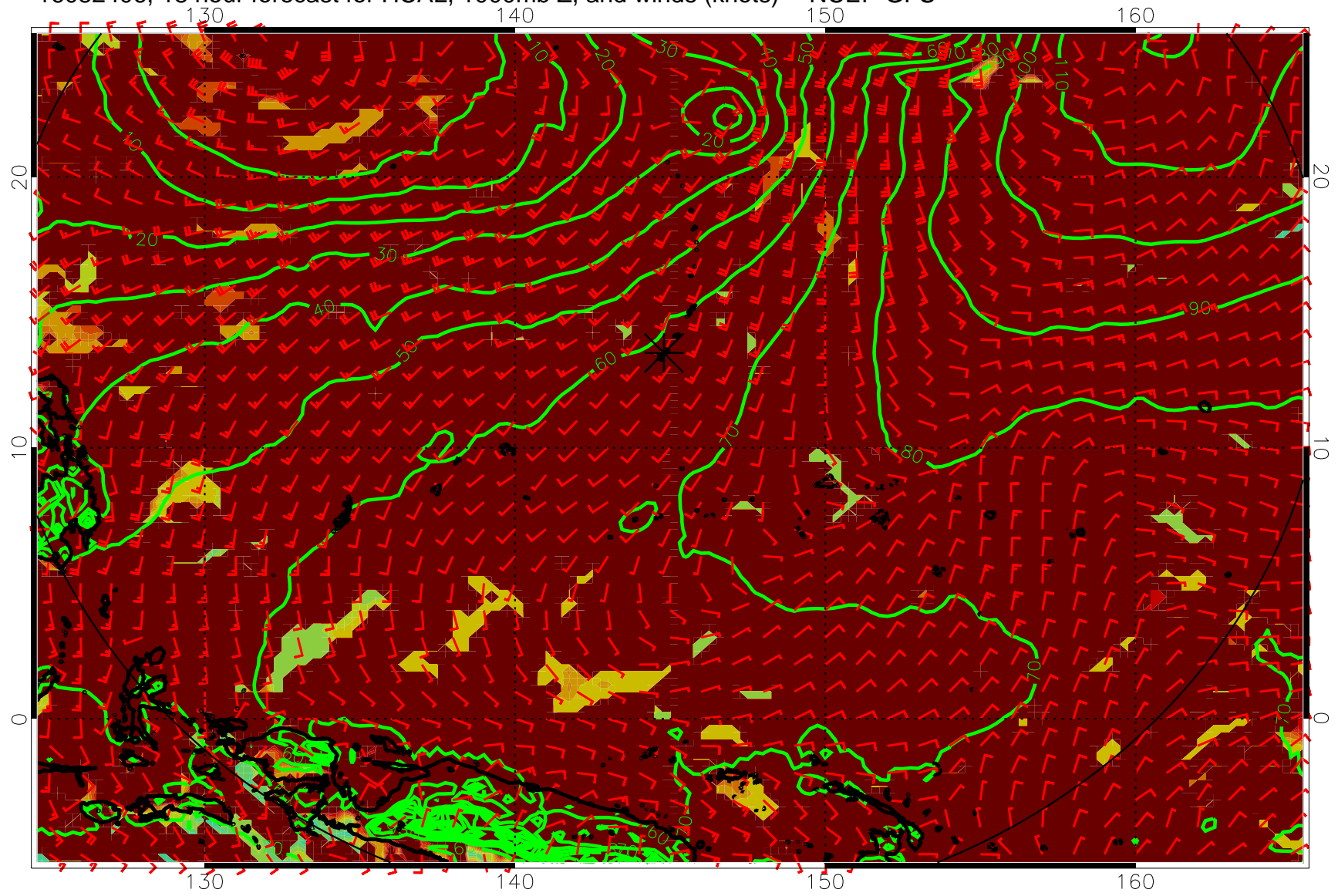
16082406, 18 hour forecast for HCAL, 1000mb Z, and winds (knots) -- NCEP GFS
