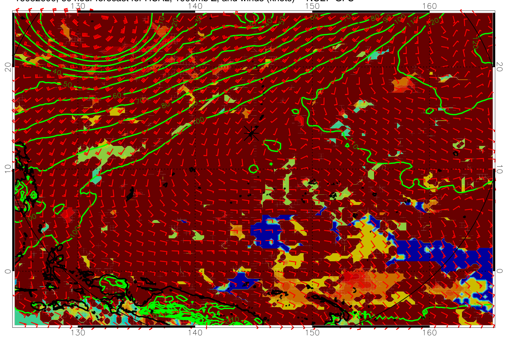
16082600, 60 hour forecast for HCAL, 1000mb Z, and winds (knots) -- NCEP GFS
