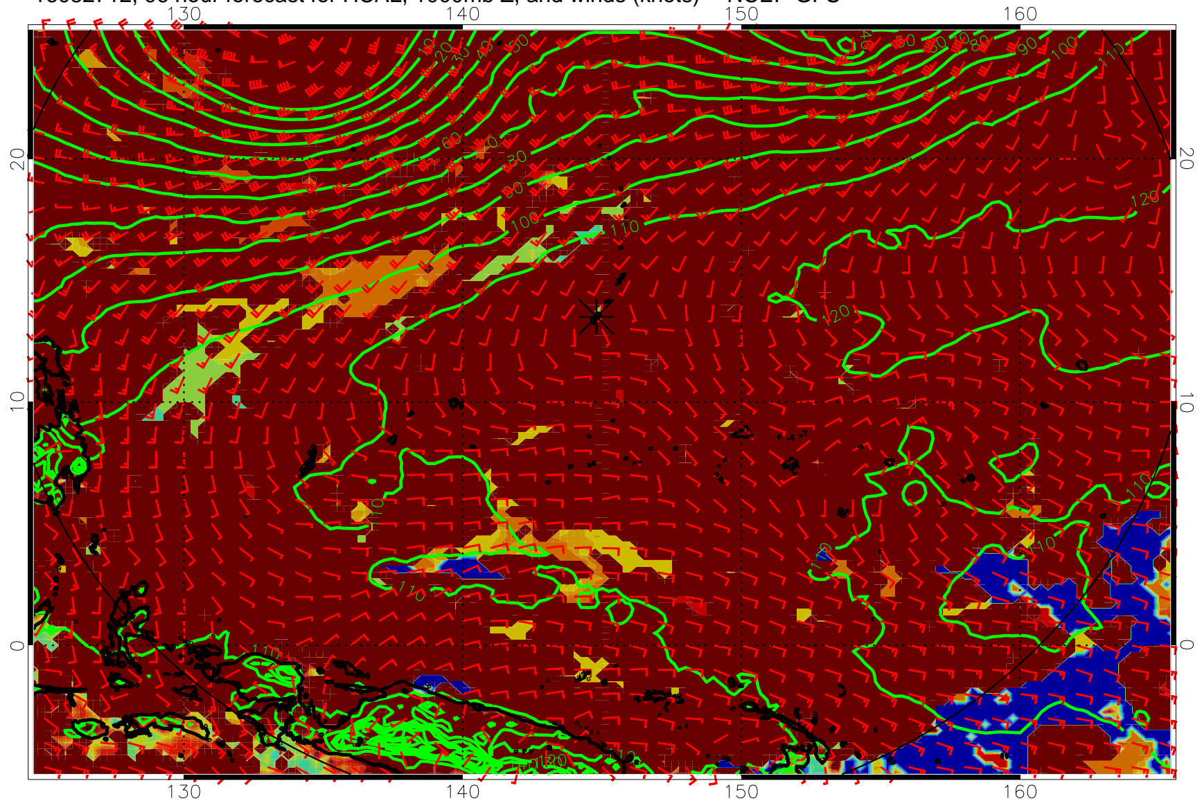
16082712, 96 hour forecast for HCAL, 1000mb Z, and winds (knots) -- NCEP GFS
