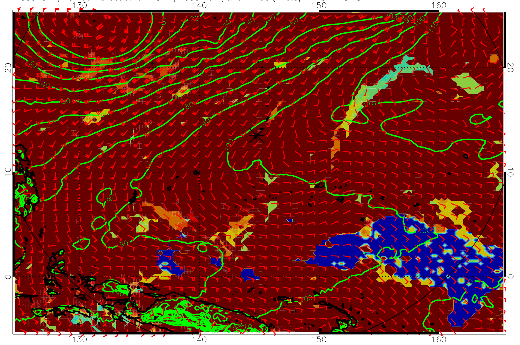
16082512, 48 hour forecast for HCAL, 1000mb Z, and winds (knots) -- NCEP GFS
