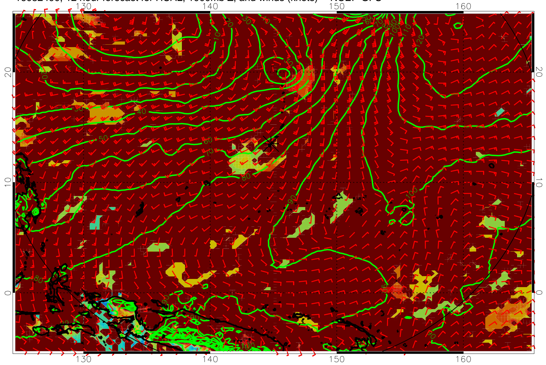
16082400, 12 hour forecast for HCAL, 1000mb Z, and winds (knots) -- NCEP GFS
