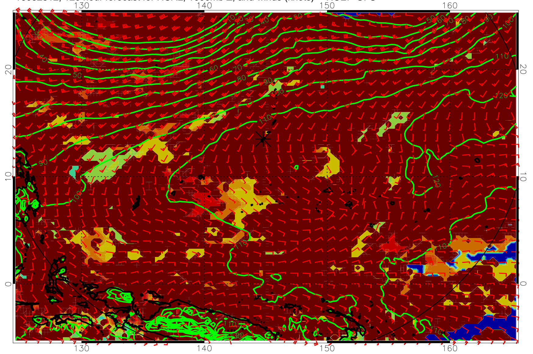
16082812, 120 hour forecast for HCAL, 1000mb Z, and winds (knots) -- NCEP GFS
