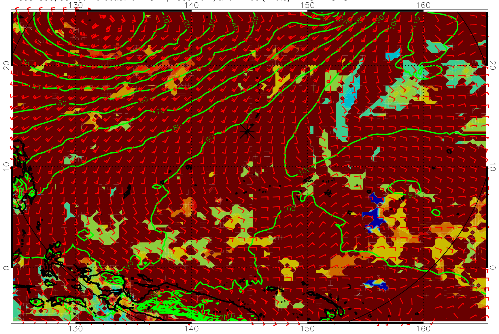
16082500, 36 hour forecast for HCAL, 1000mb Z, and winds (knots) -- NCEP GFS
