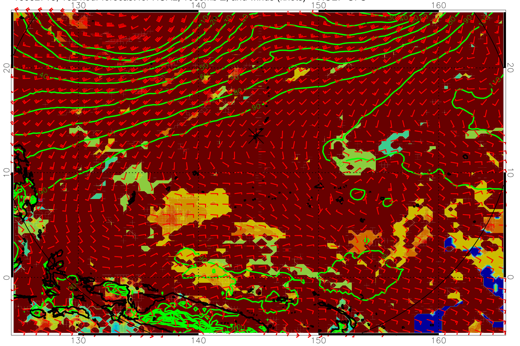
16082718, 102 hour forecast for HCAL, 1000mb Z, and winds (knots) -- NCEP GFS
