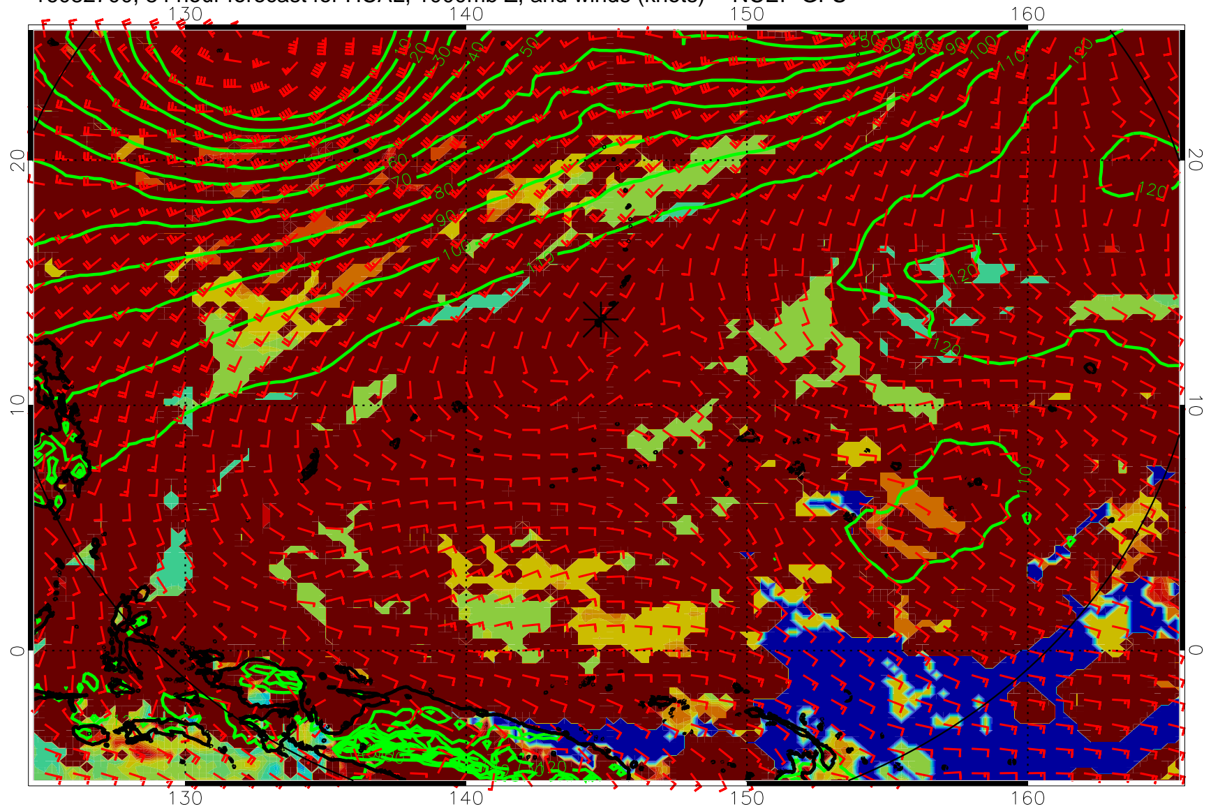
16082700, 84 hour forecast for HCAL, 1000mb Z, and winds (knots) -- NCEP GFS
