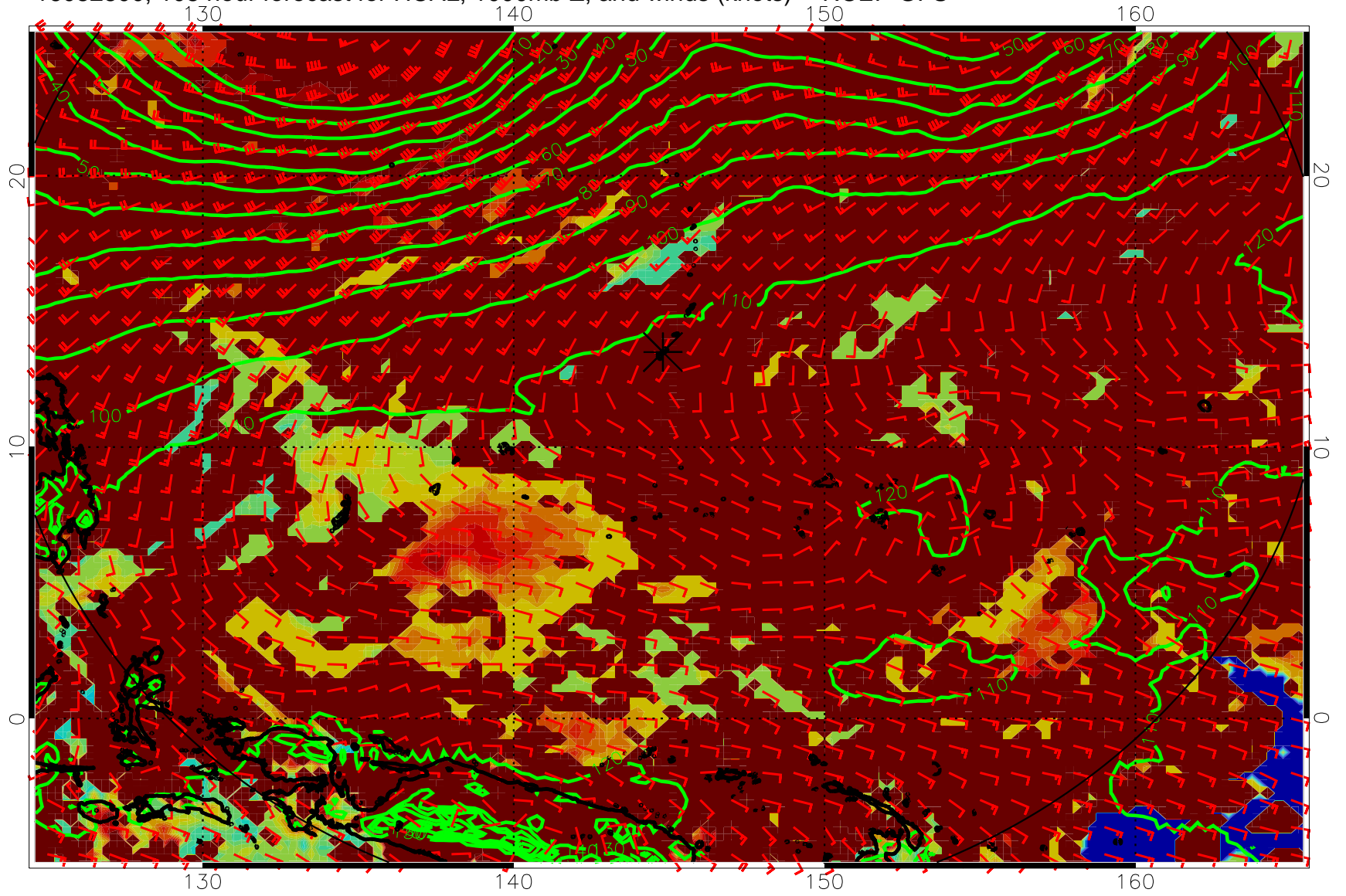
16082800, 108 hour forecast for HCAL, 1000mb Z, and winds (knots) -- NCEP GFS
