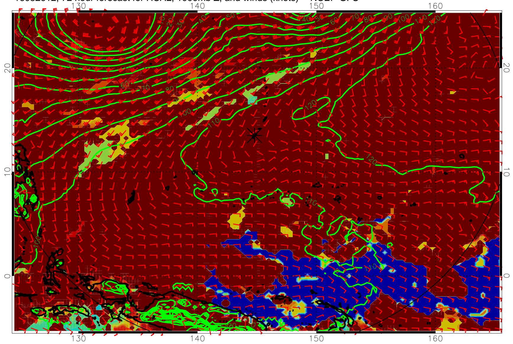
16082612, 72 hour forecast for HCAL, 1000mb Z, and winds (knots) -- NCEP GFS
