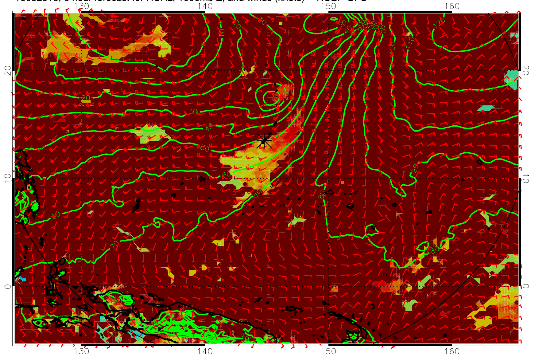
16082318, 6 hour forecast for HCAL, 1000mb Z, and winds (knots) -- NCEP GFS
