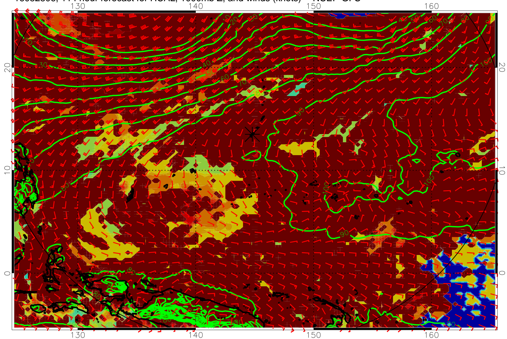
16082806, 114 hour forecast for HCAL, 1000mb Z, and winds (knots) -- NCEP GFS
