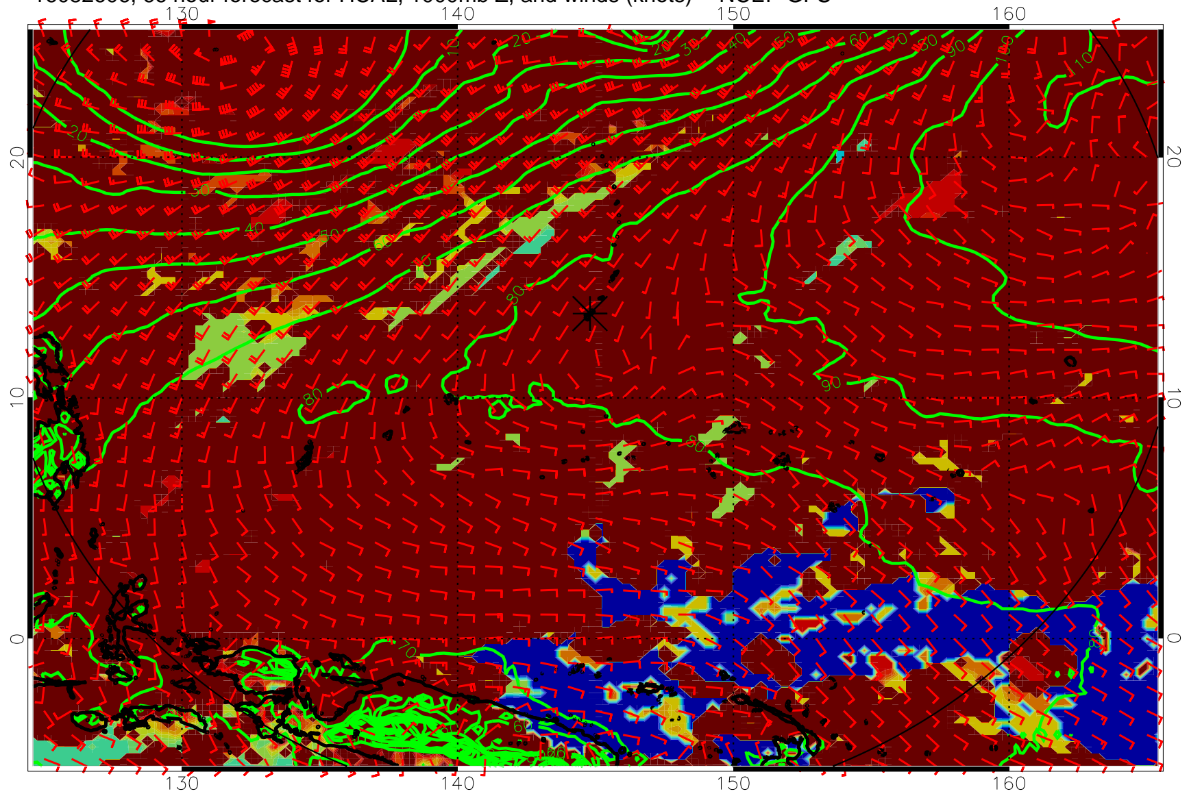
16082606, 66 hour forecast for HCAL, 1000mb Z, and winds (knots) -- NCEP GFS
