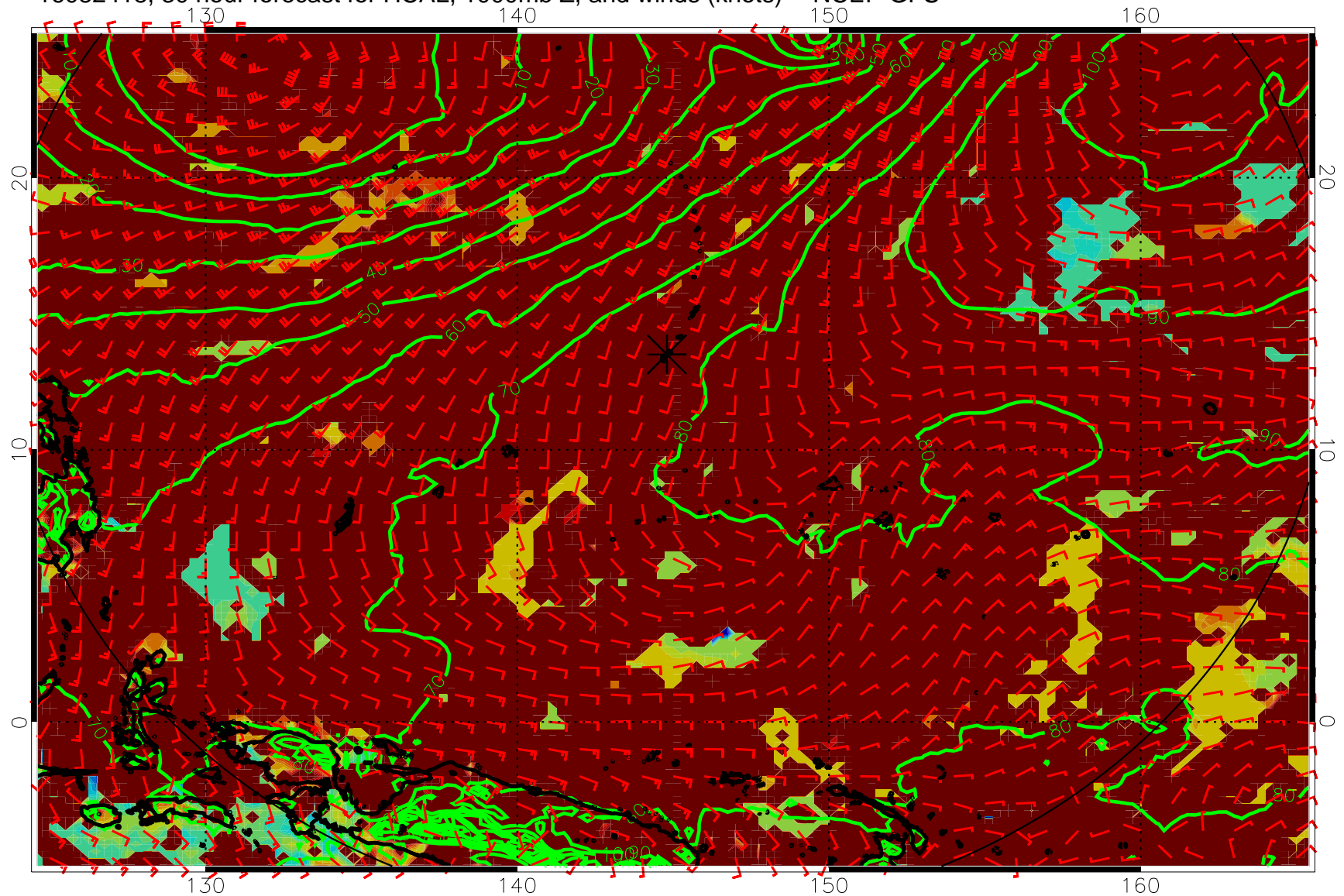
16082418, 30 hour forecast for HCAL, 1000mb Z, and winds (knots) -- NCEP GFS
