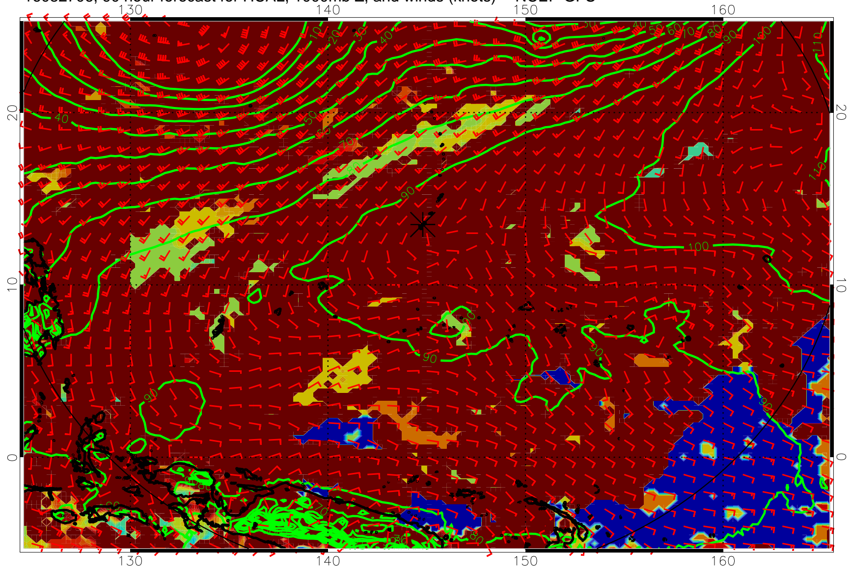
16082706, 90 hour forecast for HCAL, 1000mb Z, and winds (knots) -- NCEP GFS
