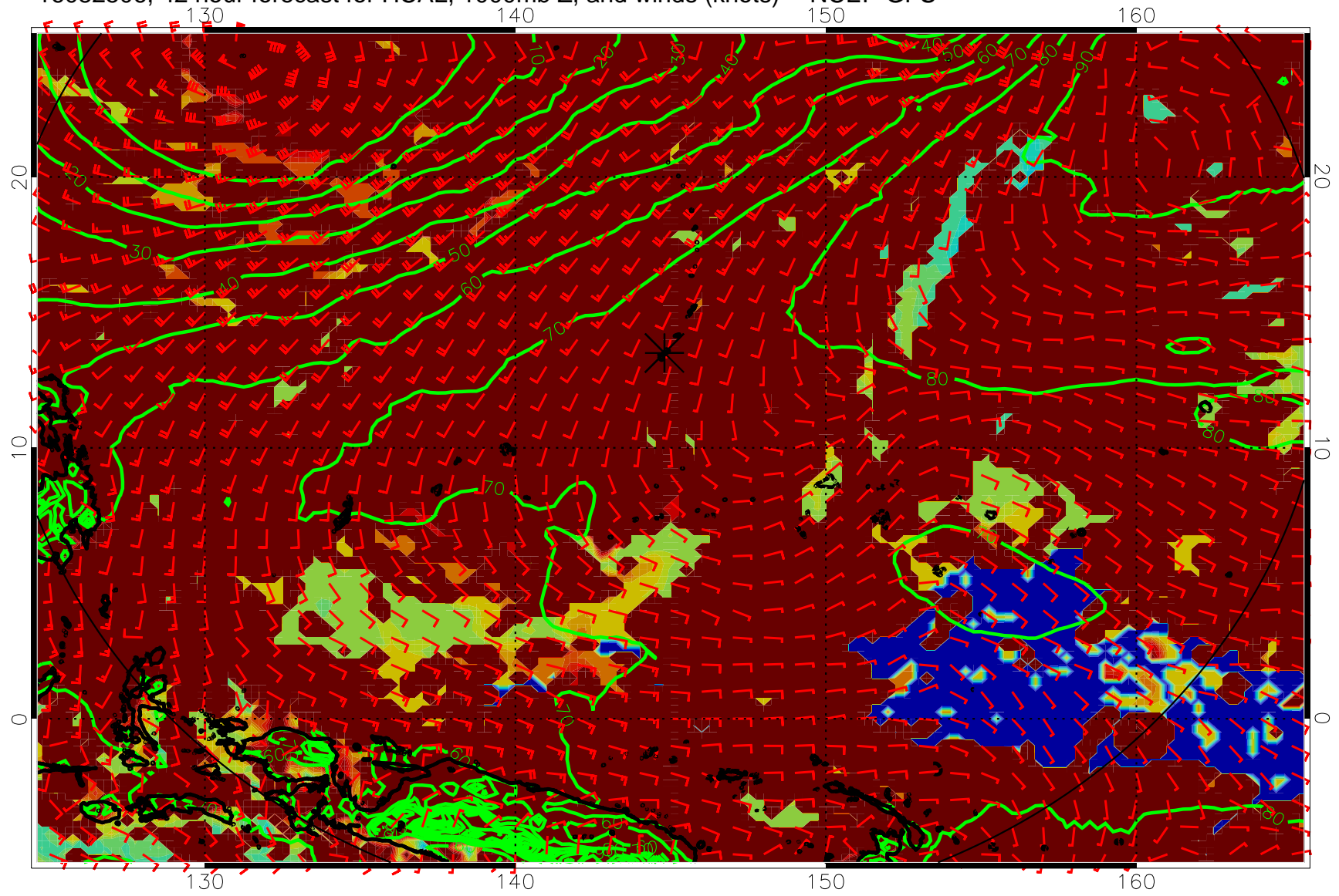
16082506, 42 hour forecast for HCAL, 1000mb Z, and winds (knots) -- NCEP GFS
