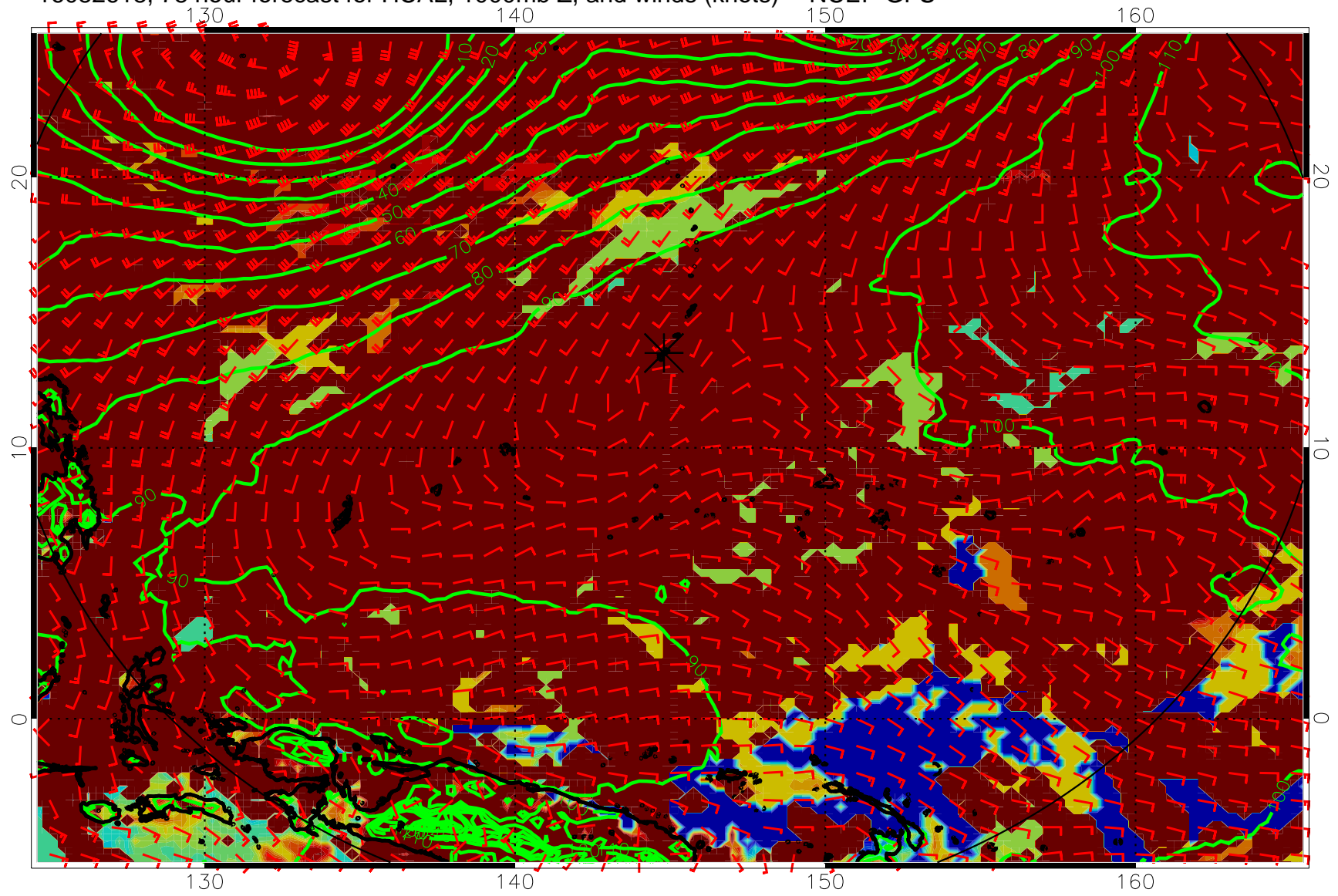
16082618, 78 hour forecast for HCAL, 1000mb Z, and winds (knots) -- NCEP GFS
