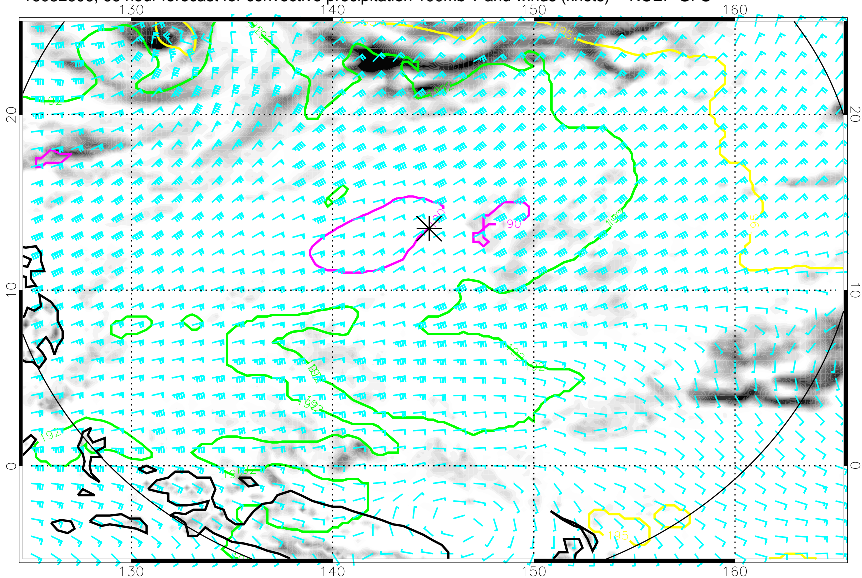
16082606, 66 hour forecast for convective precipitation 100mb T and winds (knots) -- NCEP GFS
