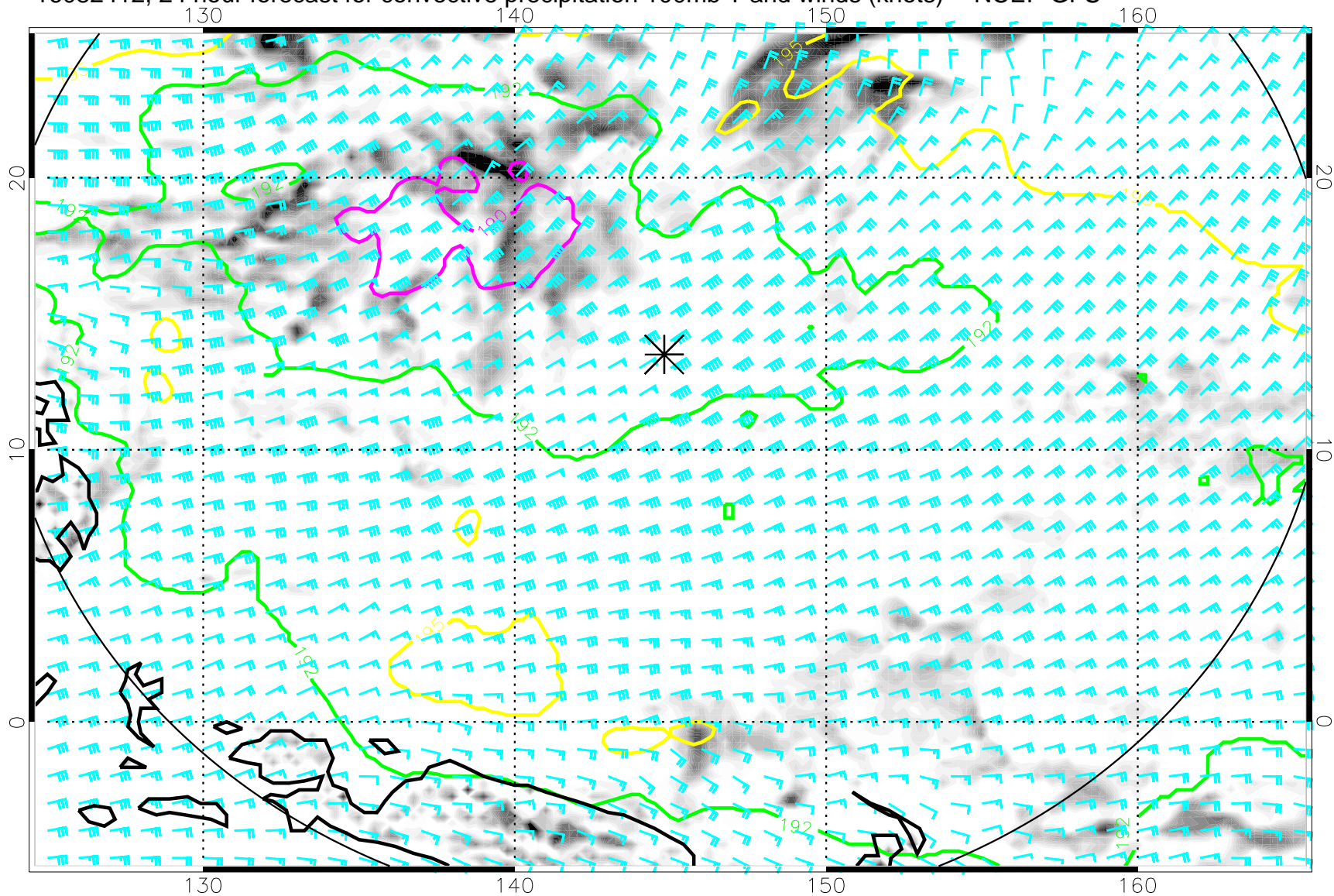
16082412, 24 hour forecast for convective precipitation 100mb T and winds (knots) -- NCEP GFS
