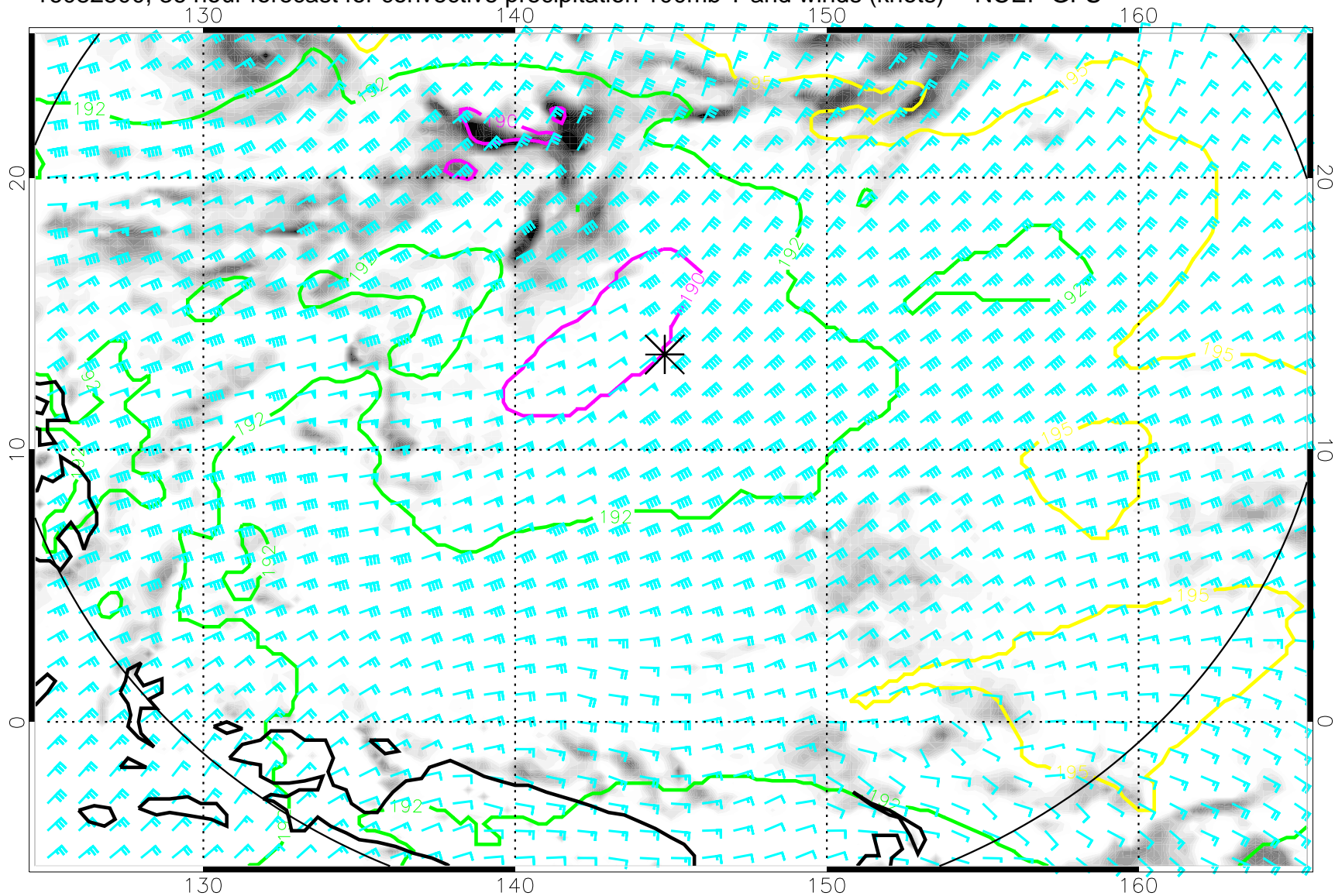
16082500, 36 hour forecast for convective precipitation 100mb T and winds (knots) -- NCEP GFS
