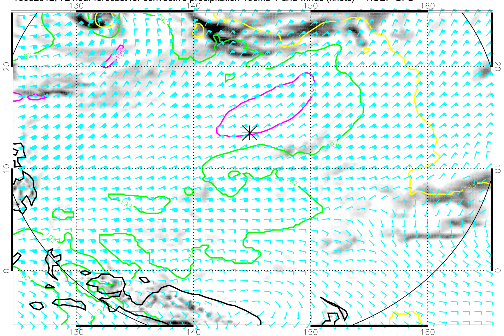
16082612, 72 hour forecast for convective precipitation 100mb T and winds (knots) -- NCEP GFS
