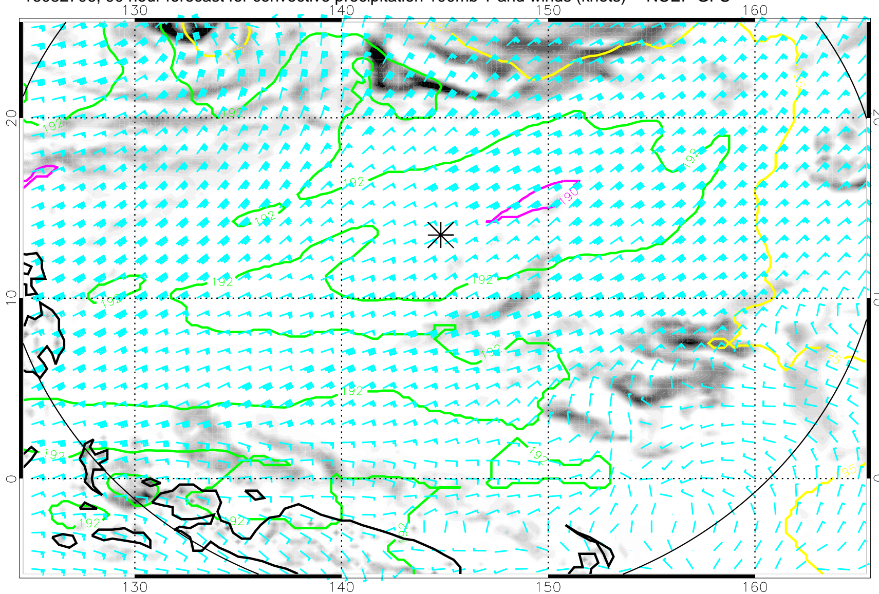
16082706, 90 hour forecast for convective precipitation 100mb T and winds (knots) -- NCEP GFS
