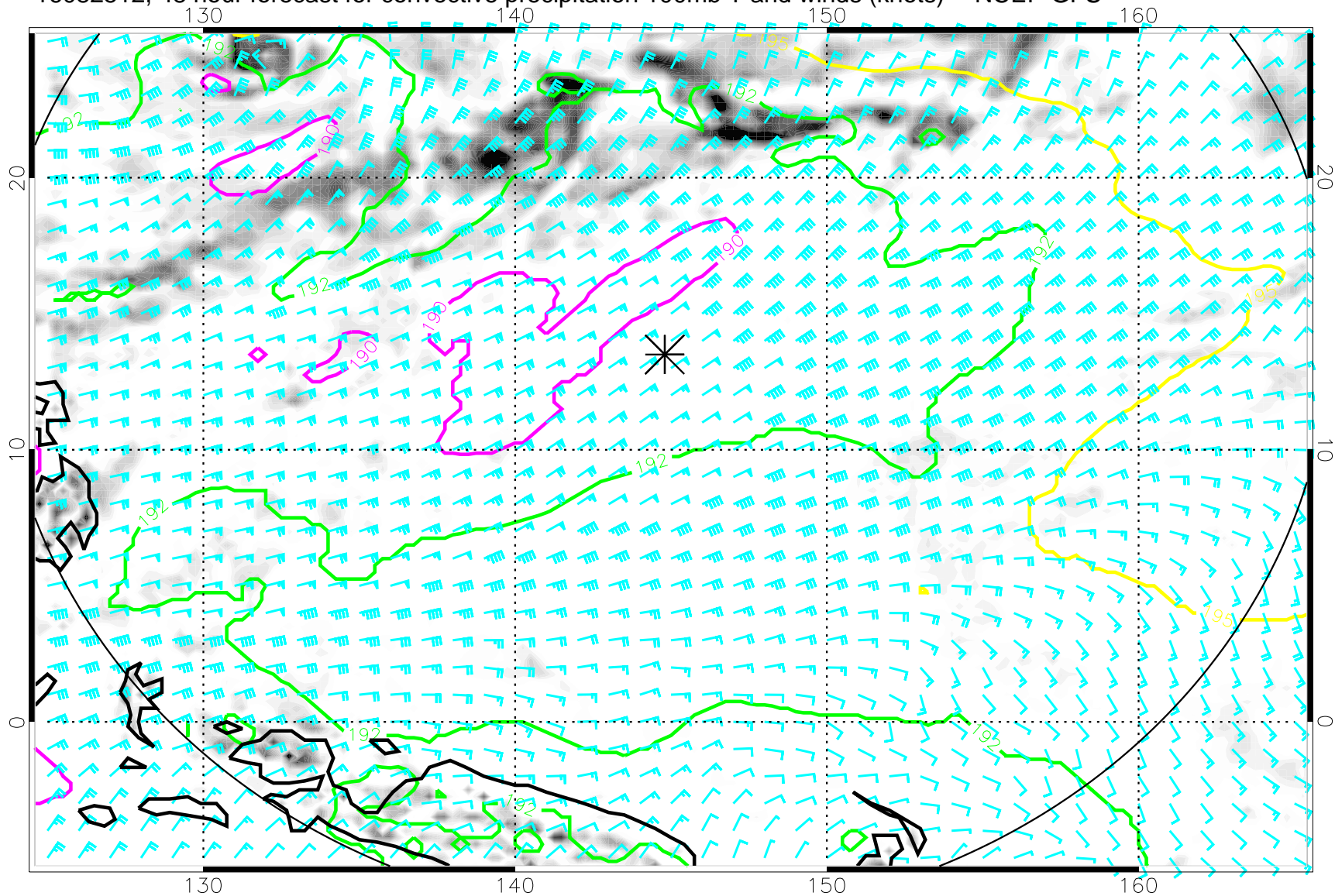
16082512, 48 hour forecast for convective precipitation 100mb T and winds (knots) -- NCEP GFS
