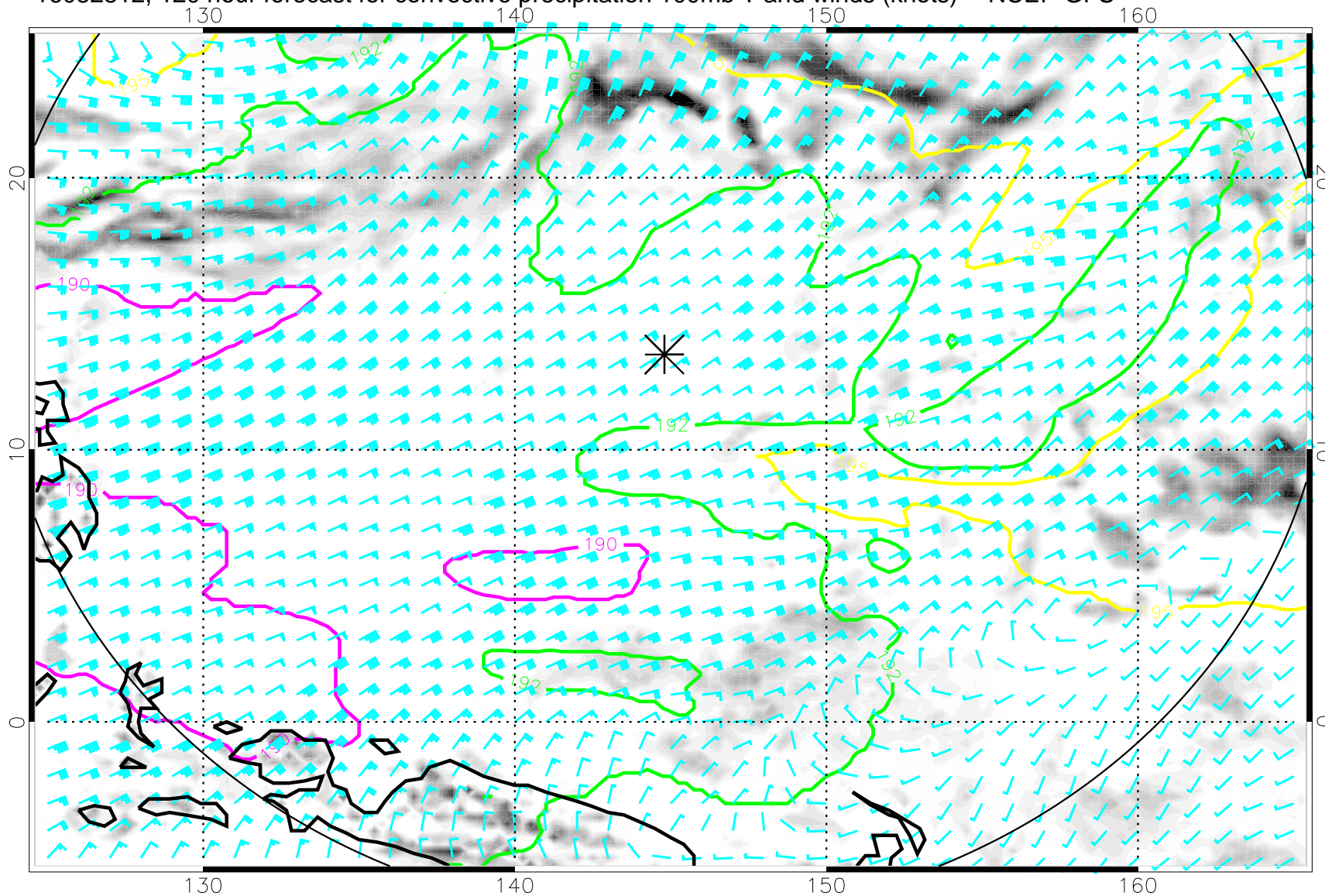
16082812, 120 hour forecast for convective precipitation 100mb T and winds (knots) -- NCEP GFS
