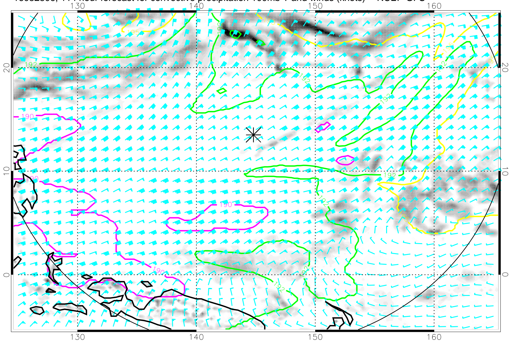
16082806, 114 hour forecast for convective precipitation 100mb T and winds (knots) -- NCEP GFS
