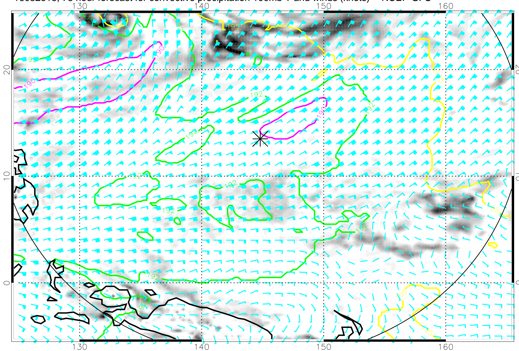
16082618, 78 hour forecast for convective precipitation 100mb T and winds (knots) -- NCEP GFS
