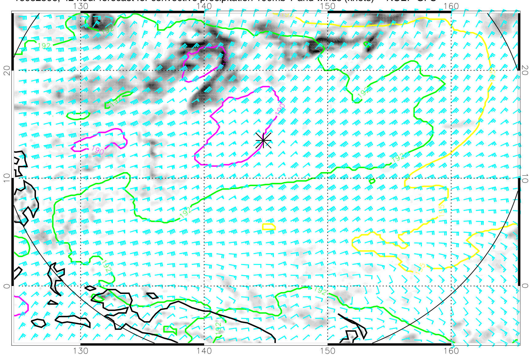
16082506, 42 hour forecast for convective precipitation 100mb T and winds (knots) -- NCEP GFS
