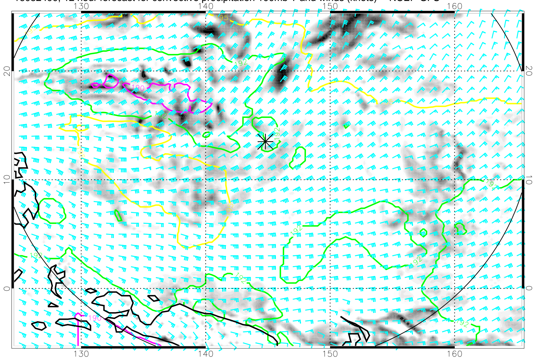
16082400, 12 hour forecast for convective precipitation 100mb T and winds (knots) -- NCEP GFS
