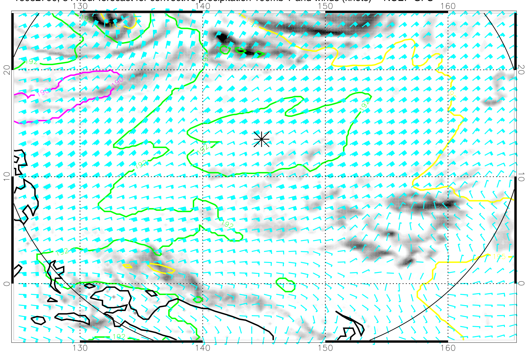
16082700, 84 hour forecast for convective precipitation 100mb T and winds (knots) -- NCEP GFS
