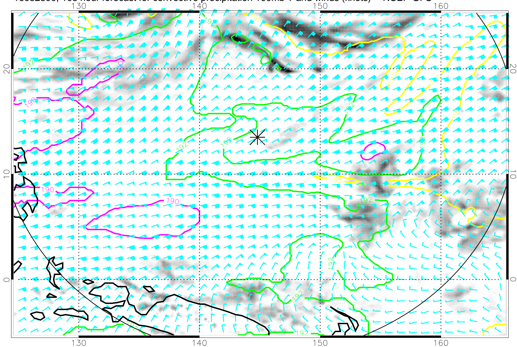
16082800, 108 hour forecast for convective precipitation 100mb T and winds (knots) -- NCEP GFS
