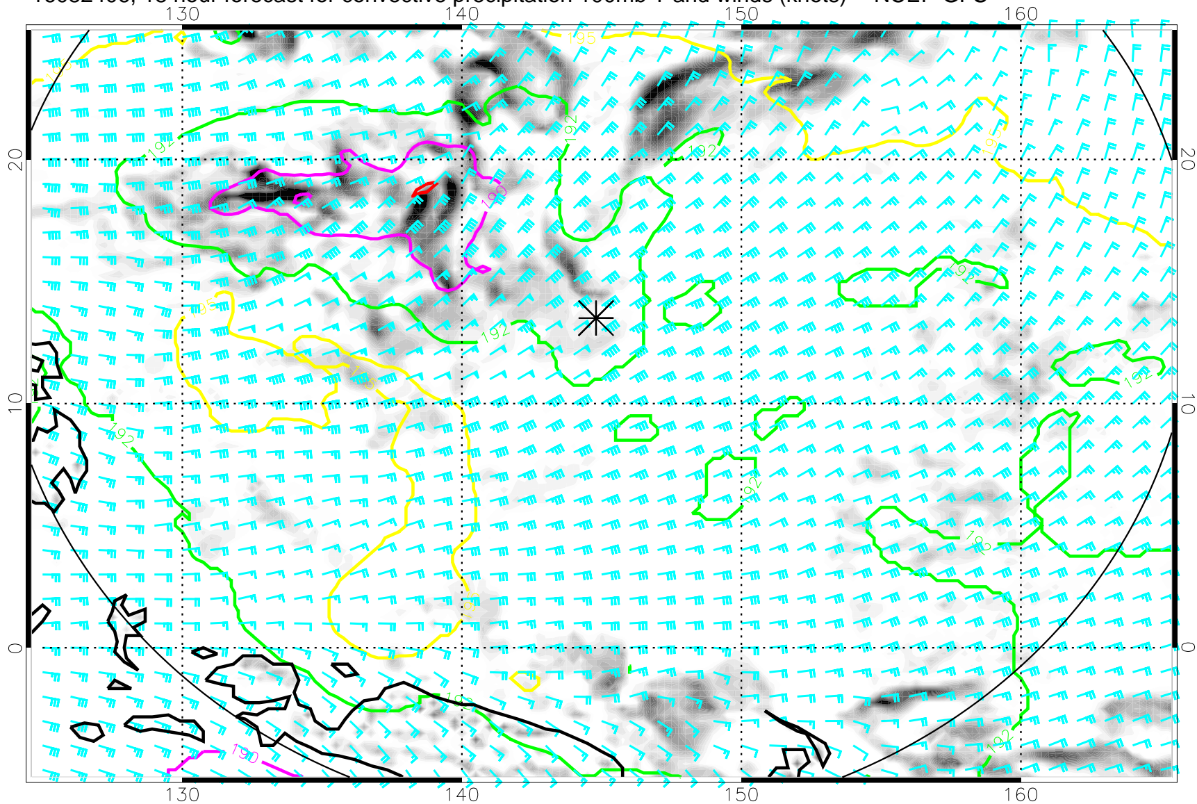
16082406, 18 hour forecast for convective precipitation 100mb T and winds (knots) -- NCEP GFS
