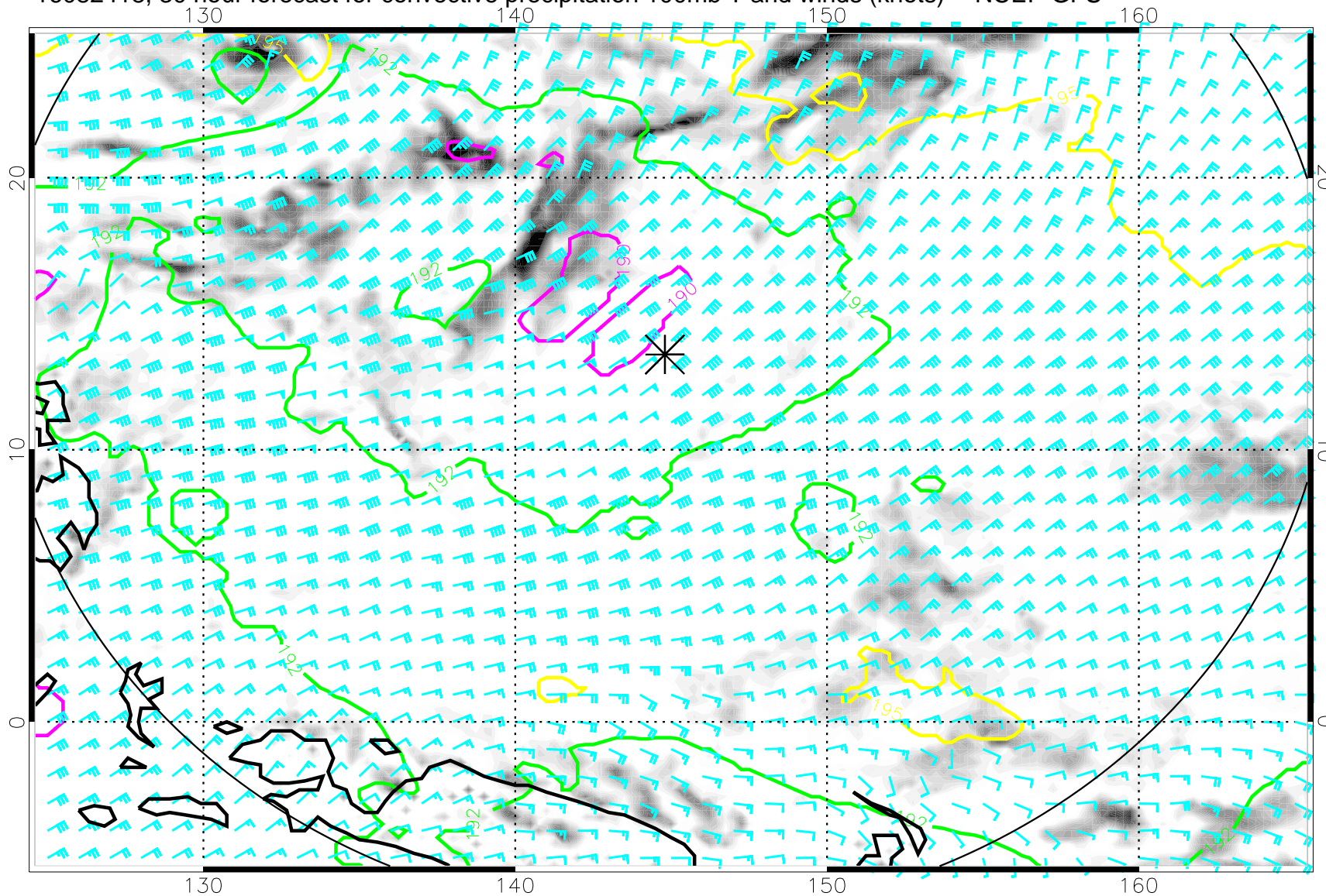
16082418, 30 hour forecast for convective precipitation 100mb T and winds (knots) -- NCEP GFS
