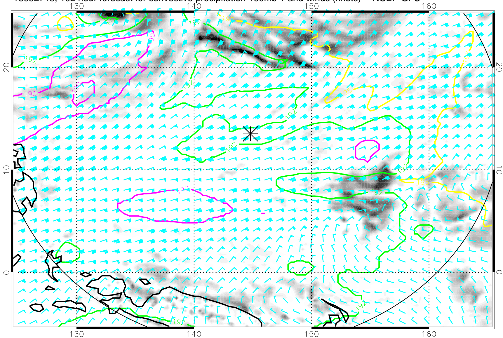
16082718, 102 hour forecast for convective precipitation 100mb T and winds (knots) -- NCEP GFS
