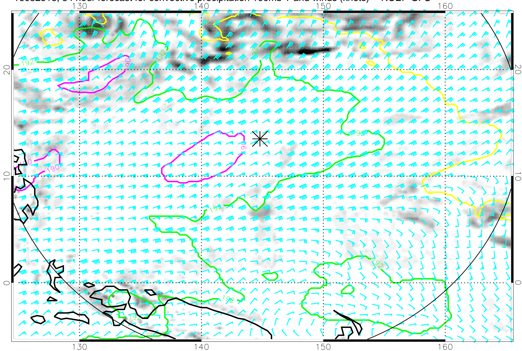
16082518, 54 hour forecast for convective precipitation 100mb T and winds (knots) -- NCEP GFS
