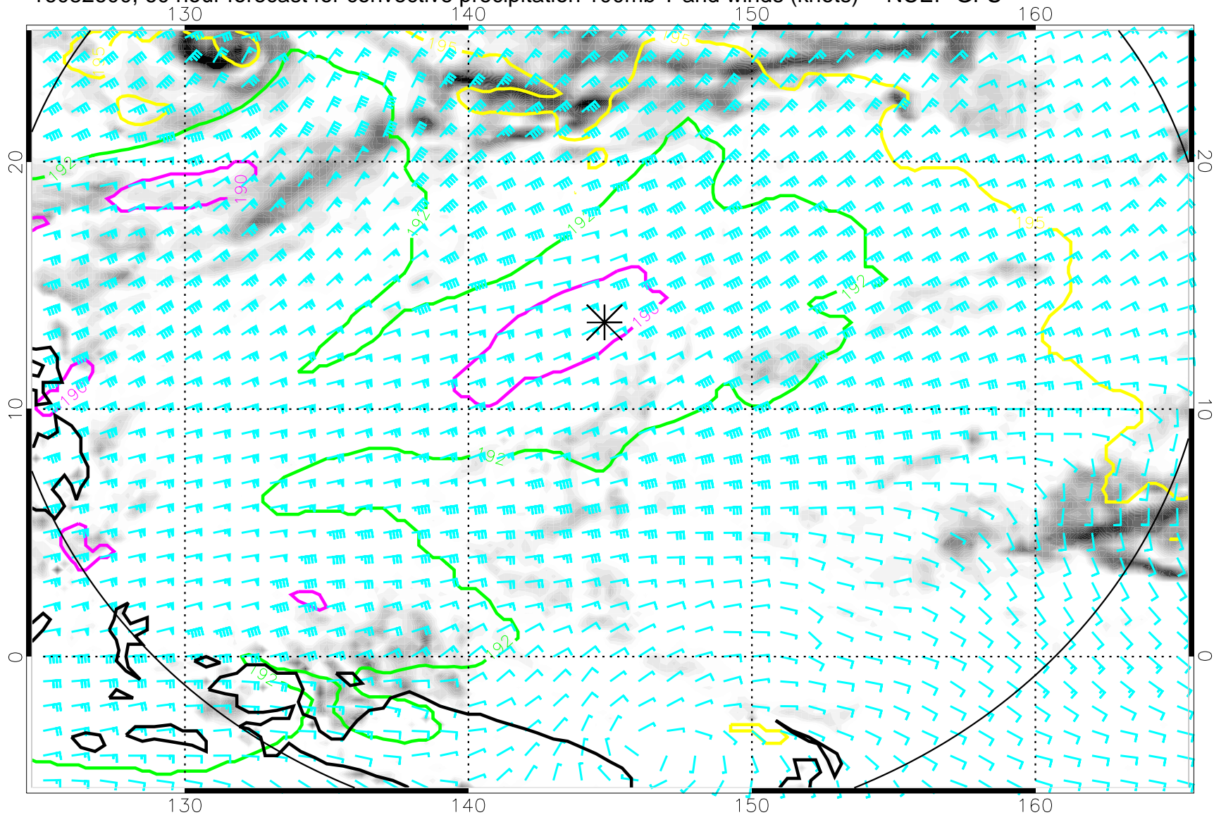
16082600, 60 hour forecast for convective precipitation 100mb T and winds (knots) -- NCEP GFS
