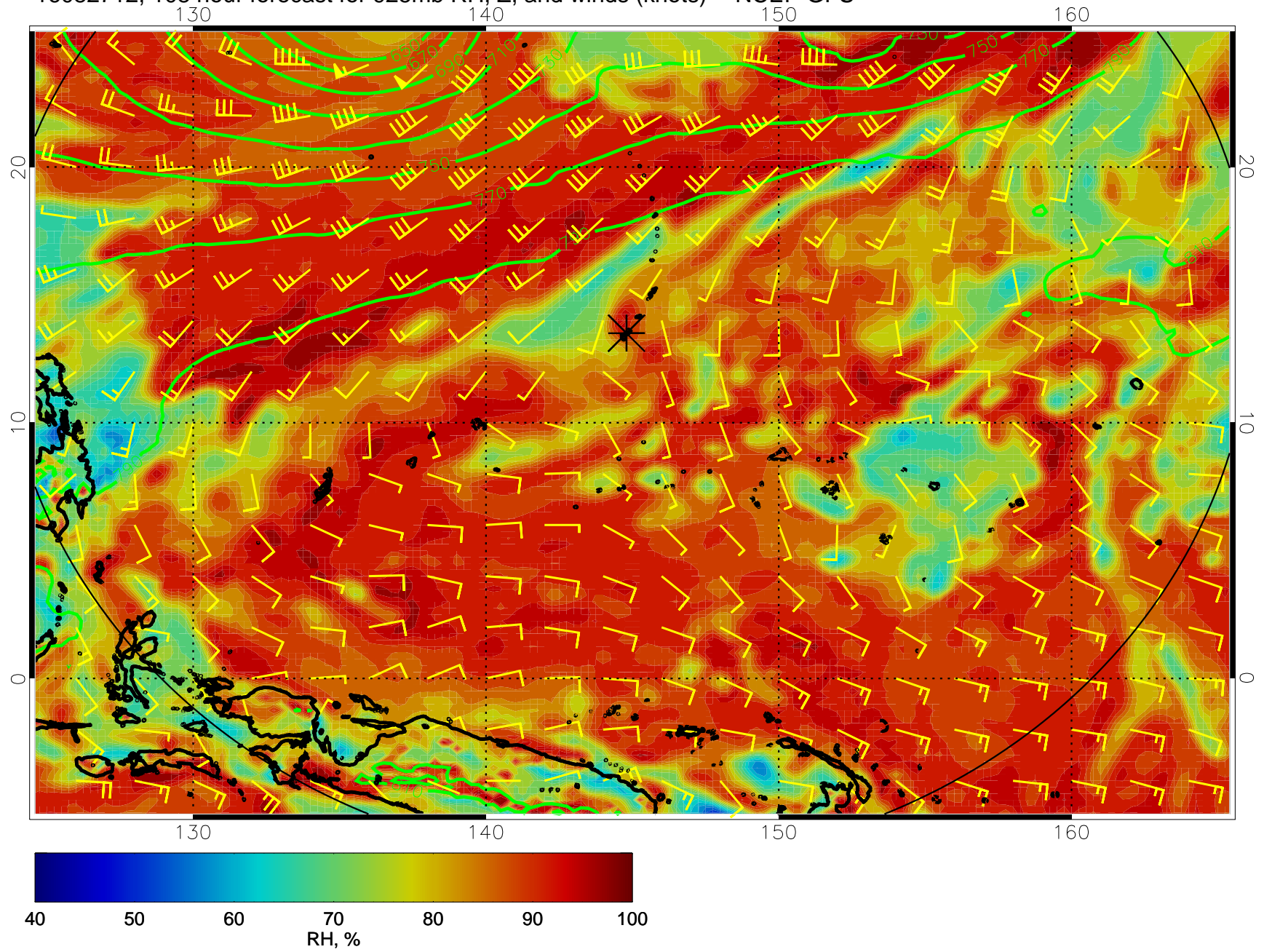
16082712, 108 hour forecast for 925mb RH, Z, and winds (knots) -- NCEP GFS
