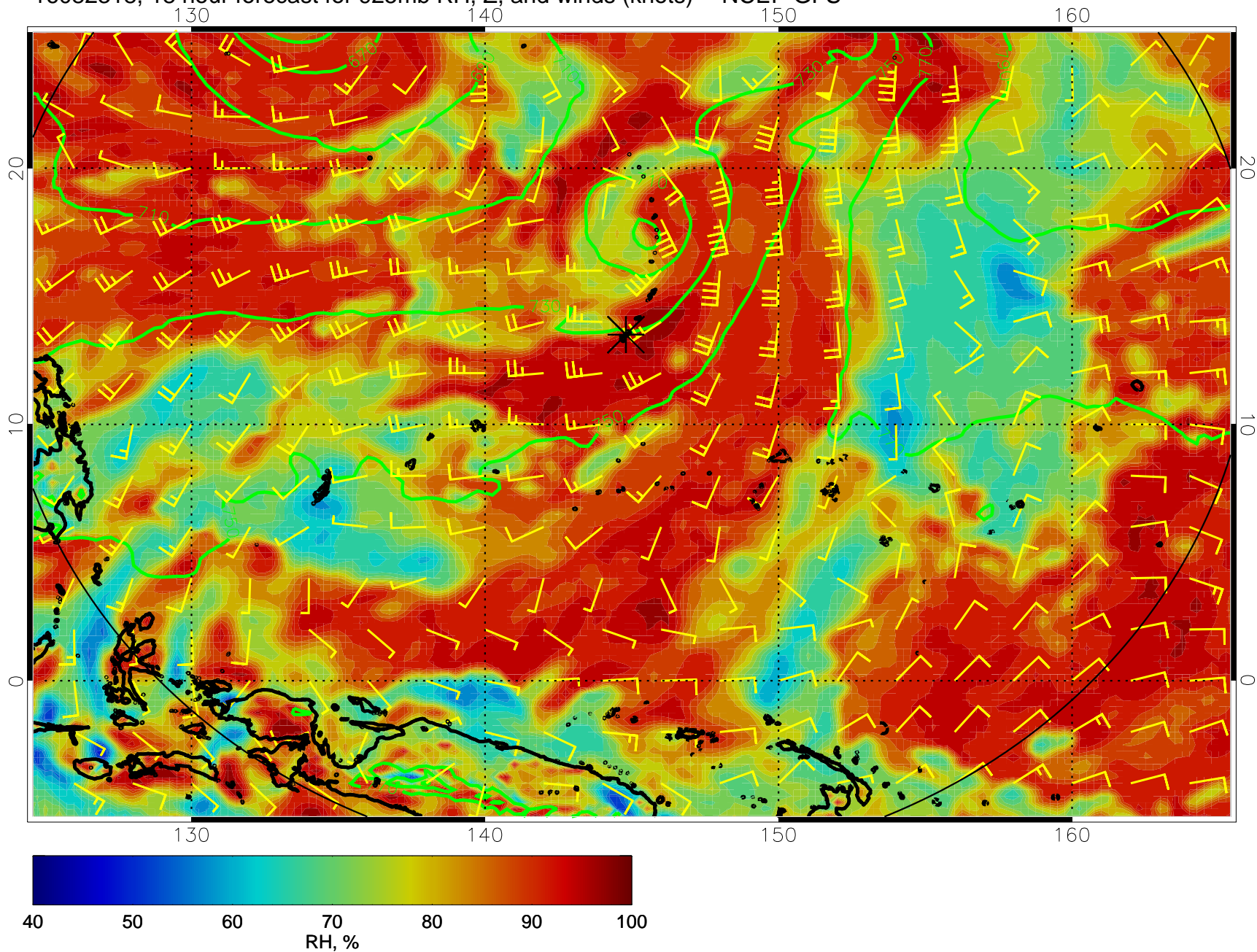
16082318, 18 hour forecast for 925mb RH, Z, and winds (knots) -- NCEP GFS
