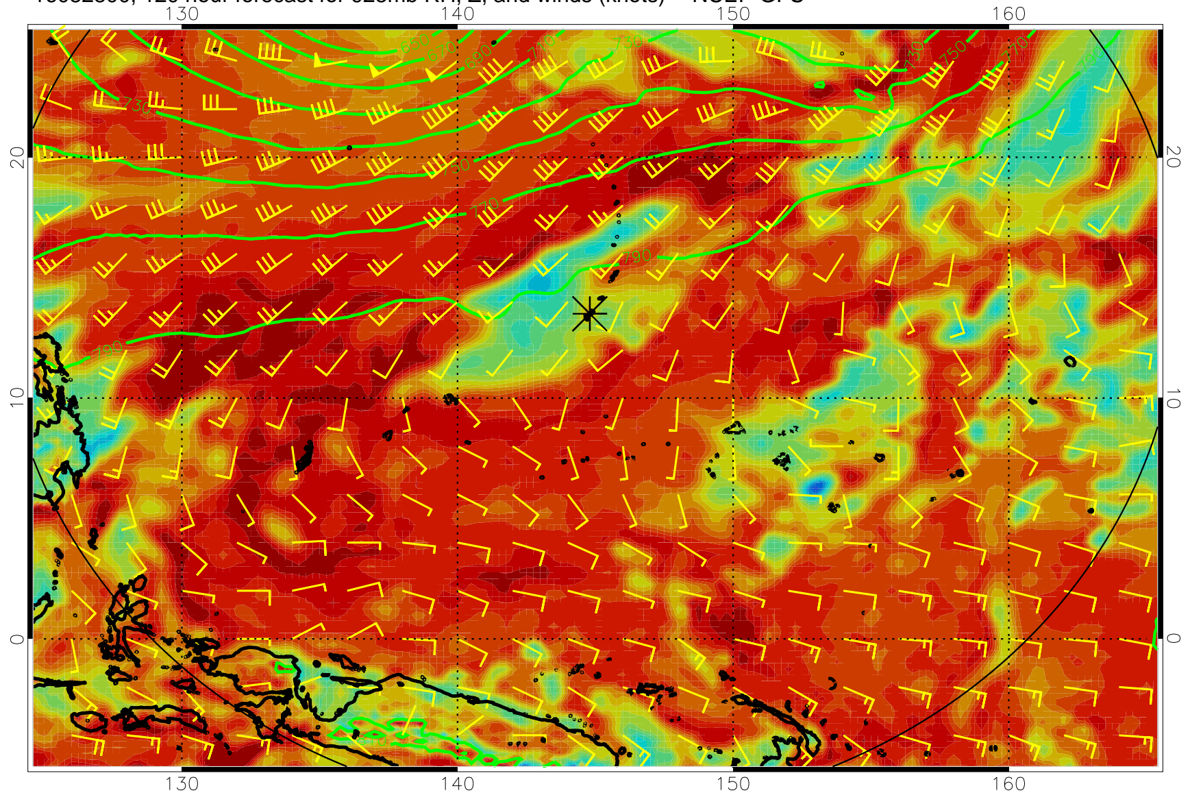
16082800, 120 hour forecast for 925mb RH, Z, and winds (knots) -- NCEP GFS
