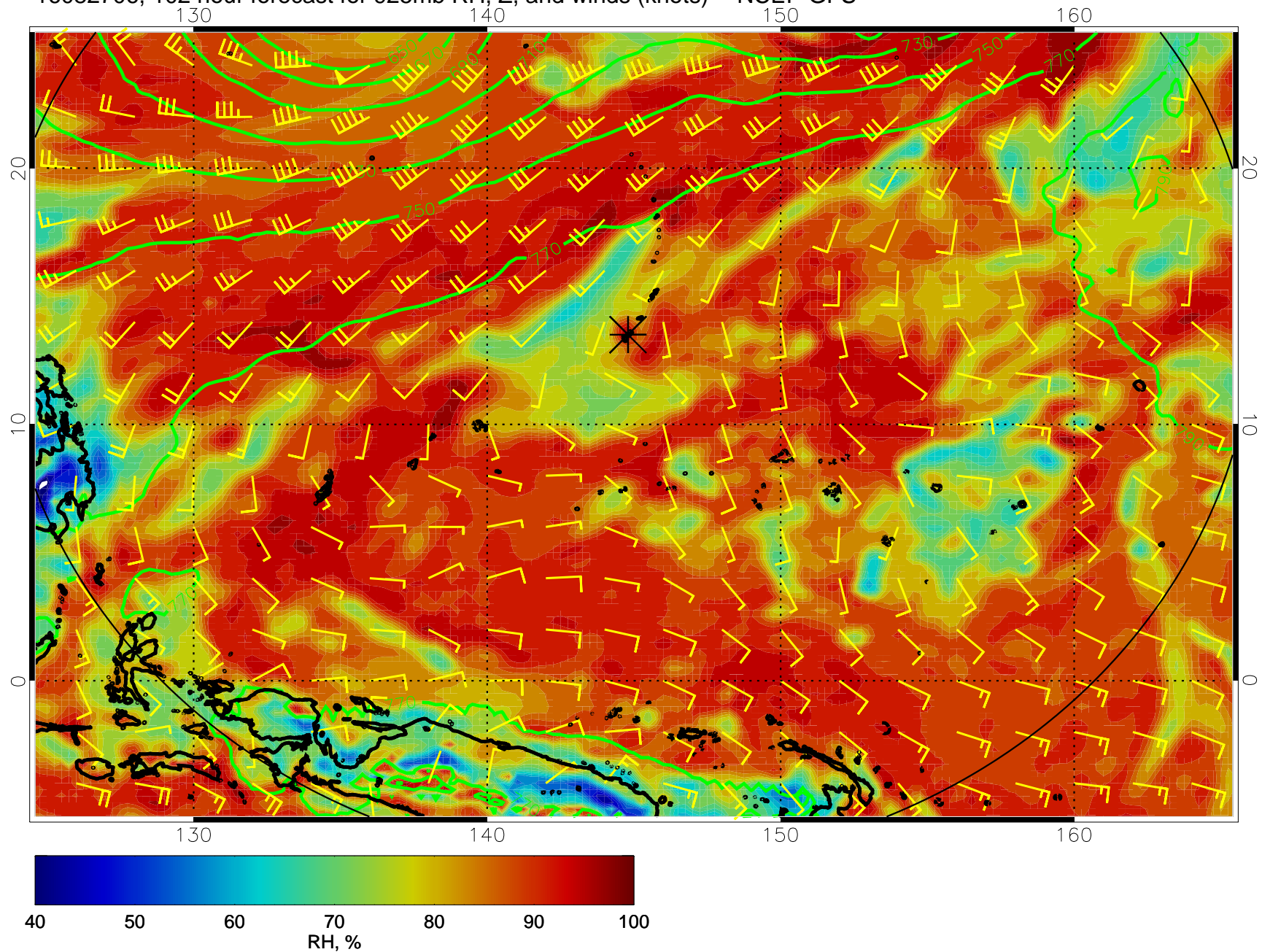
16082706, 102 hour forecast for 925mb RH, Z, and winds (knots) -- NCEP GFS
