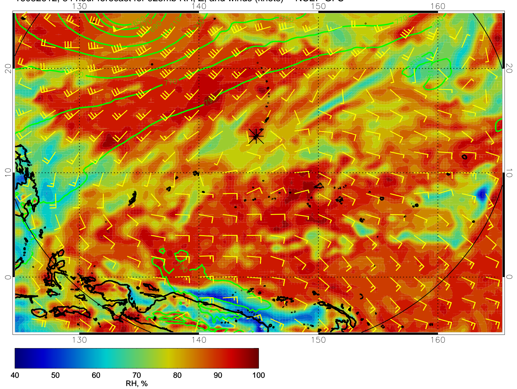
16082612, 84 hour forecast for 925mb RH, Z, and winds (knots) -- NCEP GFS
