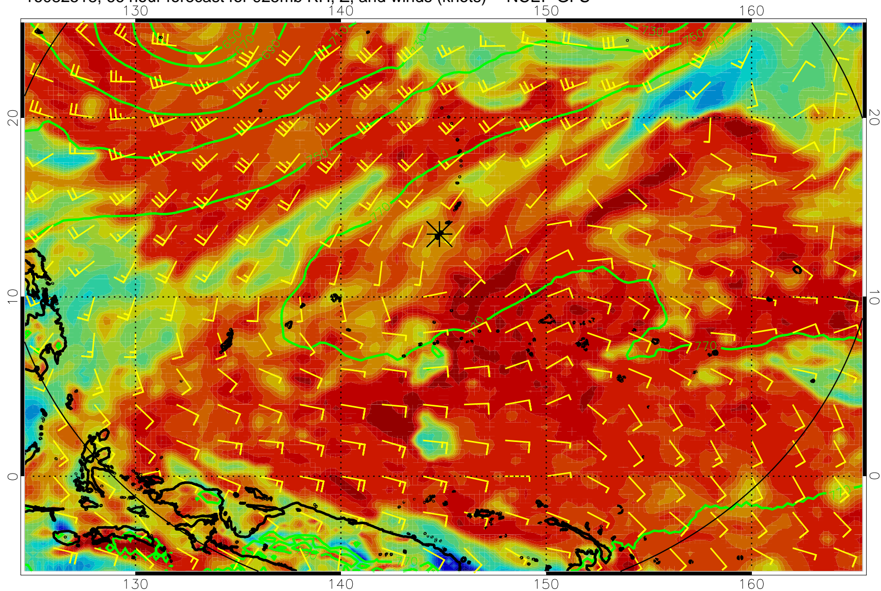
16082518, 66 hour forecast for 925mb RH, Z, and winds (knots) -- NCEP GFS
