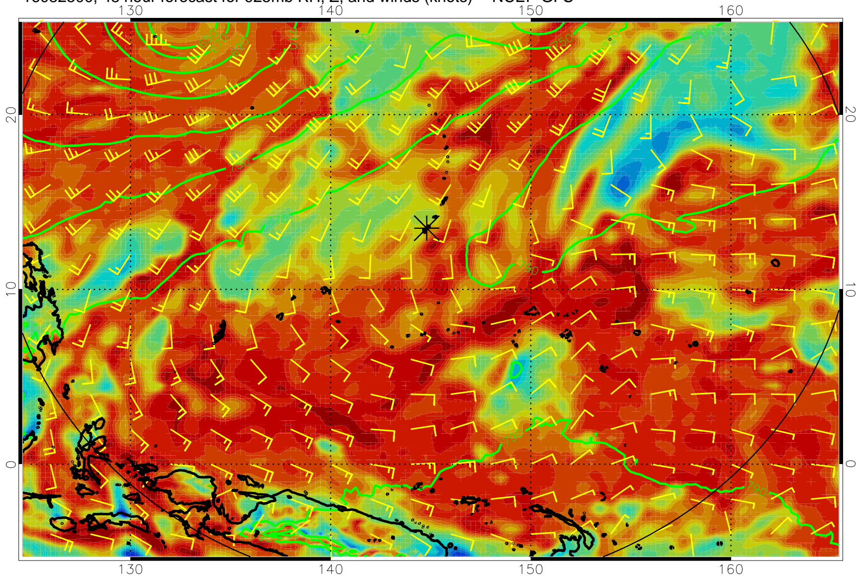
16082500, 48 hour forecast for 925mb RH, Z, and winds (knots) -- NCEP GFS
