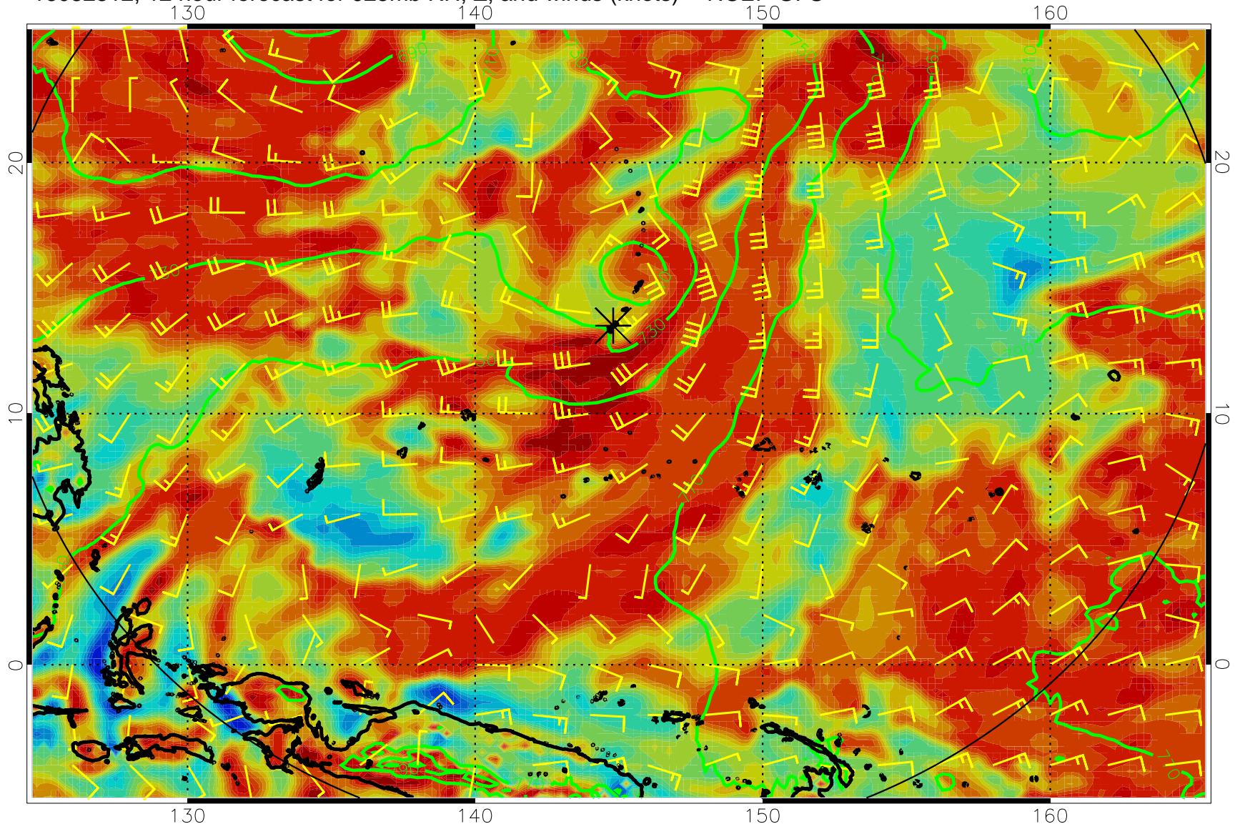
16082312, 12 hour forecast for 925mb RH, Z, and winds (knots) -- NCEP GFS
