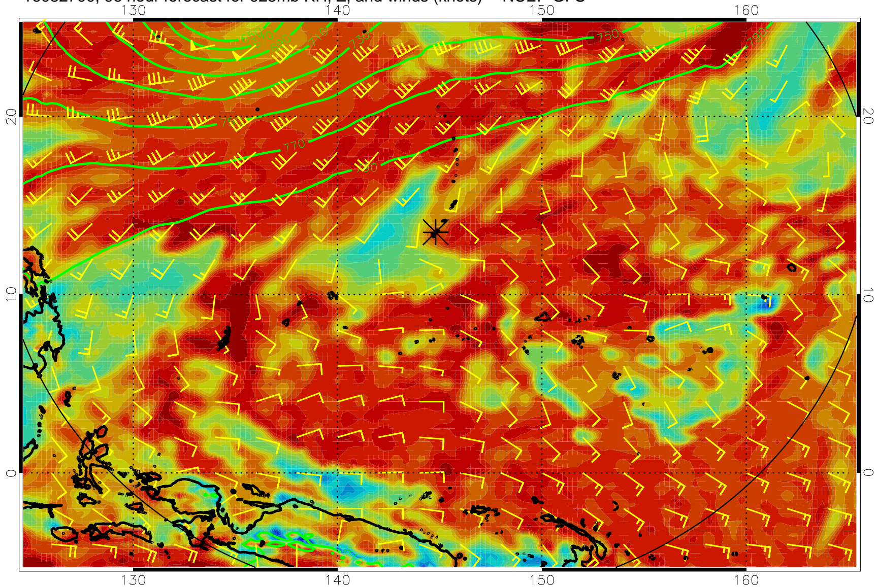
16082700, 96 hour forecast for 925mb RH, Z, and winds (knots) -- NCEP GFS
