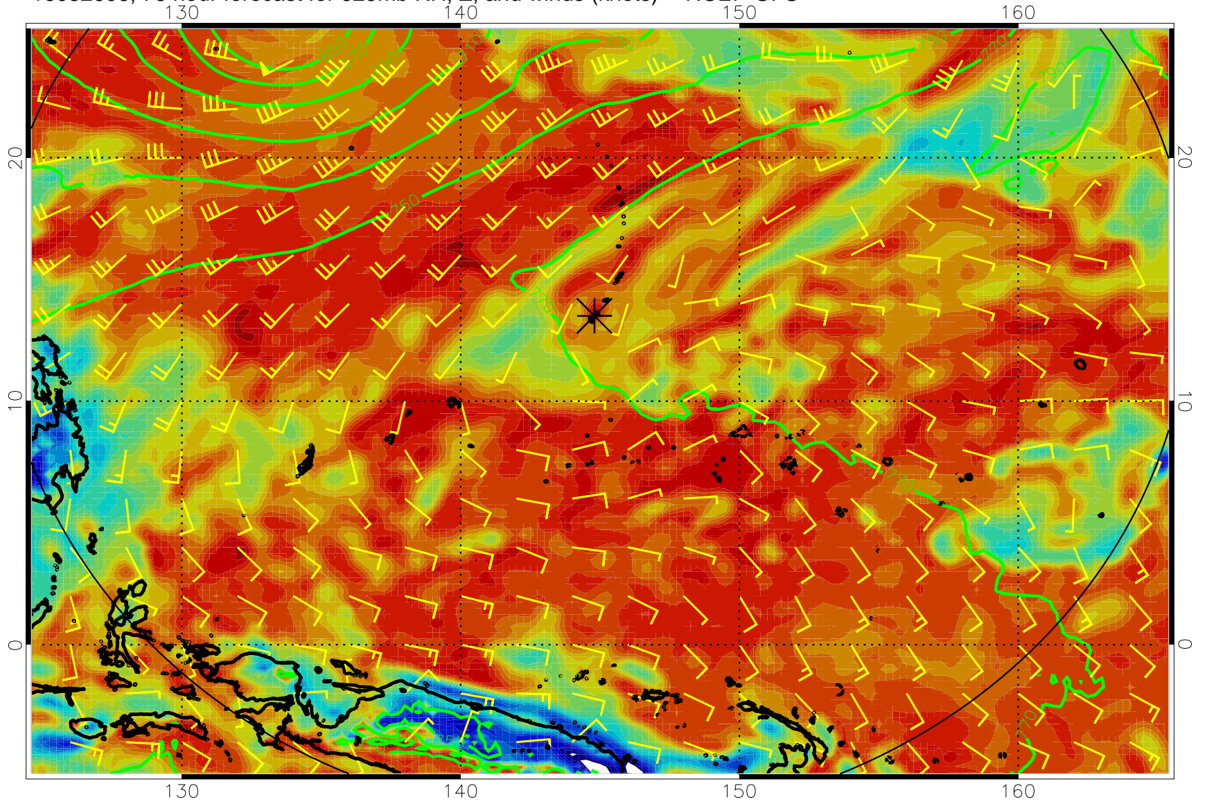
16082606, 78 hour forecast for 925mb RH, Z, and winds (knots) -- NCEP GFS
