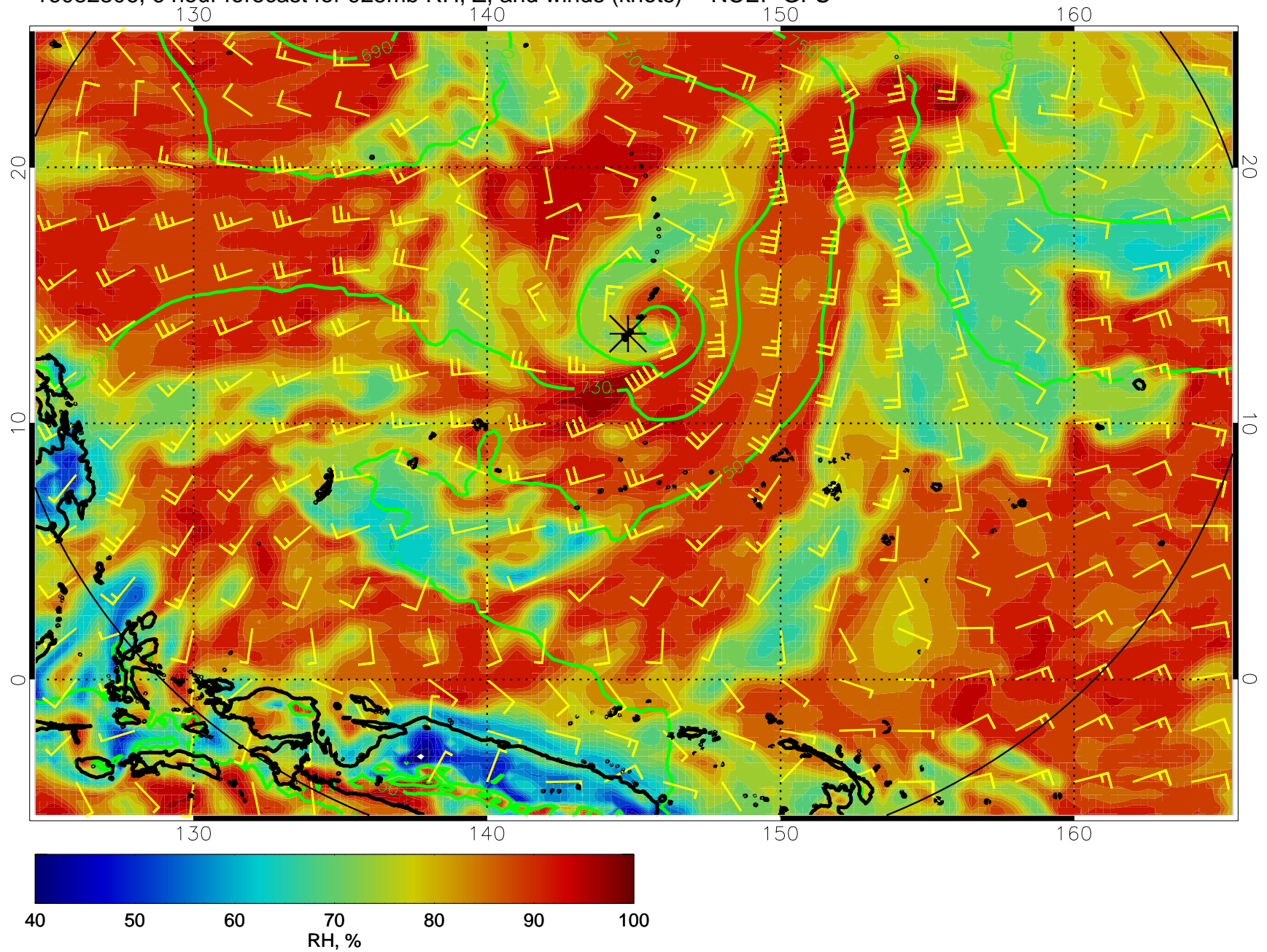
16082306, 6 hour forecast for 925mb RH, Z, and winds (knots) -- NCEP GFS
