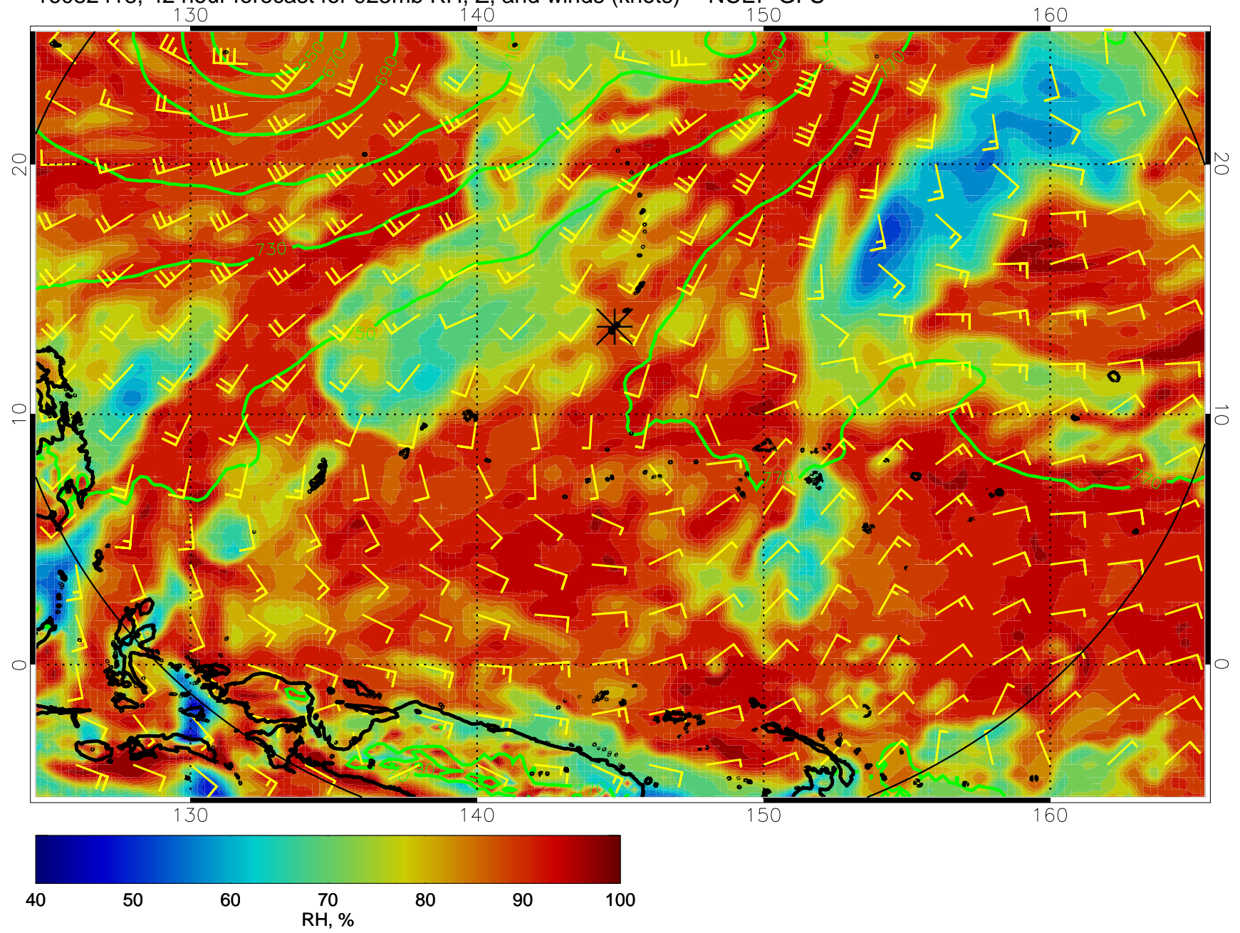
16082418, 42 hour forecast for 925mb RH, Z, and winds (knots) -- NCEP GFS
