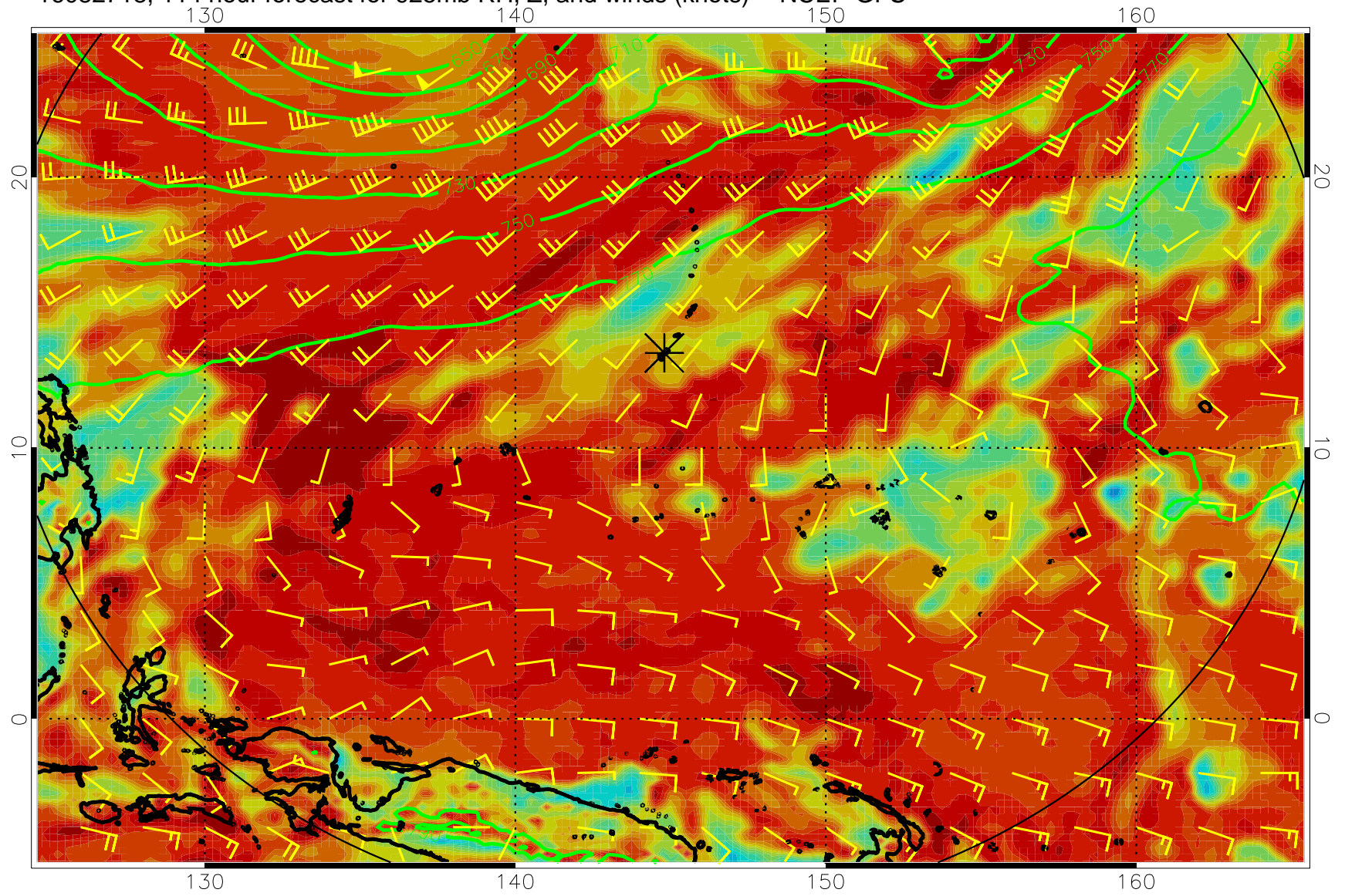
16082718, 114 hour forecast for 925mb RH, Z, and winds (knots) -- NCEP GFS
