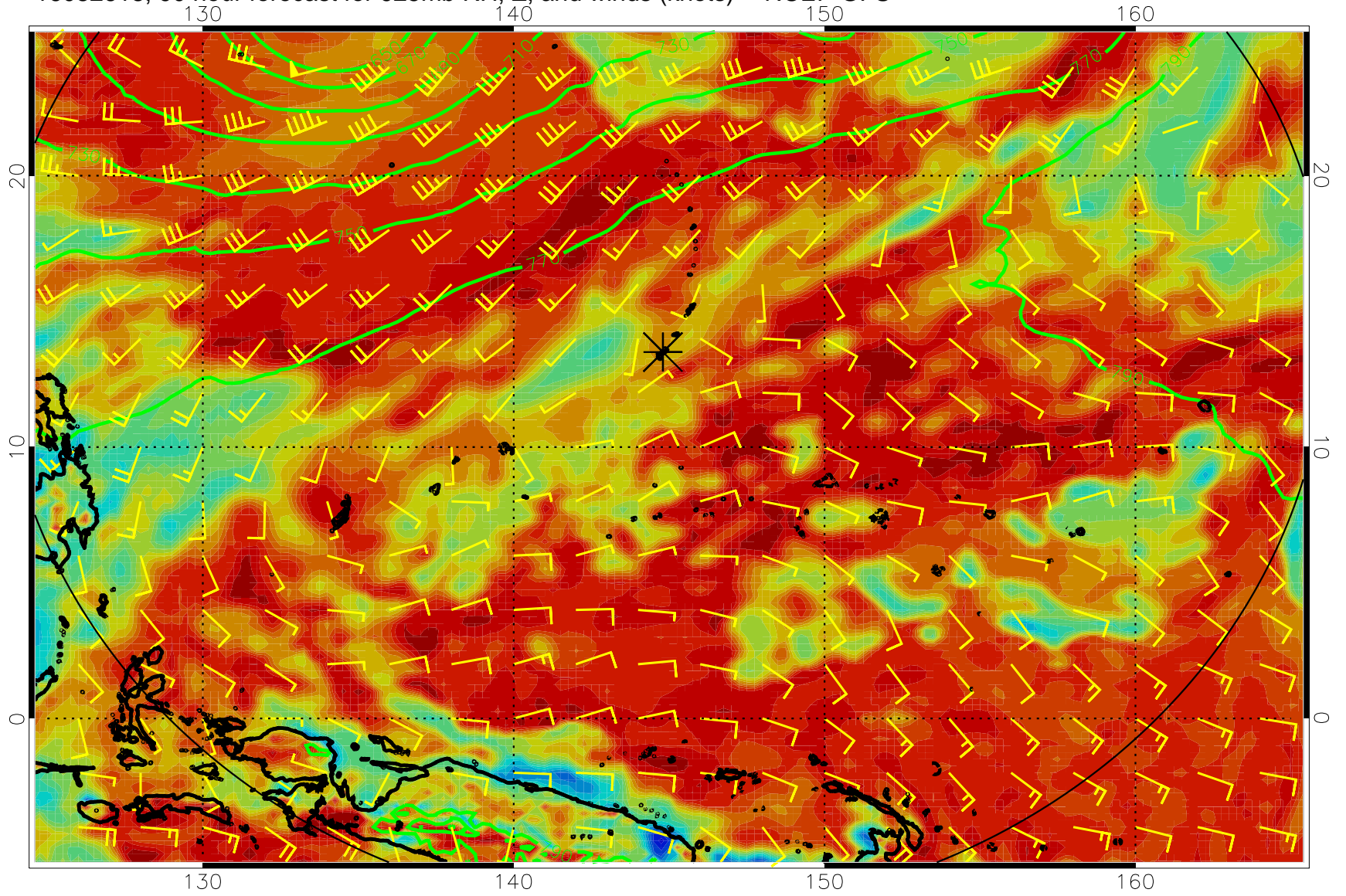
16082618, 90 hour forecast for 925mb RH, Z, and winds (knots) -- NCEP GFS
