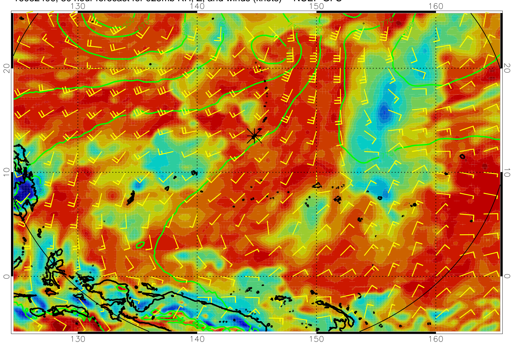
16082406, 30 hour forecast for 925mb RH, Z, and winds (knots) -- NCEP GFS
