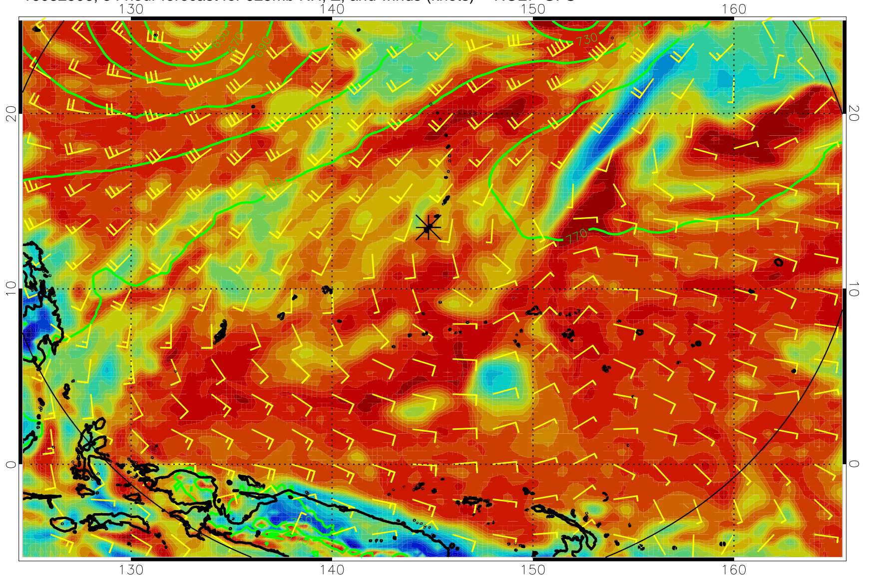
16082506, 54 hour forecast for 925mb RH, Z, and winds (knots) -- NCEP GFS
