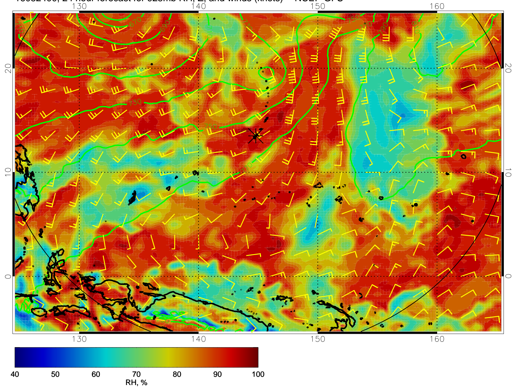
16082400, 24 hour forecast for 925mb RH, Z, and winds (knots) -- NCEP GFS
