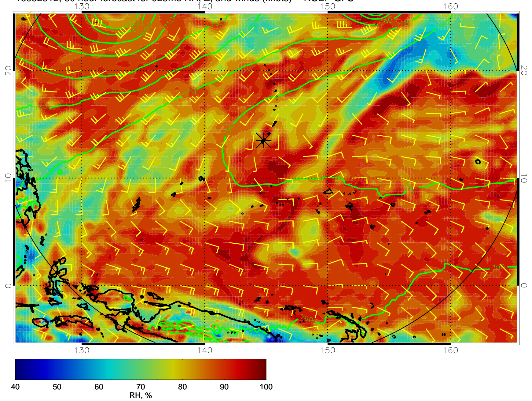
16082512, 60 hour forecast for 925mb RH, Z, and winds (knots) -- NCEP GFS
