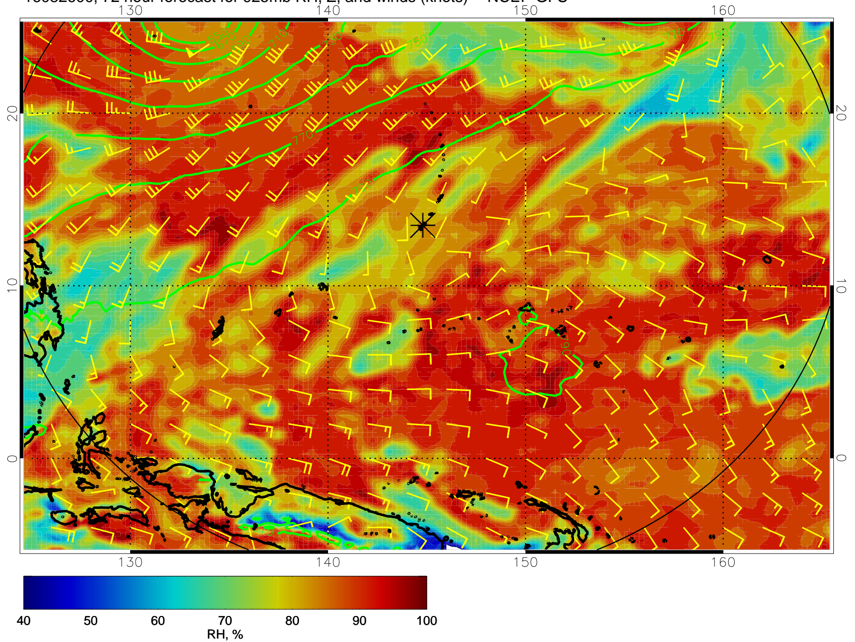
16082600, 72 hour forecast for 925mb RH, Z, and winds (knots) -- NCEP GFS
