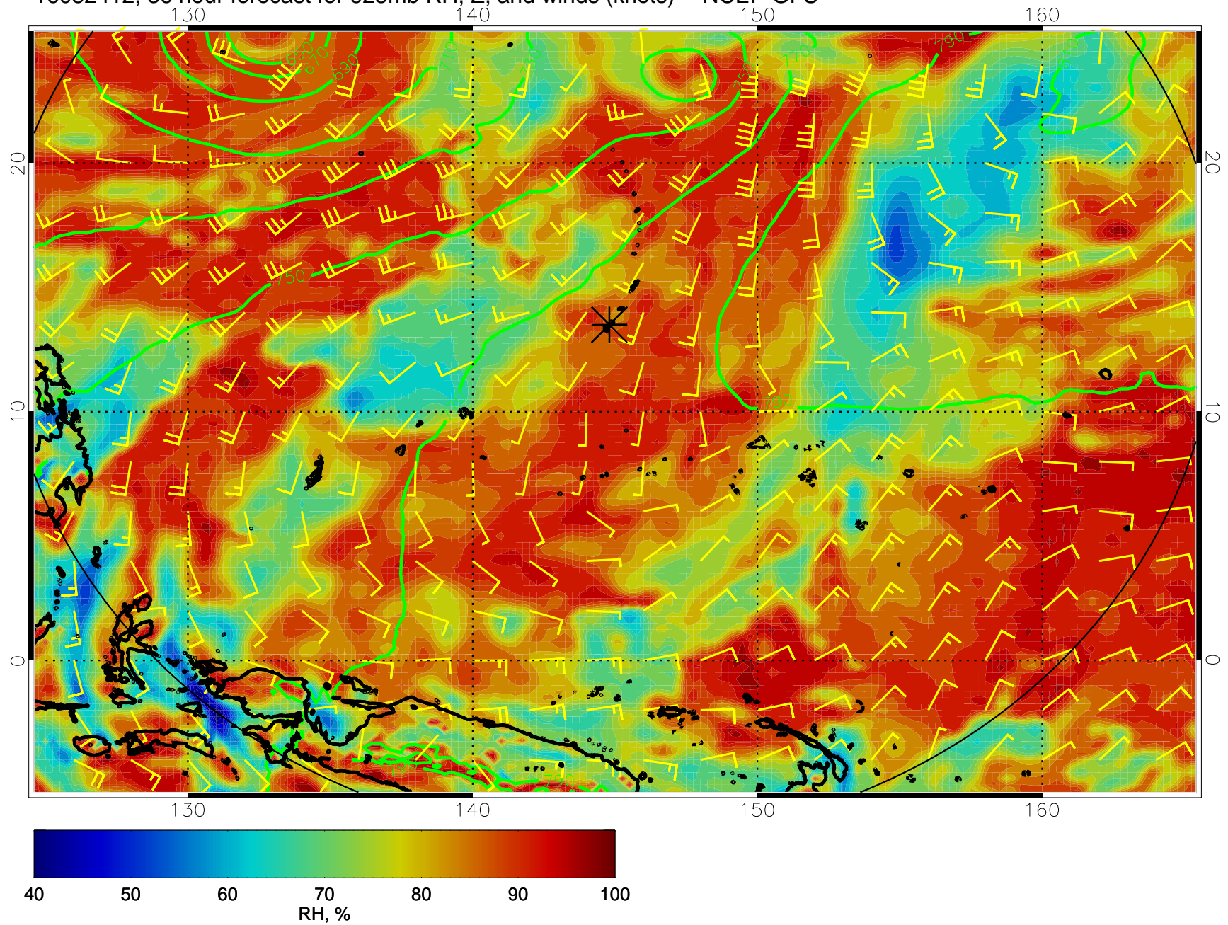
16082412, 36 hour forecast for 925mb RH, Z, and winds (knots) -- NCEP GFS
