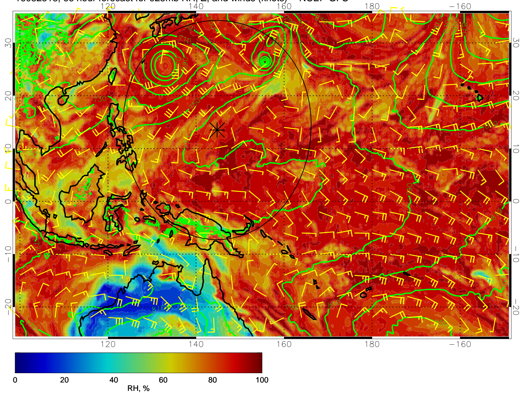
16082518, 66 hour forecast for 925mb RH, Z, and winds (knots) -- NCEP GFS
