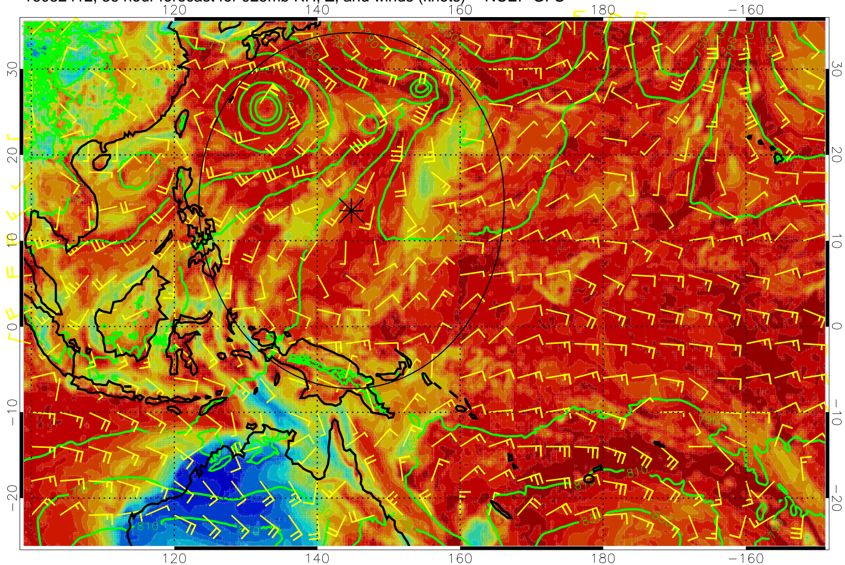
16082412, 36 hour forecast for 925mb RH, Z, and winds (knots) -- NCEP GFS
