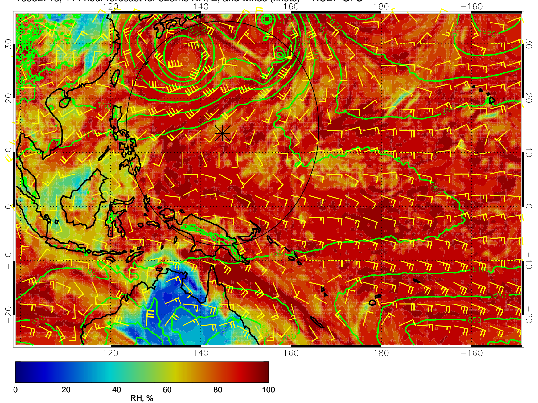
16082718, 114 hour forecast for 925mb RH, Z, and winds (knots) -- NCEP GFS
