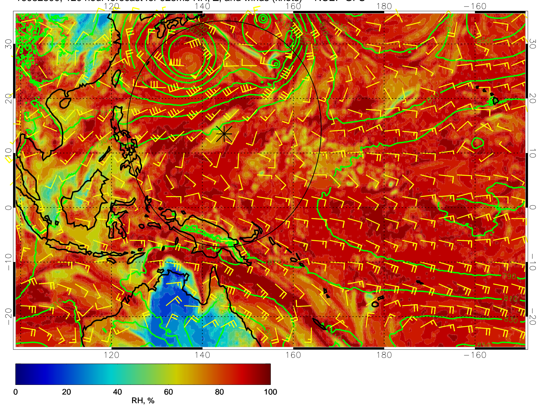
16082800, 120 hour forecast for 925mb RH, Z, and winds (knots) -- NCEP GFS
