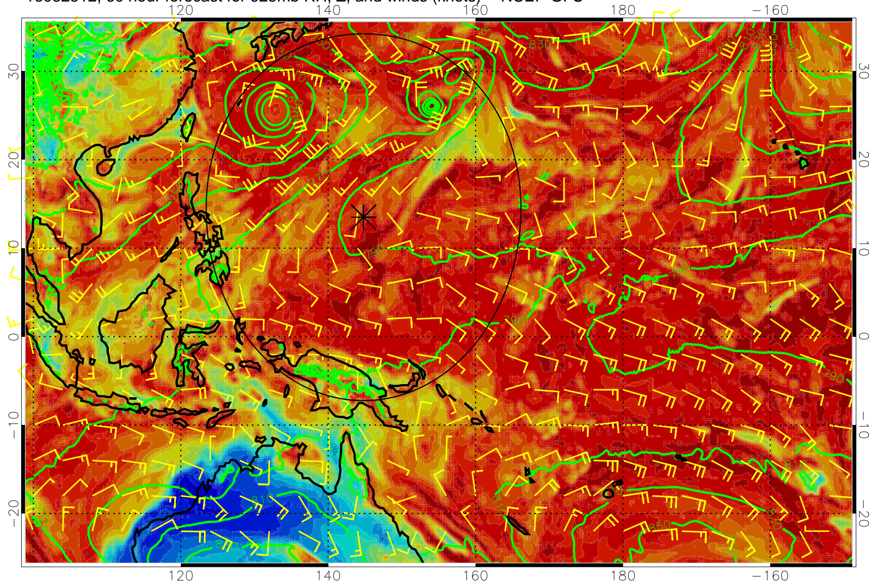
16082512, 60 hour forecast for 925mb RH, Z, and winds (knots) -- NCEP GFS
