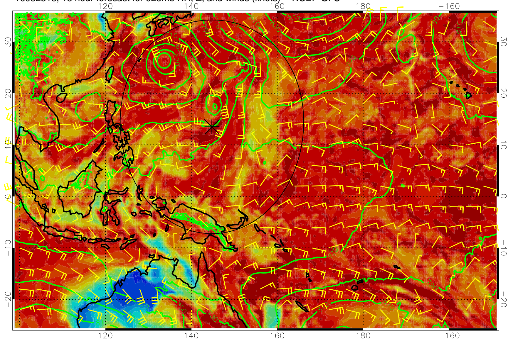
16082318, 18 hour forecast for 925mb RH, Z, and winds (knots) -- NCEP GFS
