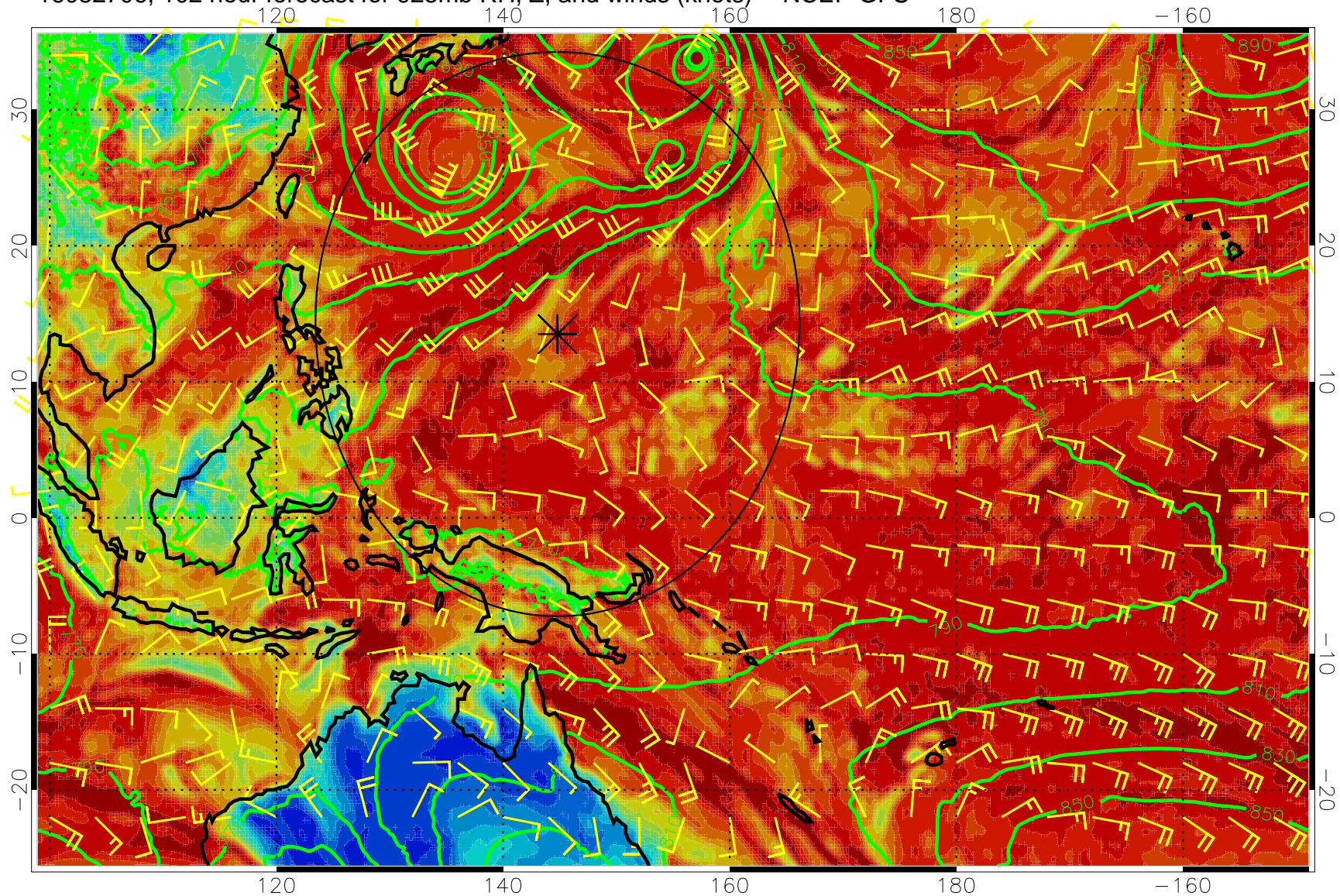
16082706, 102 hour forecast for 925mb RH, Z, and winds (knots) -- NCEP GFS
