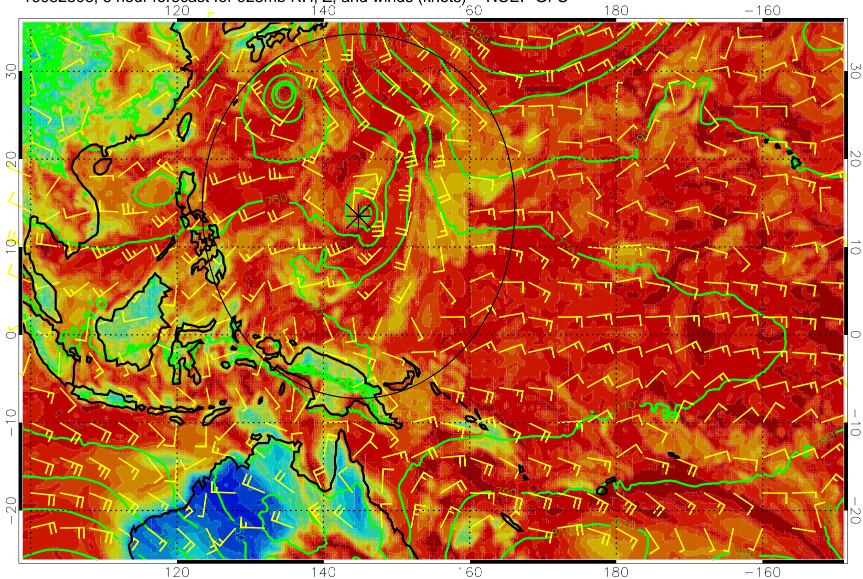
16082306, 6 hour forecast for 925mb RH, Z, and winds (knots) -- NCEP GFS
