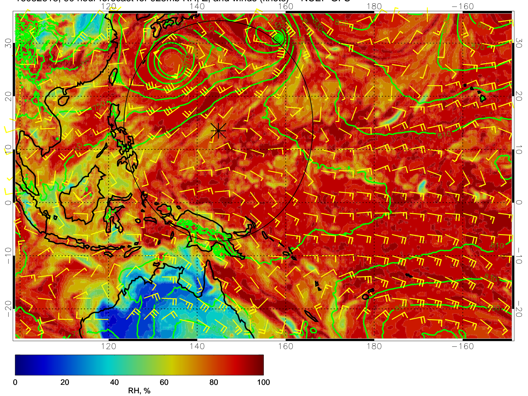
16082618, 90 hour forecast for 925mb RH, Z, and winds (knots) -- NCEP GFS
