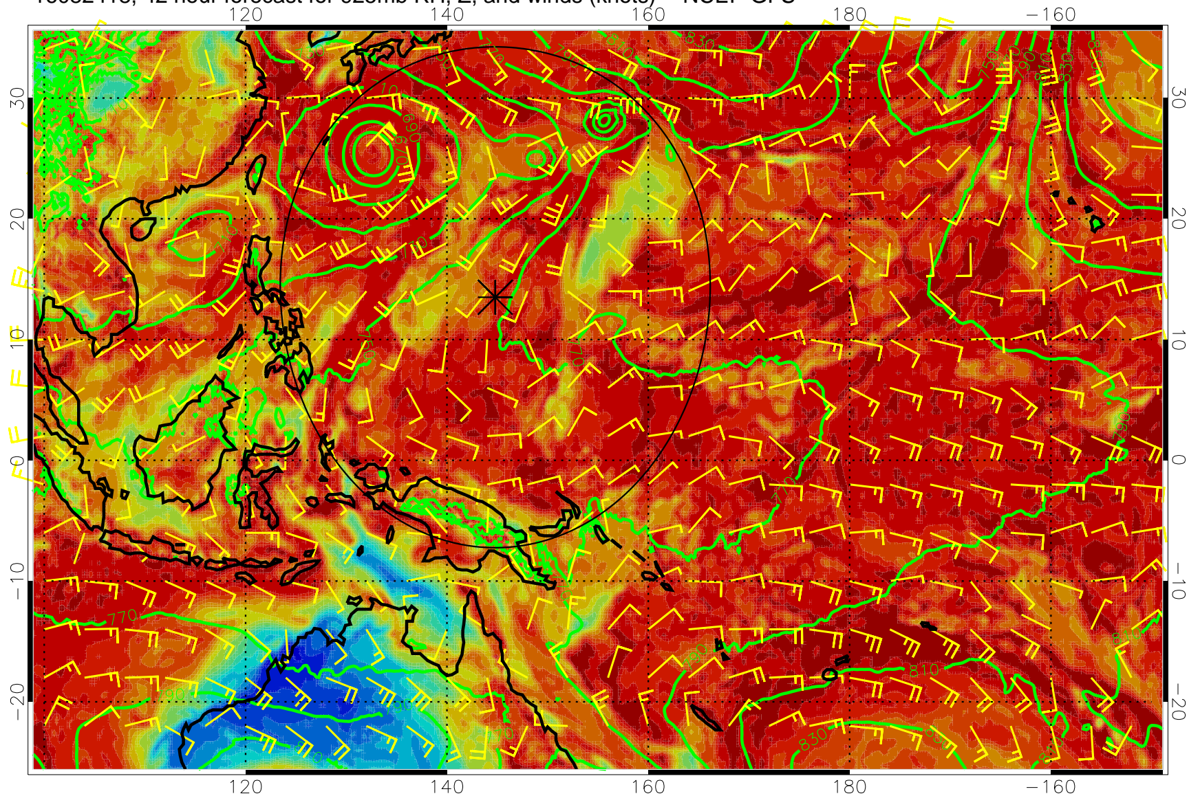
16082418, 42 hour forecast for 925mb RH, Z, and winds (knots) -- NCEP GFS
