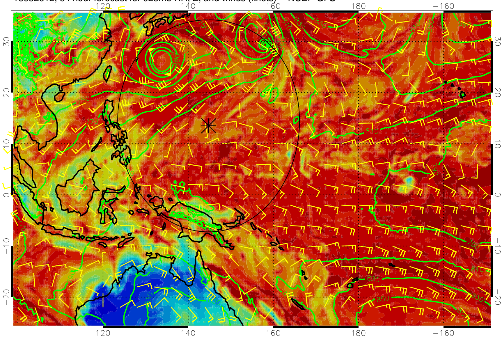
16082612, 84 hour forecast for 925mb RH, Z, and winds (knots) -- NCEP GFS
