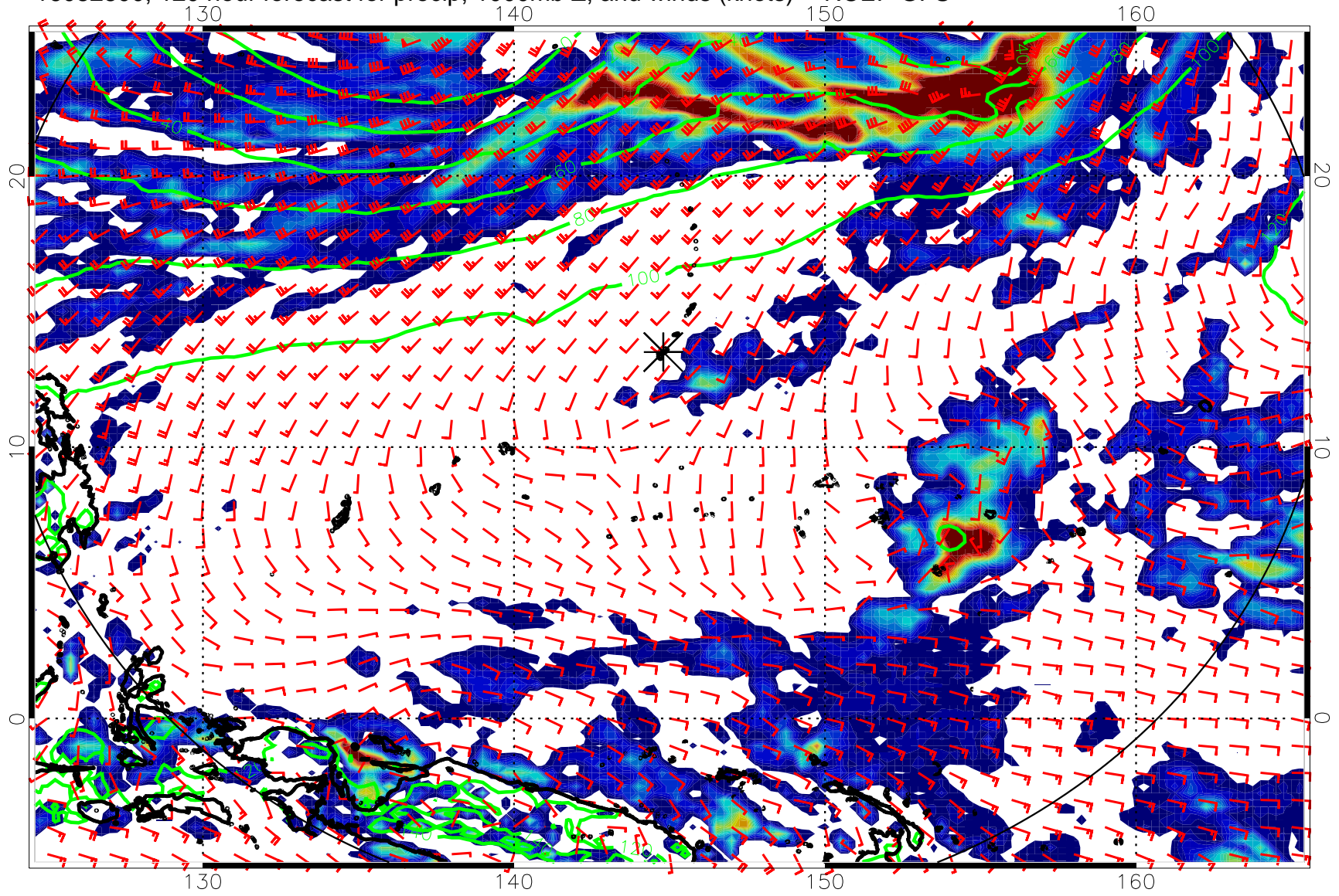
16082800, 120 hour forecast for precip, 1000mb Z, and winds (knots) -- NCEP GFS
