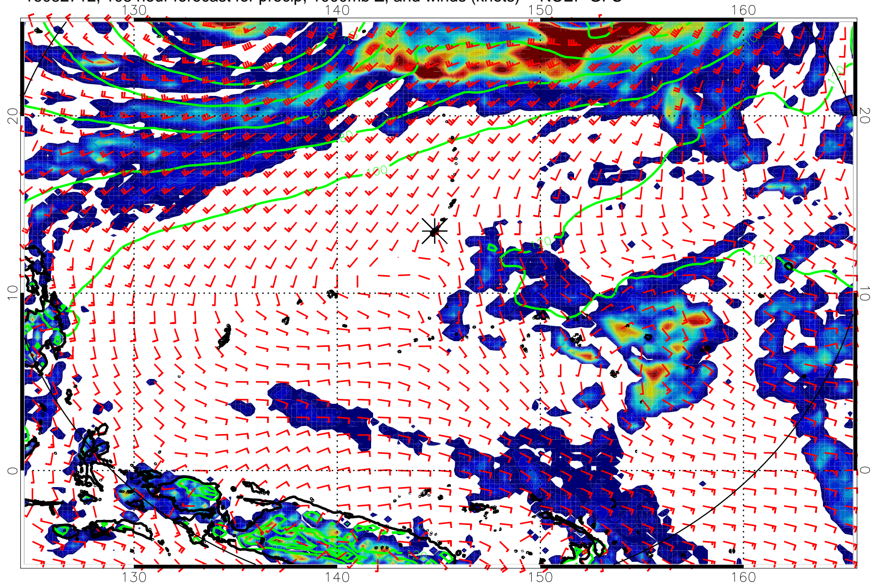
16082712, 108 hour forecast for precip, 1000mb Z, and winds (knots) -- NCEP GFS
