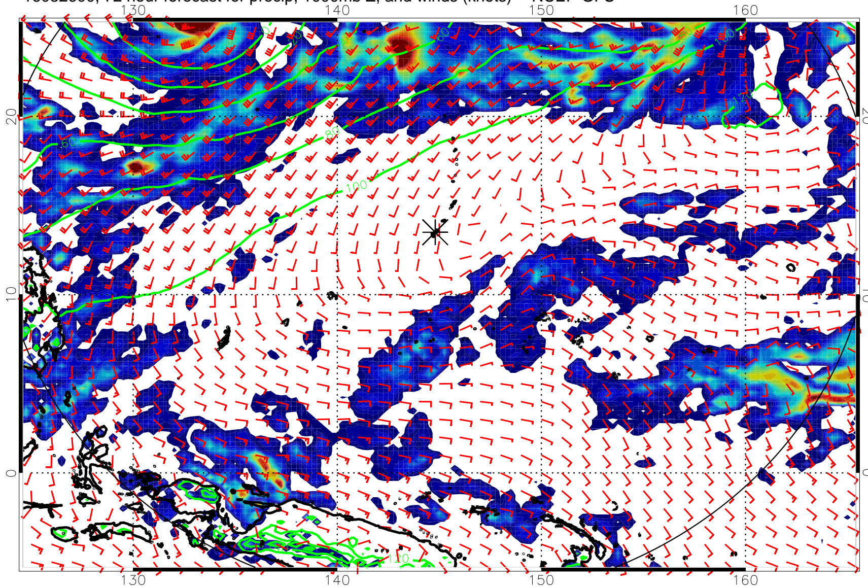
16082600, 72 hour forecast for precip, 1000mb Z, and winds (knots) -- NCEP GFS
