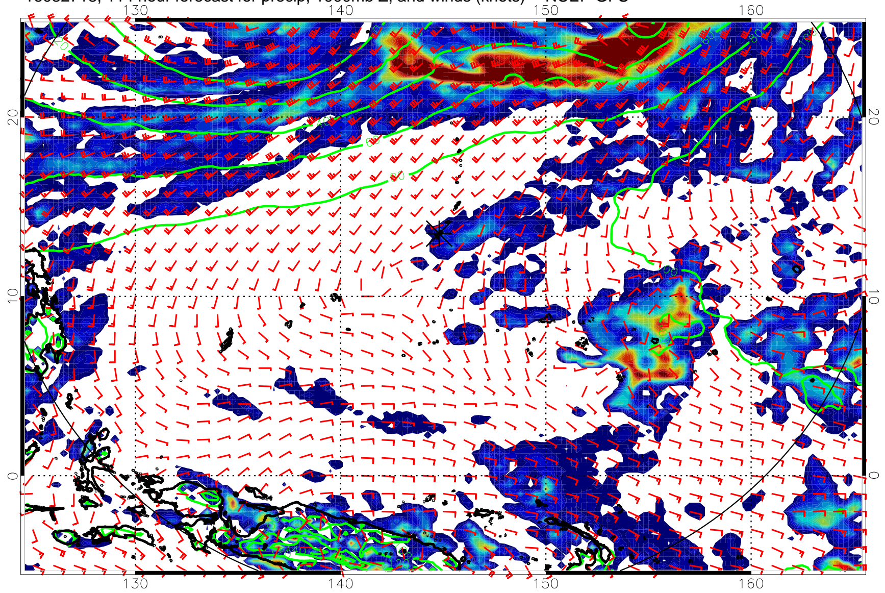
16082718, 114 hour forecast for precip, 1000mb Z, and winds (knots) -- NCEP GFS
