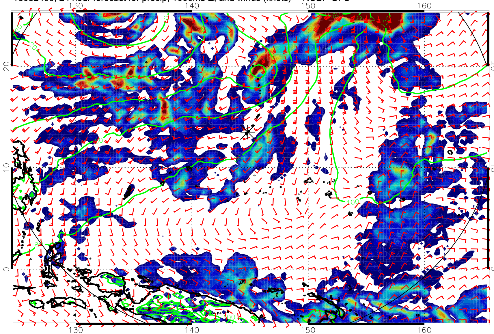
16082400, 24 hour forecast for precip, 1000mb Z, and winds (knots) -- NCEP GFS
