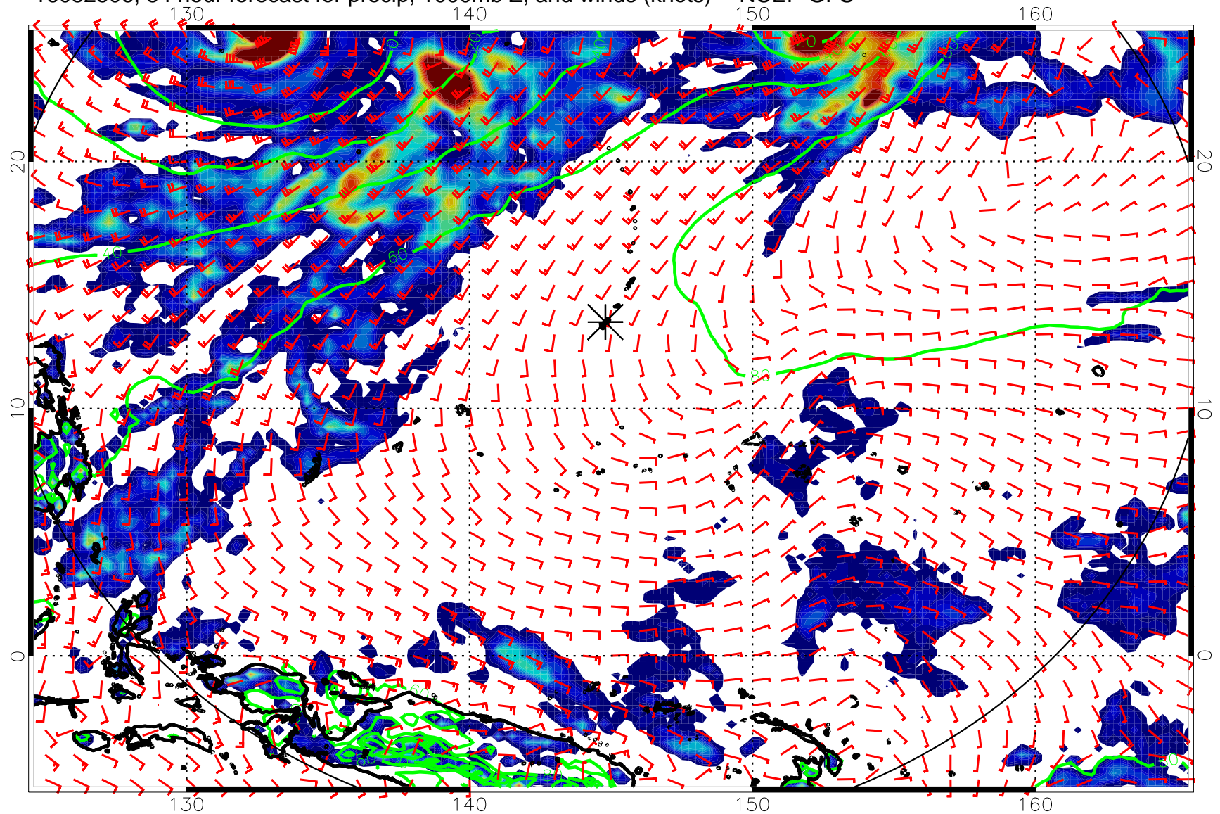
16082506, 54 hour forecast for precip, 1000mb Z, and winds (knots) -- NCEP GFS
