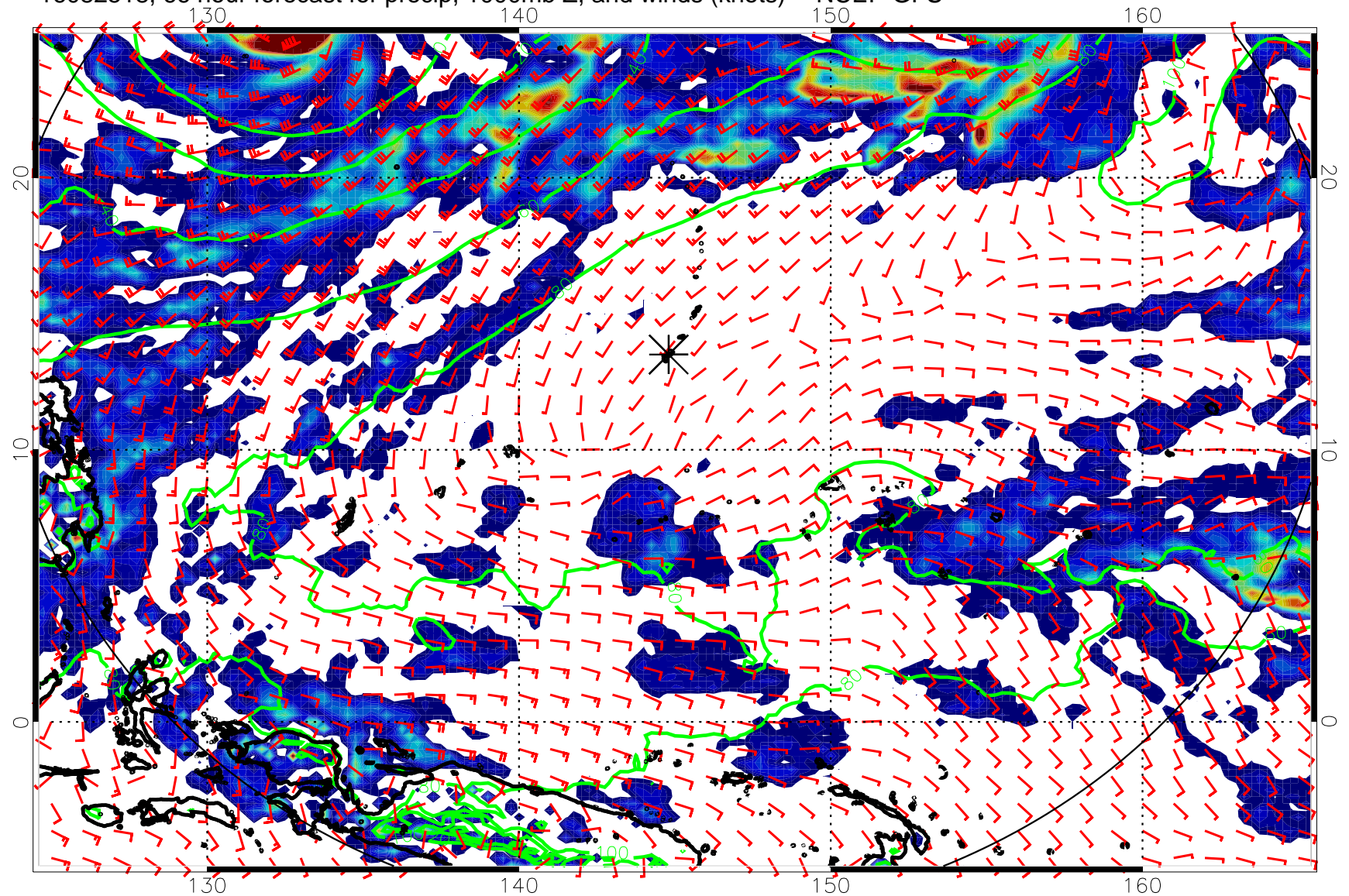
16082518, 66 hour forecast for precip, 1000mb Z, and winds (knots) -- NCEP GFS
