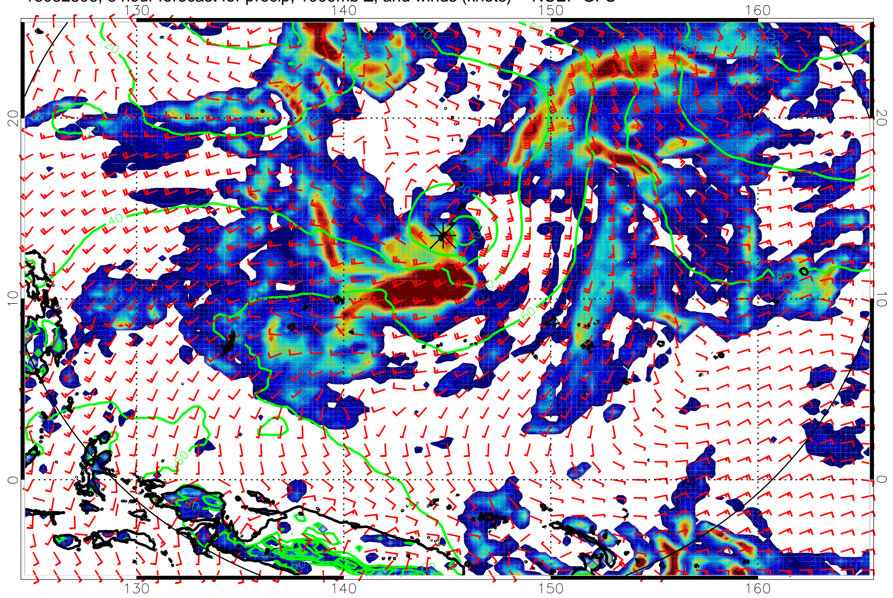
16082306, 6 hour forecast for precip, 1000mb Z, and winds (knots) -- NCEP GFS
