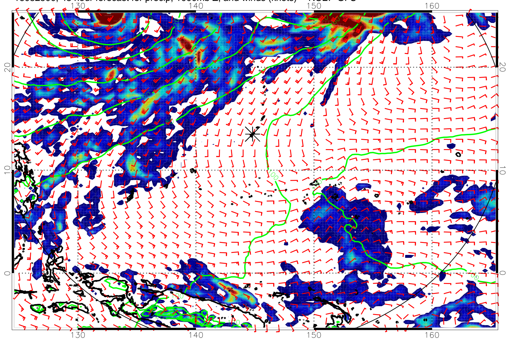
16082500, 48 hour forecast for precip, 1000mb Z, and winds (knots) -- NCEP GFS
