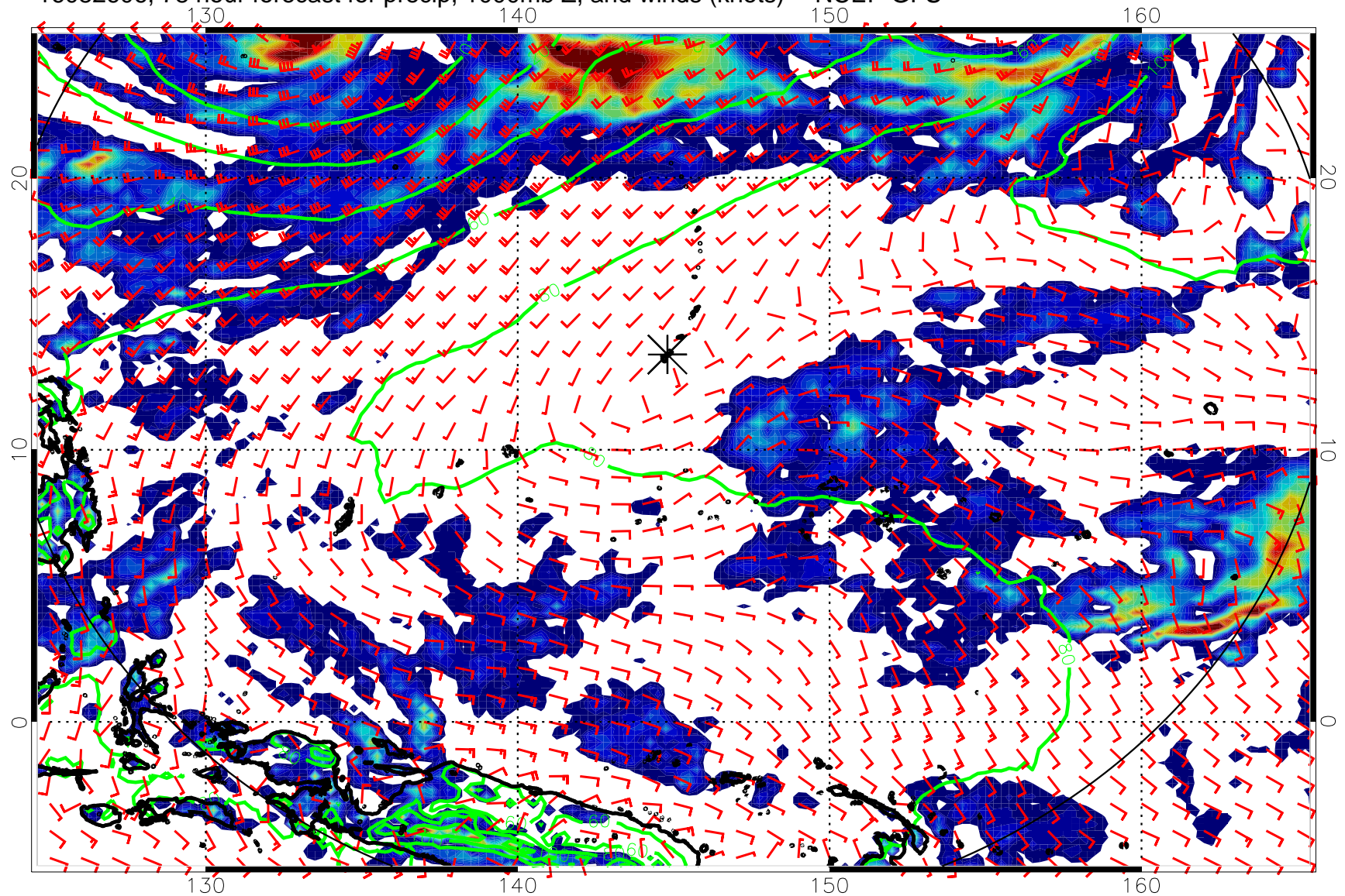
16082606, 78 hour forecast for precip, 1000mb Z, and winds (knots) -- NCEP GFS
