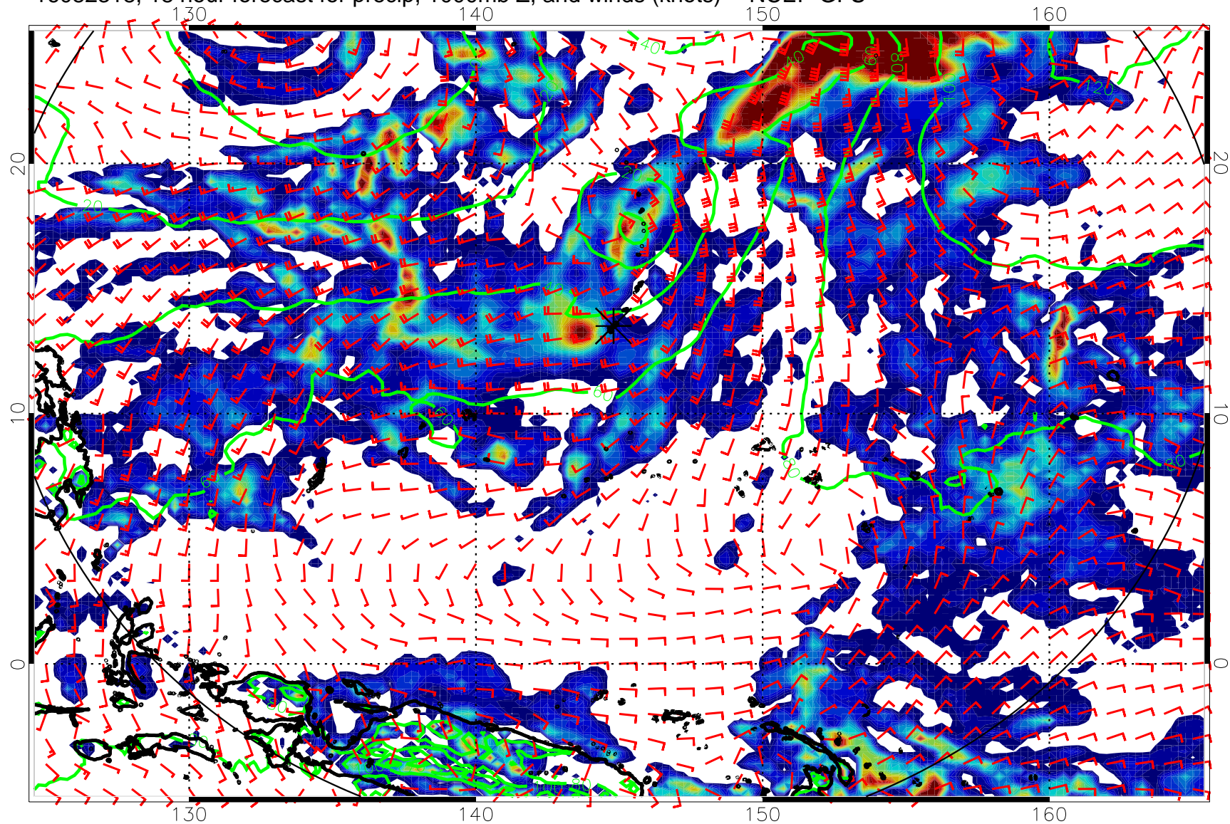
16082318, 18 hour forecast for precip, 1000mb Z, and winds (knots) -- NCEP GFS
