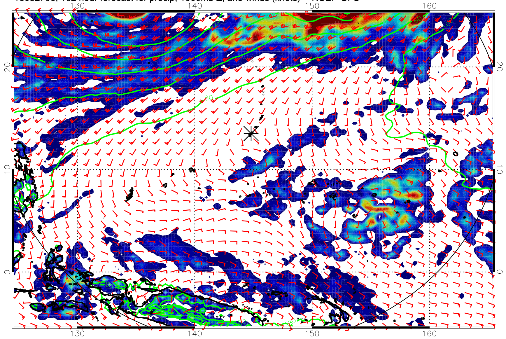
16082706, 102 hour forecast for precip, 1000mb Z, and winds (knots) -- NCEP GFS
