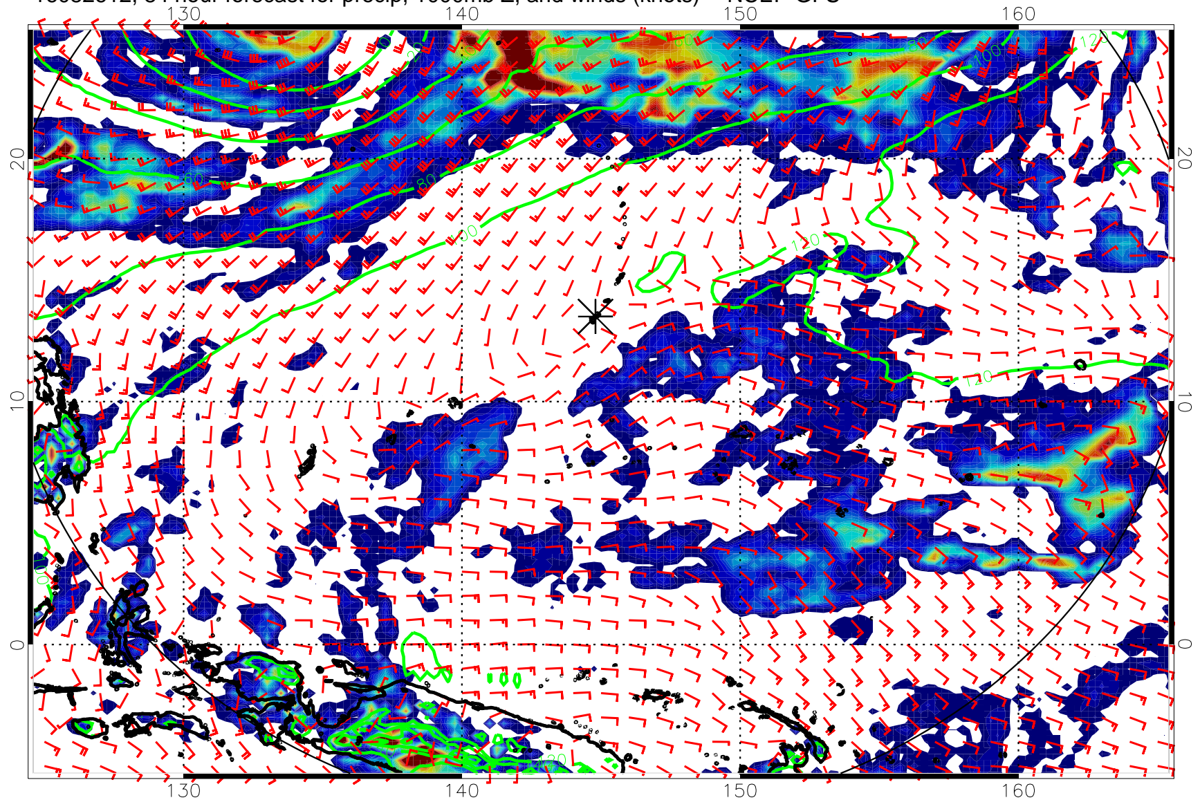
16082612, 84 hour forecast for precip, 1000mb Z, and winds (knots) -- NCEP GFS
