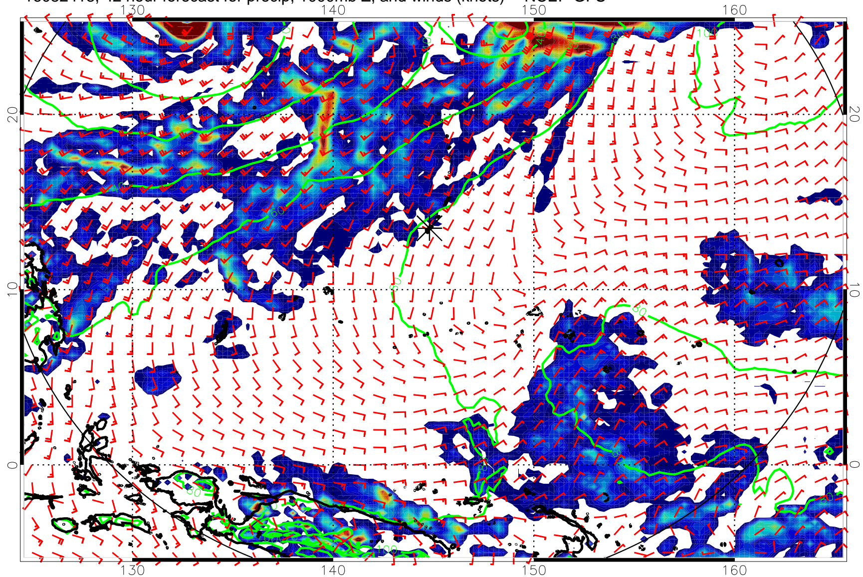
16082418, 42 hour forecast for precip, 1000mb Z, and winds (knots) -- NCEP GFS
