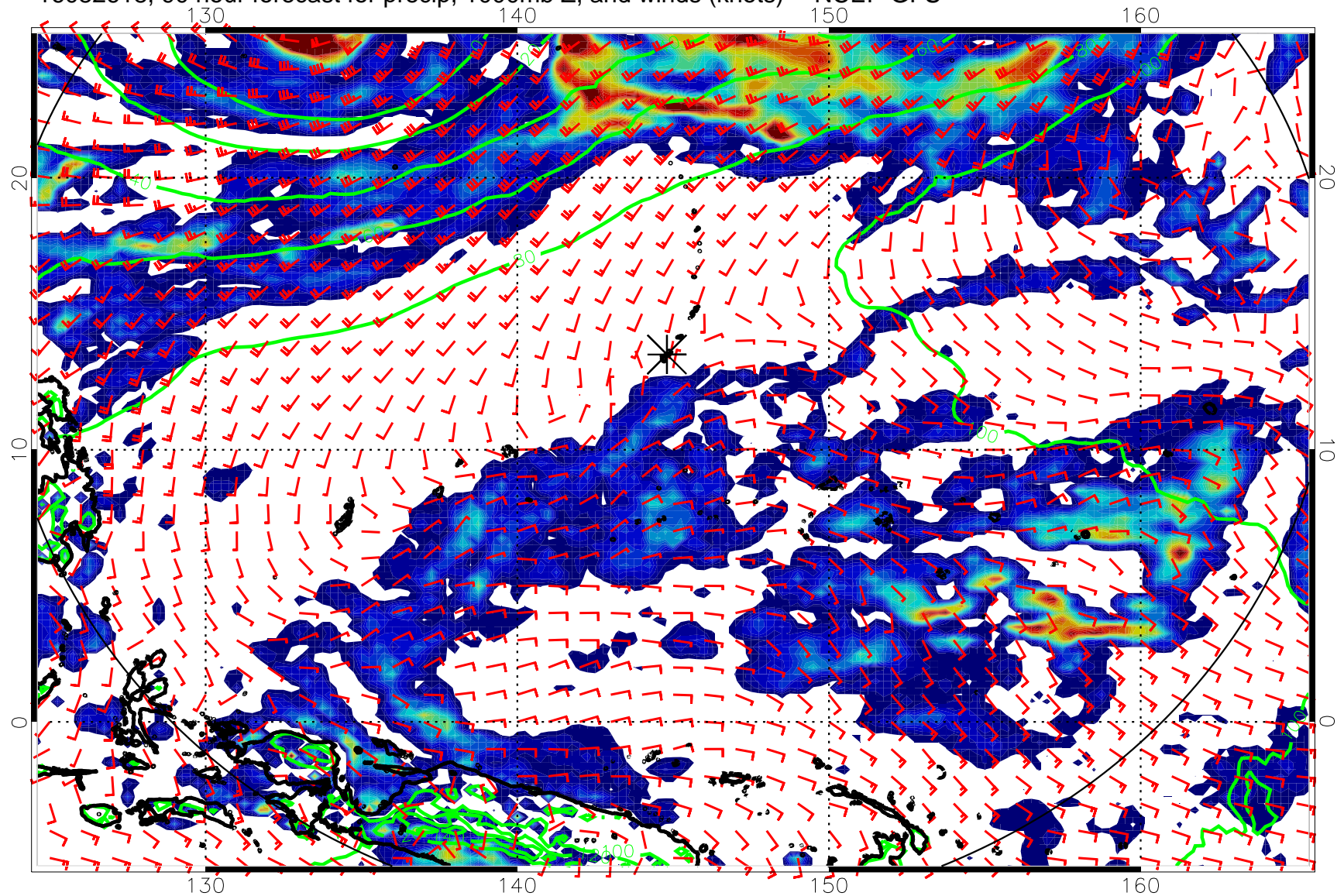
16082618, 90 hour forecast for precip, 1000mb Z, and winds (knots) -- NCEP GFS
