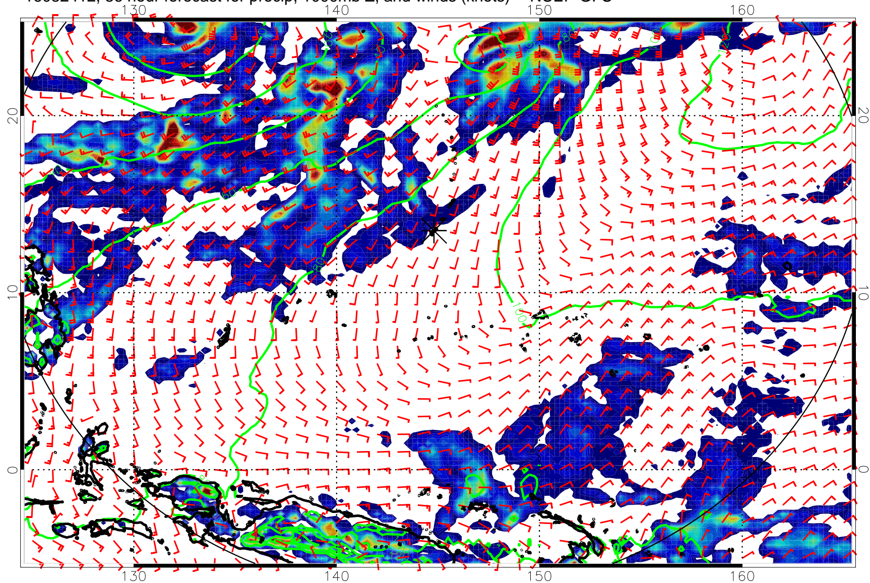
16082412, 36 hour forecast for precip, 1000mb Z, and winds (knots) -- NCEP GFS
