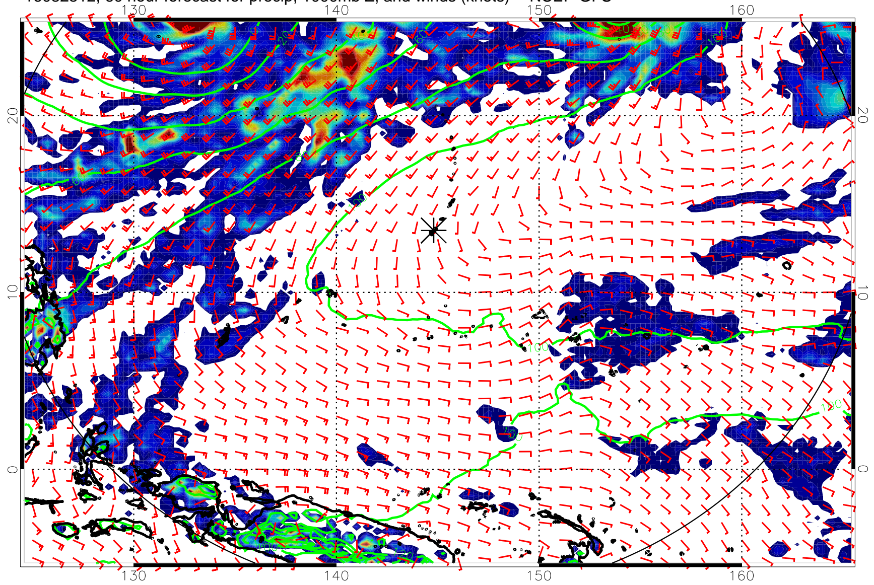
16082512, 60 hour forecast for precip, 1000mb Z, and winds (knots) -- NCEP GFS
