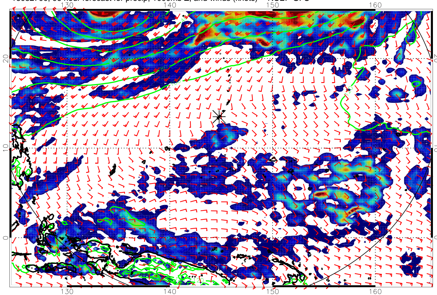
16082700, 96 hour forecast for precip, 1000mb Z, and winds (knots) -- NCEP GFS
