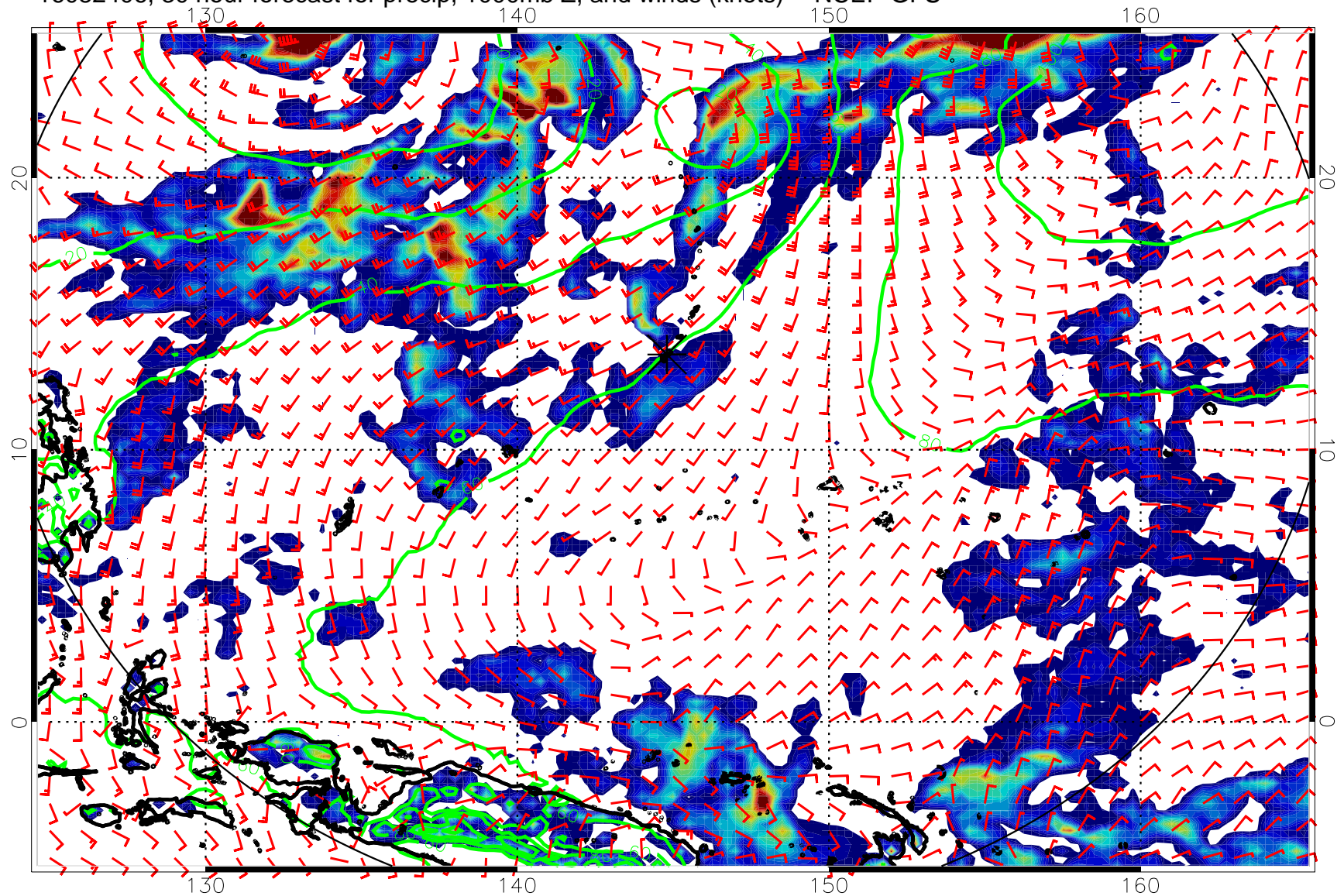
16082406, 30 hour forecast for precip, 1000mb Z, and winds (knots) -- NCEP GFS
