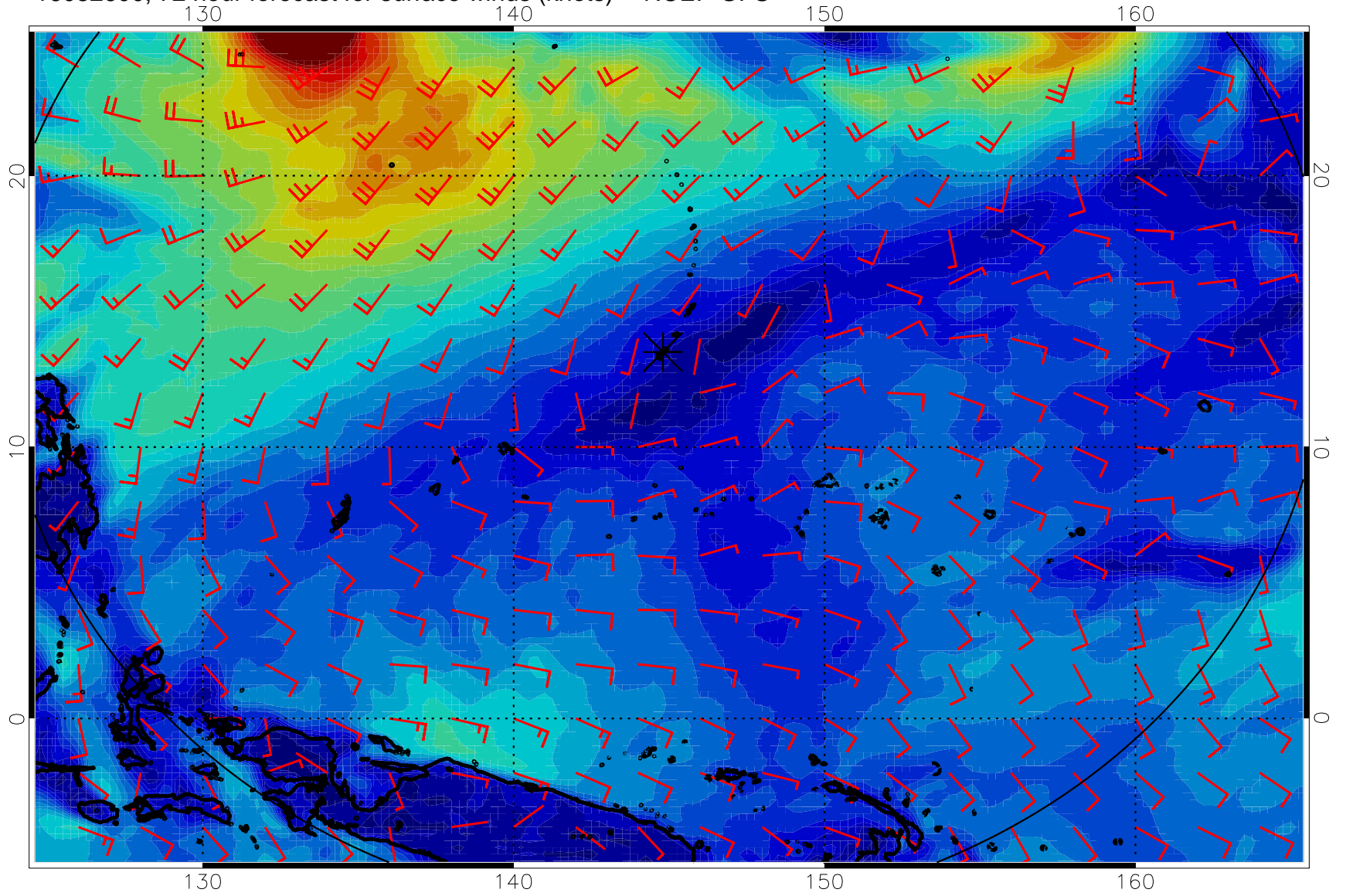
16082600, 72 hour forecast for surface winds (knots) -- NCEP GFS
