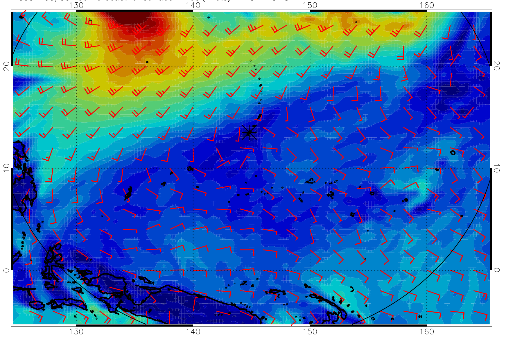
16082700, 96 hour forecast for surface winds (knots) -- NCEP GFS
