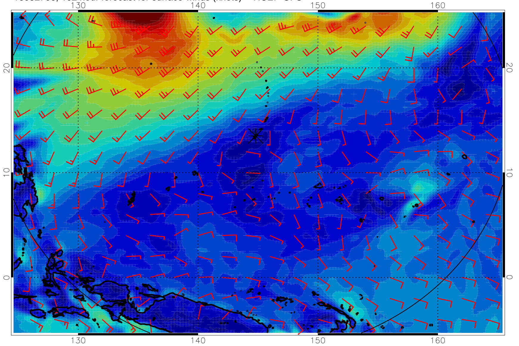
16082706, 102 hour forecast for surface winds (knots) -- NCEP GFS
