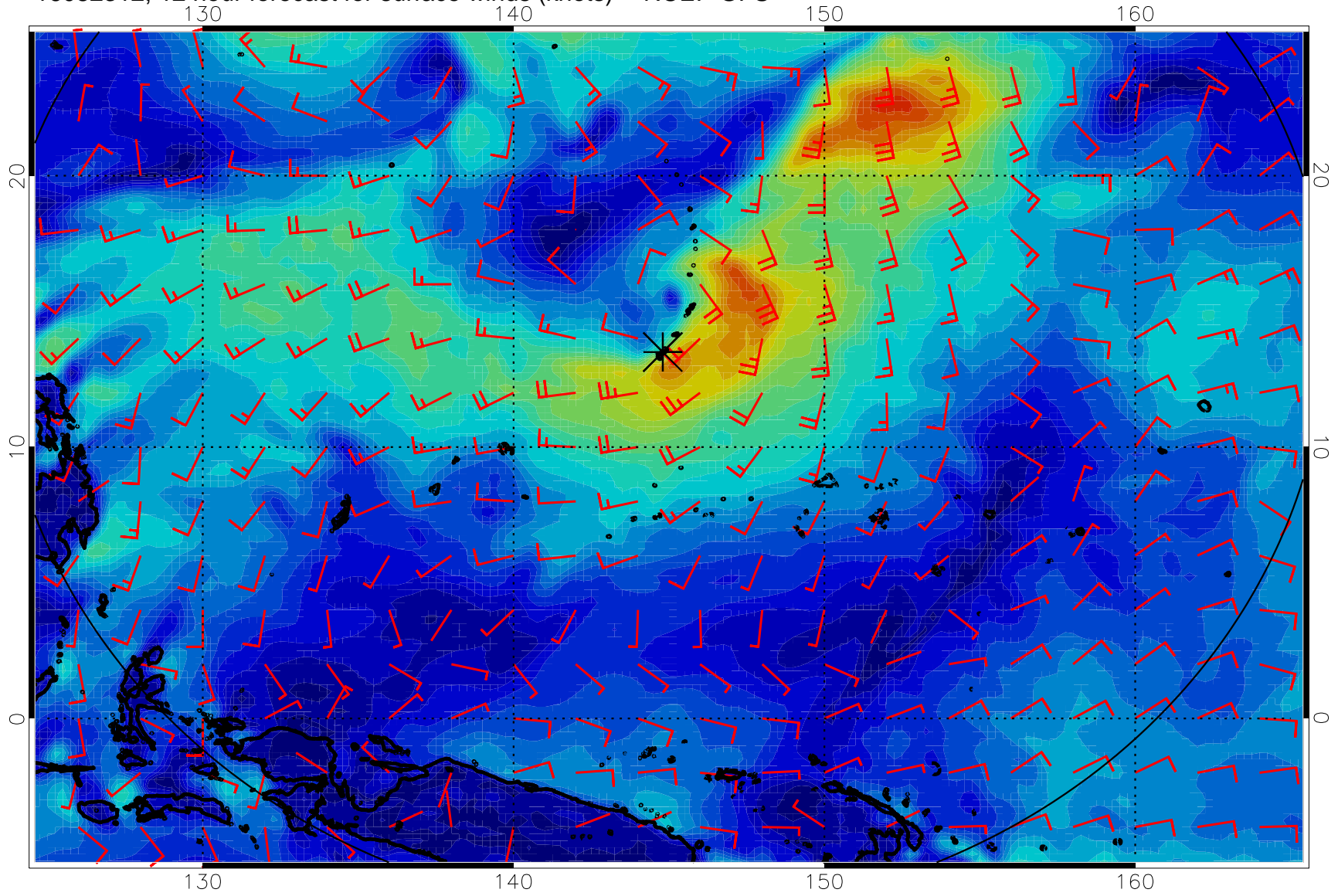
16082312, 12 hour forecast for surface winds (knots) -- NCEP GFS
