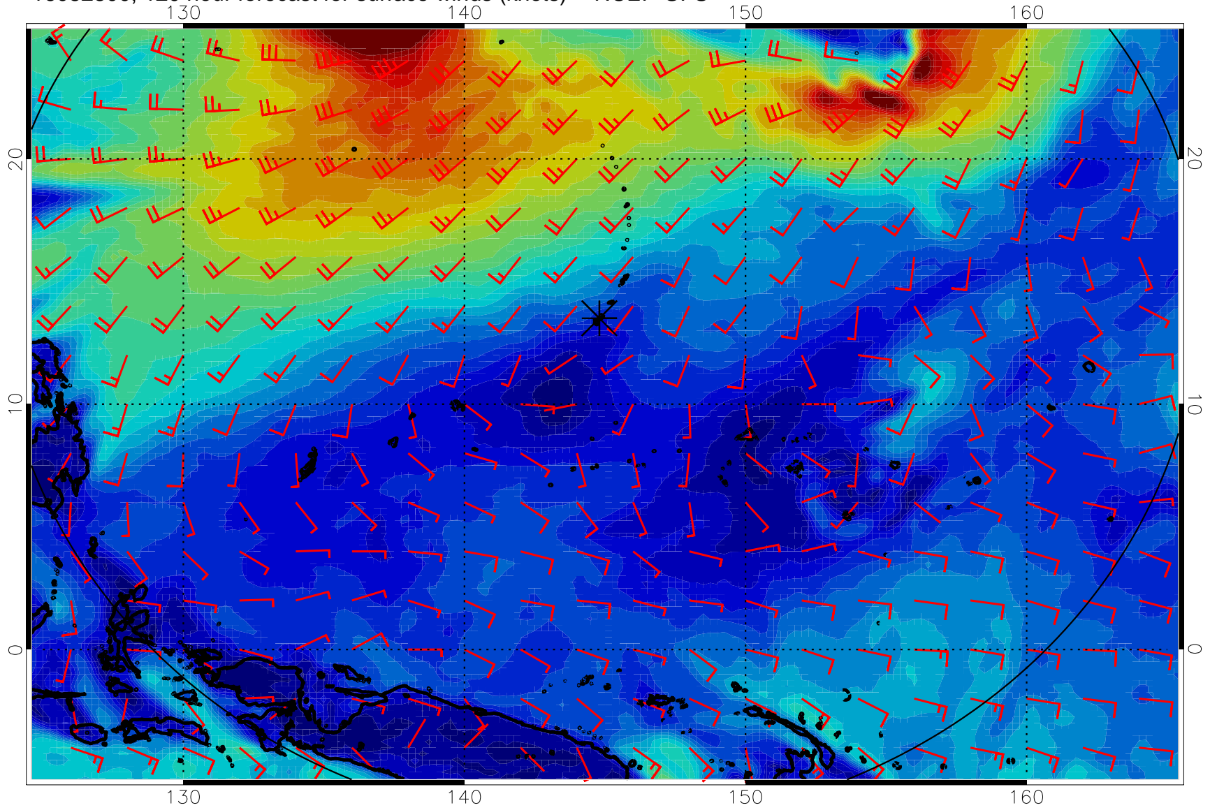
16082800, 120 hour forecast for surface winds (knots) -- NCEP GFS
