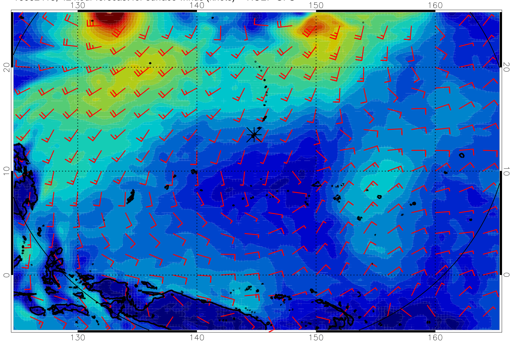
16082418, 42 hour forecast for surface winds (knots) -- NCEP GFS
