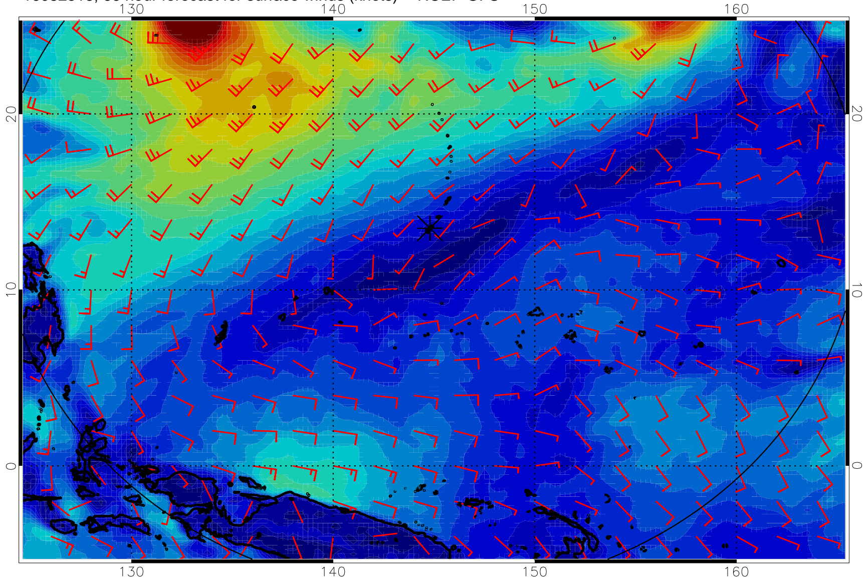
16082518, 66 hour forecast for surface winds (knots) -- NCEP GFS
