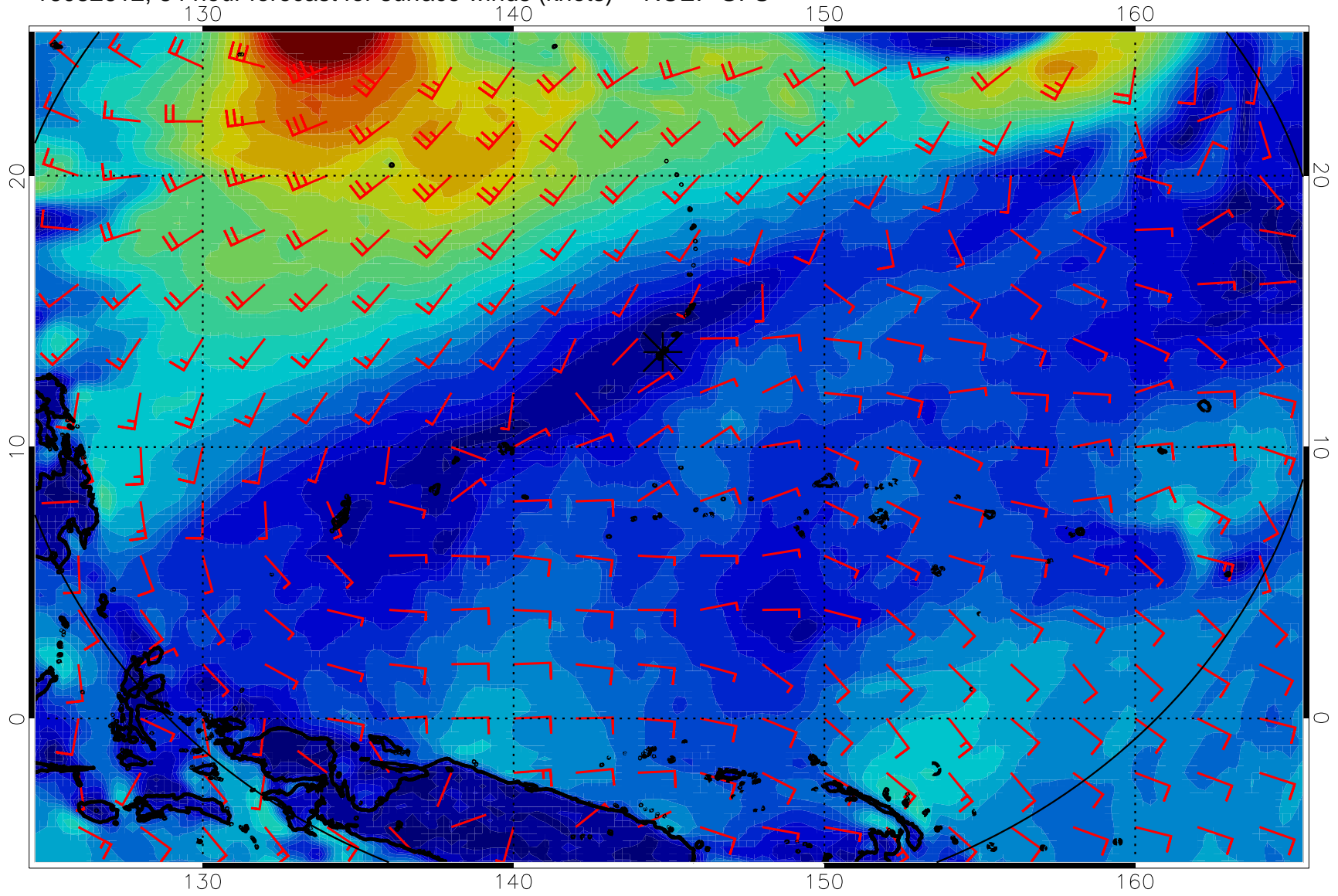
16082612, 84 hour forecast for surface winds (knots) -- NCEP GFS
