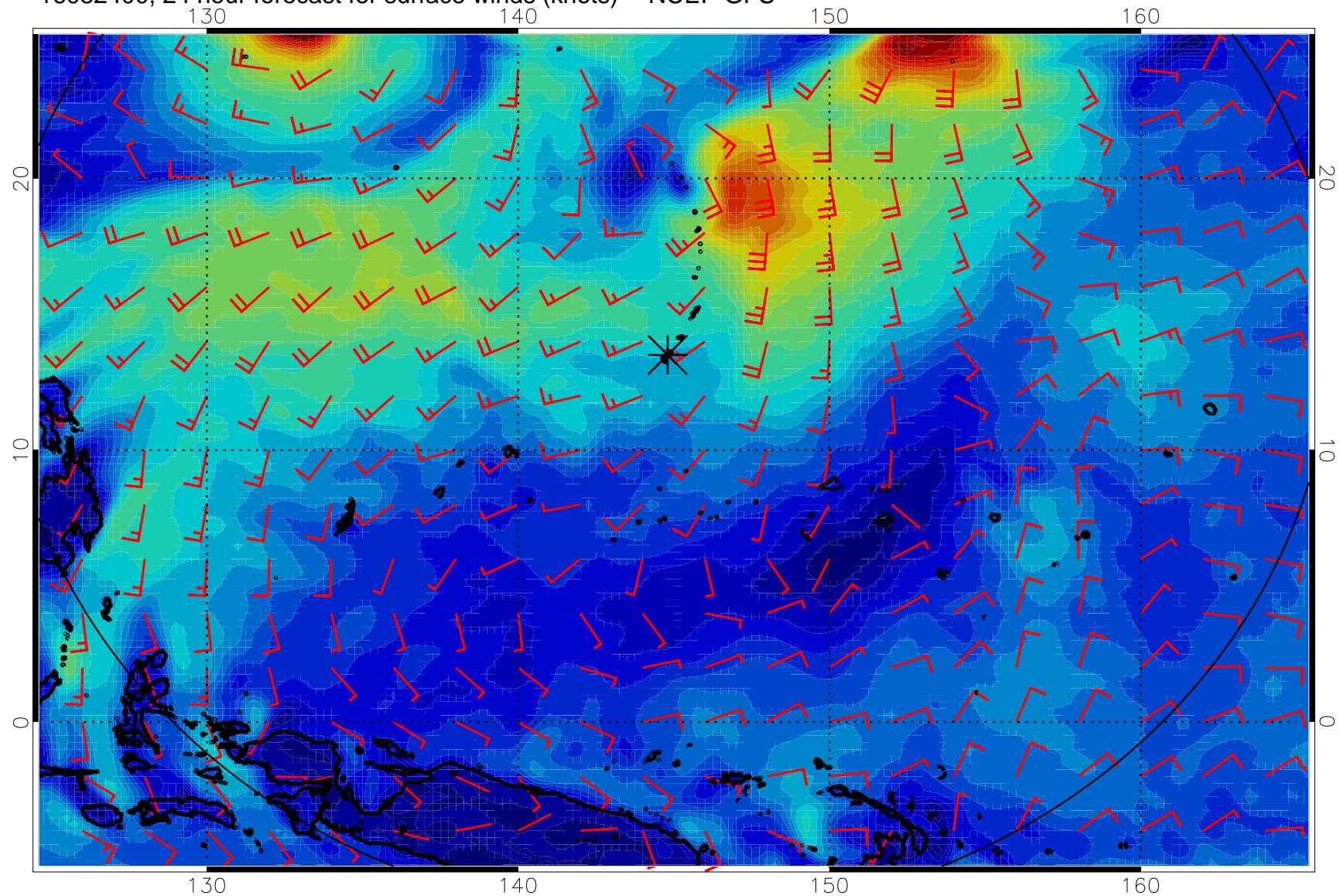
16082400, 24 hour forecast for surface winds (knots) -- NCEP GFS
