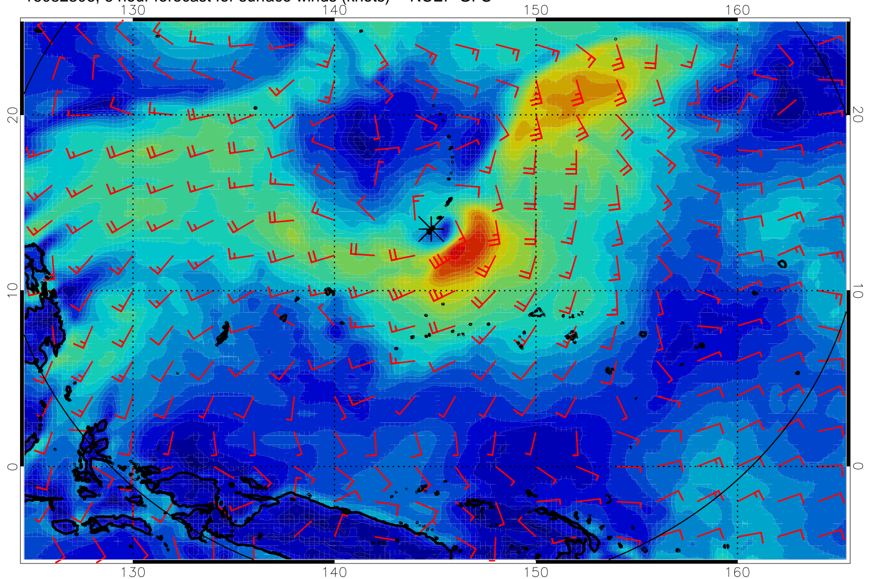
16082306, 6 hour forecast for surface winds (knots) -- NCEP GFS
