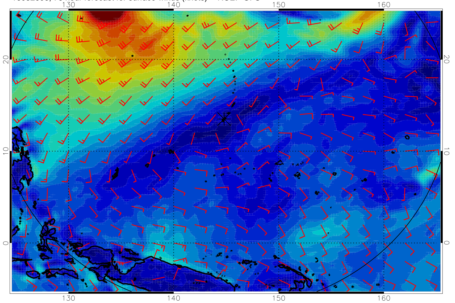
16082606, 78 hour forecast for surface winds (knots) -- NCEP GFS
