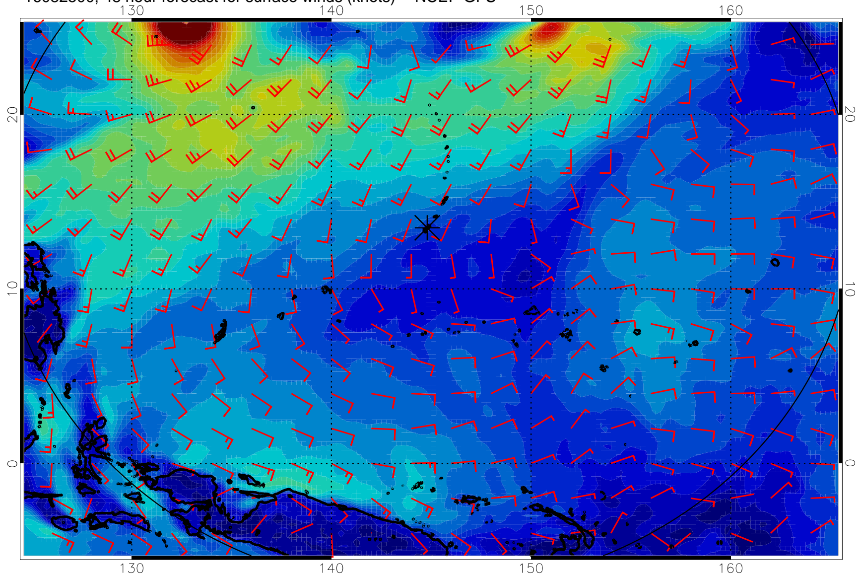
16082500, 48 hour forecast for surface winds (knots) -- NCEP GFS
