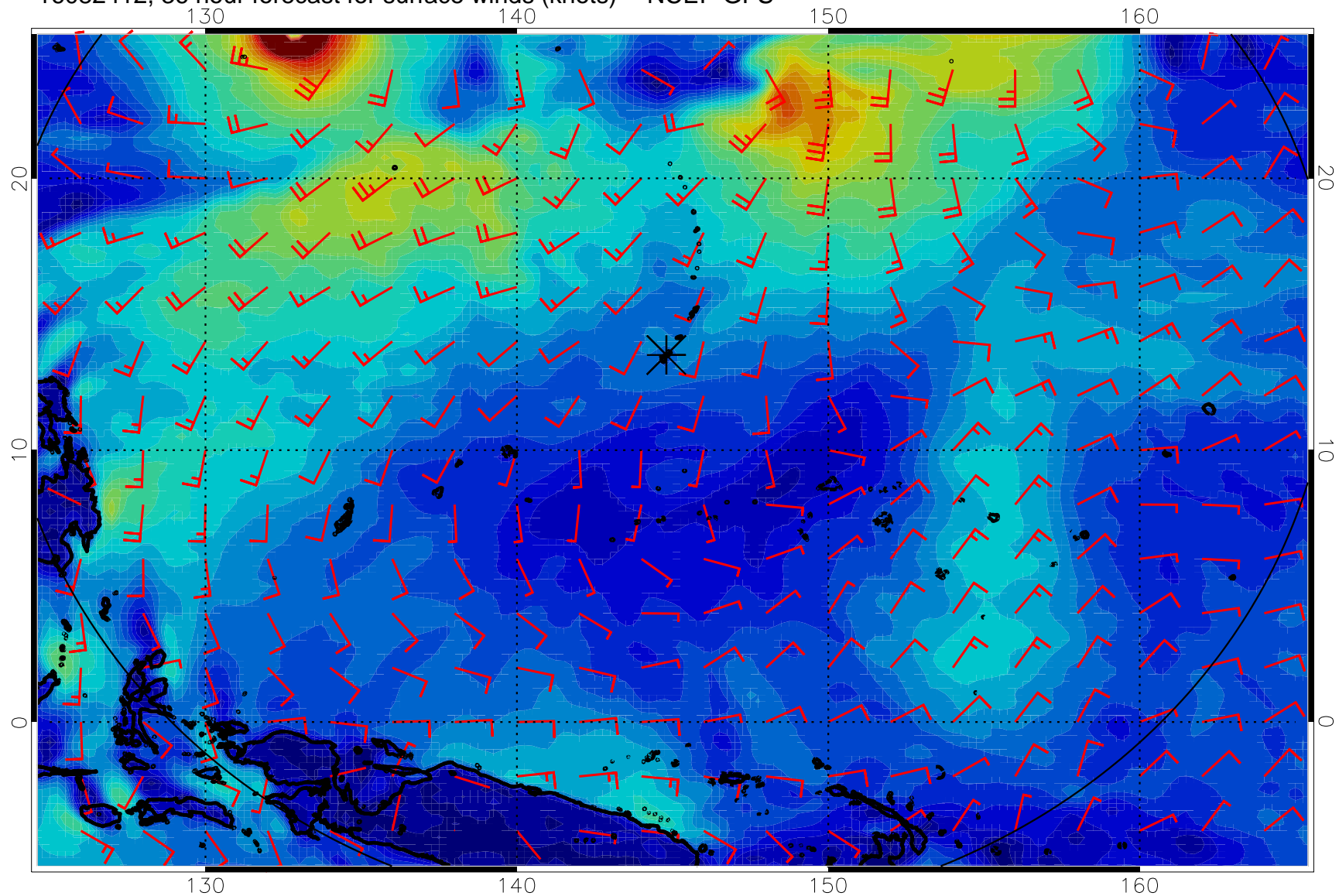
16082412, 36 hour forecast for surface winds (knots) -- NCEP GFS
