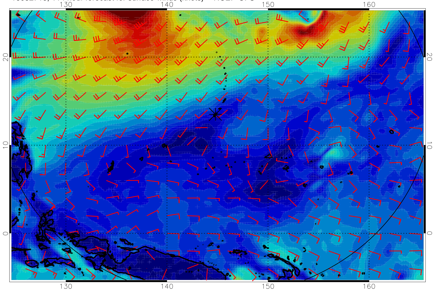
16082718, 114 hour forecast for surface winds (knots) -- NCEP GFS
