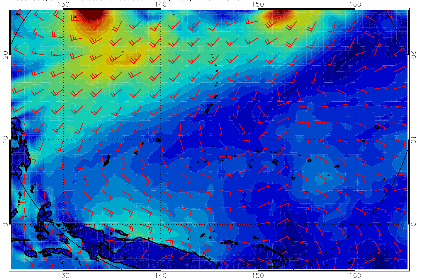
16082506, 54 hour forecast for surface winds (knots) -- NCEP GFS
