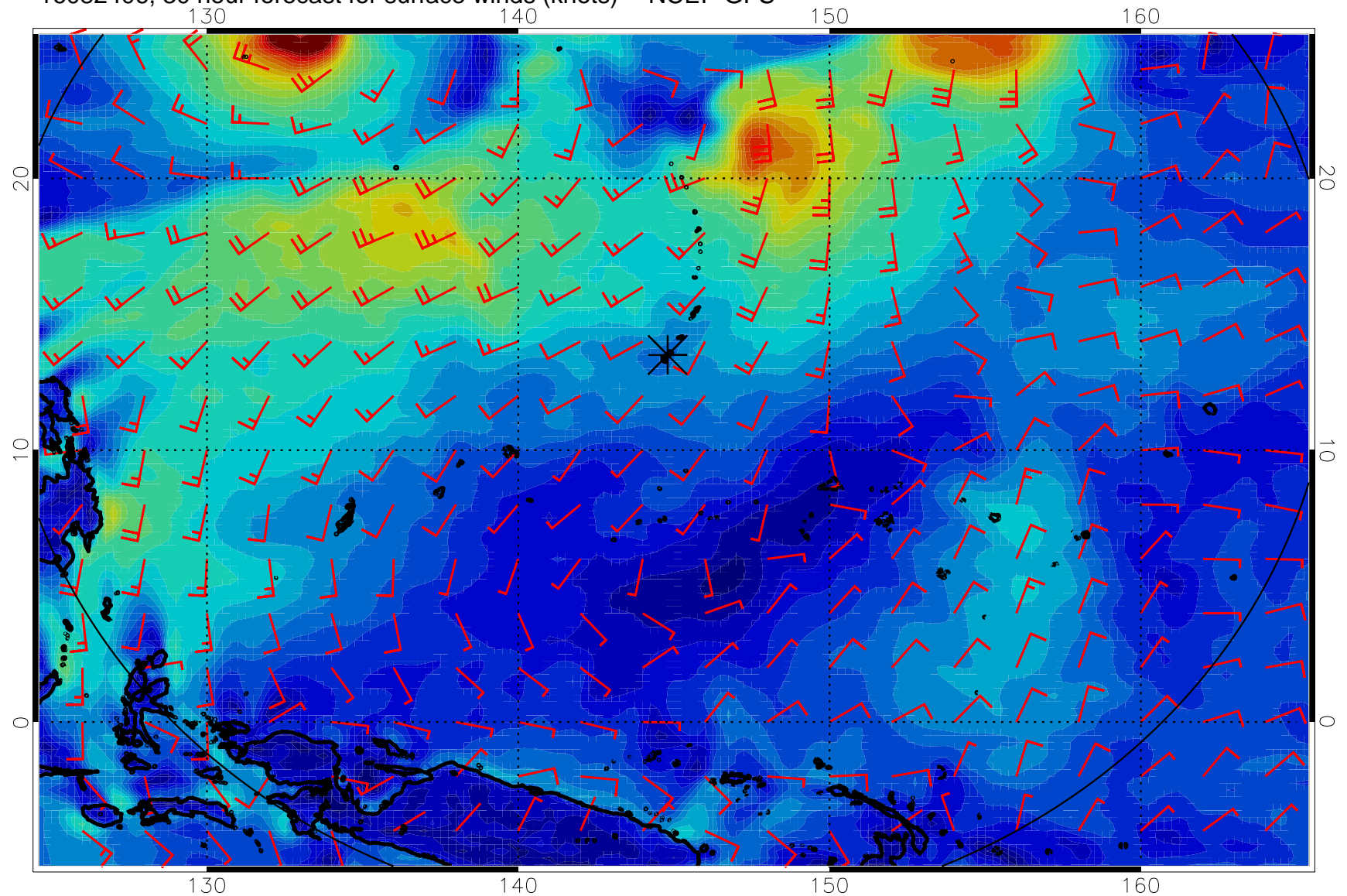
16082406, 30 hour forecast for surface winds (knots) -- NCEP GFS
