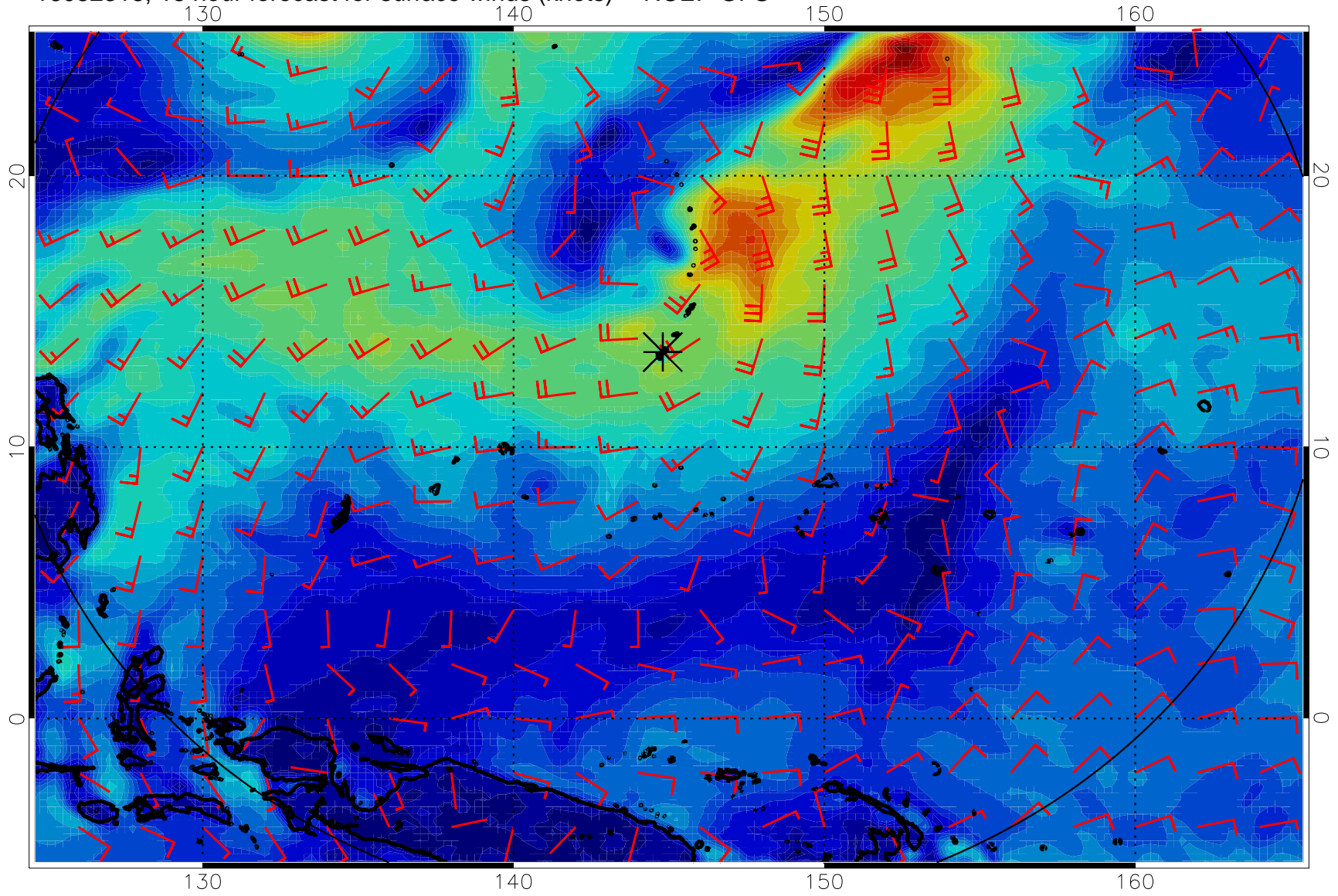
16082318, 18 hour forecast for surface winds (knots) -- NCEP GFS
