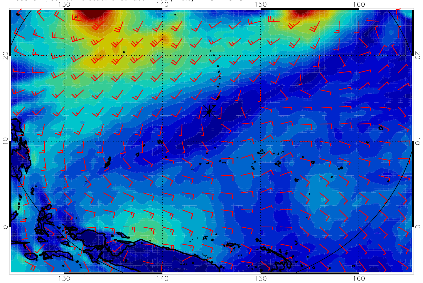
16082512, 60 hour forecast for surface winds (knots) -- NCEP GFS
