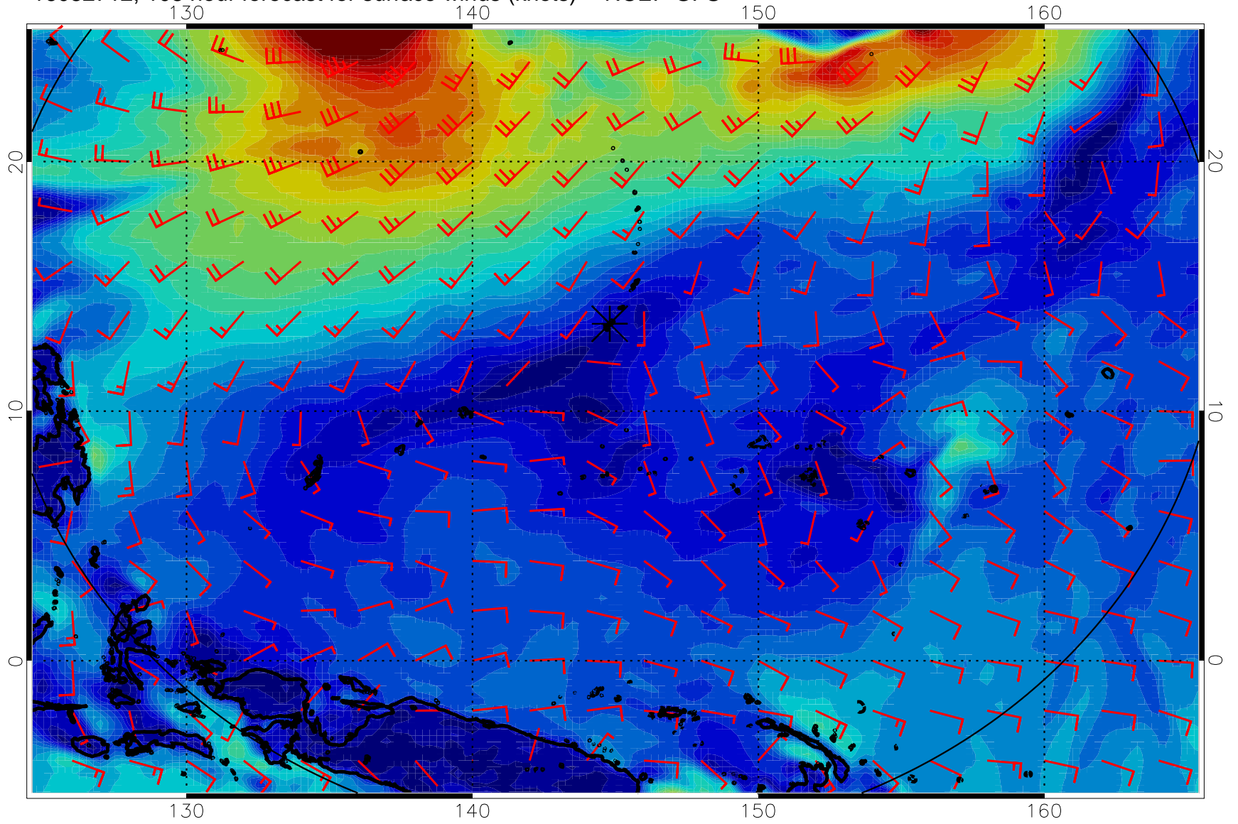
16082712, 108 hour forecast for surface winds (knots) -- NCEP GFS
