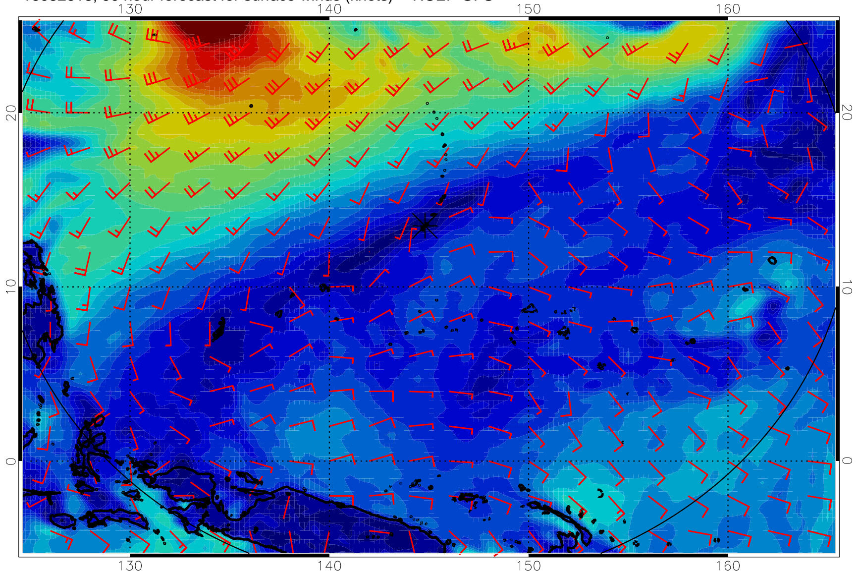
16082618, 90 hour forecast for surface winds (knots) -- NCEP GFS
