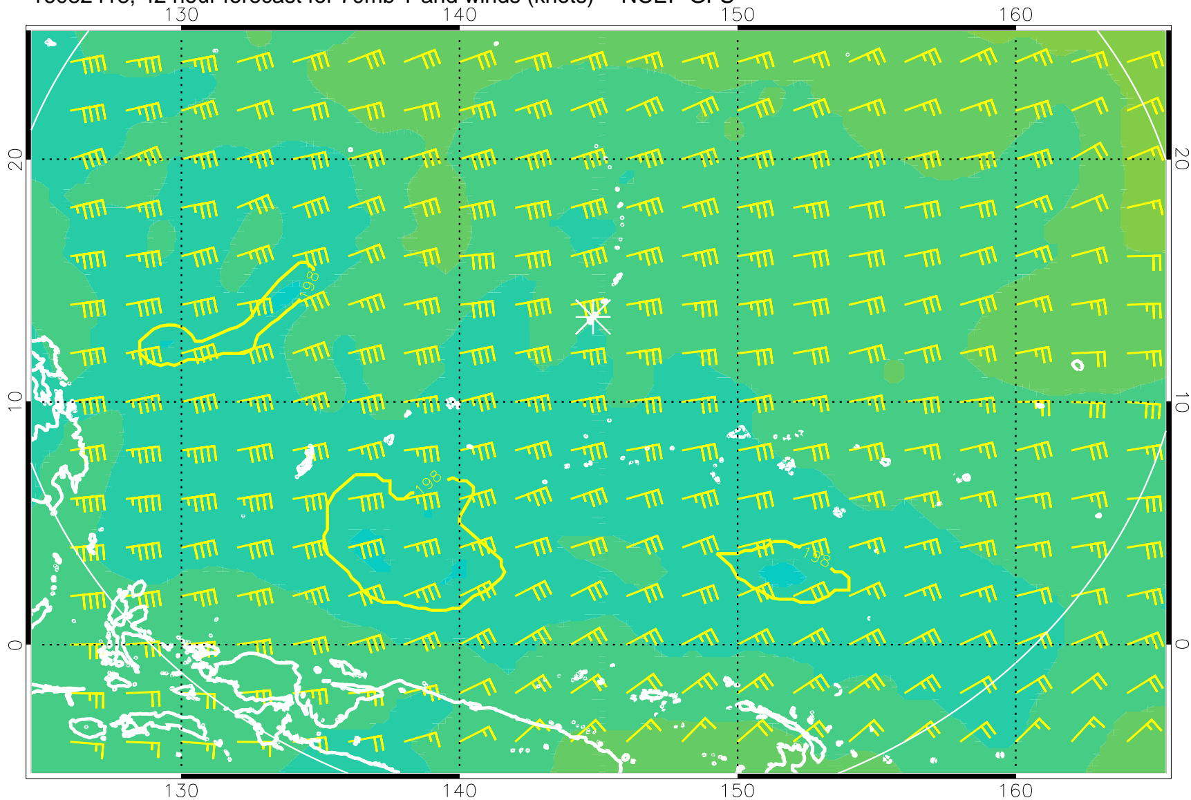
16082418, 42 hour forecast for 70mb T and winds (knots) -- NCEP GFS
