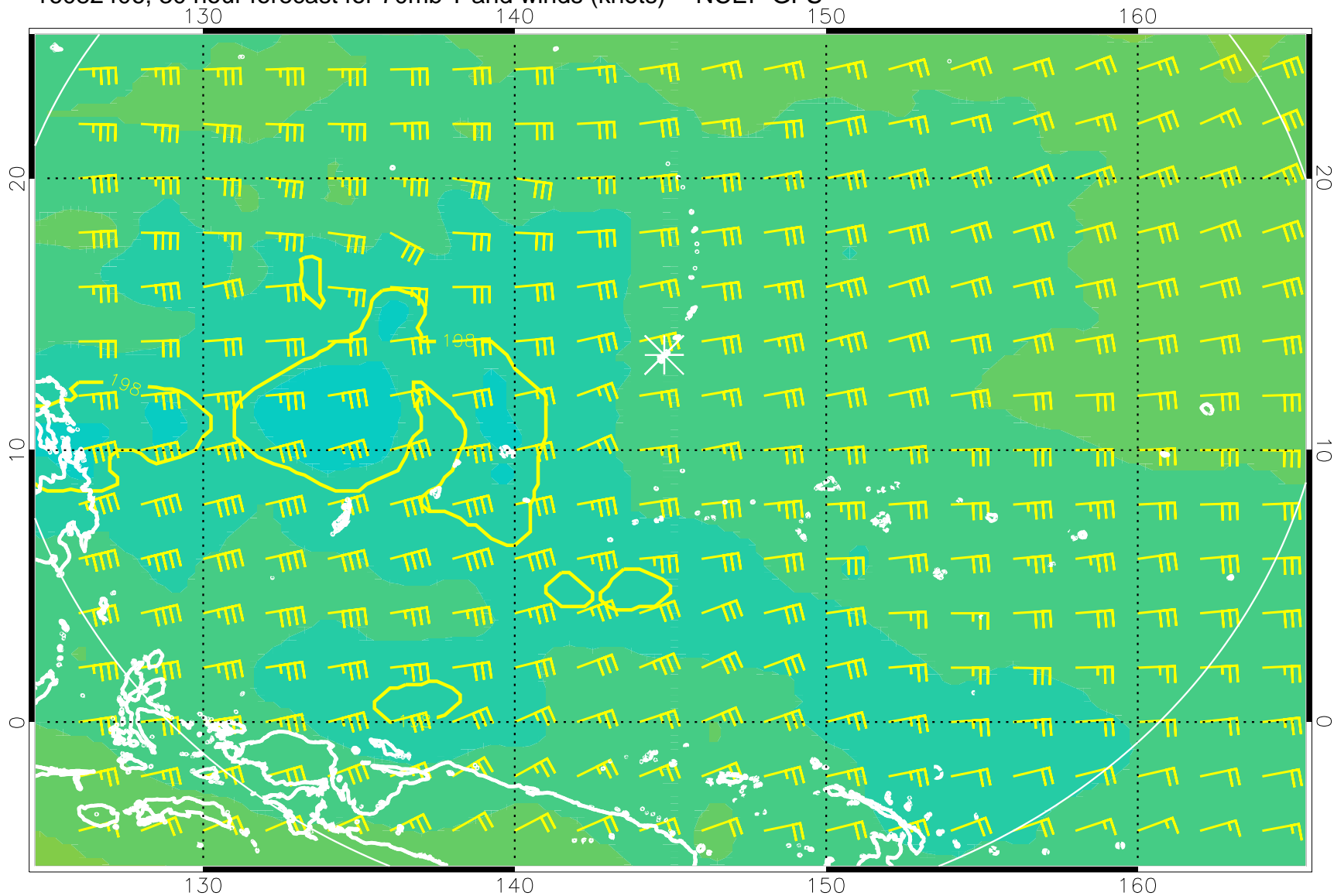
16082406, 30 hour forecast for 70mb T and winds (knots) -- NCEP GFS
