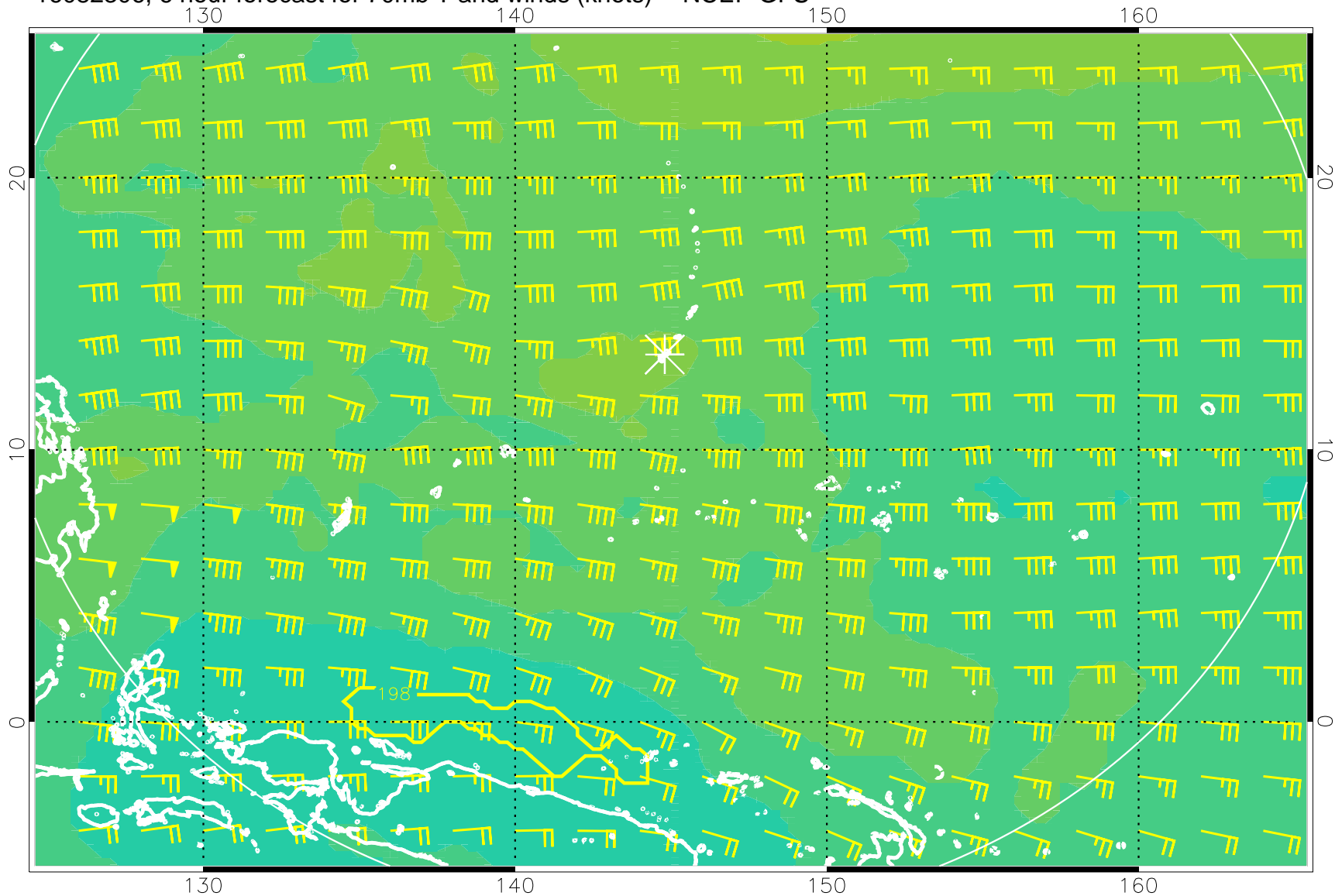
16082306, 6 hour forecast for 70mb T and winds (knots) -- NCEP GFS
