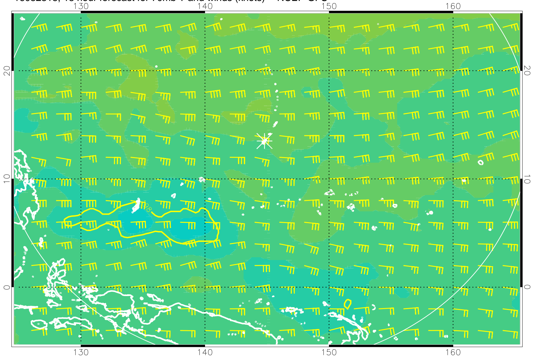
16082318, 18 hour forecast for 70mb T and winds (knots) -- NCEP GFS
