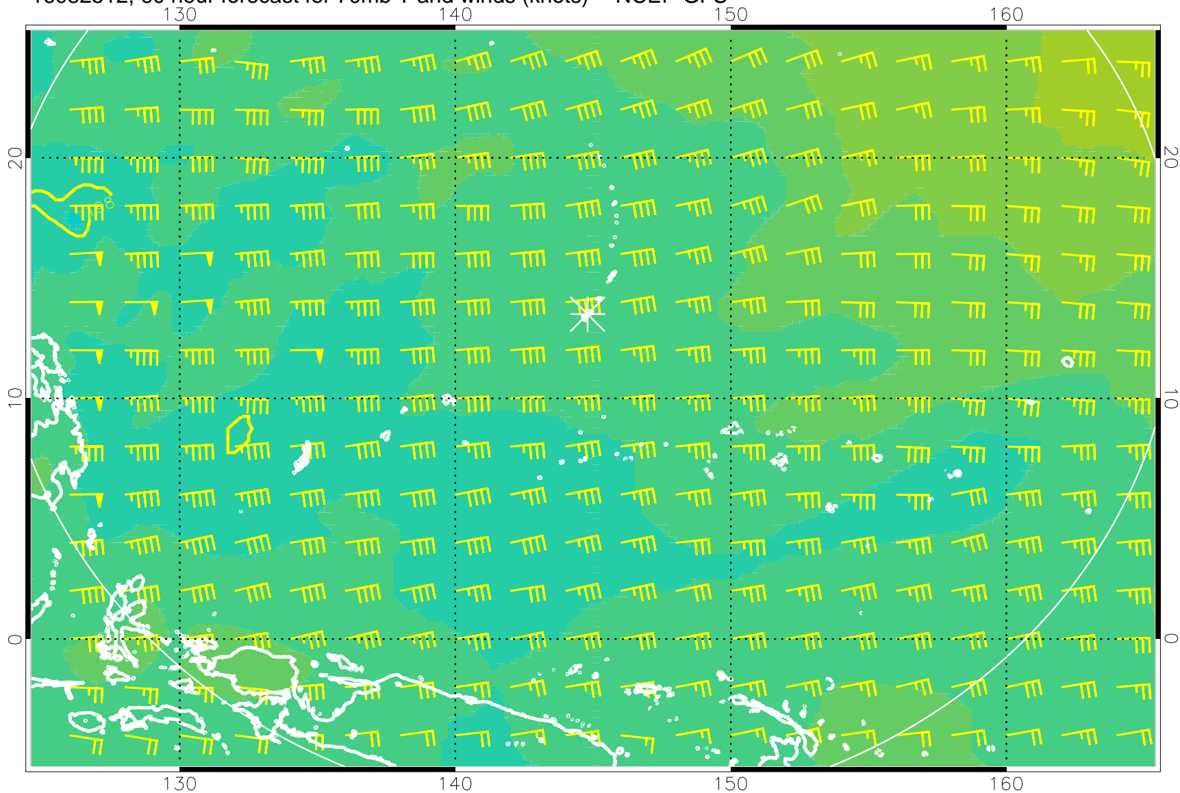
16082512, 60 hour forecast for 70mb T and winds (knots) -- NCEP GFS
