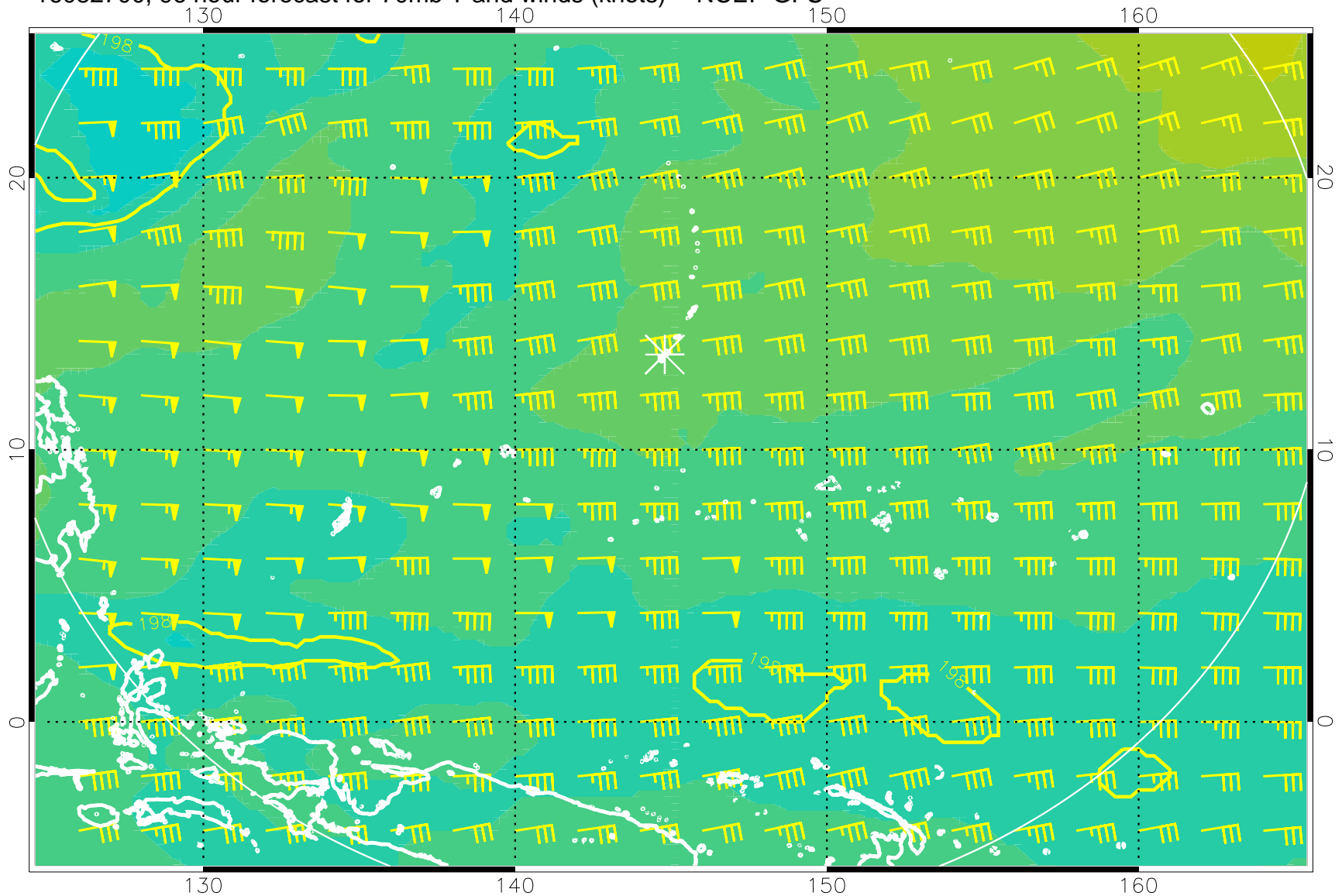
16082700, 96 hour forecast for 70mb T and winds (knots) -- NCEP GFS
