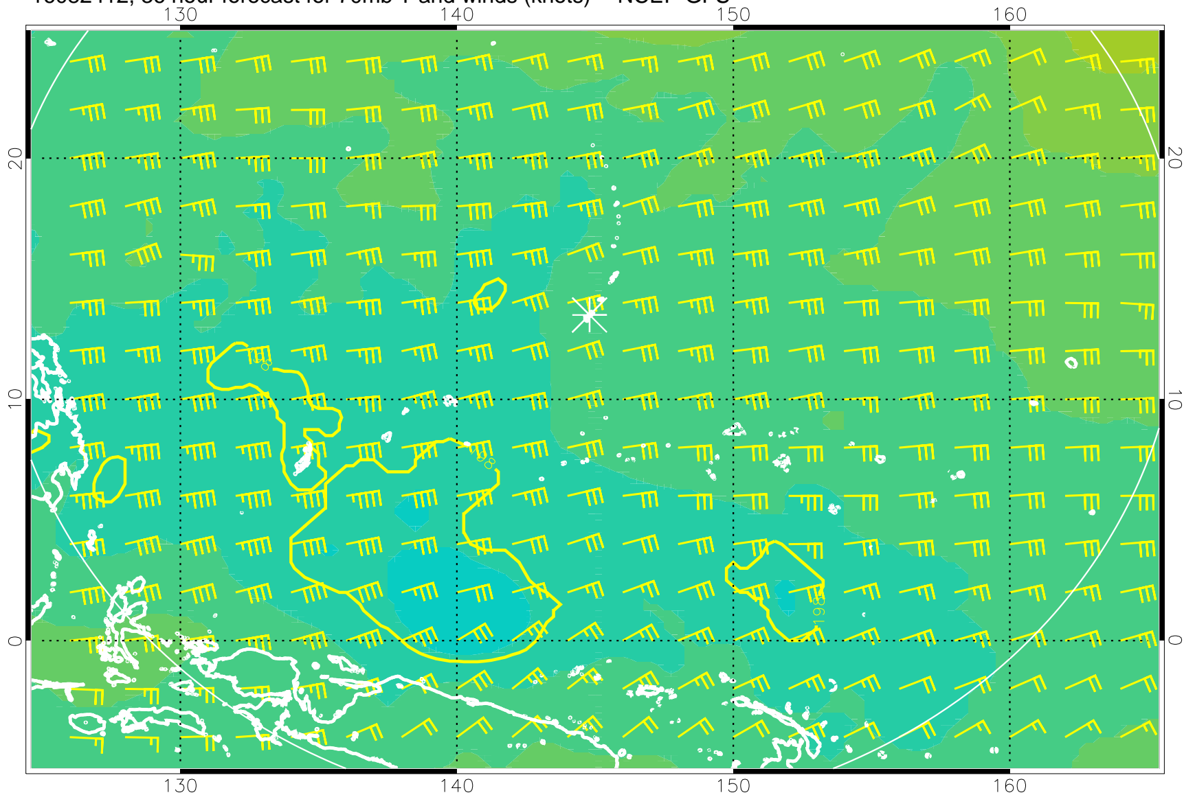
16082412, 36 hour forecast for 70mb T and winds (knots) -- NCEP GFS
