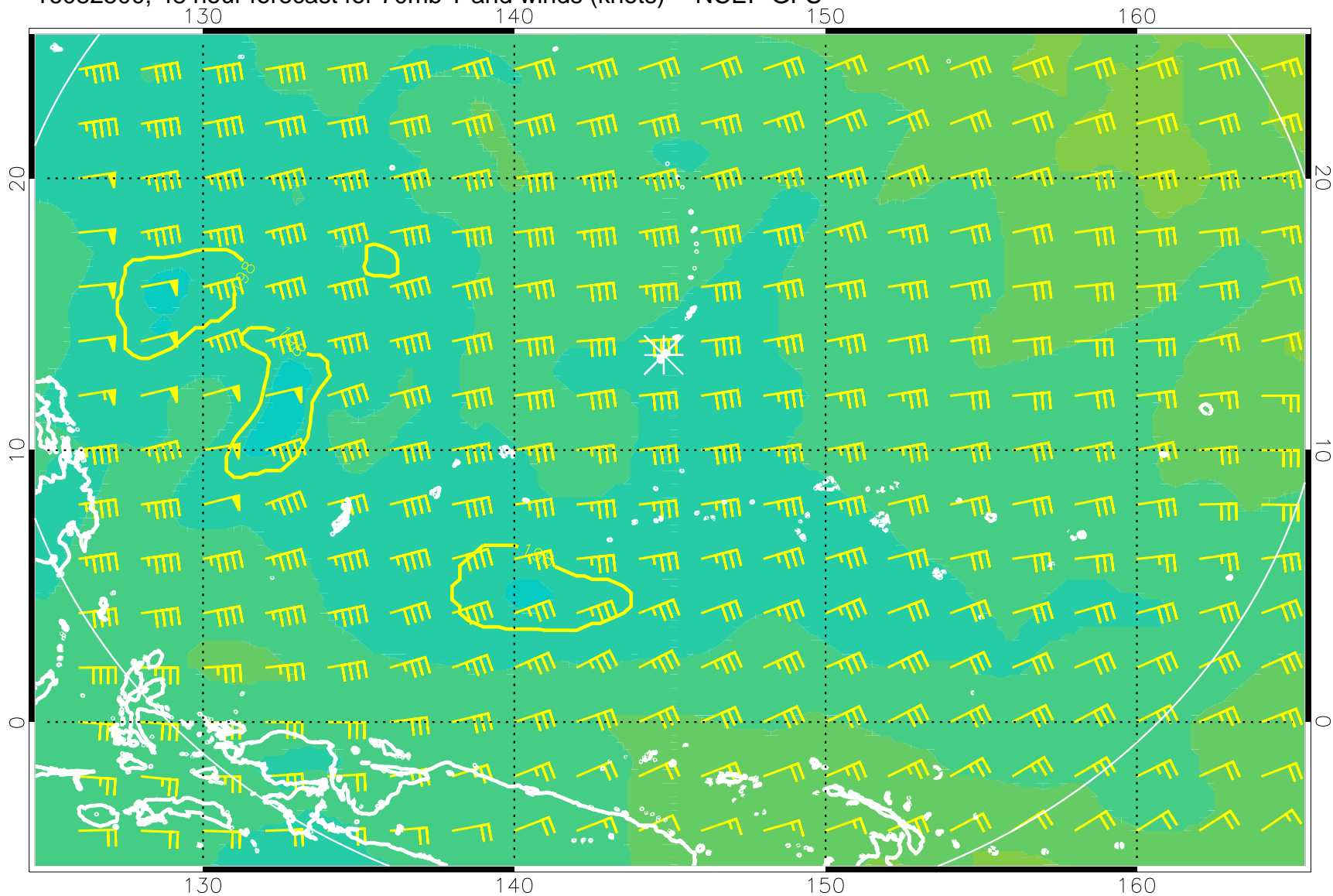
16082500, 48 hour forecast for 70mb T and winds (knots) -- NCEP GFS
