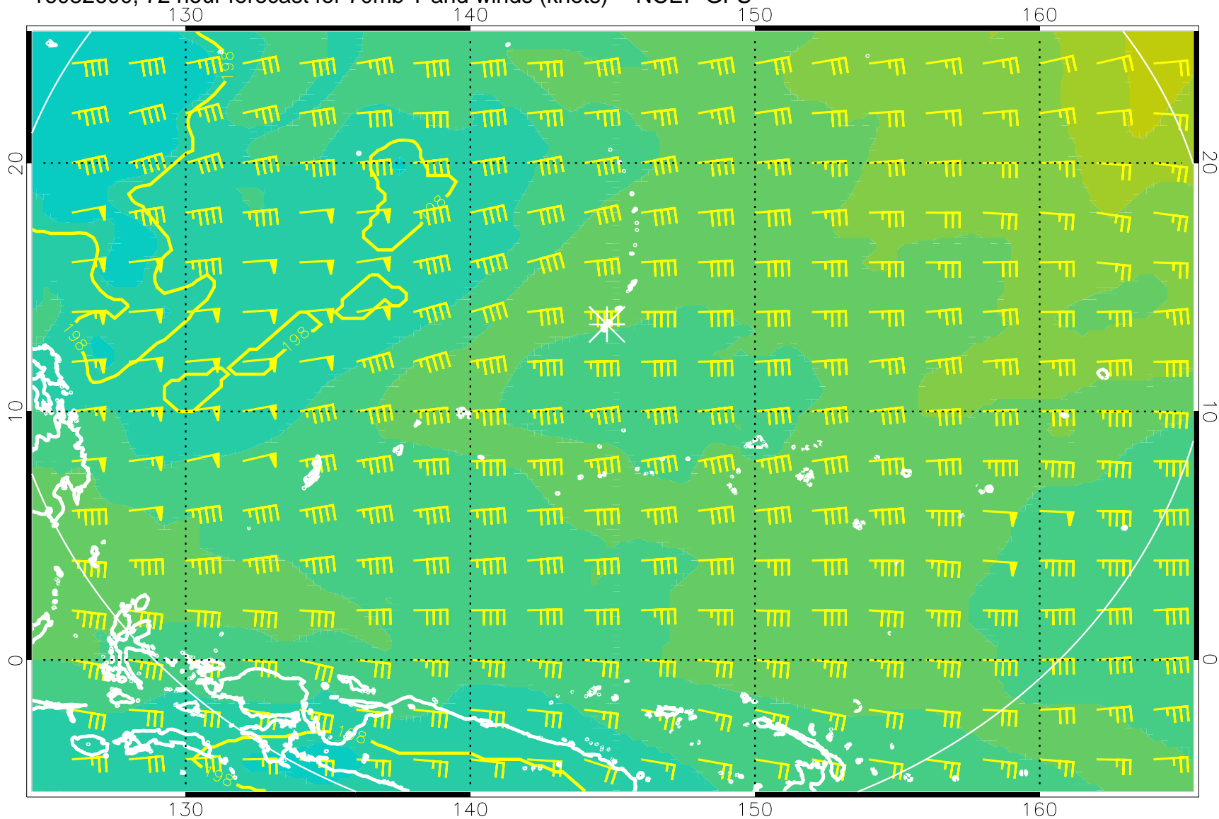
16082600, 72 hour forecast for 70mb T and winds (knots) -- NCEP GFS
