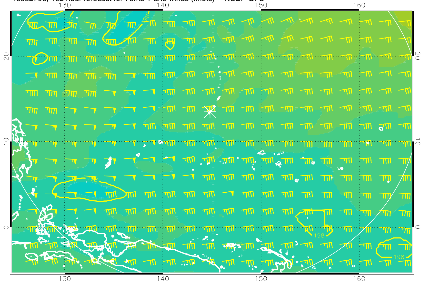
16082706, 102 hour forecast for 70mb T and winds (knots) -- NCEP GFS
