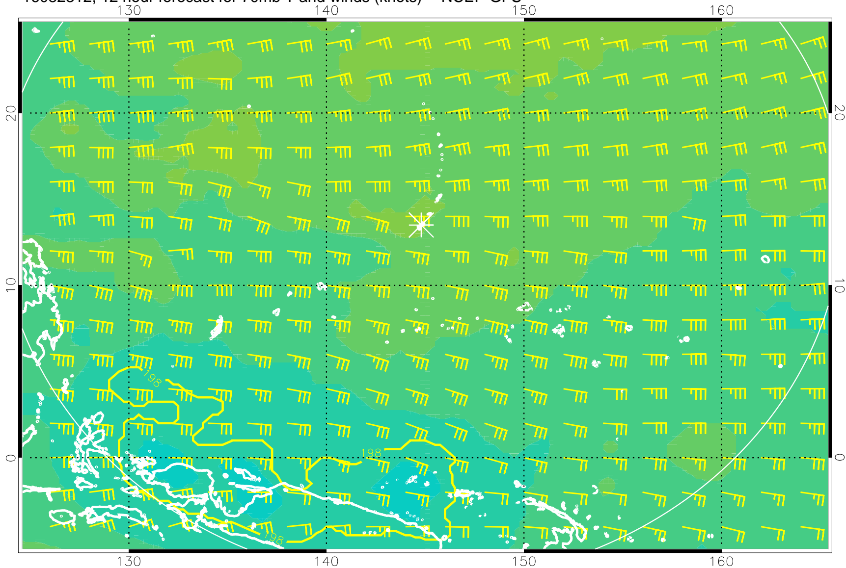
16082312, 12 hour forecast for 70mb T and winds (knots) -- NCEP GFS
