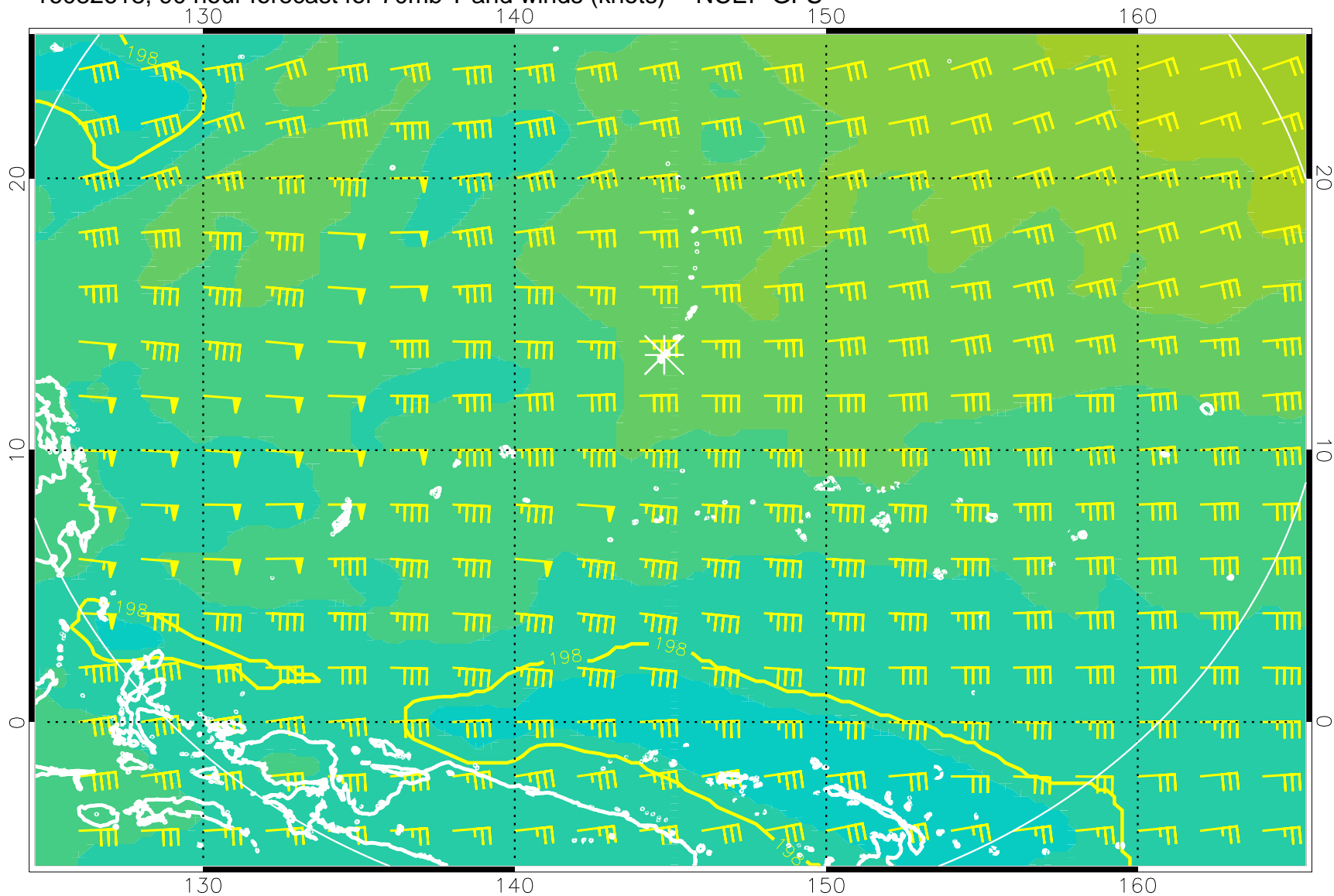
16082618, 90 hour forecast for 70mb T and winds (knots) -- NCEP GFS
