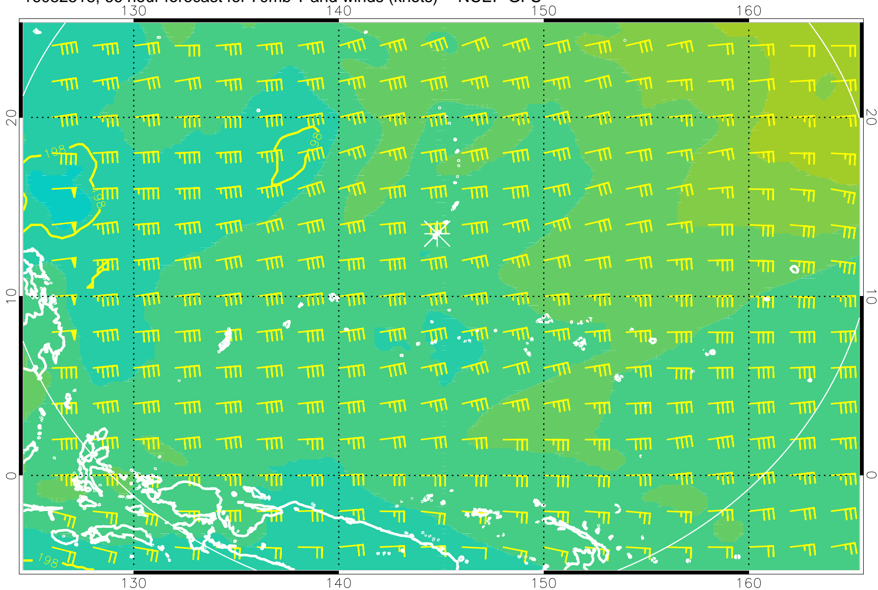
16082518, 66 hour forecast for 70mb T and winds (knots) -- NCEP GFS
