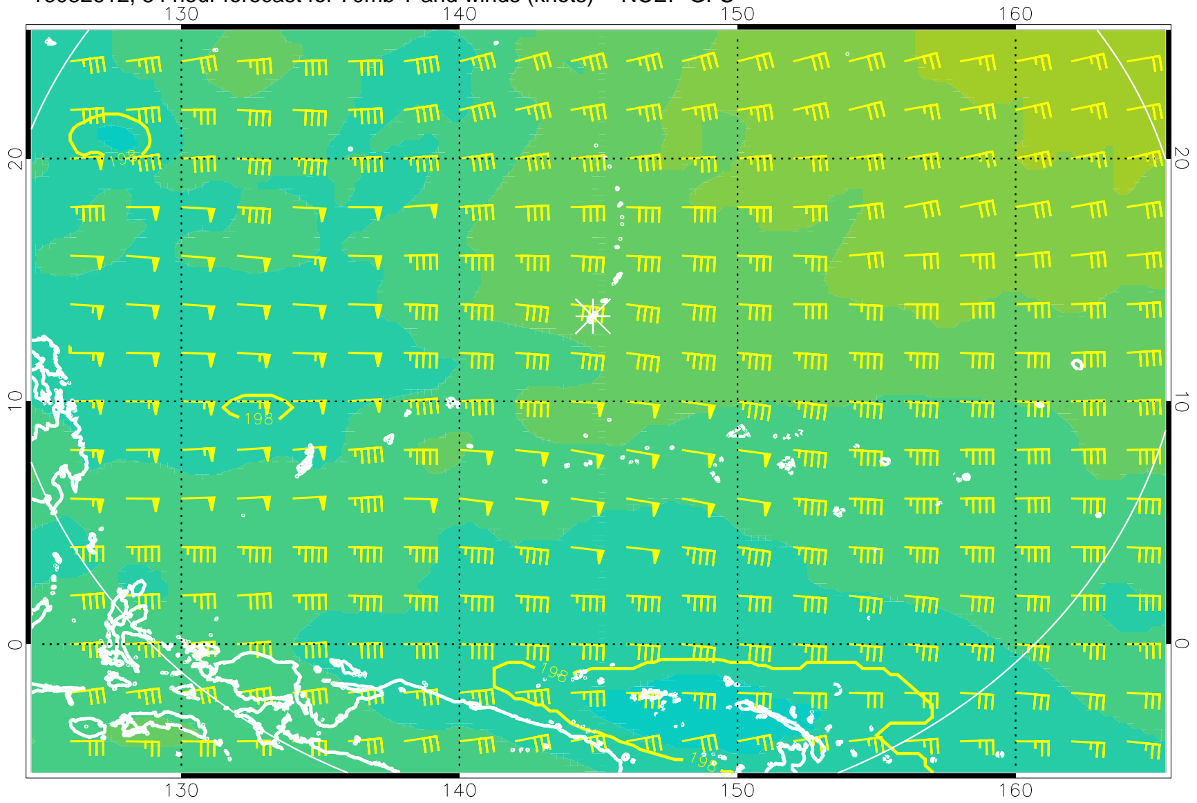
16082612, 84 hour forecast for 70mb T and winds (knots) -- NCEP GFS
