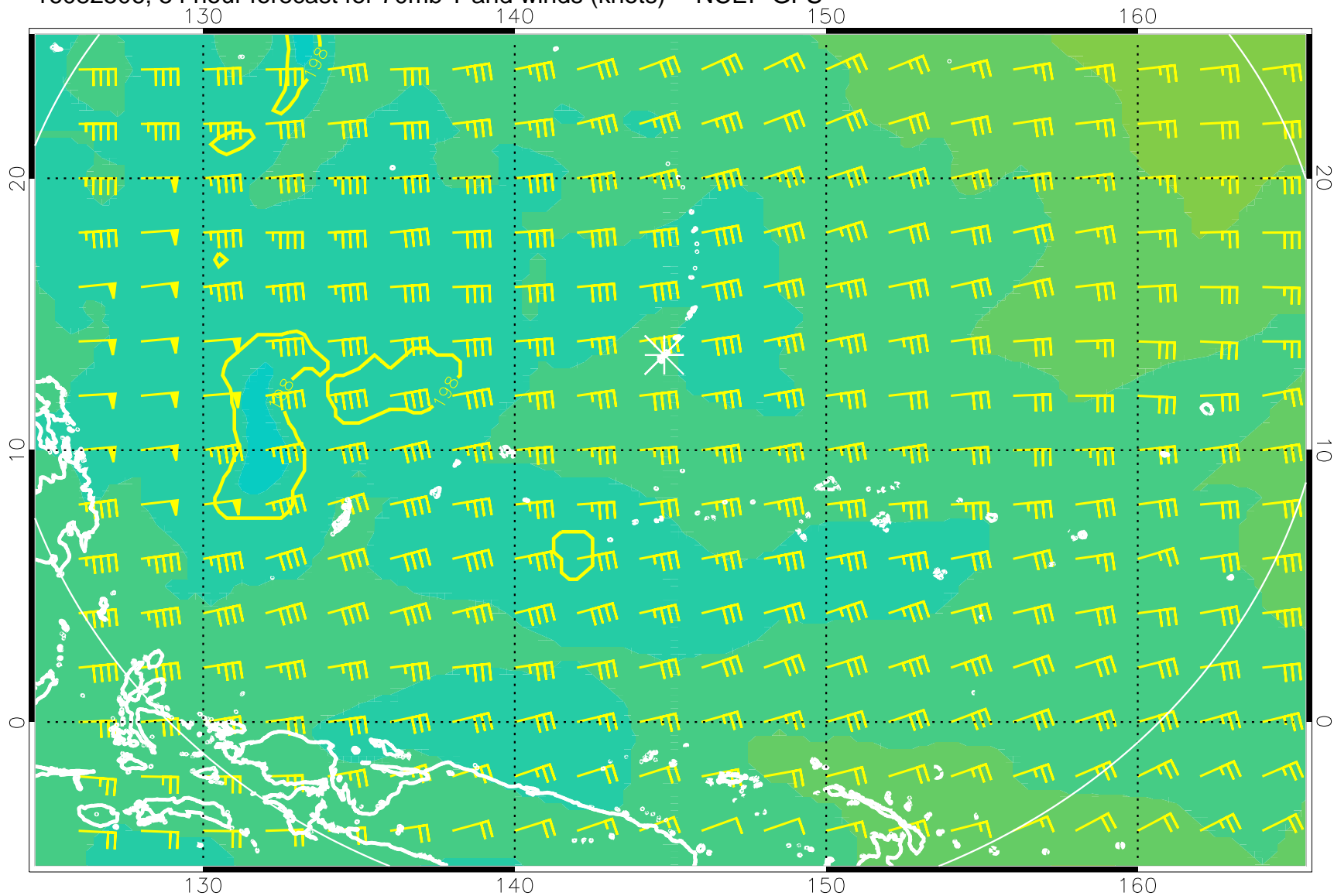
16082506, 54 hour forecast for 70mb T and winds (knots) -- NCEP GFS
