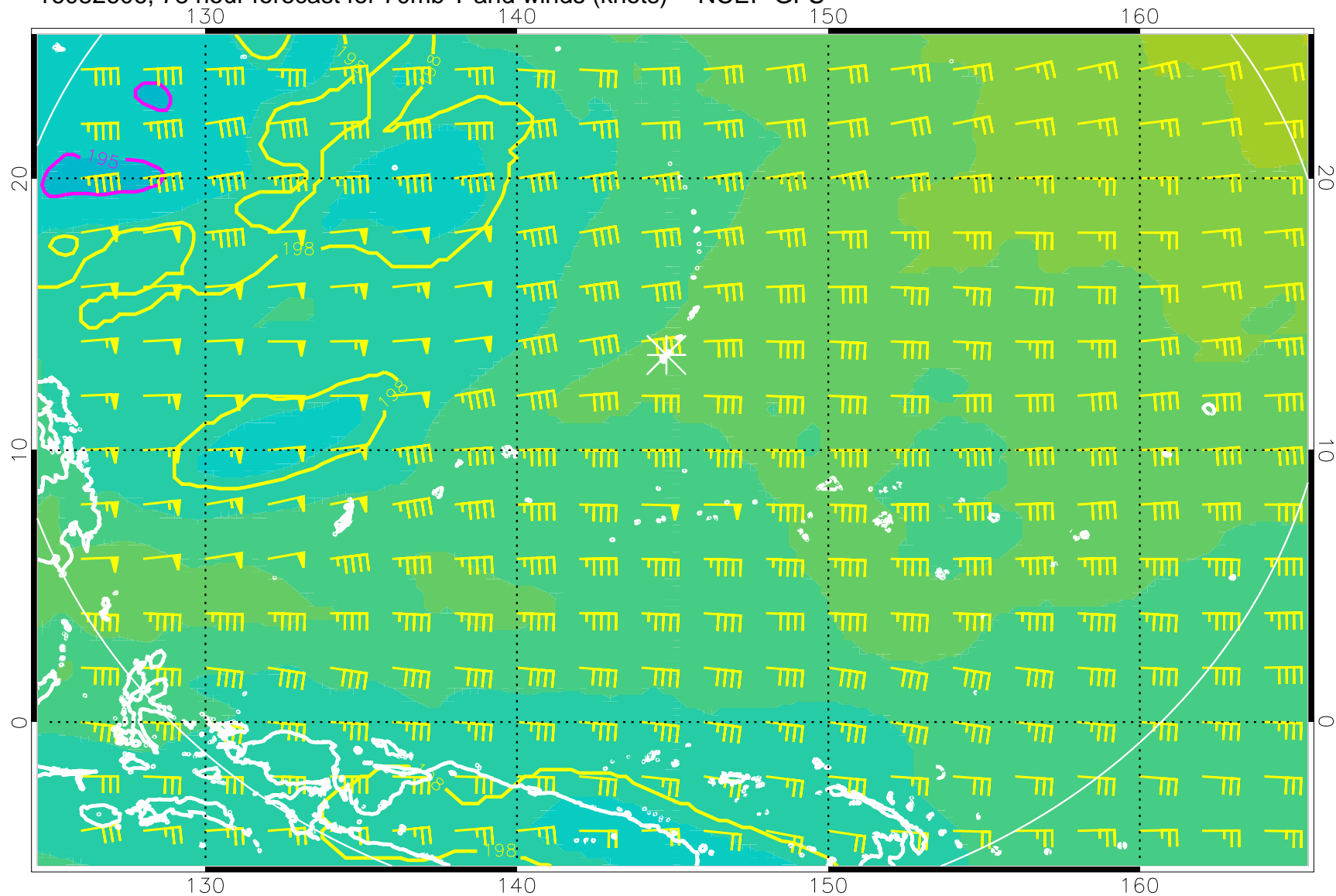
16082606, 78 hour forecast for 70mb T and winds (knots) -- NCEP GFS
