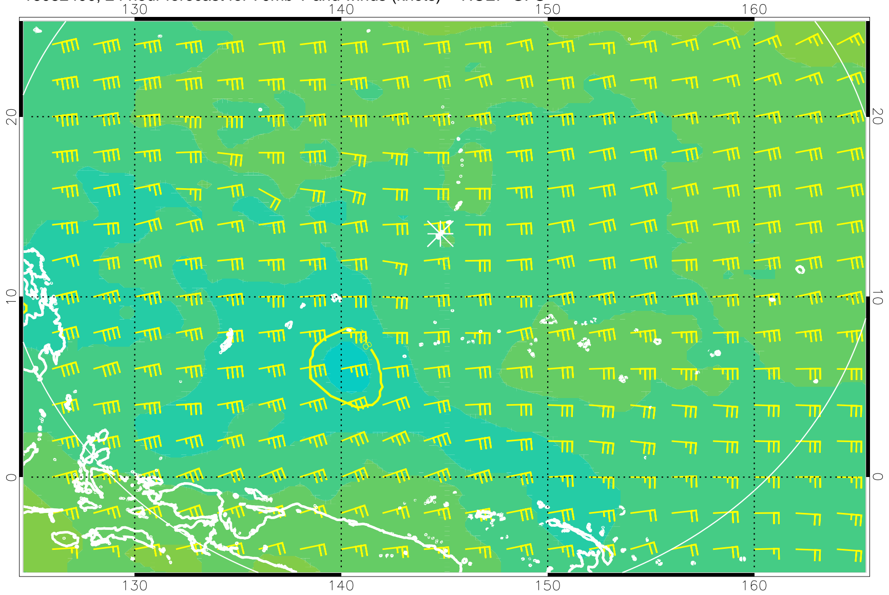
16082400, 24 hour forecast for 70mb T and winds (knots) -- NCEP GFS
