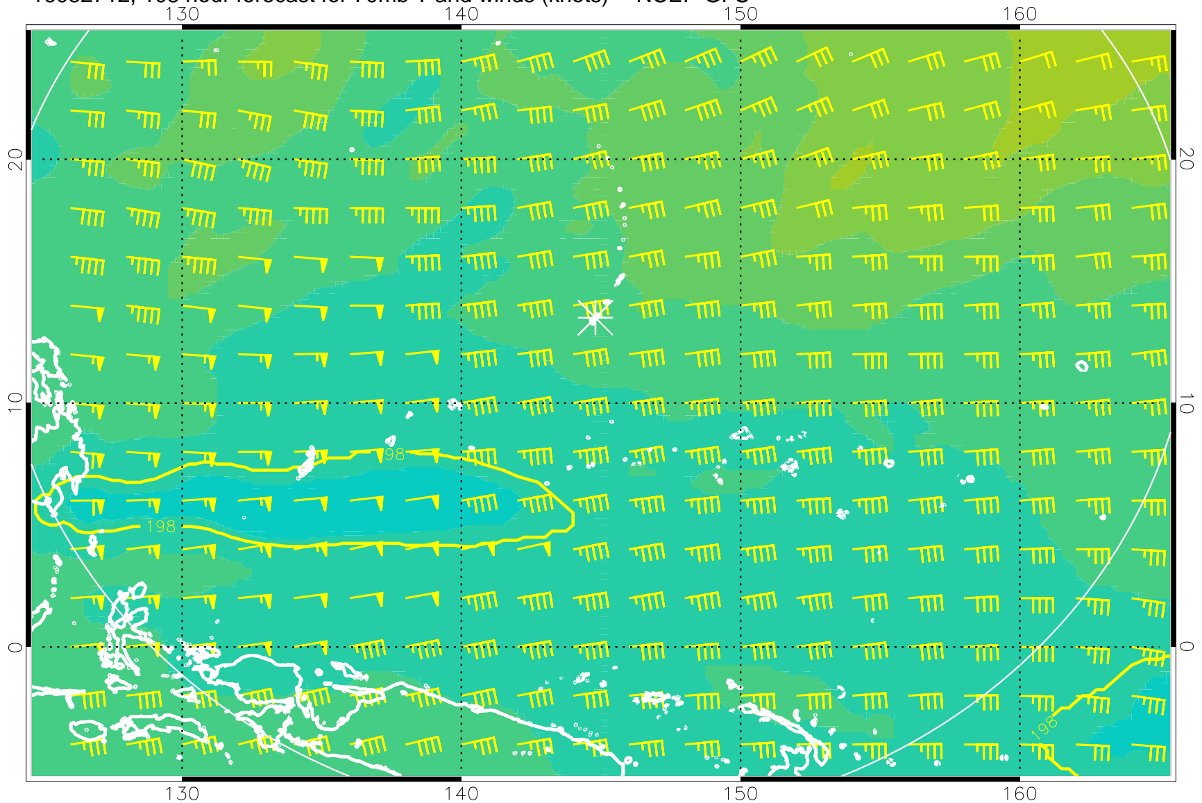
16082712, 108 hour forecast for 70mb T and winds (knots) -- NCEP GFS
