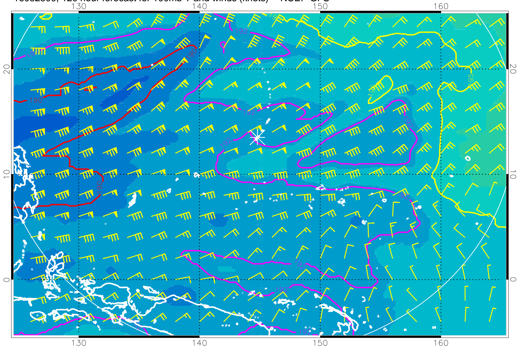
16082800, 120 hour forecast for 100mb T and winds (knots) -- NCEP GFS
