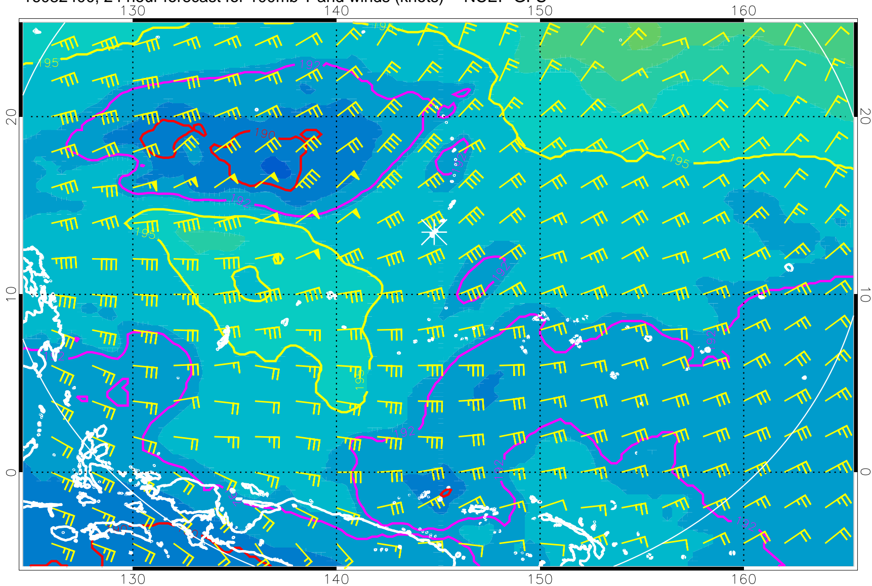
16082400, 24 hour forecast for 100mb T and winds (knots) -- NCEP GFS
