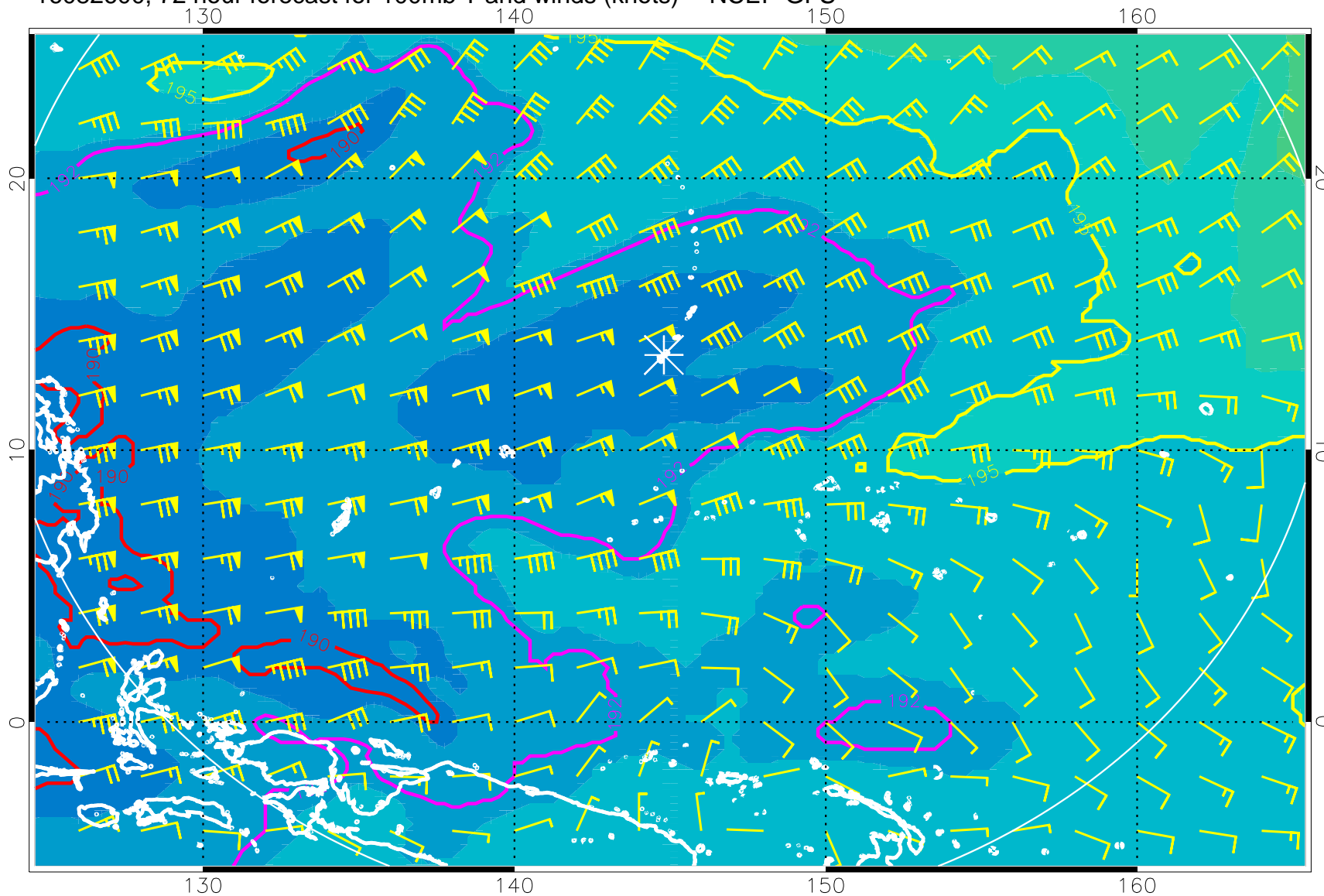
16082600, 72 hour forecast for 100mb T and winds (knots) -- NCEP GFS
