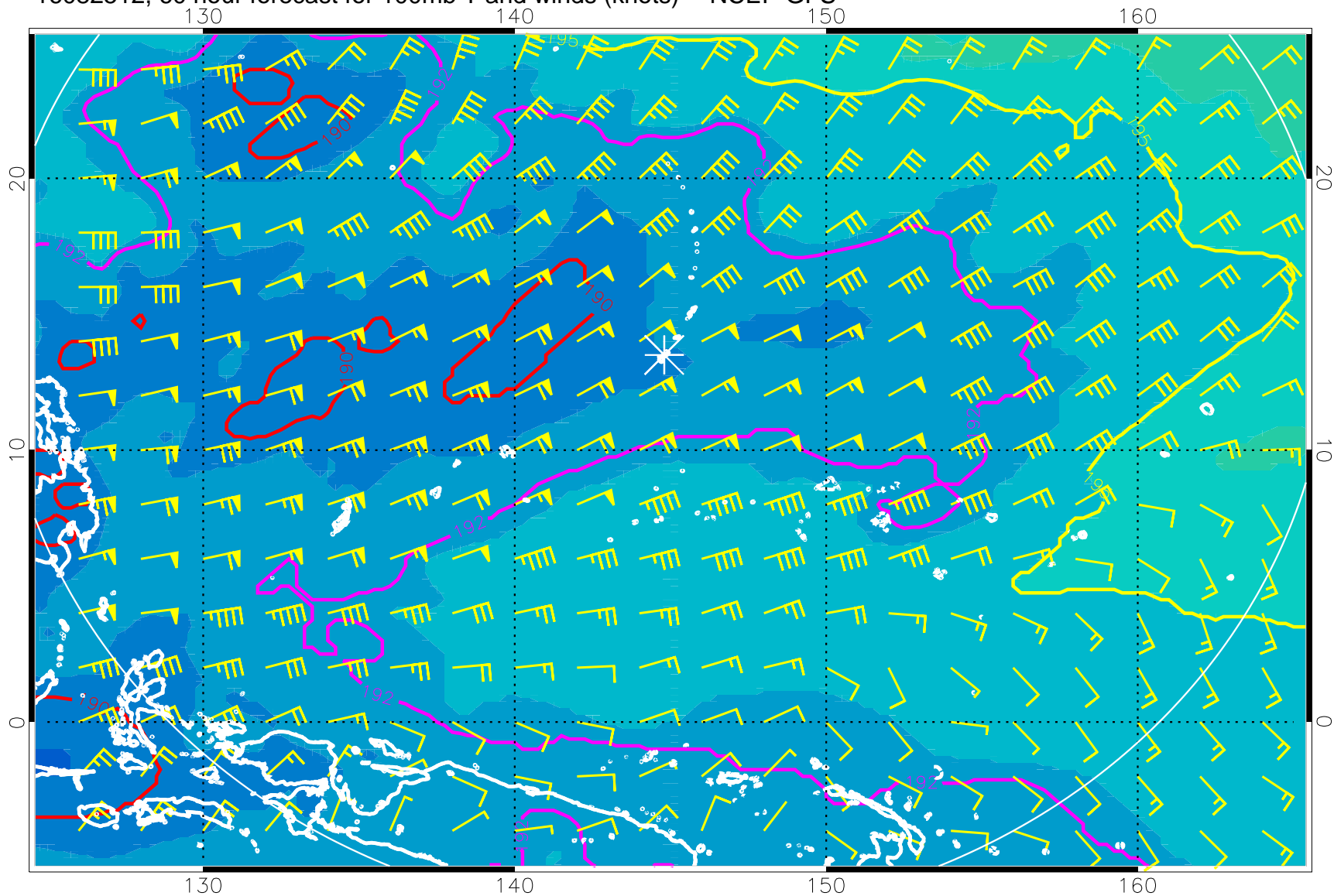
16082512, 60 hour forecast for 100mb T and winds (knots) -- NCEP GFS
