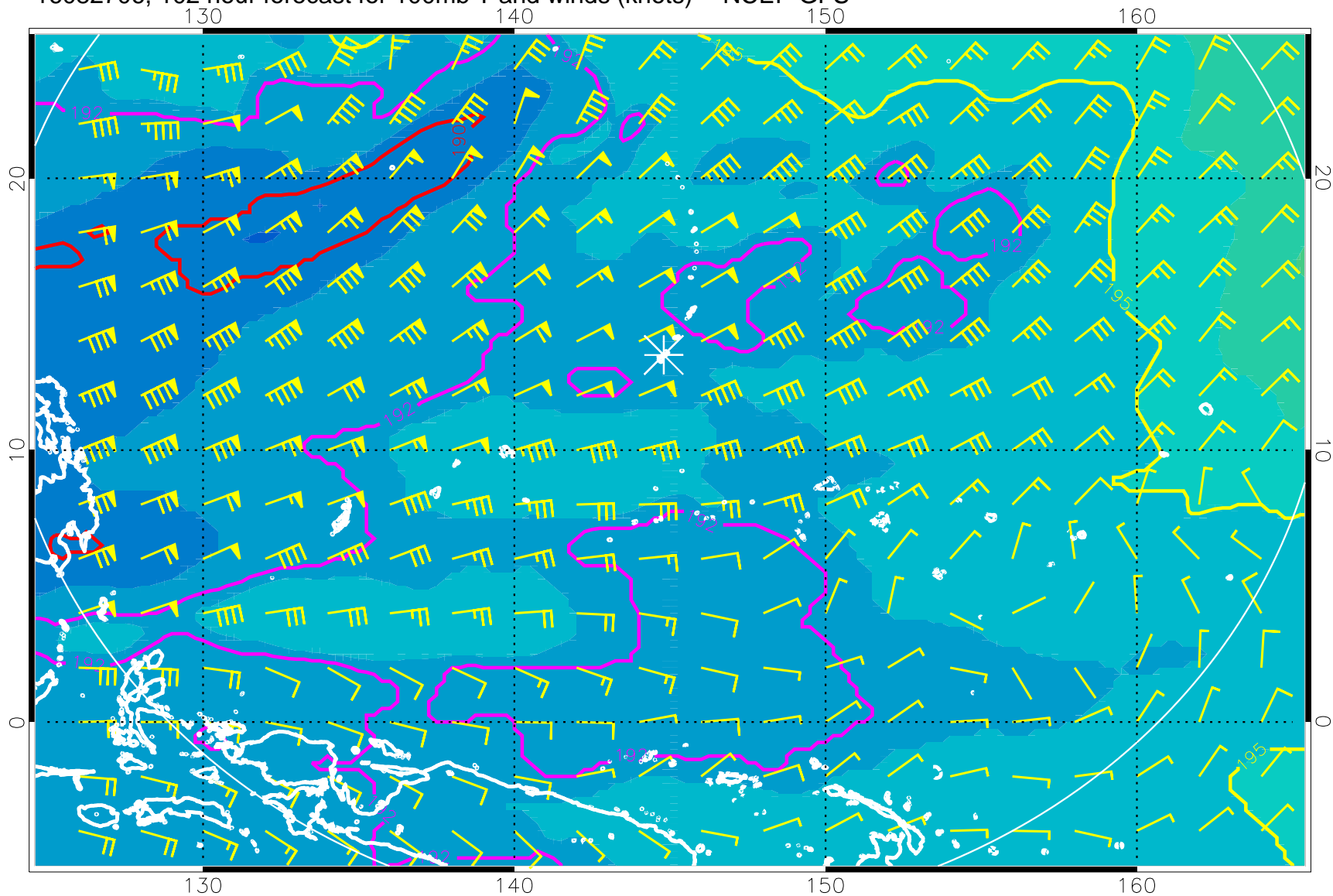
16082706, 102 hour forecast for 100mb T and winds (knots) -- NCEP GFS
