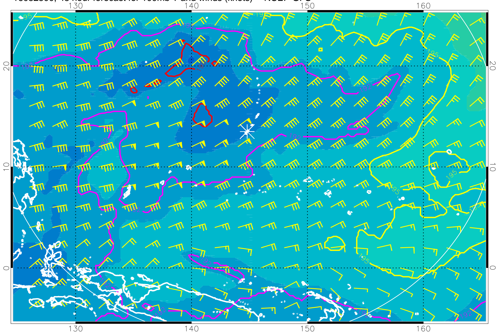
16082500, 48 hour forecast for 100mb T and winds (knots) -- NCEP GFS
