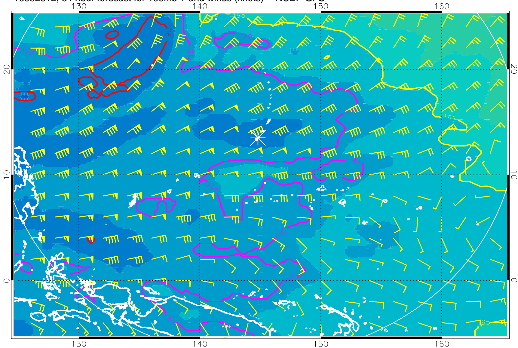
16082612, 84 hour forecast for 100mb T and winds (knots) -- NCEP GFS
