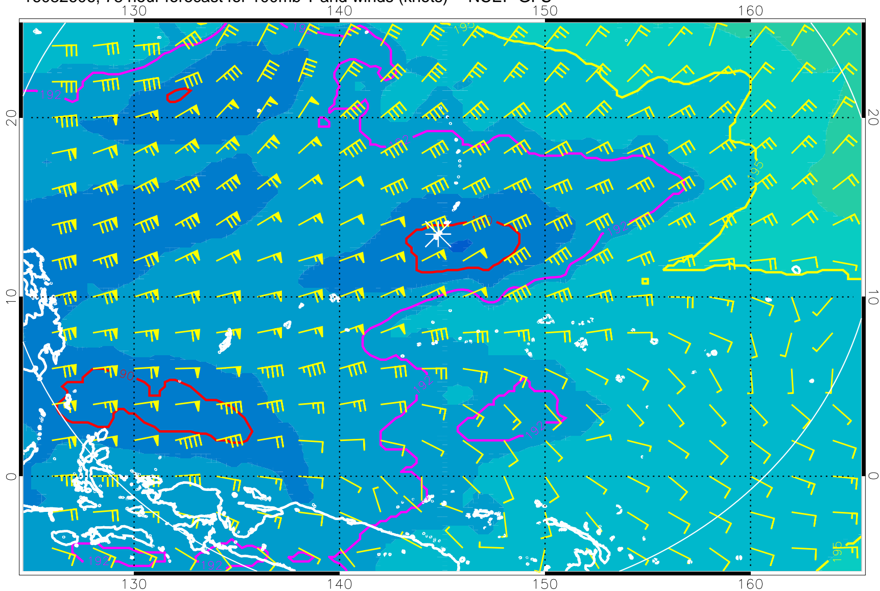
16082606, 78 hour forecast for 100mb T and winds (knots) -- NCEP GFS
