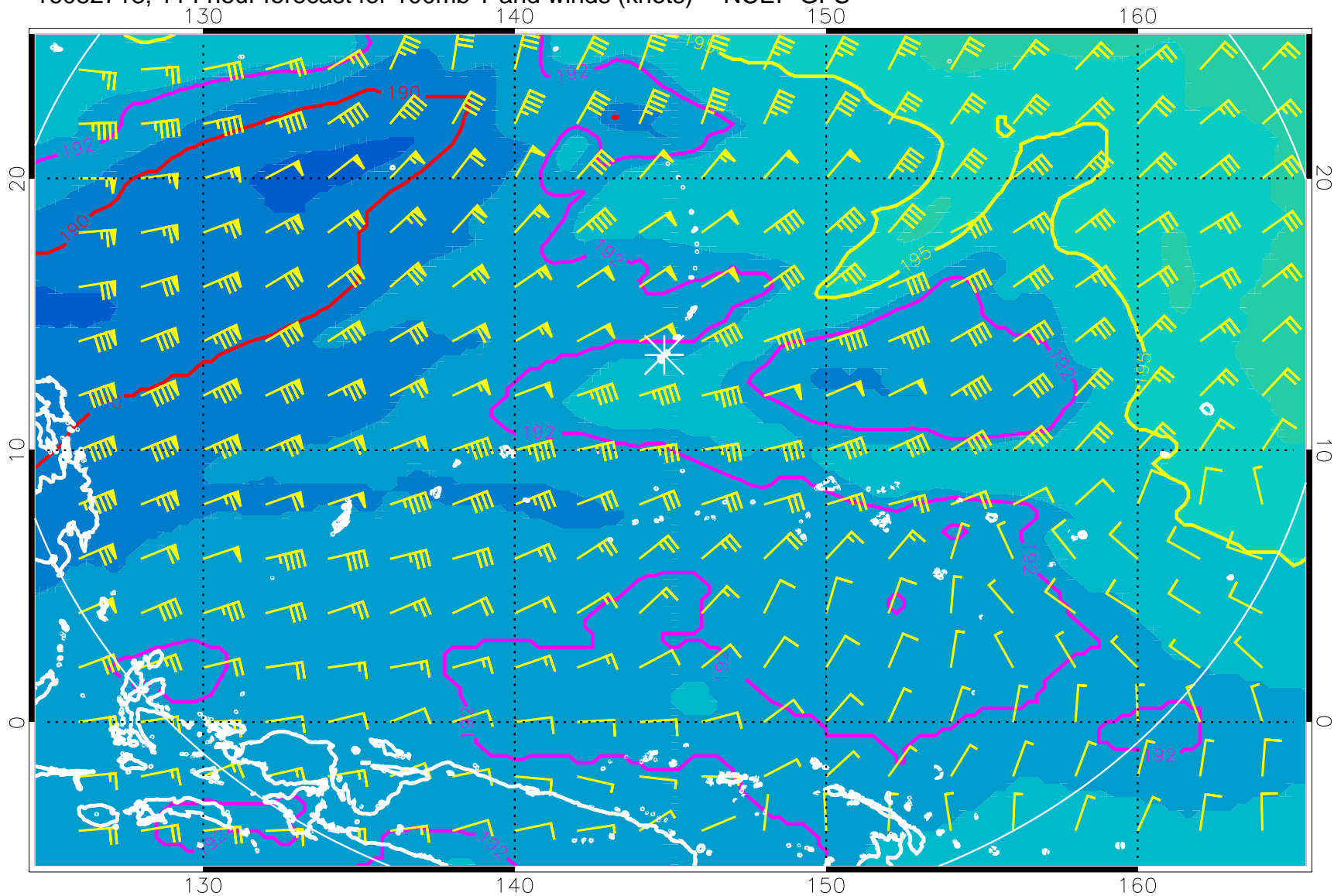
16082718, 114 hour forecast for 100mb T and winds (knots) -- NCEP GFS
