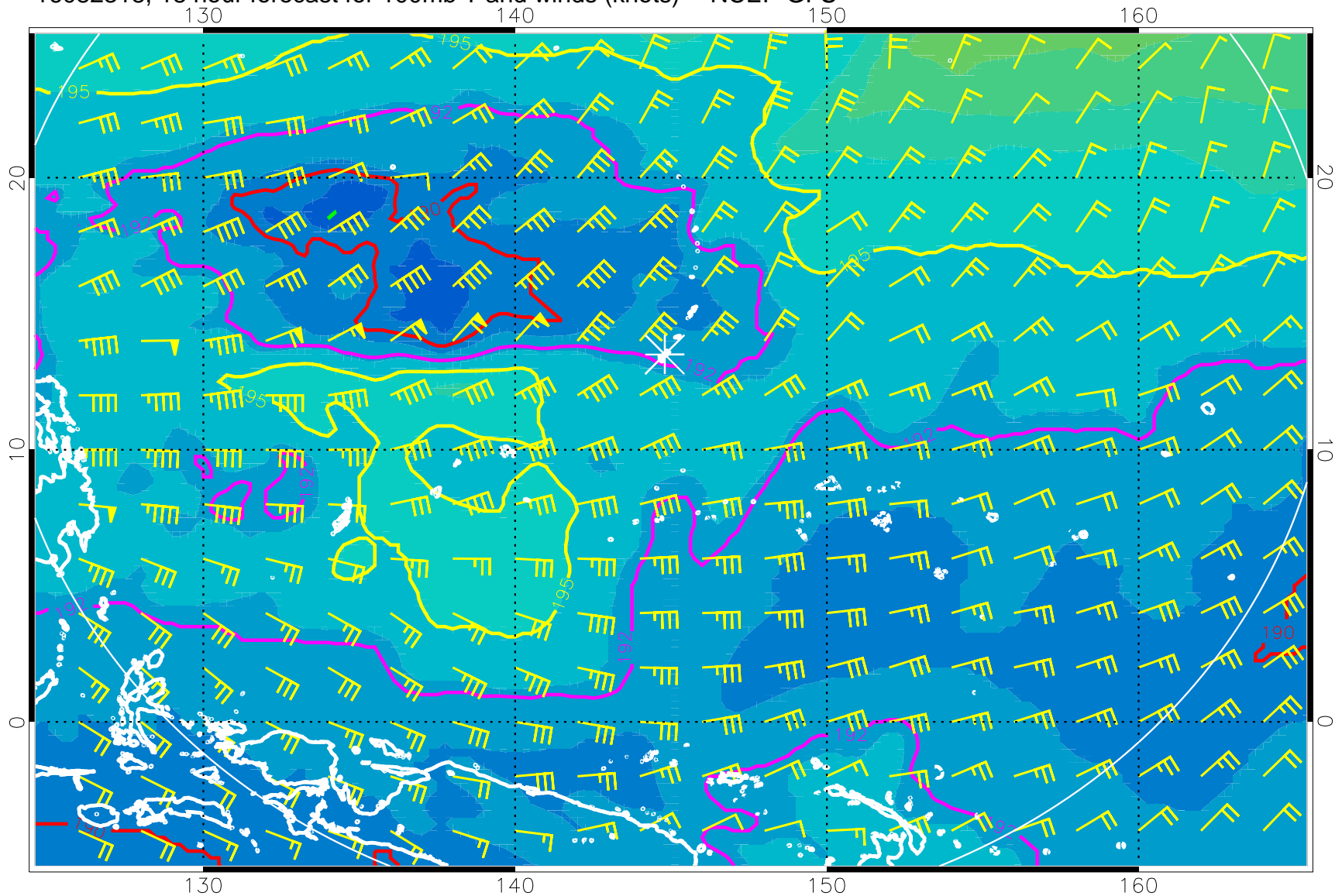
16082318, 18 hour forecast for 100mb T and winds (knots) -- NCEP GFS
