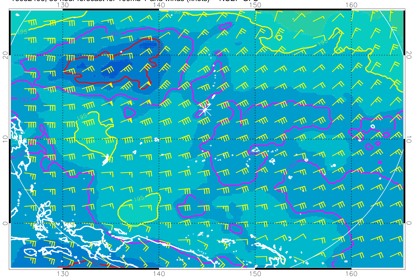
16082406, 30 hour forecast for 100mb T and winds (knots) -- NCEP GFS
