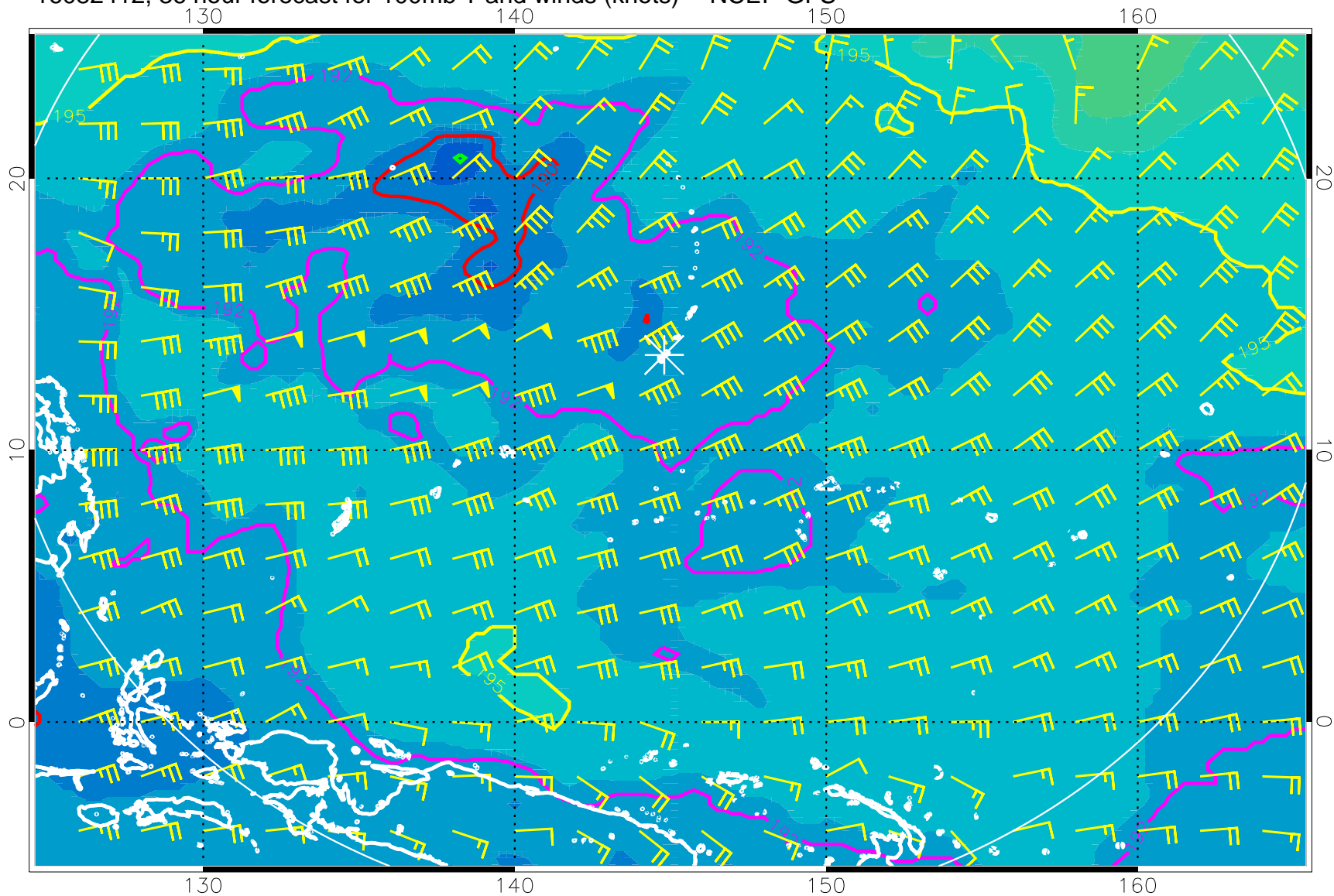
16082412, 36 hour forecast for 100mb T and winds (knots) -- NCEP GFS
