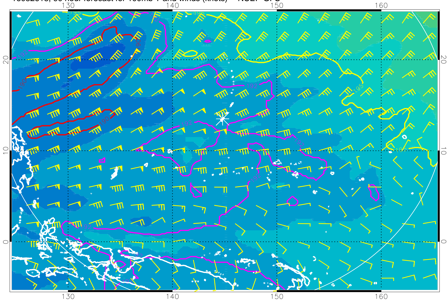
16082618, 90 hour forecast for 100mb T and winds (knots) -- NCEP GFS
