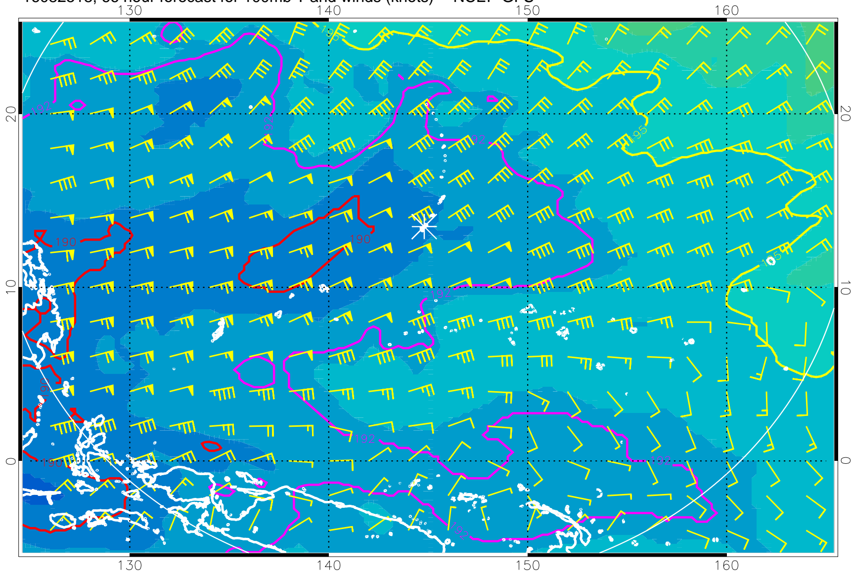
16082518, 66 hour forecast for 100mb T and winds (knots) -- NCEP GFS
