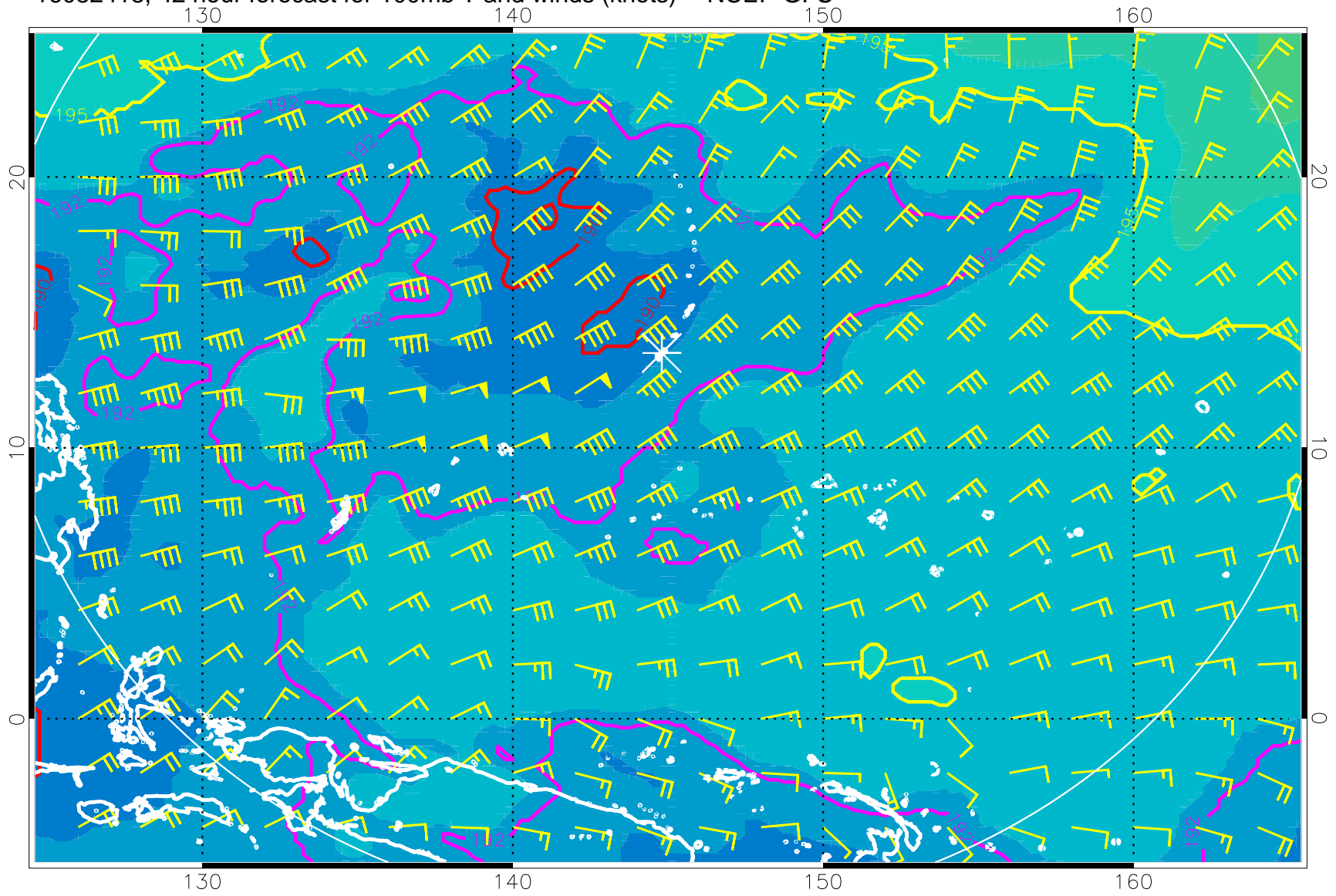
16082418, 42 hour forecast for 100mb T and winds (knots) -- NCEP GFS
