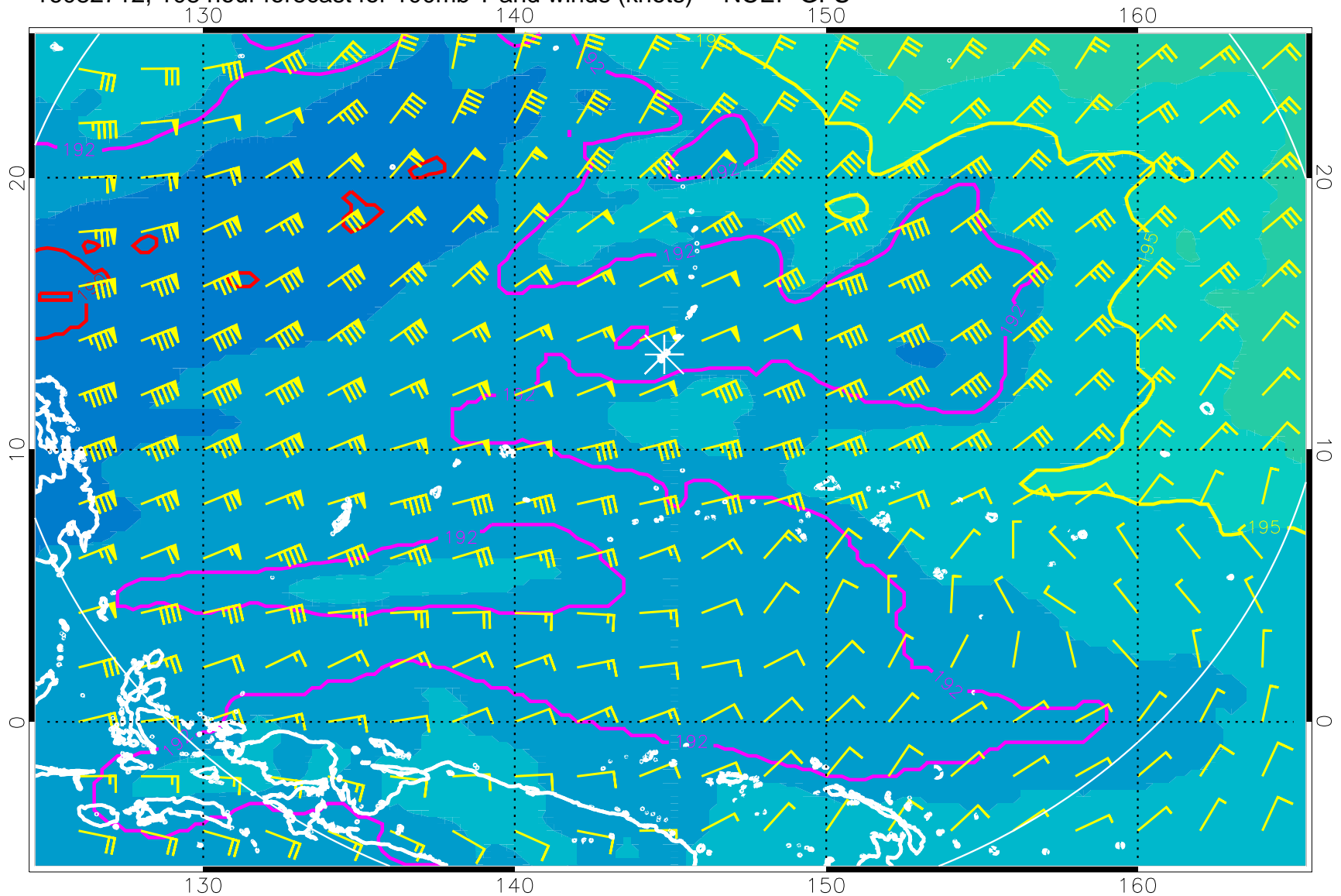
16082712, 108 hour forecast for 100mb T and winds (knots) -- NCEP GFS
