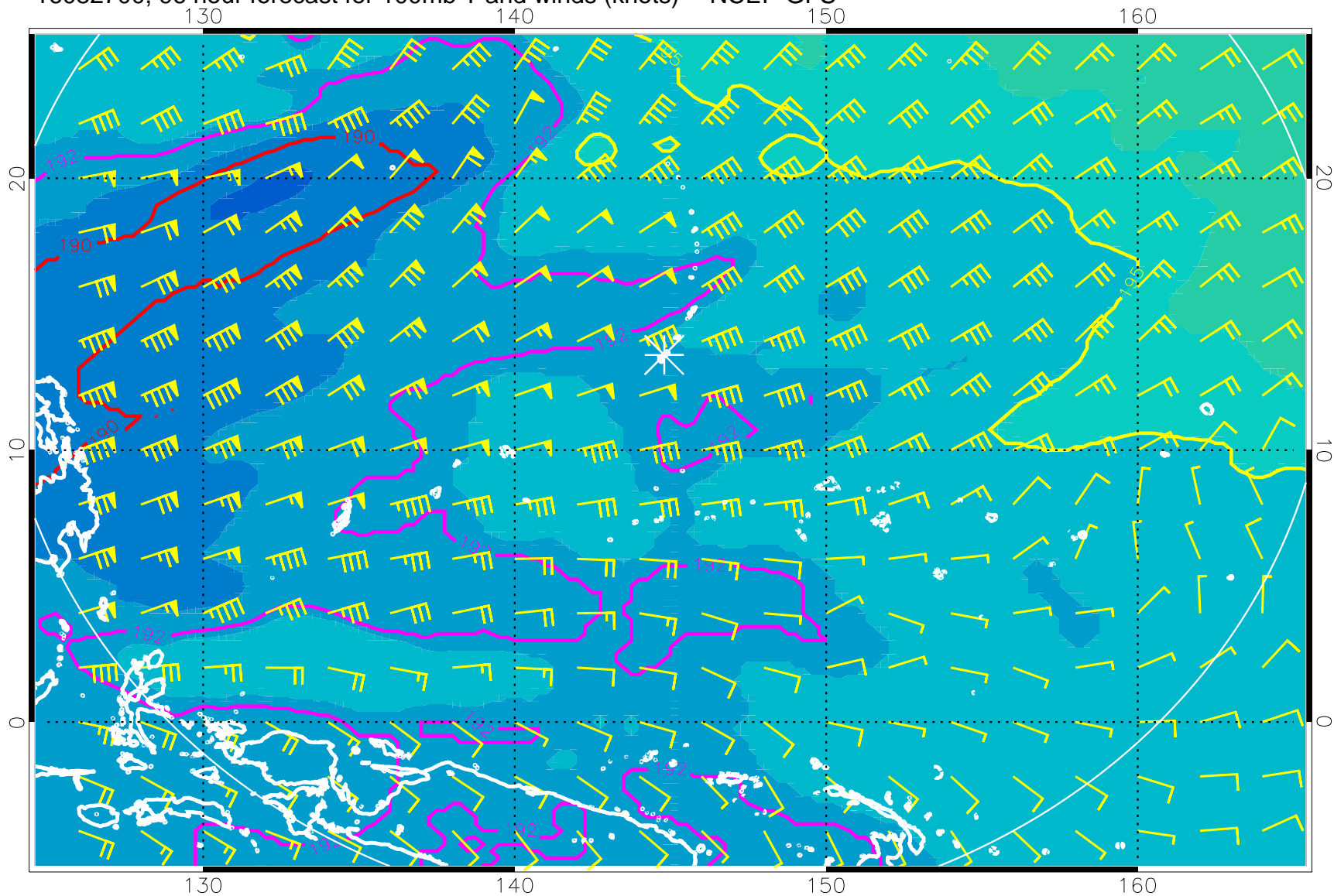
16082700, 96 hour forecast for 100mb T and winds (knots) -- NCEP GFS
