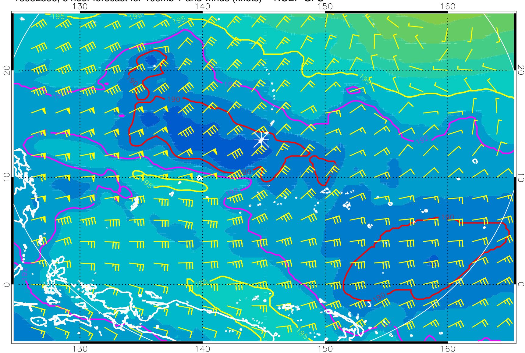
16082306, 6 hour forecast for 100mb T and winds (knots) -- NCEP GFS
