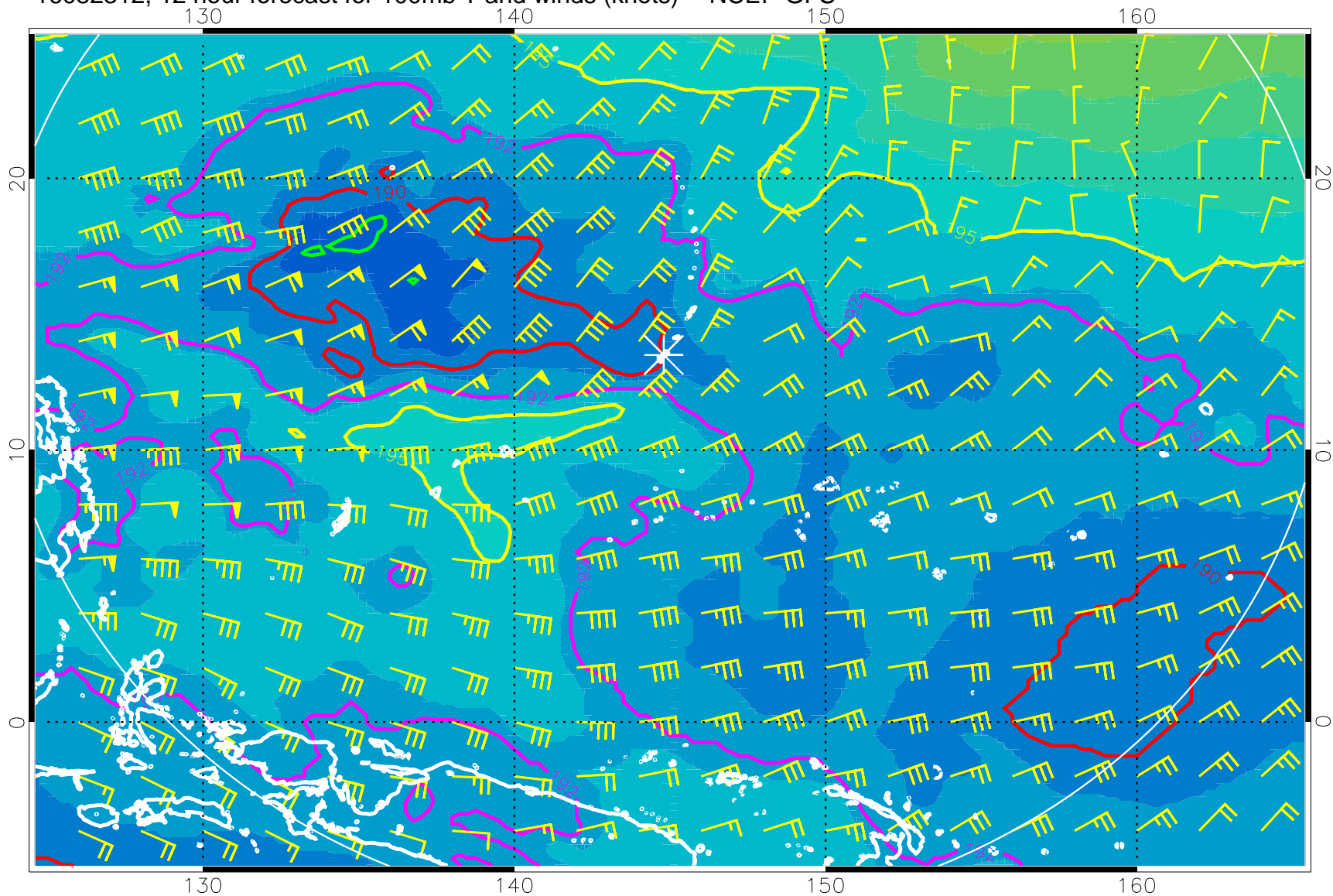
16082312, 12 hour forecast for 100mb T and winds (knots) -- NCEP GFS
