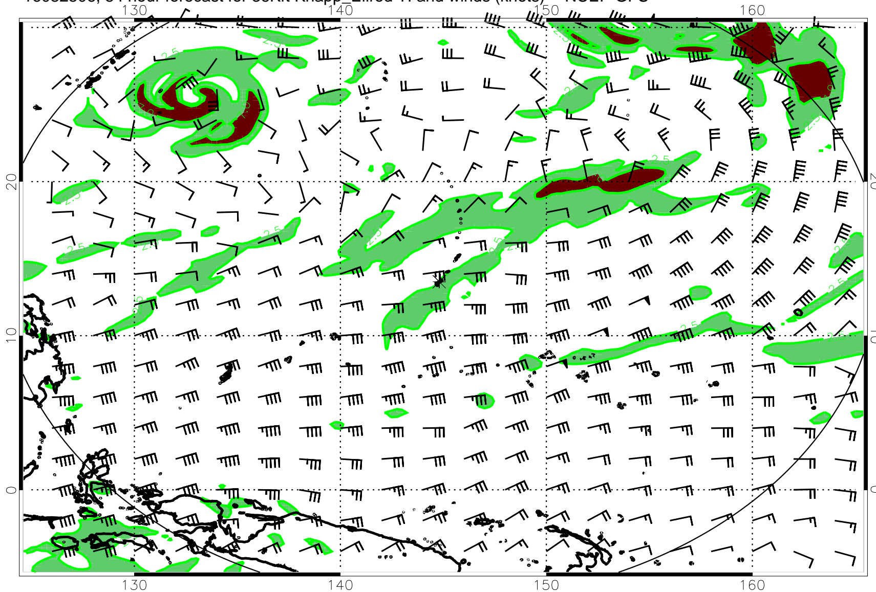
16082506, 54 hour forecast for 36Kft Knapp_Ellrod TI and winds (knots) -- NCEP GFS
