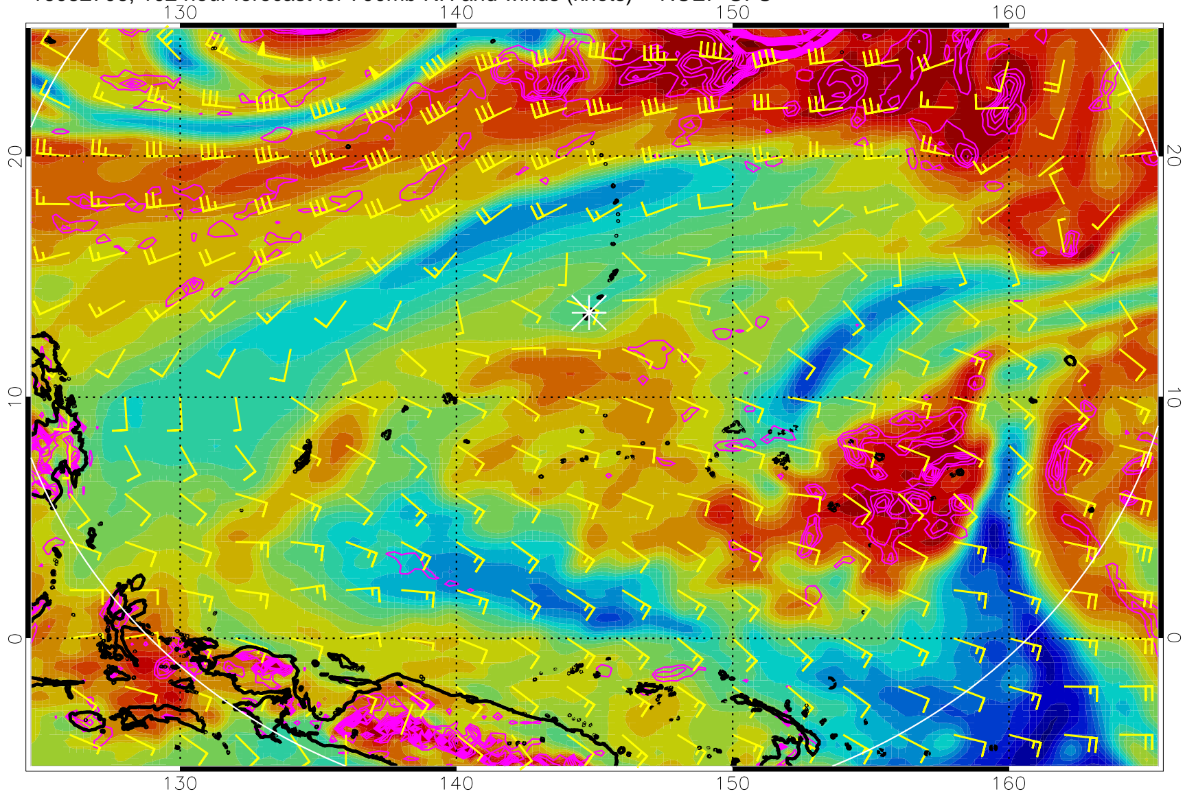
16082706, 102 hour forecast for 700mb RH and winds (knots) -- NCEP GFS
