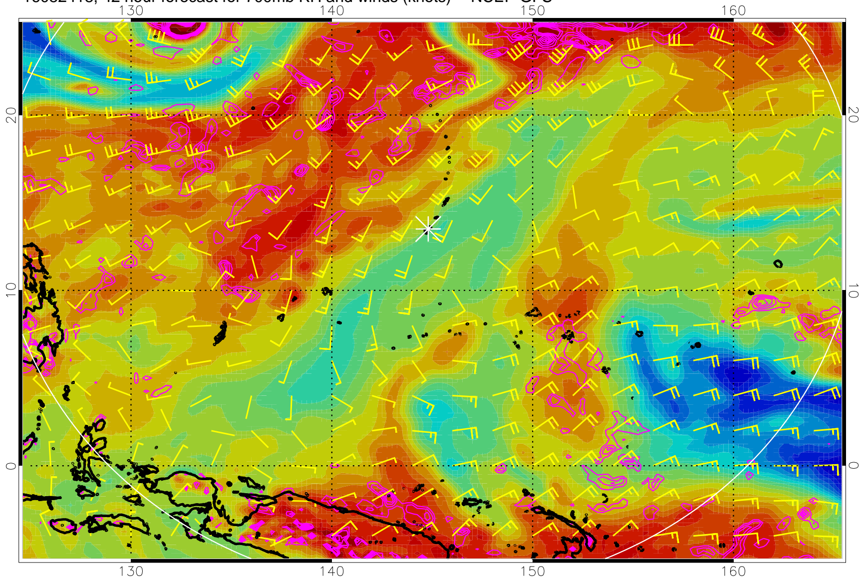
16082418, 42 hour forecast for 700mb RH and winds (knots) -- NCEP GFS
