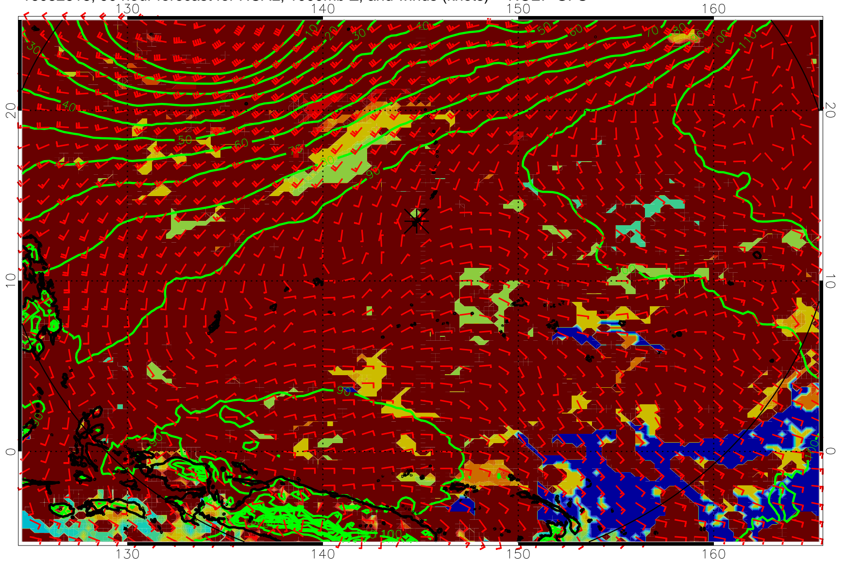
16082618, 90 hour forecast for HCAL, 1000mb Z, and winds (knots) -- NCEP GFS
