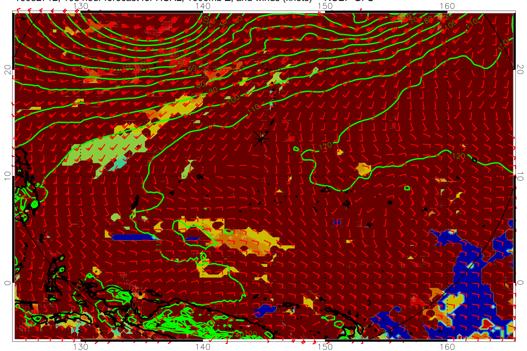
16082712, 108 hour forecast for HCAL, 1000mb Z, and winds (knots) -- NCEP GFS
