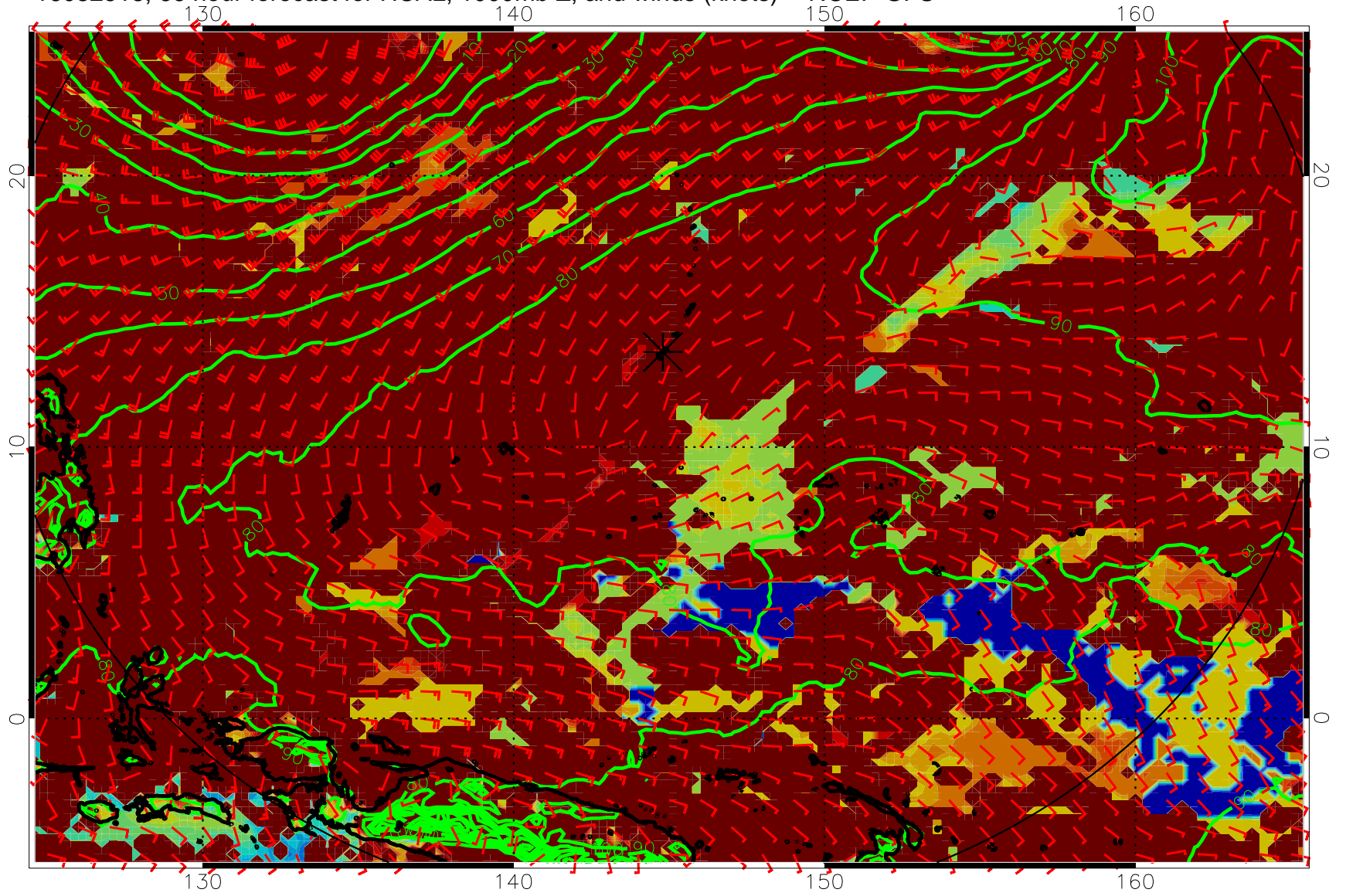
16082518, 66 hour forecast for HCAL, 1000mb Z, and winds (knots) -- NCEP GFS
