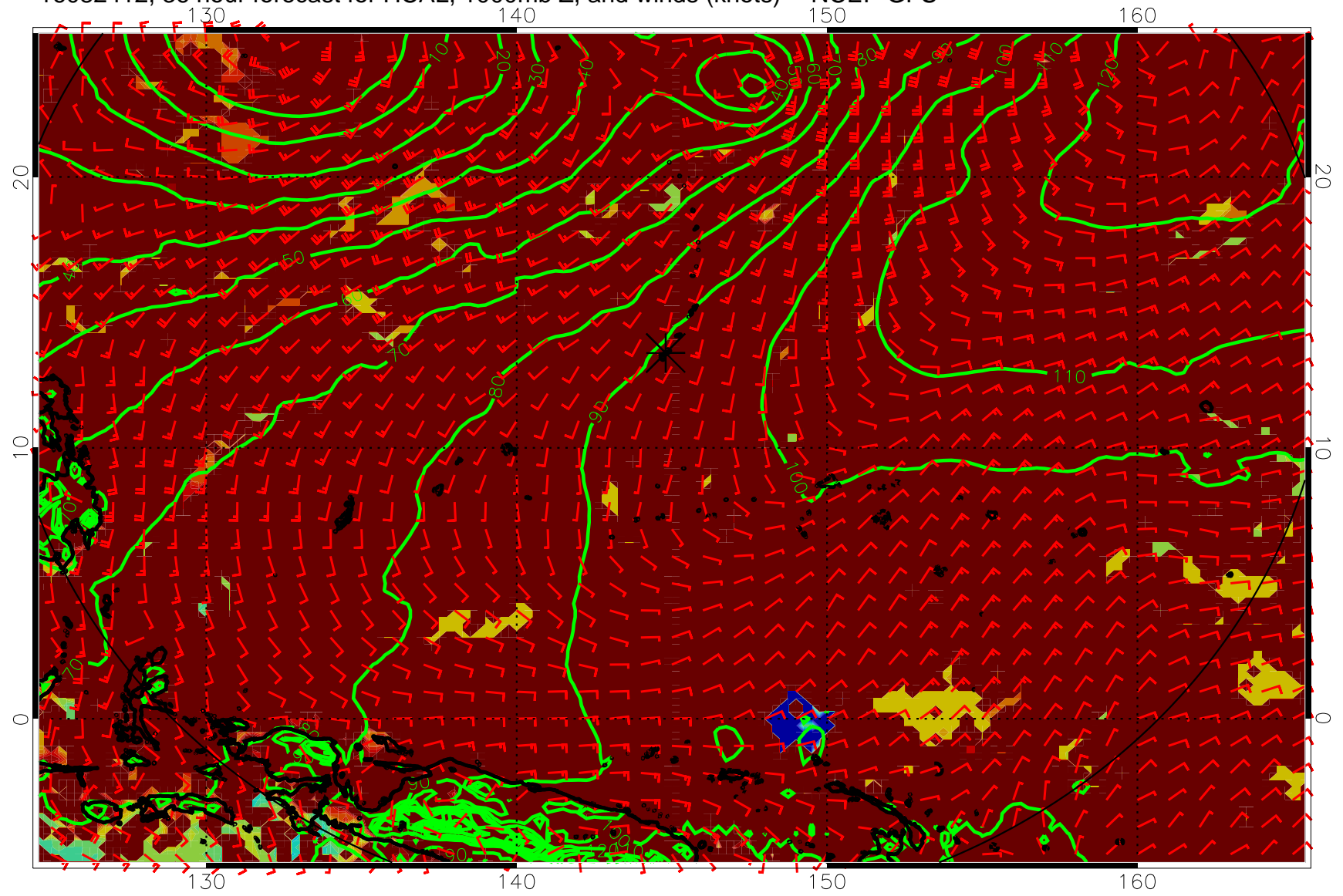
16082412, 36 hour forecast for HCAL, 1000mb Z, and winds (knots) -- NCEP GFS
