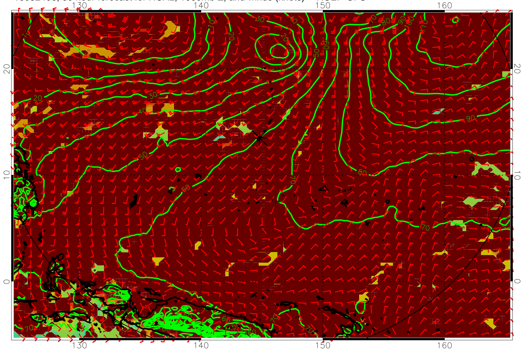
16082406, 30 hour forecast for HCAL, 1000mb Z, and winds (knots) -- NCEP GFS
