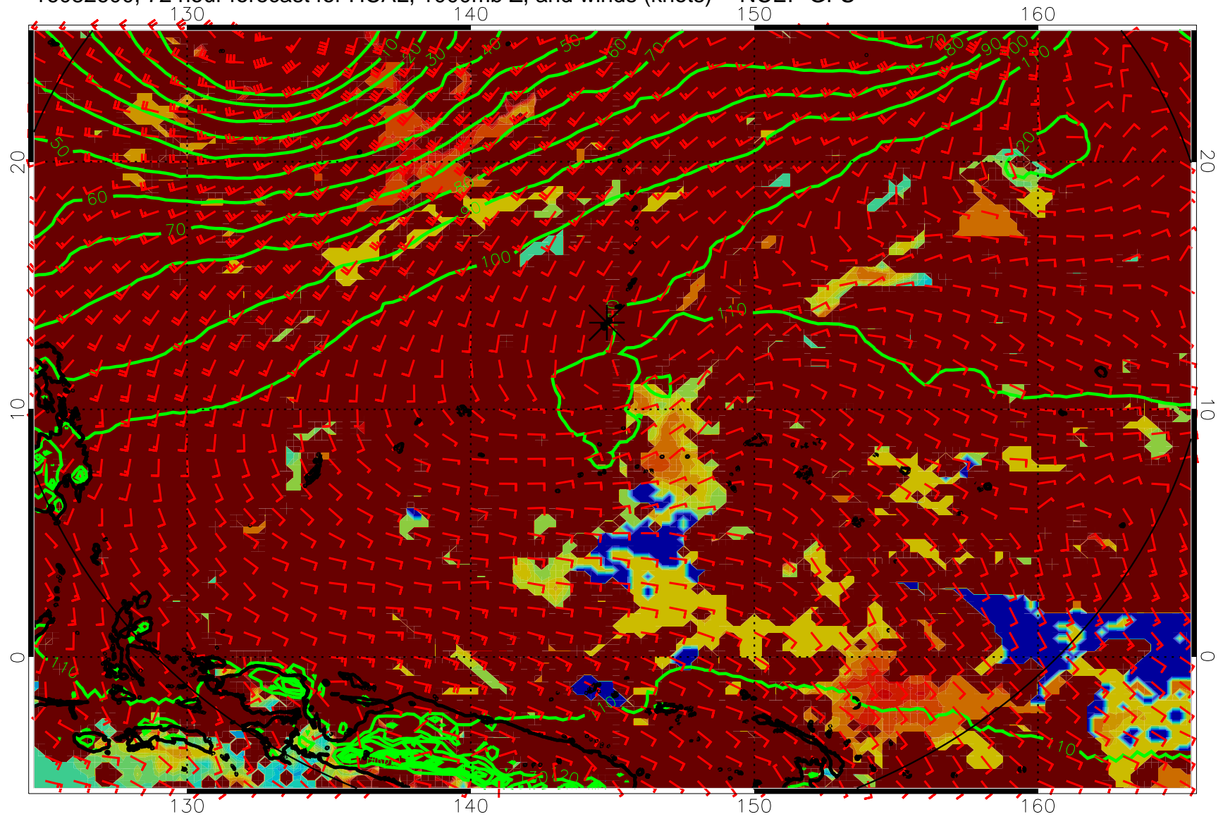
16082600, 72 hour forecast for HCAL, 1000mb Z, and winds (knots) -- NCEP GFS
