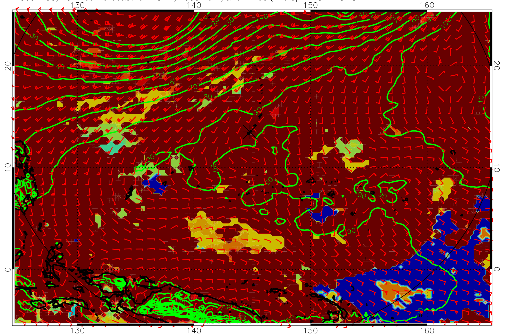
16082706, 102 hour forecast for HCAL, 1000mb Z, and winds (knots) -- NCEP GFS
