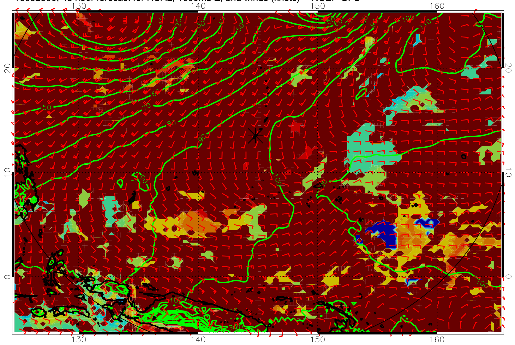
16082500, 48 hour forecast for HCAL, 1000mb Z, and winds (knots) -- NCEP GFS
