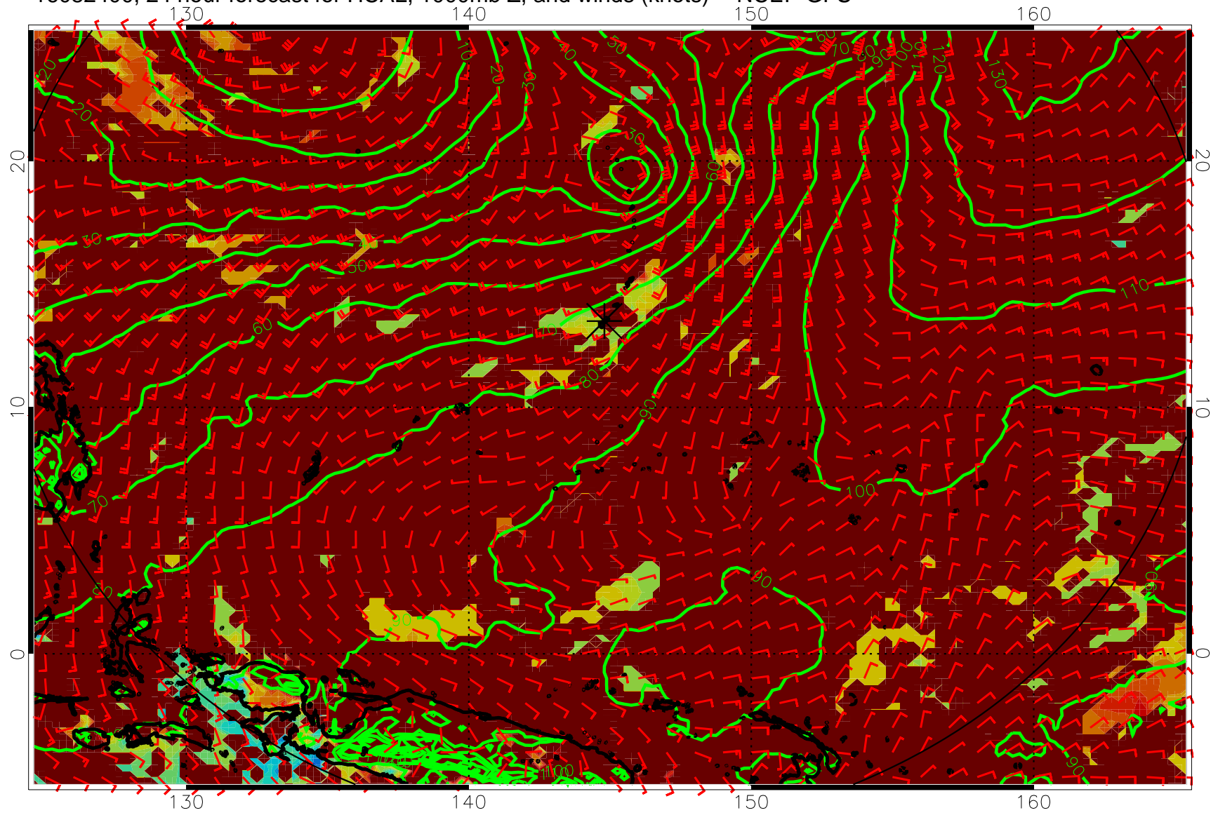
16082400, 24 hour forecast for HCAL, 1000mb Z, and winds (knots) -- NCEP GFS
