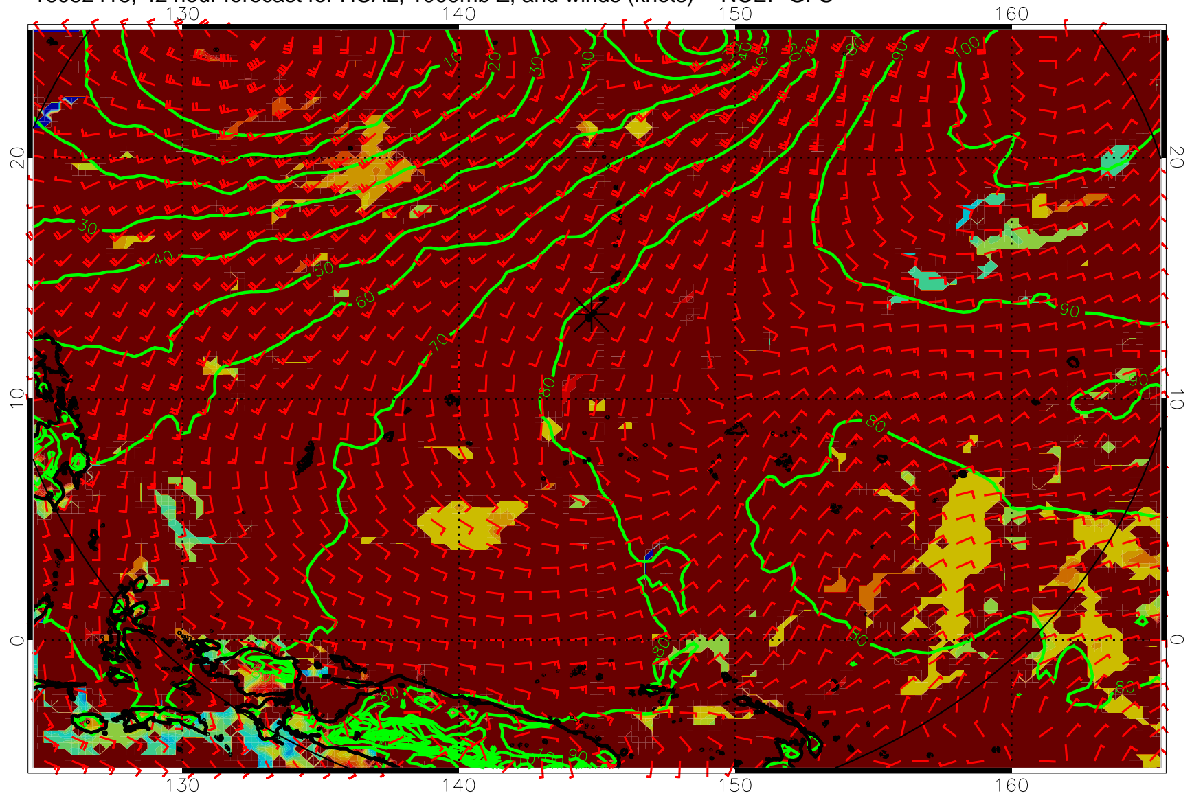
16082418, 42 hour forecast for HCAL, 1000mb Z, and winds (knots) -- NCEP GFS
