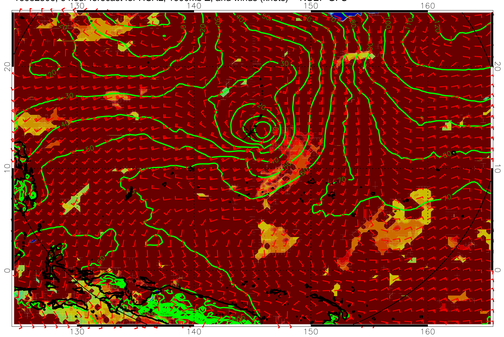
16082306, 6 hour forecast for HCAL, 1000mb Z, and winds (knots) -- NCEP GFS
