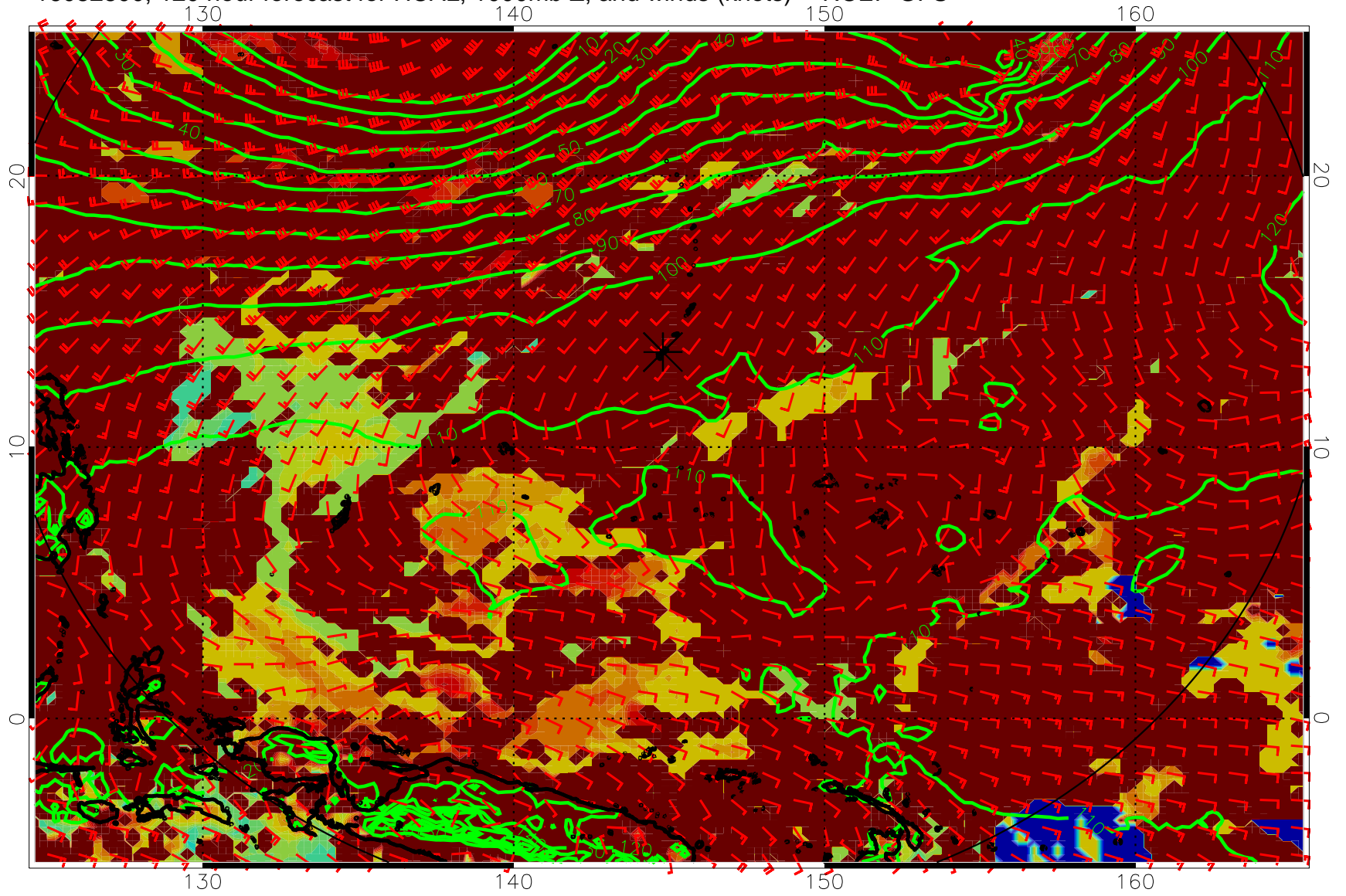
16082800, 120 hour forecast for HCAL, 1000mb Z, and winds (knots) -- NCEP GFS
