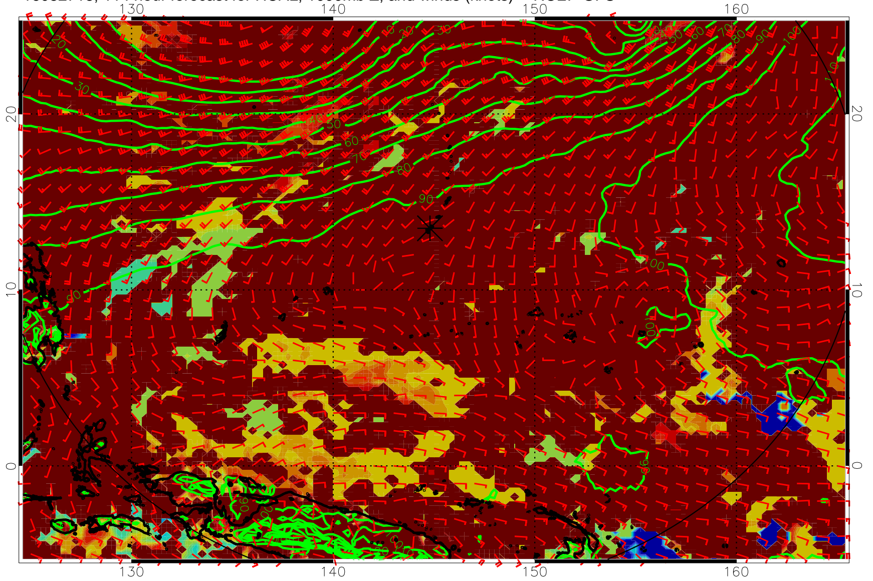
16082718, 114 hour forecast for HCAL, 1000mb Z, and winds (knots) -- NCEP GFS
