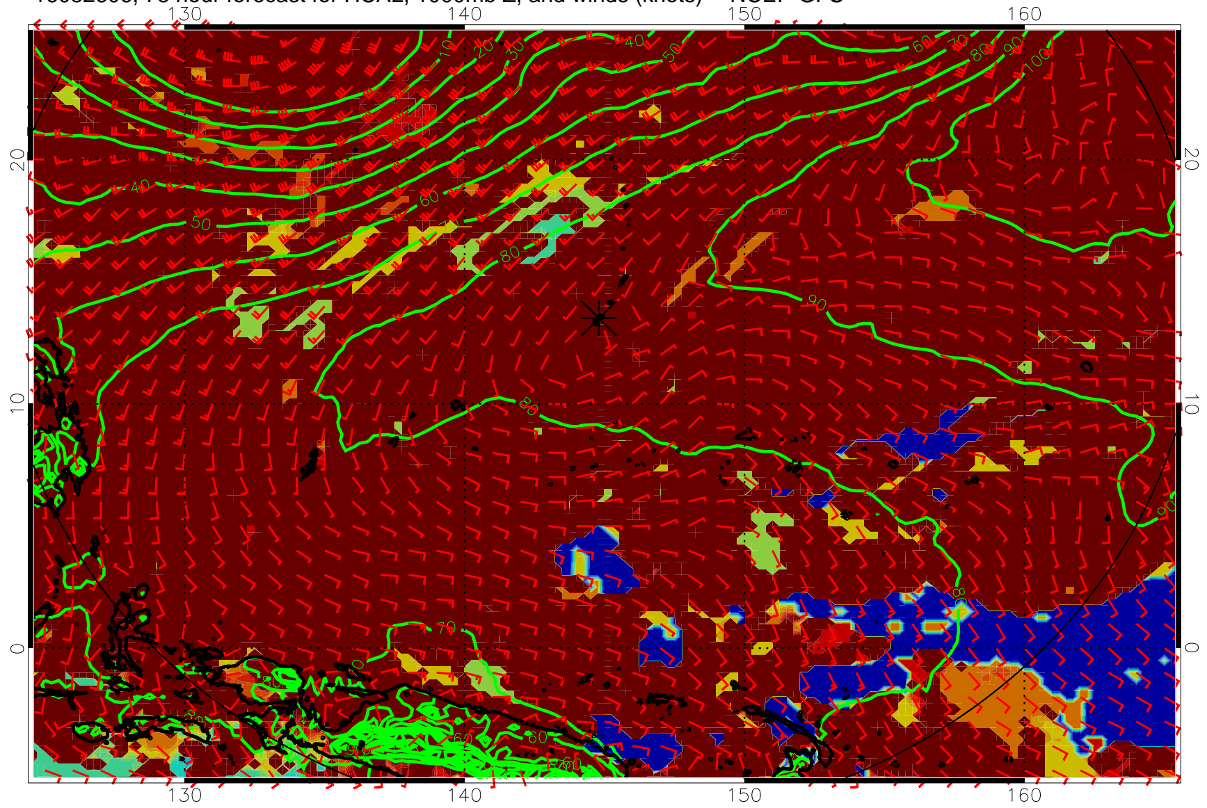
16082606, 78 hour forecast for HCAL, 1000mb Z, and winds (knots) -- NCEP GFS
