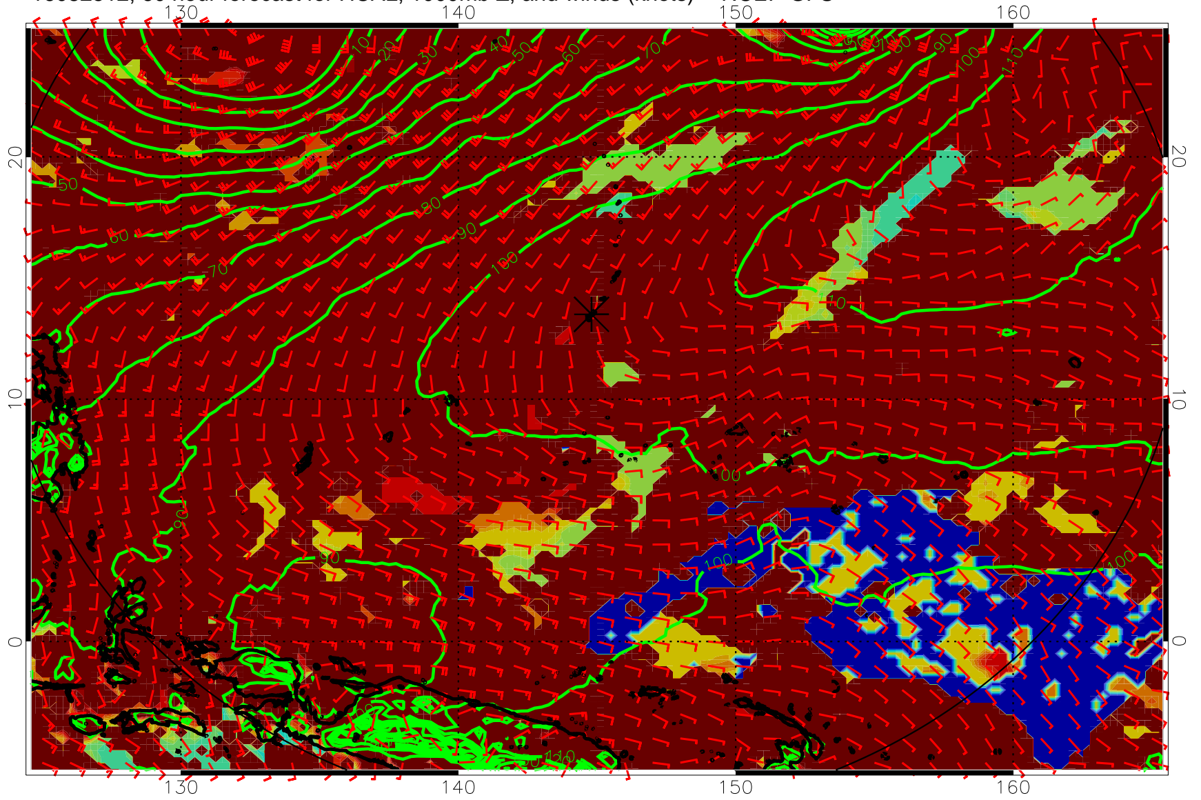
16082512, 60 hour forecast for HCAL, 1000mb Z, and winds (knots) -- NCEP GFS
