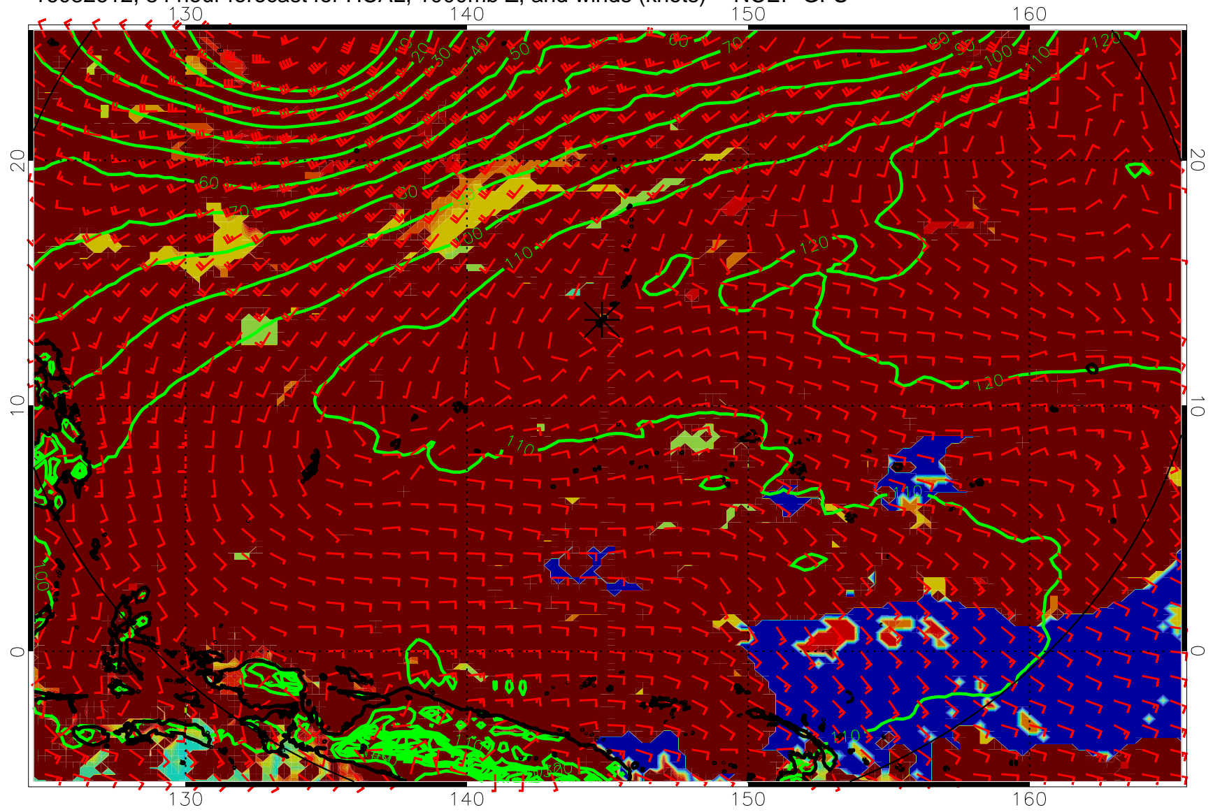
16082612, 84 hour forecast for HCAL, 1000mb Z, and winds (knots) -- NCEP GFS
