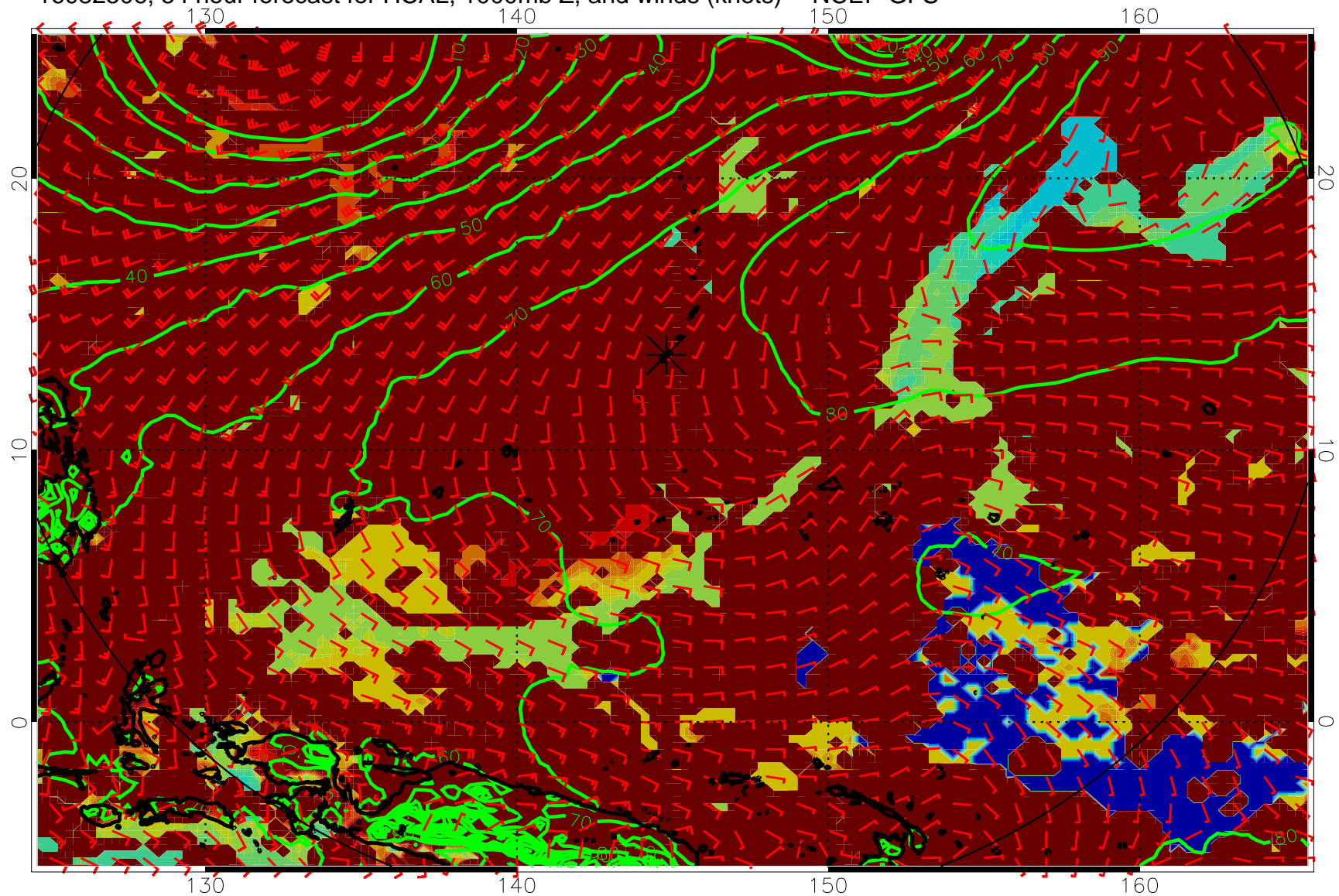
16082506, 54 hour forecast for HCAL, 1000mb Z, and winds (knots) -- NCEP GFS
