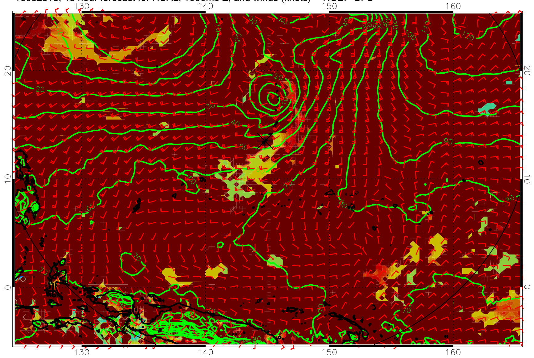
16082318, 18 hour forecast for HCAL, 1000mb Z, and winds (knots) -- NCEP GFS
