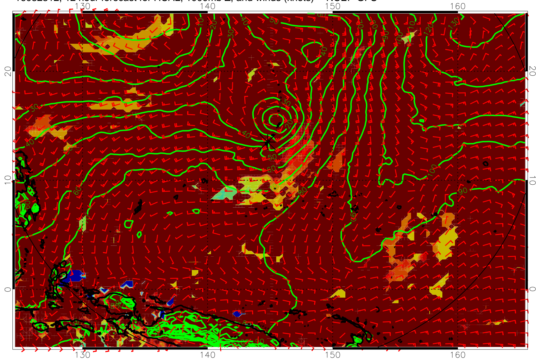
16082312, 12 hour forecast for HCAL, 1000mb Z, and winds (knots) -- NCEP GFS
