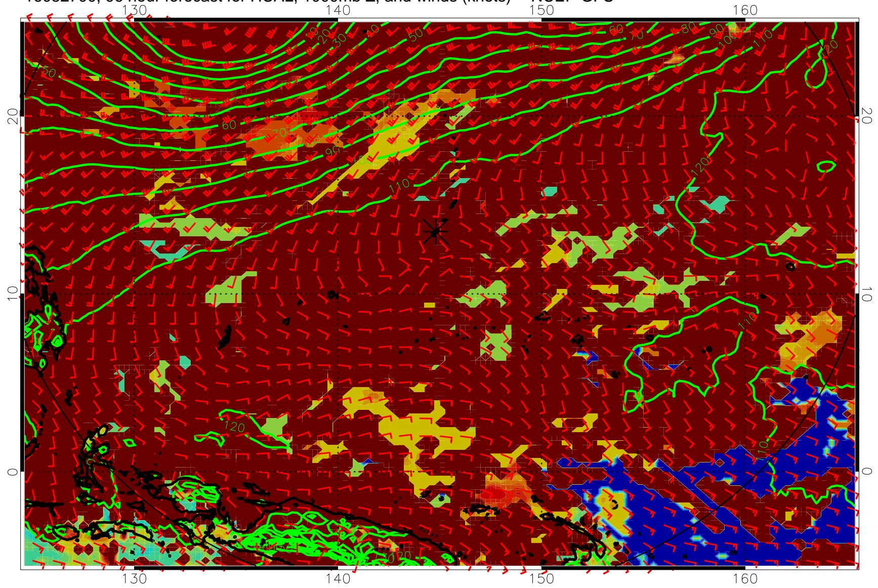
16082700, 96 hour forecast for HCAL, 1000mb Z, and winds (knots) -- NCEP GFS
