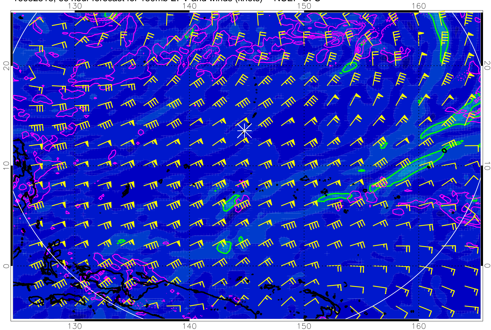
16082518, 66 hour forecast for 150mb EPV and winds (knots) -- NCEP GFS
