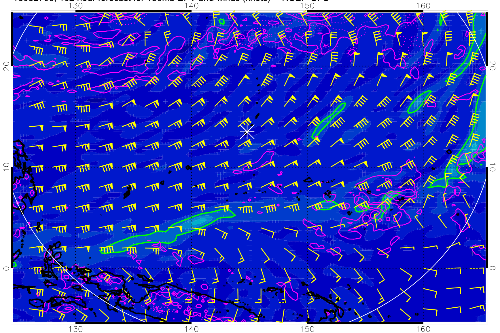
16082706, 102 hour forecast for 150mb EPV and winds (knots) -- NCEP GFS
