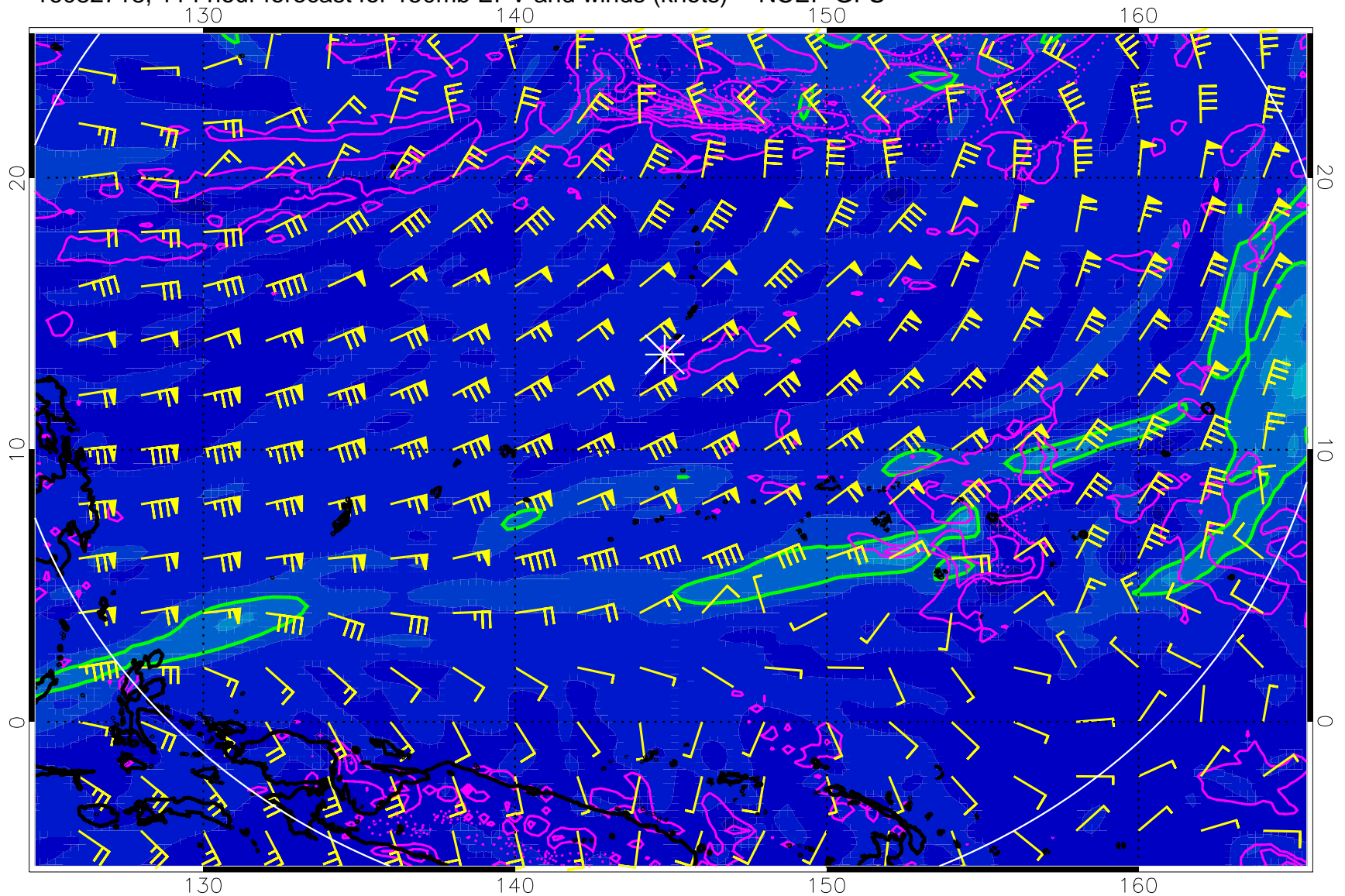
16082718, 114 hour forecast for 150mb EPV and winds (knots) -- NCEP GFS
