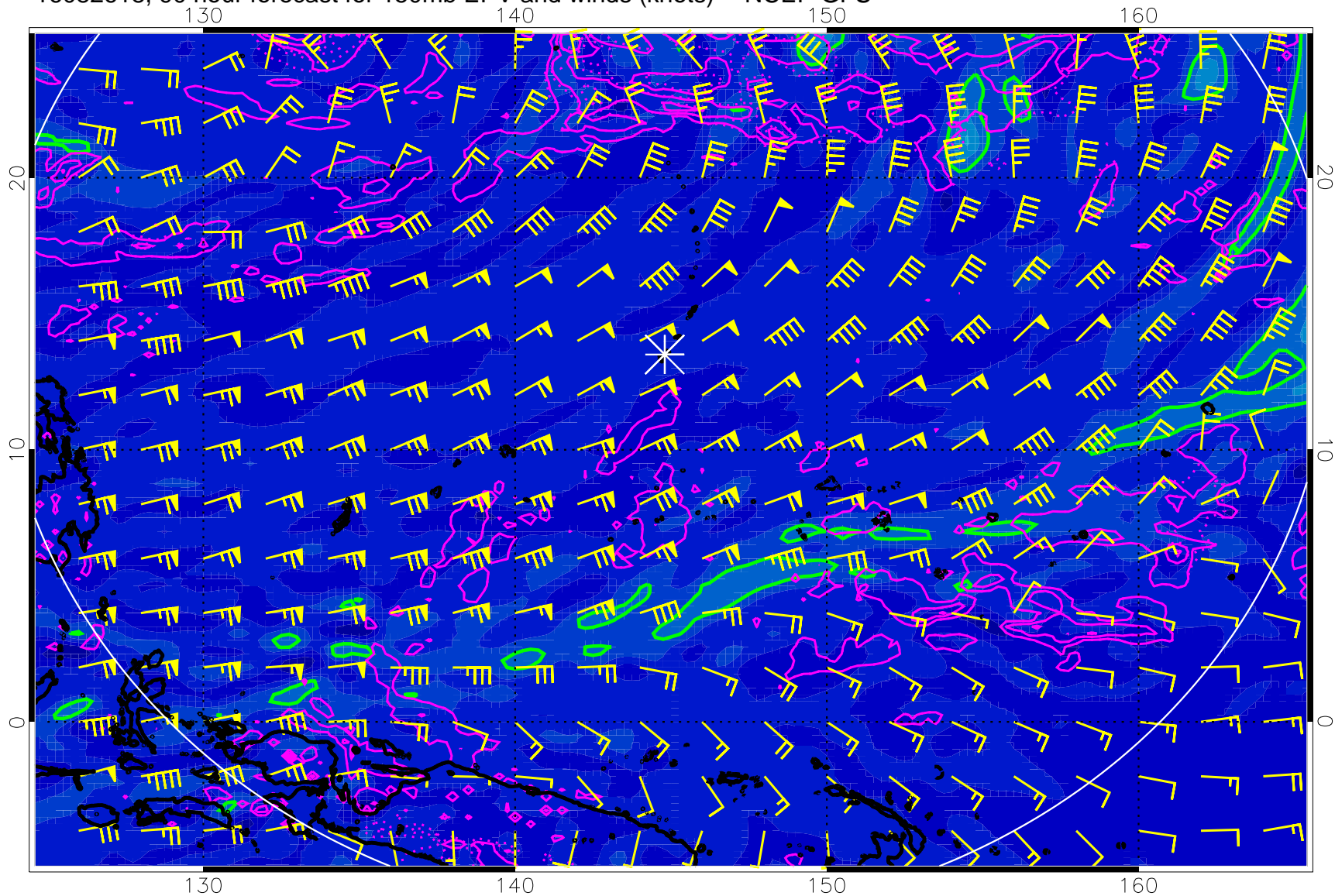
16082618, 90 hour forecast for 150mb EPV and winds (knots) -- NCEP GFS
