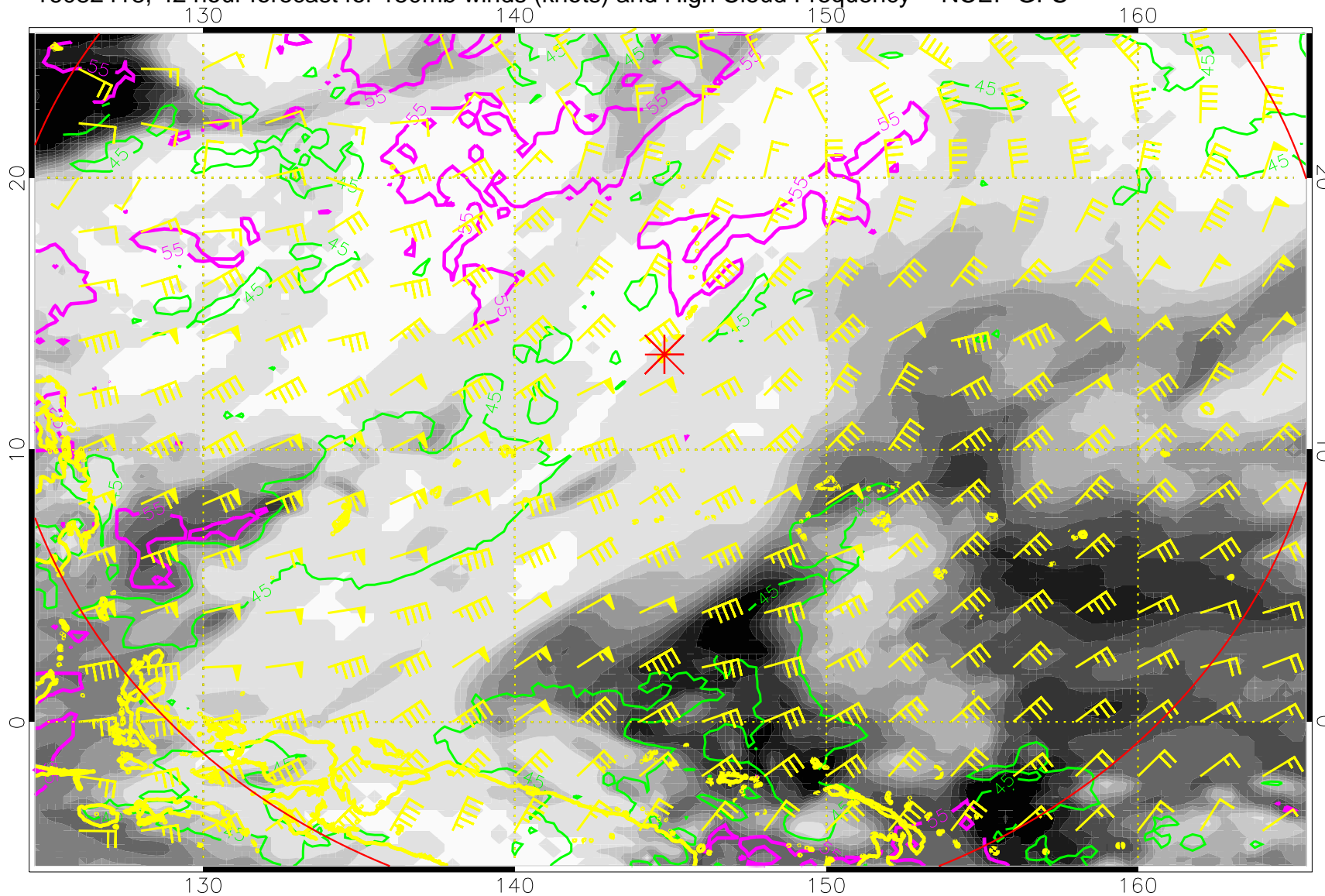
16082418, 42 hour forecast for 150mb winds (knots) and High Cloud Frequency -- NCEP GFS
