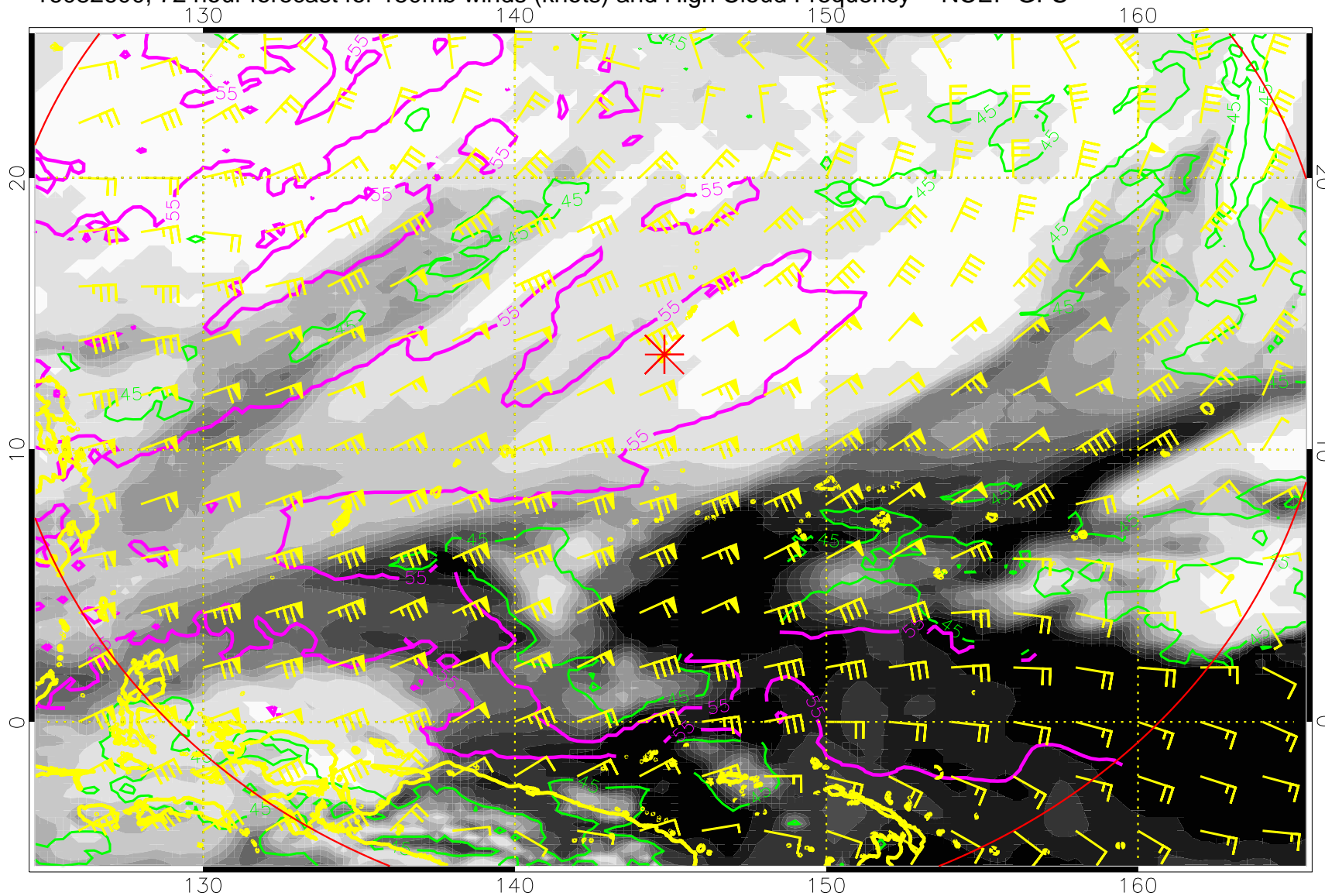
16082600, 72 hour forecast for 150mb winds (knots) and High Cloud Frequency -- NCEP GFS
