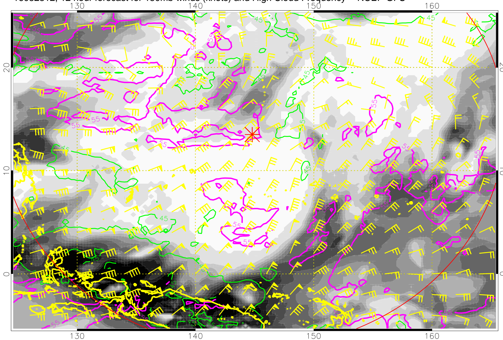
16082312, 12 hour forecast for 150mb winds (knots) and High Cloud Frequency -- NCEP GFS
