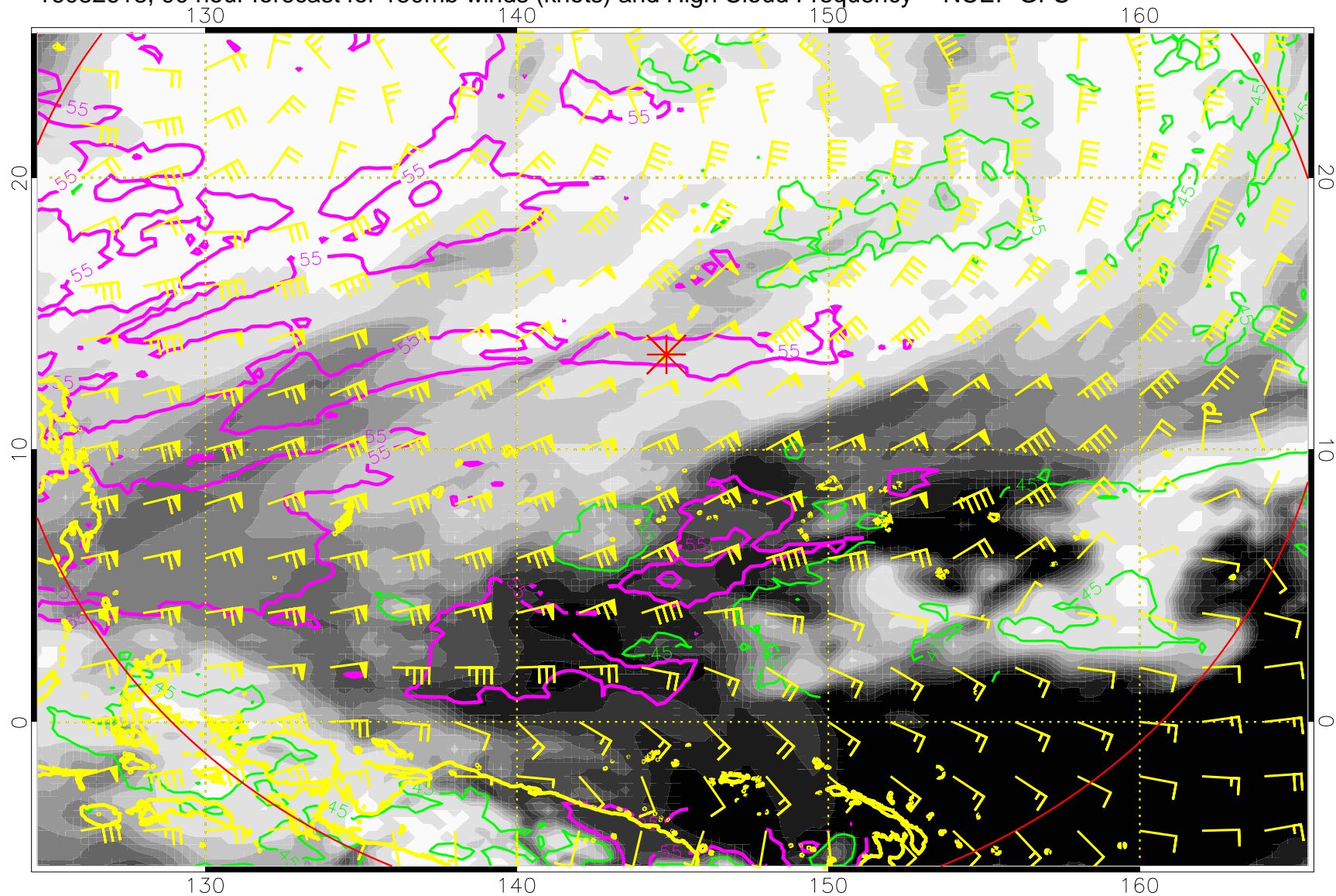
16082618, 90 hour forecast for 150mb winds (knots) and High Cloud Frequency -- NCEP GFS
