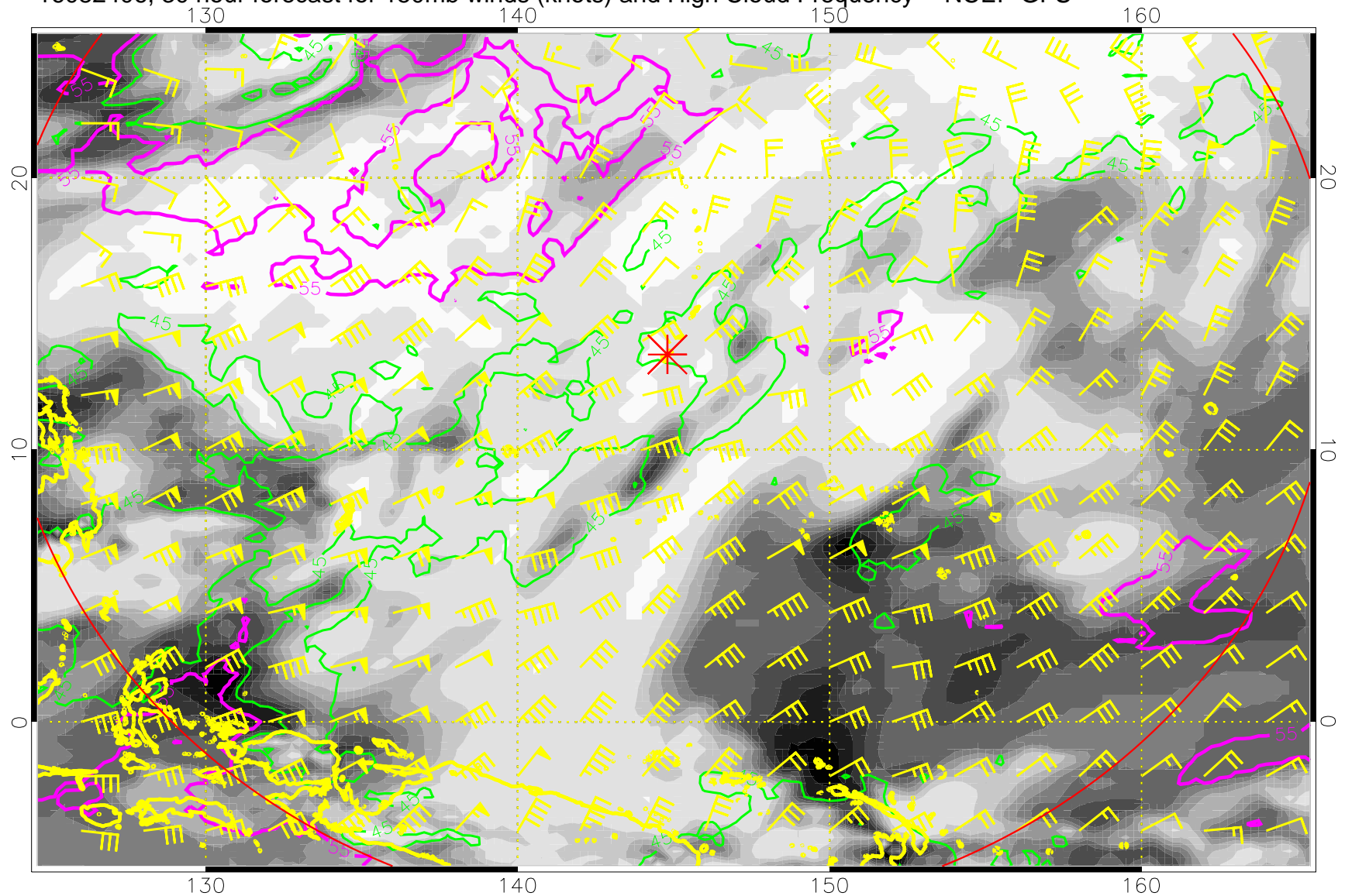
16082406, 30 hour forecast for 150mb winds (knots) and High Cloud Frequency -- NCEP GFS
