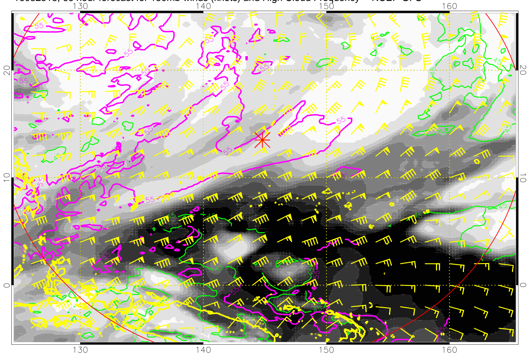
16082518, 66 hour forecast for 150mb winds (knots) and High Cloud Frequency -- NCEP GFS
