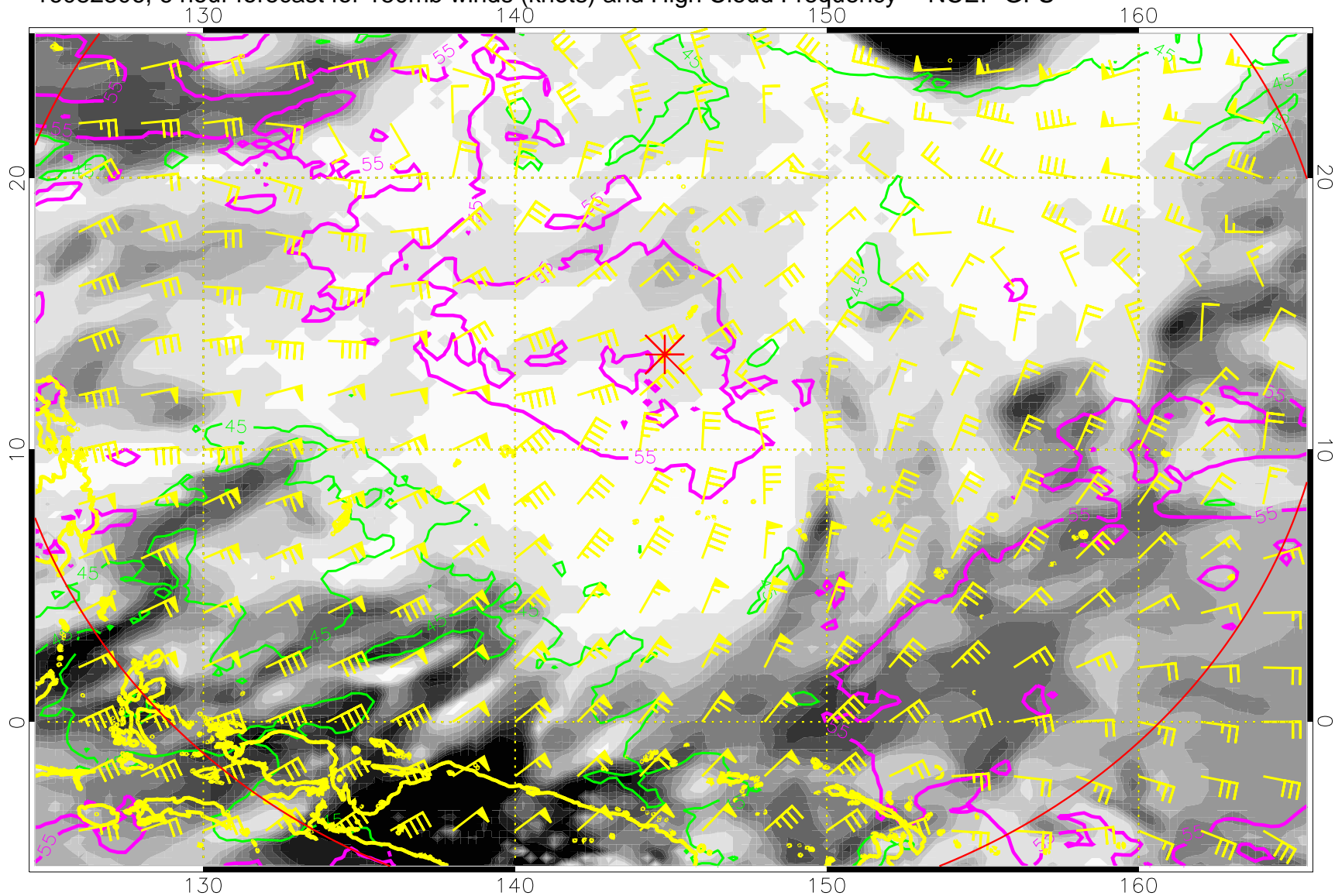
16082306, 6 hour forecast for 150mb winds (knots) and High Cloud Frequency -- NCEP GFS
