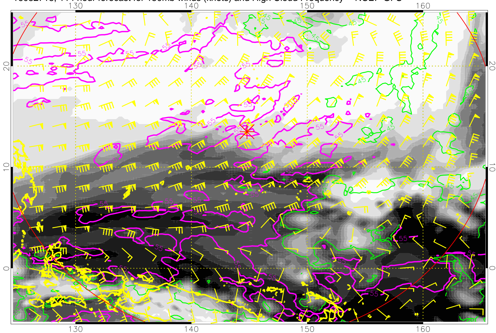
16082718, 114 hour forecast for 150mb winds (knots) and High Cloud Frequency -- NCEP GFS
