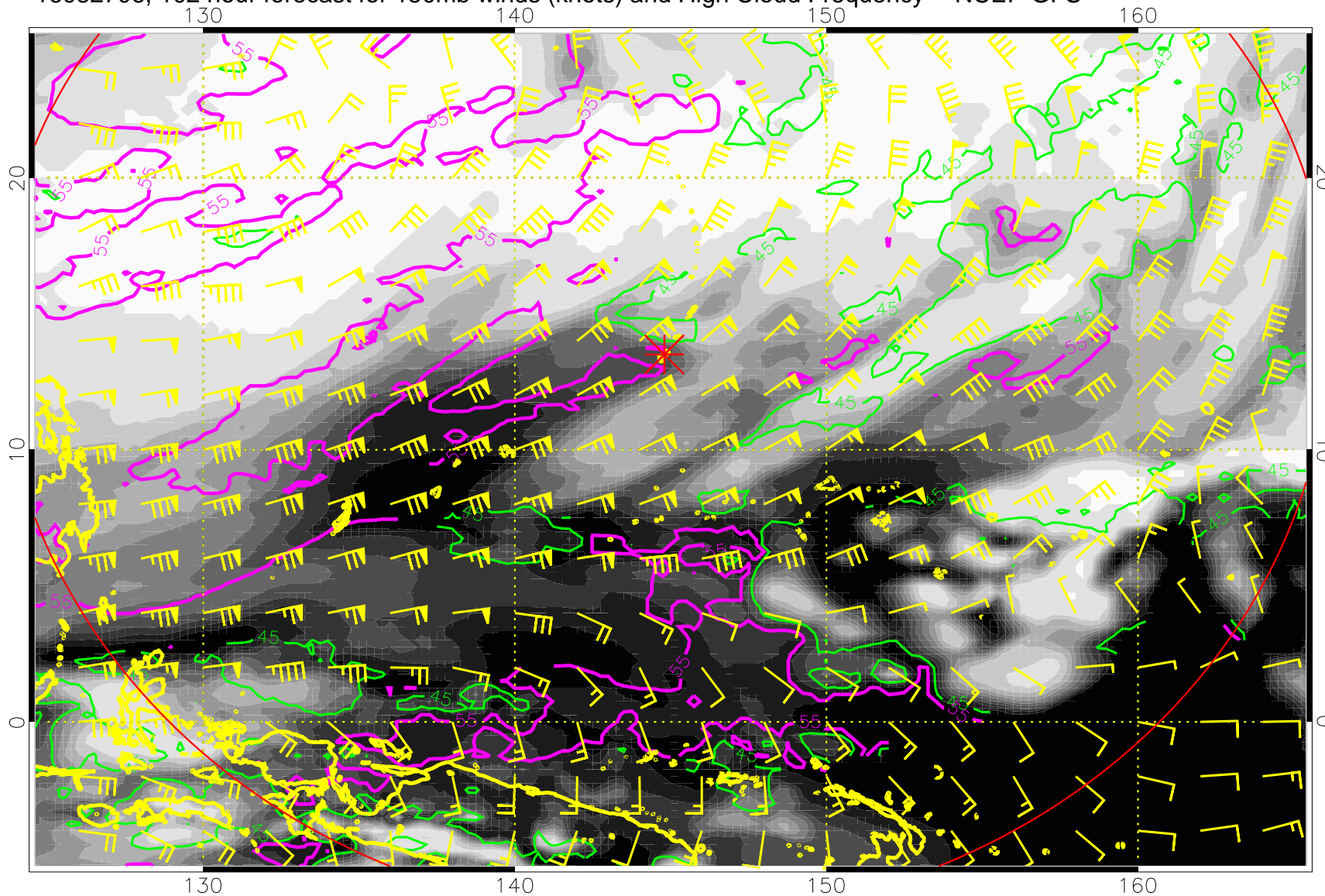
16082706, 102 hour forecast for 150mb winds (knots) and High Cloud Frequency -- NCEP GFS
