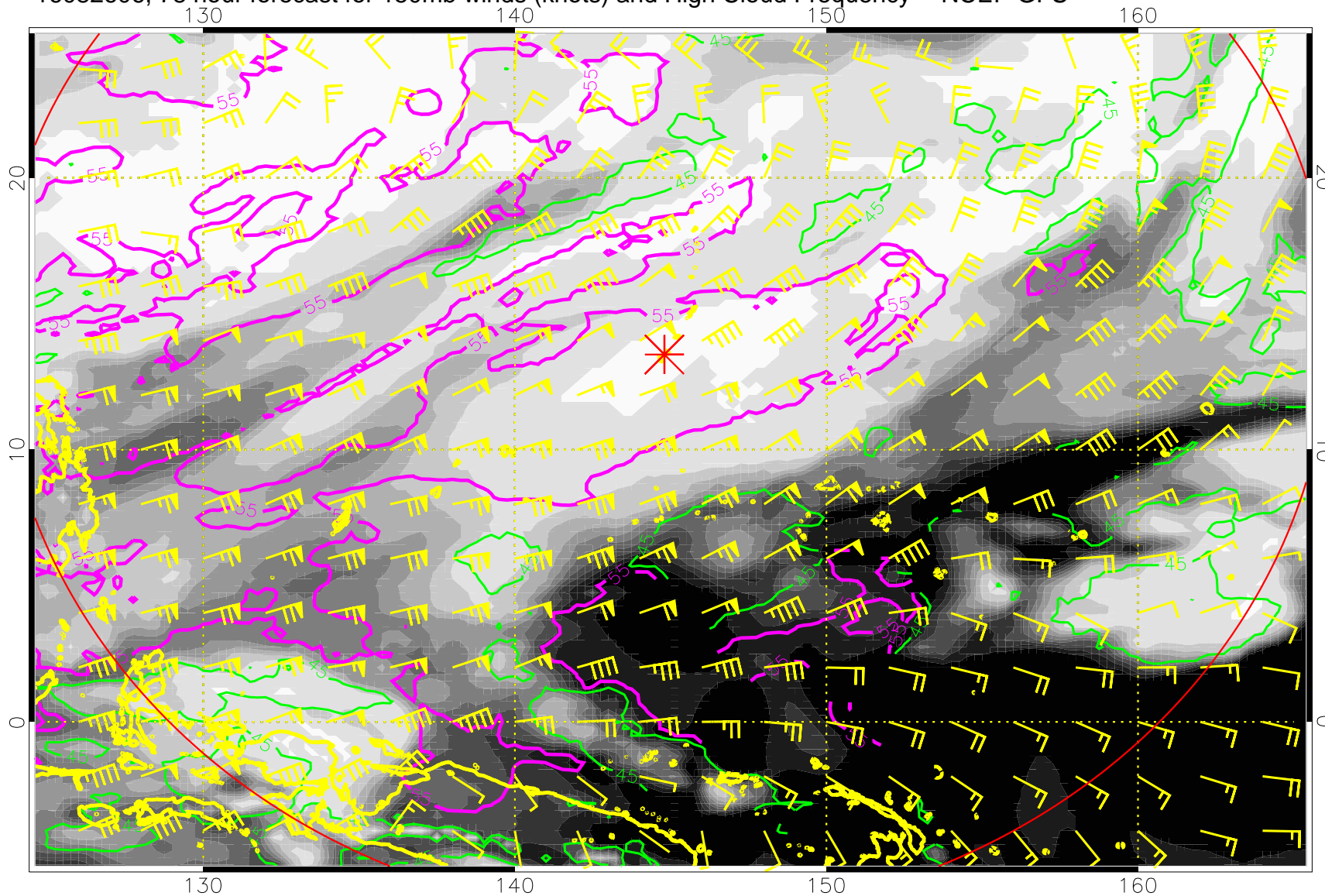
16082606, 78 hour forecast for 150mb winds (knots) and High Cloud Frequency -- NCEP GFS
