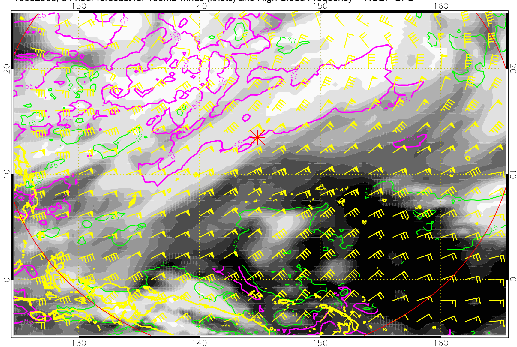
16082506, 54 hour forecast for 150mb winds (knots) and High Cloud Frequency -- NCEP GFS
