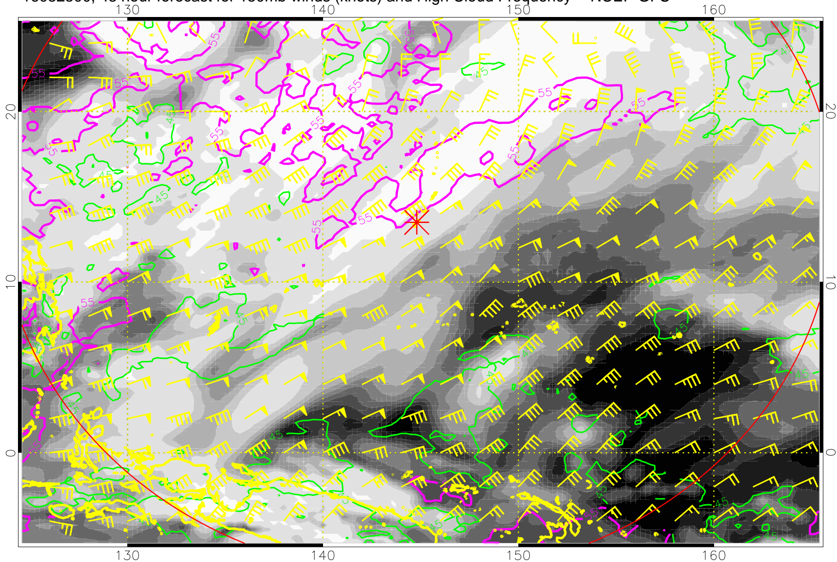
16082500, 48 hour forecast for 150mb winds (knots) and High Cloud Frequency -- NCEP GFS
