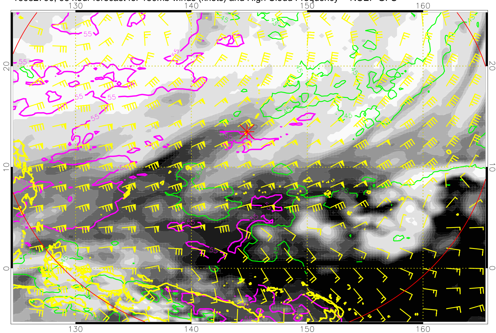
16082700, 96 hour forecast for 150mb winds (knots) and High Cloud Frequency -- NCEP GFS
