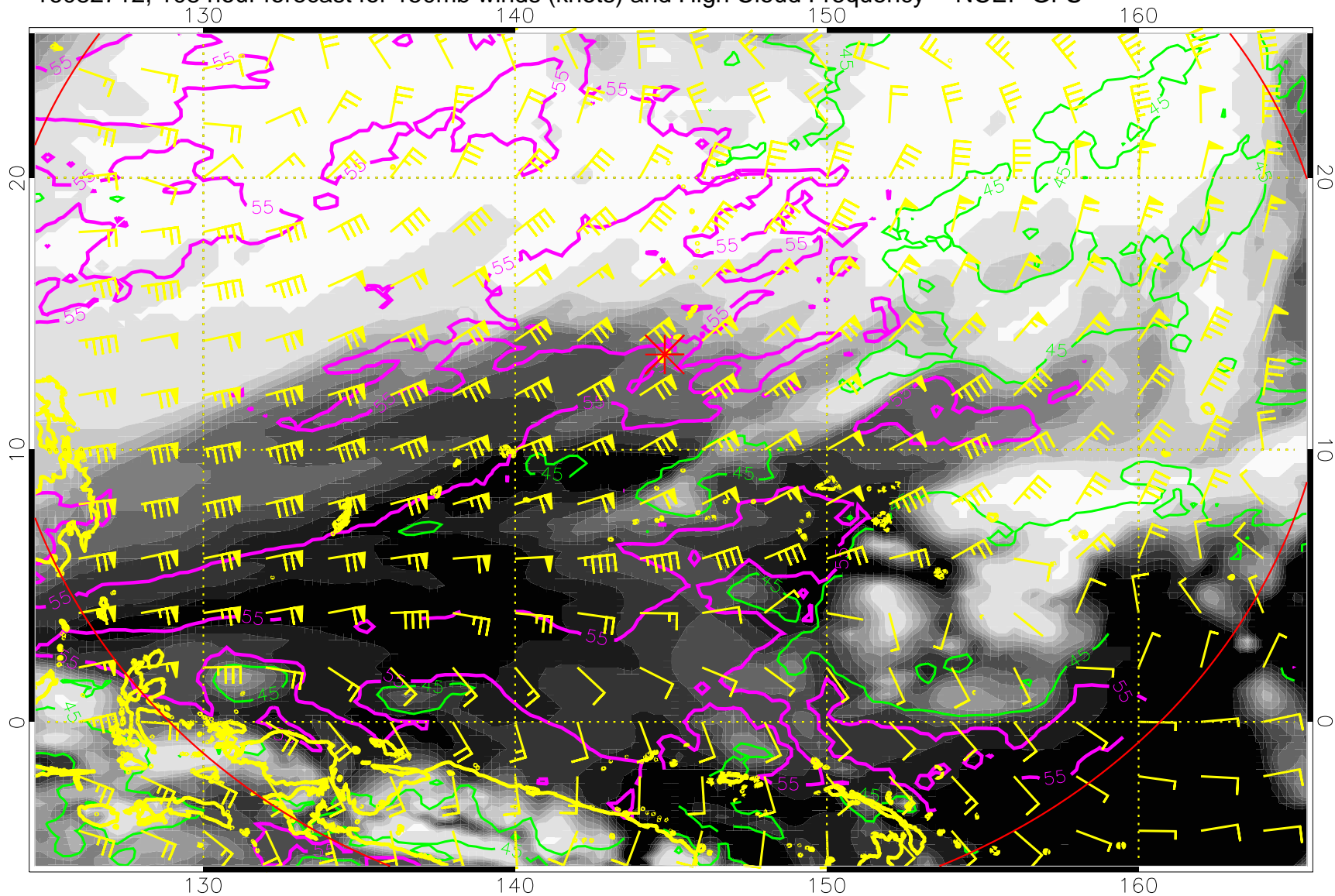
16082712, 108 hour forecast for 150mb winds (knots) and High Cloud Frequency -- NCEP GFS
