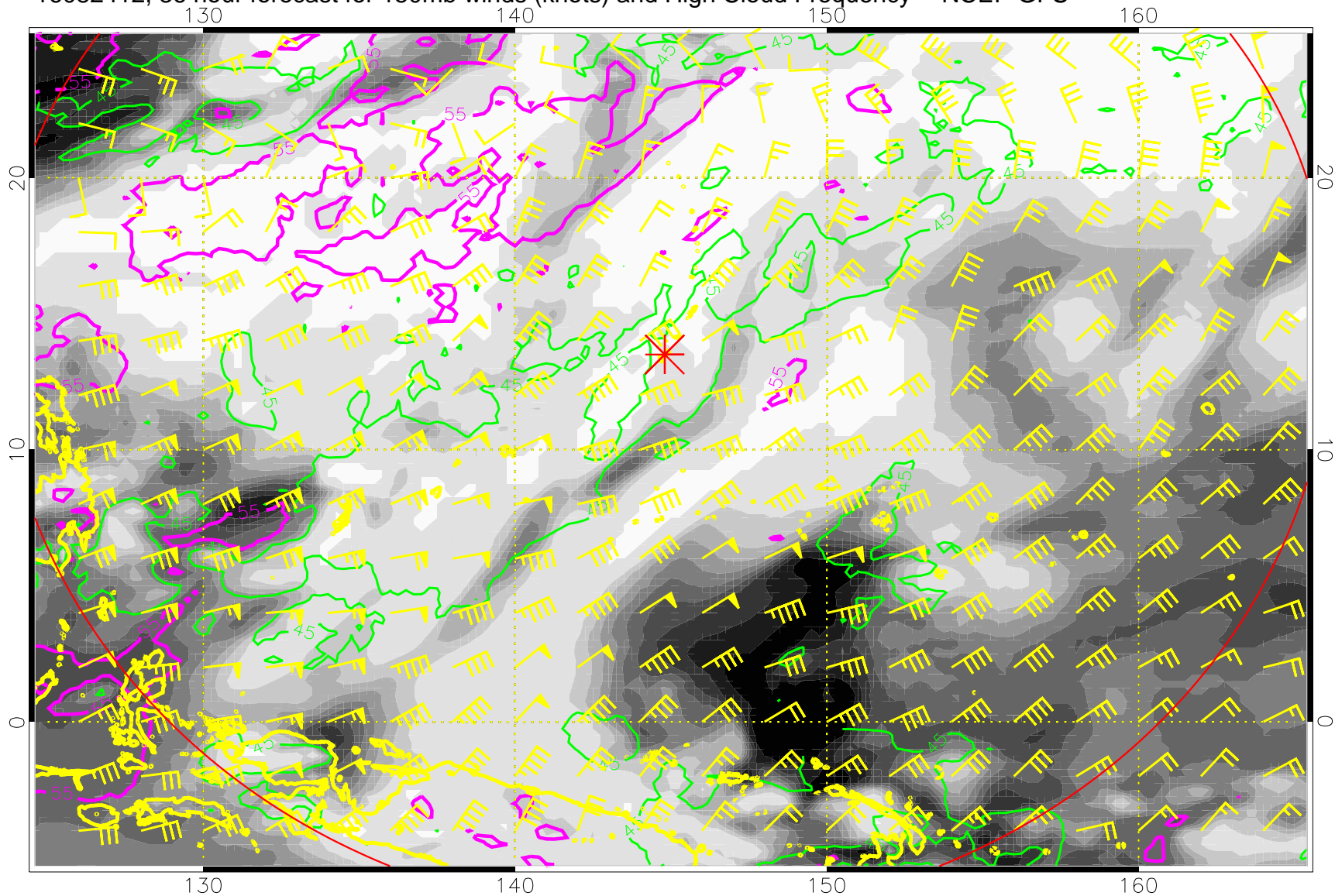
16082412, 36 hour forecast for 150mb winds (knots) and High Cloud Frequency -- NCEP GFS
