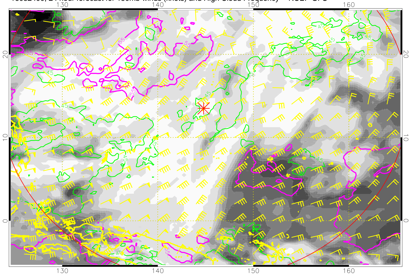
16082400, 24 hour forecast for 150mb winds (knots) and High Cloud Frequency -- NCEP GFS
