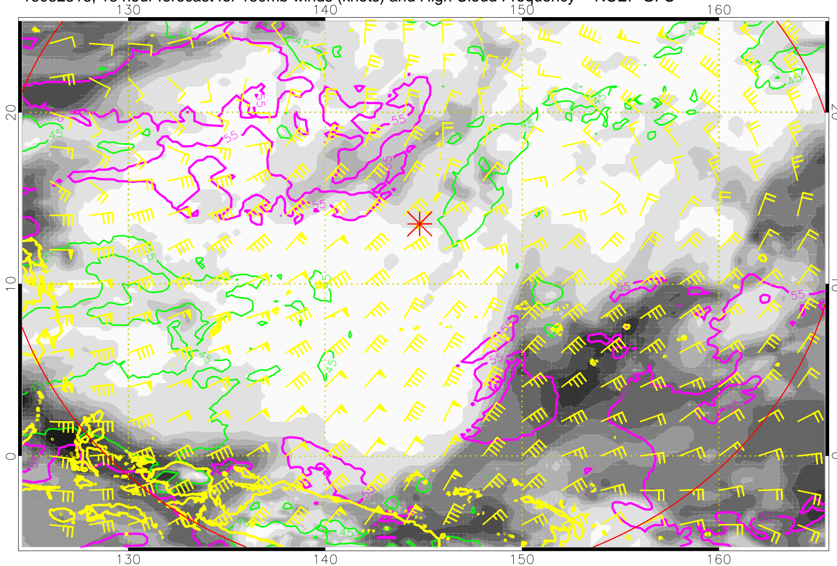
16082318, 18 hour forecast for 150mb winds (knots) and High Cloud Frequency -- NCEP GFS
