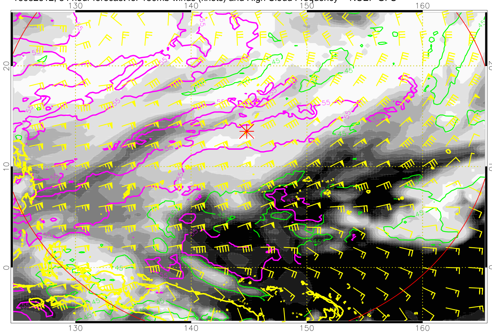
16082612, 84 hour forecast for 150mb winds (knots) and High Cloud Frequency -- NCEP GFS
