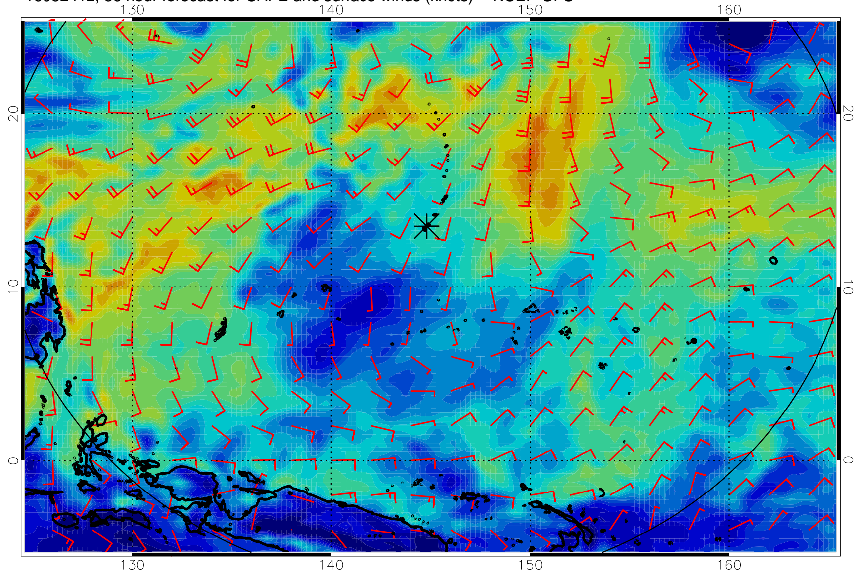
16082412, 36 hour forecast for CAPE and surface winds (knots) -- NCEP GFS
