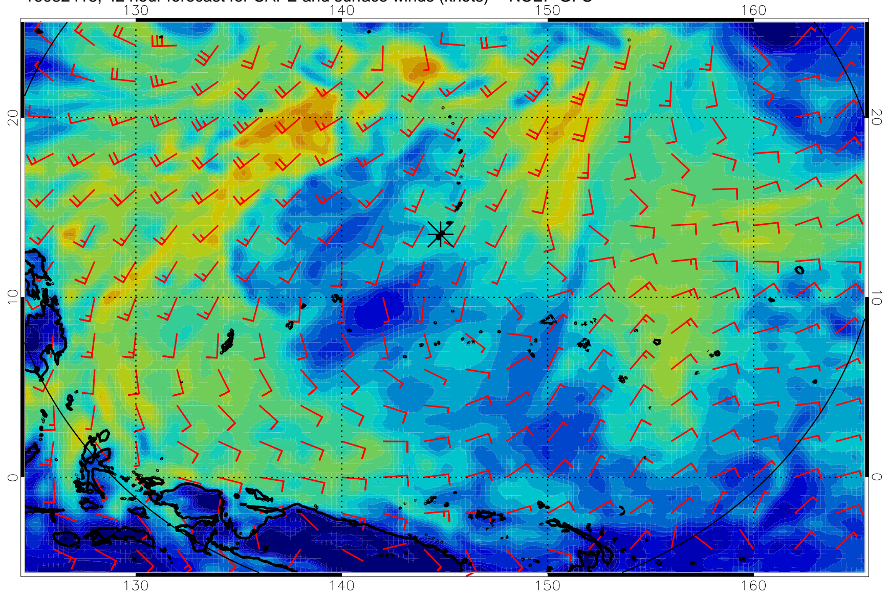
16082418, 42 hour forecast for CAPE and surface winds (knots) -- NCEP GFS
