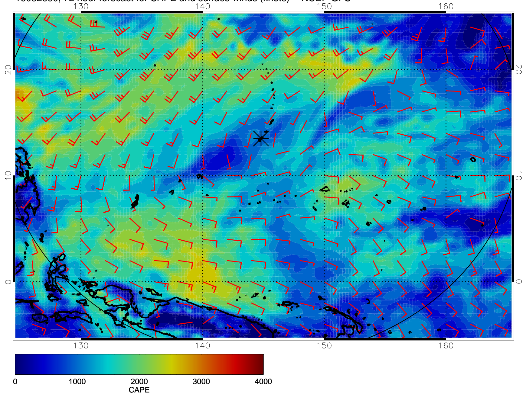
16082600, 72 hour forecast for CAPE and surface winds (knots) -- NCEP GFS
