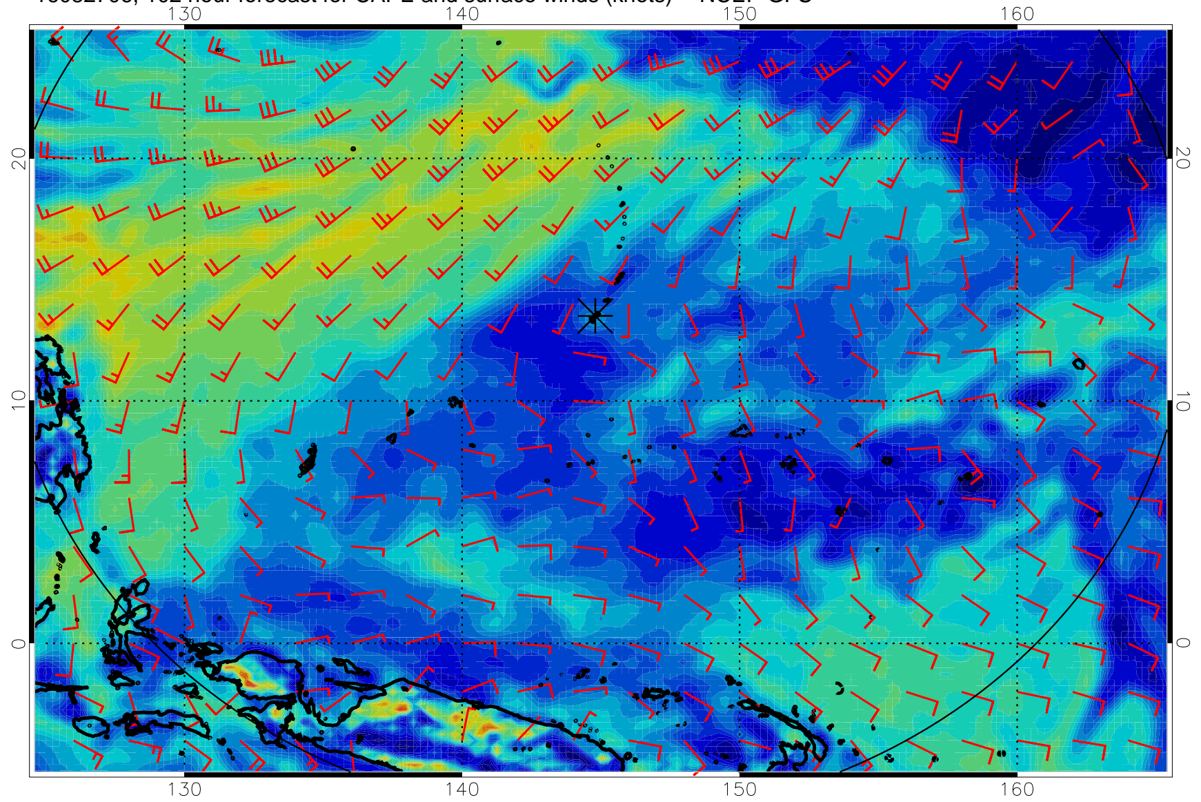
16082706, 102 hour forecast for CAPE and surface winds (knots) -- NCEP GFS
