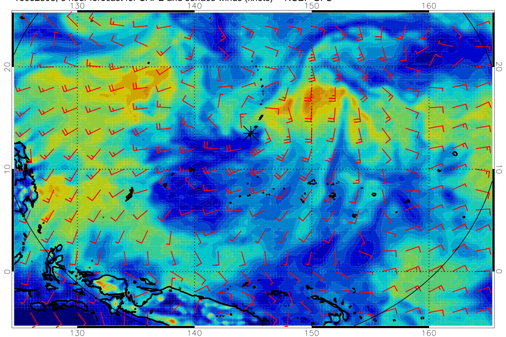
16082306, 6 hour forecast for CAPE and surface winds (knots) -- NCEP GFS
