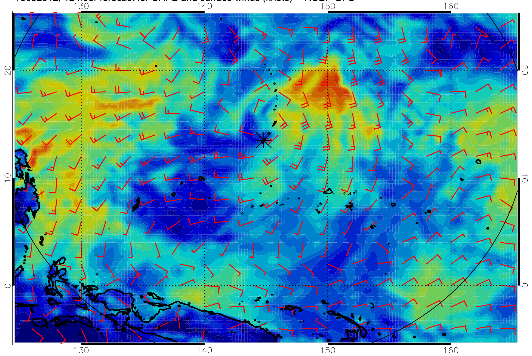
16082312, 12 hour forecast for CAPE and surface winds (knots) -- NCEP GFS
