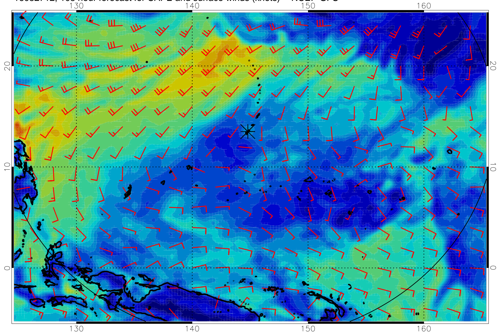
16082712, 108 hour forecast for CAPE and surface winds (knots) -- NCEP GFS
