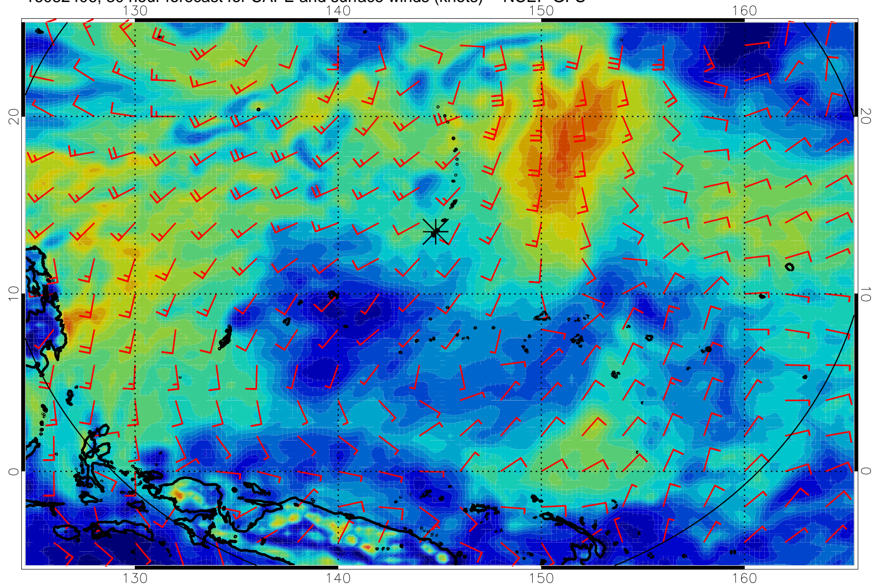
16082406, 30 hour forecast for CAPE and surface winds (knots) -- NCEP GFS
