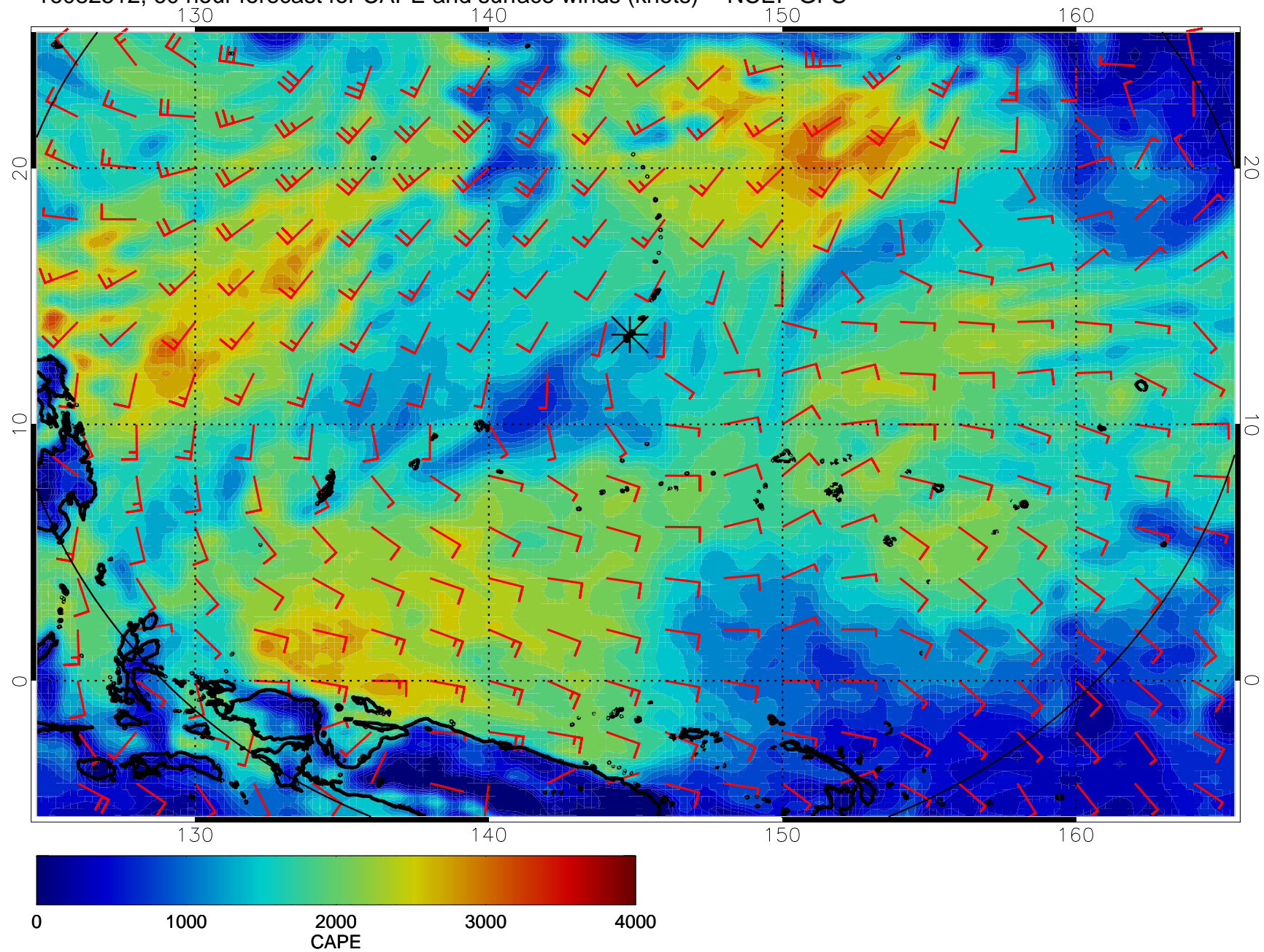
16082512, 60 hour forecast for CAPE and surface winds (knots) -- NCEP GFS
