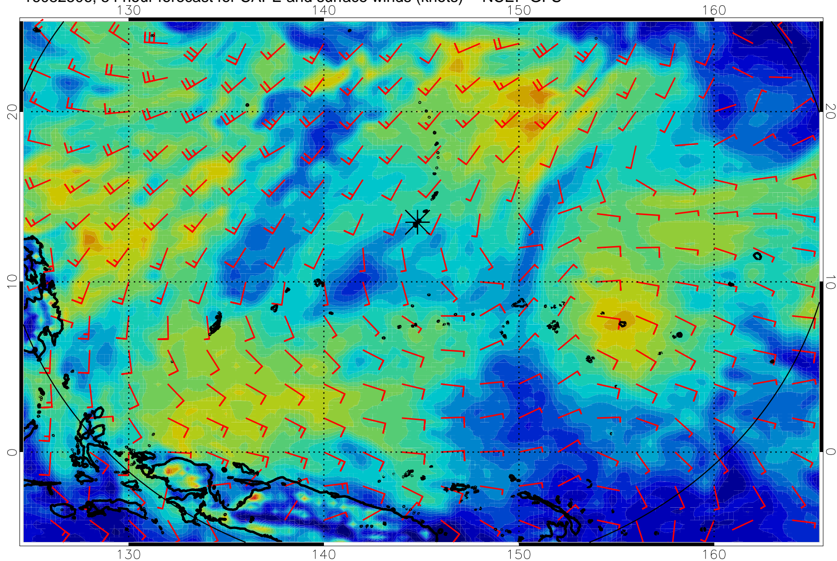
16082506, 54 hour forecast for CAPE and surface winds (knots) -- NCEP GFS
