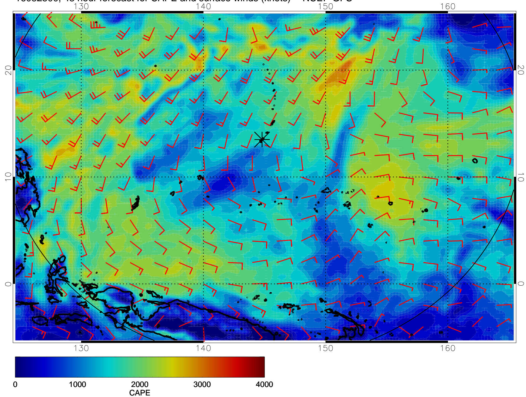
16082500, 48 hour forecast for CAPE and surface winds (knots) -- NCEP GFS
