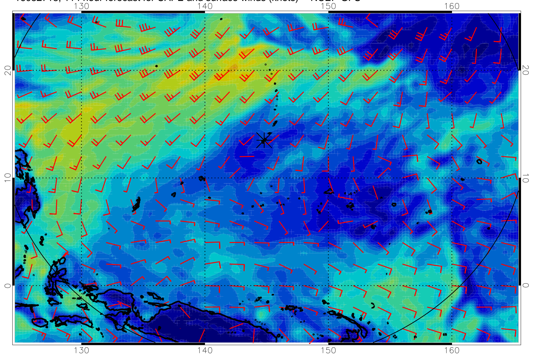
16082718, 114 hour forecast for CAPE and surface winds (knots) -- NCEP GFS
