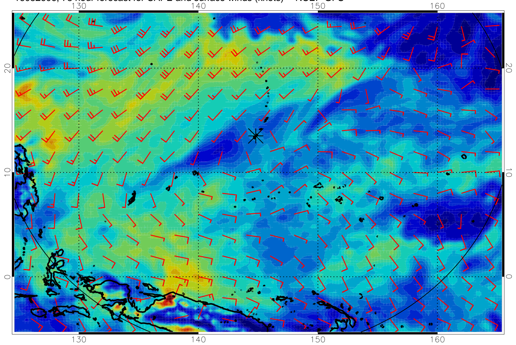
16082606, 78 hour forecast for CAPE and surface winds (knots) -- NCEP GFS
