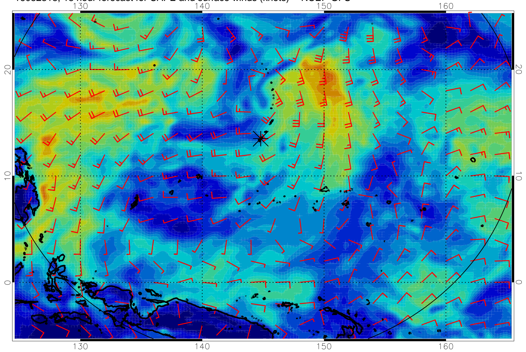
16082318, 18 hour forecast for CAPE and surface winds (knots) -- NCEP GFS
