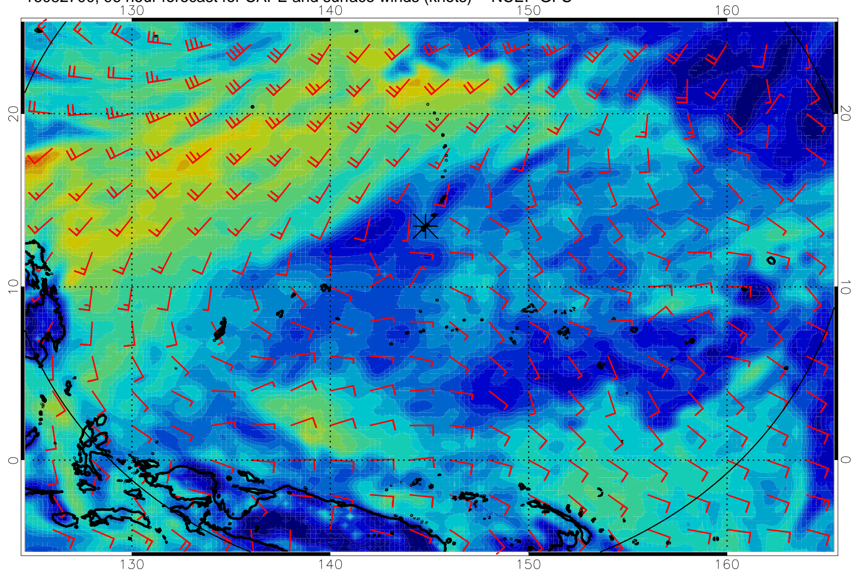
16082700, 96 hour forecast for CAPE and surface winds (knots) -- NCEP GFS
