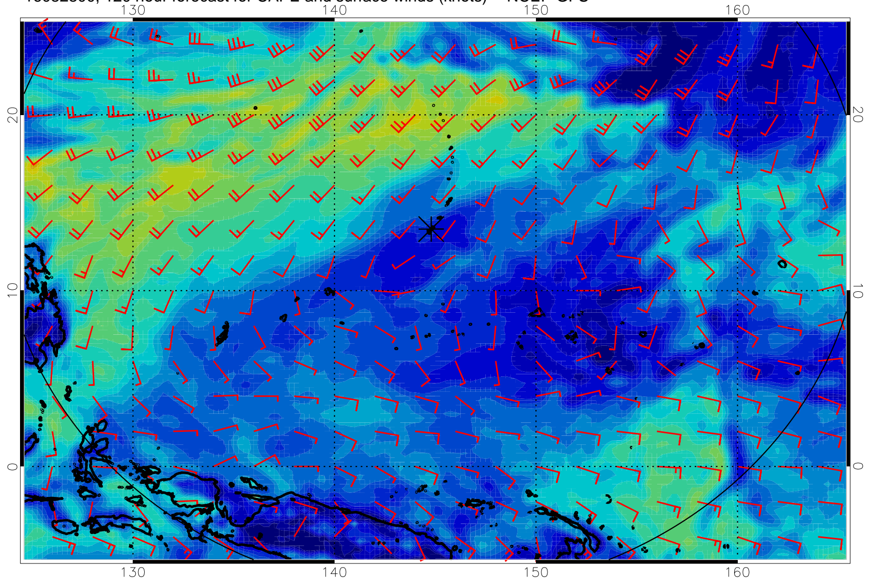
16082800, 120 hour forecast for CAPE and surface winds (knots) -- NCEP GFS
