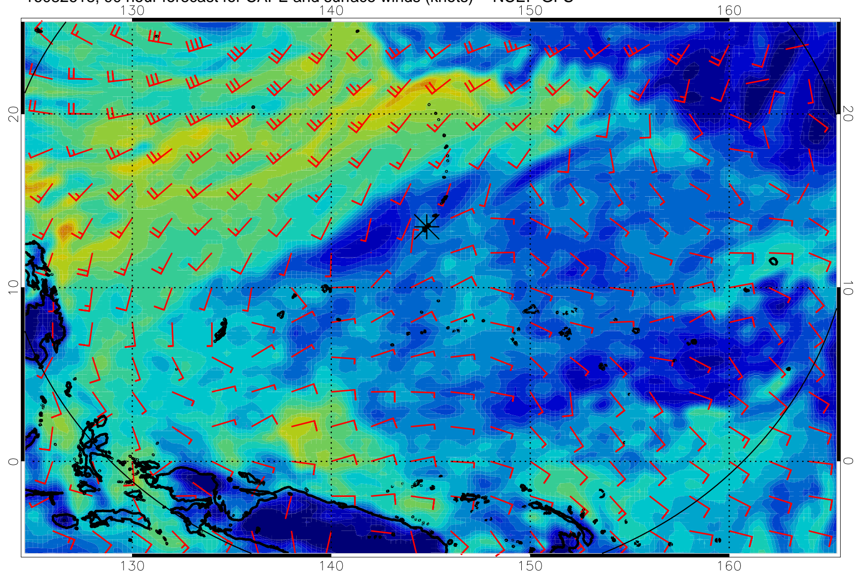
16082618, 90 hour forecast for CAPE and surface winds (knots) -- NCEP GFS
