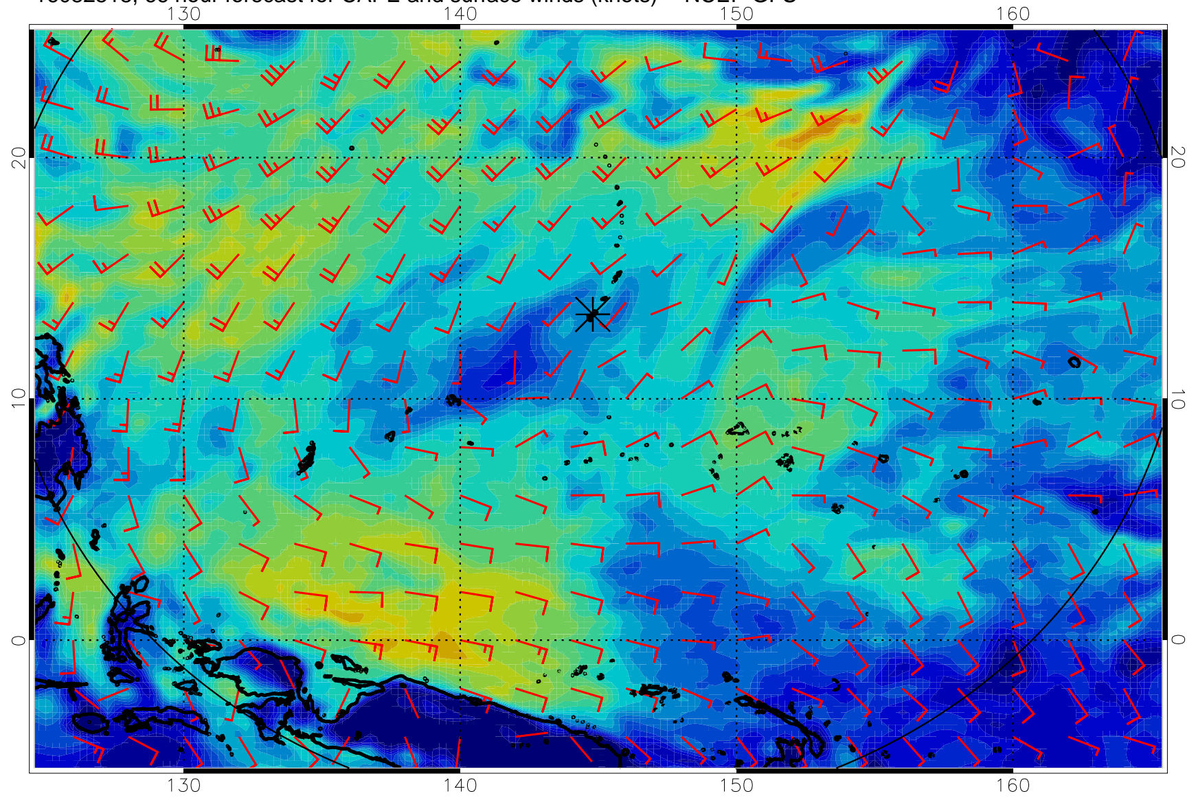
16082518, 66 hour forecast for CAPE and surface winds (knots) -- NCEP GFS
