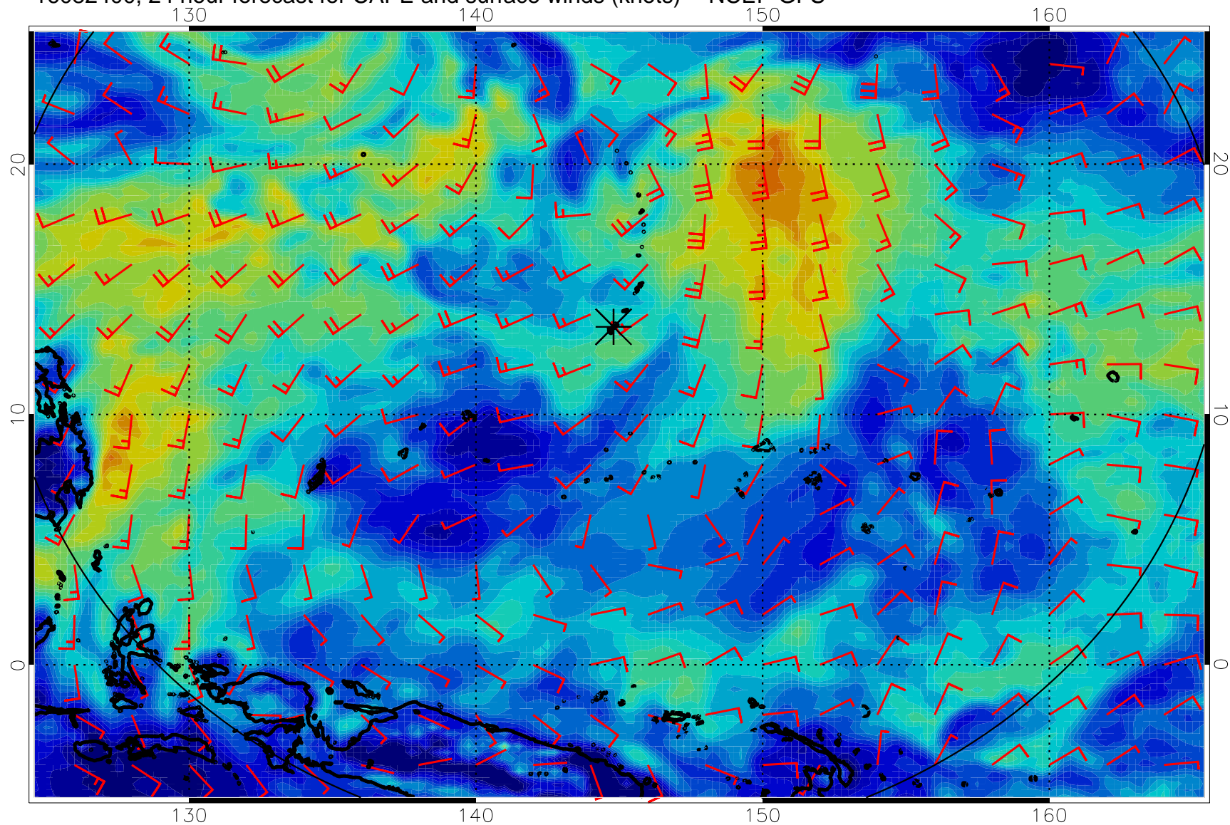
16082400, 24 hour forecast for CAPE and surface winds (knots) -- NCEP GFS
