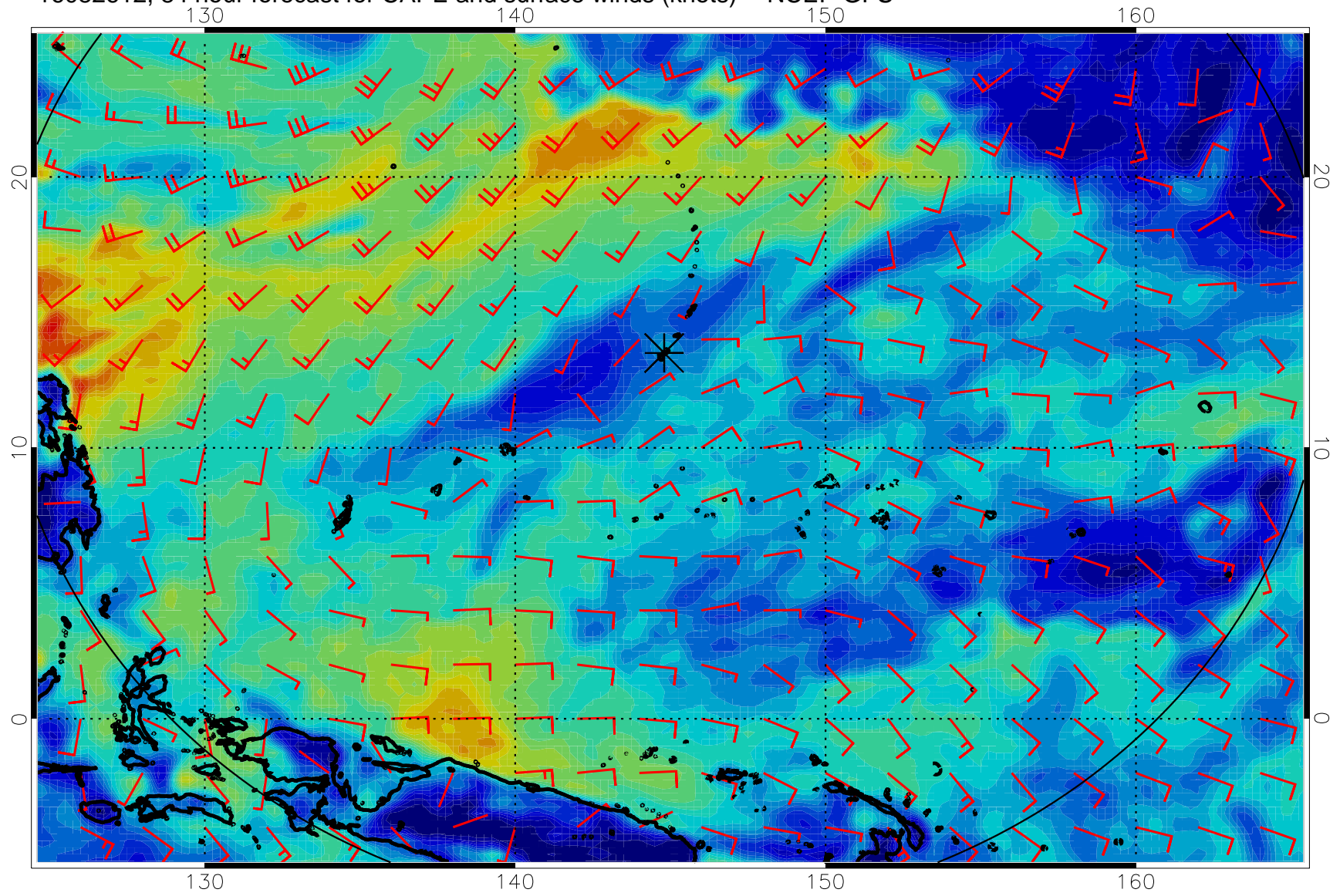
16082612, 84 hour forecast for CAPE and surface winds (knots) -- NCEP GFS
