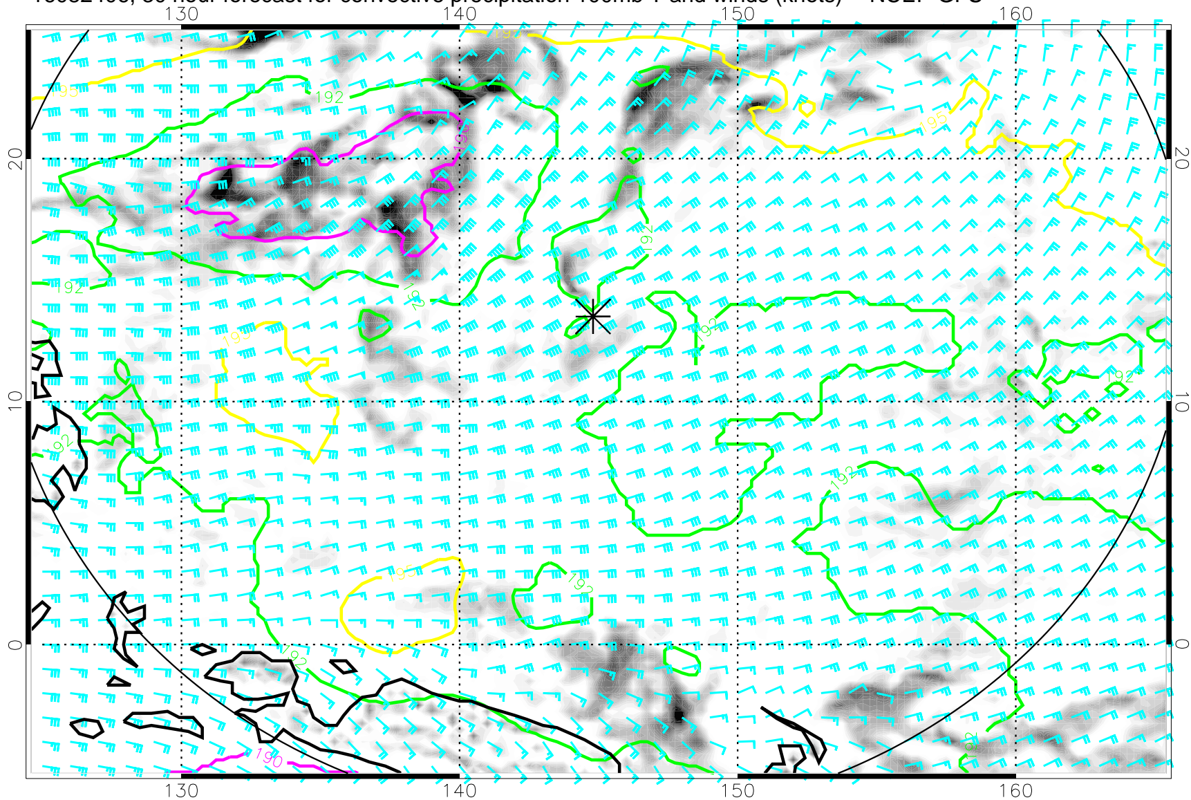
16082406, 30 hour forecast for convective precipitation 100mb T and winds (knots) -- NCEP GFS
