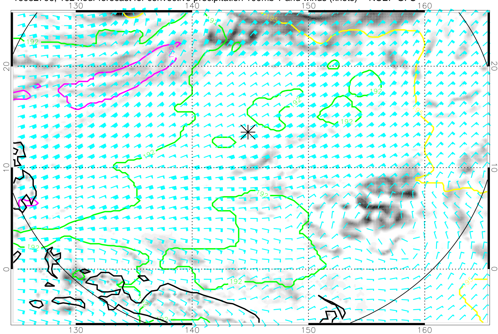
16082706, 102 hour forecast for convective precipitation 100mb T and winds (knots) -- NCEP GFS
