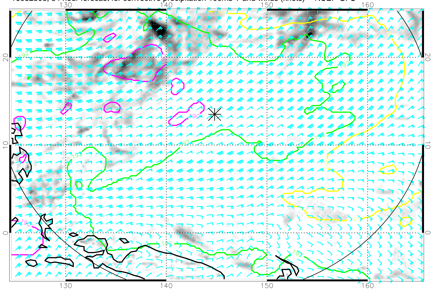
16082506, 54 hour forecast for convective precipitation 100mb T and winds (knots) -- NCEP GFS
