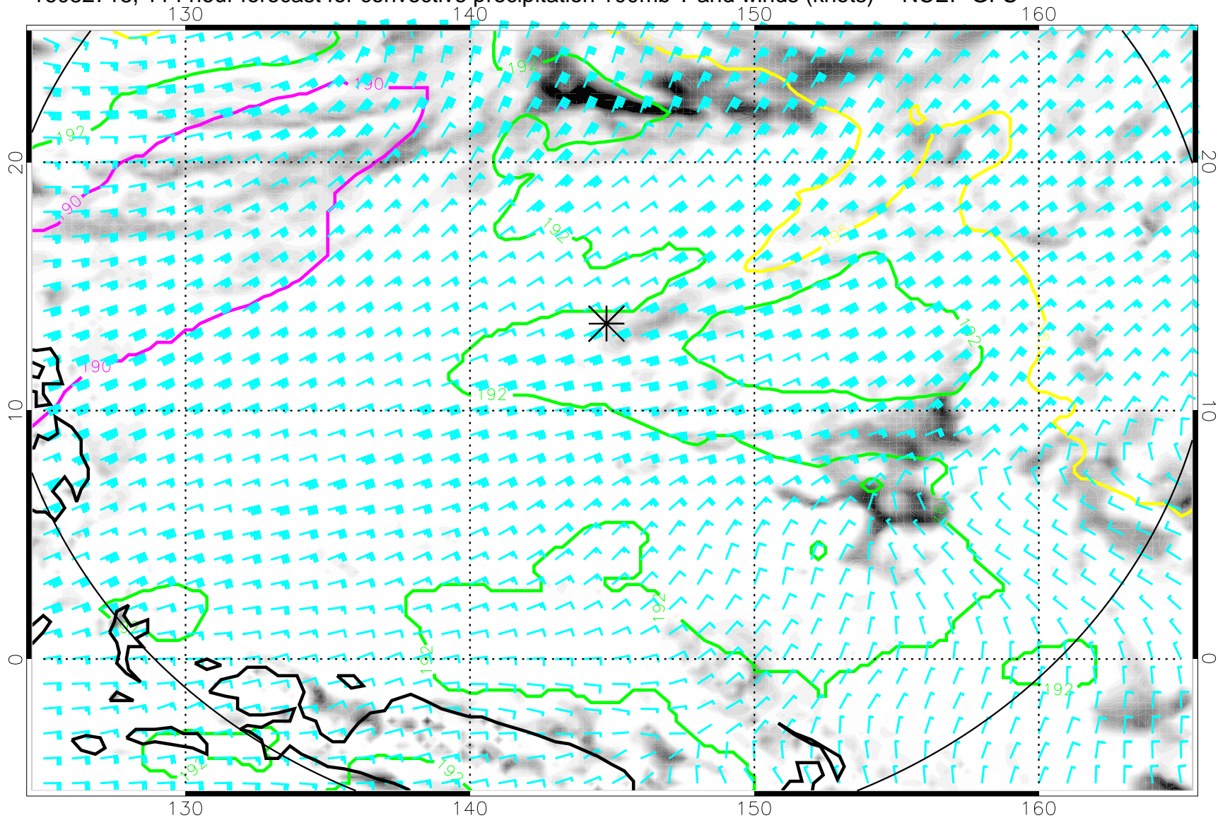
16082718, 114 hour forecast for convective precipitation 100mb T and winds (knots) -- NCEP GFS
