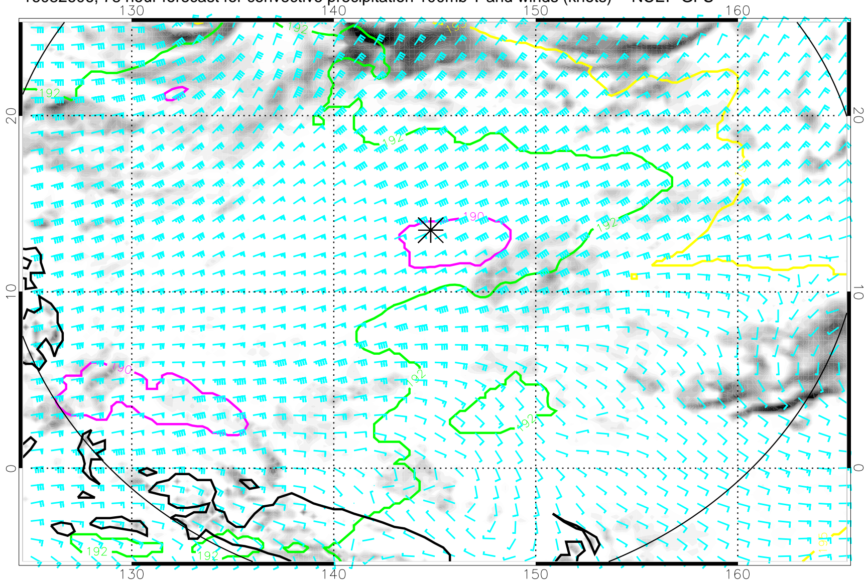
16082606, 78 hour forecast for convective precipitation 100mb T and winds (knots) -- NCEP GFS
