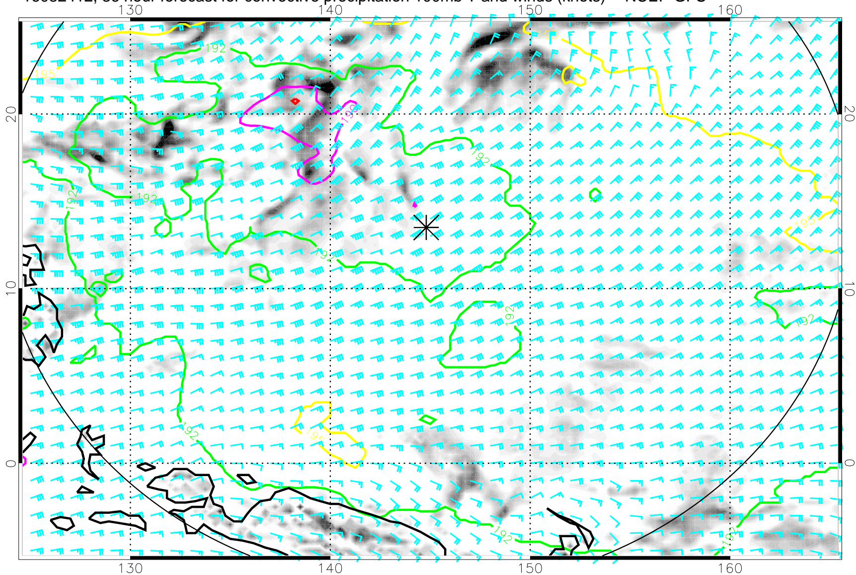
16082412, 36 hour forecast for convective precipitation 100mb T and winds (knots) -- NCEP GFS
