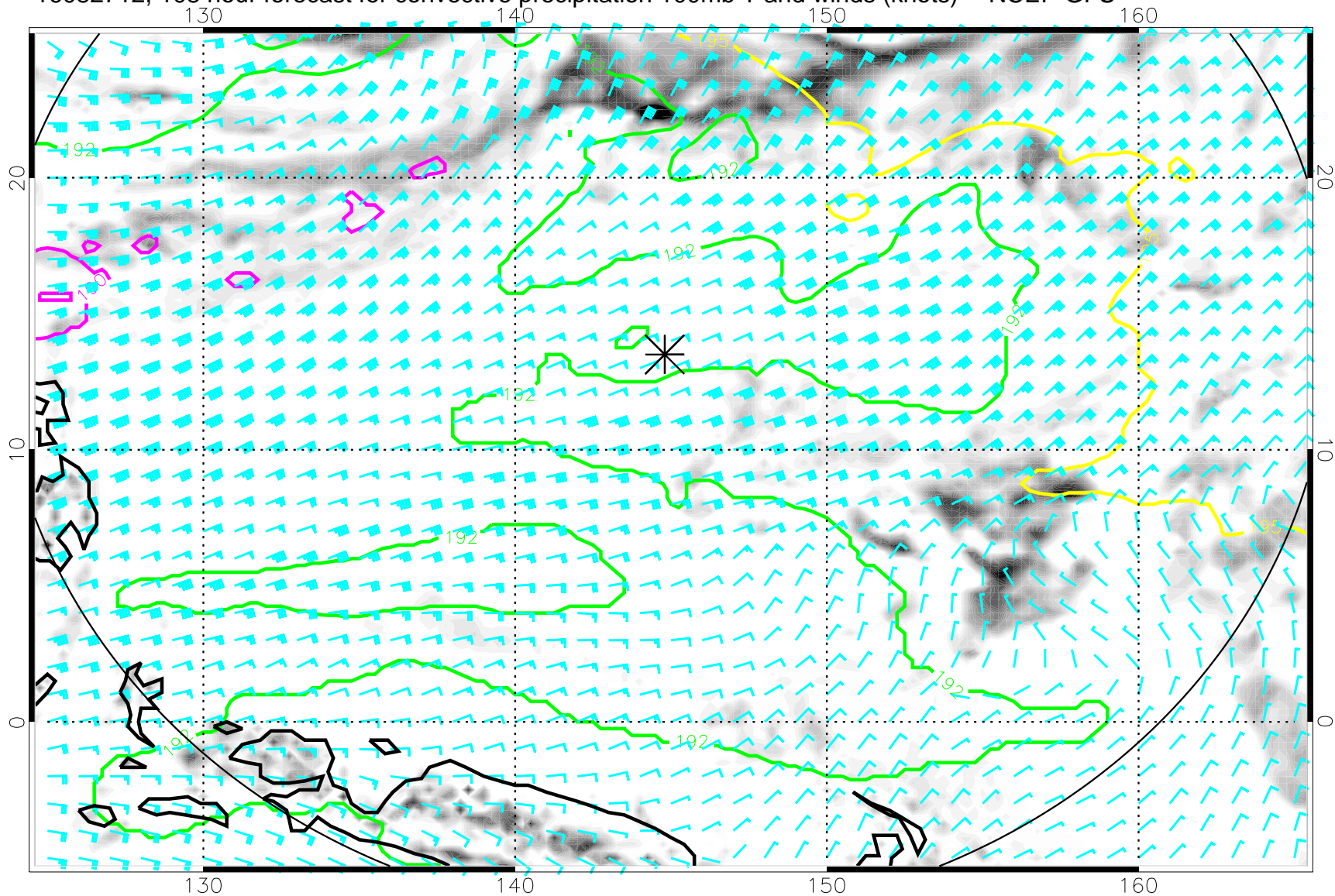
16082712, 108 hour forecast for convective precipitation 100mb T and winds (knots) -- NCEP GFS
