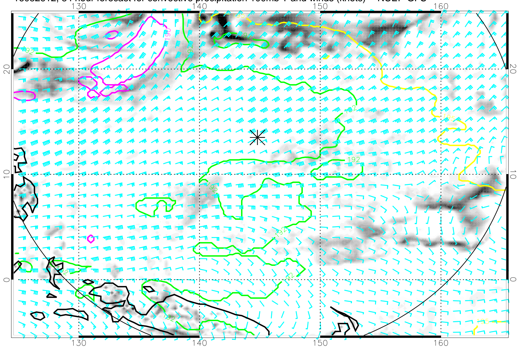
16082612, 84 hour forecast for convective precipitation 100mb T and winds (knots) -- NCEP GFS
