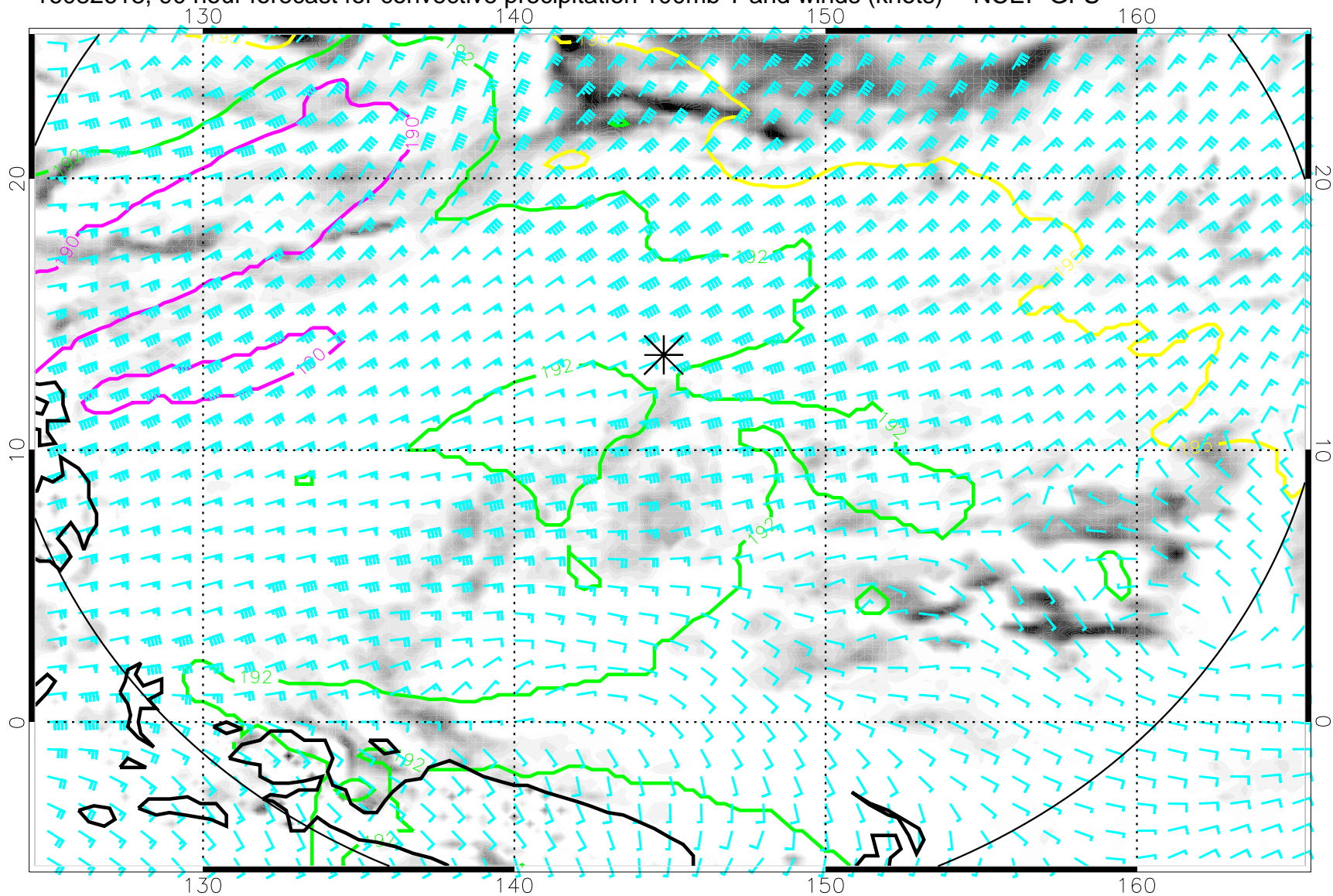
16082618, 90 hour forecast for convective precipitation 100mb T and winds (knots) -- NCEP GFS
