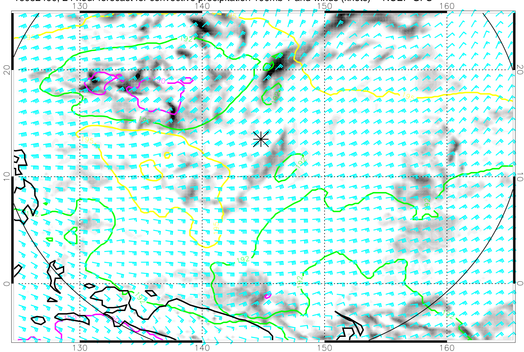
16082400, 24 hour forecast for convective precipitation 100mb T and winds (knots) -- NCEP GFS
