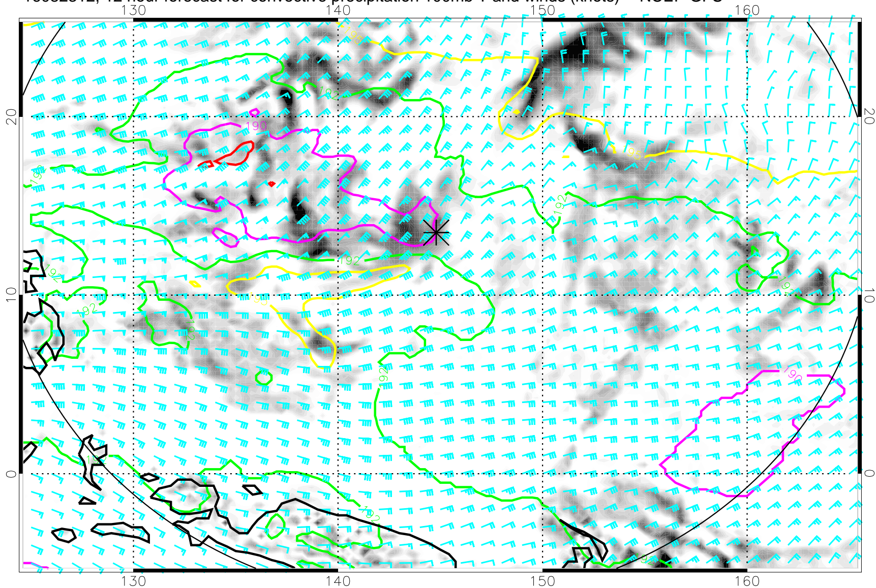
16082312, 12 hour forecast for convective precipitation 100mb T and winds (knots) -- NCEP GFS
