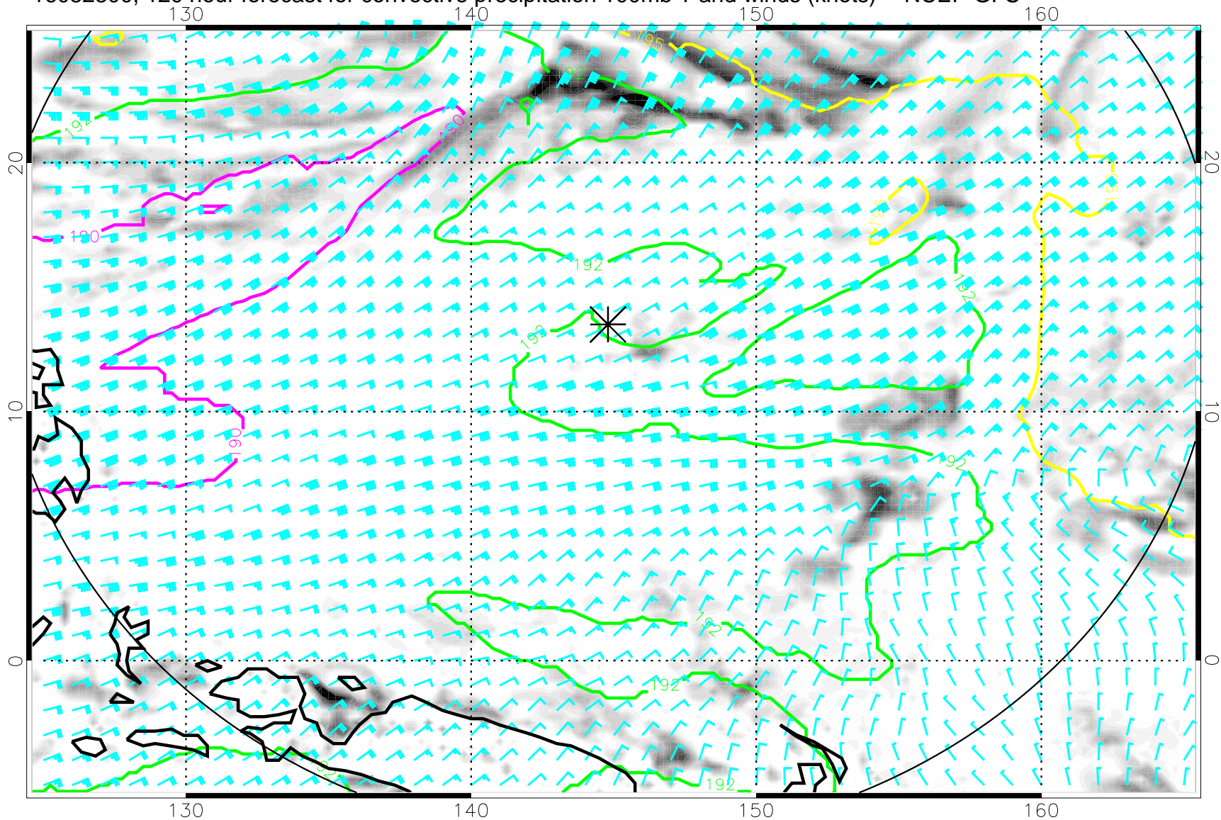
16082800, 120 hour forecast for convective precipitation 100mb T and winds (knots) -- NCEP GFS
