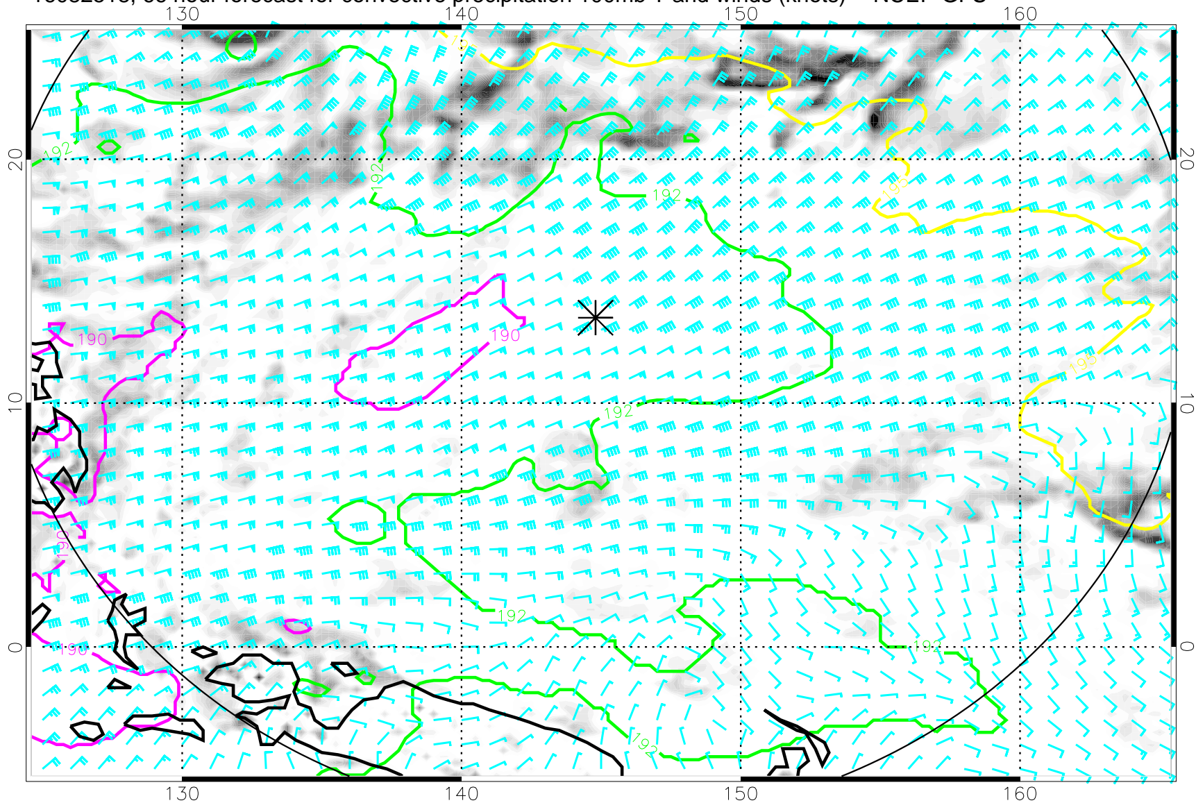
16082518, 66 hour forecast for convective precipitation 100mb T and winds (knots) -- NCEP GFS
