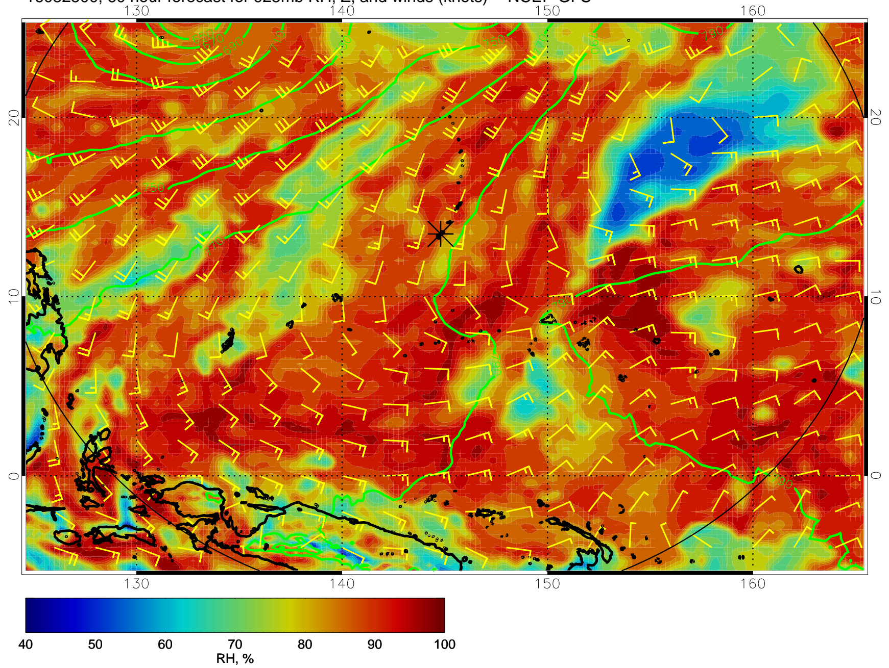
16082500, 60 hour forecast for 925mb RH, Z, and winds (knots) -- NCEP GFS
