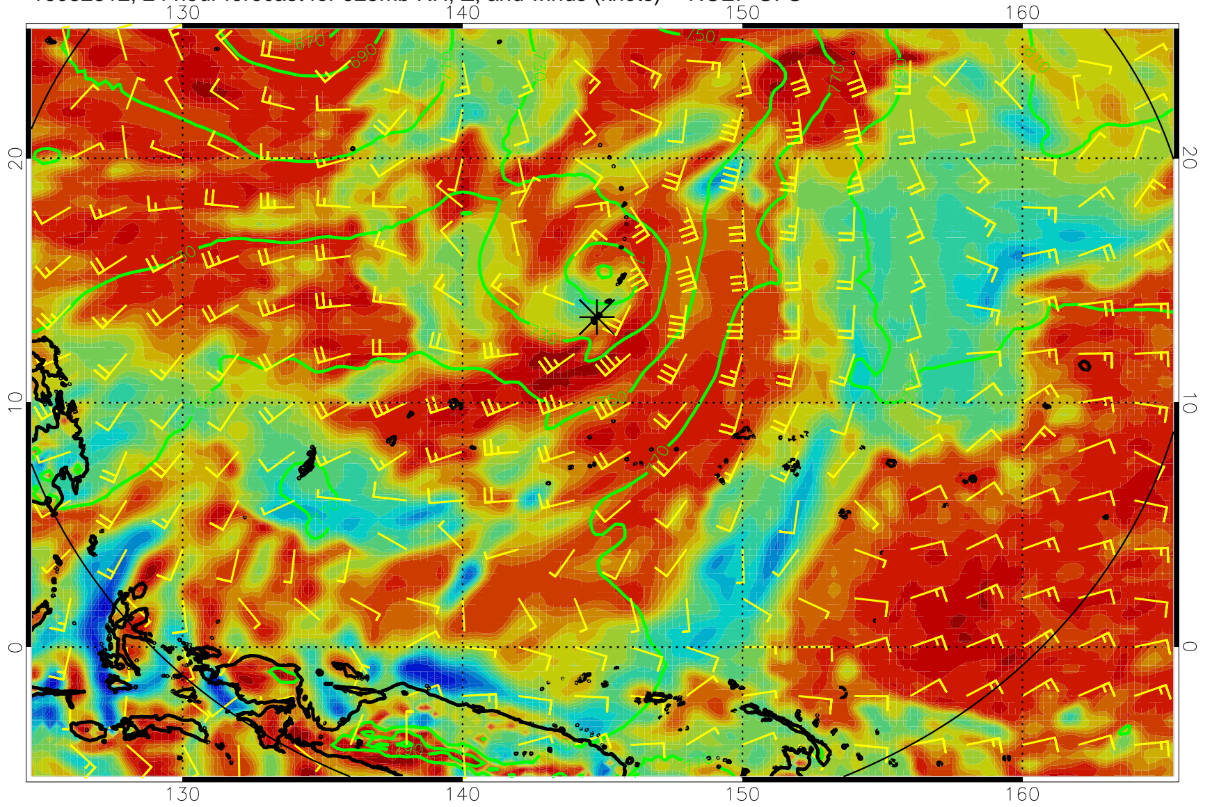
16082312, 24 hour forecast for 925mb RH, Z, and winds (knots) -- NCEP GFS
