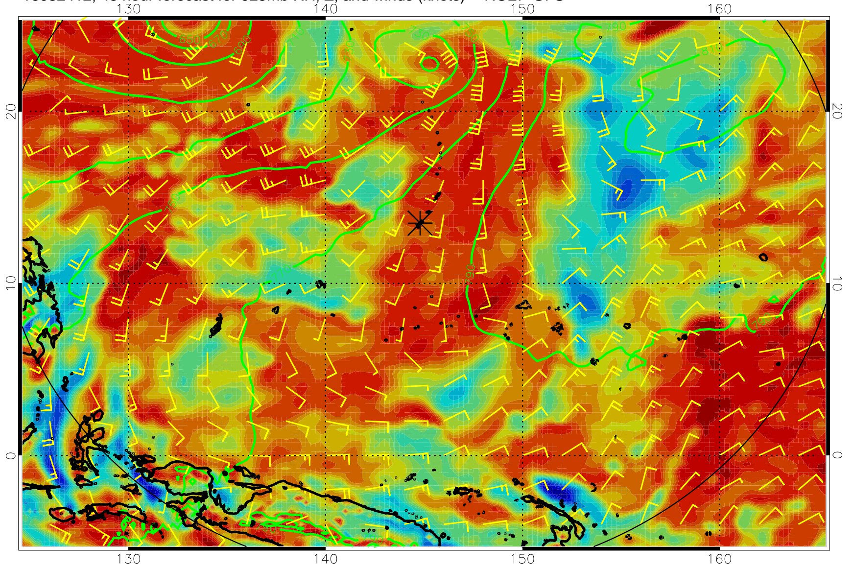
16082412, 48 hour forecast for 925mb RH, Z, and winds (knots) -- NCEP GFS
