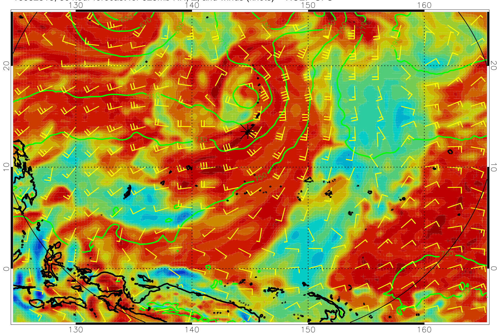
16082318, 30 hour forecast for 925mb RH, Z, and winds (knots) -- NCEP GFS
