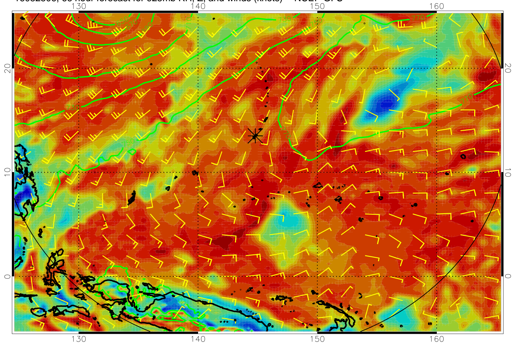
16082506, 66 hour forecast for 925mb RH, Z, and winds (knots) -- NCEP GFS
