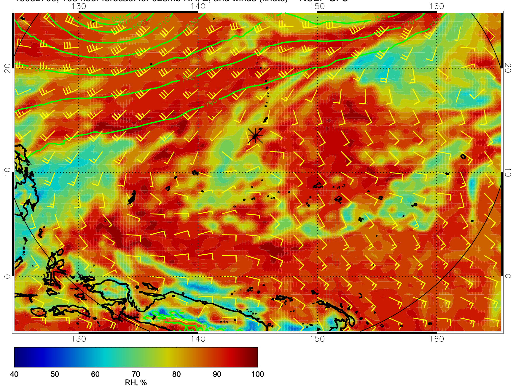
16082700, 108 hour forecast for 925mb RH, Z, and winds (knots) -- NCEP GFS
