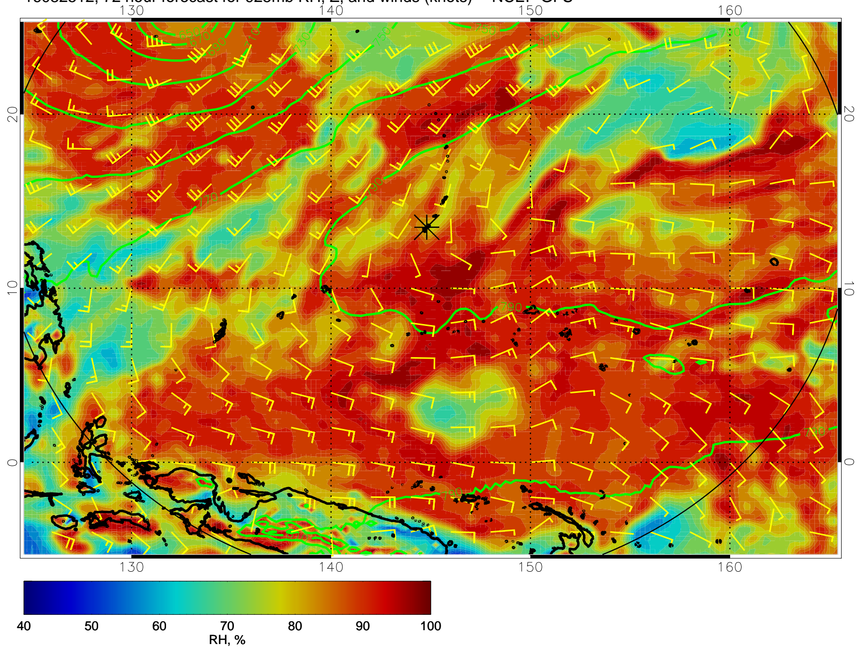
16082512, 72 hour forecast for 925mb RH, Z, and winds (knots) -- NCEP GFS
