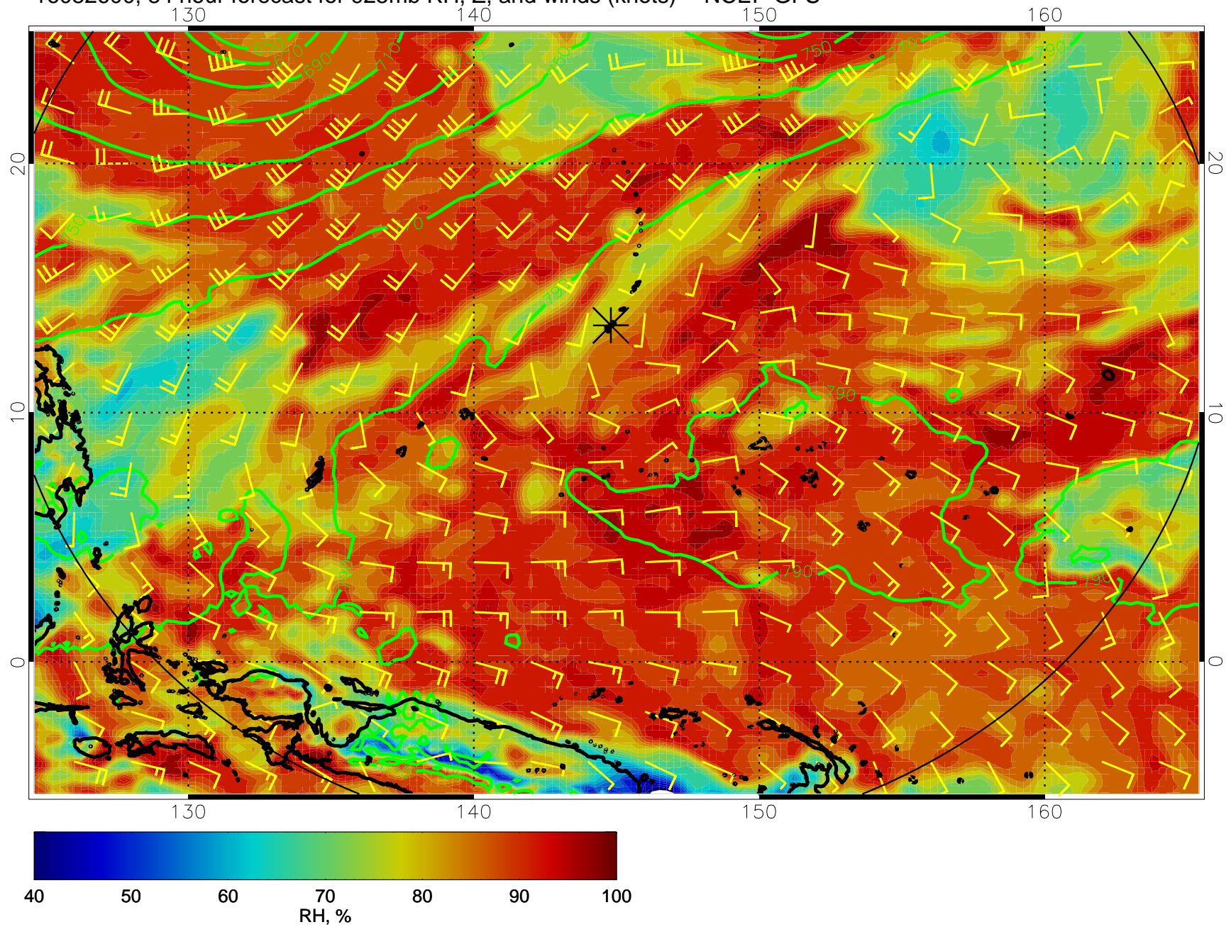
16082600, 84 hour forecast for 925mb RH, Z, and winds (knots) -- NCEP GFS
