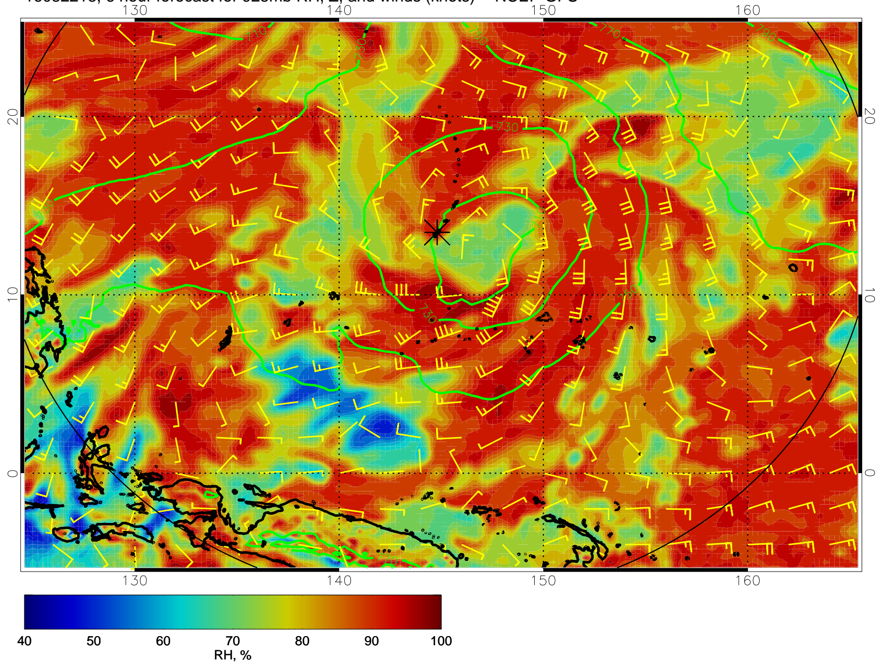
16082218, 6 hour forecast for 925mb RH, Z, and winds (knots) -- NCEP GFS
