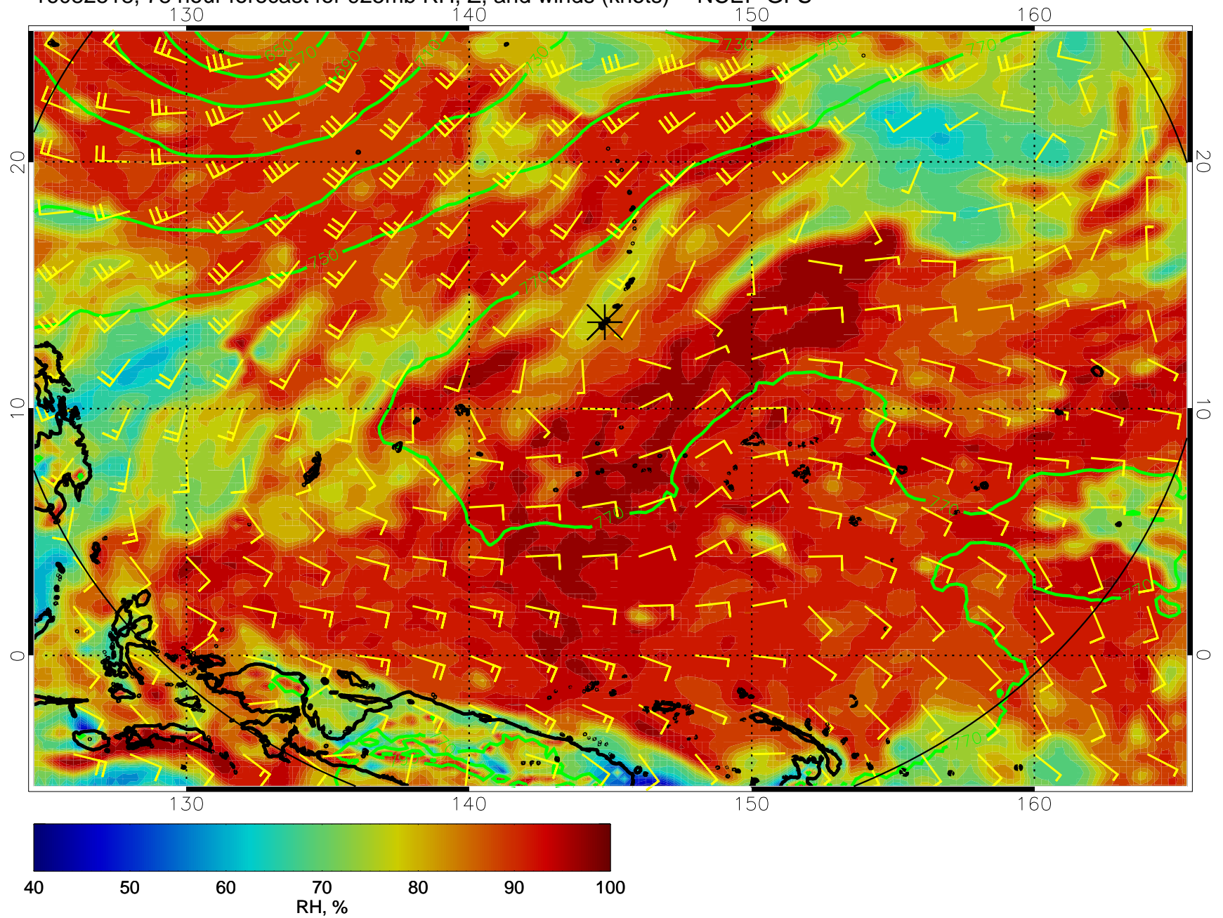
16082518, 78 hour forecast for 925mb RH, Z, and winds (knots) -- NCEP GFS
