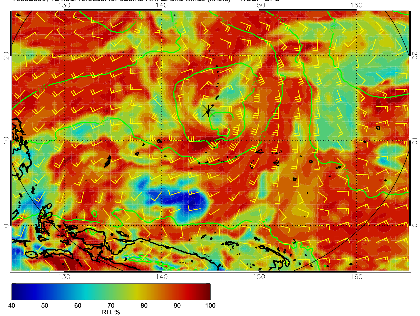
16082300, 12 hour forecast for 925mb RH, Z, and winds (knots) -- NCEP GFS
