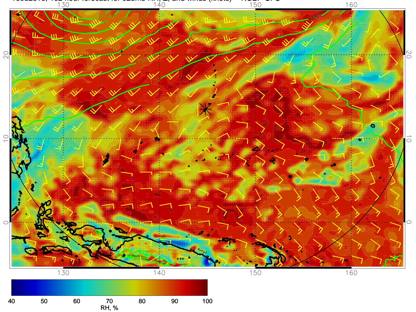
16082618, 102 hour forecast for 925mb RH, Z, and winds (knots) -- NCEP GFS
