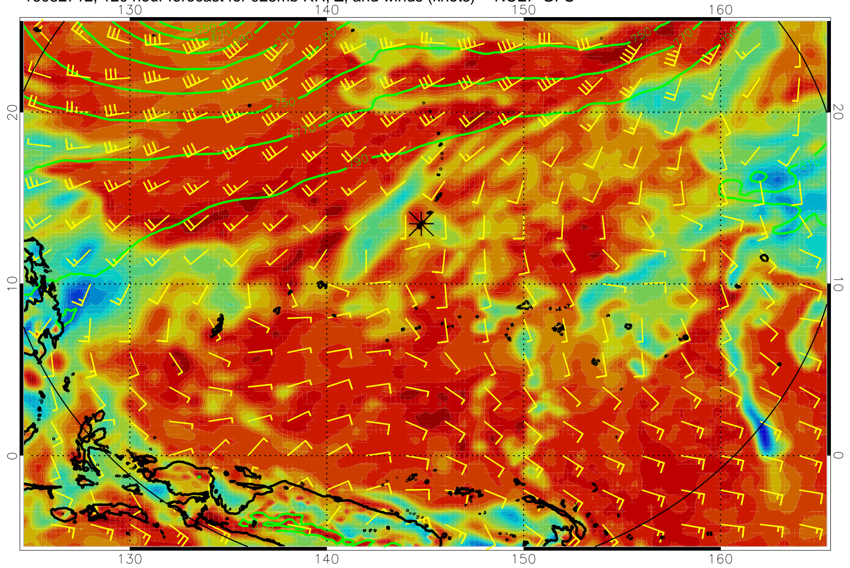
16082712, 120 hour forecast for 925mb RH, Z, and winds (knots) -- NCEP GFS
