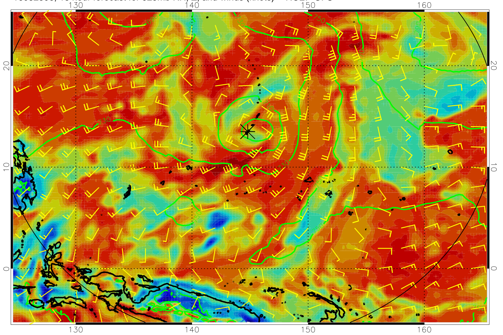
16082306, 18 hour forecast for 925mb RH, Z, and winds (knots) -- NCEP GFS
