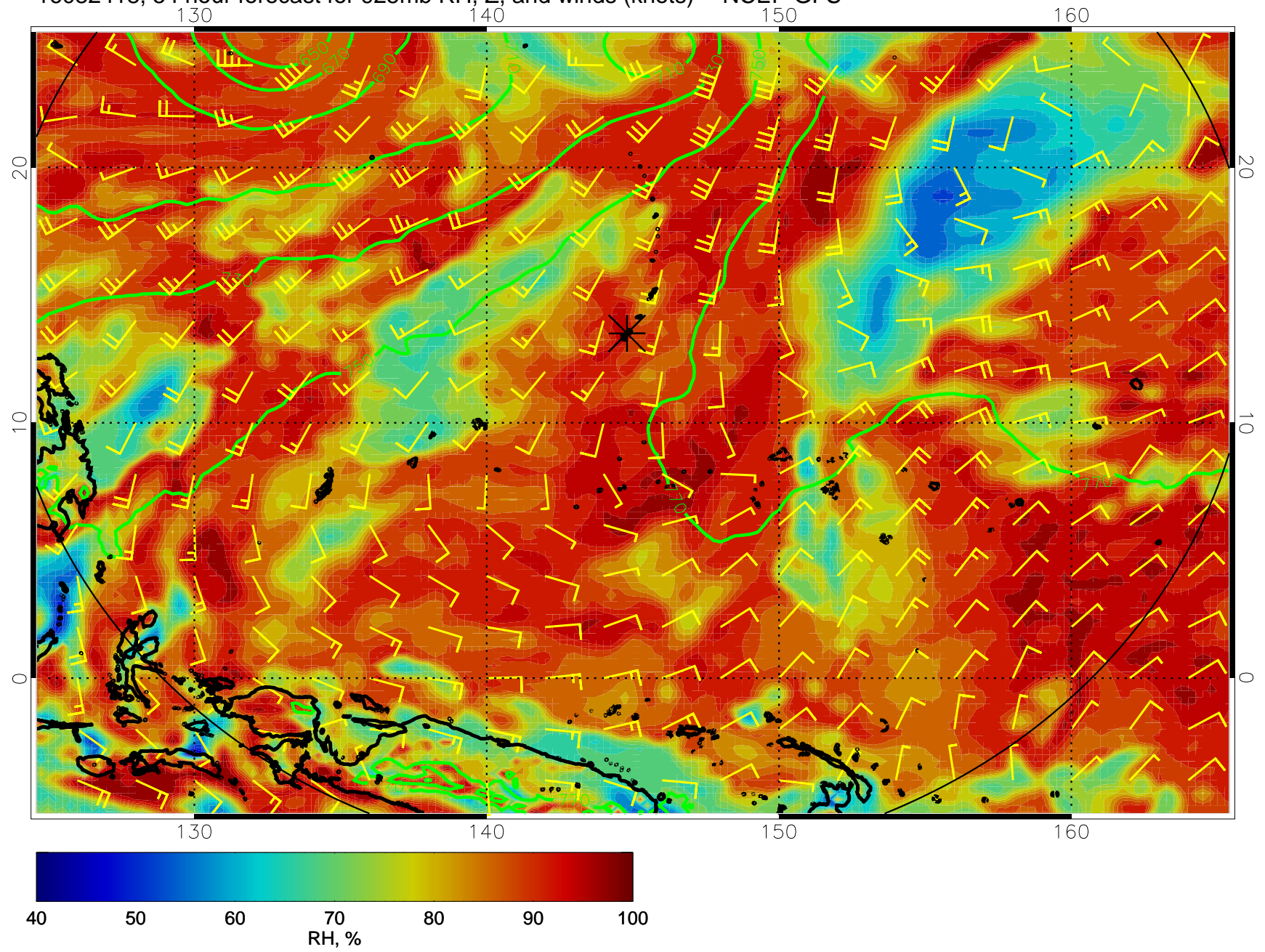
16082418, 54 hour forecast for 925mb RH, Z, and winds (knots) -- NCEP GFS
