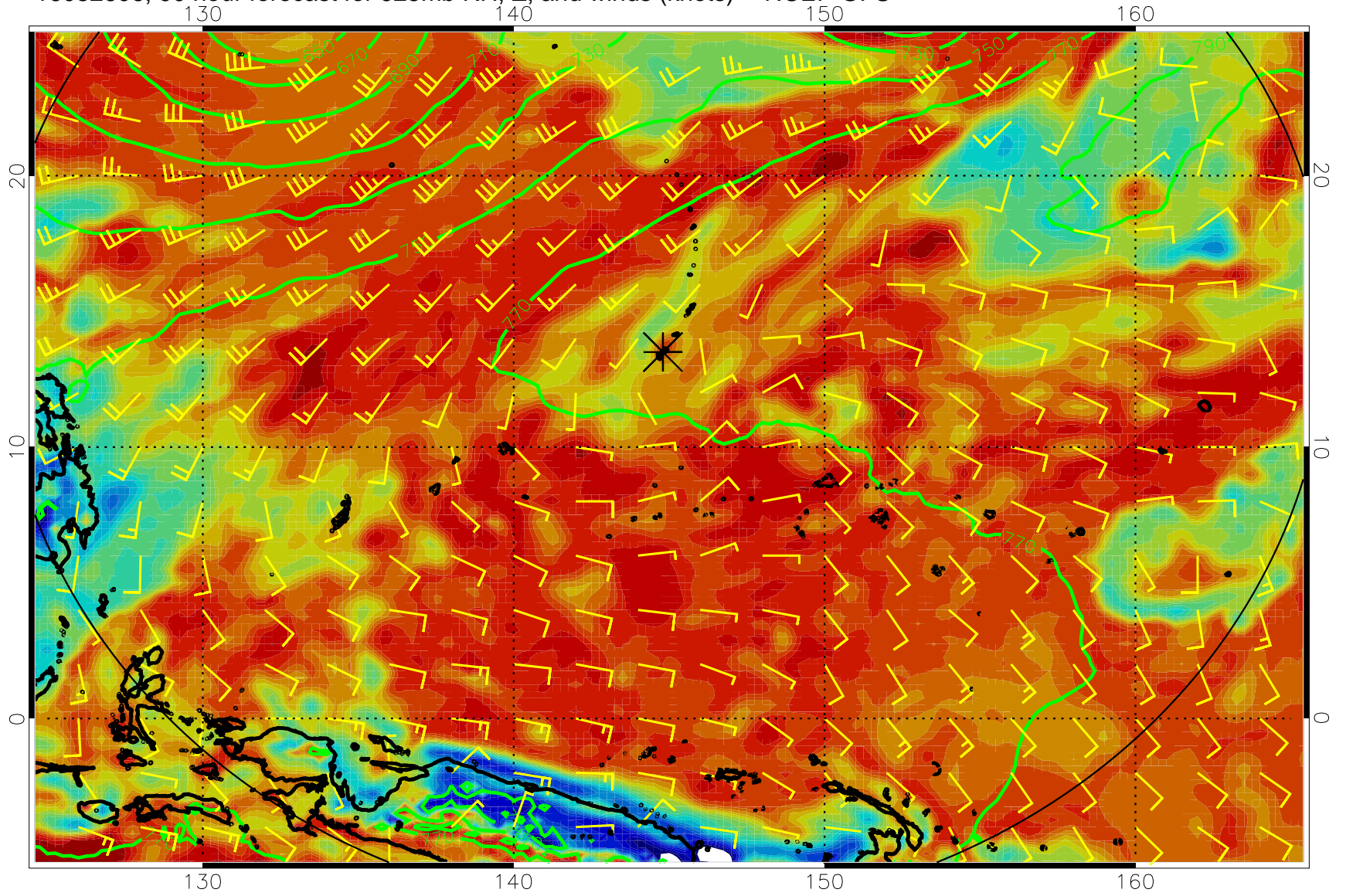
16082606, 90 hour forecast for 925mb RH, Z, and winds (knots) -- NCEP GFS
