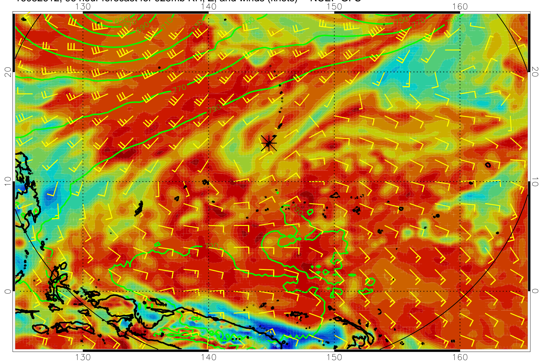
16082612, 96 hour forecast for 925mb RH, Z, and winds (knots) -- NCEP GFS
