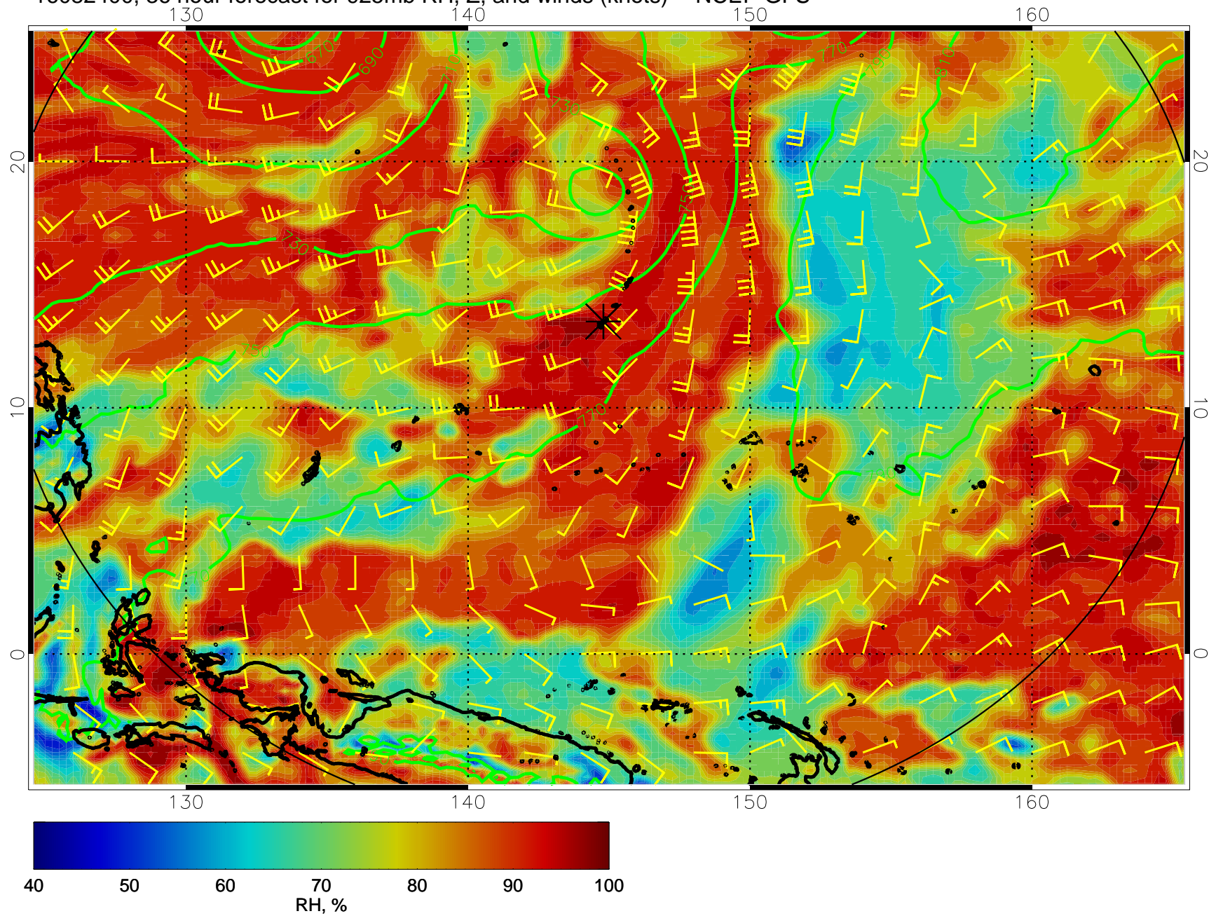
16082400, 36 hour forecast for 925mb RH, Z, and winds (knots) -- NCEP GFS
