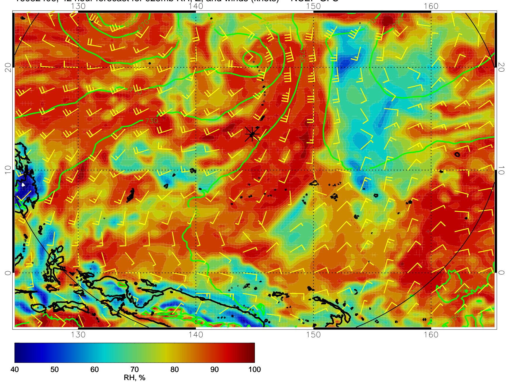
16082406, 42 hour forecast for 925mb RH, Z, and winds (knots) -- NCEP GFS
