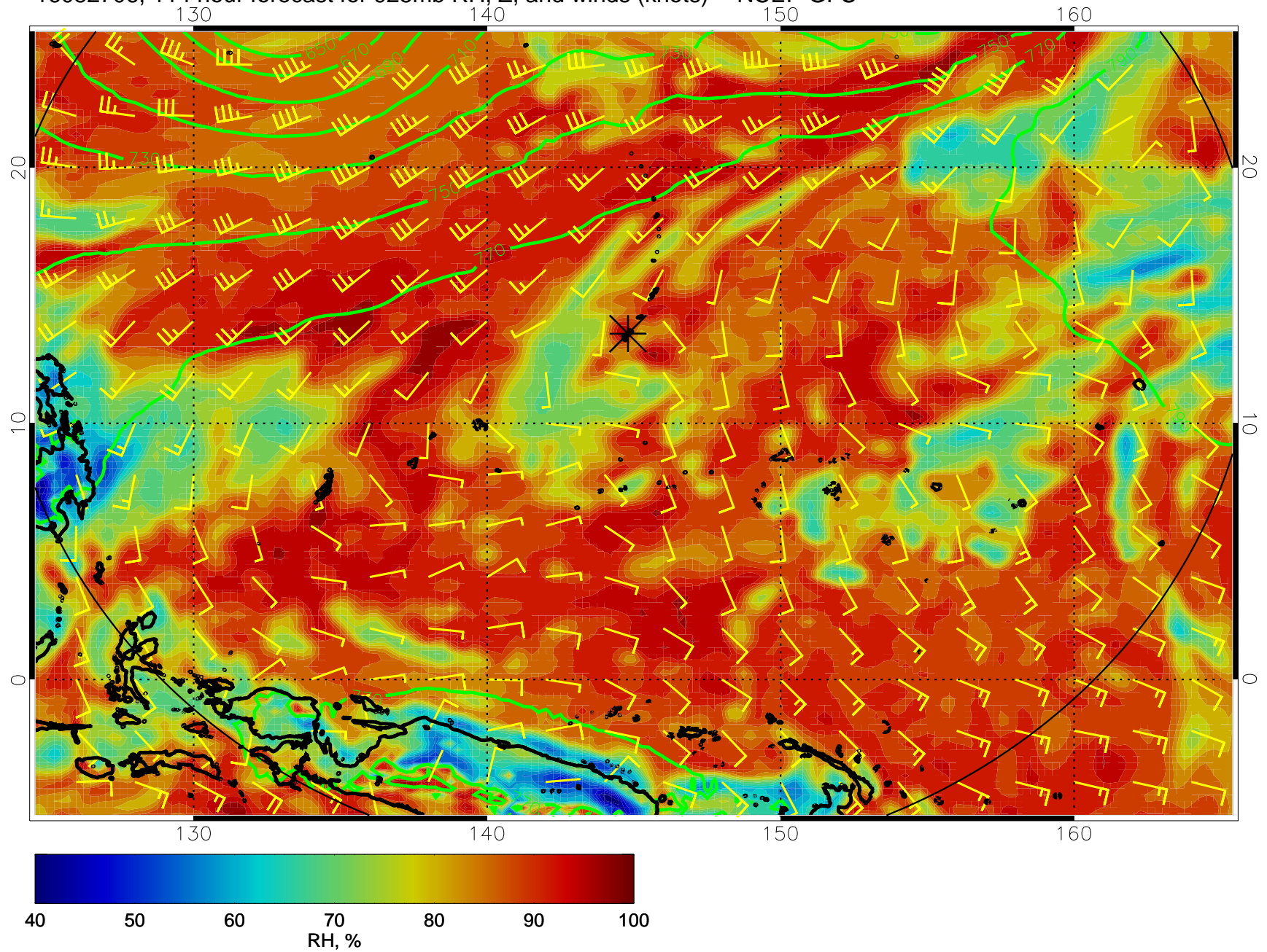
16082706, 114 hour forecast for 925mb RH, Z, and winds (knots) -- NCEP GFS
