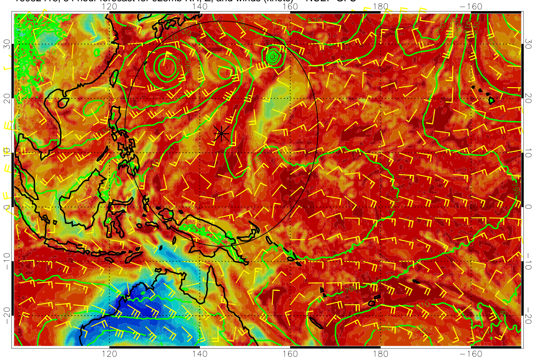
16082418, 54 hour forecast for 925mb RH, Z, and winds (knots) -- NCEP GFS
