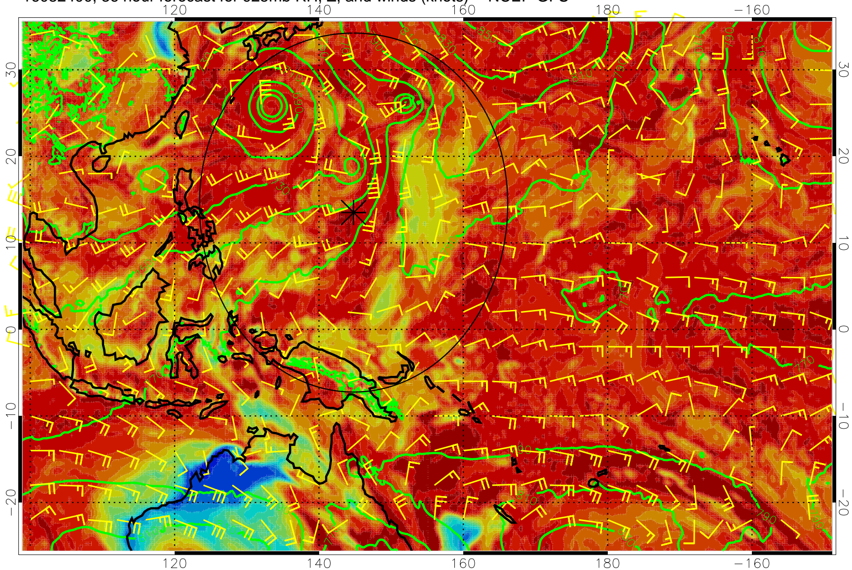
16082400, 36 hour forecast for 925mb RH, Z, and winds (knots) -- NCEP GFS
