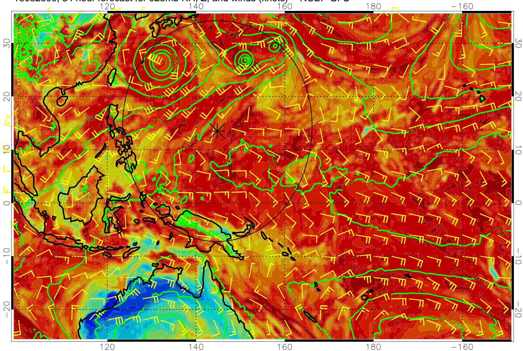
16082600, 84 hour forecast for 925mb RH, Z, and winds (knots) -- NCEP GFS
