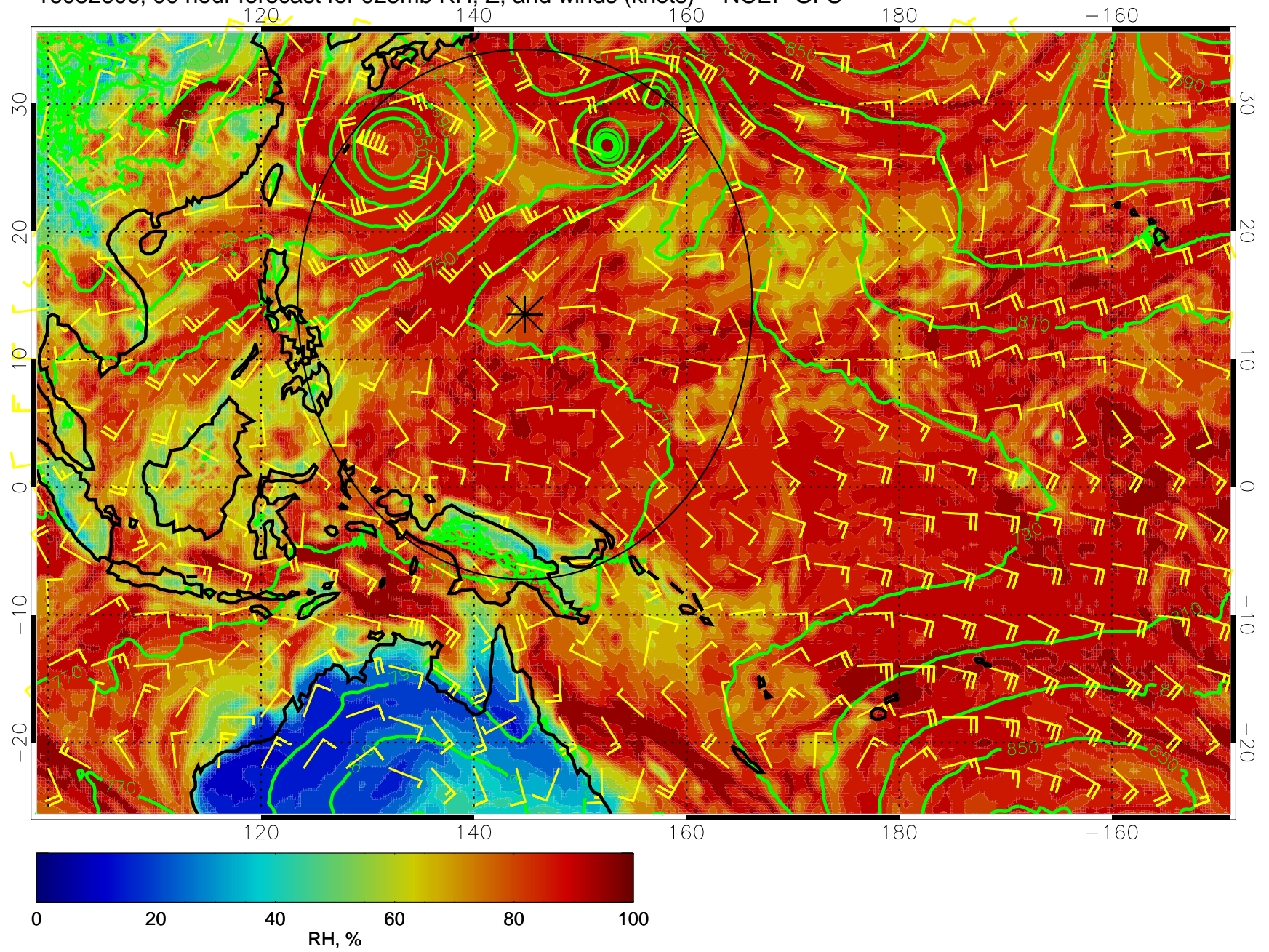
16082606, 90 hour forecast for 925mb RH, Z, and winds (knots) -- NCEP GFS
