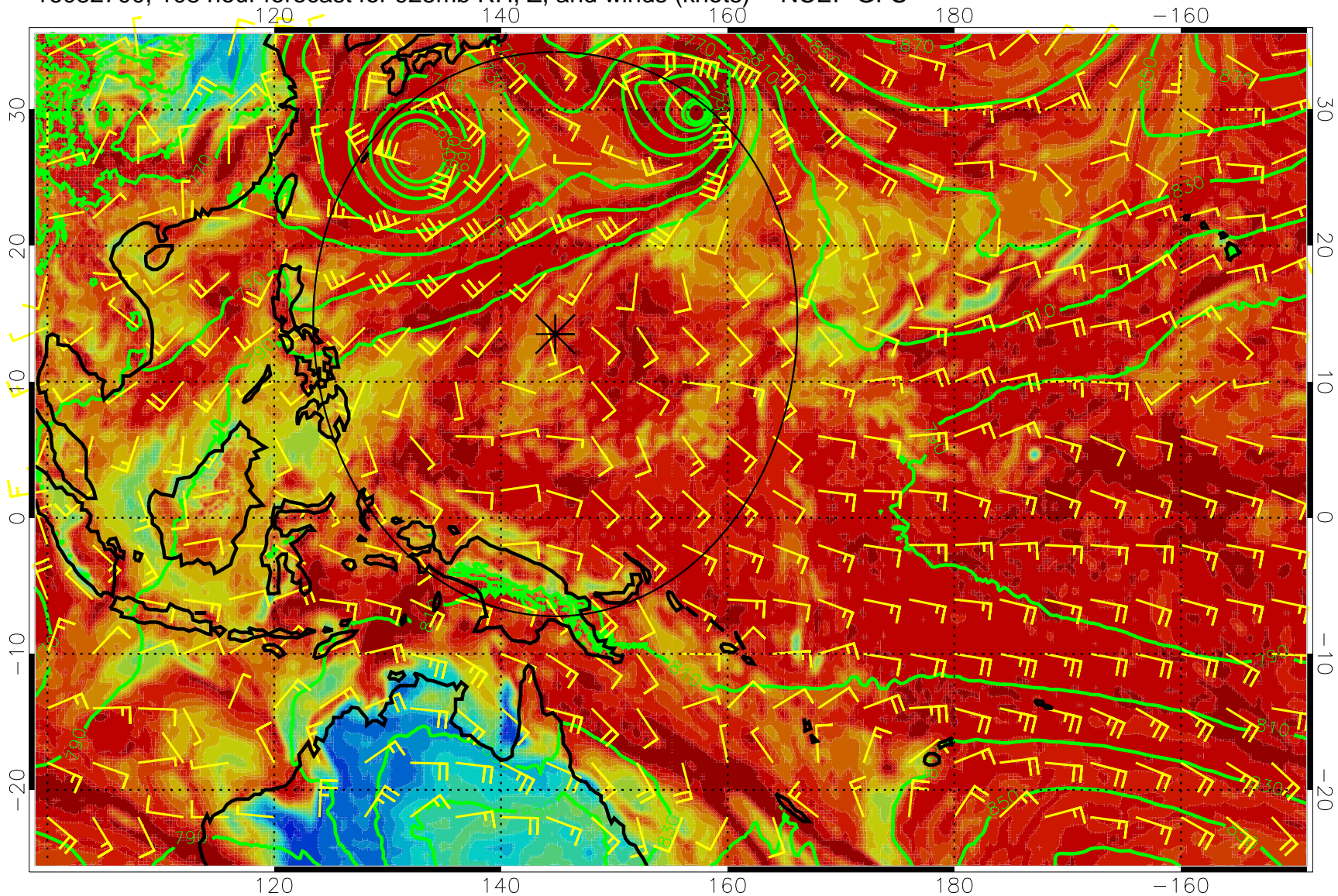
16082700, 108 hour forecast for 925mb RH, Z, and winds (knots) -- NCEP GFS
