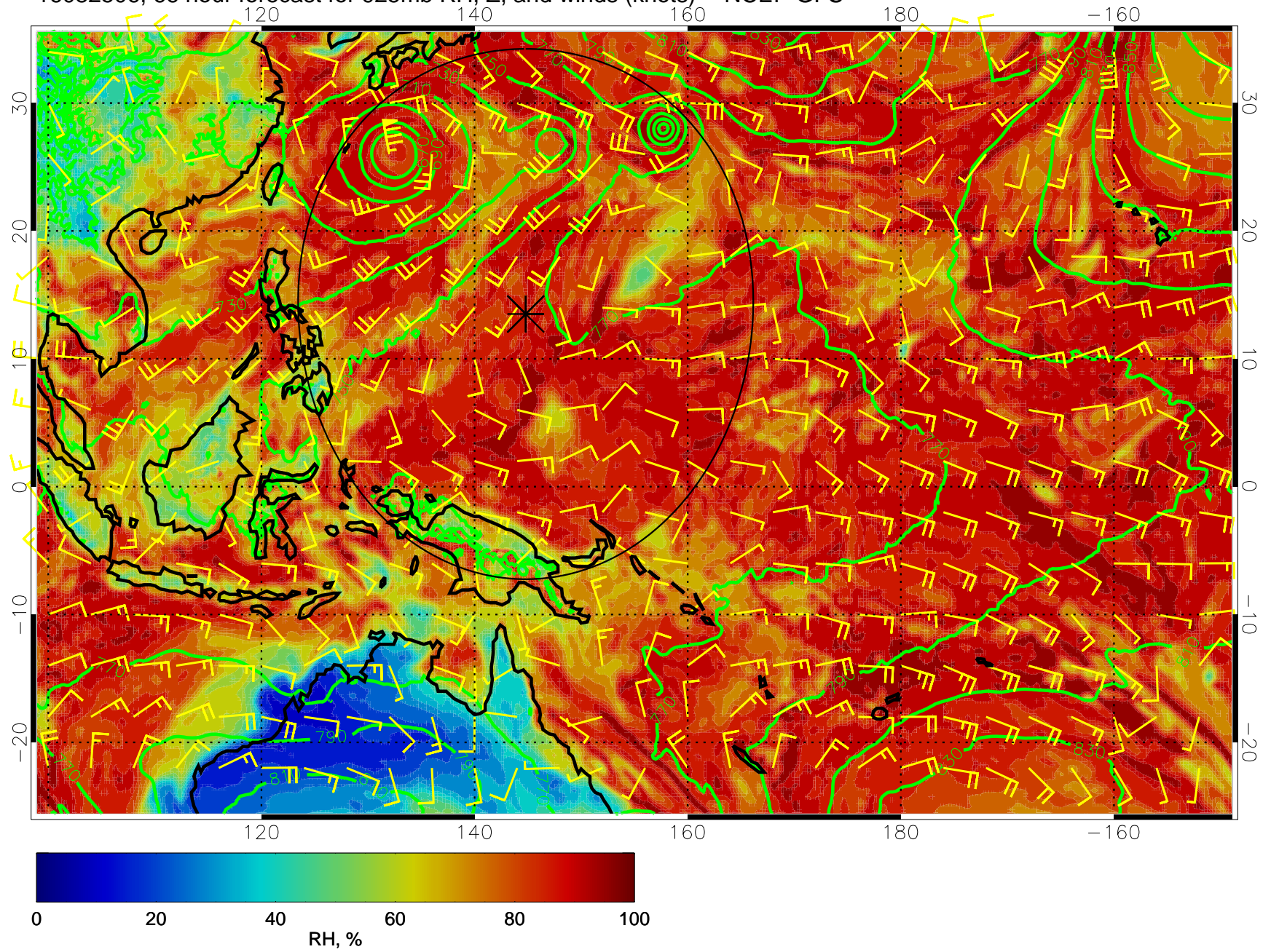
16082506, 66 hour forecast for 925mb RH, Z, and winds (knots) -- NCEP GFS
