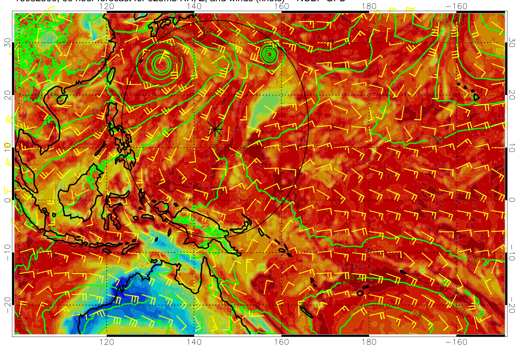
16082500, 60 hour forecast for 925mb RH, Z, and winds (knots) -- NCEP GFS
