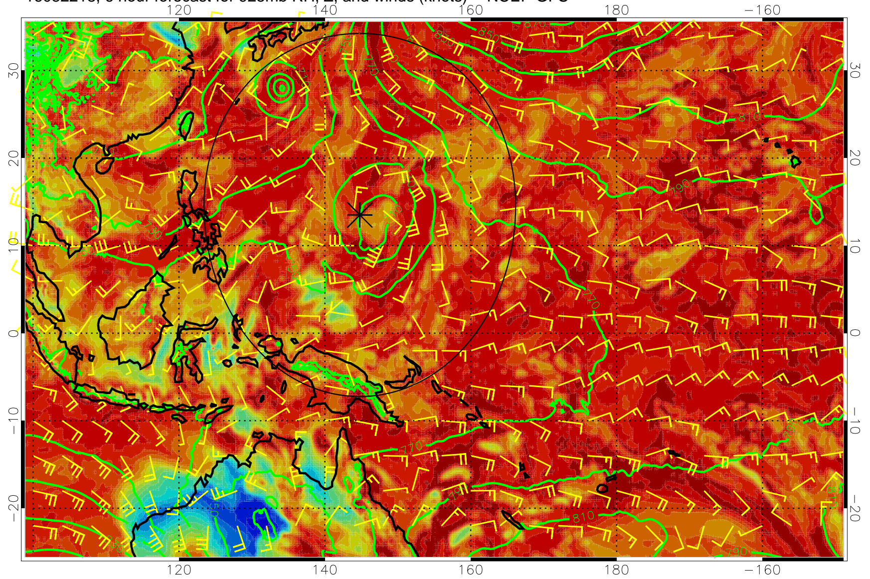
16082218, 6 hour forecast for 925mb RH, Z, and winds (knots) -- NCEP GFS
