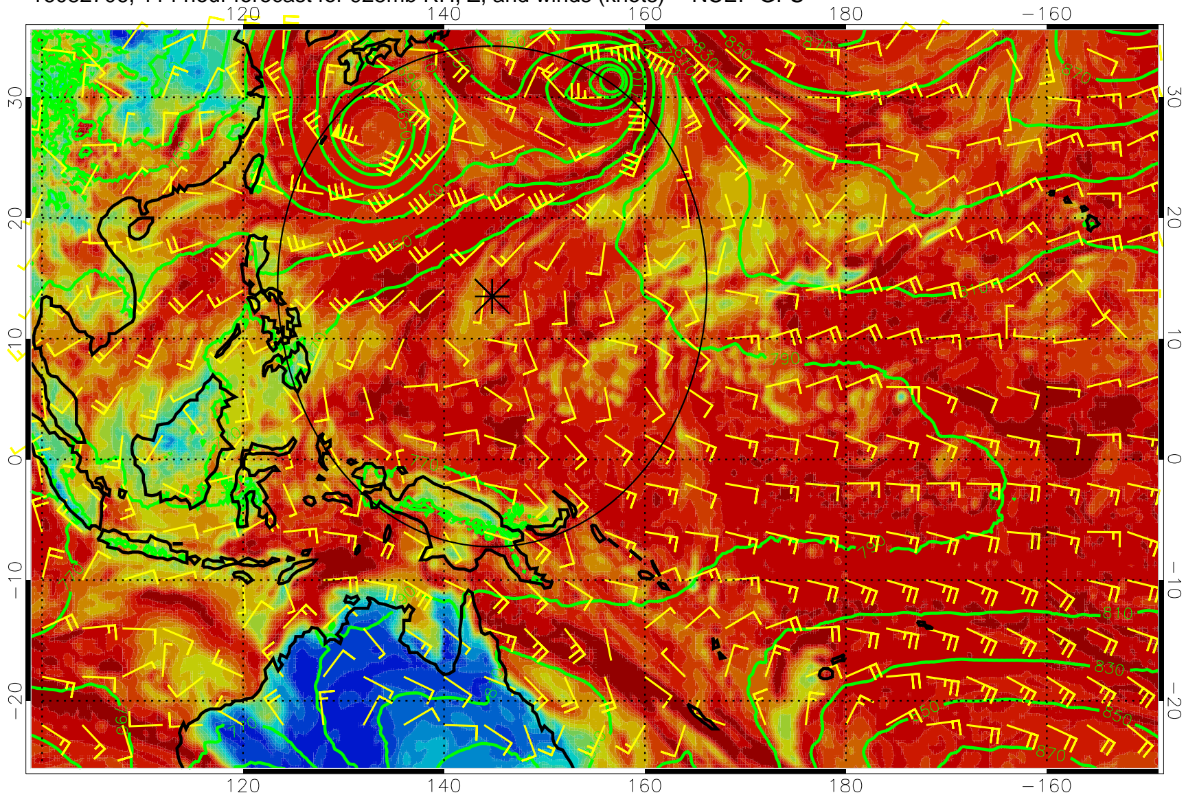
16082706, 114 hour forecast for 925mb RH, Z, and winds (knots) -- NCEP GFS
