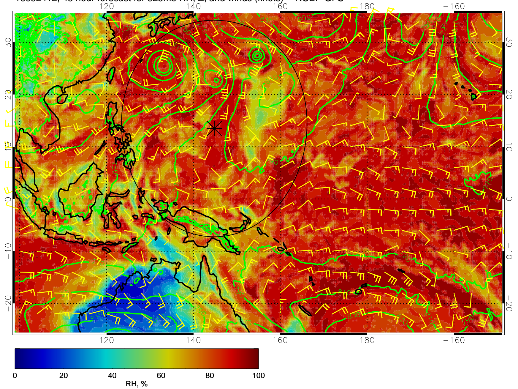
16082412, 48 hour forecast for 925mb RH, Z, and winds (knots) -- NCEP GFS
