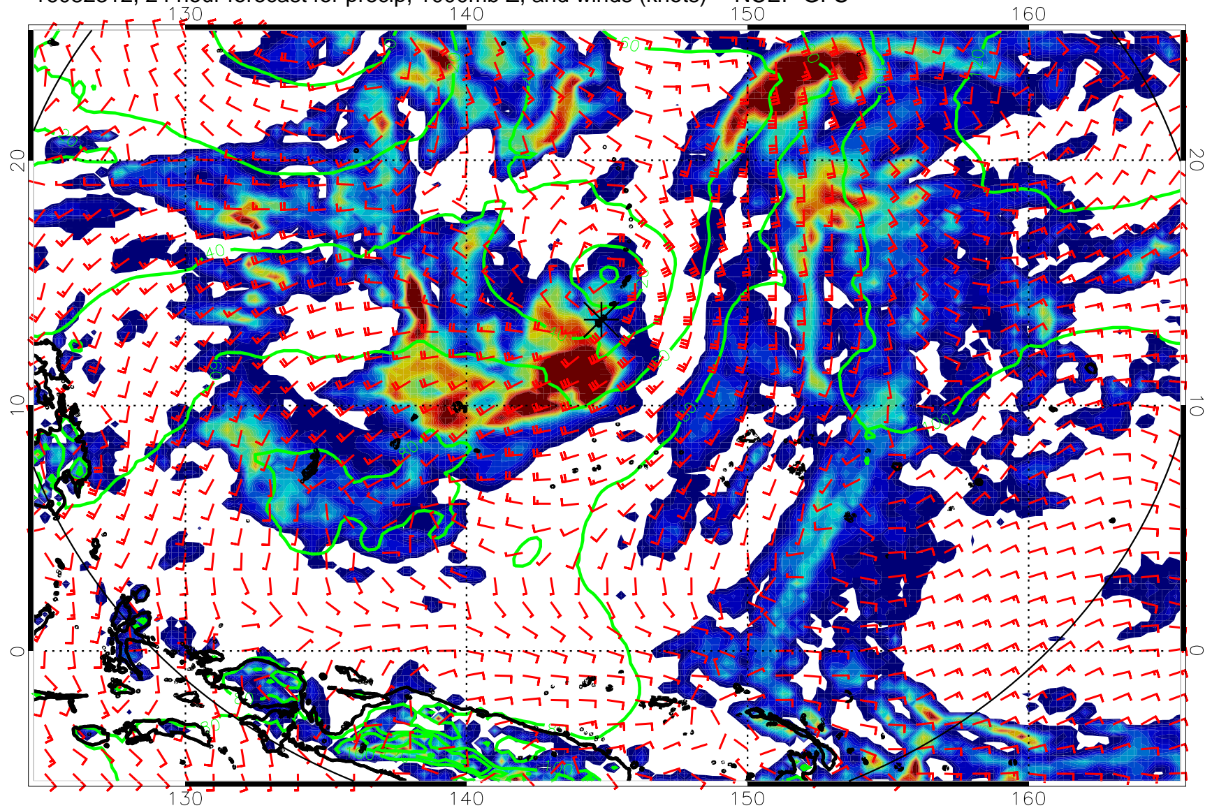
16082312, 24 hour forecast for precip, 1000mb Z, and winds (knots) -- NCEP GFS
