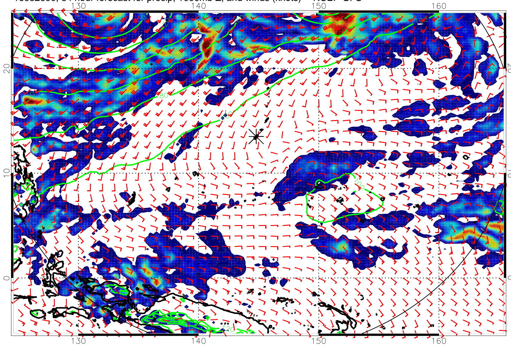
16082600, 84 hour forecast for precip, 1000mb Z, and winds (knots) -- NCEP GFS
