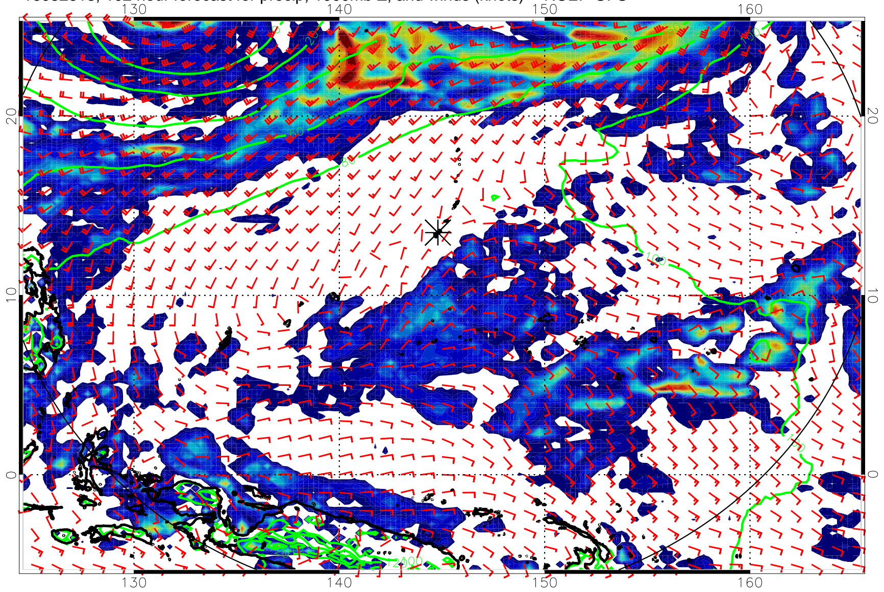
16082618, 102 hour forecast for precip, 1000mb Z, and winds (knots) -- NCEP GFS
