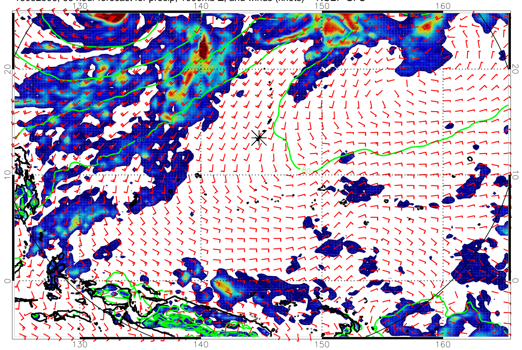
16082506, 66 hour forecast for precip, 1000mb Z, and winds (knots) -- NCEP GFS
