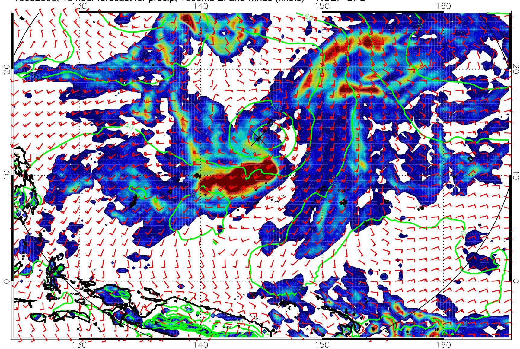
16082306, 18 hour forecast for precip, 1000mb Z, and winds (knots) -- NCEP GFS
