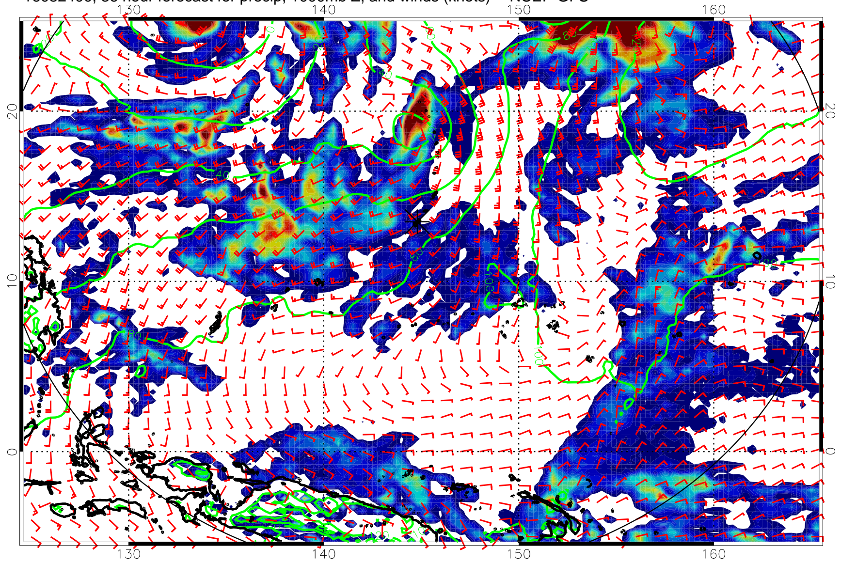
16082400, 36 hour forecast for precip, 1000mb Z, and winds (knots) -- NCEP GFS
