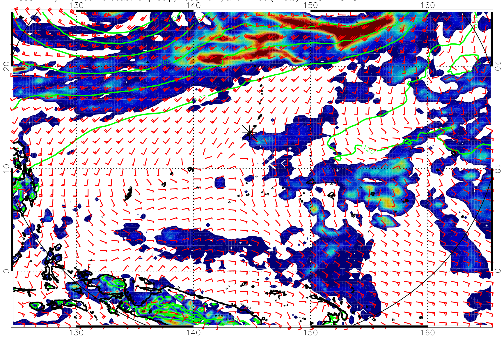
16082712, 120 hour forecast for precip, 1000mb Z, and winds (knots) -- NCEP GFS
