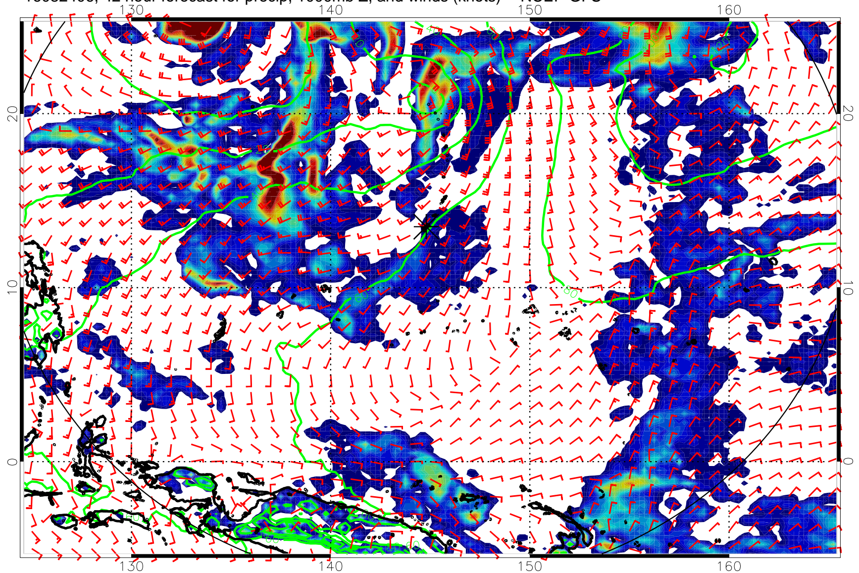
16082406, 42 hour forecast for precip, 1000mb Z, and winds (knots) -- NCEP GFS
