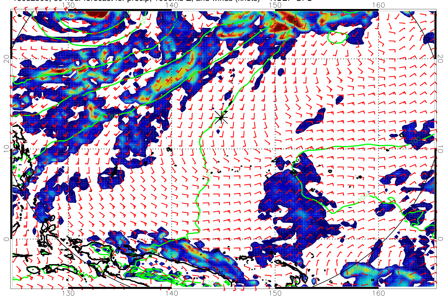
16082500, 60 hour forecast for precip, 1000mb Z, and winds (knots) -- NCEP GFS
