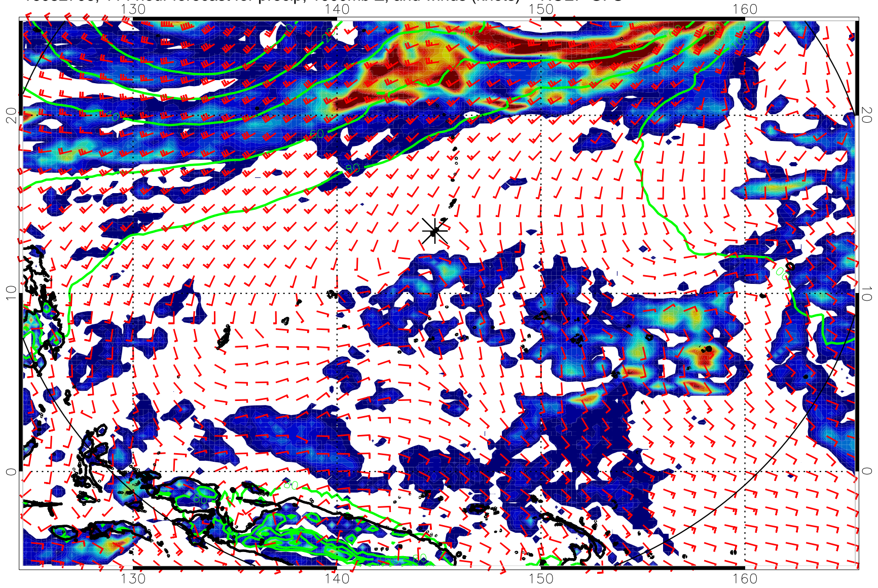
16082706, 114 hour forecast for precip, 1000mb Z, and winds (knots) -- NCEP GFS
