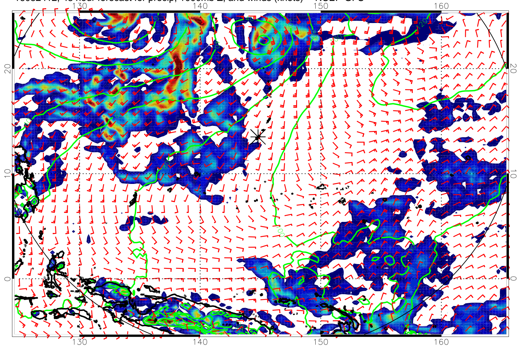
16082412, 48 hour forecast for precip, 1000mb Z, and winds (knots) -- NCEP GFS
