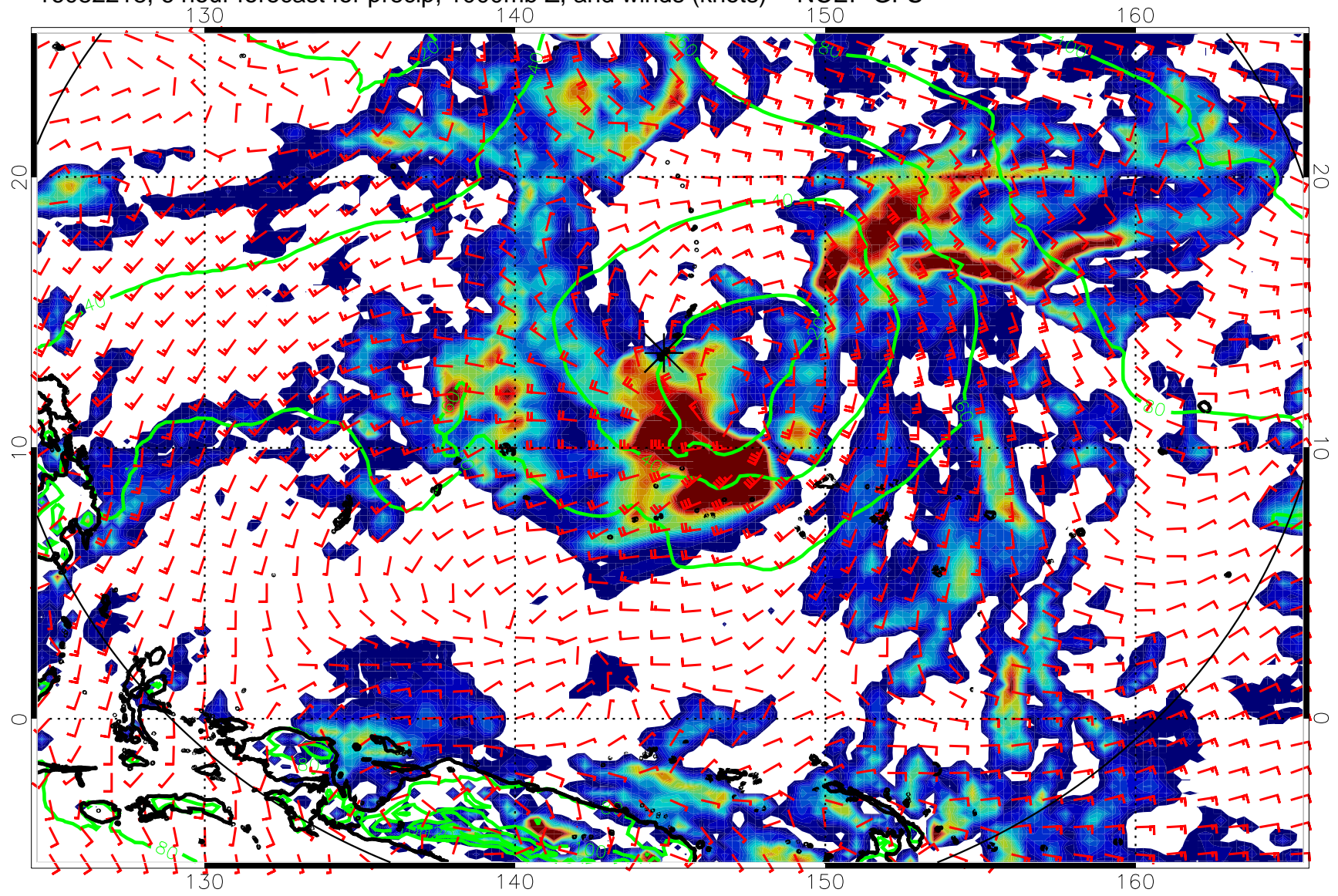
16082218, 6 hour forecast for precip, 1000mb Z, and winds (knots) -- NCEP GFS
