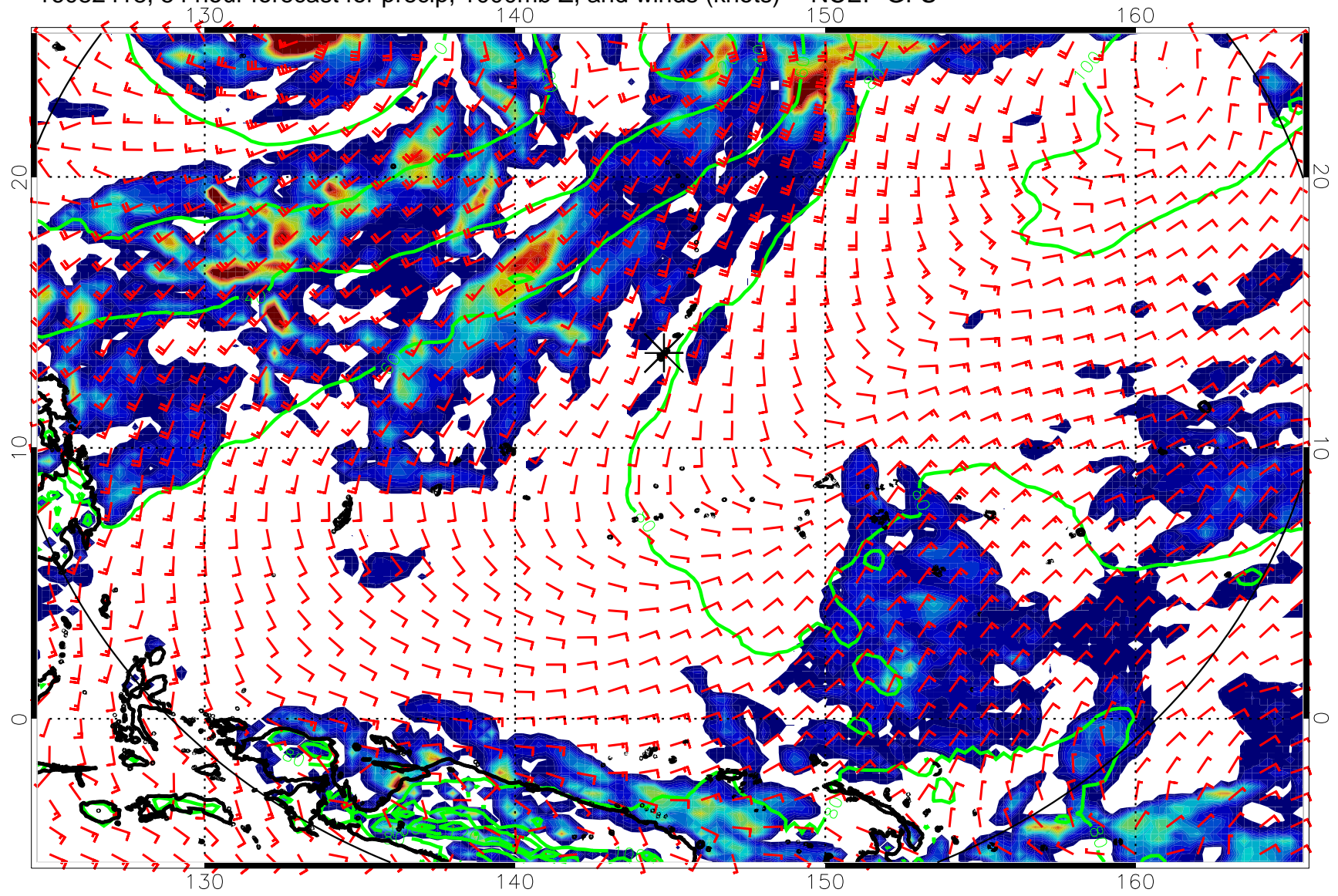
16082418, 54 hour forecast for precip, 1000mb Z, and winds (knots) -- NCEP GFS
