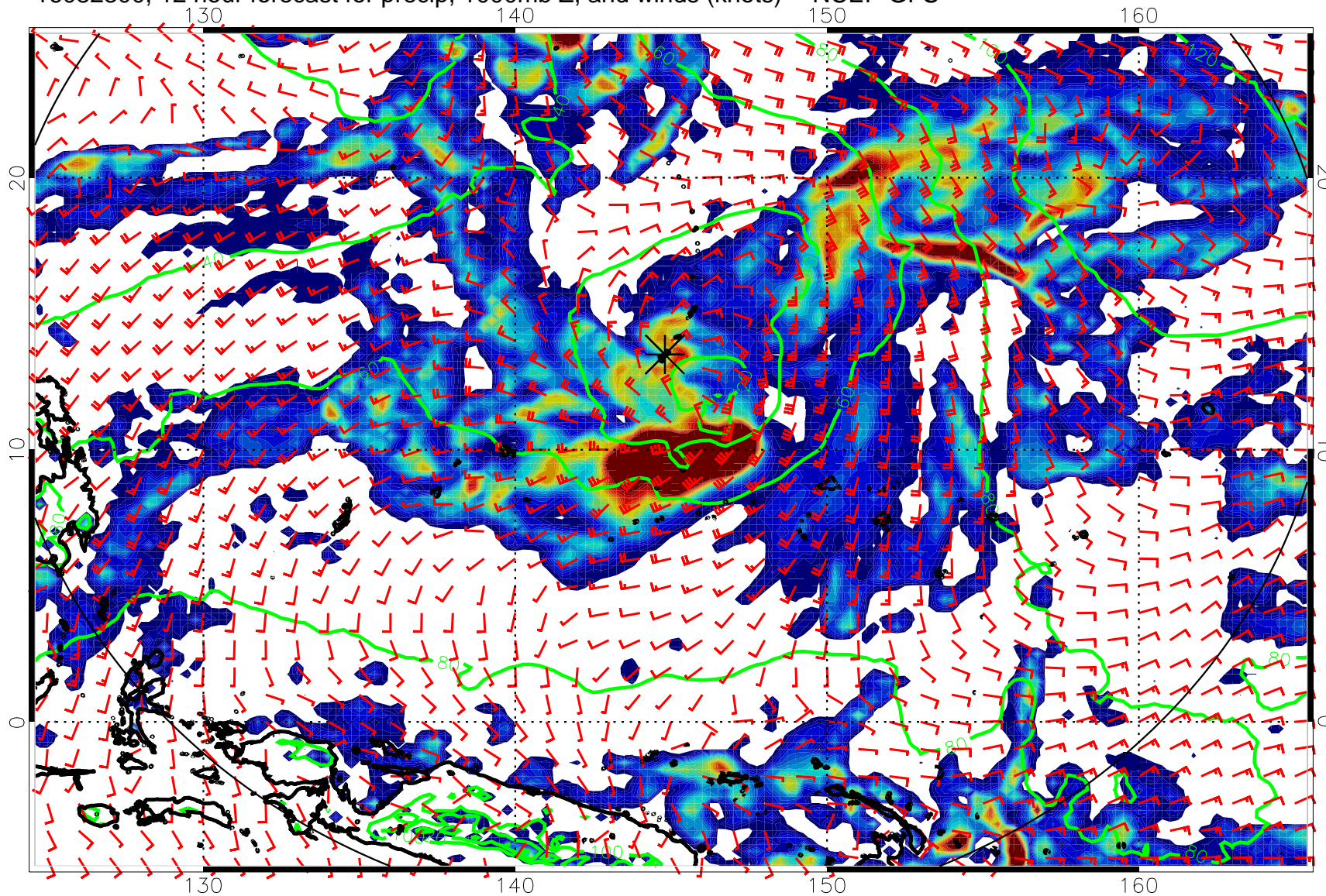
16082300, 12 hour forecast for precip, 1000mb Z, and winds (knots) -- NCEP GFS
