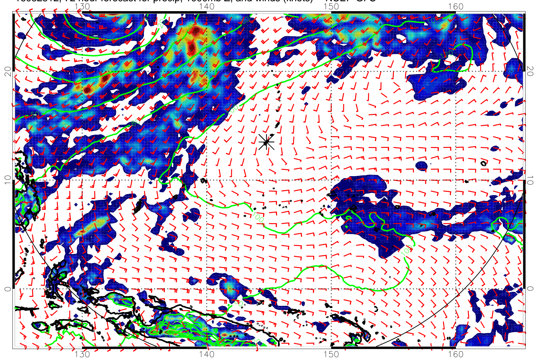
16082512, 72 hour forecast for precip, 1000mb Z, and winds (knots) -- NCEP GFS
