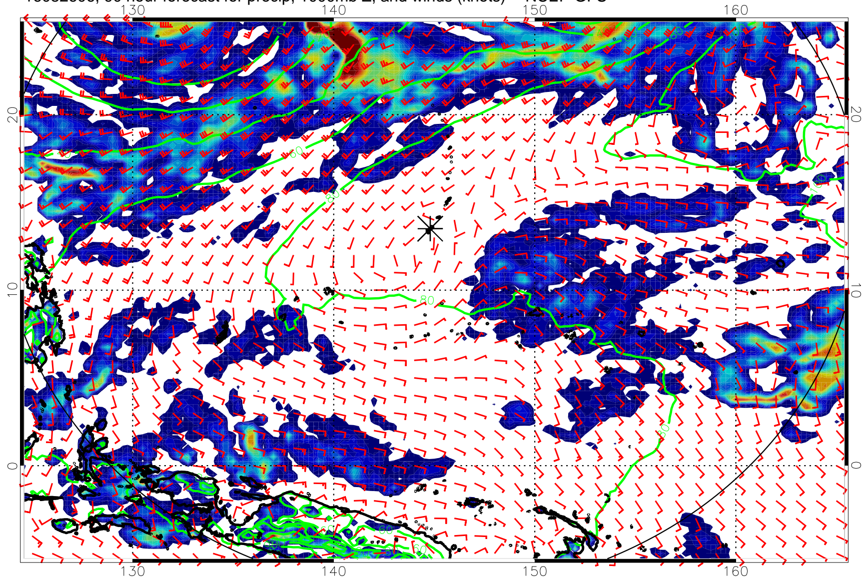
16082606, 90 hour forecast for precip, 1000mb Z, and winds (knots) -- NCEP GFS
