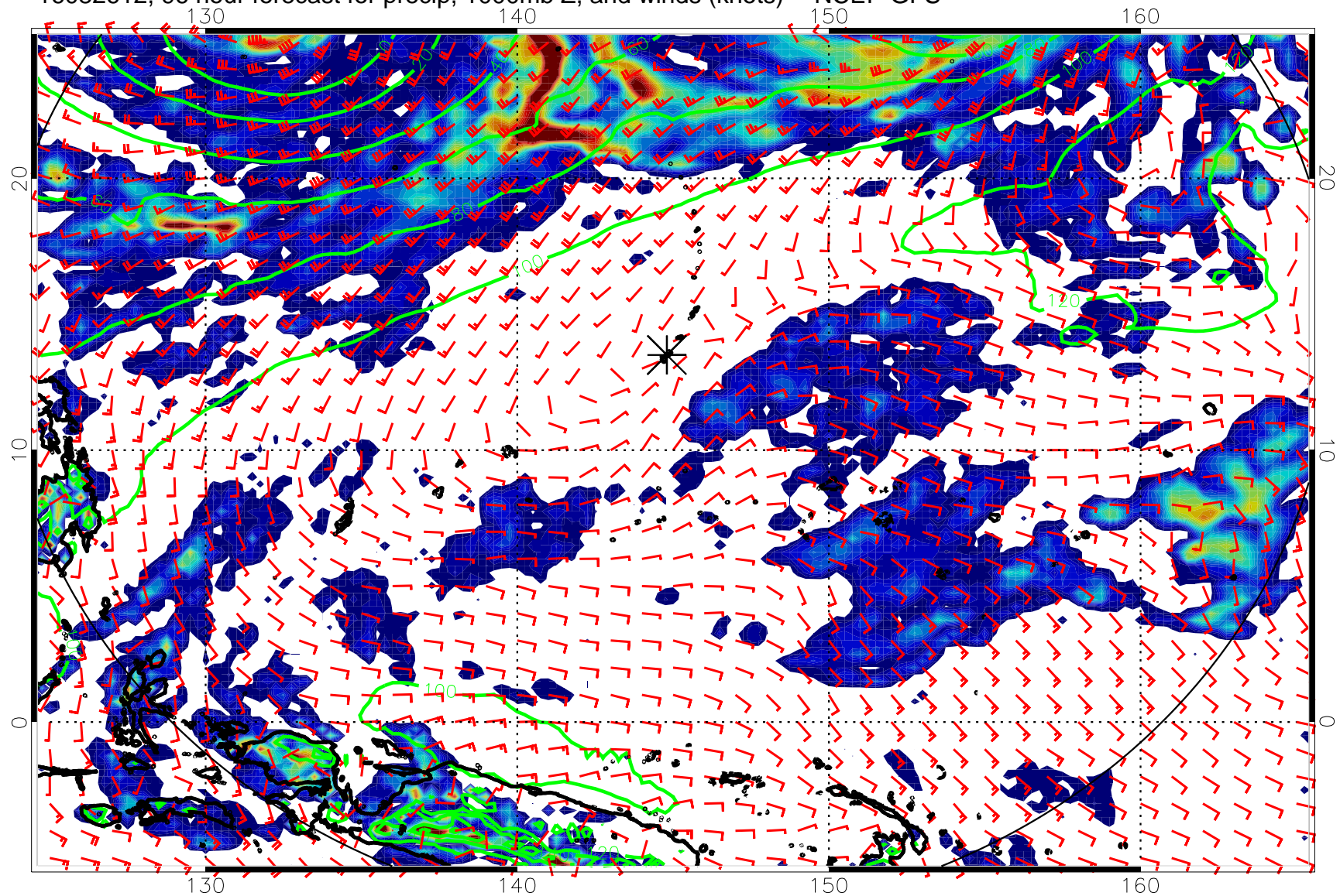
16082612, 96 hour forecast for precip, 1000mb Z, and winds (knots) -- NCEP GFS
