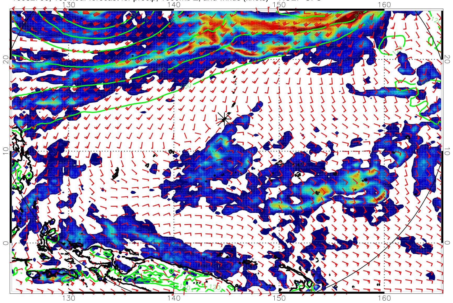
16082700, 108 hour forecast for precip, 1000mb Z, and winds (knots) -- NCEP GFS
