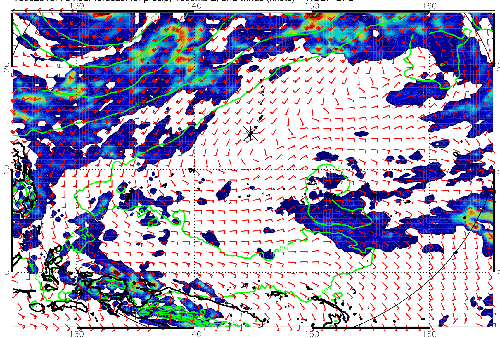
16082518, 78 hour forecast for precip, 1000mb Z, and winds (knots) -- NCEP GFS
