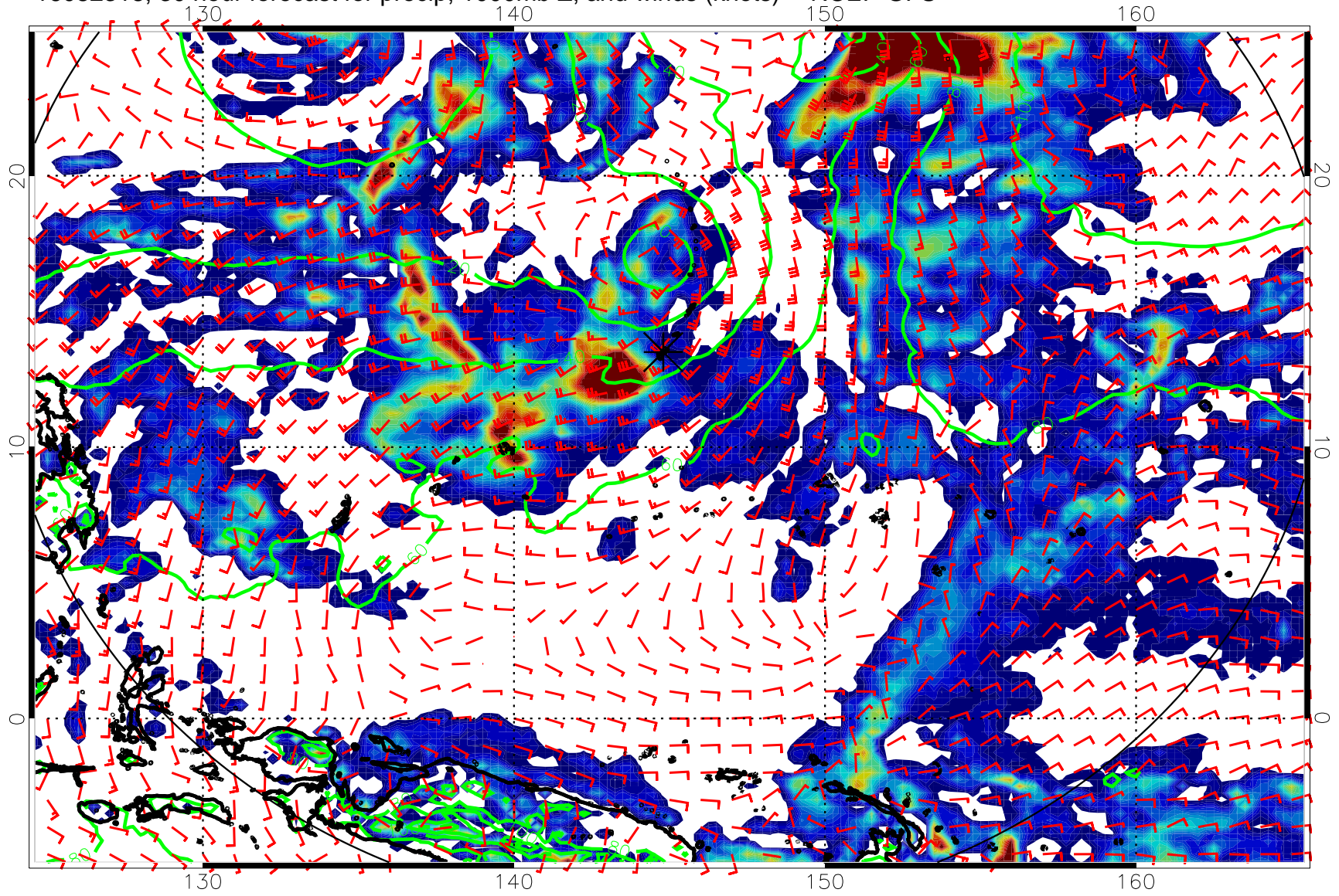
16082318, 30 hour forecast for precip, 1000mb Z, and winds (knots) -- NCEP GFS
