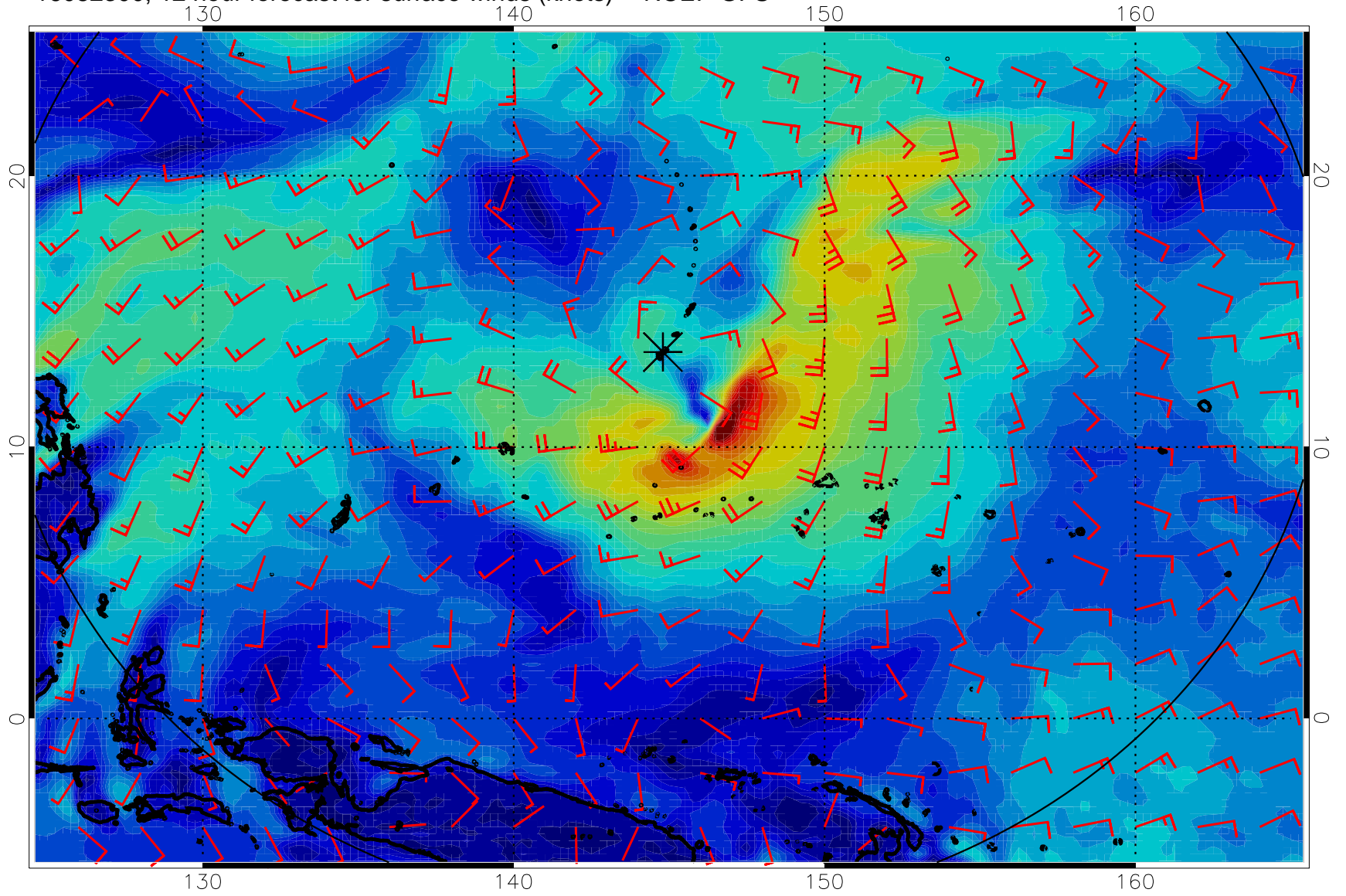
16082300, 12 hour forecast for surface winds (knots) -- NCEP GFS
