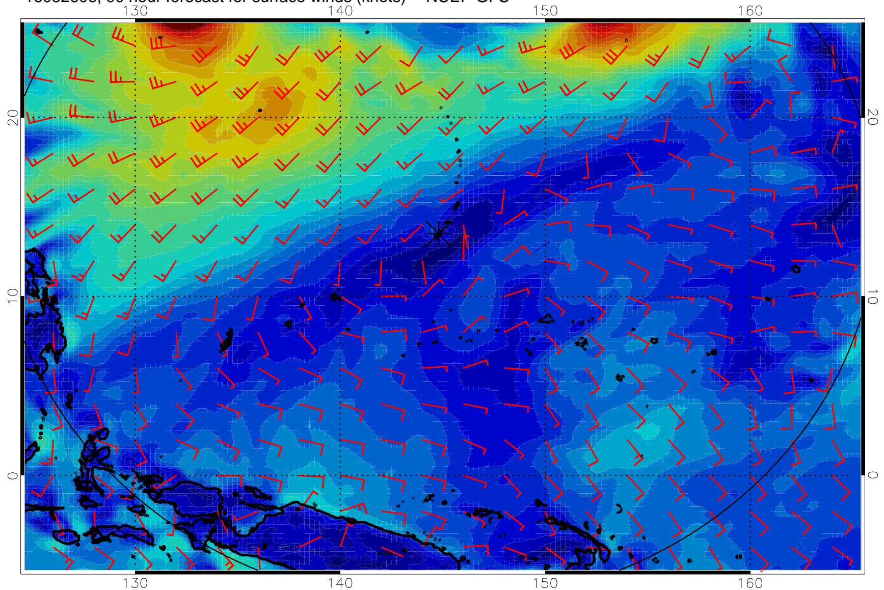
16082606, 90 hour forecast for surface winds (knots) -- NCEP GFS
