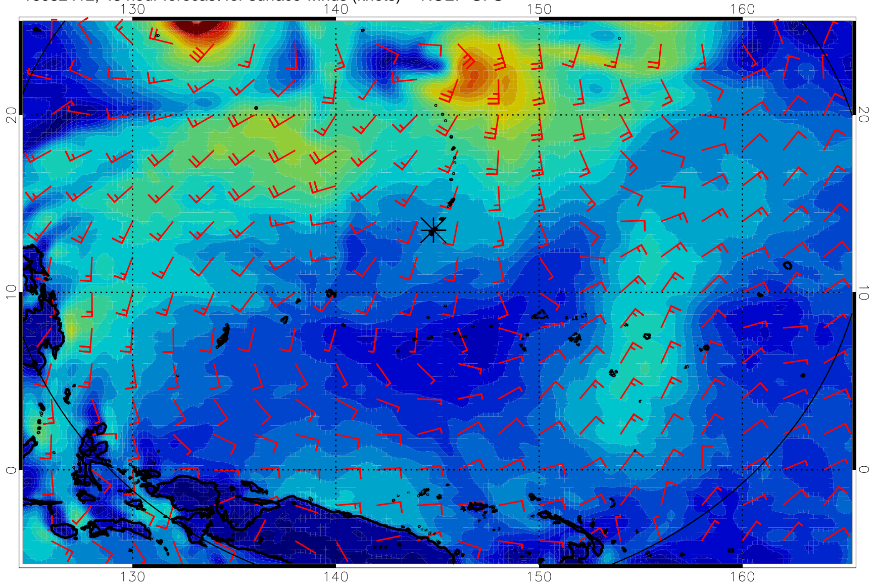
16082412, 48 hour forecast for surface winds (knots) -- NCEP GFS
