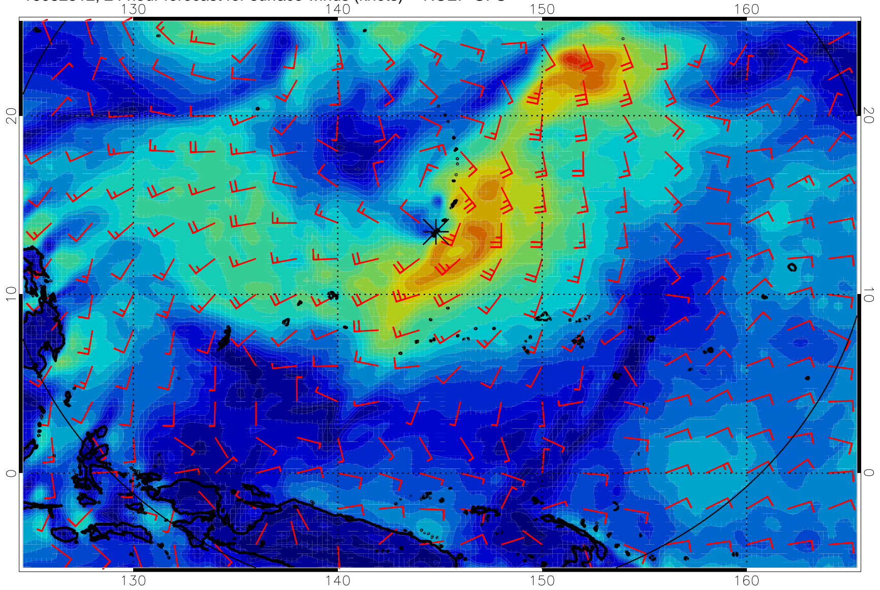
16082312, 24 hour forecast for surface winds (knots) -- NCEP GFS
