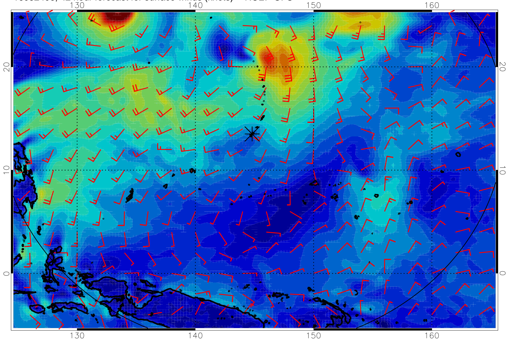
16082406, 42 hour forecast for surface winds (knots) -- NCEP GFS
