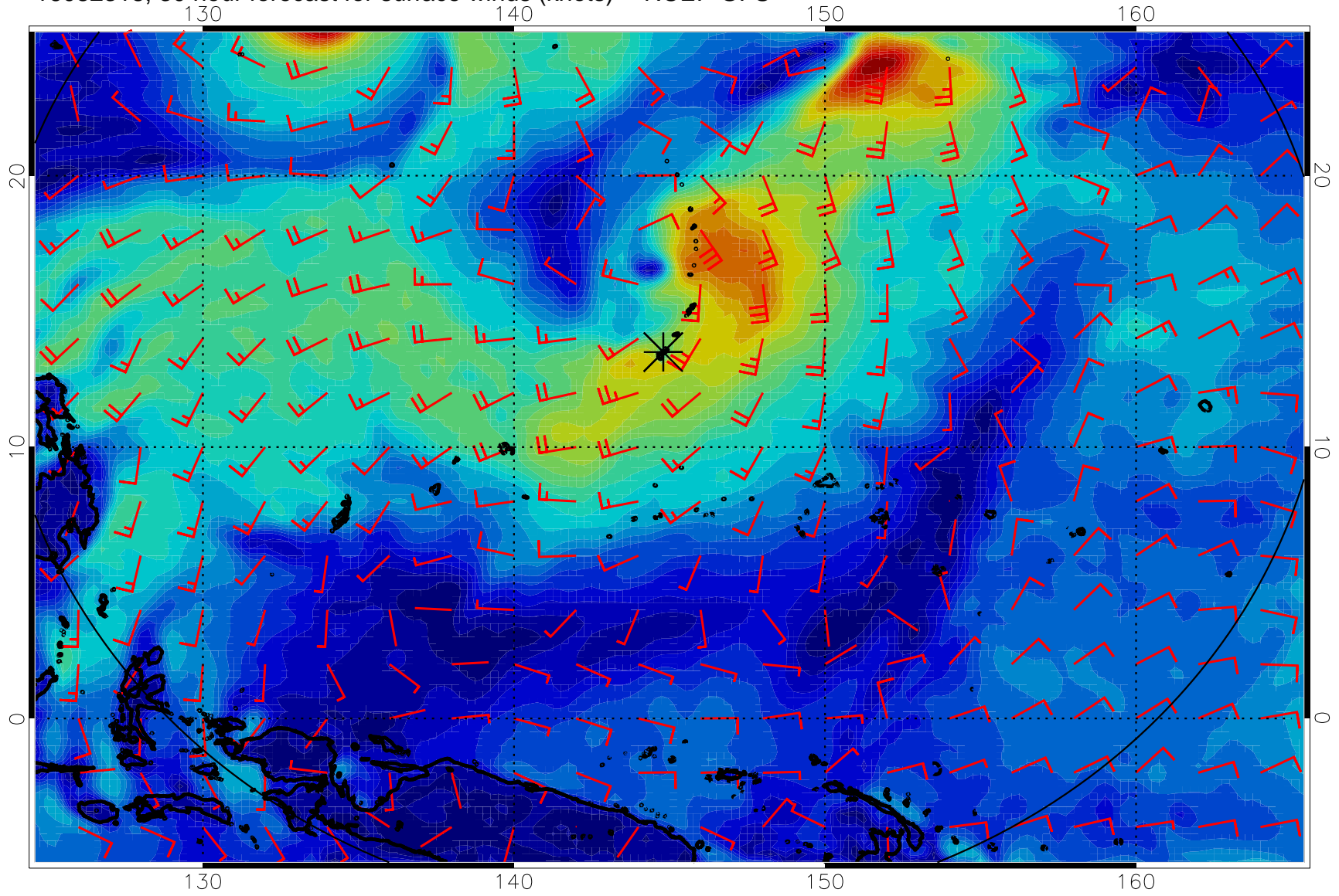
16082318, 30 hour forecast for surface winds (knots) -- NCEP GFS
