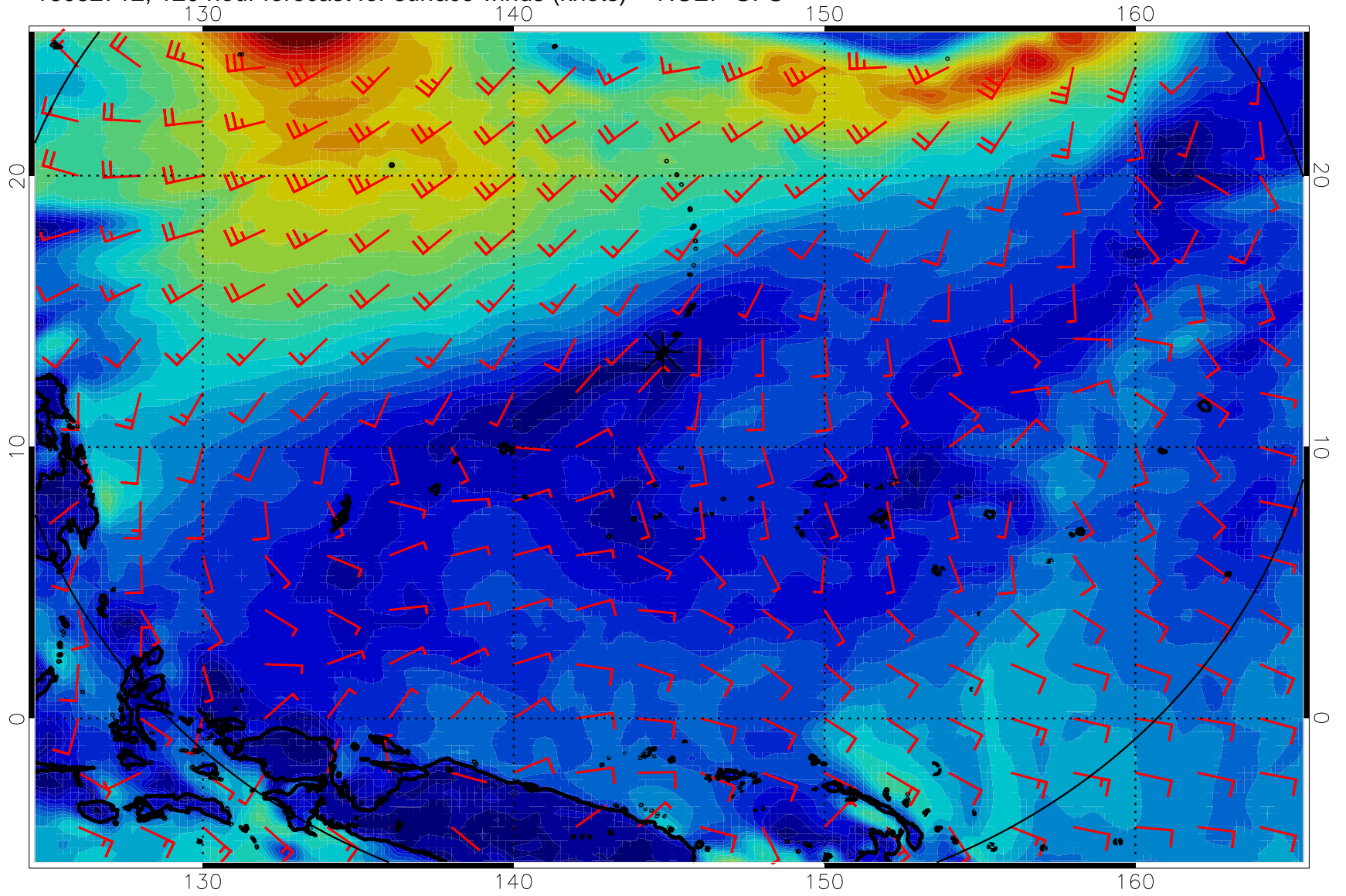
16082712, 120 hour forecast for surface winds (knots) -- NCEP GFS
