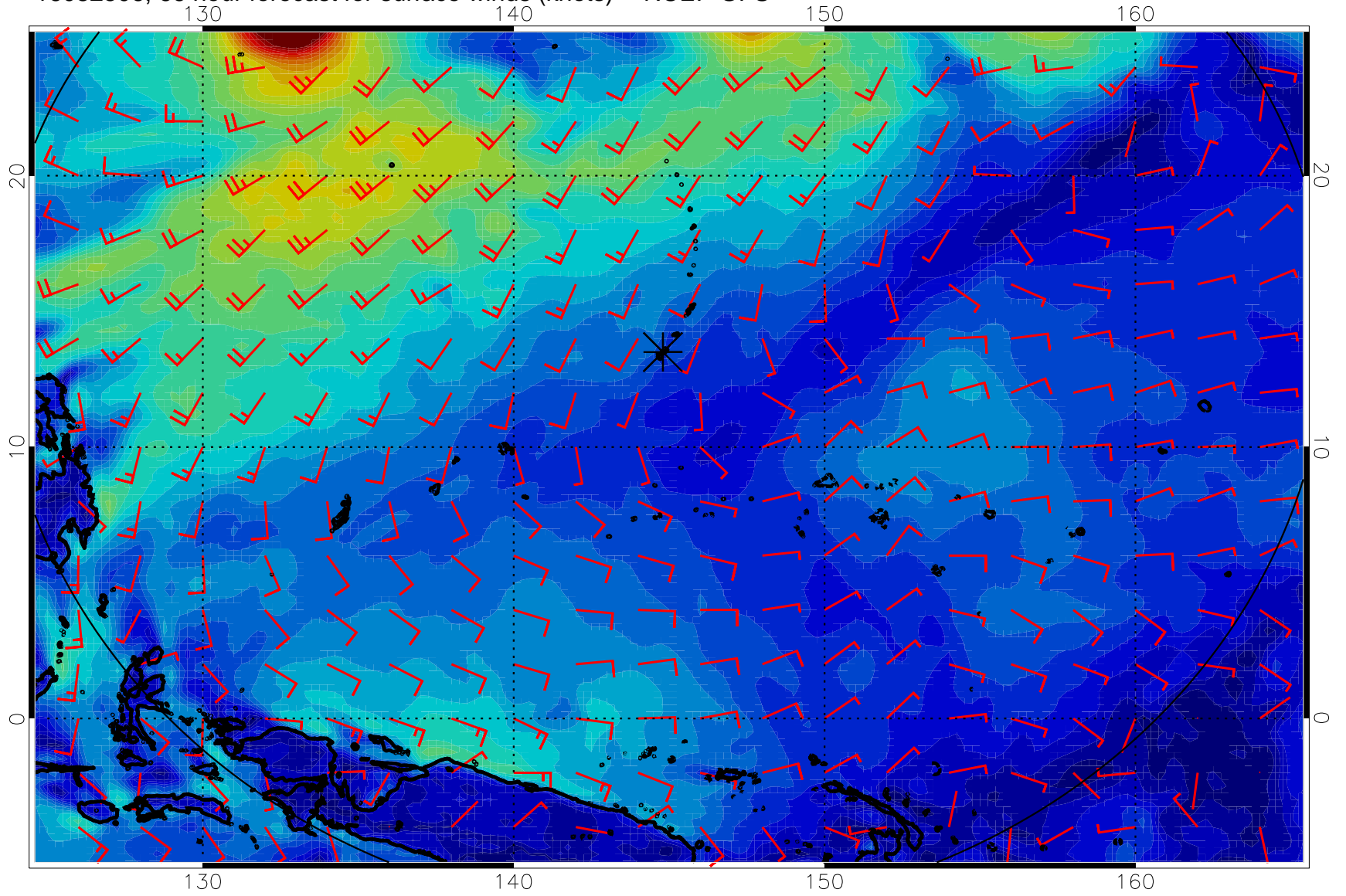
16082506, 66 hour forecast for surface winds (knots) -- NCEP GFS
