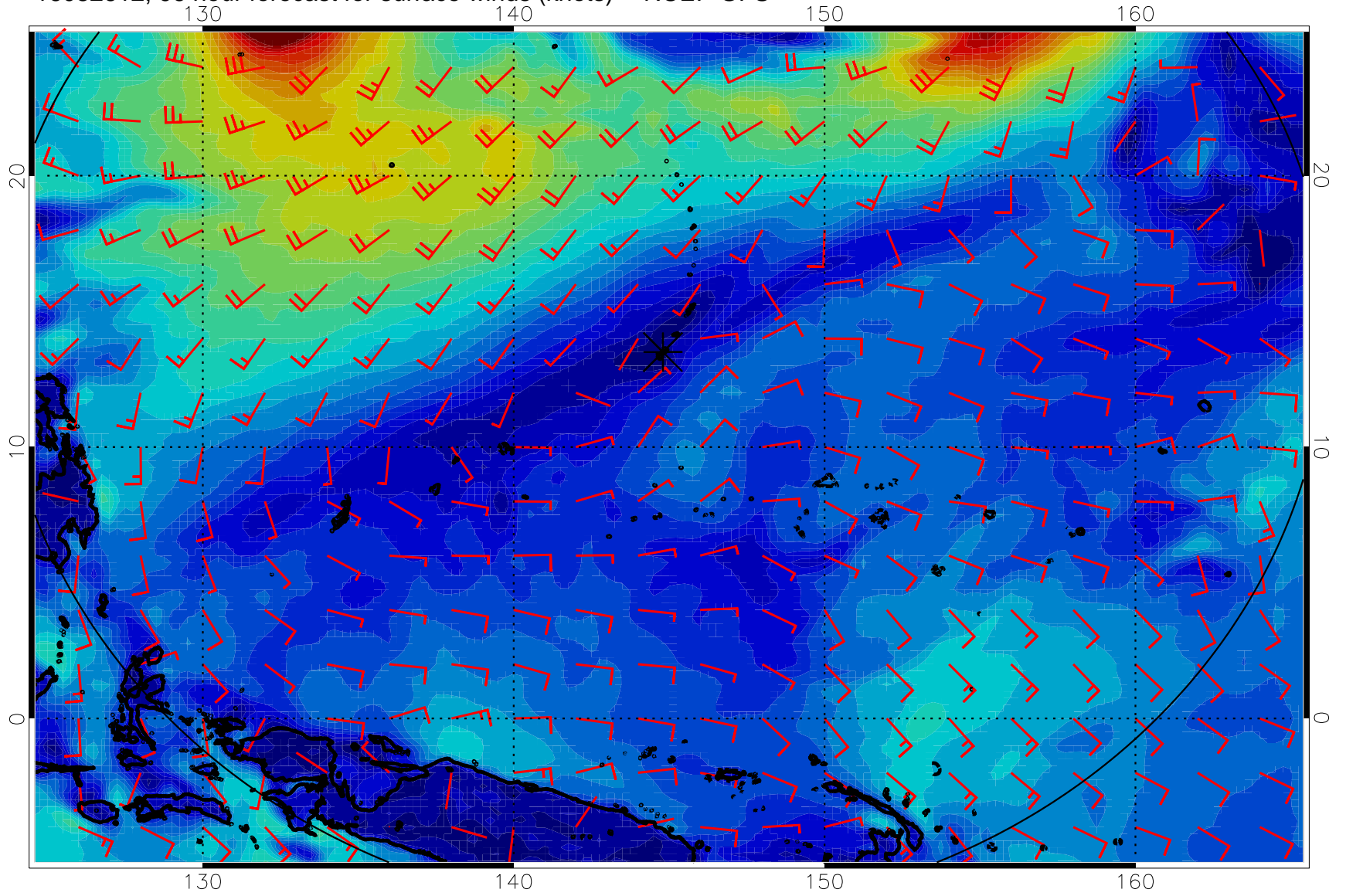
16082612, 96 hour forecast for surface winds (knots) -- NCEP GFS
