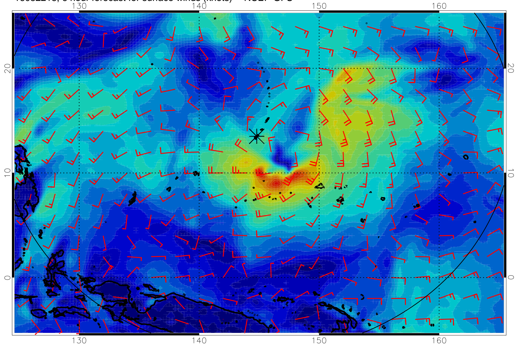
16082218, 6 hour forecast for surface winds (knots) -- NCEP GFS
