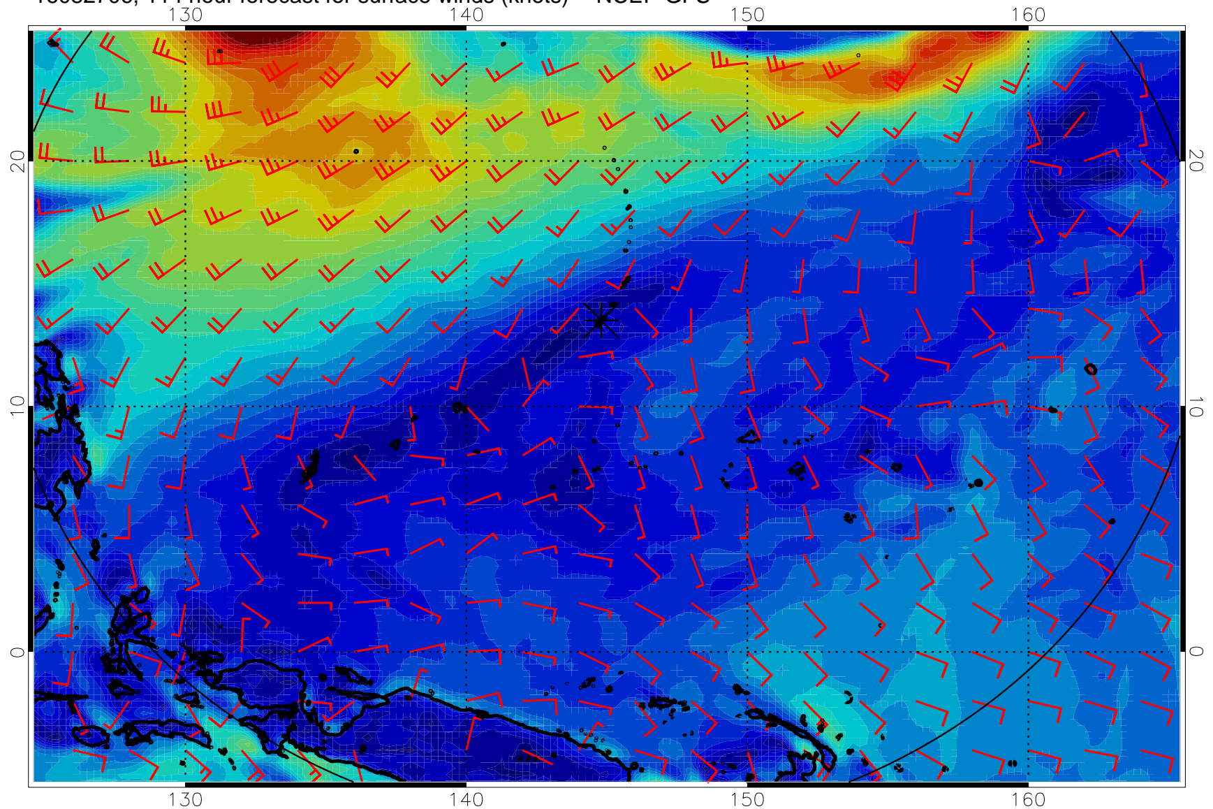
16082706, 114 hour forecast for surface winds (knots) -- NCEP GFS
