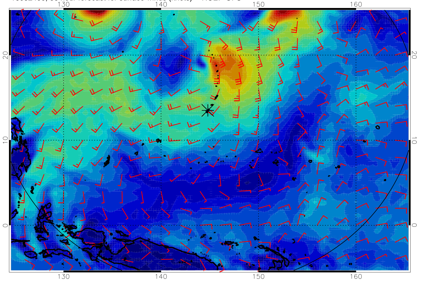
16082400, 36 hour forecast for surface winds (knots) -- NCEP GFS
