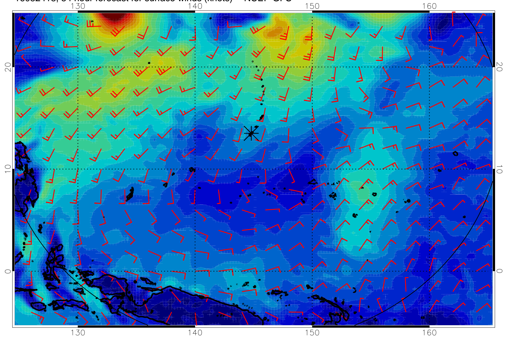
16082418, 54 hour forecast for surface winds (knots) -- NCEP GFS
