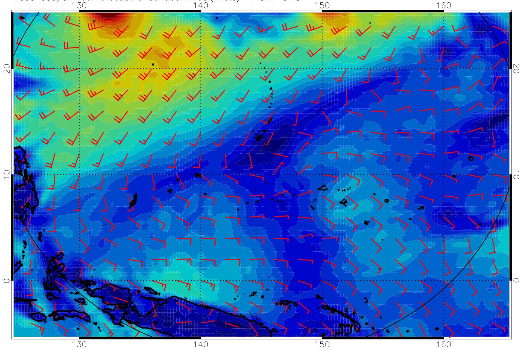
16082600, 84 hour forecast for surface winds (knots) -- NCEP GFS
