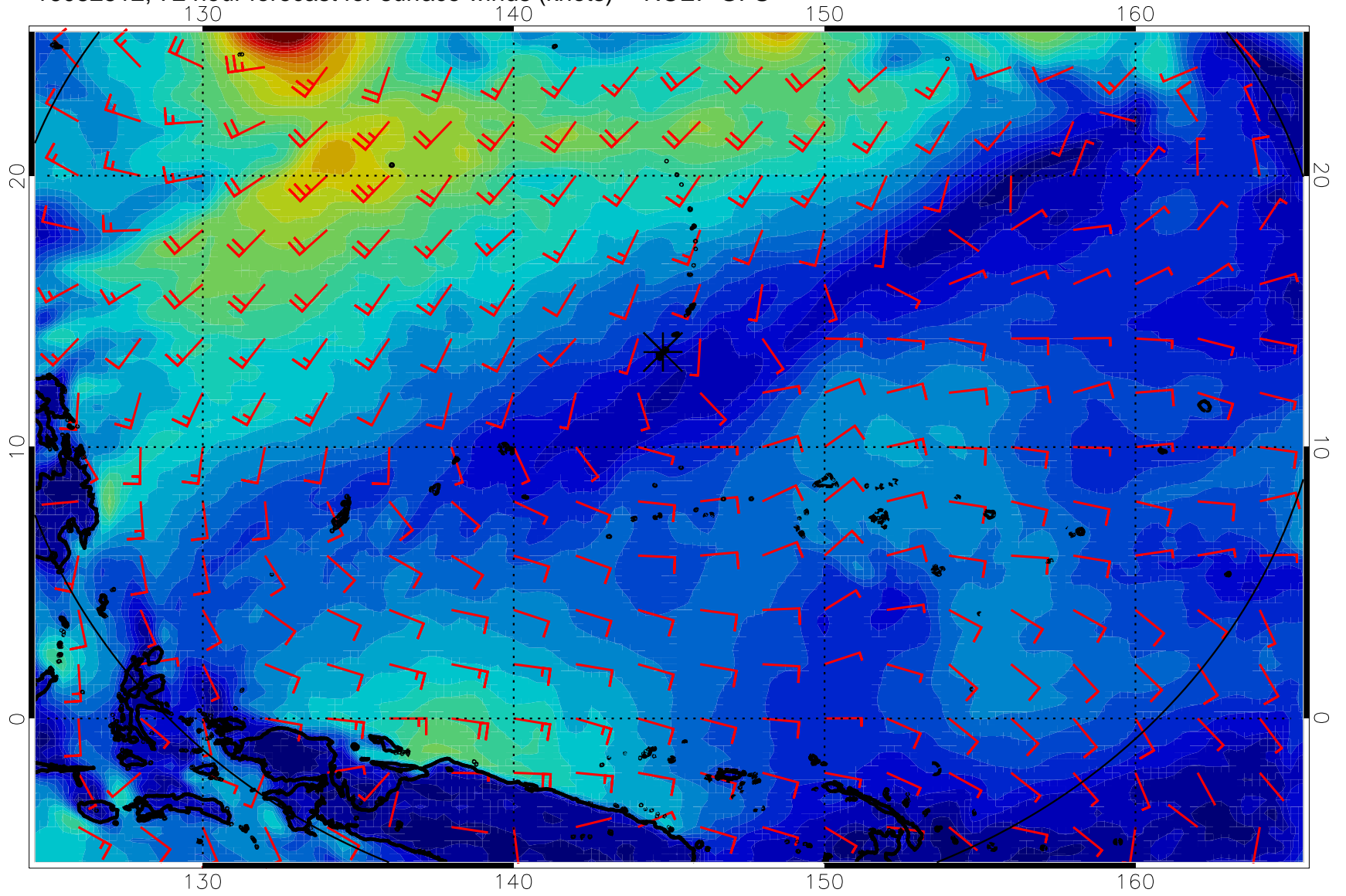
16082512, 72 hour forecast for surface winds (knots) -- NCEP GFS
