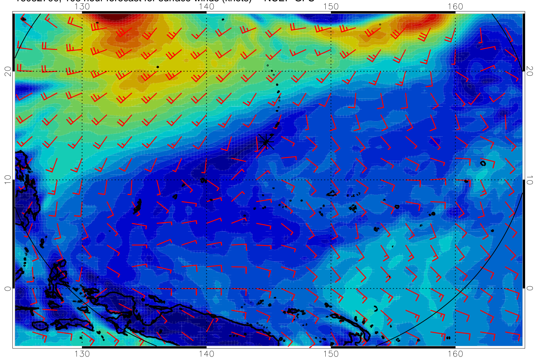
16082700, 108 hour forecast for surface winds (knots) -- NCEP GFS
