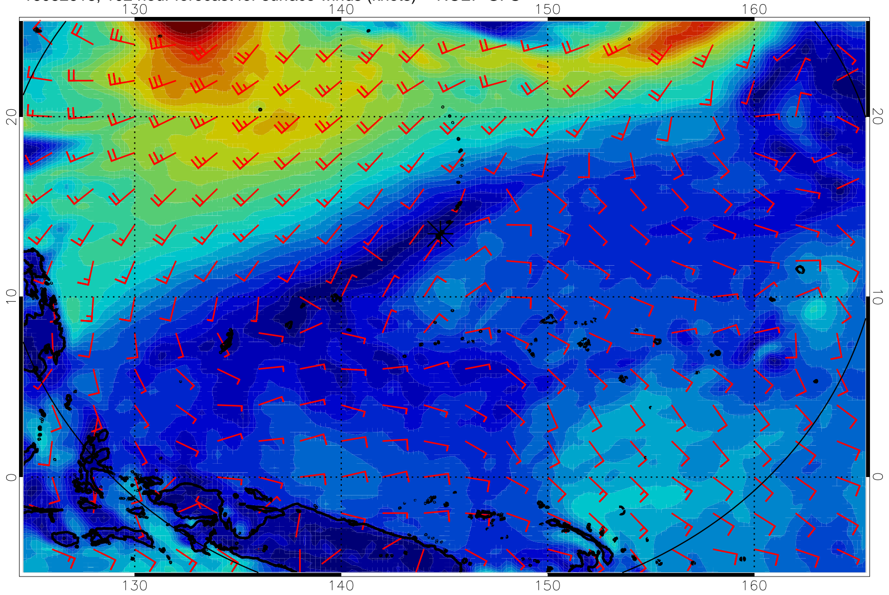
16082618, 102 hour forecast for surface winds (knots) -- NCEP GFS
