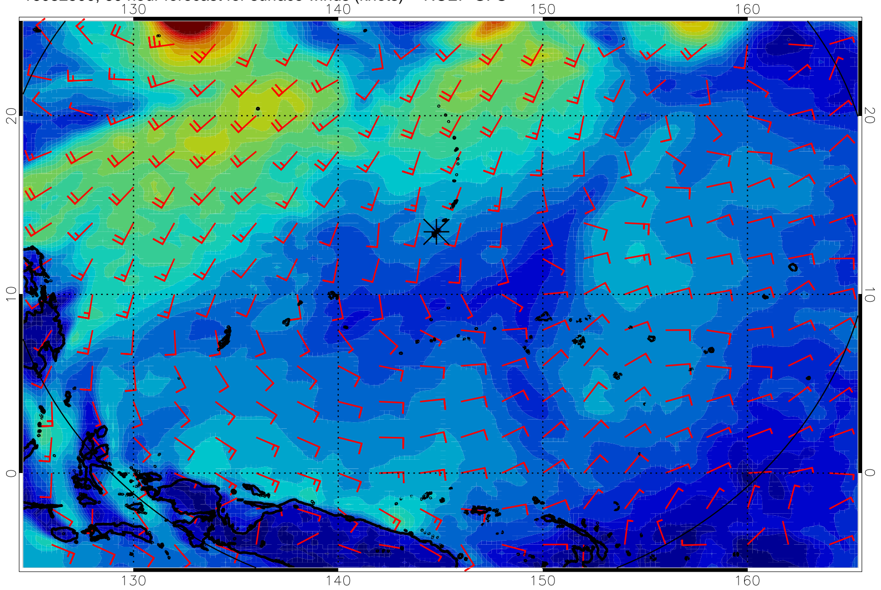
16082500, 60 hour forecast for surface winds (knots) -- NCEP GFS
