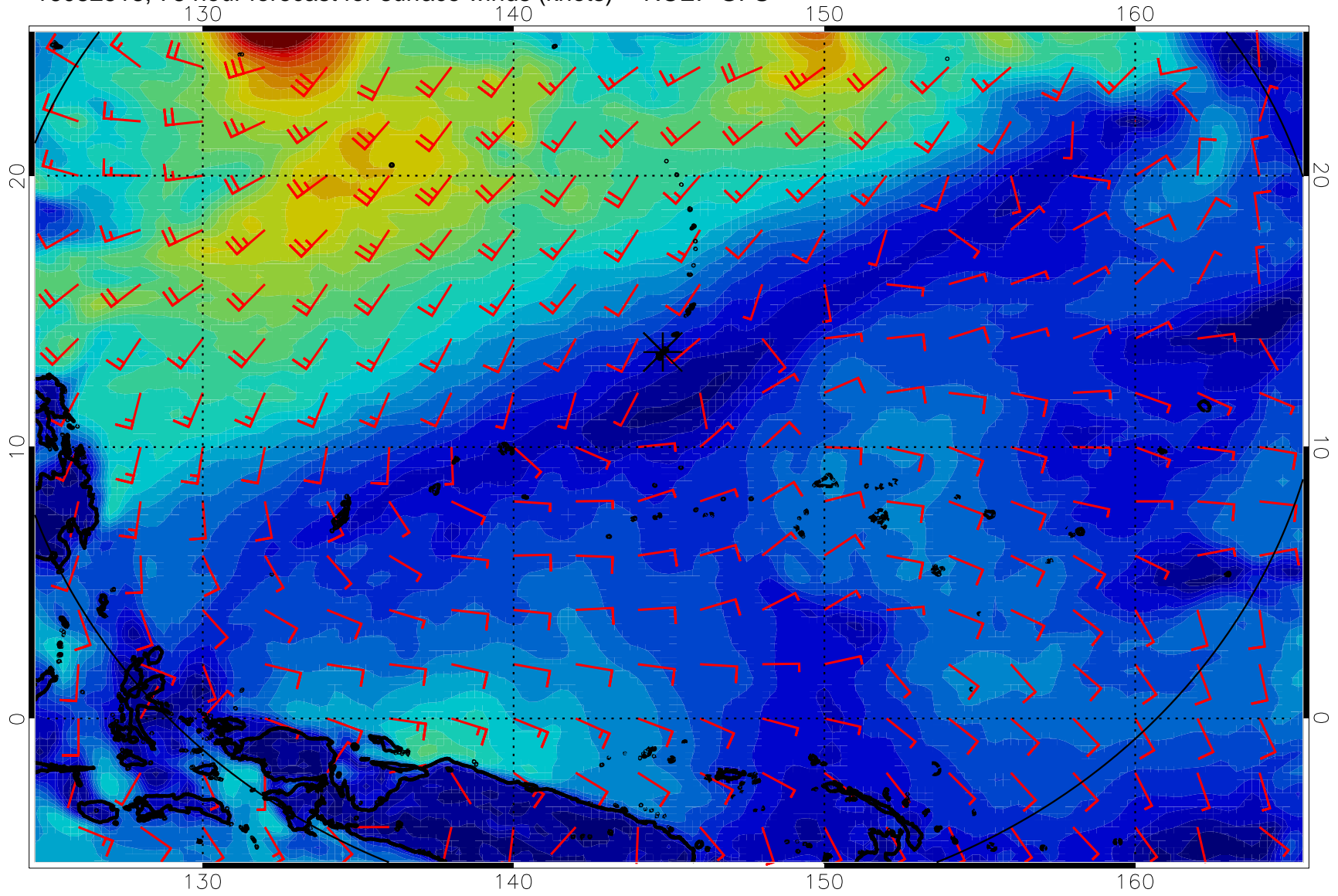
16082518, 78 hour forecast for surface winds (knots) -- NCEP GFS
