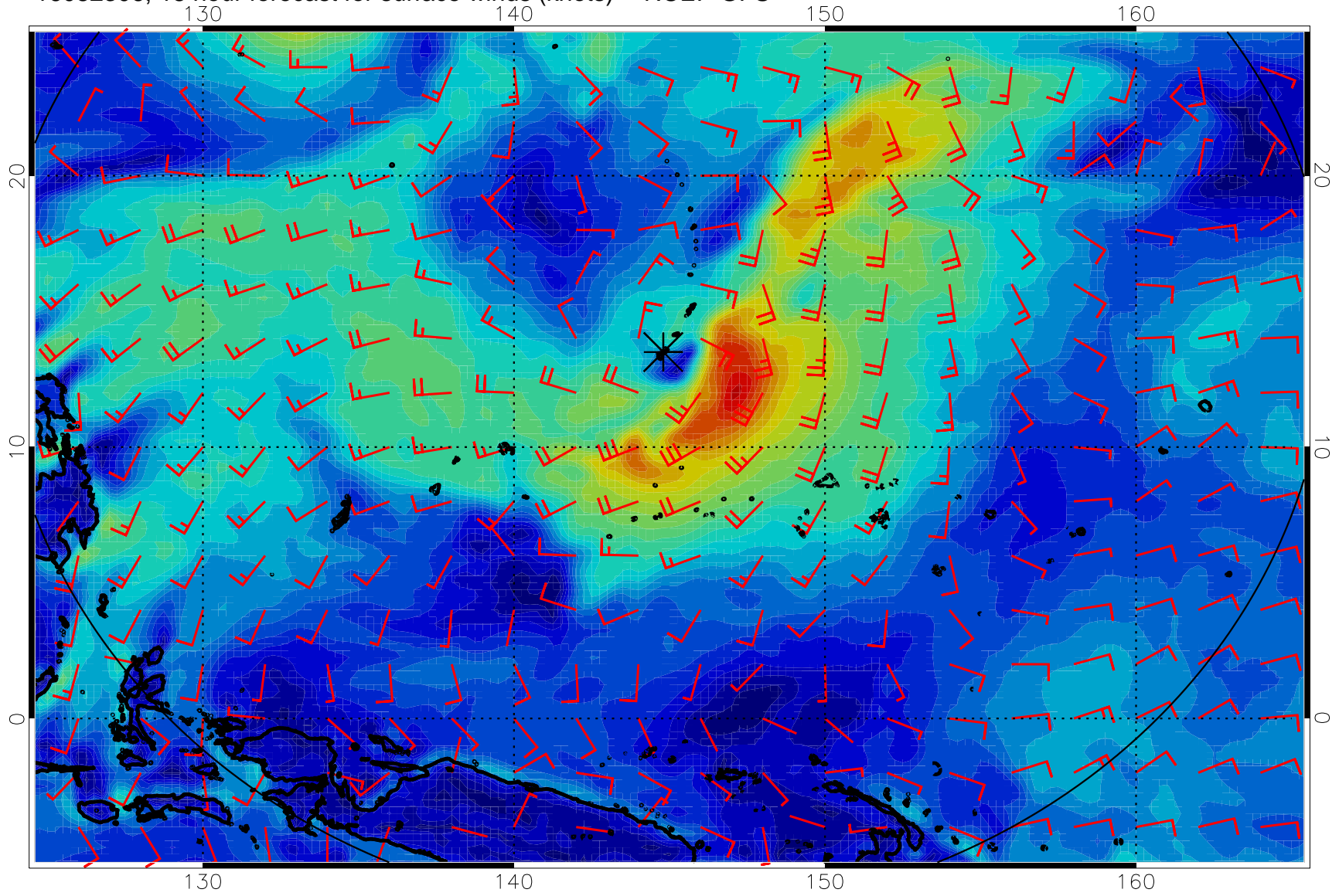
16082306, 18 hour forecast for surface winds (knots) -- NCEP GFS
