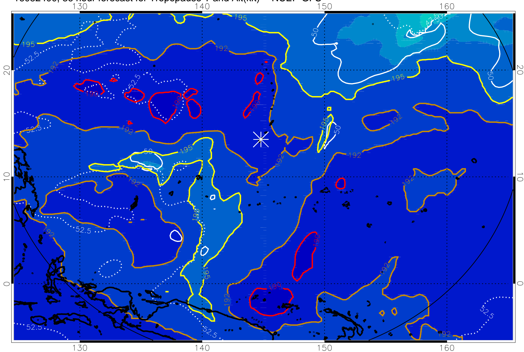
16082400, 36 hour forecast for Tropopause T and Alt(kft) -- NCEP GFS
