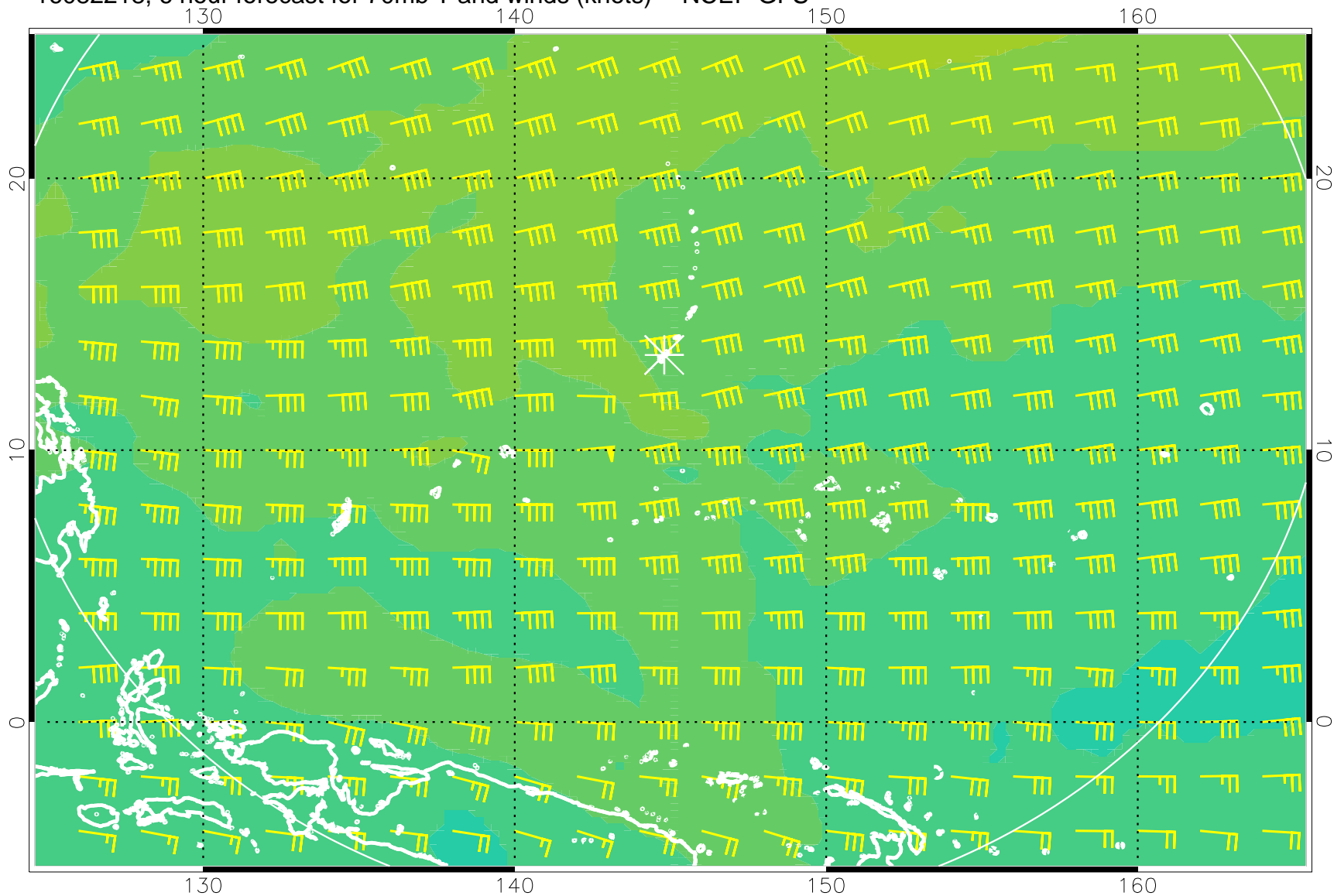
16082218, 6 hour forecast for 70mb T and winds (knots) -- NCEP GFS
