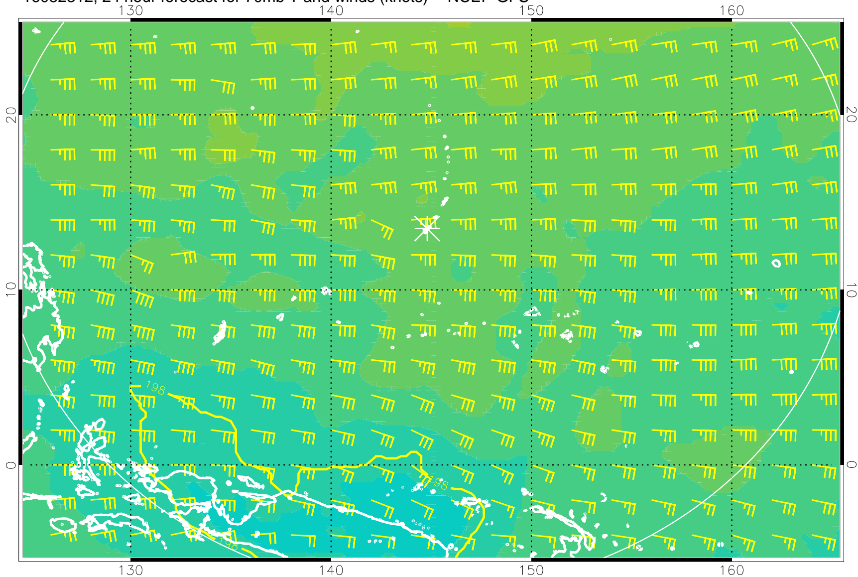
16082312, 24 hour forecast for 70mb T and winds (knots) -- NCEP GFS
