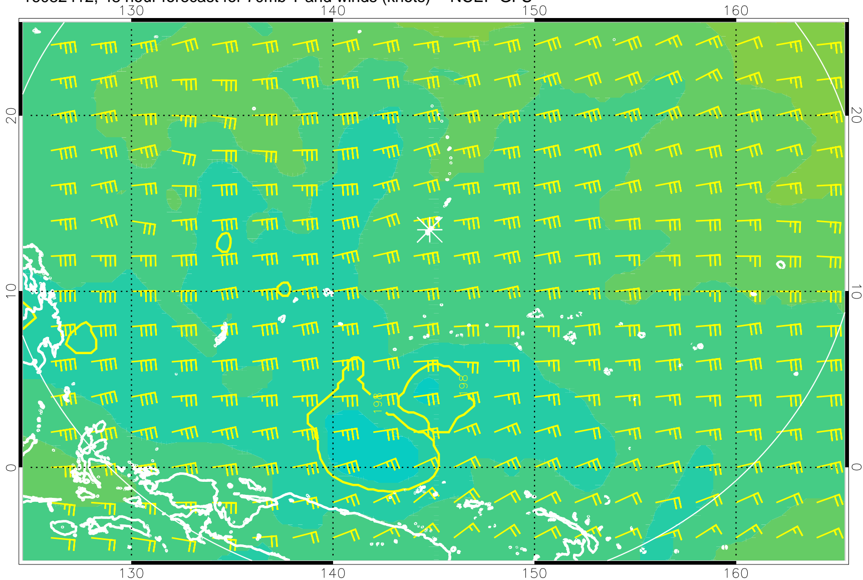
16082412, 48 hour forecast for 70mb T and winds (knots) -- NCEP GFS
