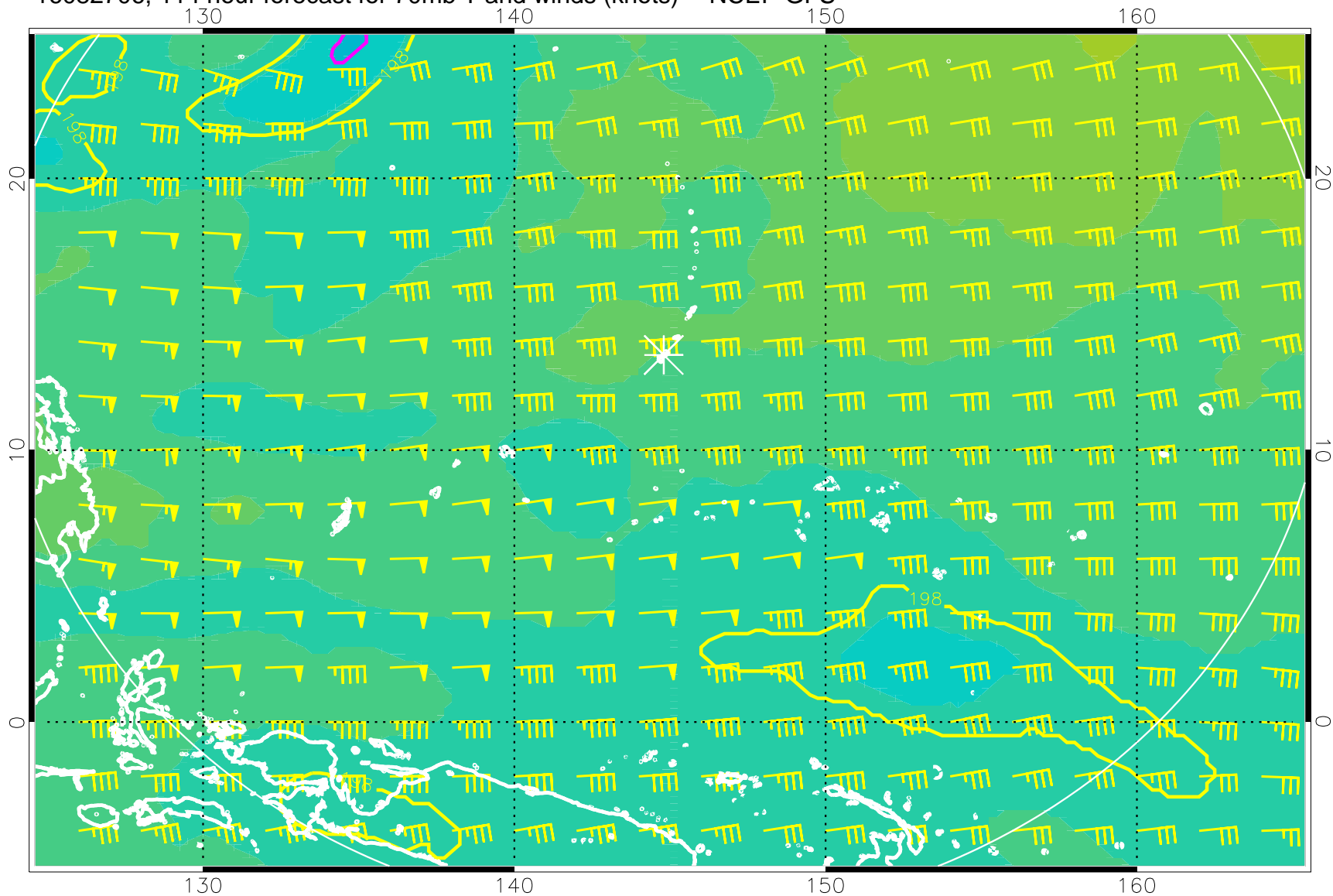
16082706, 114 hour forecast for 70mb T and winds (knots) -- NCEP GFS
