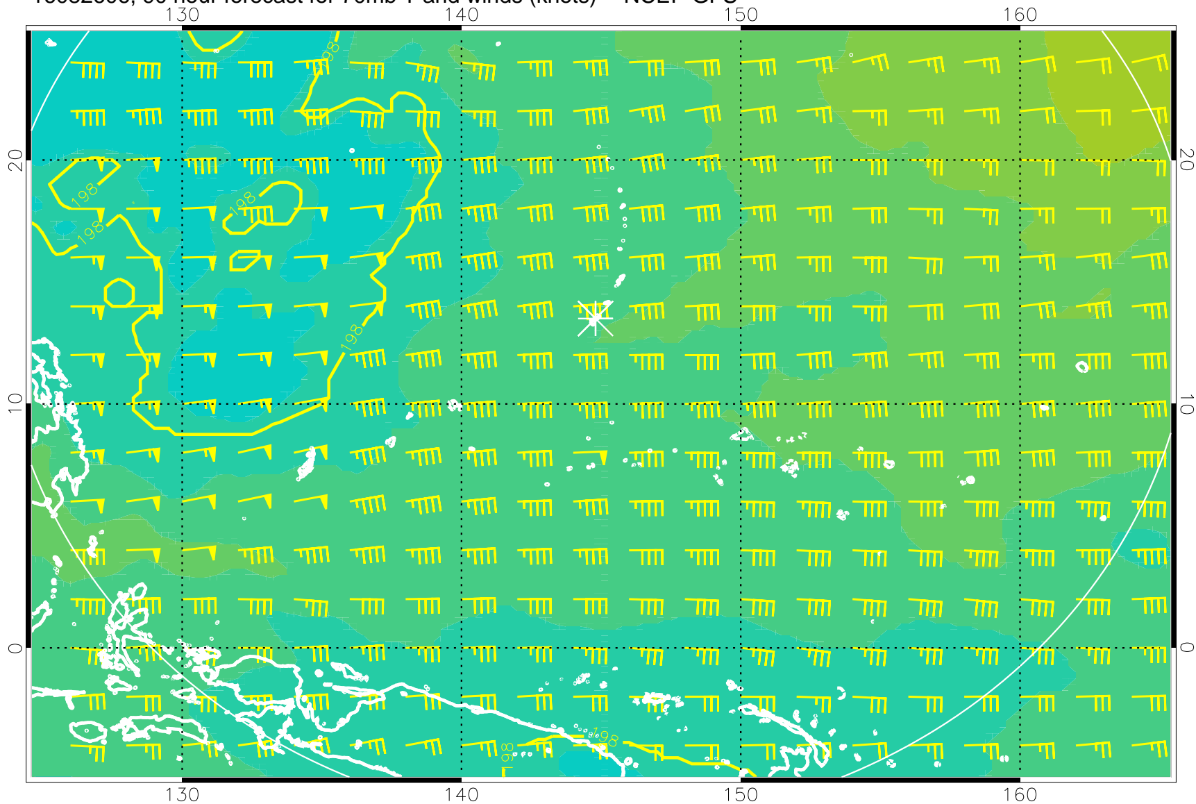
16082606, 90 hour forecast for 70mb T and winds (knots) -- NCEP GFS
