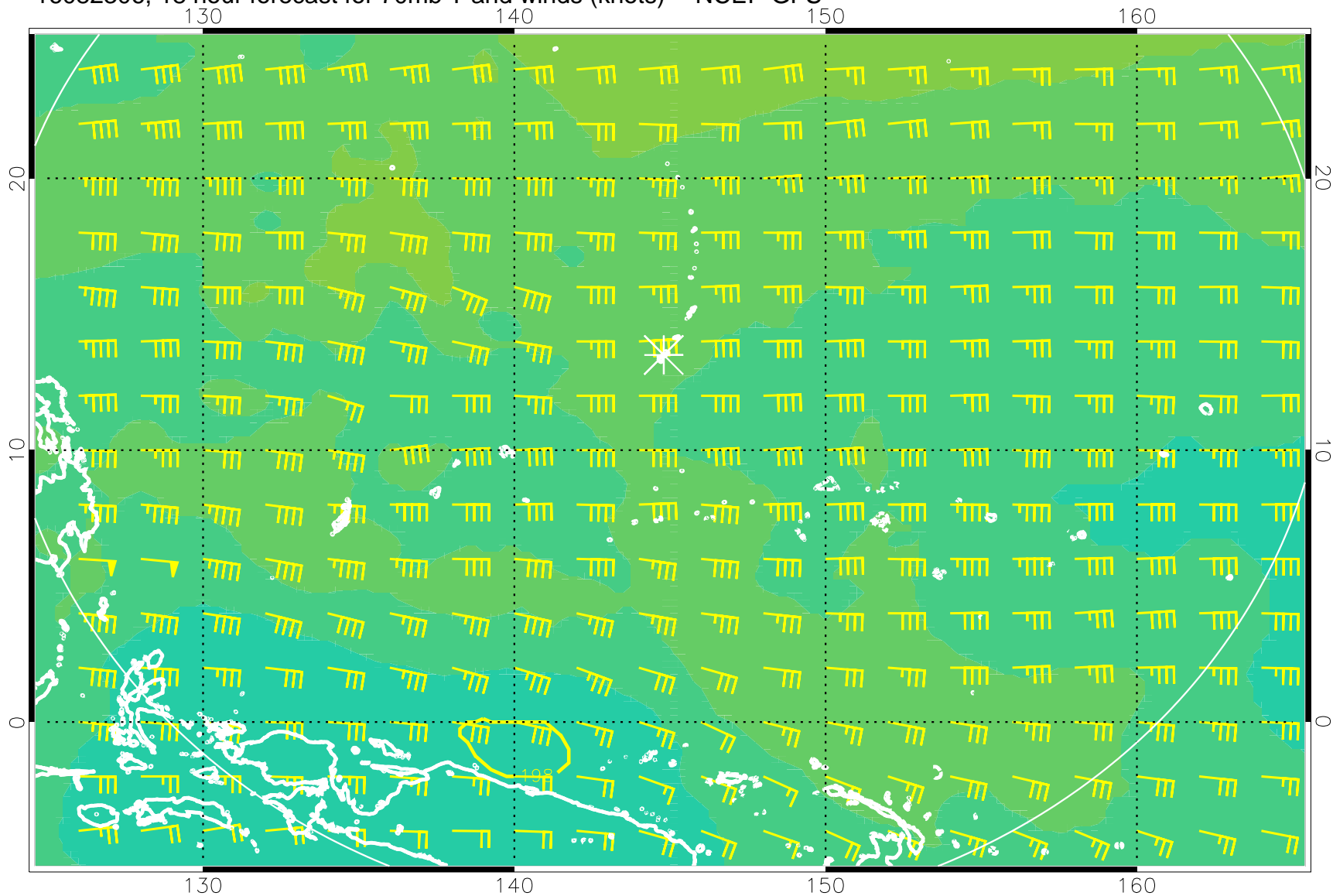
16082306, 18 hour forecast for 70mb T and winds (knots) -- NCEP GFS
