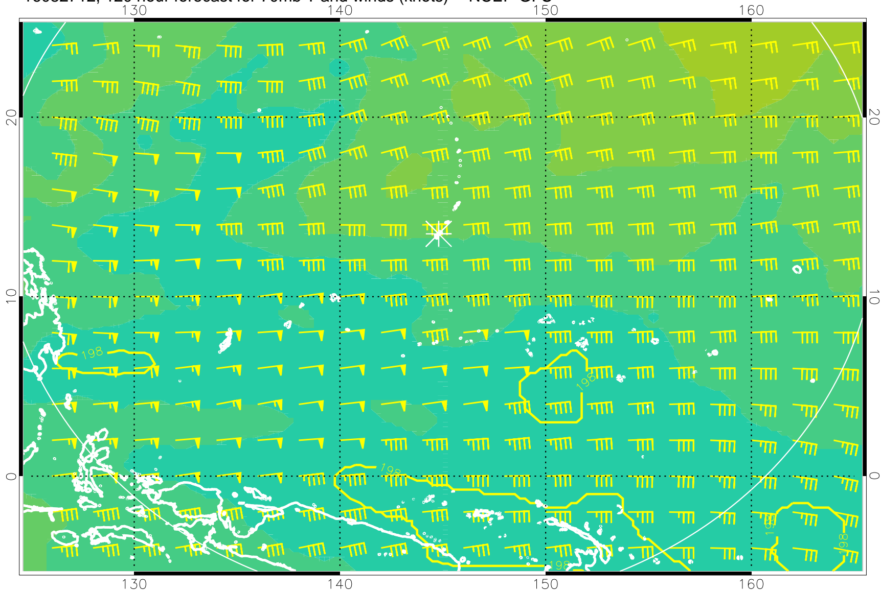
16082712, 120 hour forecast for 70mb T and winds (knots) -- NCEP GFS
