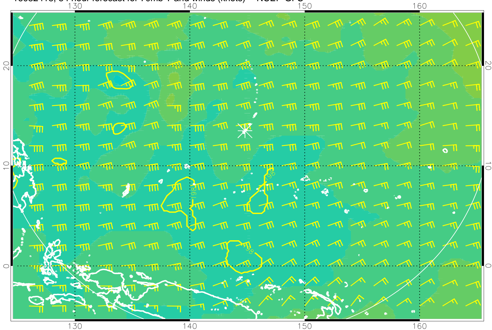
16082418, 54 hour forecast for 70mb T and winds (knots) -- NCEP GFS
