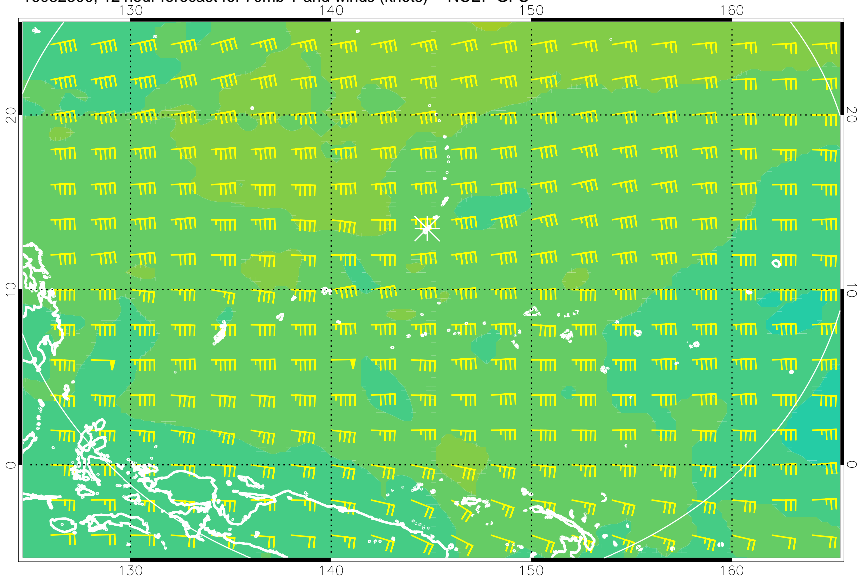
16082300, 12 hour forecast for 70mb T and winds (knots) -- NCEP GFS
