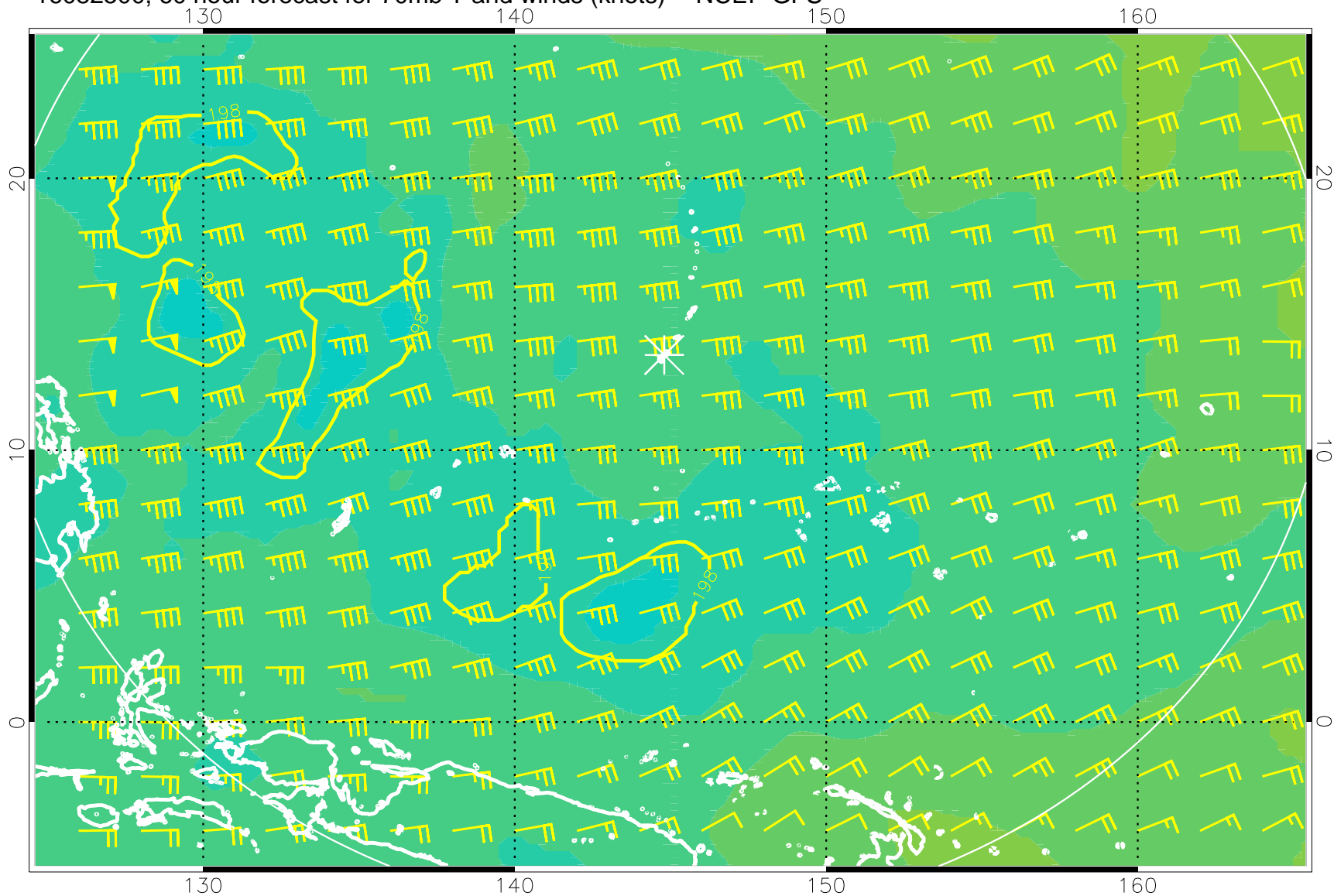
16082500, 60 hour forecast for 70mb T and winds (knots) -- NCEP GFS
