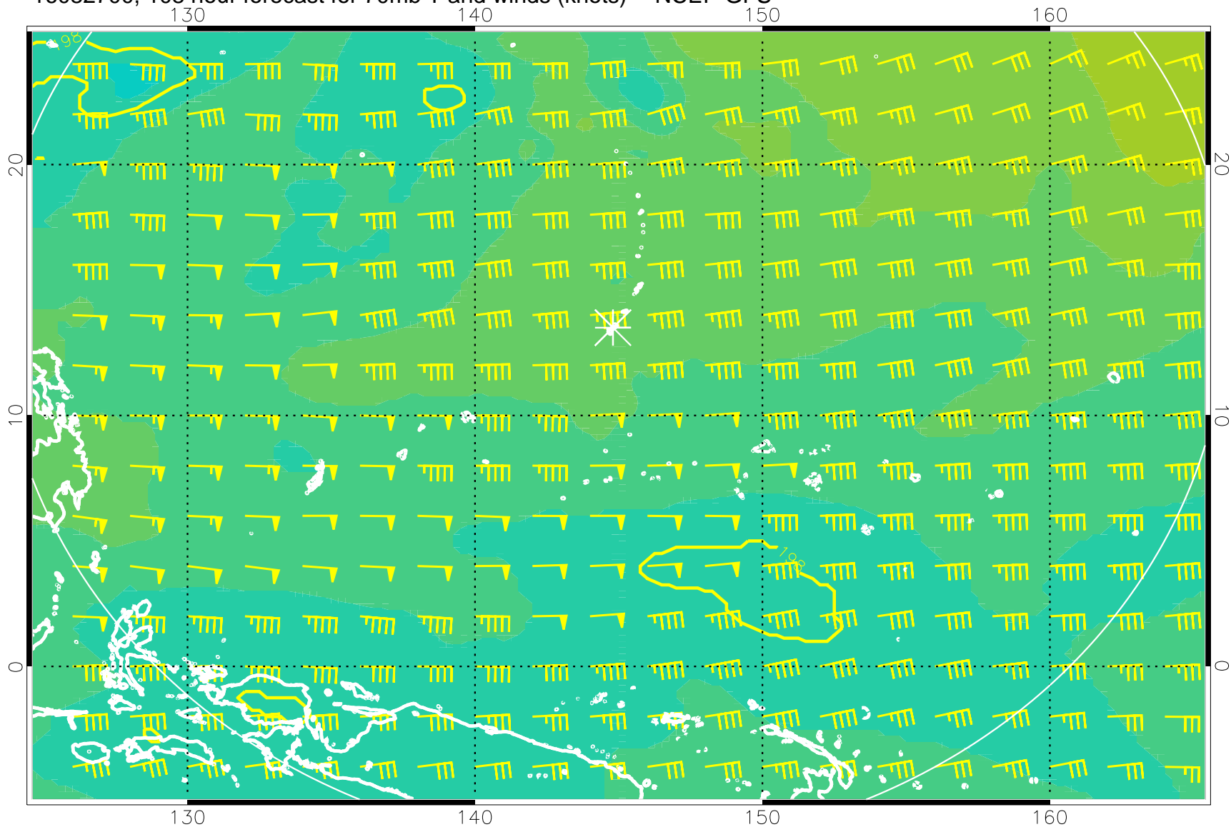
16082700, 108 hour forecast for 70mb T and winds (knots) -- NCEP GFS
