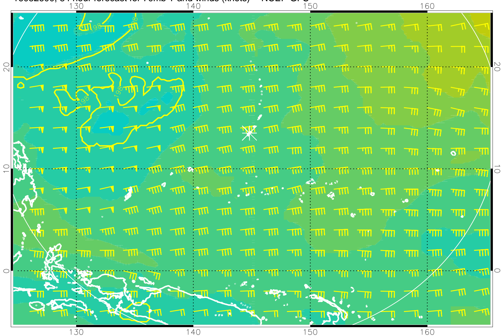
16082600, 84 hour forecast for 70mb T and winds (knots) -- NCEP GFS
