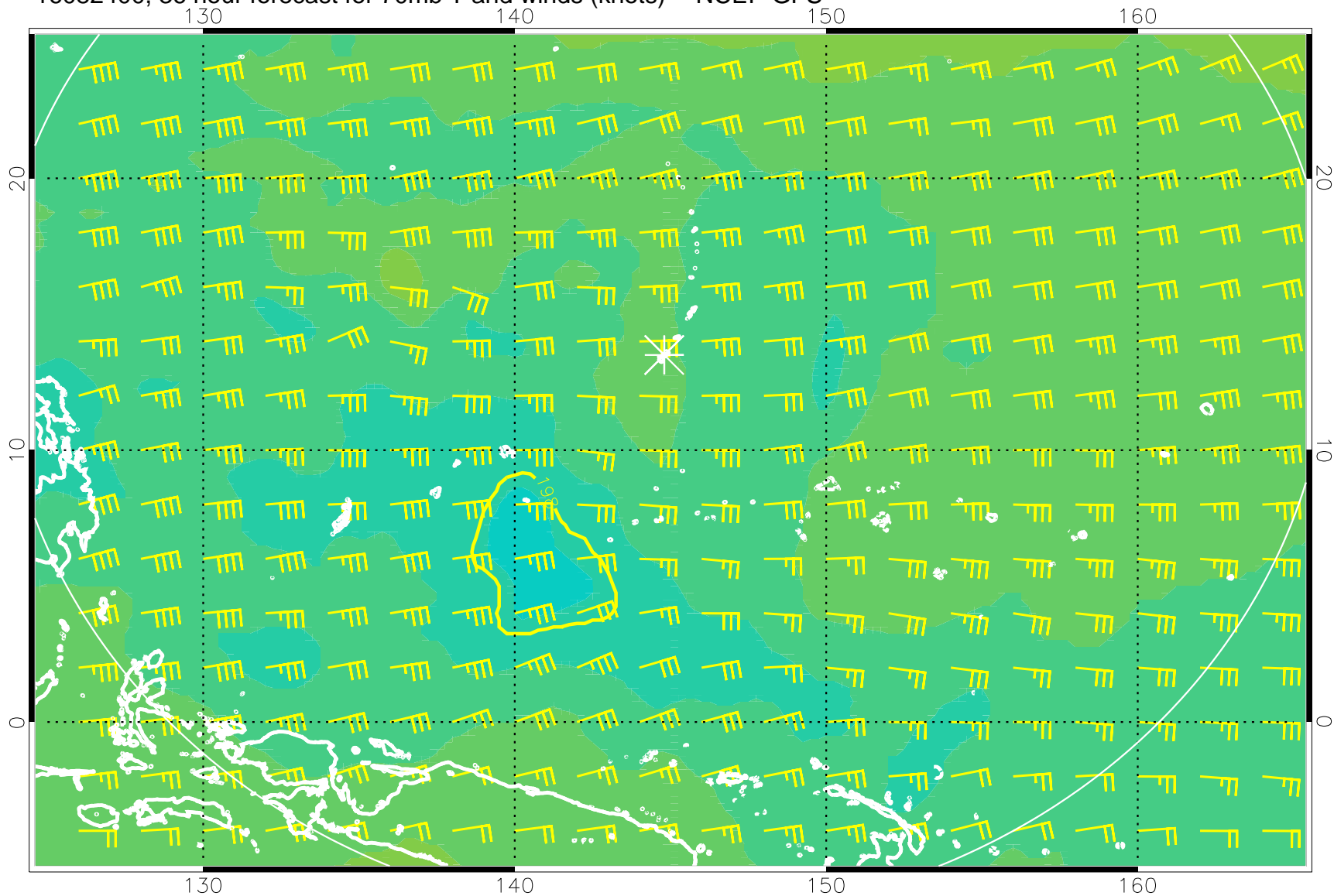
16082400, 36 hour forecast for 70mb T and winds (knots) -- NCEP GFS
