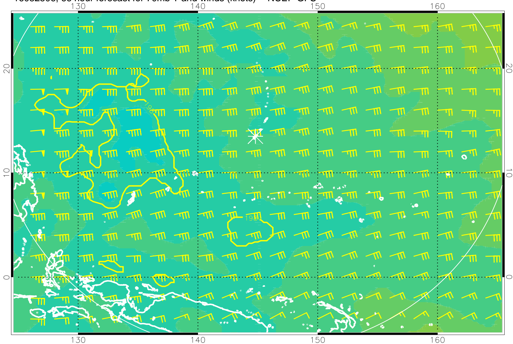
16082506, 66 hour forecast for 70mb T and winds (knots) -- NCEP GFS
