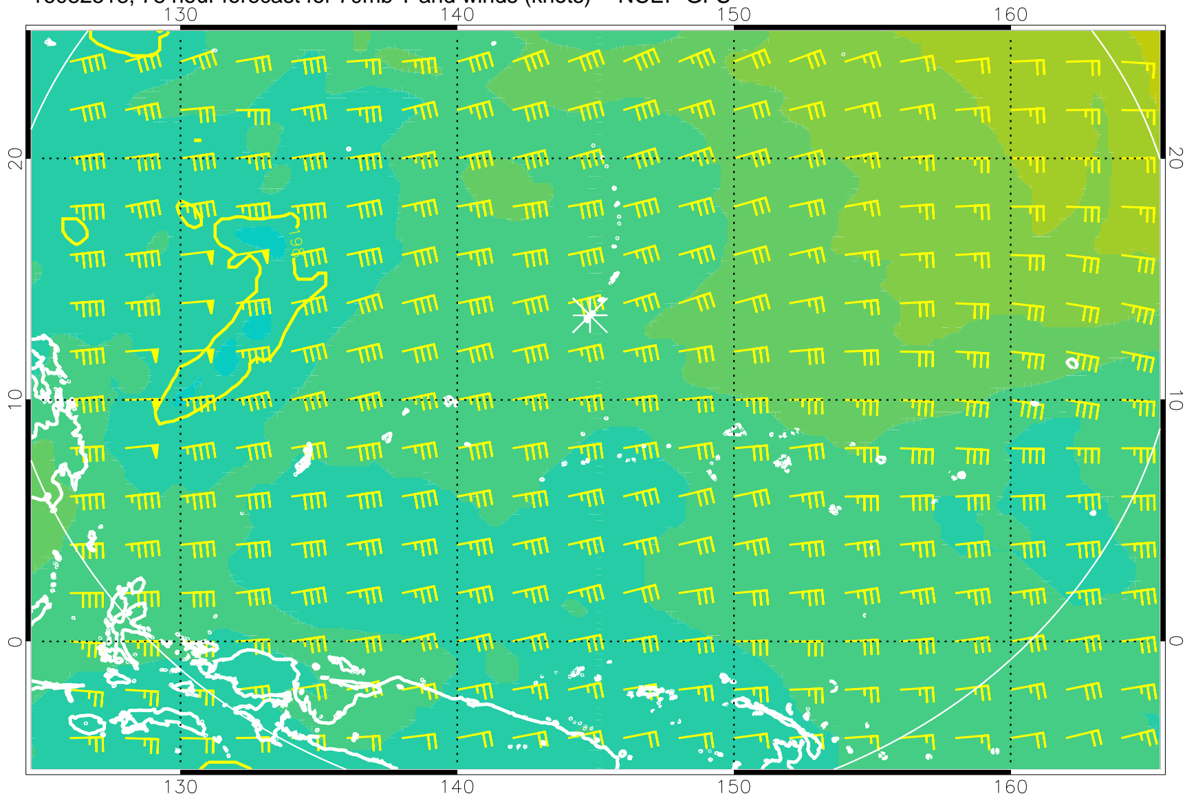
16082518, 78 hour forecast for 70mb T and winds (knots) -- NCEP GFS
