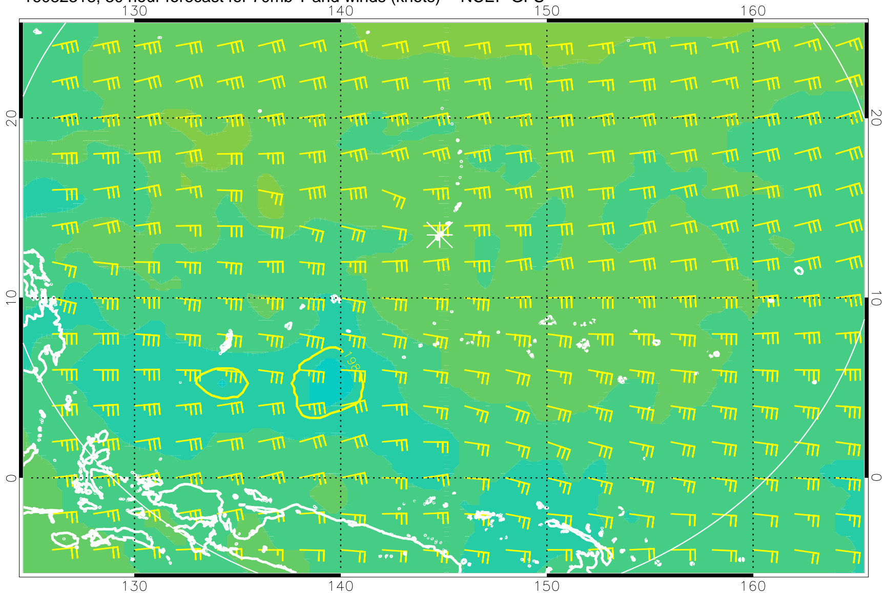
16082318, 30 hour forecast for 70mb T and winds (knots) -- NCEP GFS
