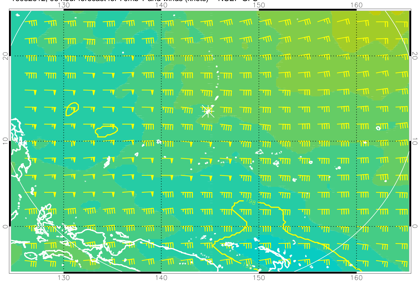
16082612, 96 hour forecast for 70mb T and winds (knots) -- NCEP GFS
