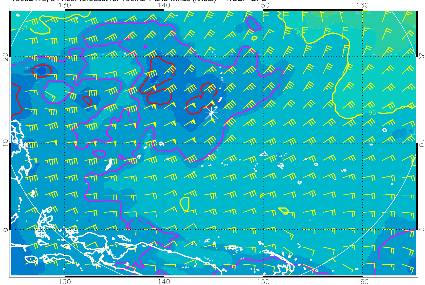
16082418, 54 hour forecast for 100mb T and winds (knots) -- NCEP GFS
