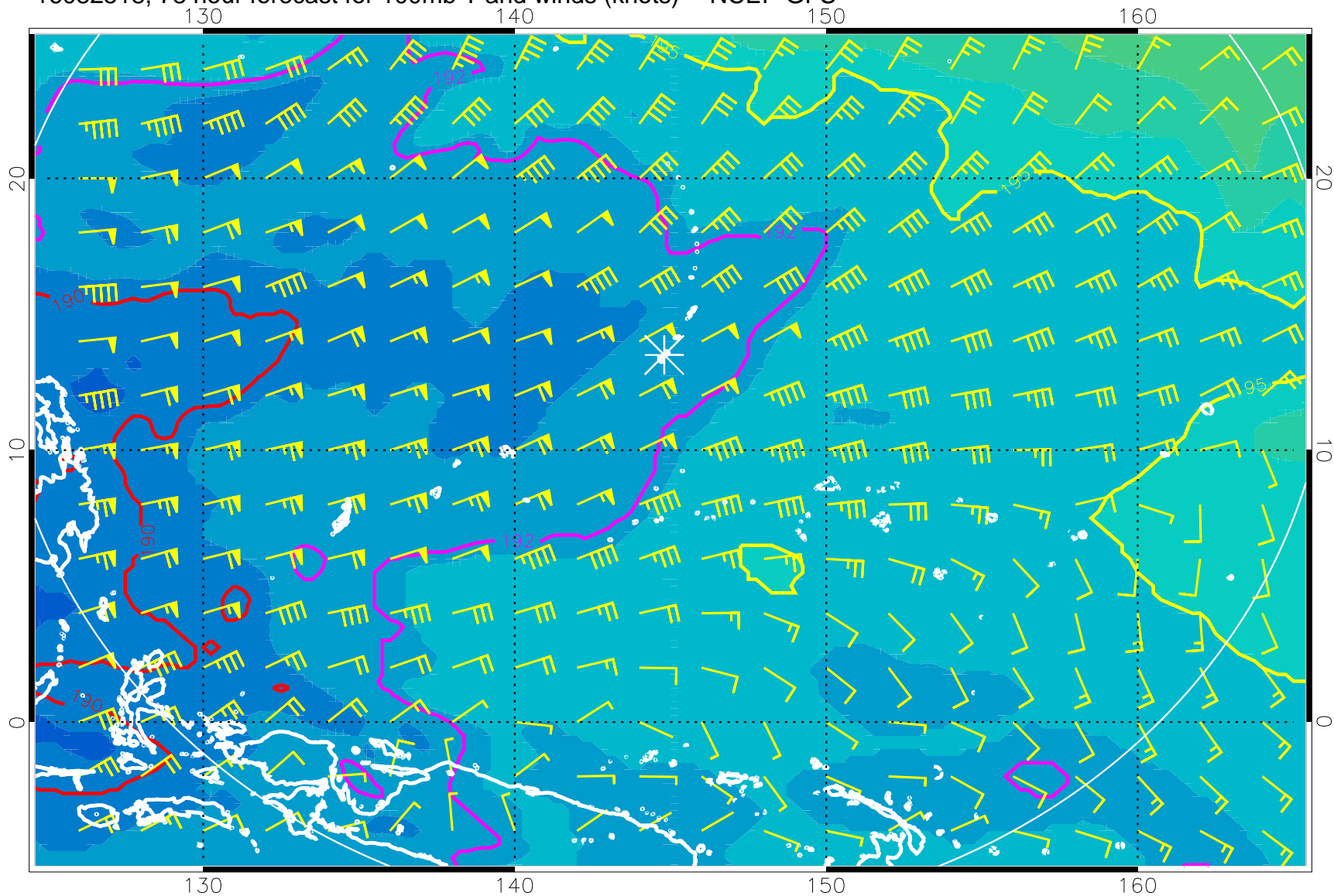
16082518, 78 hour forecast for 100mb T and winds (knots) -- NCEP GFS
