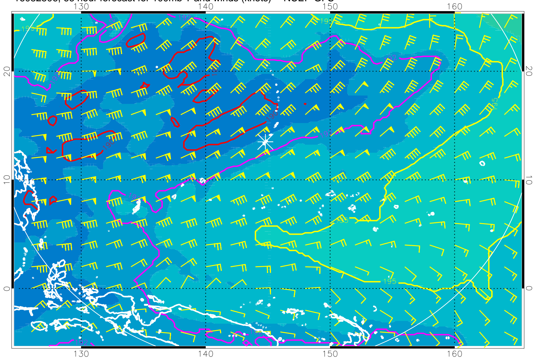
16082506, 66 hour forecast for 100mb T and winds (knots) -- NCEP GFS
