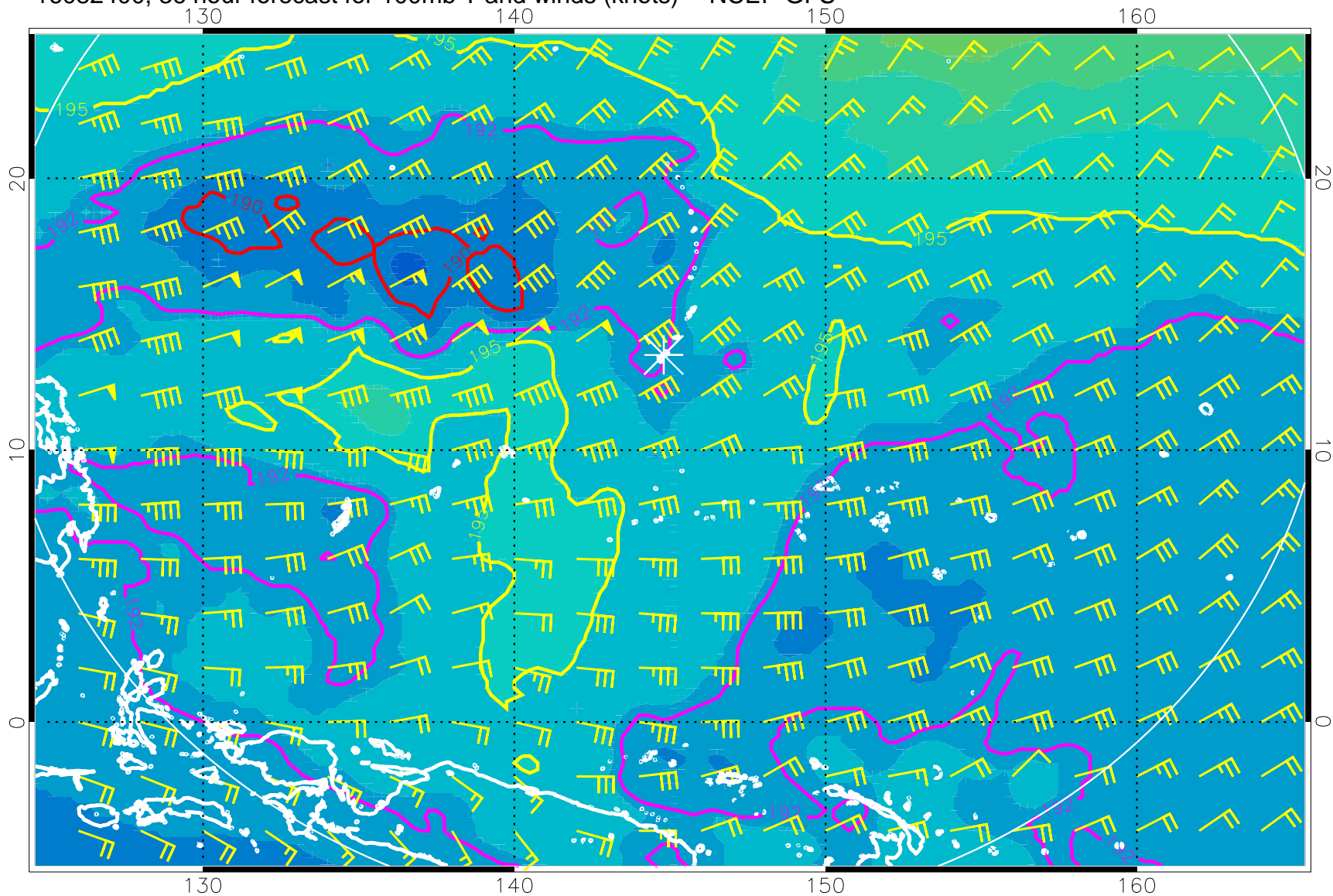
16082400, 36 hour forecast for 100mb T and winds (knots) -- NCEP GFS
