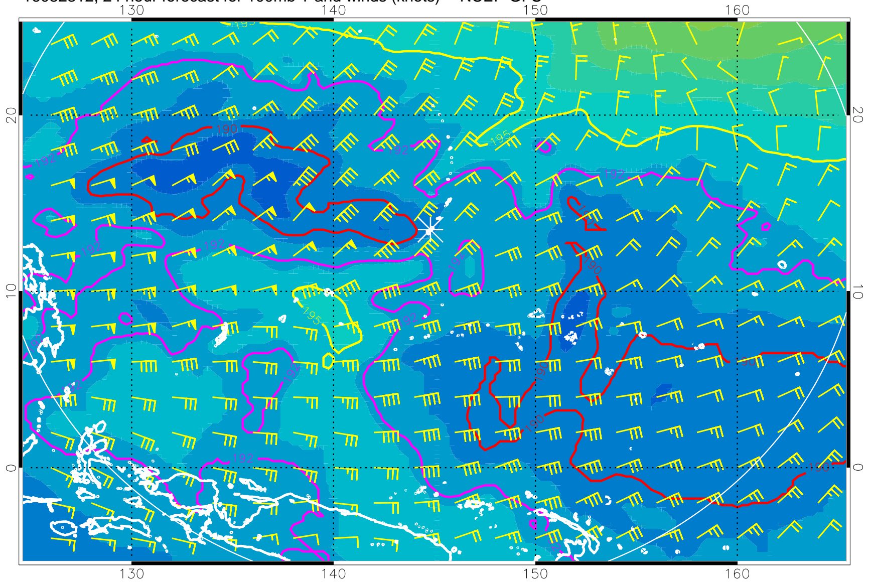
16082312, 24 hour forecast for 100mb T and winds (knots) -- NCEP GFS
