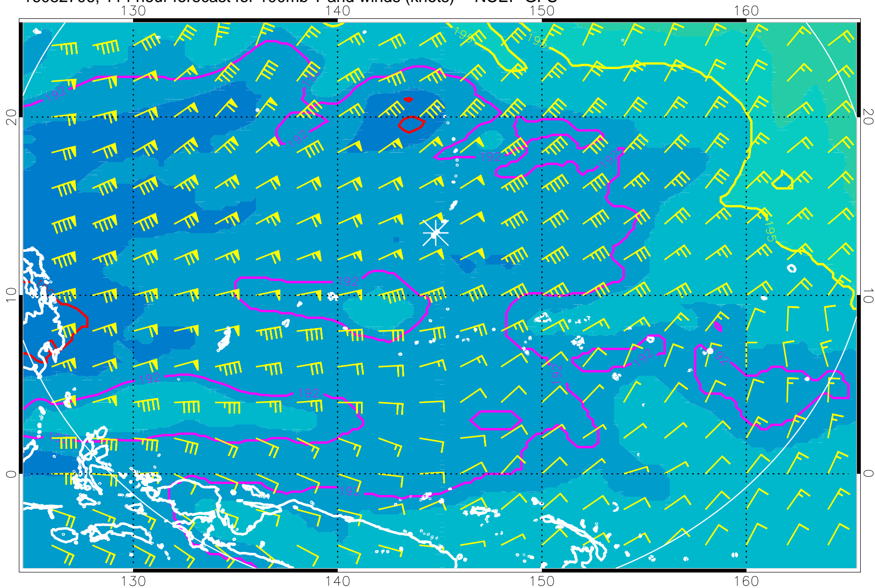
16082706, 114 hour forecast for 100mb T and winds (knots) -- NCEP GFS
