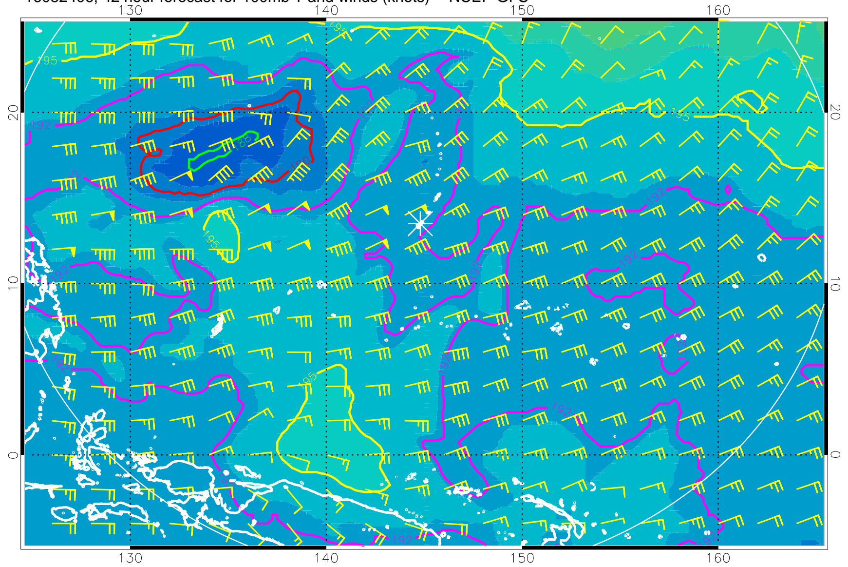
16082406, 42 hour forecast for 100mb T and winds (knots) -- NCEP GFS
