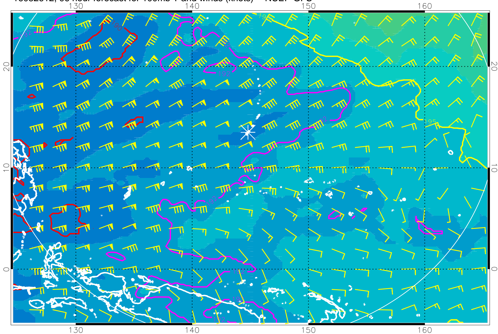
16082612, 96 hour forecast for 100mb T and winds (knots) -- NCEP GFS
