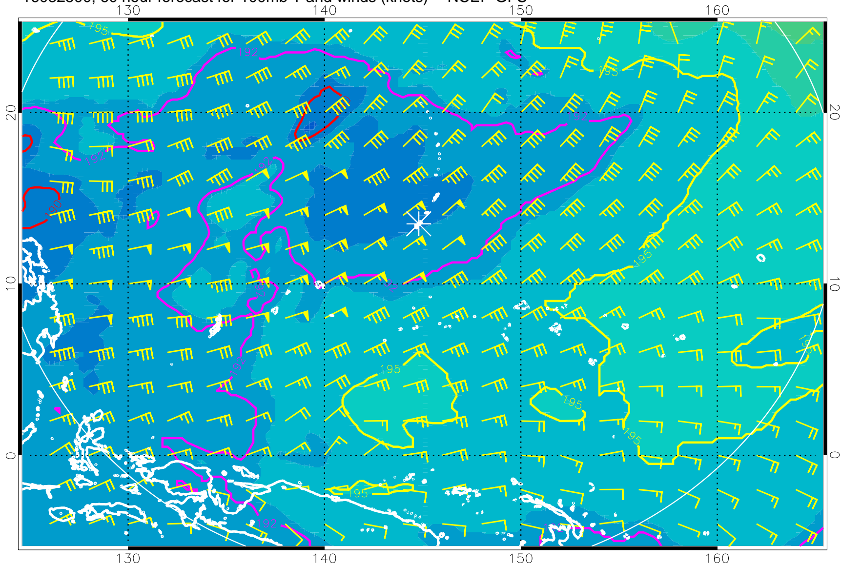
16082500, 60 hour forecast for 100mb T and winds (knots) -- NCEP GFS
