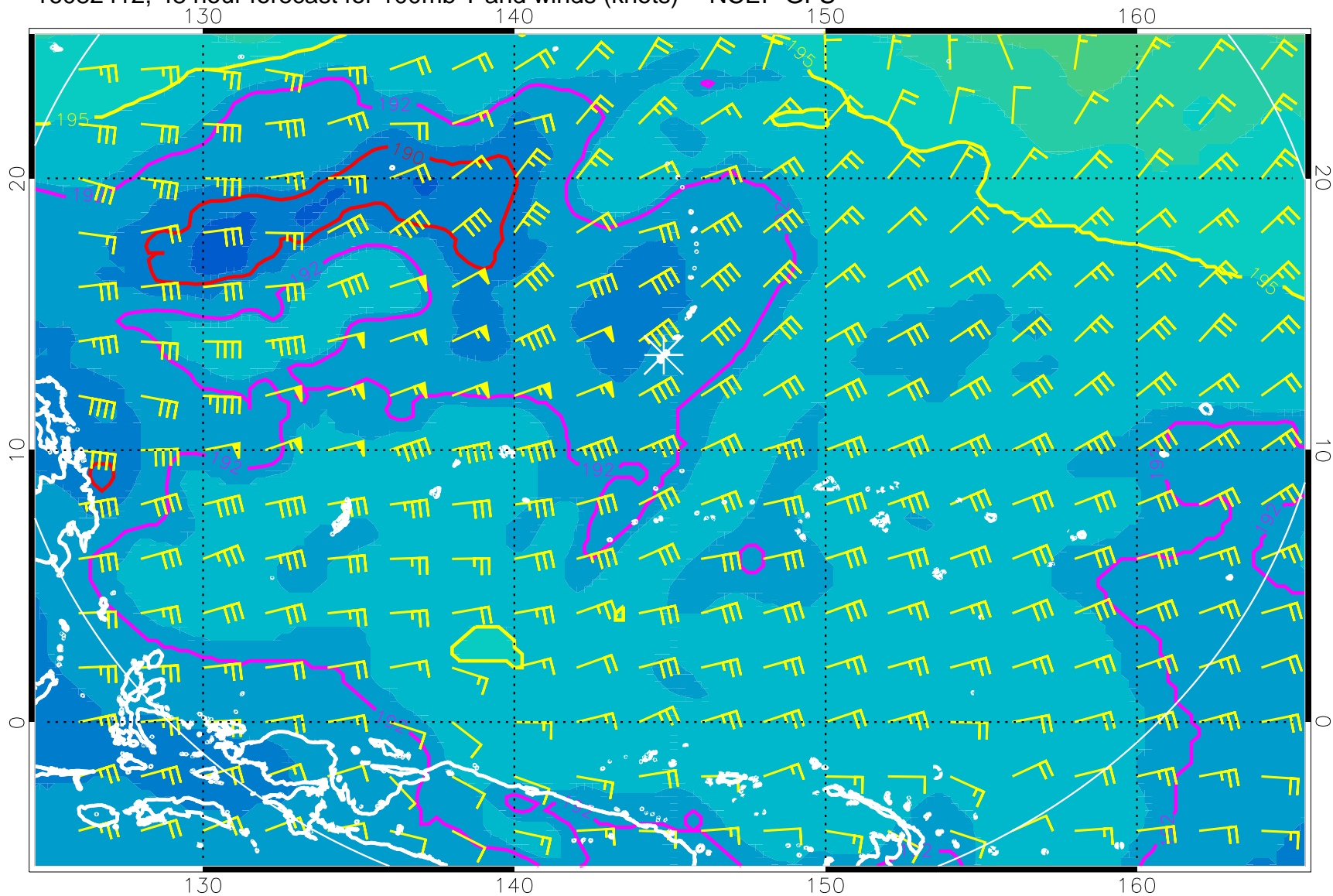
16082412, 48 hour forecast for 100mb T and winds (knots) -- NCEP GFS
