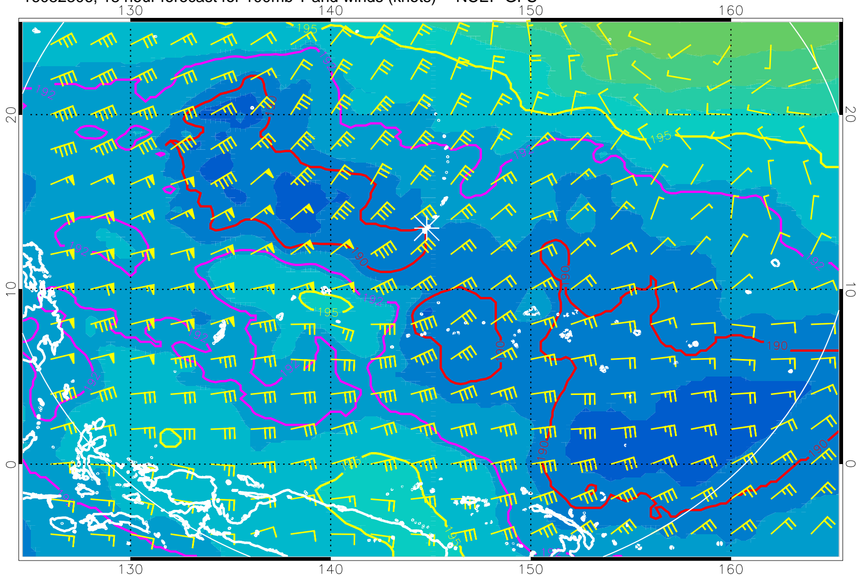
16082306, 18 hour forecast for 100mb T and winds (knots) -- NCEP GFS
