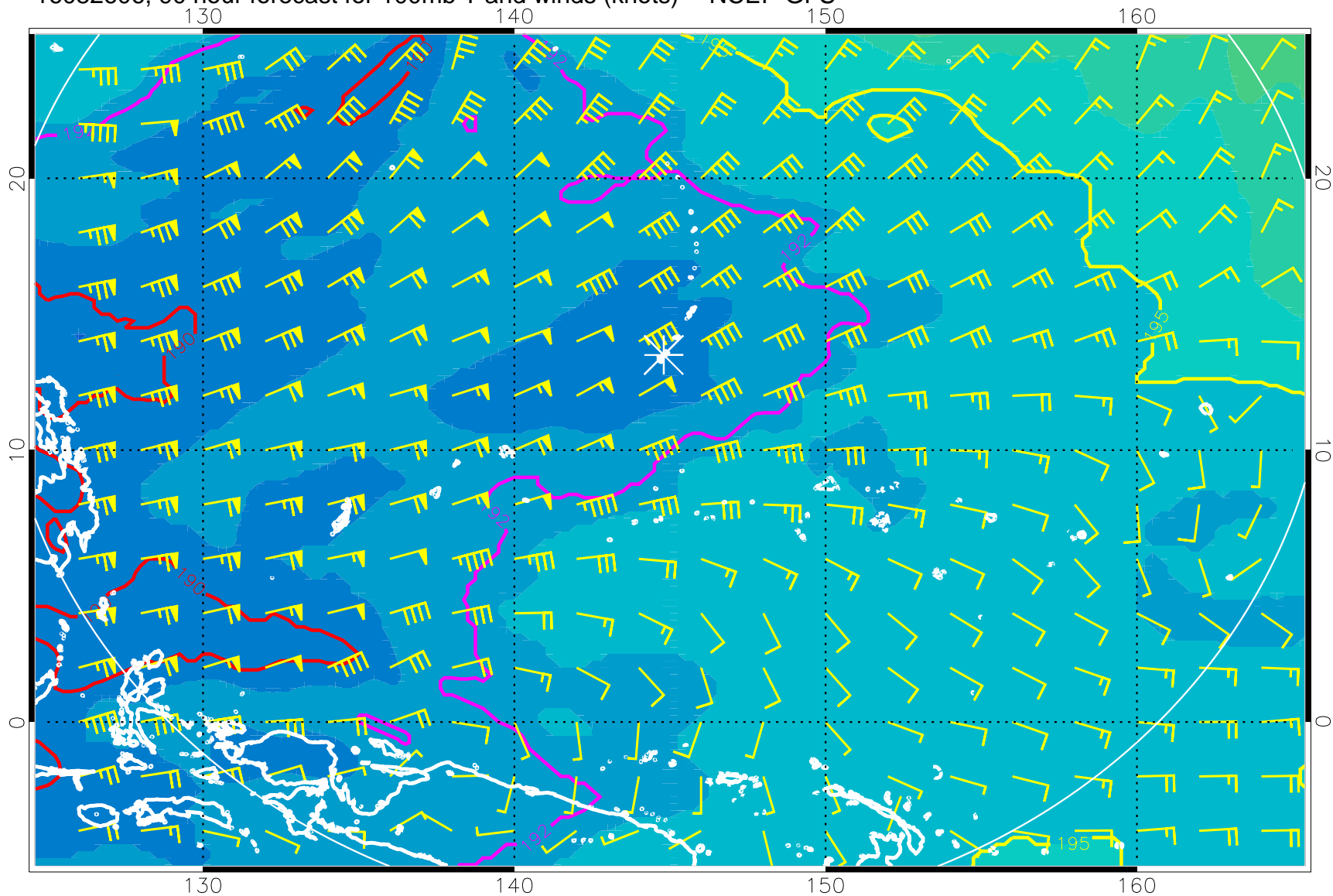
16082606, 90 hour forecast for 100mb T and winds (knots) -- NCEP GFS
