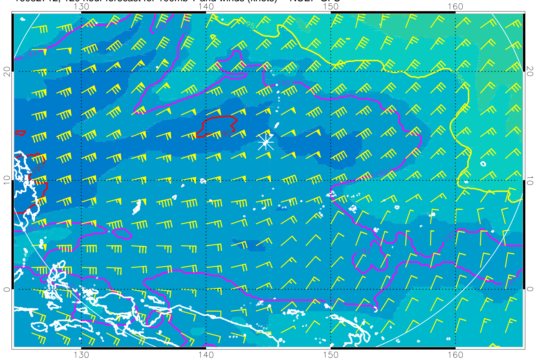
16082712, 120 hour forecast for 100mb T and winds (knots) -- NCEP GFS
