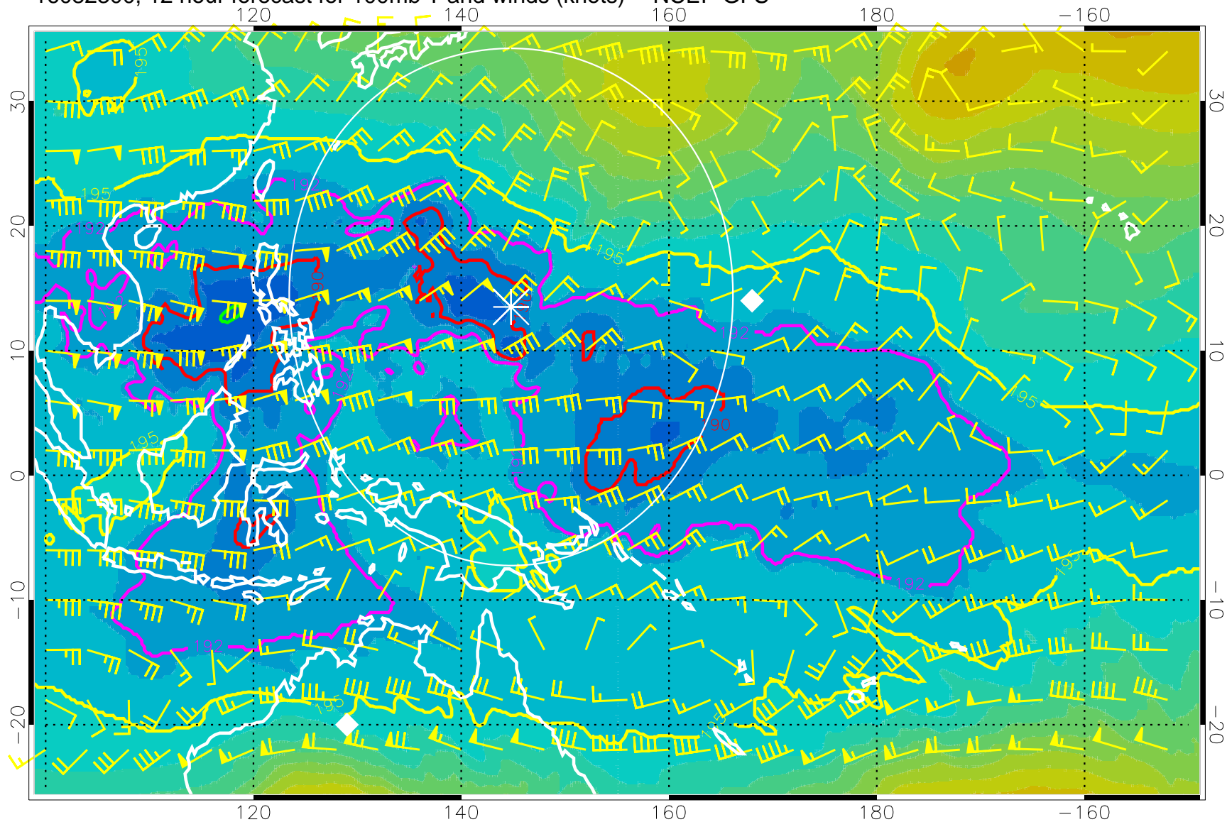
16082300, 12 hour forecast for 100mb T and winds (knots) -- NCEP GFS
