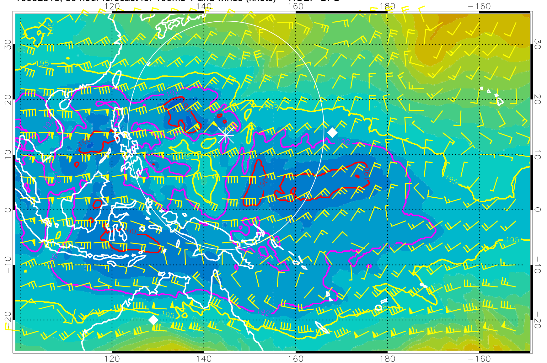
16082318, 30 hour forecast for 100mb T and winds (knots) -- NCEP GFS
