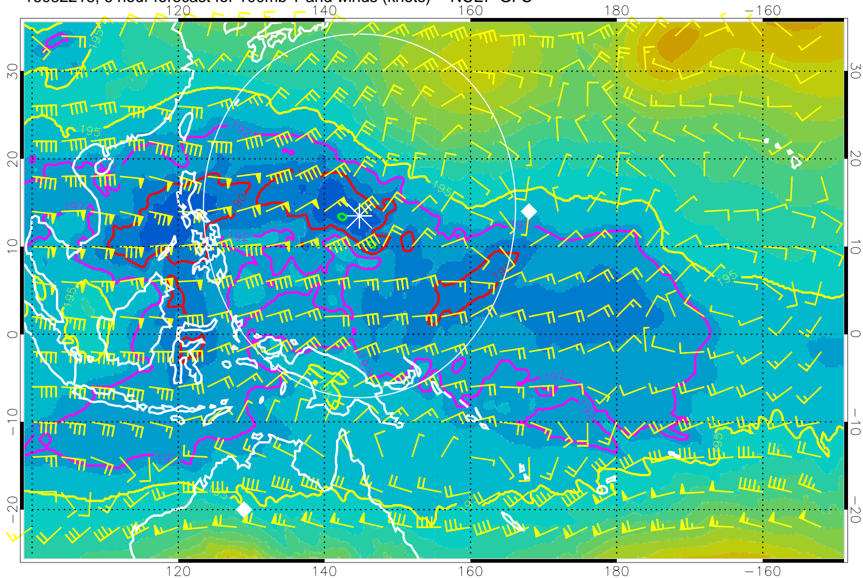
16082218, 6 hour forecast for 100mb T and winds (knots) -- NCEP GFS
