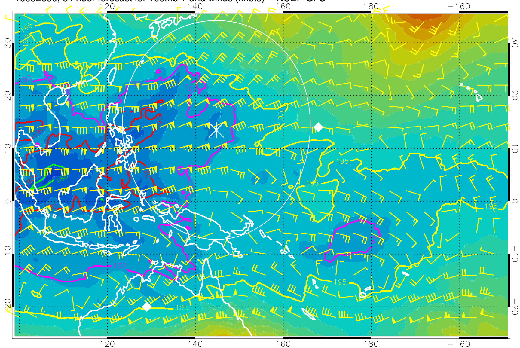
16082600, 84 hour forecast for 100mb T and winds (knots) -- NCEP GFS
