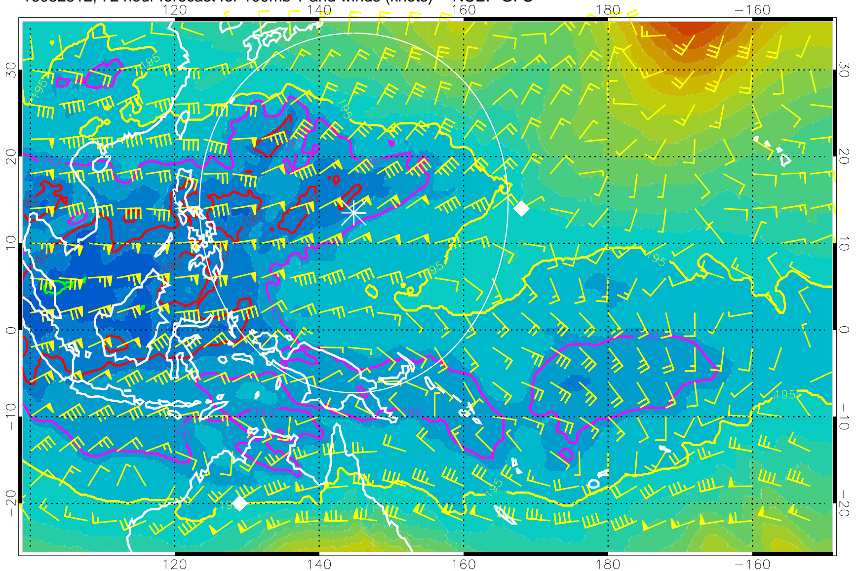
16082512, 72 hour forecast for 100mb T and winds (knots) -- NCEP GFS
