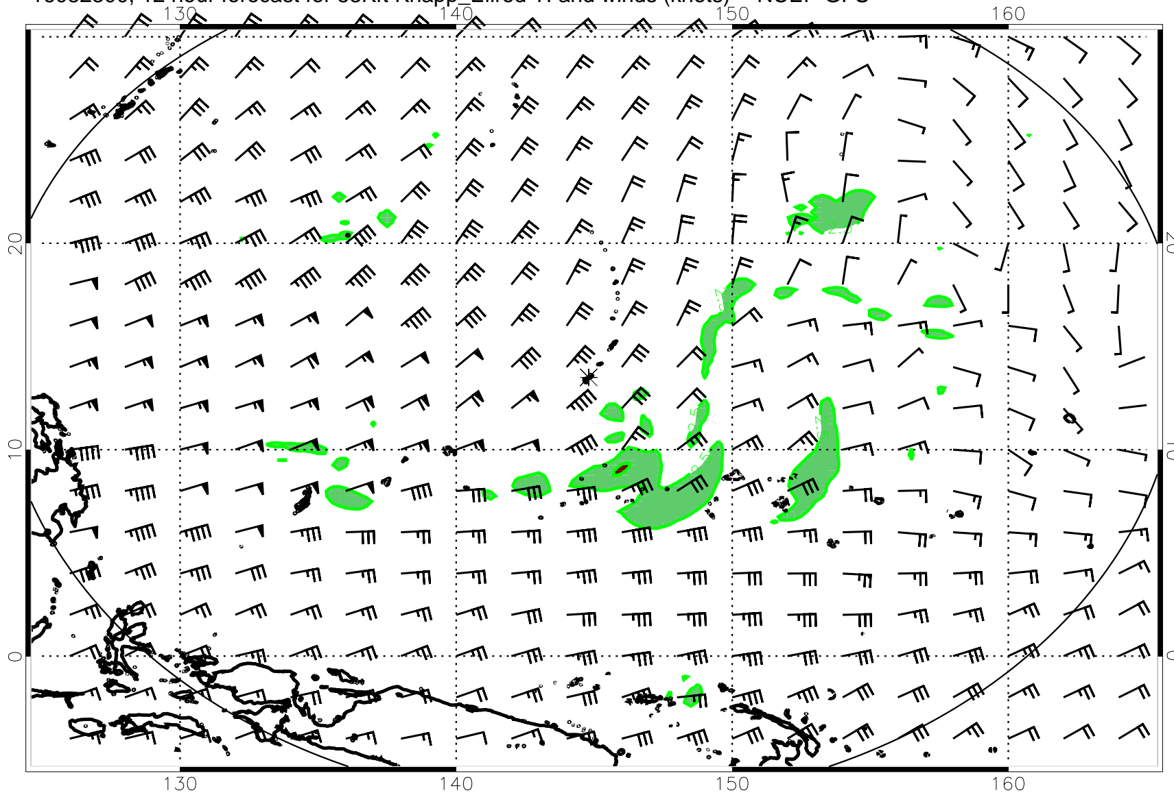
16082300, 12 hour forecast for 53Kft Knapp_Ellrod TI and winds (knots) -- NCEP GFS
