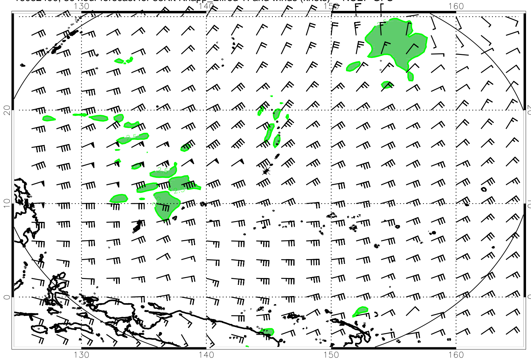
16082400, 36 hour forecast for 53Kft Knapp_Ellrod TI and winds (knots) -- NCEP GFS
