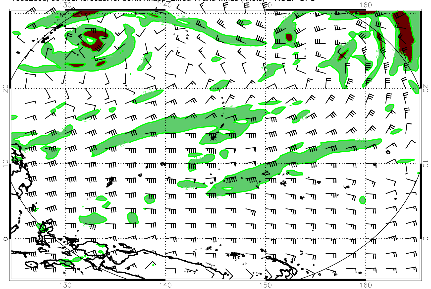
16082606, 90 hour forecast for 36Kft Knapp_Ellrod TI and winds (knots) -- NCEP GFS
