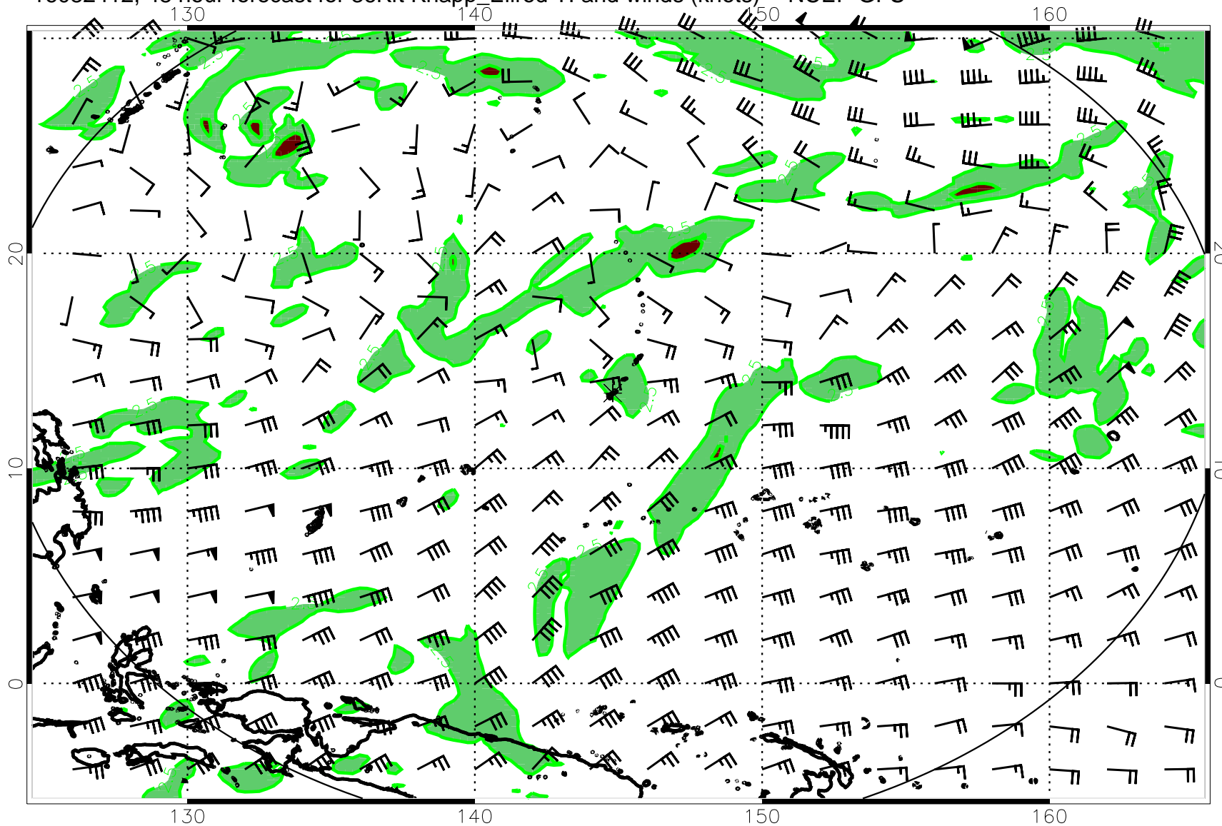
16082412, 48 hour forecast for 36Kft Knapp_Ellrod TI and winds (knots) -- NCEP GFS
