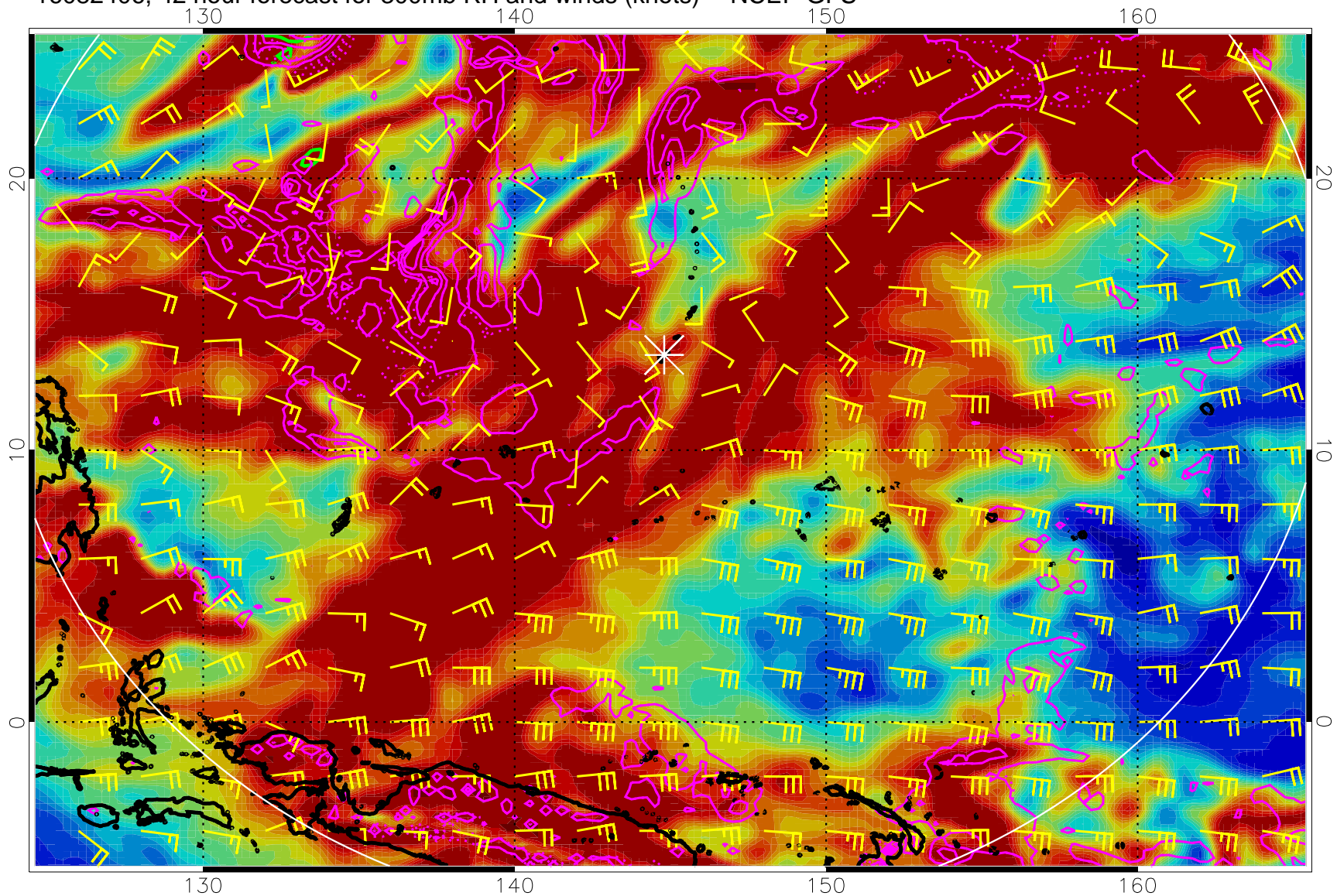
16082406, 42 hour forecast for 300mb RH and winds (knots) -- NCEP GFS
