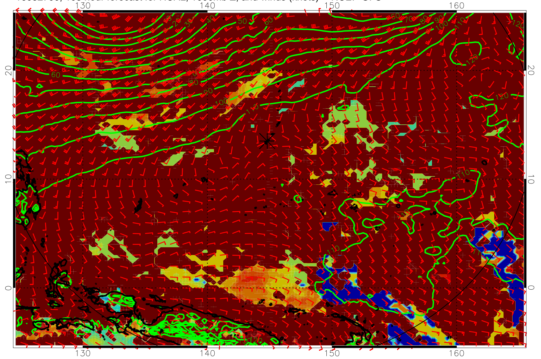
16082700, 108 hour forecast for HCAL, 1000mb Z, and winds (knots) -- NCEP GFS
