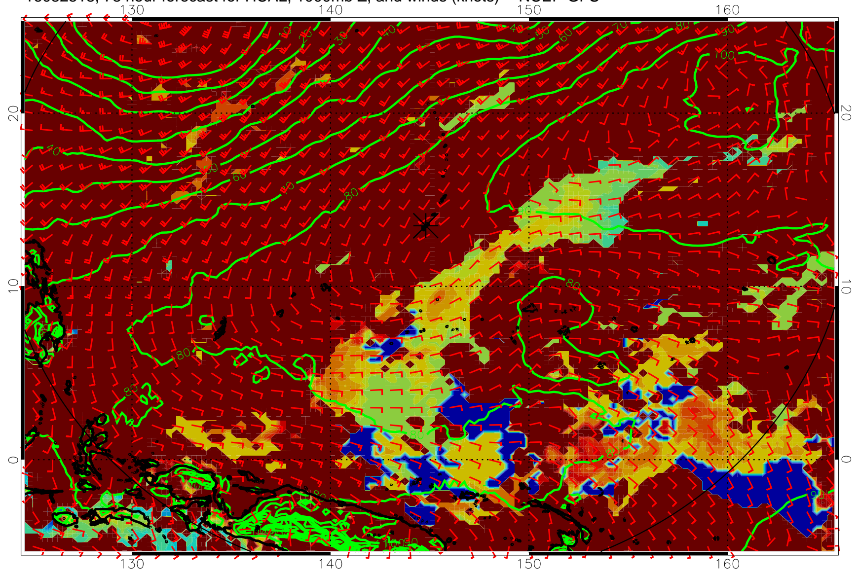
16082518, 78 hour forecast for HCAL, 1000mb Z, and winds (knots) -- NCEP GFS
