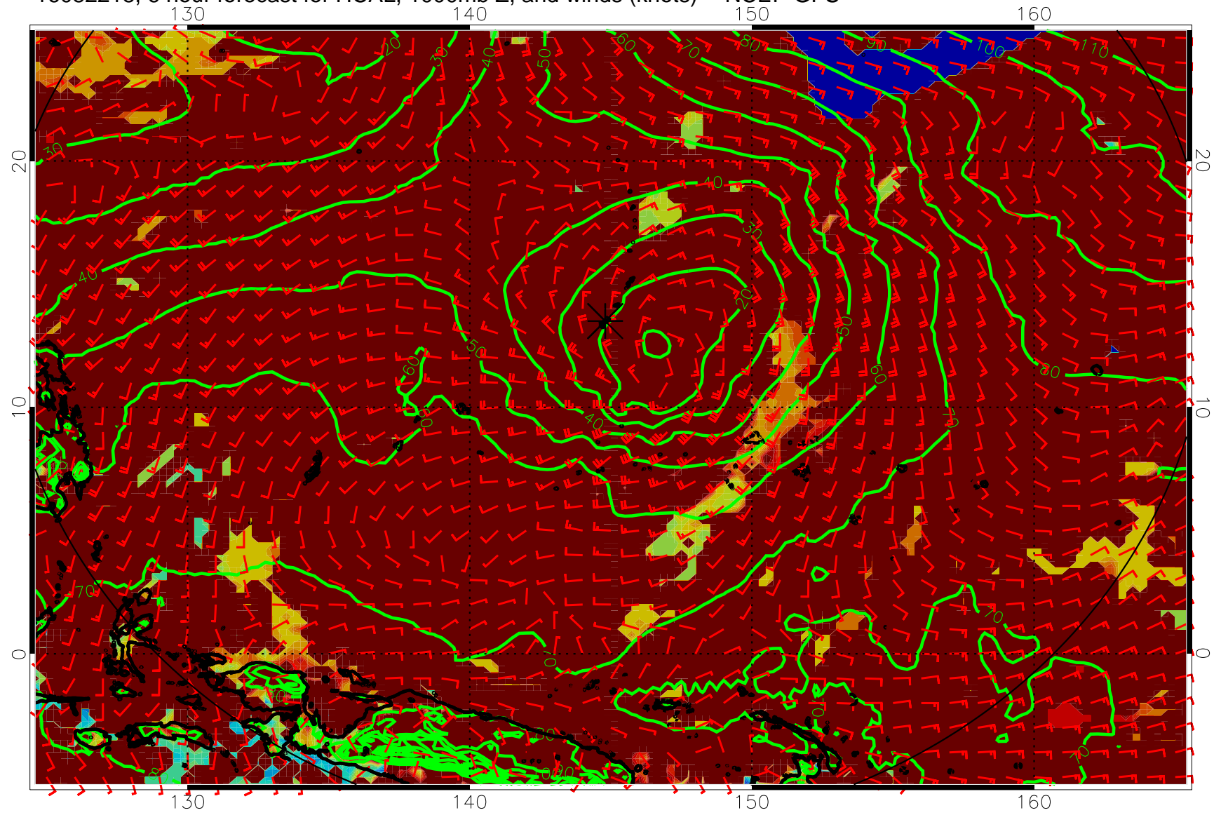
16082218, 6 hour forecast for HCAL, 1000mb Z, and winds (knots) -- NCEP GFS
