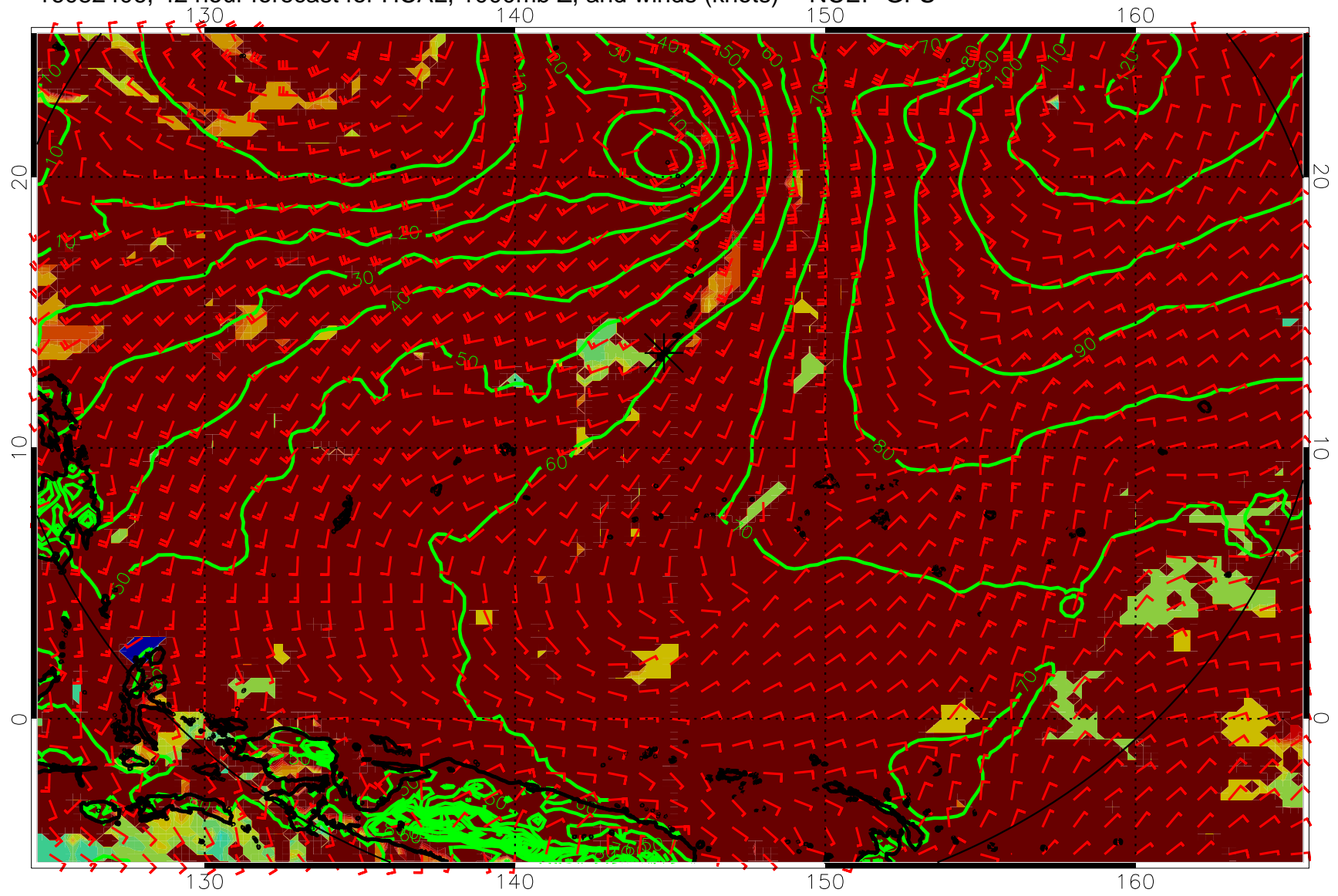
16082406, 42 hour forecast for HCAL, 1000mb Z, and winds (knots) -- NCEP GFS
