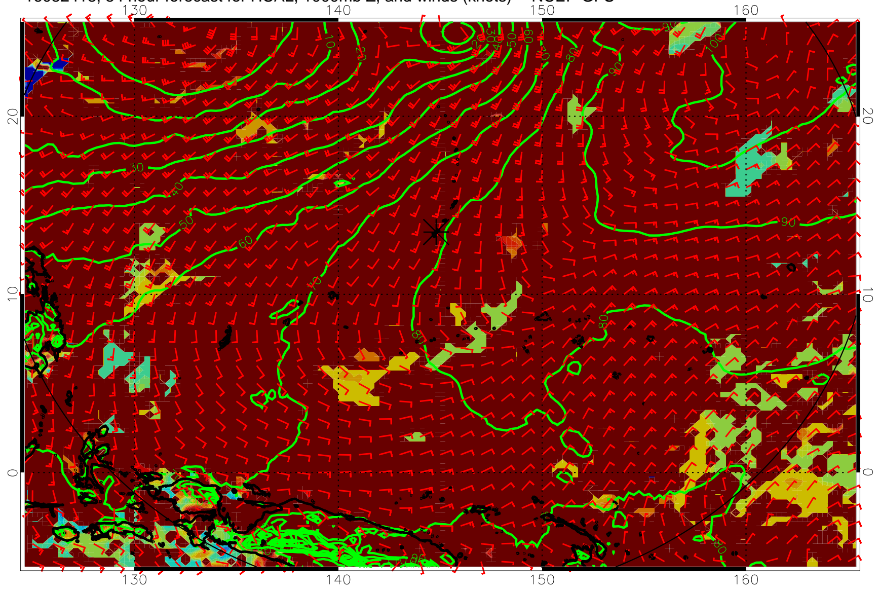
16082418, 54 hour forecast for HCAL, 1000mb Z, and winds (knots) -- NCEP GFS
