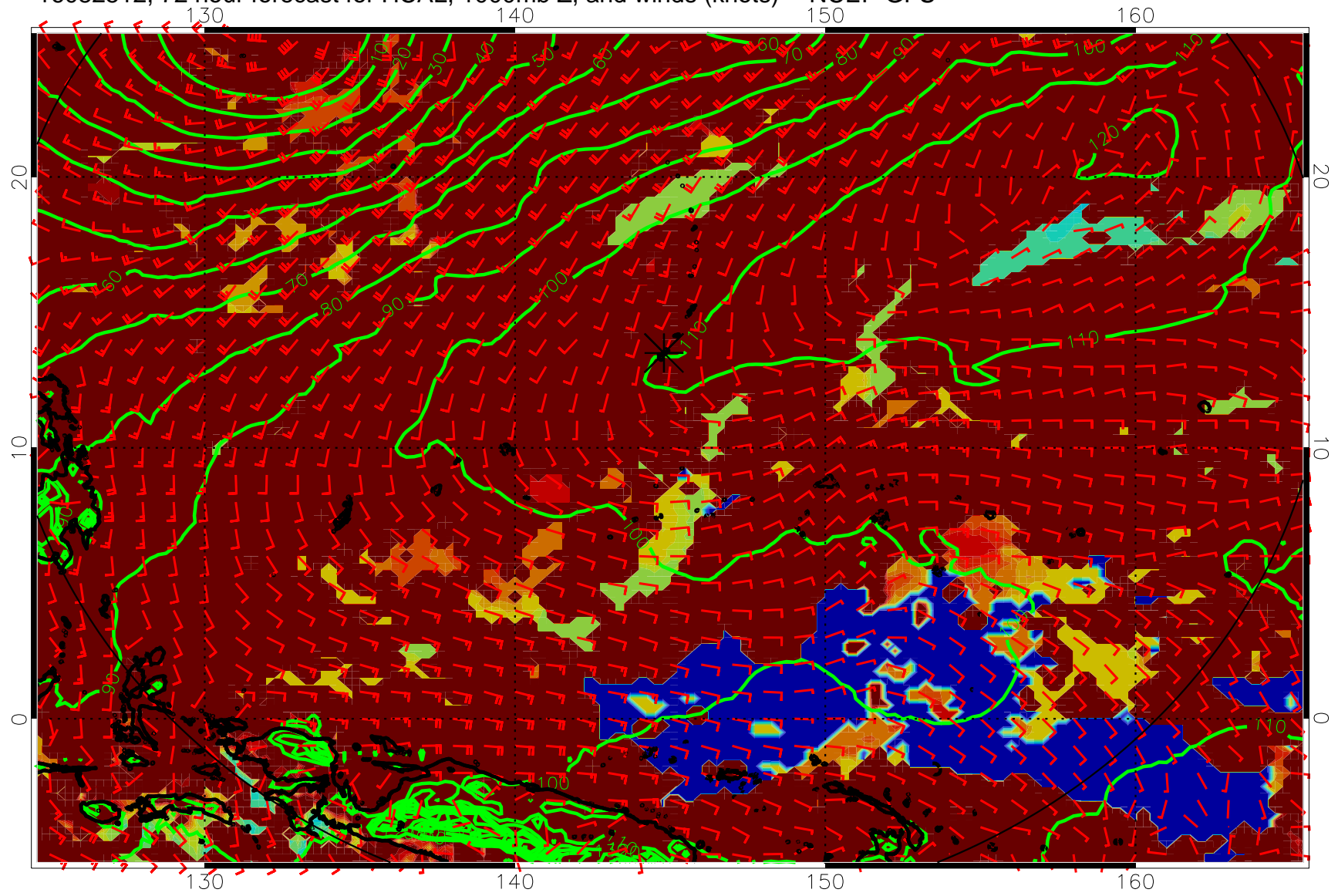
16082512, 72 hour forecast for HCAL, 1000mb Z, and winds (knots) -- NCEP GFS
