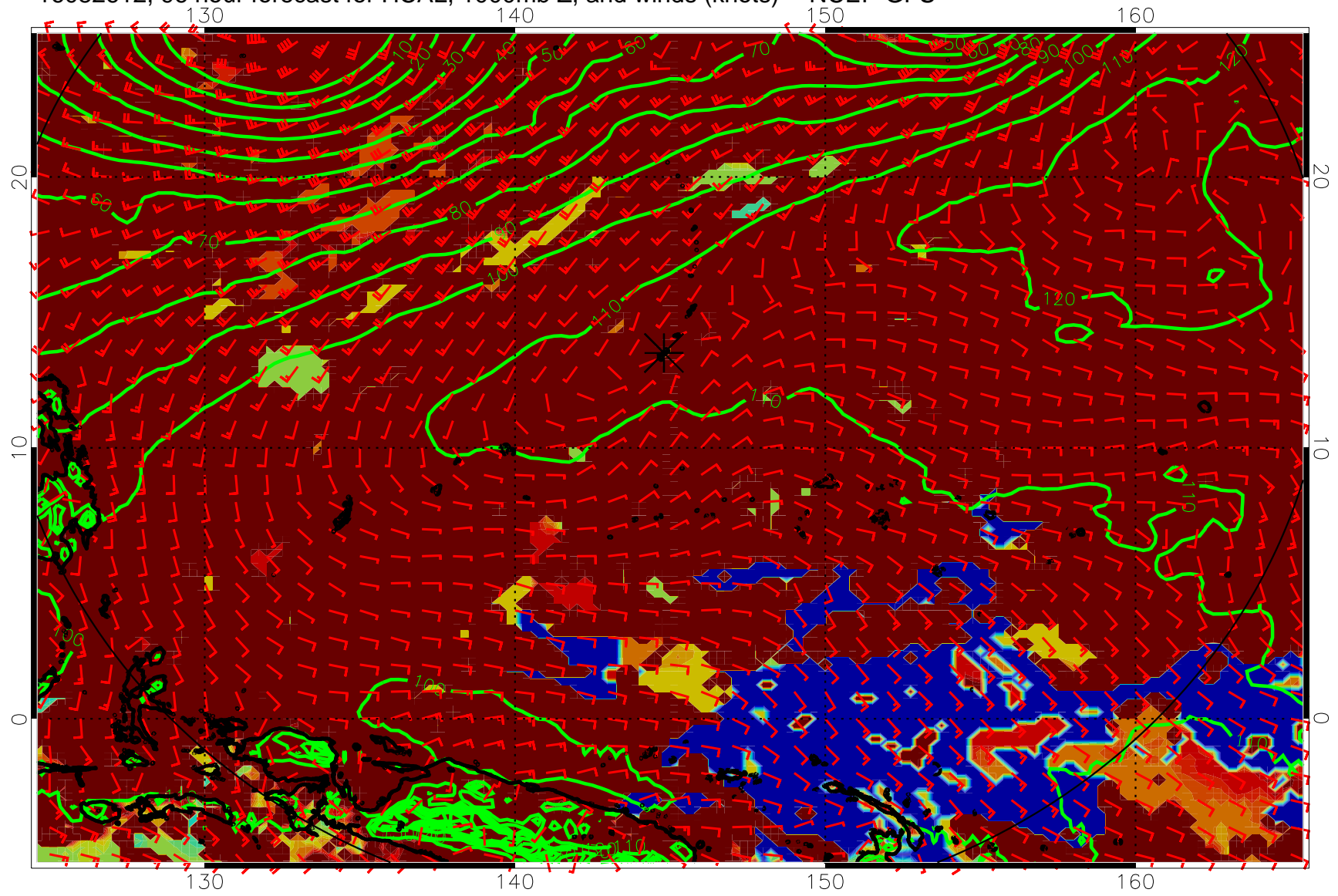
16082612, 96 hour forecast for HCAL, 1000mb Z, and winds (knots) -- NCEP GFS
