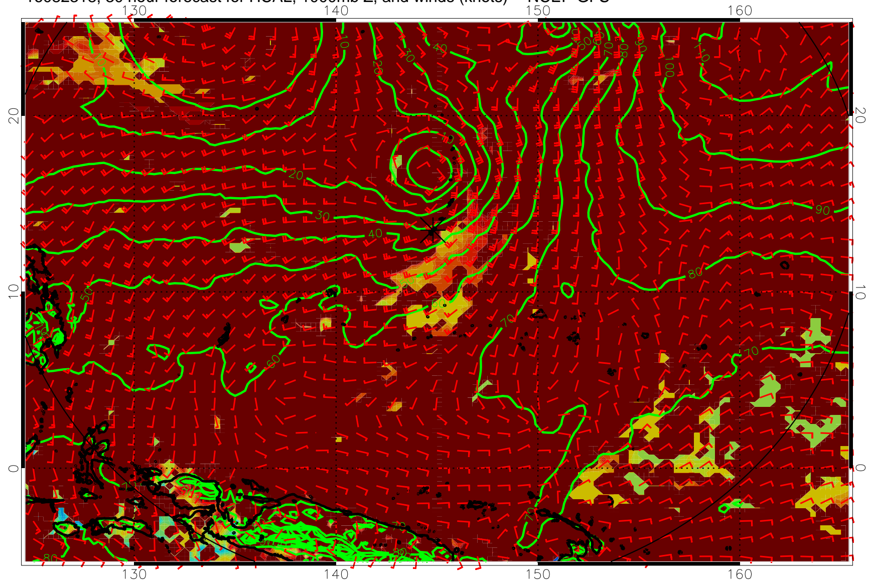
16082318, 30 hour forecast for HCAL, 1000mb Z, and winds (knots) -- NCEP GFS
