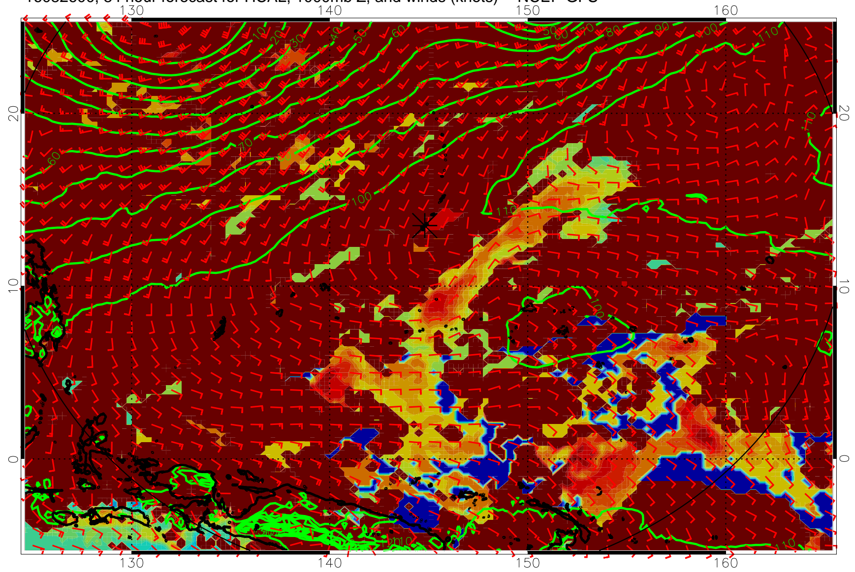
16082600, 84 hour forecast for HCAL, 1000mb Z, and winds (knots) -- NCEP GFS
