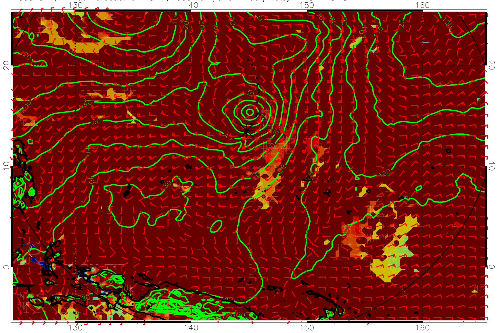
16082312, 24 hour forecast for HCAL, 1000mb Z, and winds (knots) -- NCEP GFS
