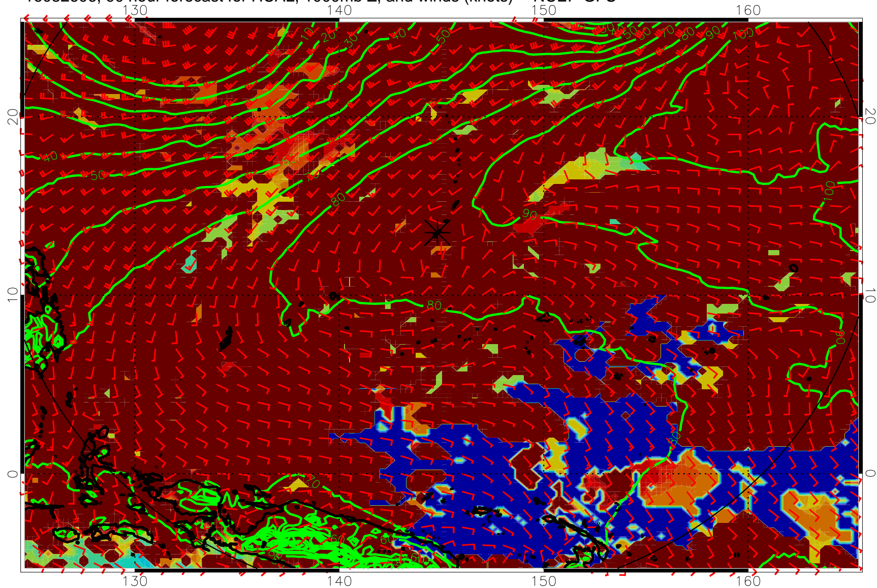
16082606, 90 hour forecast for HCAL, 1000mb Z, and winds (knots) -- NCEP GFS
