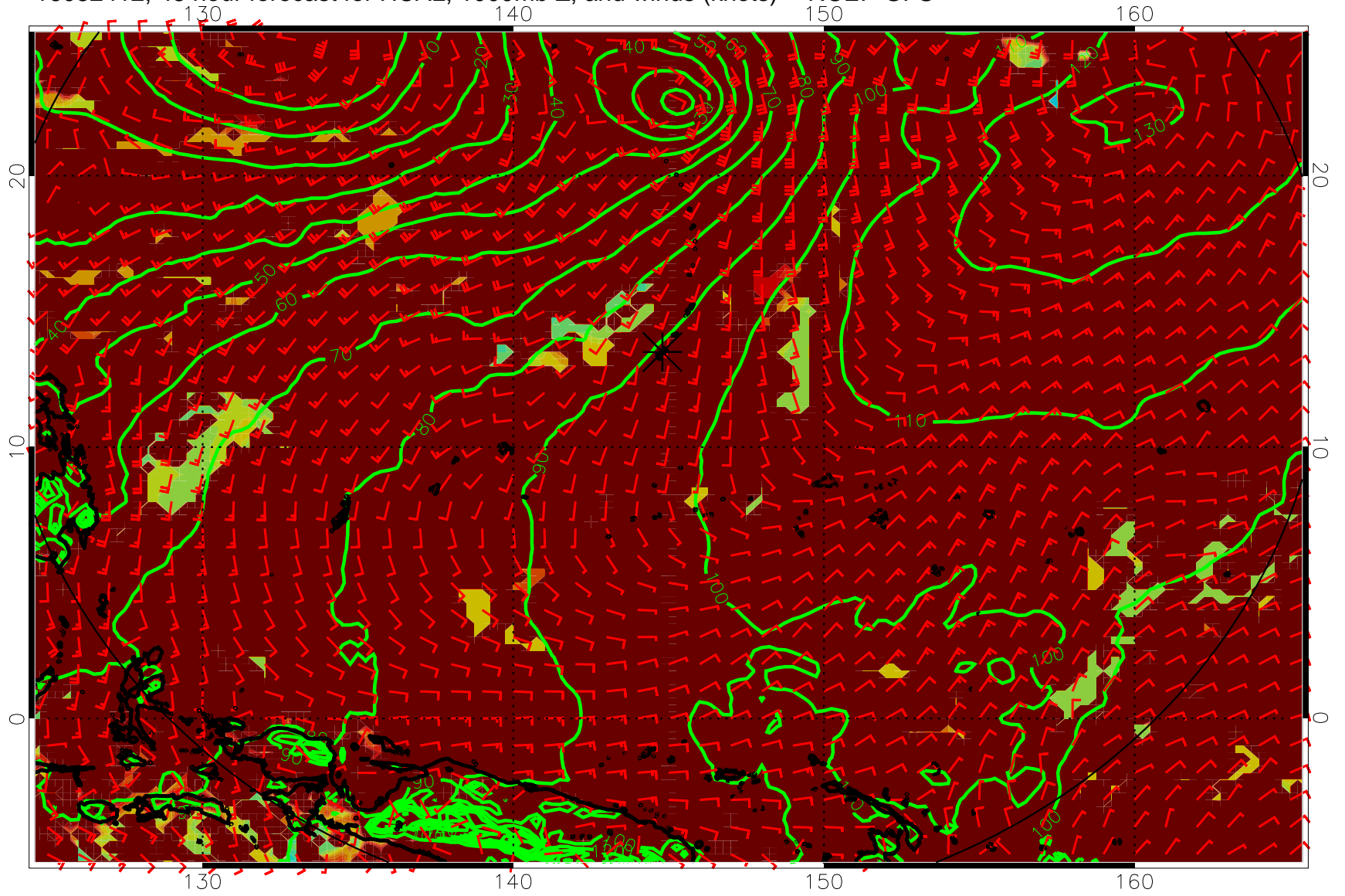
16082412, 48 hour forecast for HCAL, 1000mb Z, and winds (knots) -- NCEP GFS
