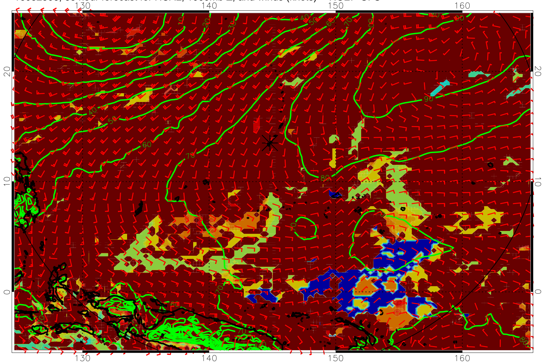
16082506, 66 hour forecast for HCAL, 1000mb Z, and winds (knots) -- NCEP GFS
