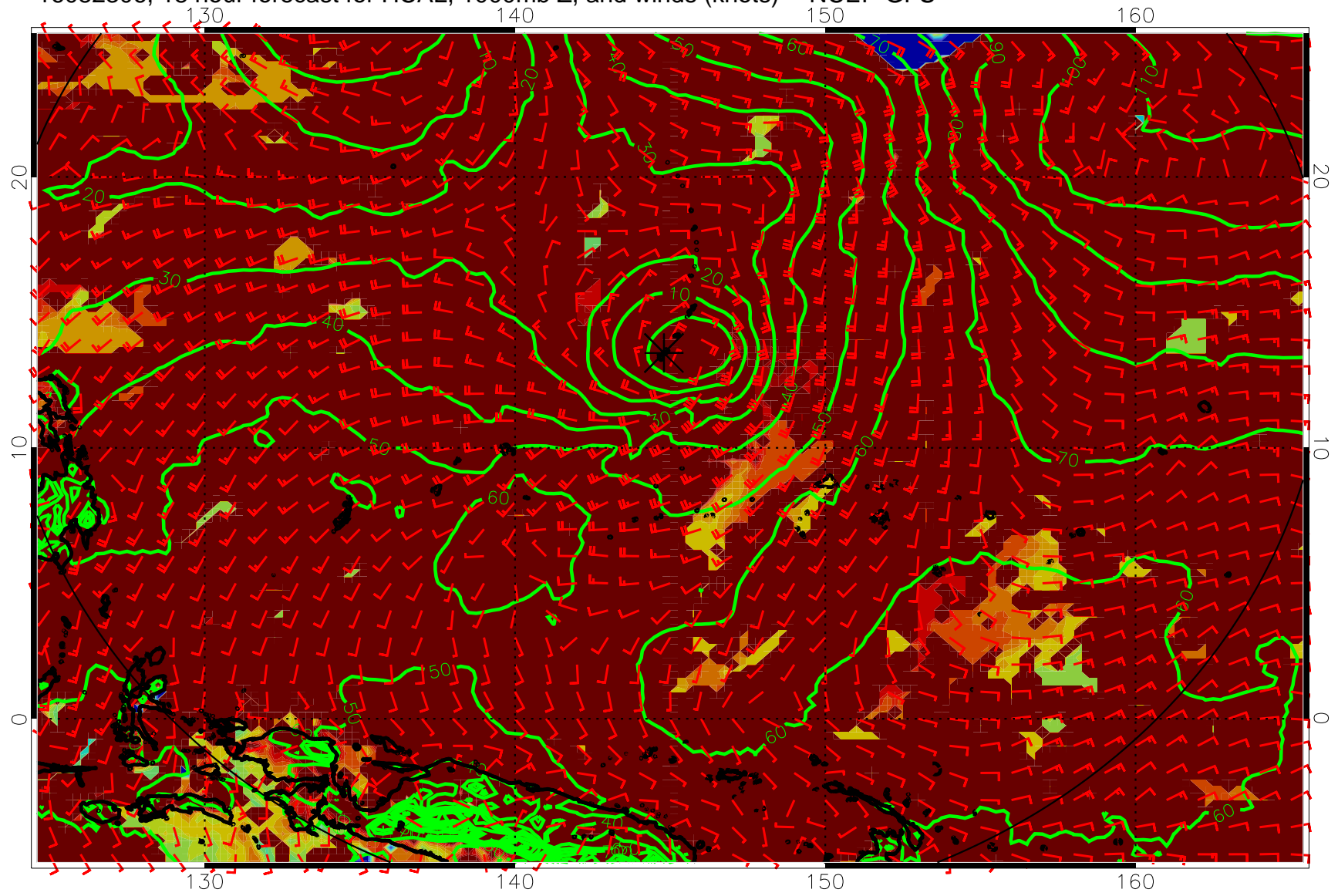
16082306, 18 hour forecast for HCAL, 1000mb Z, and winds (knots) -- NCEP GFS
