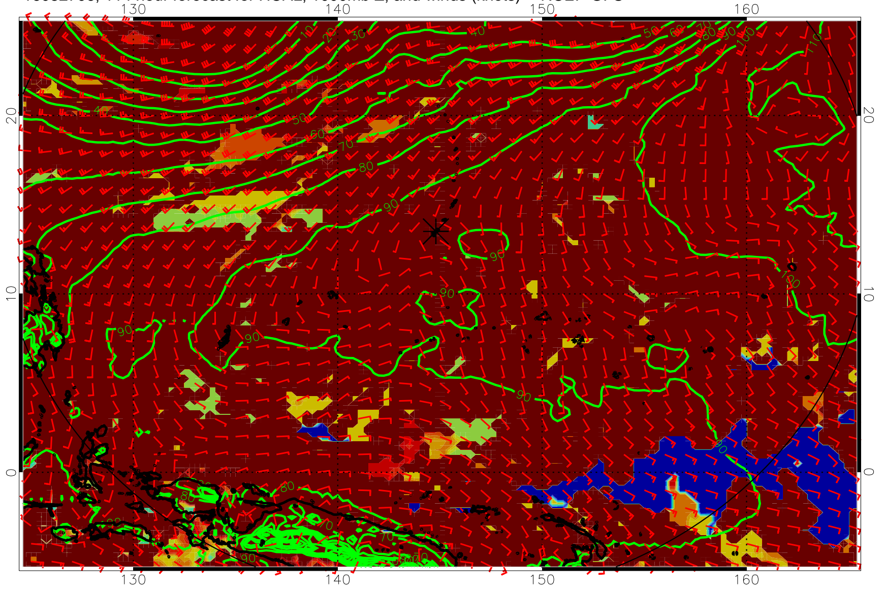
16082706, 114 hour forecast for HCAL, 1000mb Z, and winds (knots) -- NCEP GFS
