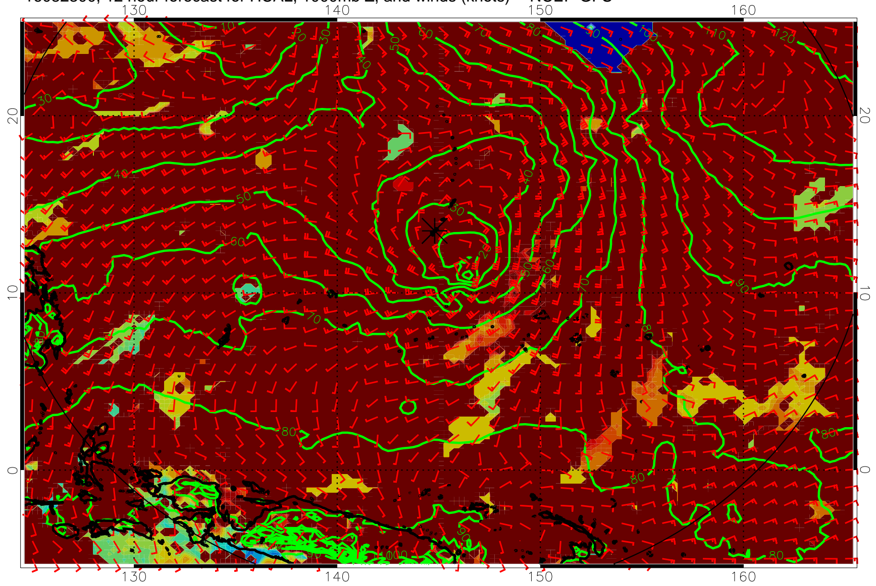
16082300, 12 hour forecast for HCAL, 1000mb Z, and winds (knots) -- NCEP GFS
