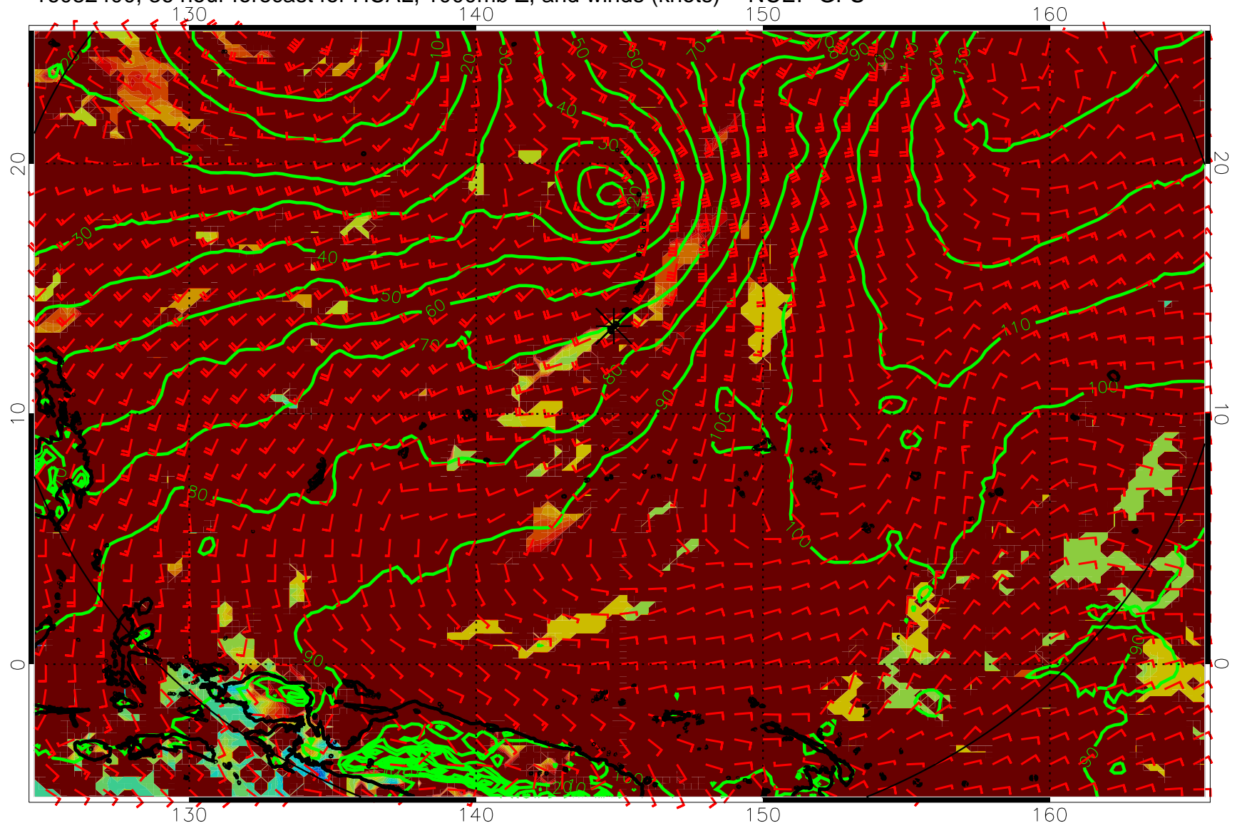
16082400, 36 hour forecast for HCAL, 1000mb Z, and winds (knots) -- NCEP GFS
