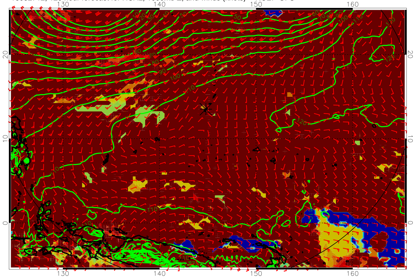
16082712, 120 hour forecast for HCAL, 1000mb Z, and winds (knots) -- NCEP GFS
