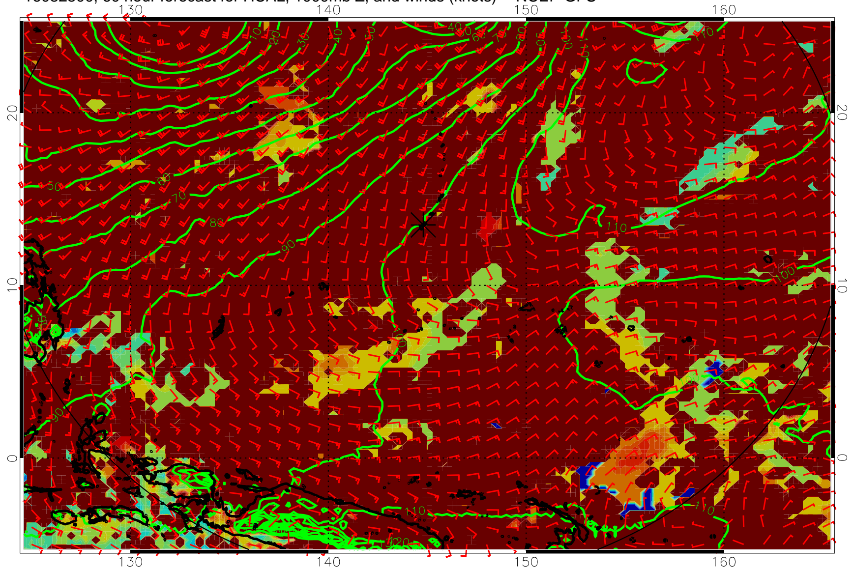
16082500, 60 hour forecast for HCAL, 1000mb Z, and winds (knots) -- NCEP GFS
