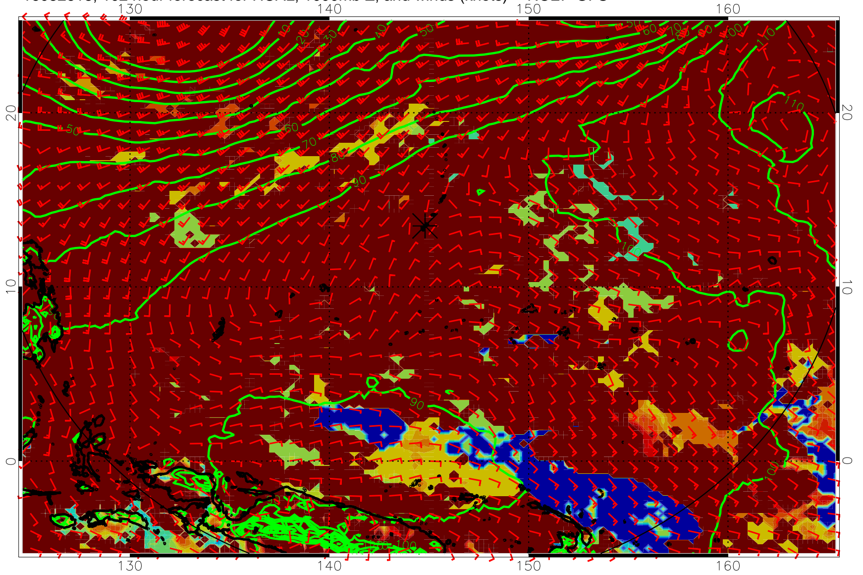
16082618, 102 hour forecast for HCAL, 1000mb Z, and winds (knots) -- NCEP GFS
