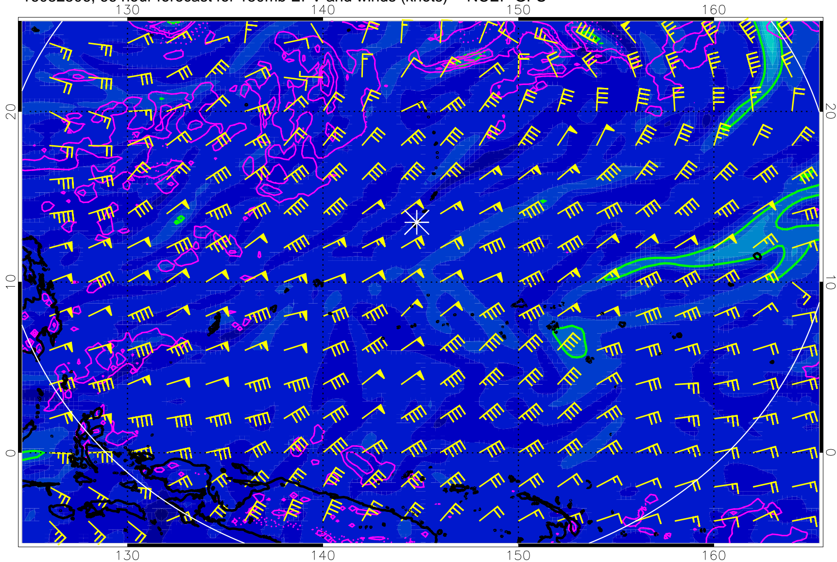
16082506, 66 hour forecast for 150mb EPV and winds (knots) -- NCEP GFS
