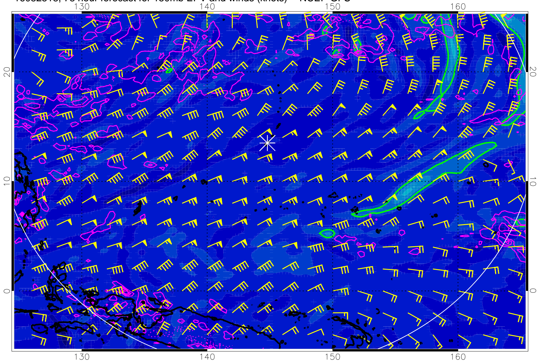
16082518, 78 hour forecast for 150mb EPV and winds (knots) -- NCEP GFS
