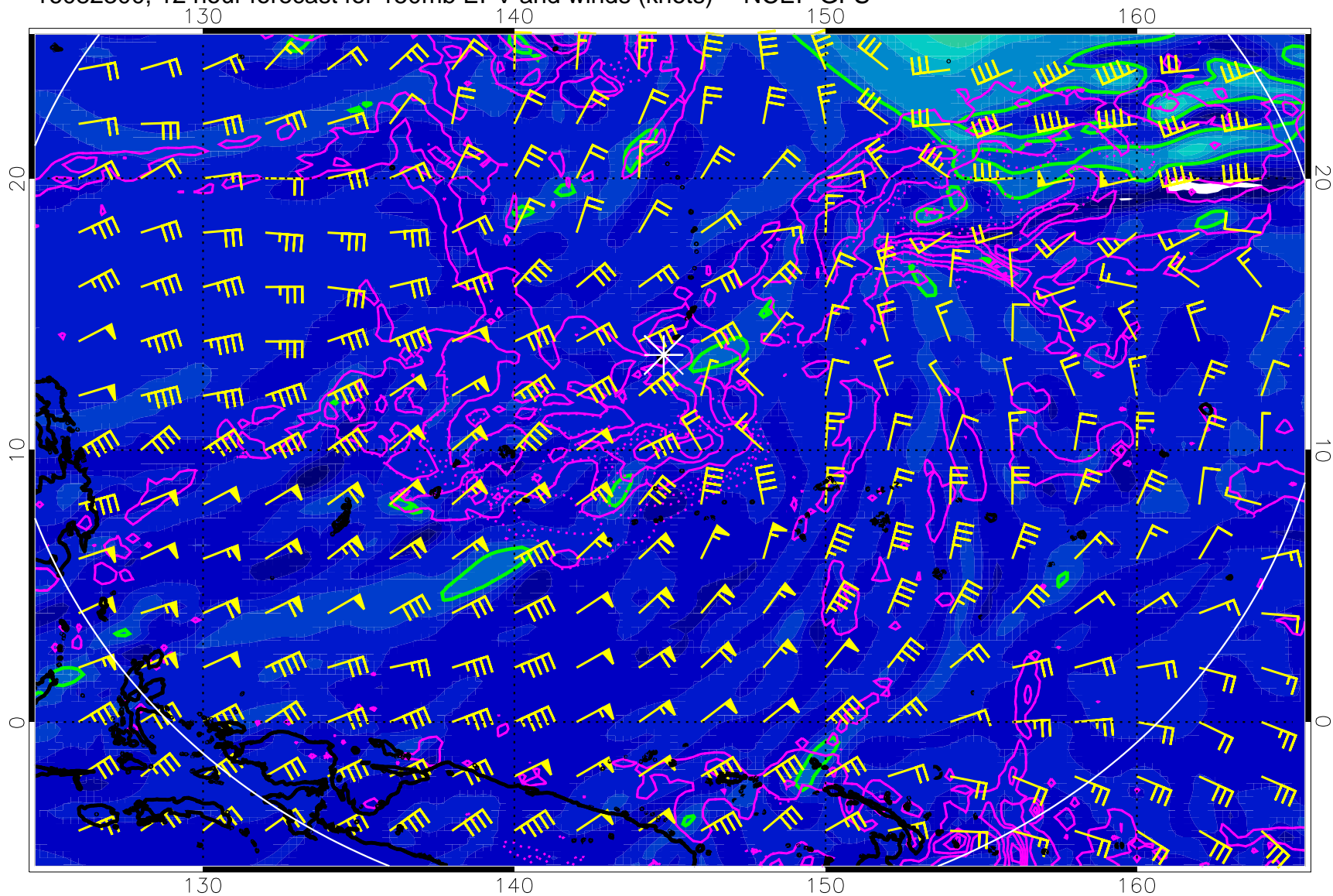
16082300, 12 hour forecast for 150mb EPV and winds (knots) -- NCEP GFS
