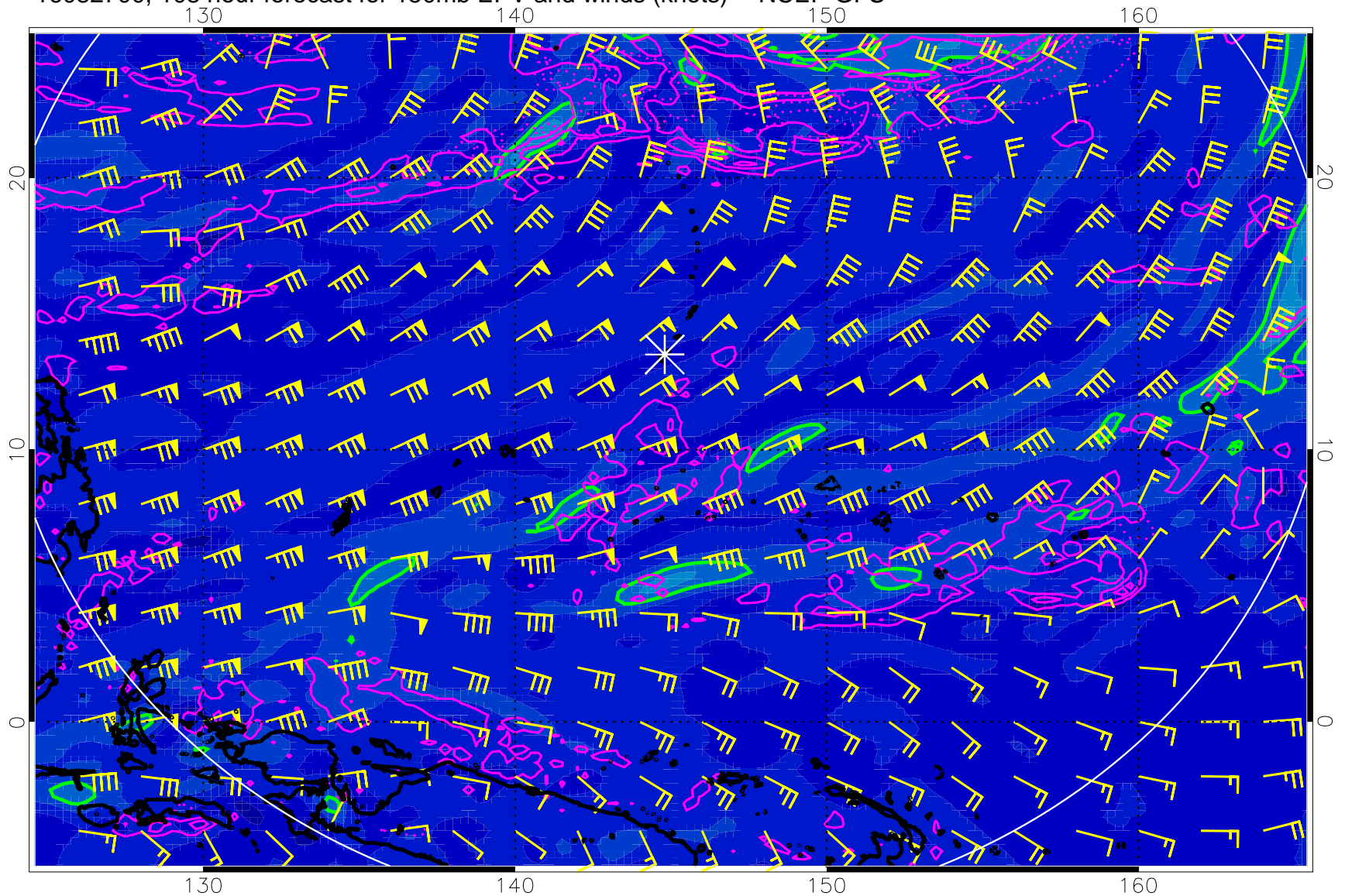
16082700, 108 hour forecast for 150mb EPV and winds (knots) -- NCEP GFS
