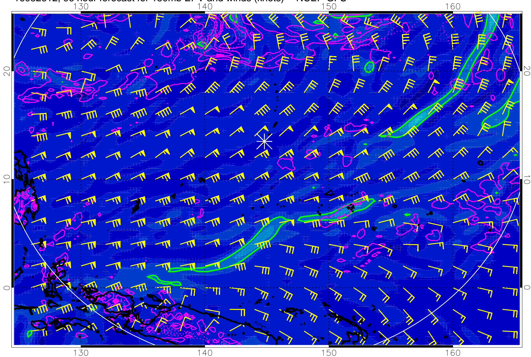
16082612, 96 hour forecast for 150mb EPV and winds (knots) -- NCEP GFS
