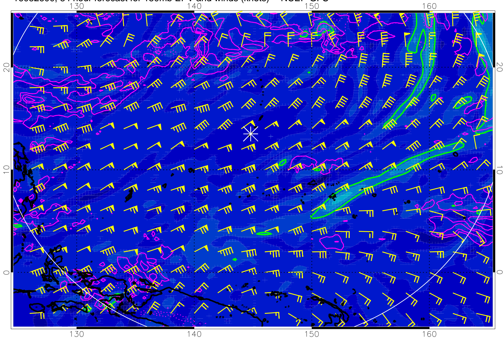
16082600, 84 hour forecast for 150mb EPV and winds (knots) -- NCEP GFS
