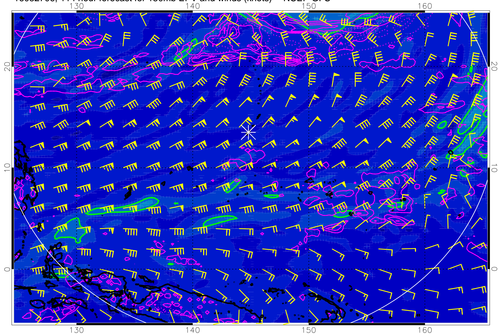
16082706, 114 hour forecast for 150mb EPV and winds (knots) -- NCEP GFS
