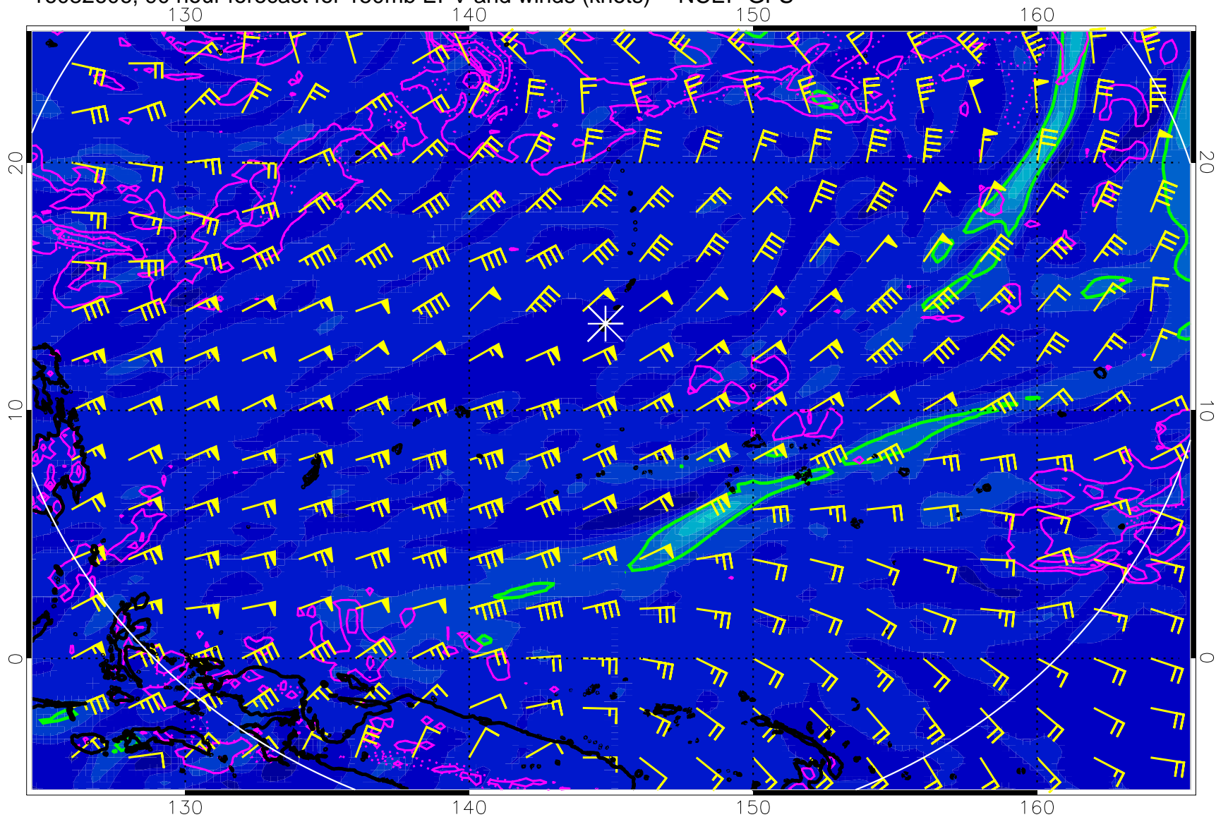
16082606, 90 hour forecast for 150mb EPV and winds (knots) -- NCEP GFS
