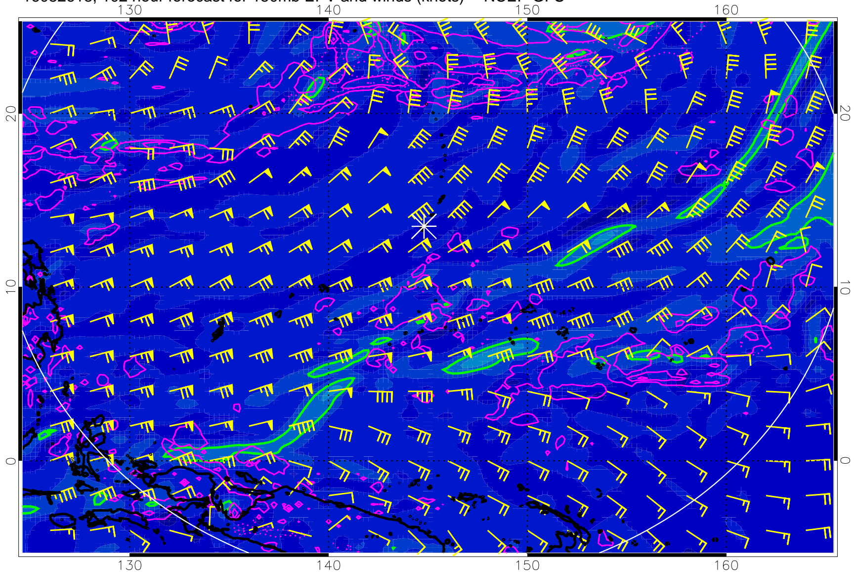
16082618, 102 hour forecast for 150mb EPV and winds (knots) -- NCEP GFS
