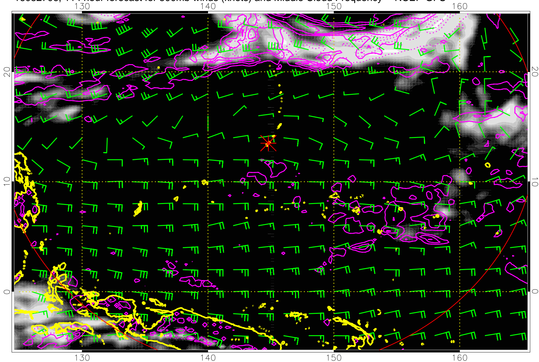
16082706, 114 hour forecast for 500mb winds (knots) and Middle Cloud Frequency -- NCEP GFS
