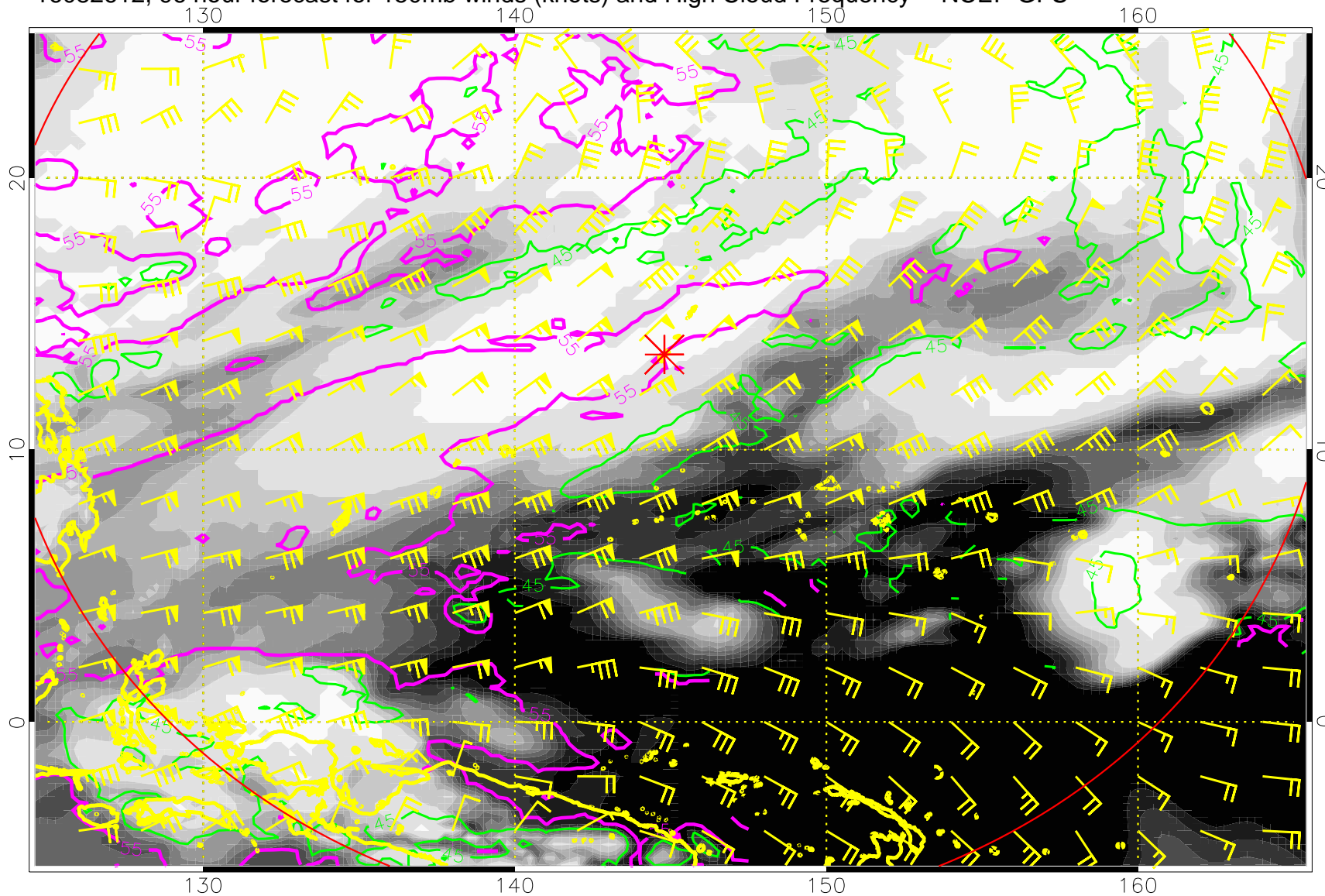
16082612, 96 hour forecast for 150mb winds (knots) and High Cloud Frequency -- NCEP GFS
