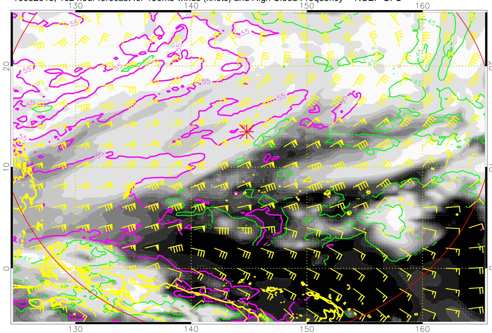
16082618, 102 hour forecast for 150mb winds (knots) and High Cloud Frequency -- NCEP GFS
