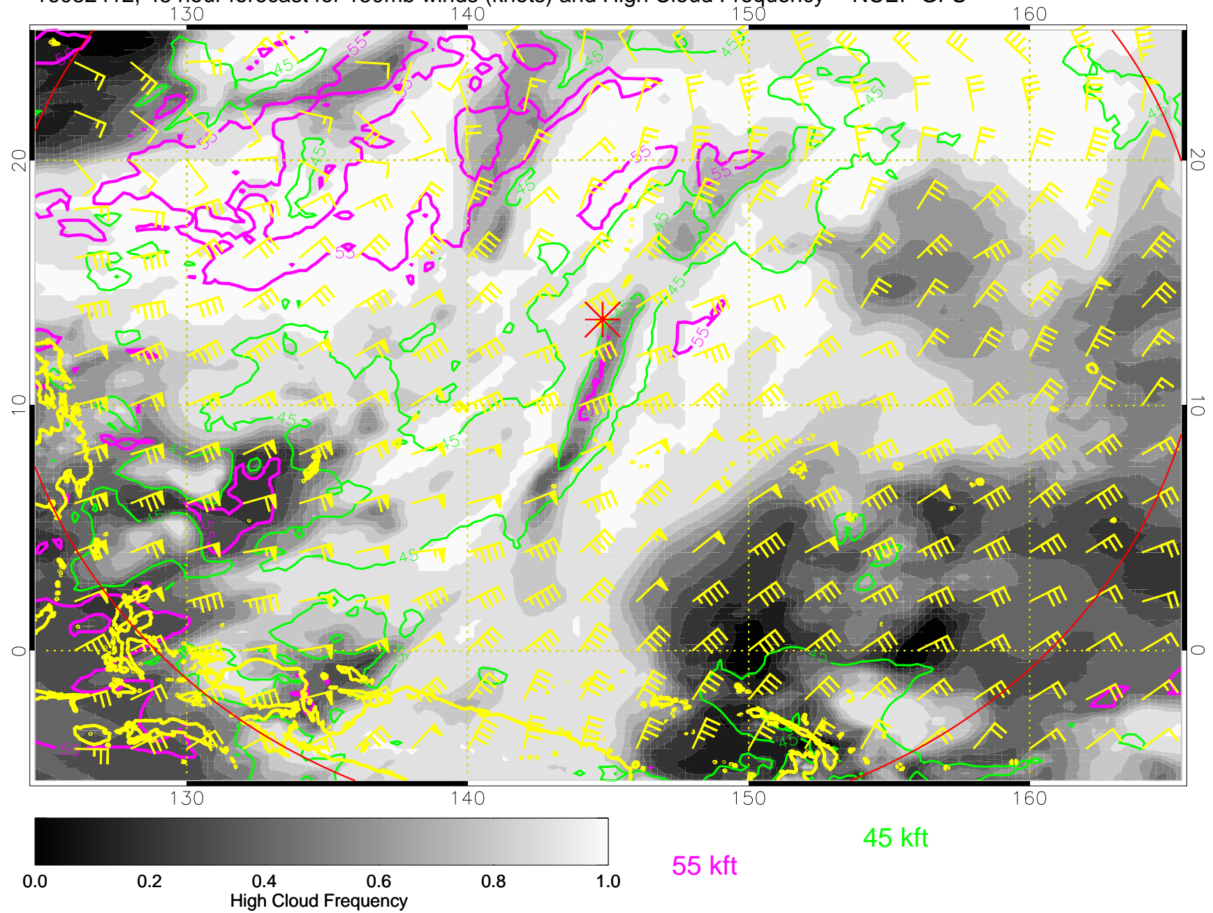
16082412, 48 hour forecast for 150mb winds (knots) and High Cloud Frequency -- NCEP GFS
