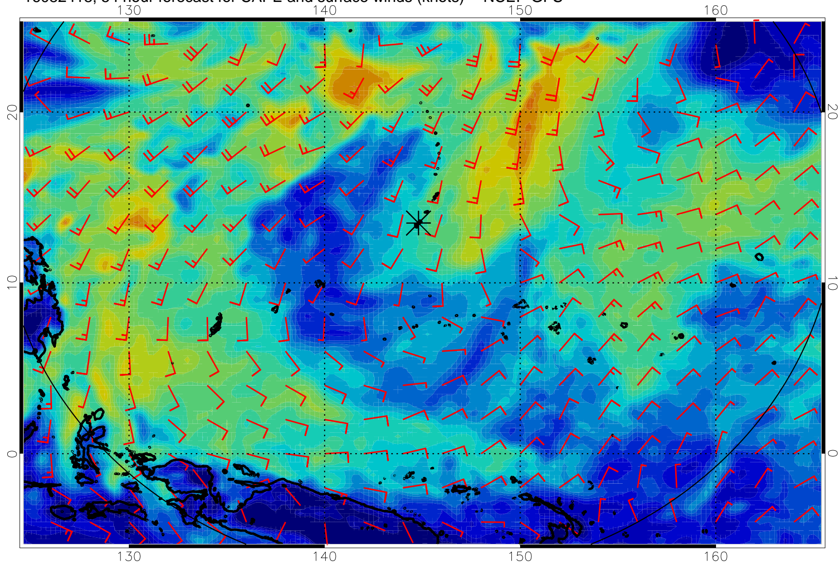
16082418, 54 hour forecast for CAPE and surface winds (knots) -- NCEP GFS
