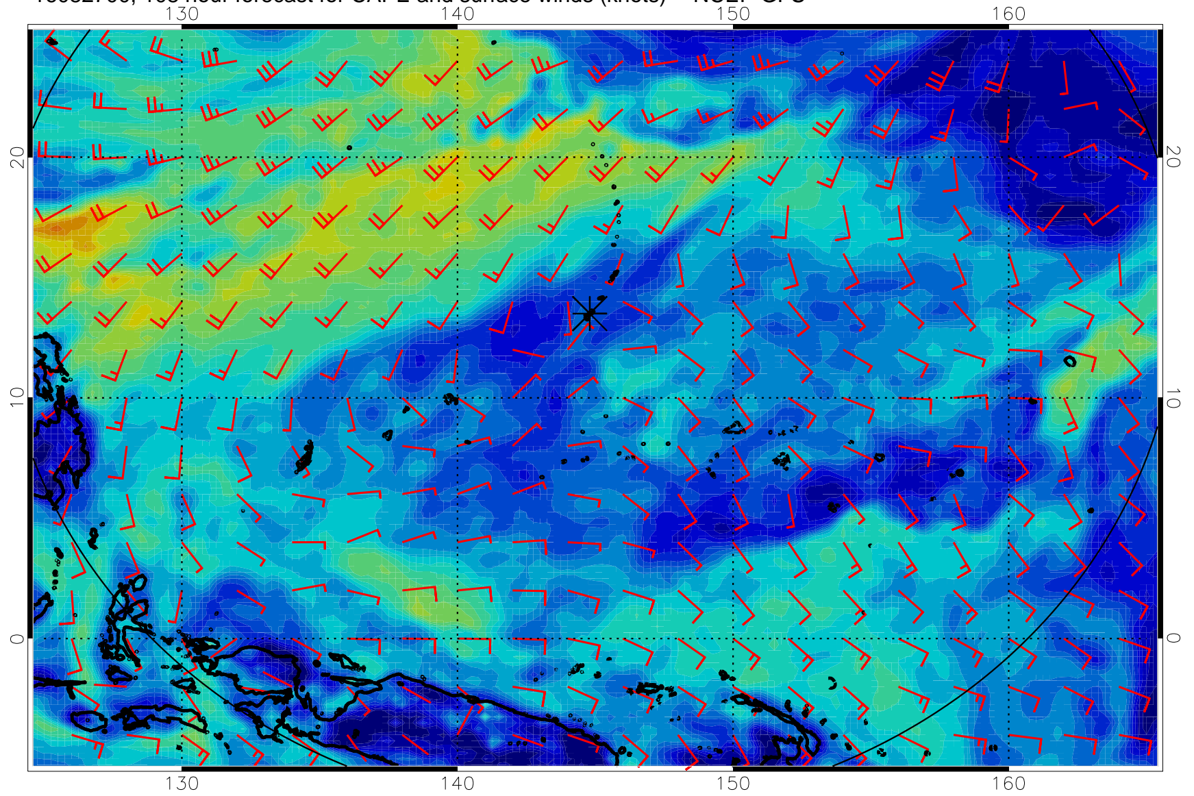
16082700, 108 hour forecast for CAPE and surface winds (knots) -- NCEP GFS
