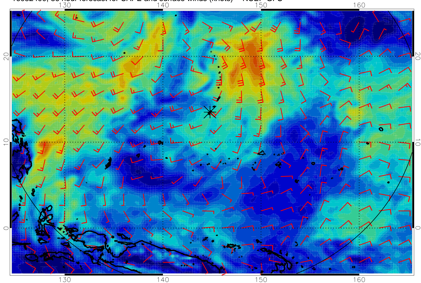
16082400, 36 hour forecast for CAPE and surface winds (knots) -- NCEP GFS
