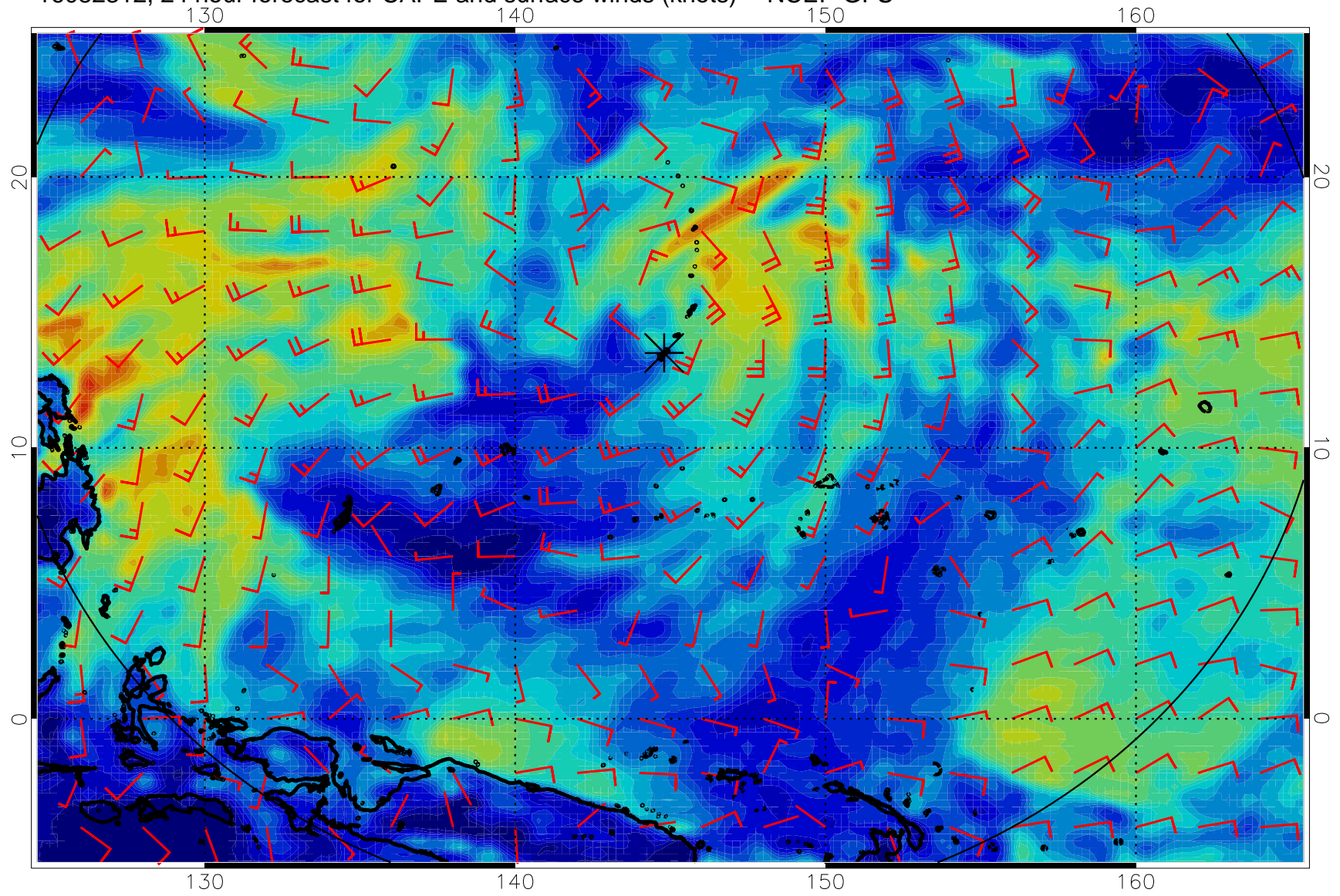
16082312, 24 hour forecast for CAPE and surface winds (knots) -- NCEP GFS
