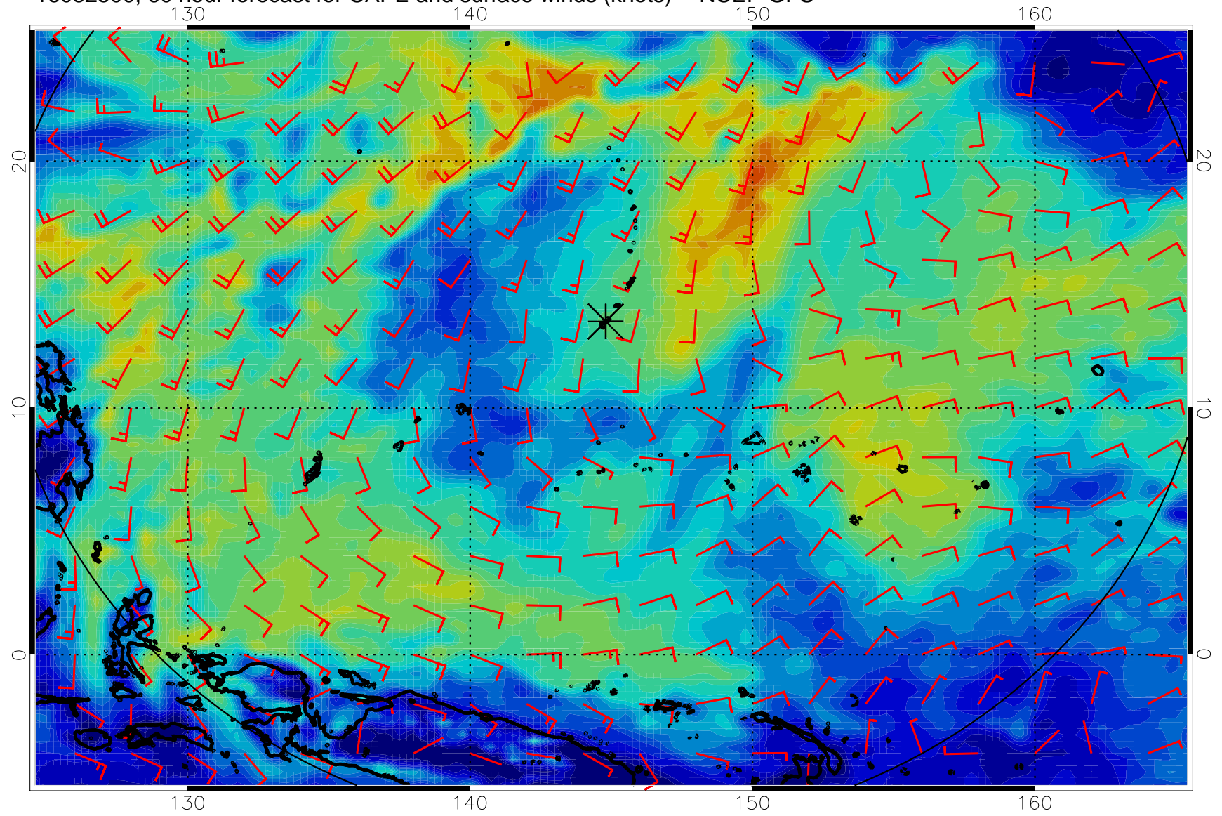
16082500, 60 hour forecast for CAPE and surface winds (knots) -- NCEP GFS
