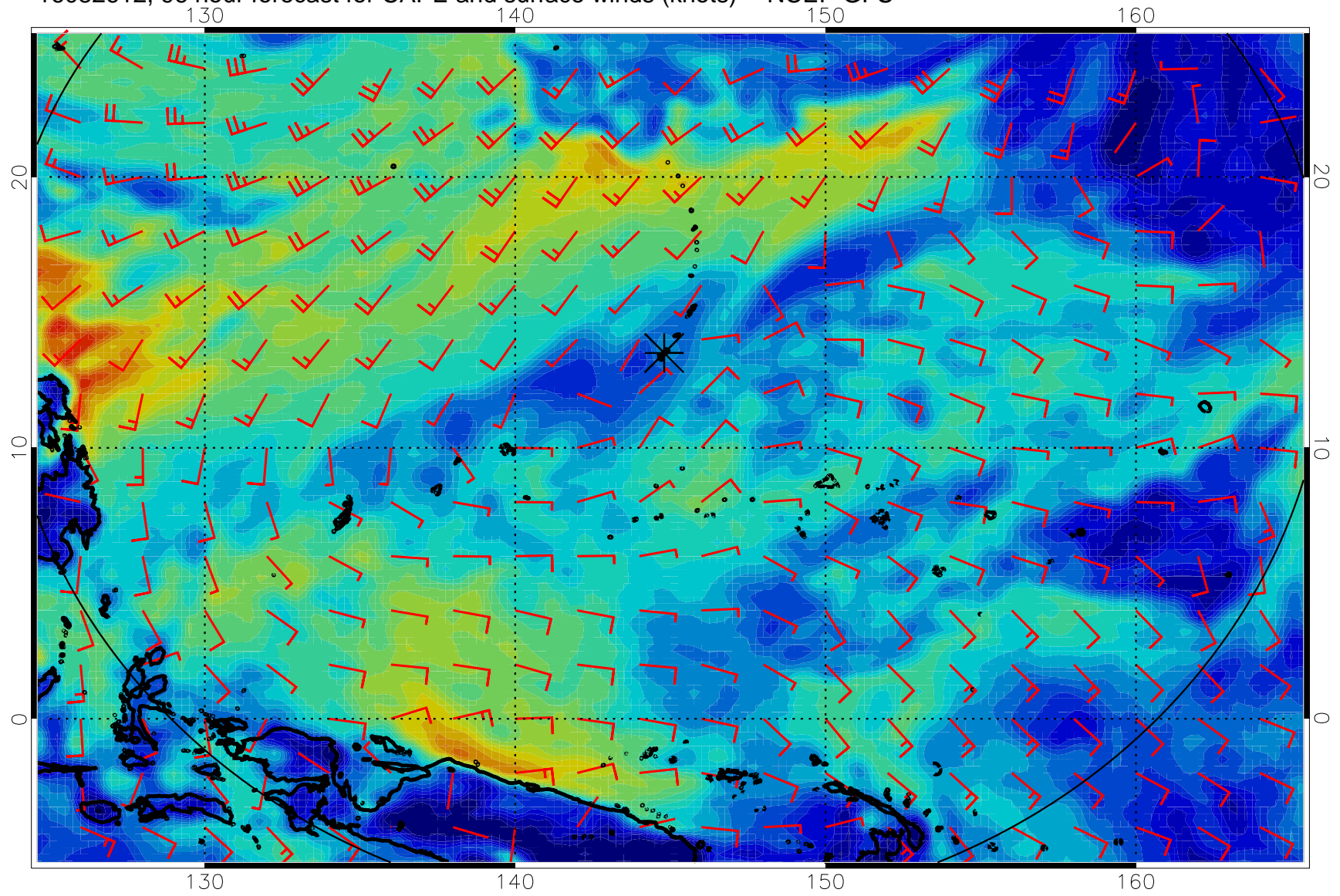
16082612, 96 hour forecast for CAPE and surface winds (knots) -- NCEP GFS
