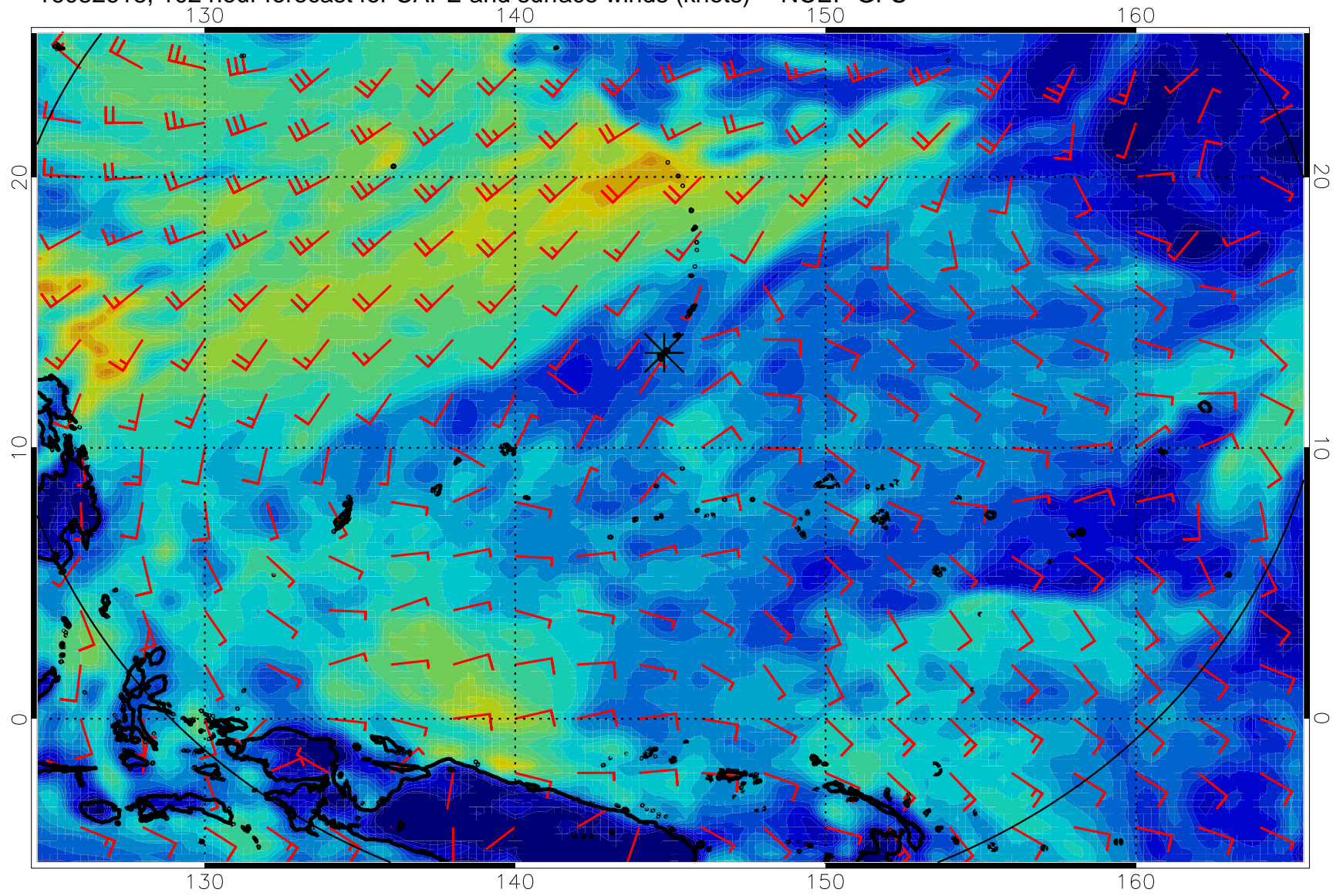
16082618, 102 hour forecast for CAPE and surface winds (knots) -- NCEP GFS
