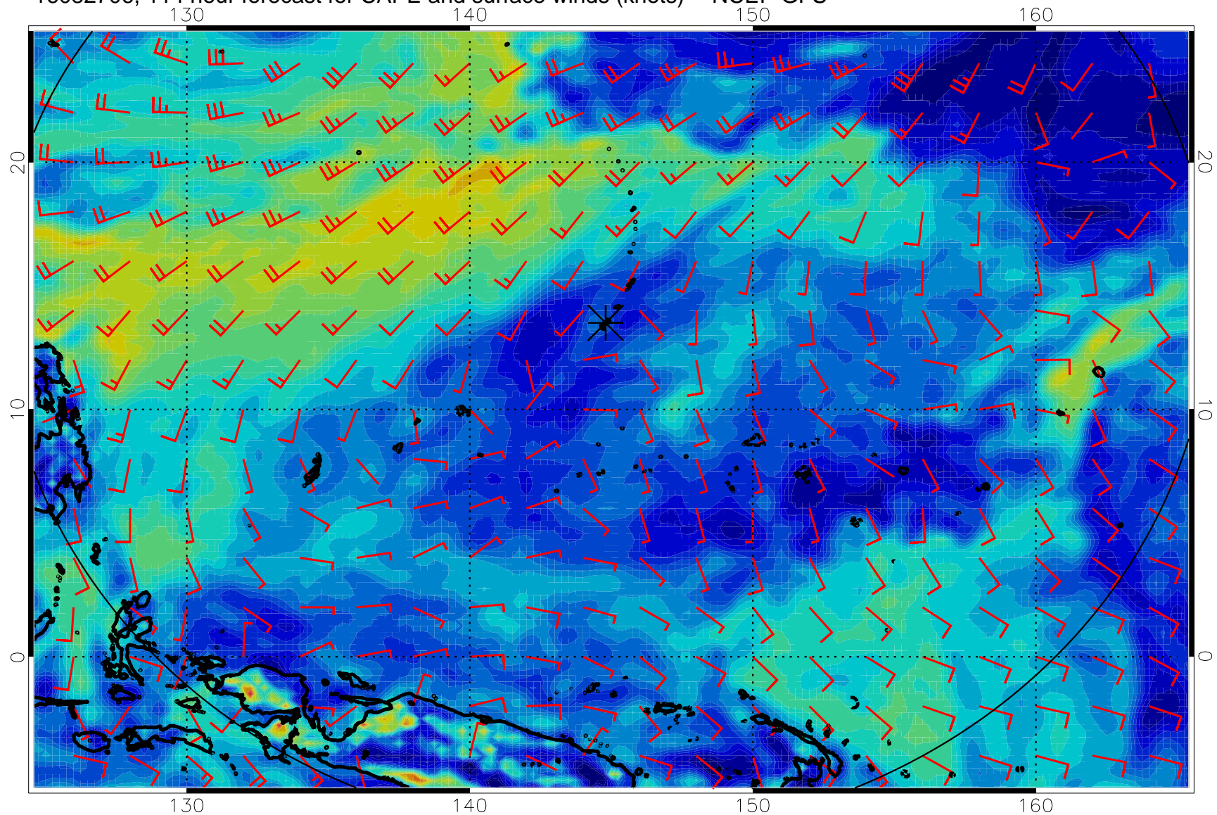
16082706, 114 hour forecast for CAPE and surface winds (knots) -- NCEP GFS
