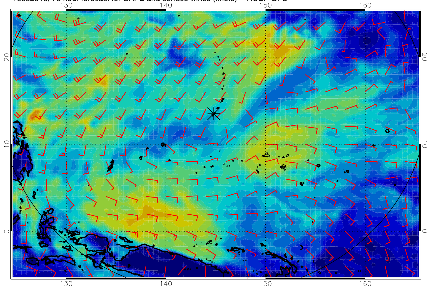
16082518, 78 hour forecast for CAPE and surface winds (knots) -- NCEP GFS
