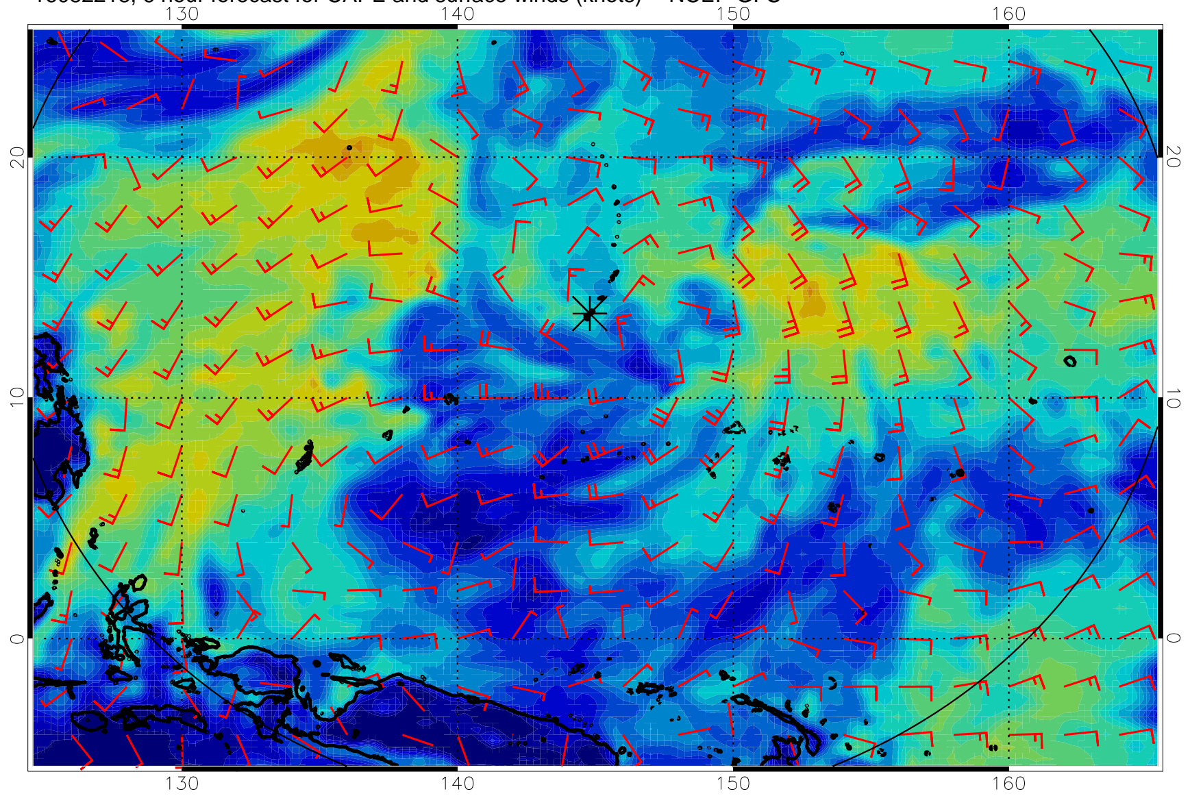
16082218, 6 hour forecast for CAPE and surface winds (knots) -- NCEP GFS
