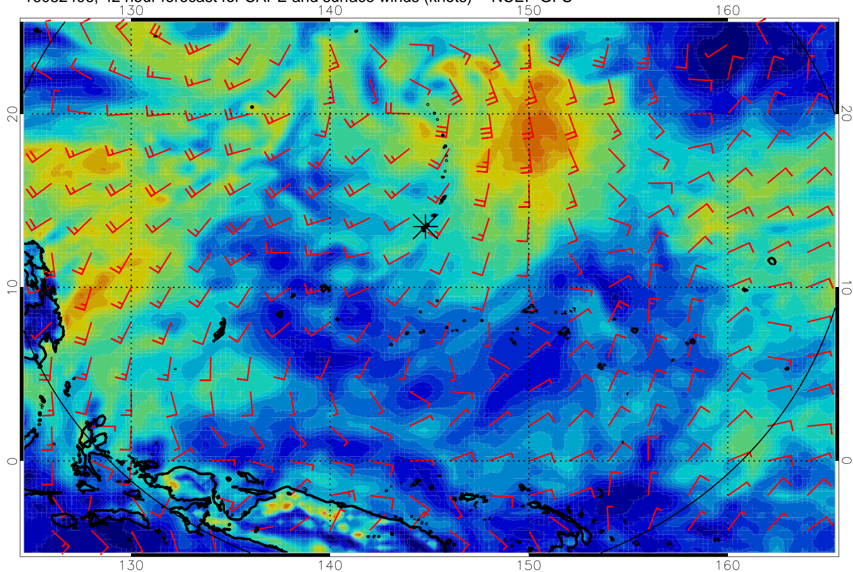
16082406, 42 hour forecast for CAPE and surface winds (knots) -- NCEP GFS
