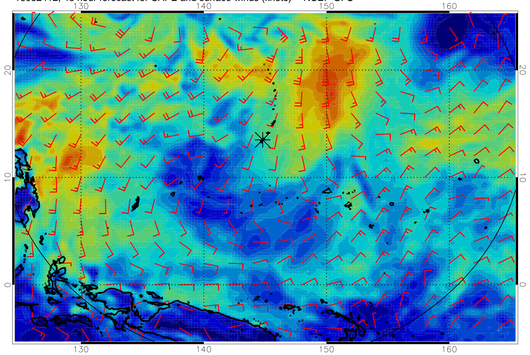
16082412, 48 hour forecast for CAPE and surface winds (knots) -- NCEP GFS
