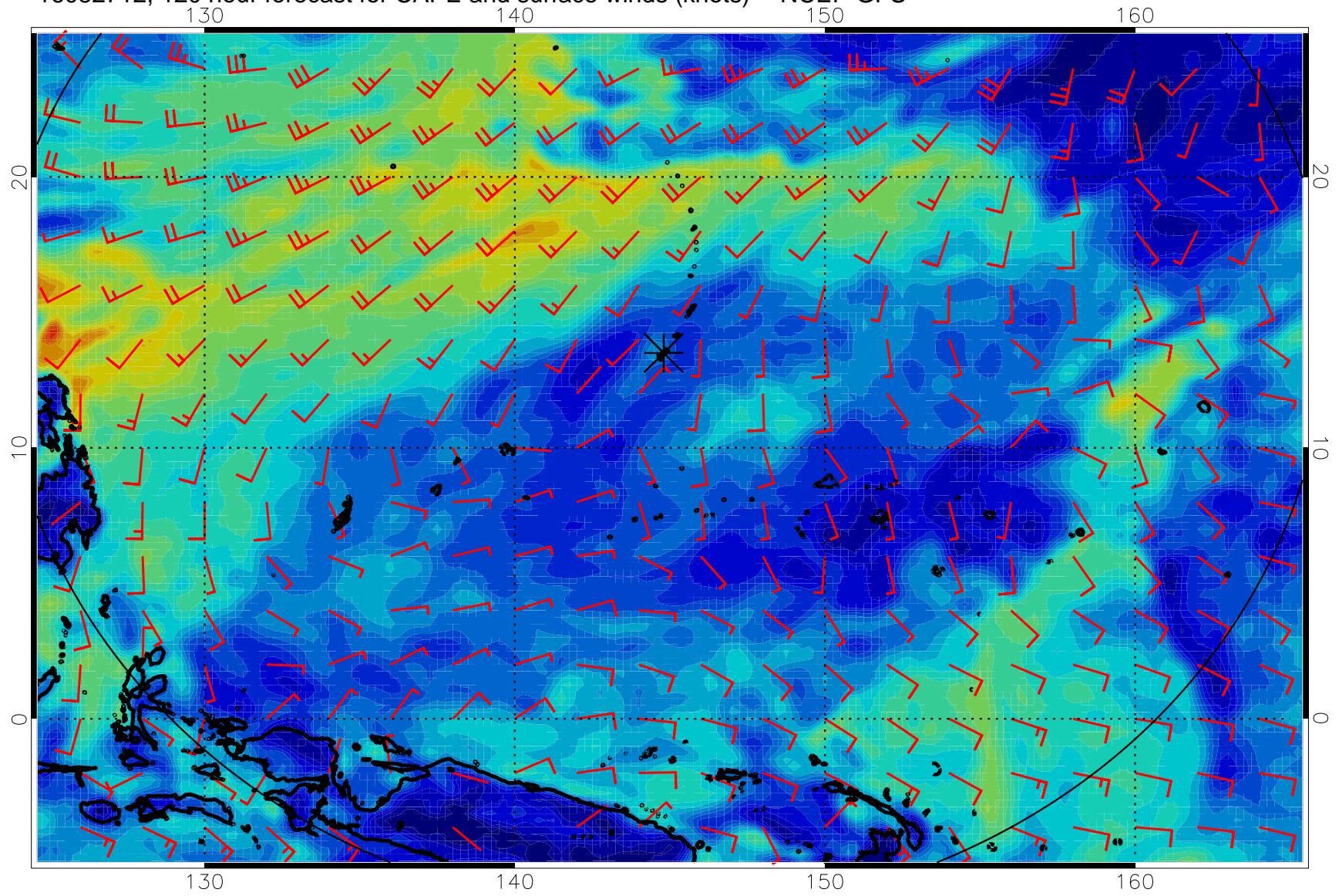
16082712, 120 hour forecast for CAPE and surface winds (knots) -- NCEP GFS
