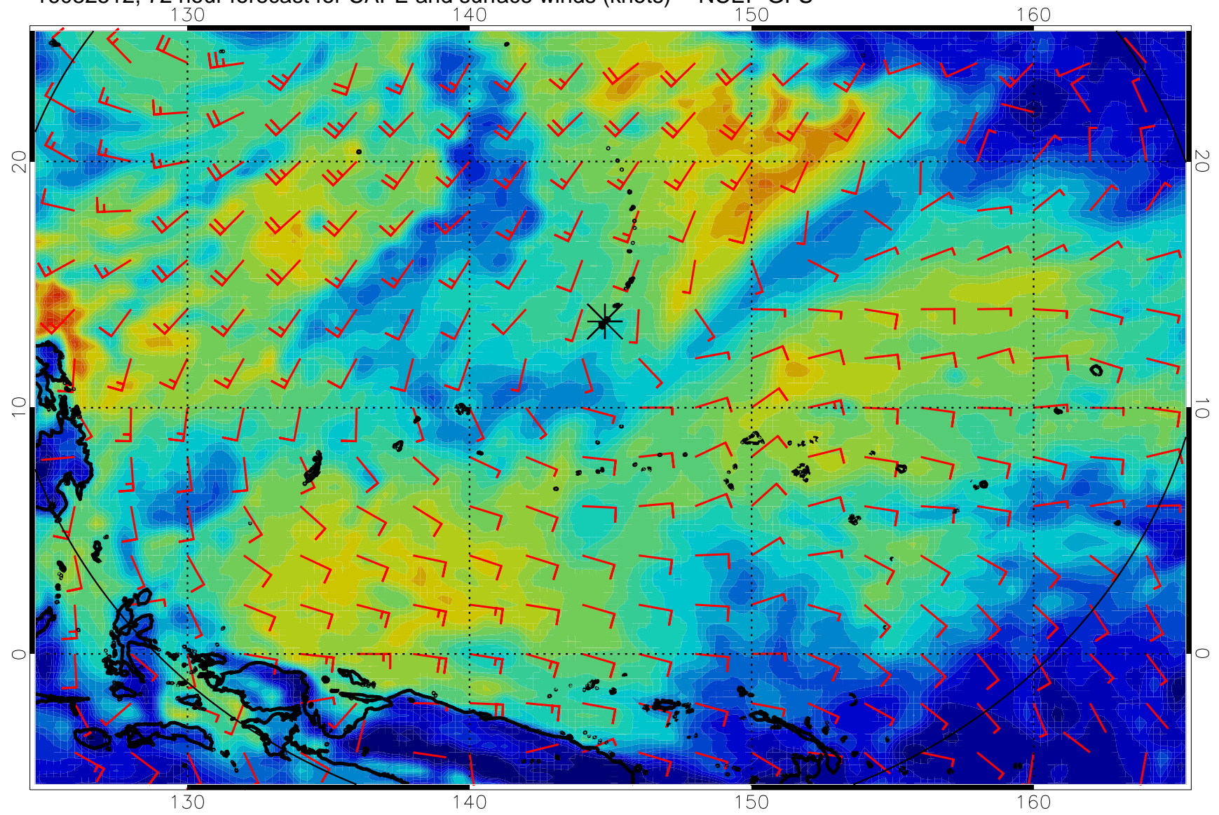
16082512, 72 hour forecast for CAPE and surface winds (knots) -- NCEP GFS
