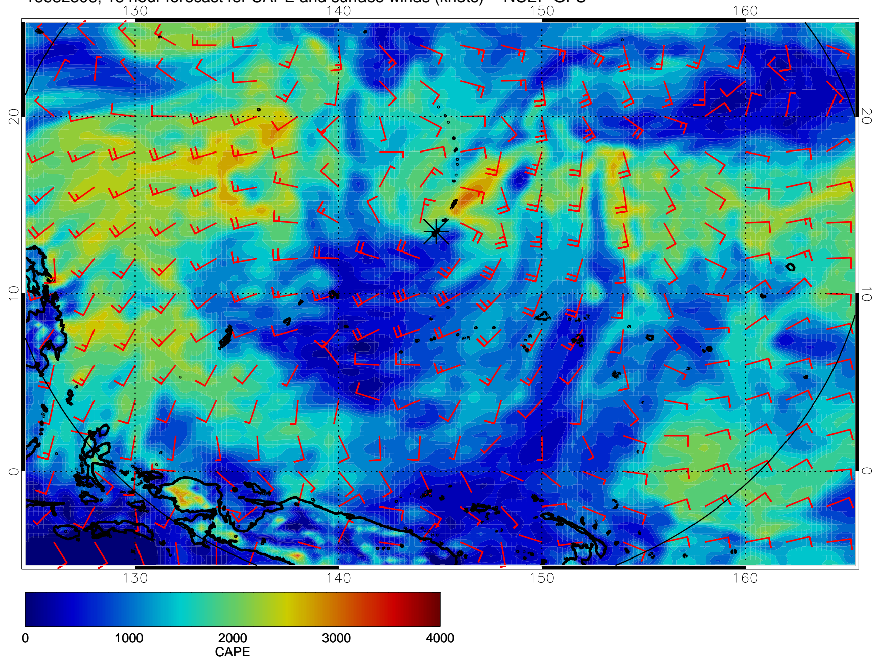
16082306, 18 hour forecast for CAPE and surface winds (knots) -- NCEP GFS
