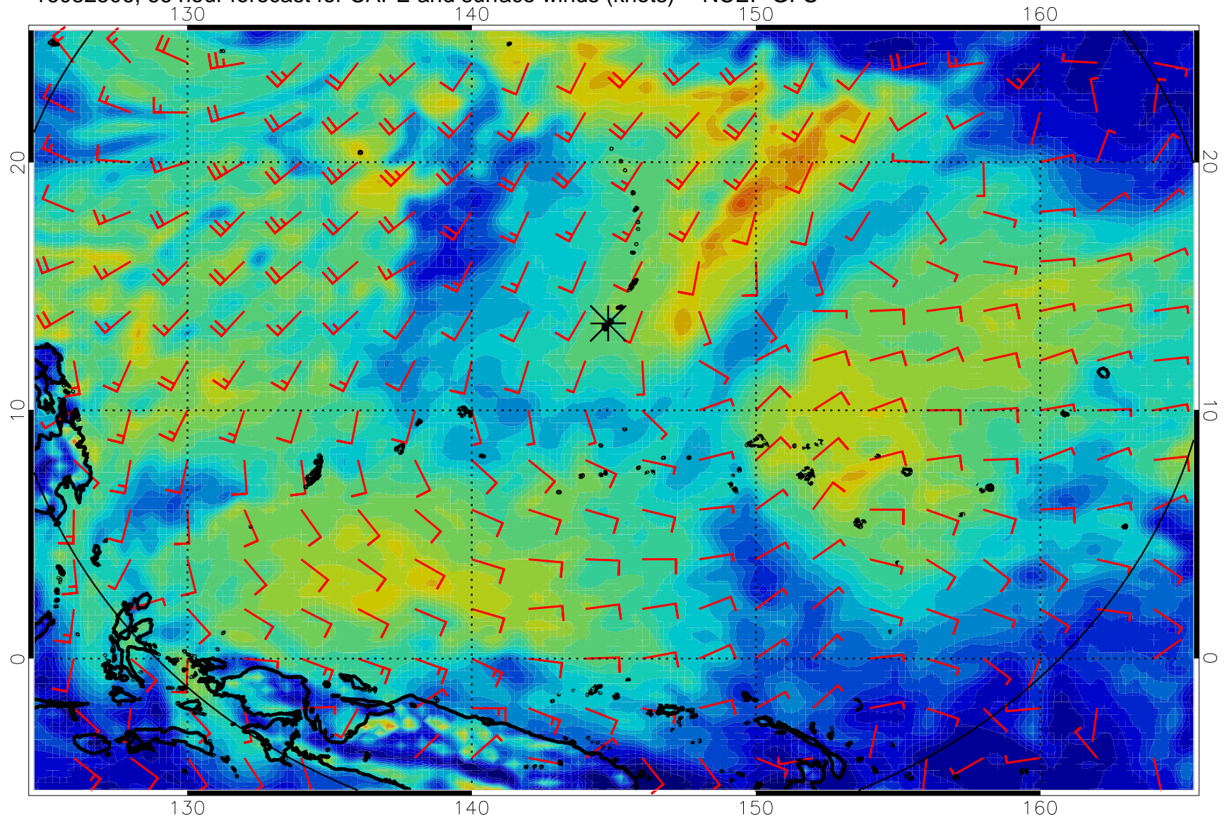
16082506, 66 hour forecast for CAPE and surface winds (knots) -- NCEP GFS
