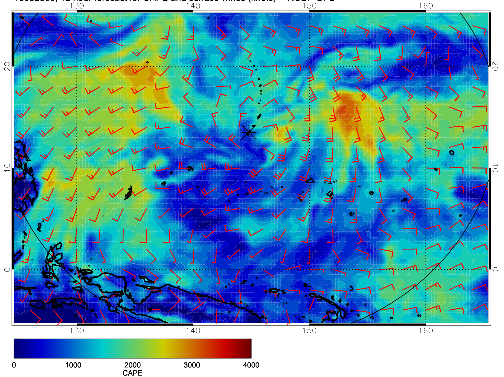
16082300, 12 hour forecast for CAPE and surface winds (knots) -- NCEP GFS
