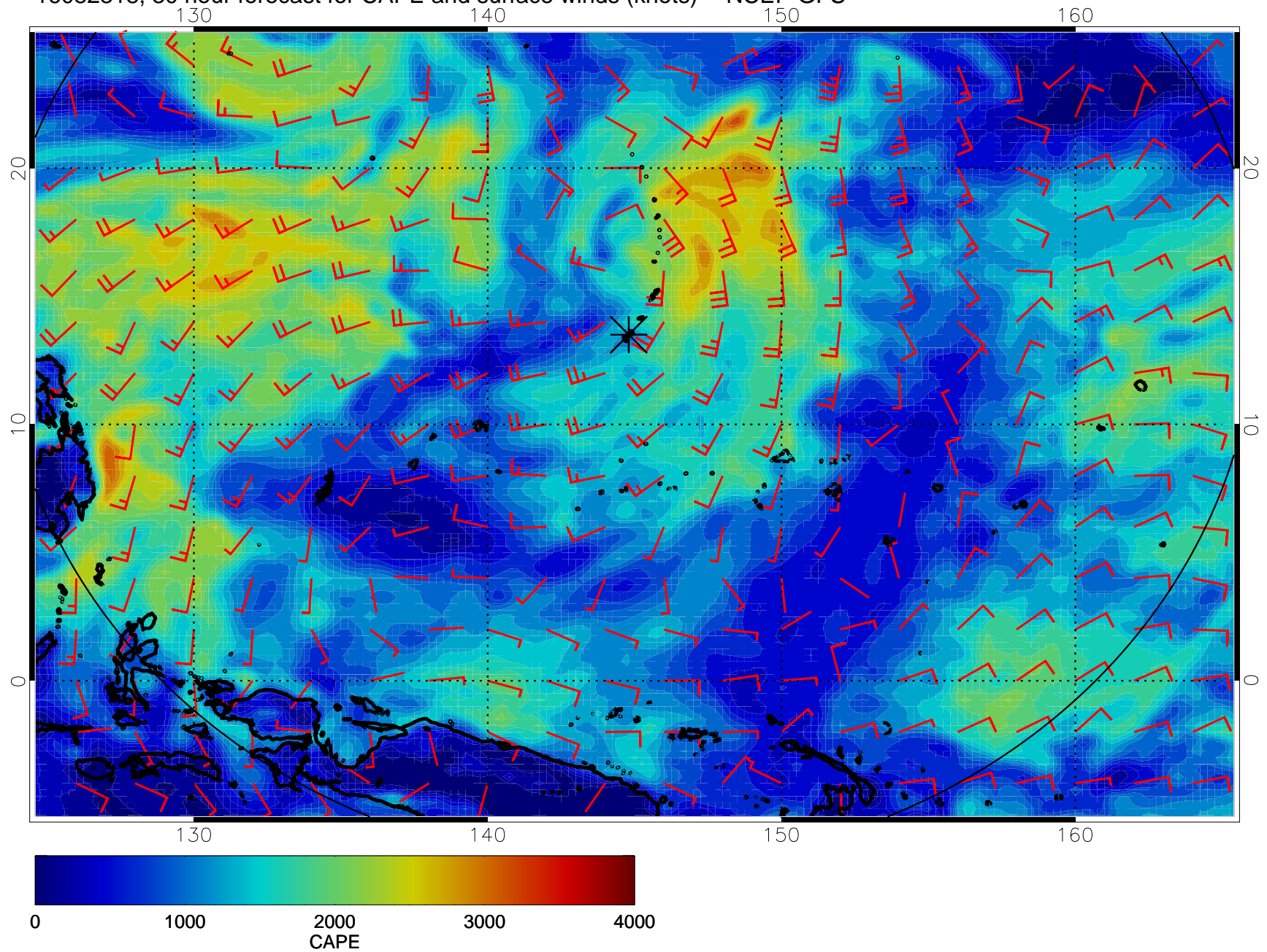
16082318, 30 hour forecast for CAPE and surface winds (knots) -- NCEP GFS
