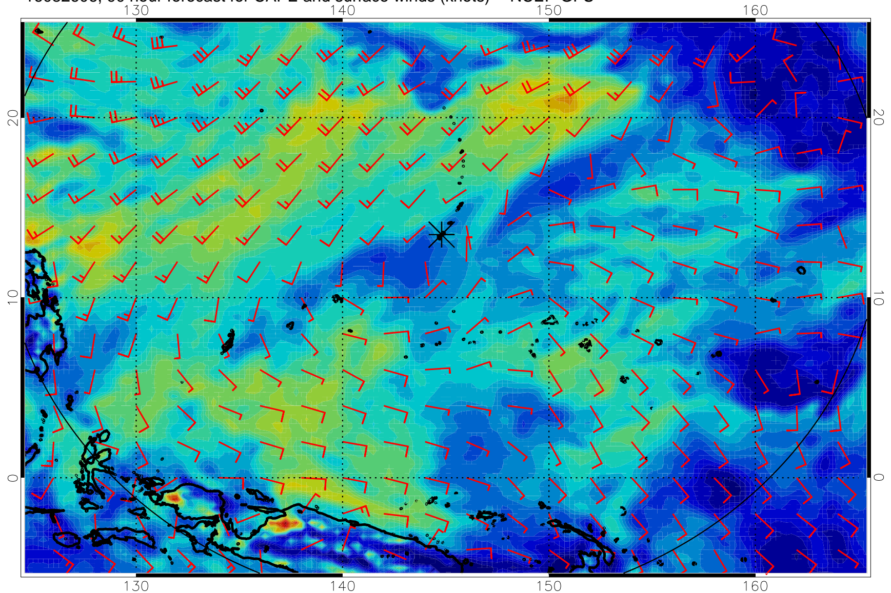
16082606, 90 hour forecast for CAPE and surface winds (knots) -- NCEP GFS
