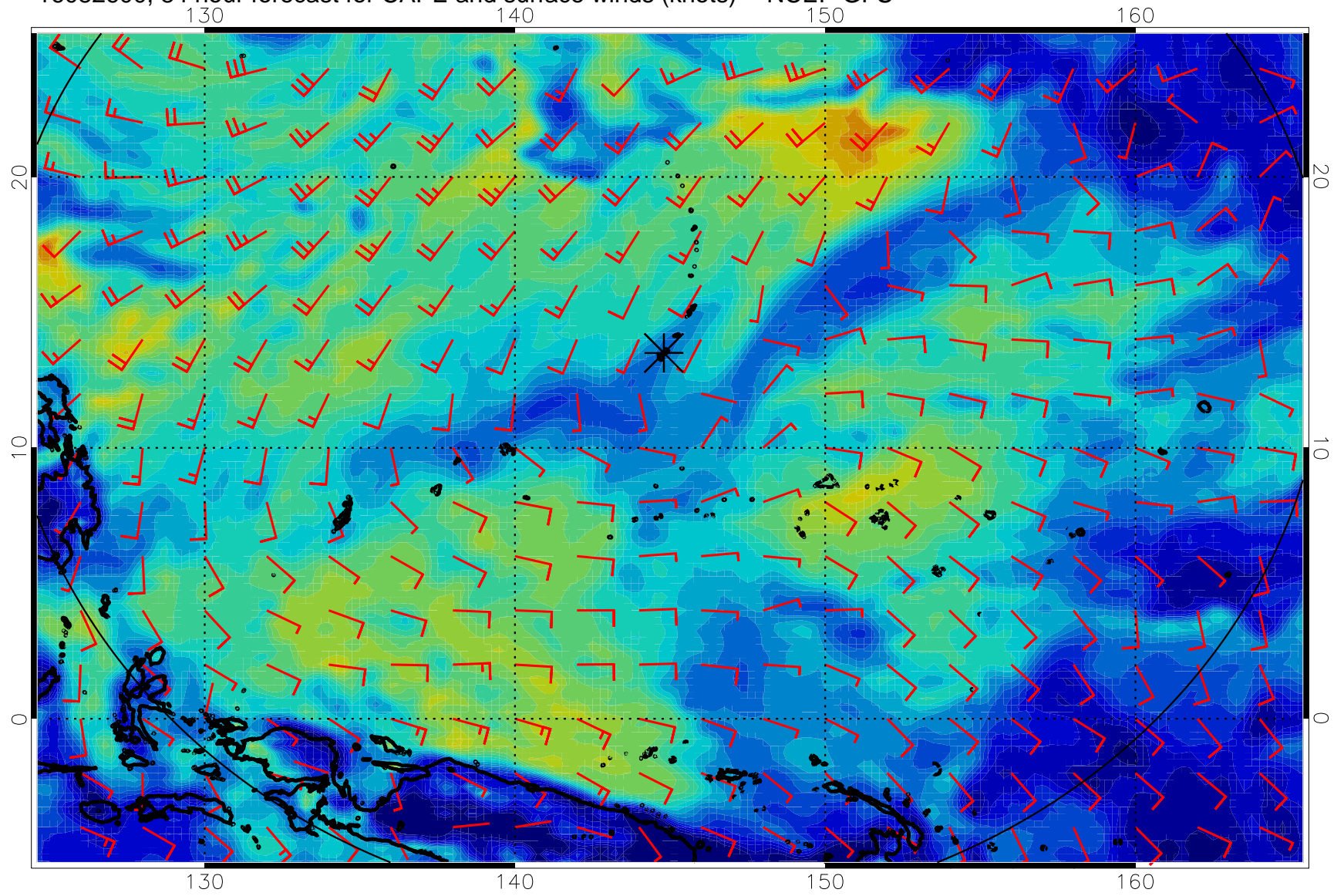
16082600, 84 hour forecast for CAPE and surface winds (knots) -- NCEP GFS
