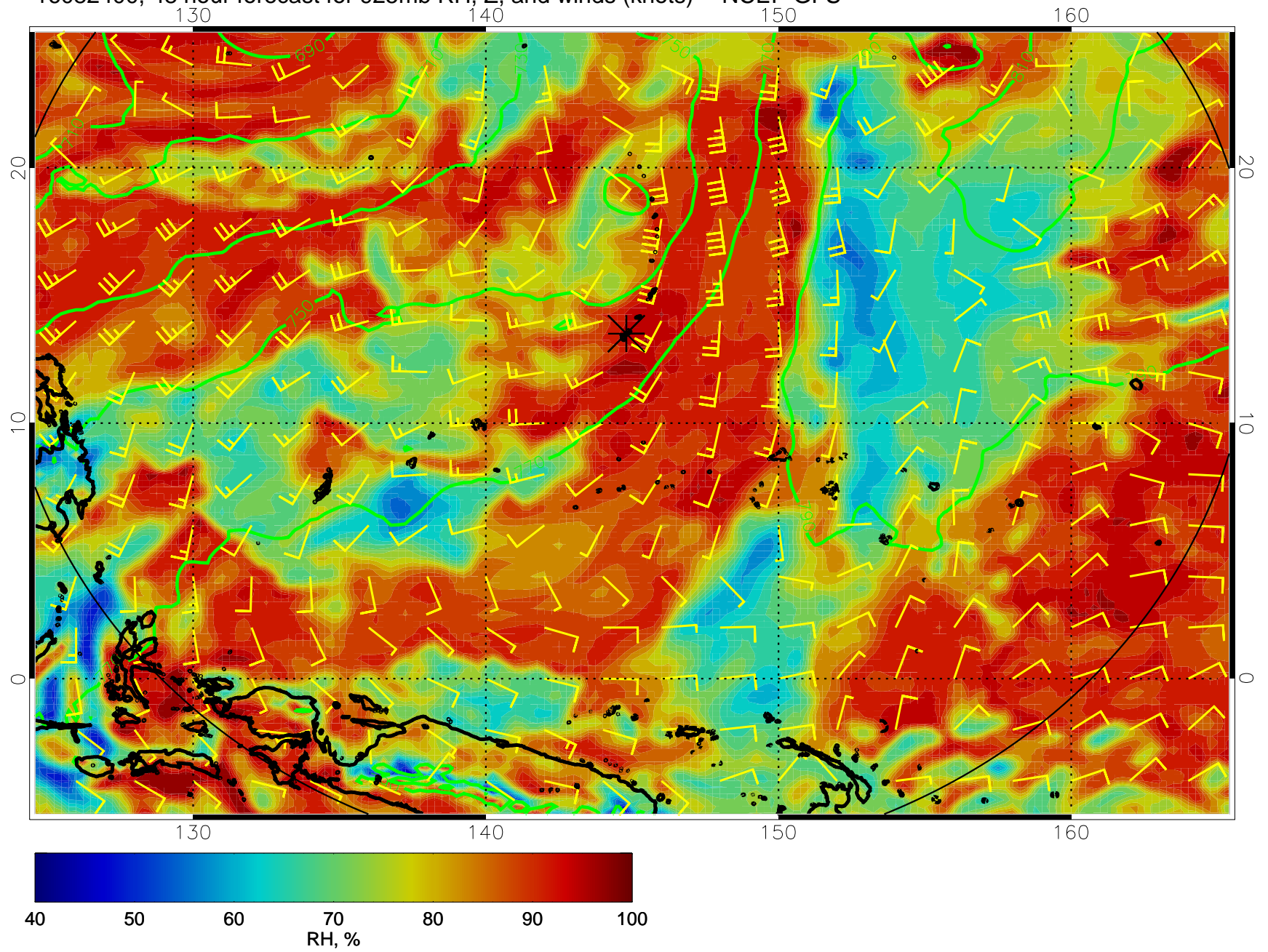
16082400, 48 hour forecast for 925mb RH, Z, and winds (knots) -- NCEP GFS
