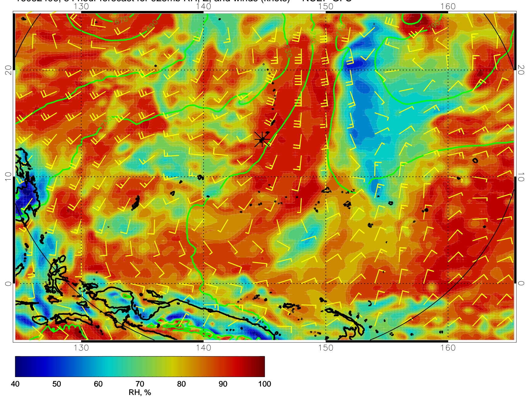
16082406, 54 hour forecast for 925mb RH, Z, and winds (knots) -- NCEP GFS
