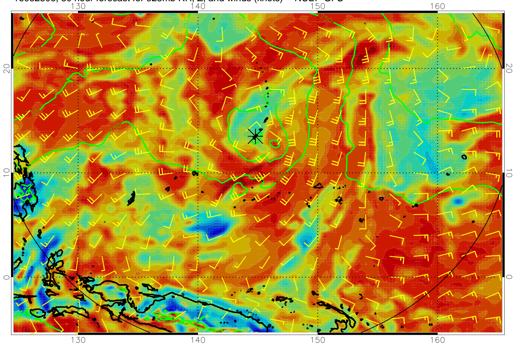
16082306, 30 hour forecast for 925mb RH, Z, and winds (knots) -- NCEP GFS
