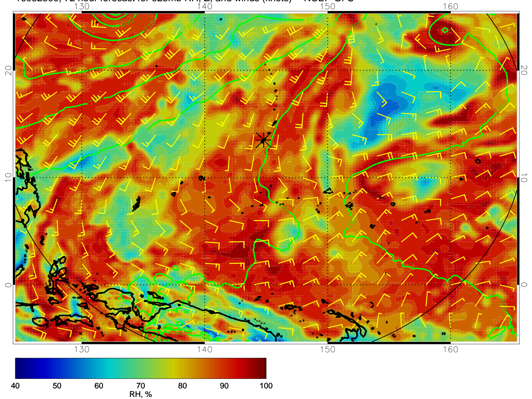
16082500, 72 hour forecast for 925mb RH, Z, and winds (knots) -- NCEP GFS
