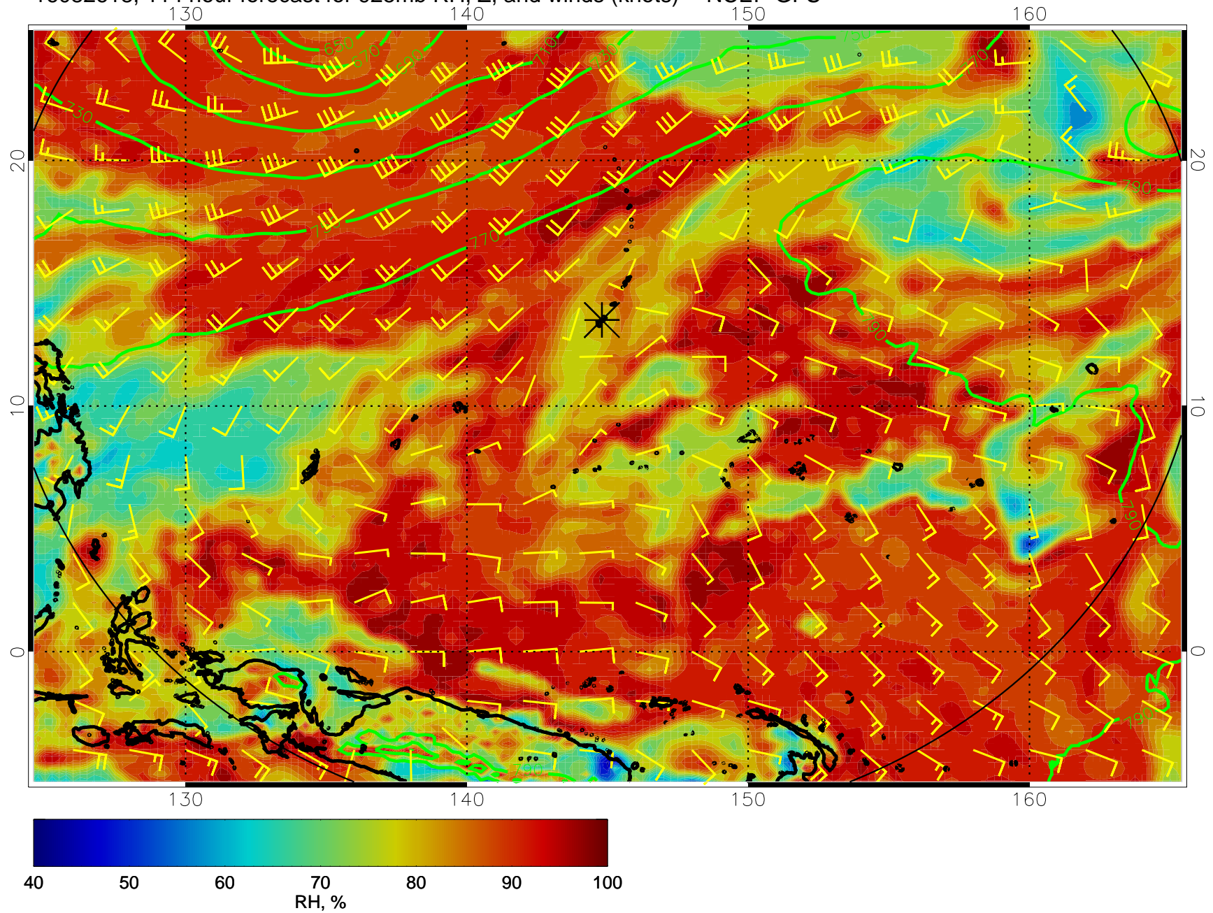
16082618, 114 hour forecast for 925mb RH, Z, and winds (knots) -- NCEP GFS
