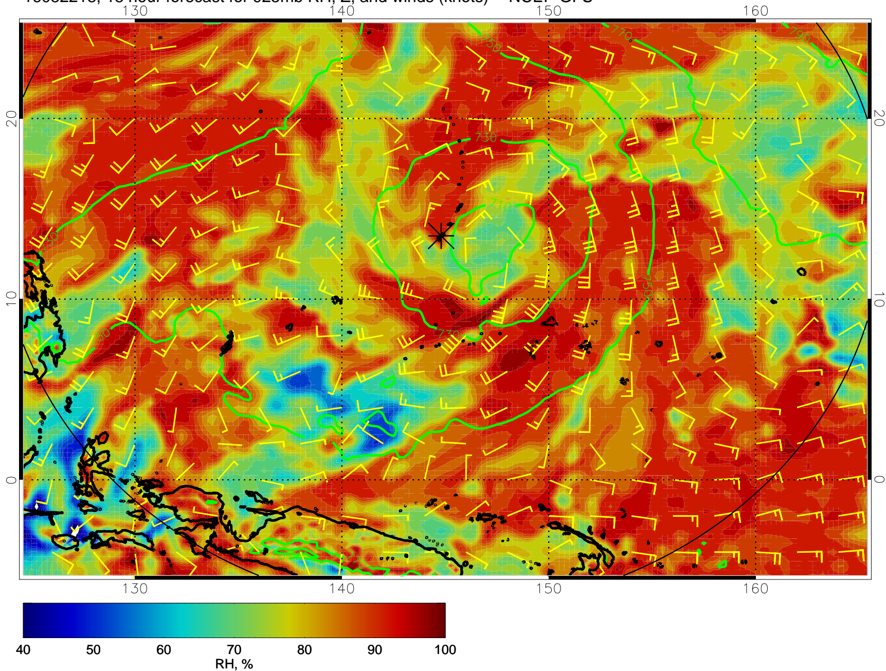
16082218, 18 hour forecast for 925mb RH, Z, and winds (knots) -- NCEP GFS
