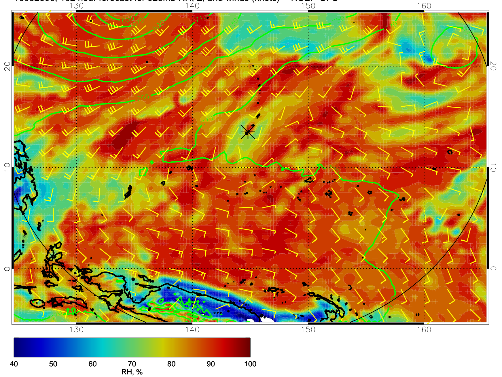
16082606, 102 hour forecast for 925mb RH, Z, and winds (knots) -- NCEP GFS
