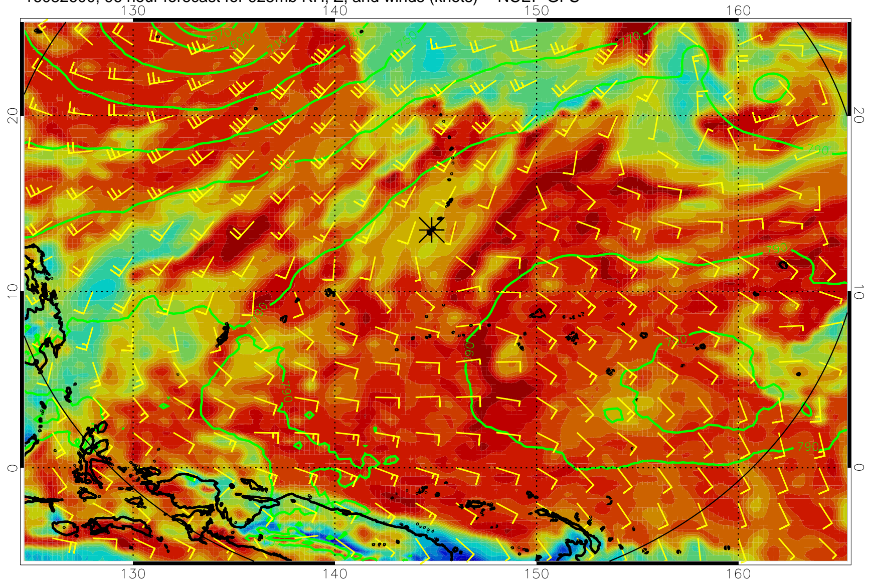
16082600, 96 hour forecast for 925mb RH, Z, and winds (knots) -- NCEP GFS
