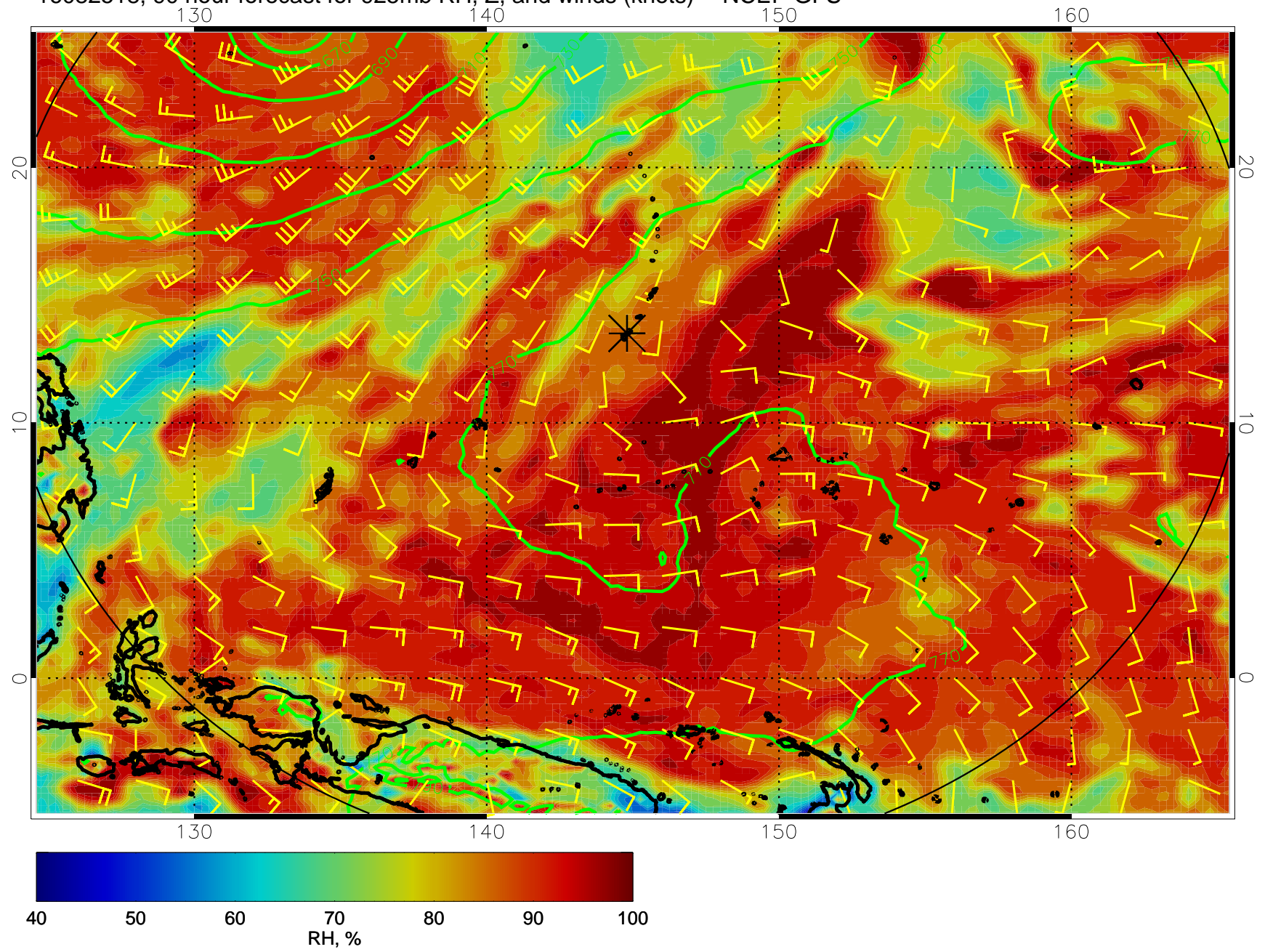
16082518, 90 hour forecast for 925mb RH, Z, and winds (knots) -- NCEP GFS
