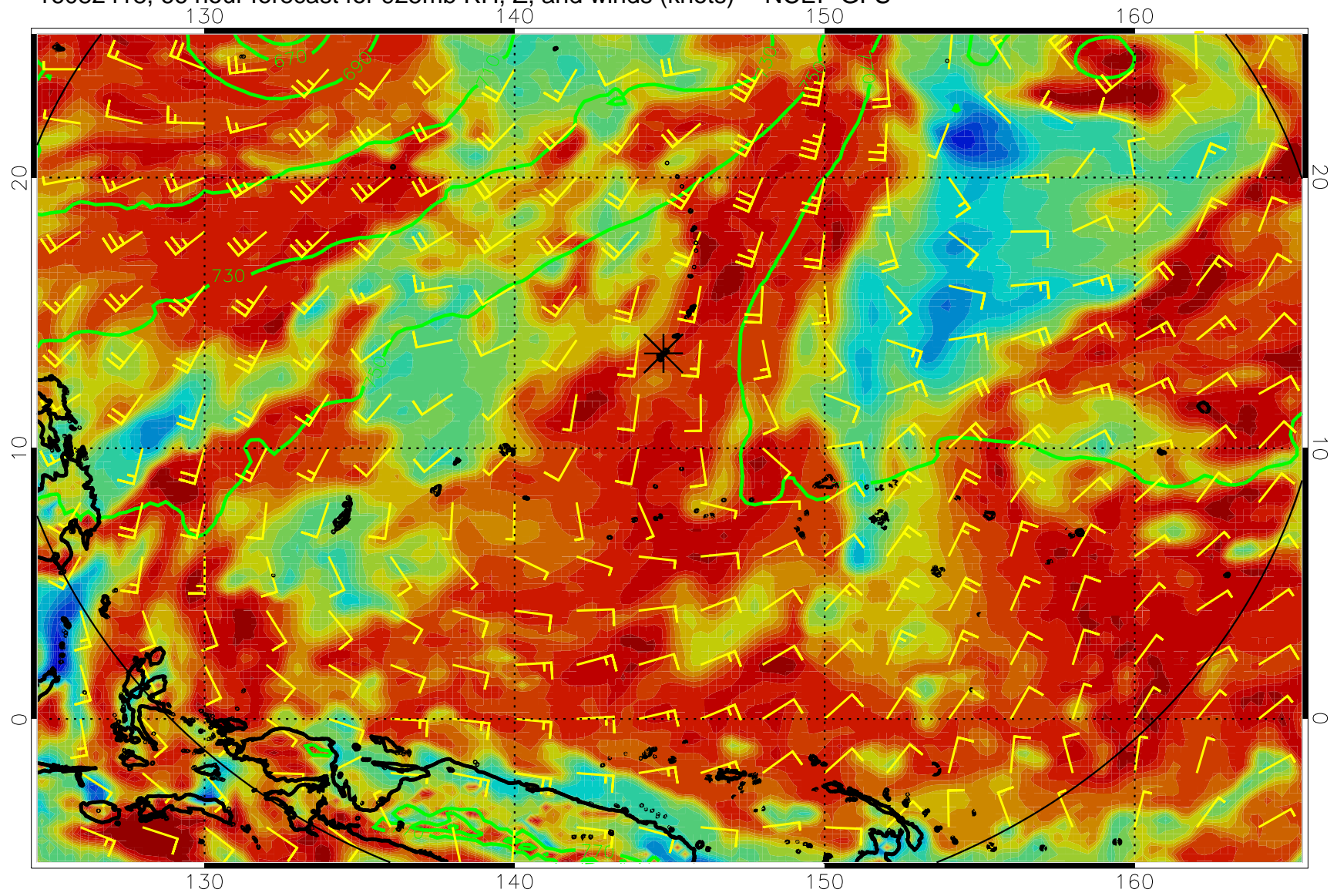
16082418, 66 hour forecast for 925mb RH, Z, and winds (knots) -- NCEP GFS
