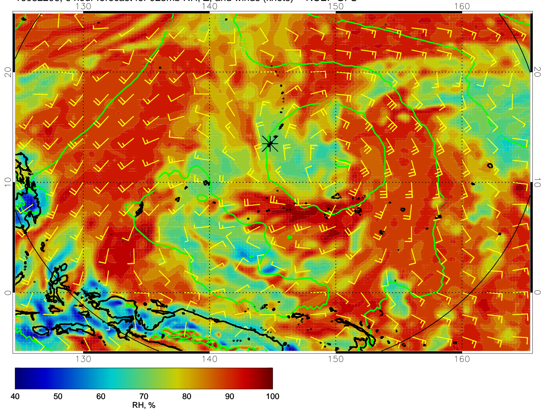
16082206, 6 hour forecast for 925mb RH, Z, and winds (knots) -- NCEP GFS
