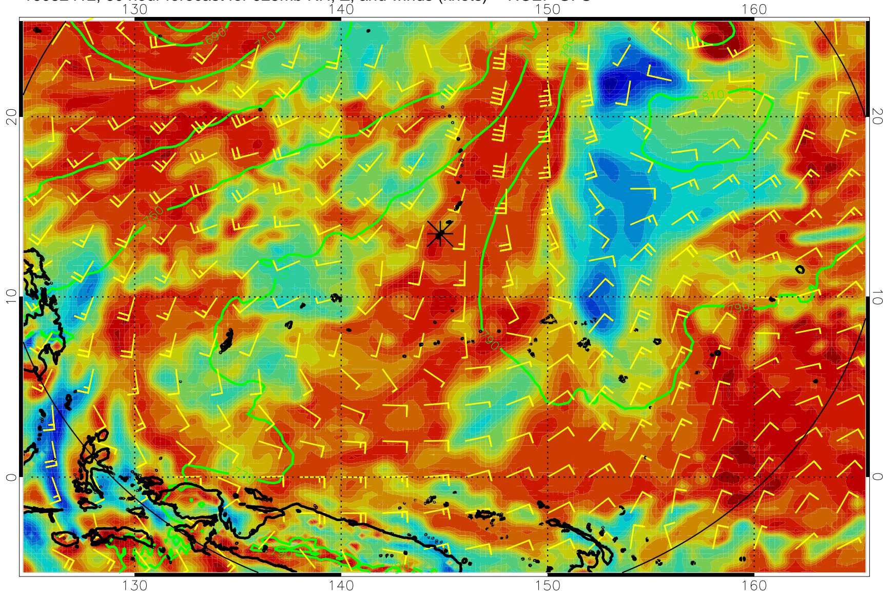
16082412, 60 hour forecast for 925mb RH, Z, and winds (knots) -- NCEP GFS
