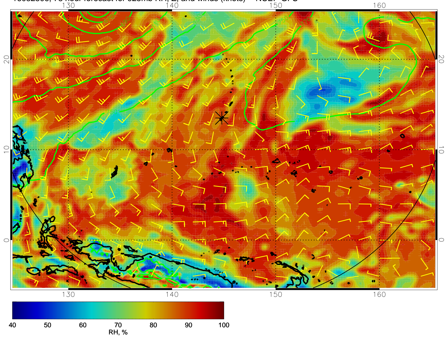
16082506, 78 hour forecast for 925mb RH, Z, and winds (knots) -- NCEP GFS
