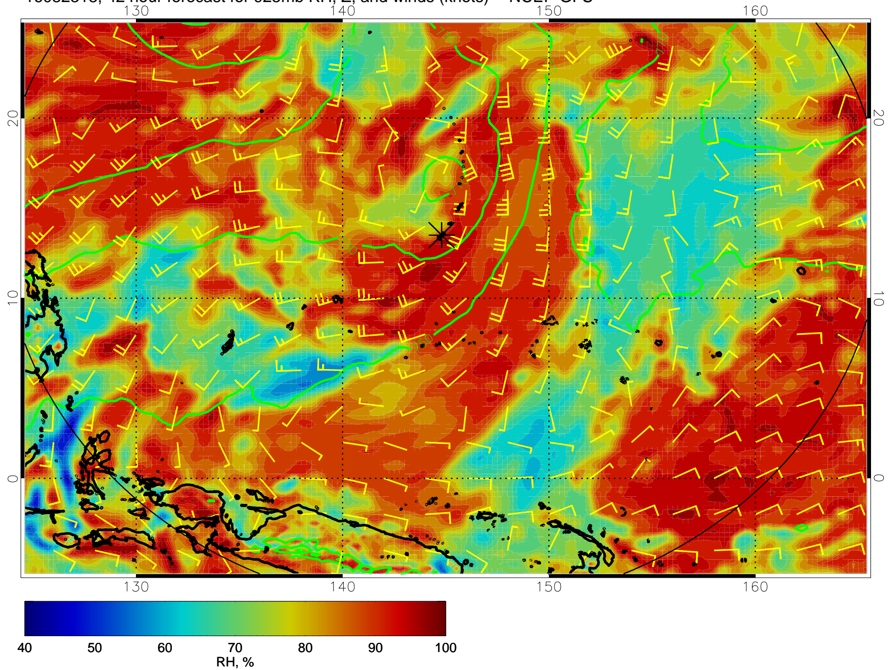
16082318, 42 hour forecast for 925mb RH, Z, and winds (knots) -- NCEP GFS
