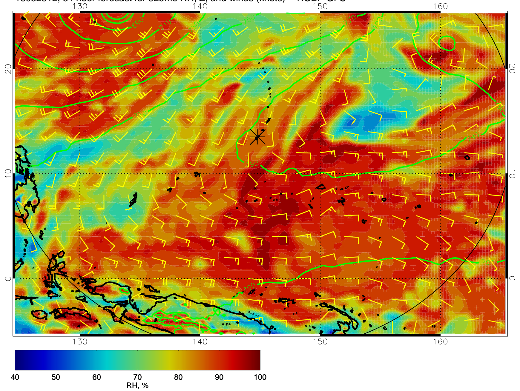
16082512, 84 hour forecast for 925mb RH, Z, and winds (knots) -- NCEP GFS
