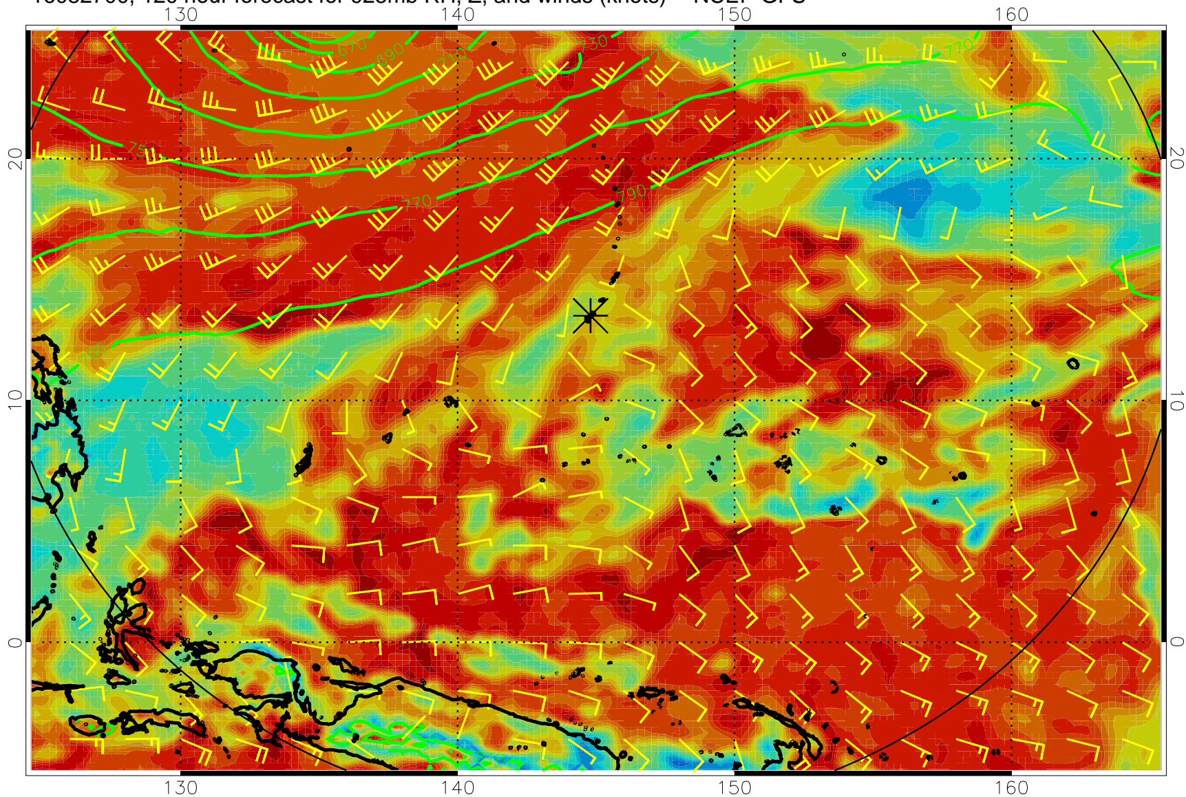
16082700, 120 hour forecast for 925mb RH, Z, and winds (knots) -- NCEP GFS
