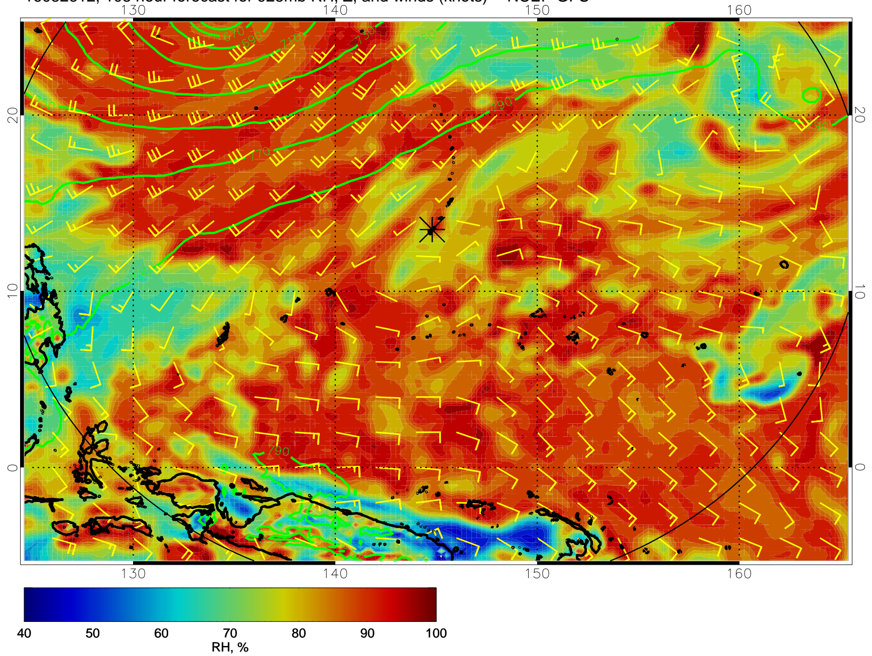
16082612, 108 hour forecast for 925mb RH, Z, and winds (knots) -- NCEP GFS
