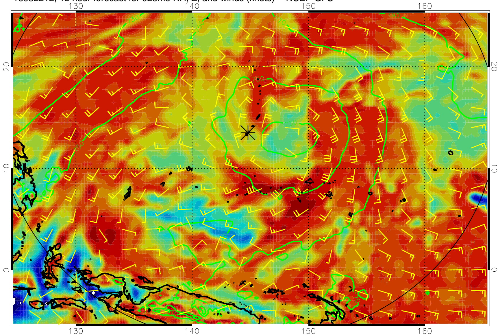
16082212, 12 hour forecast for 925mb RH, Z, and winds (knots) -- NCEP GFS
