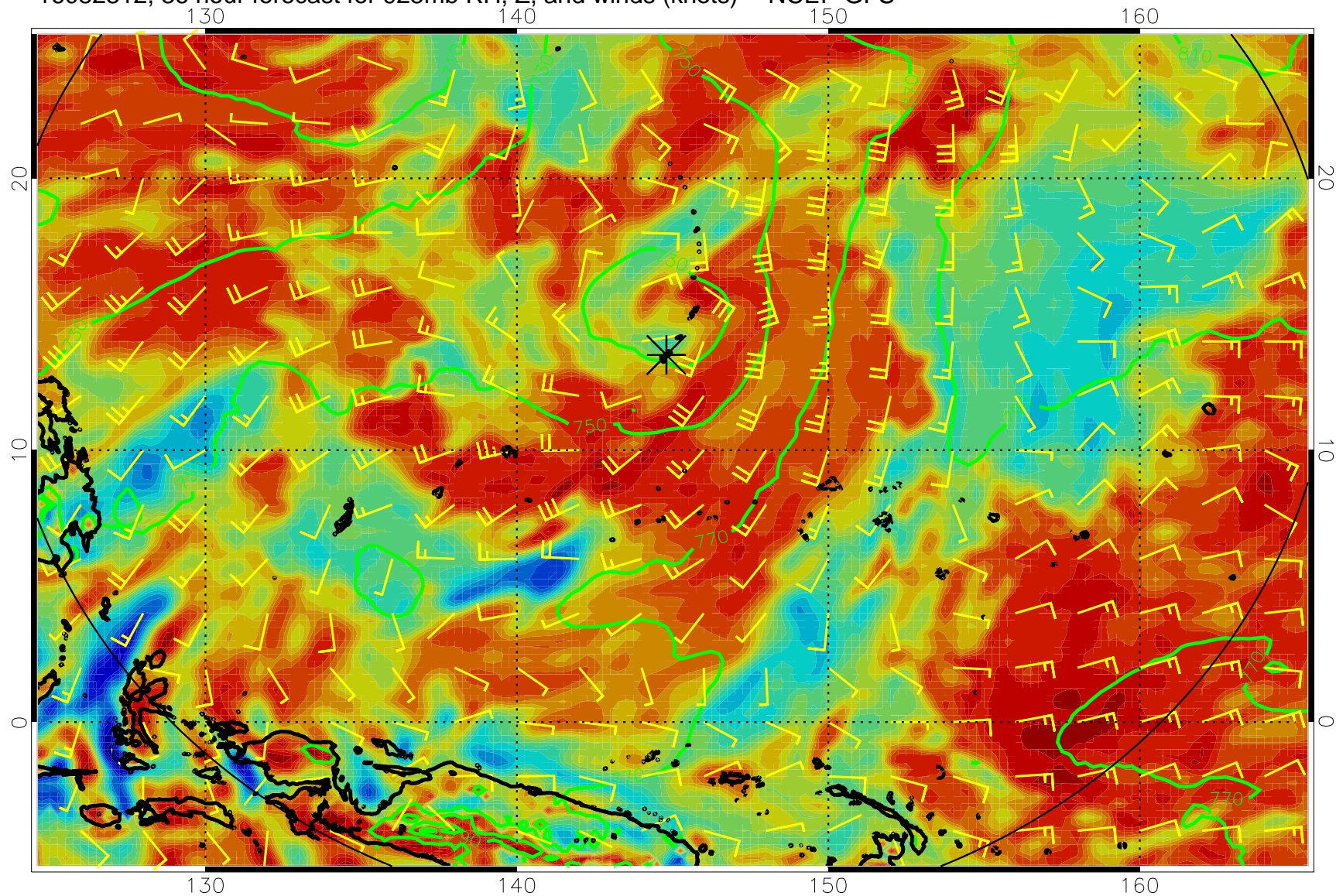
16082312, 36 hour forecast for 925mb RH, Z, and winds (knots) -- NCEP GFS
