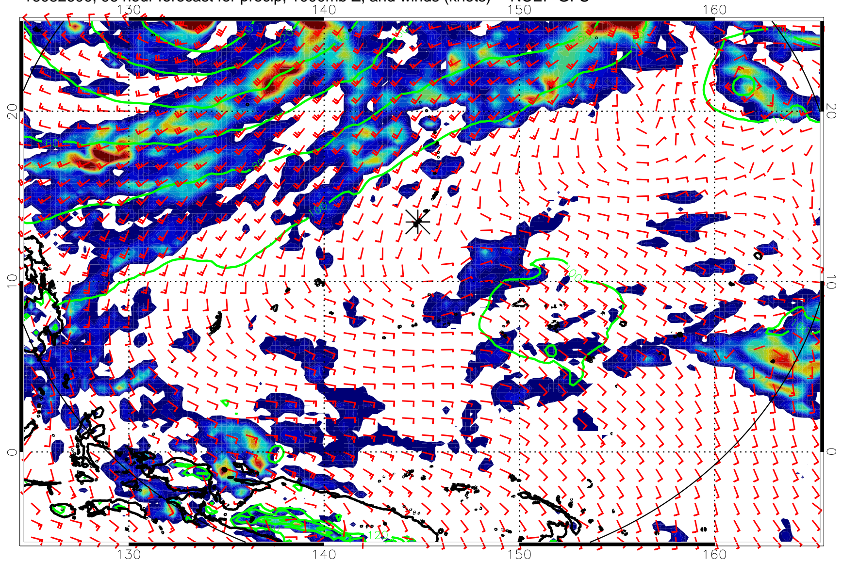
16082600, 96 hour forecast for precip, 1000mb Z, and winds (knots) -- NCEP GFS
