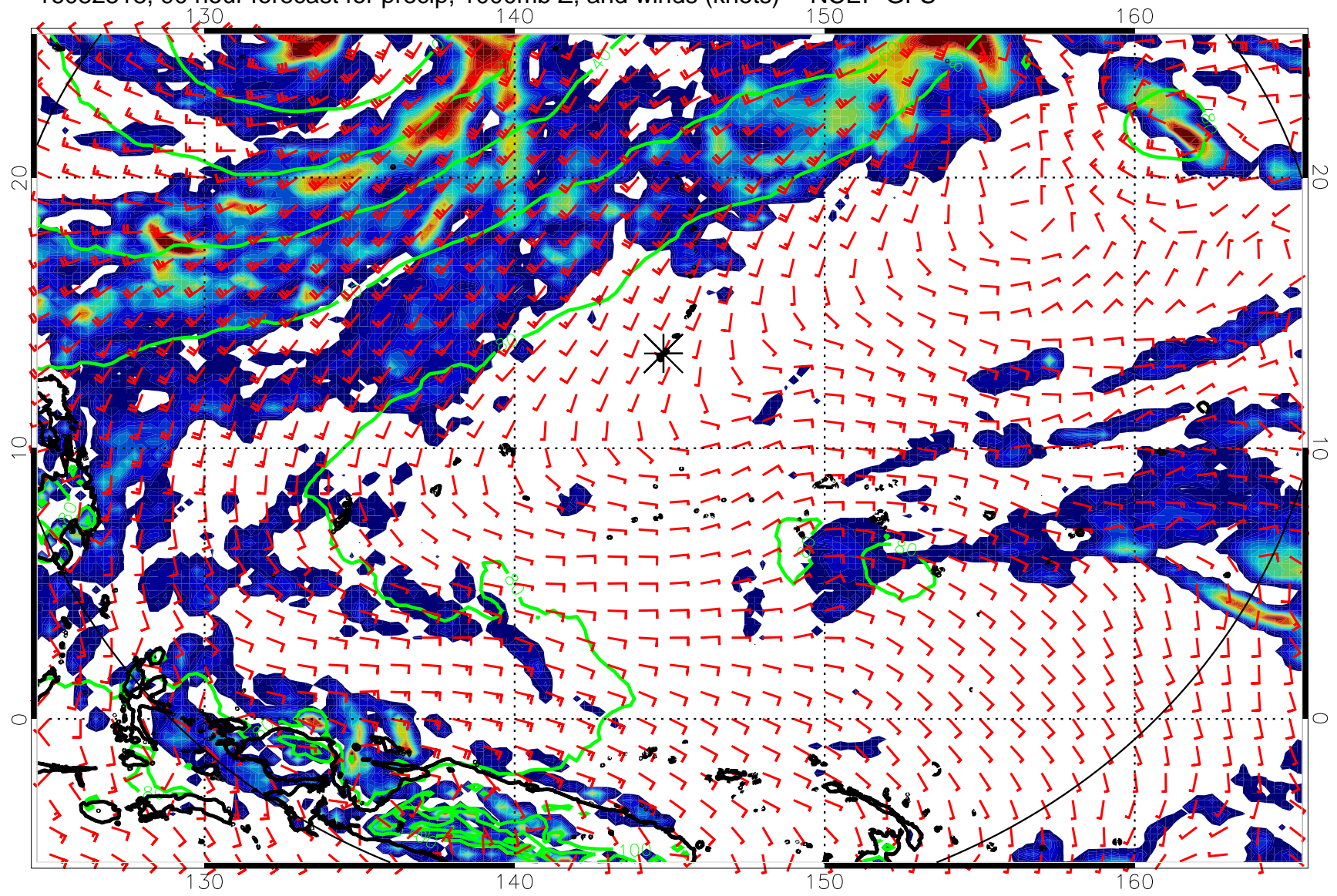
16082518, 90 hour forecast for precip, 1000mb Z, and winds (knots) -- NCEP GFS
