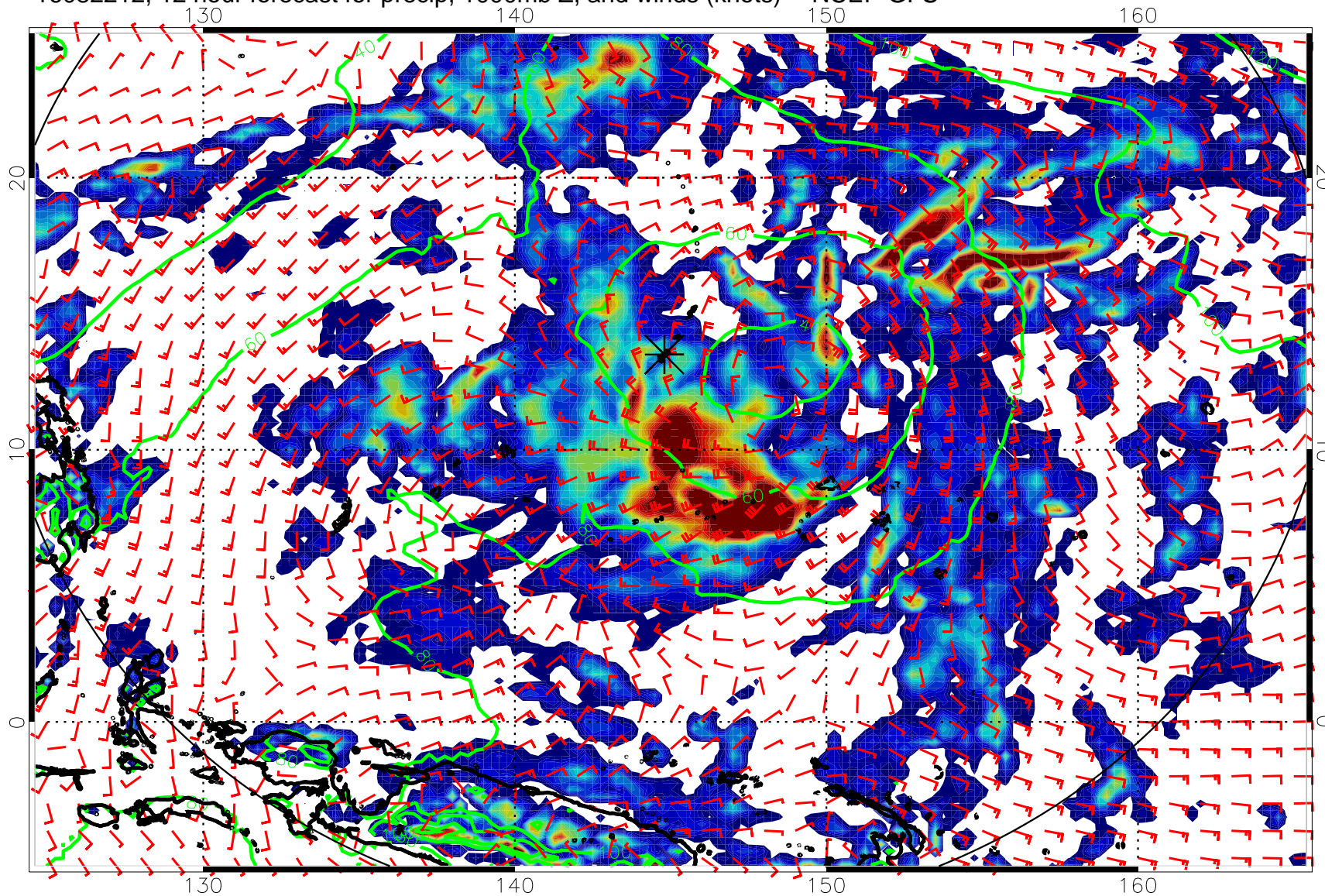
16082212, 12 hour forecast for precip, 1000mb Z, and winds (knots) -- NCEP GFS
