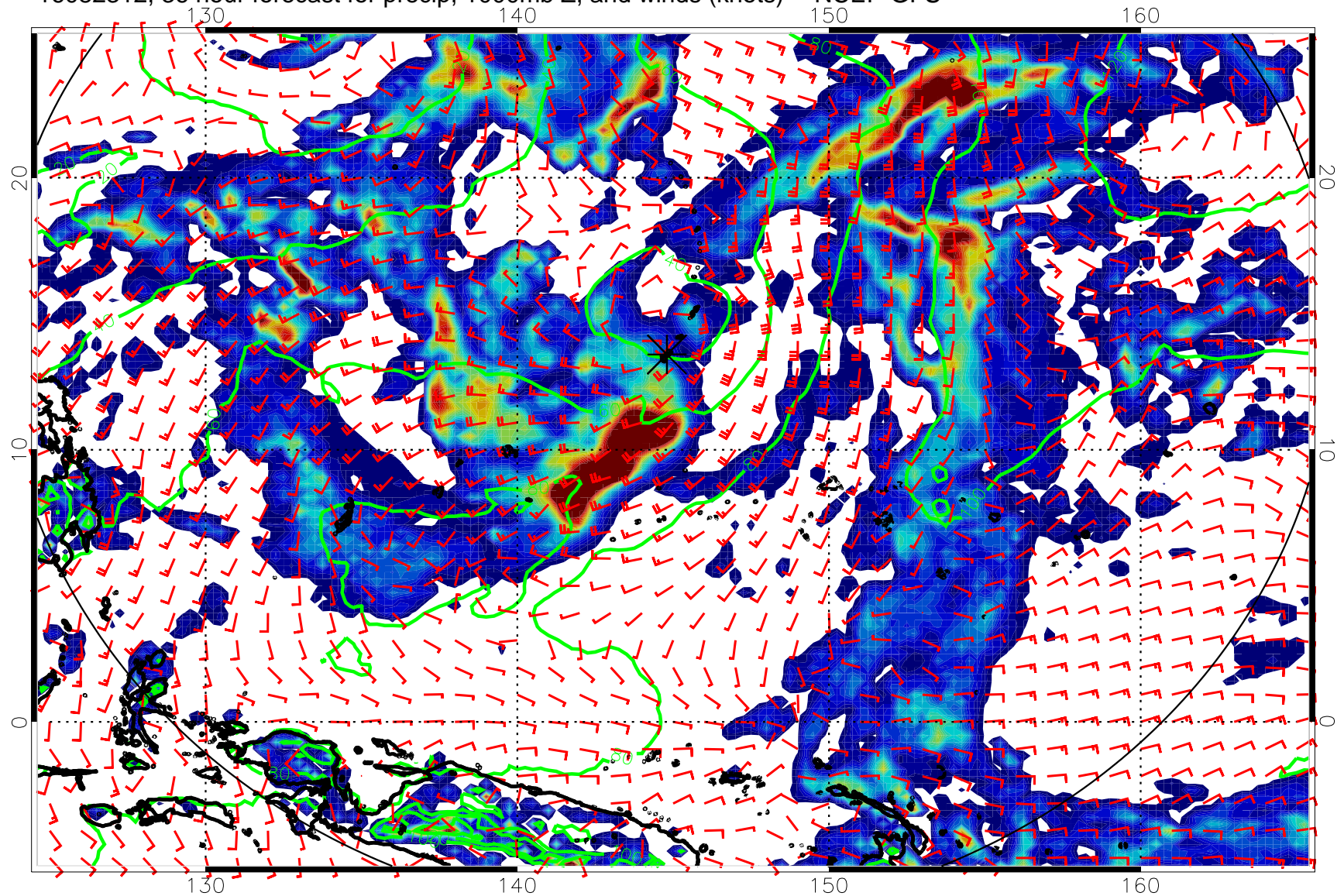
16082312, 36 hour forecast for precip, 1000mb Z, and winds (knots) -- NCEP GFS
