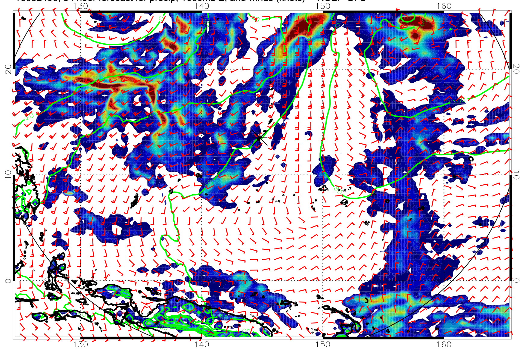
16082406, 54 hour forecast for precip, 1000mb Z, and winds (knots) -- NCEP GFS
