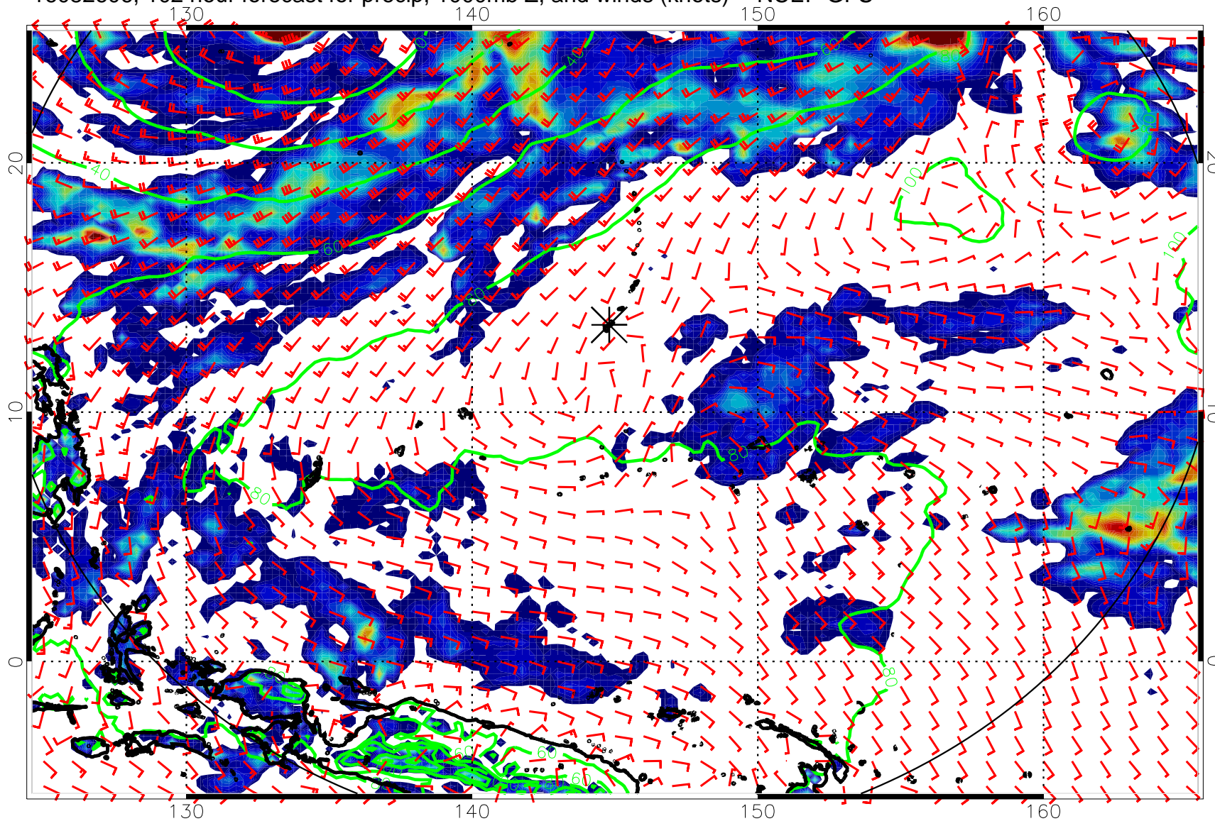
16082606, 102 hour forecast for precip, 1000mb Z, and winds (knots) -- NCEP GFS
