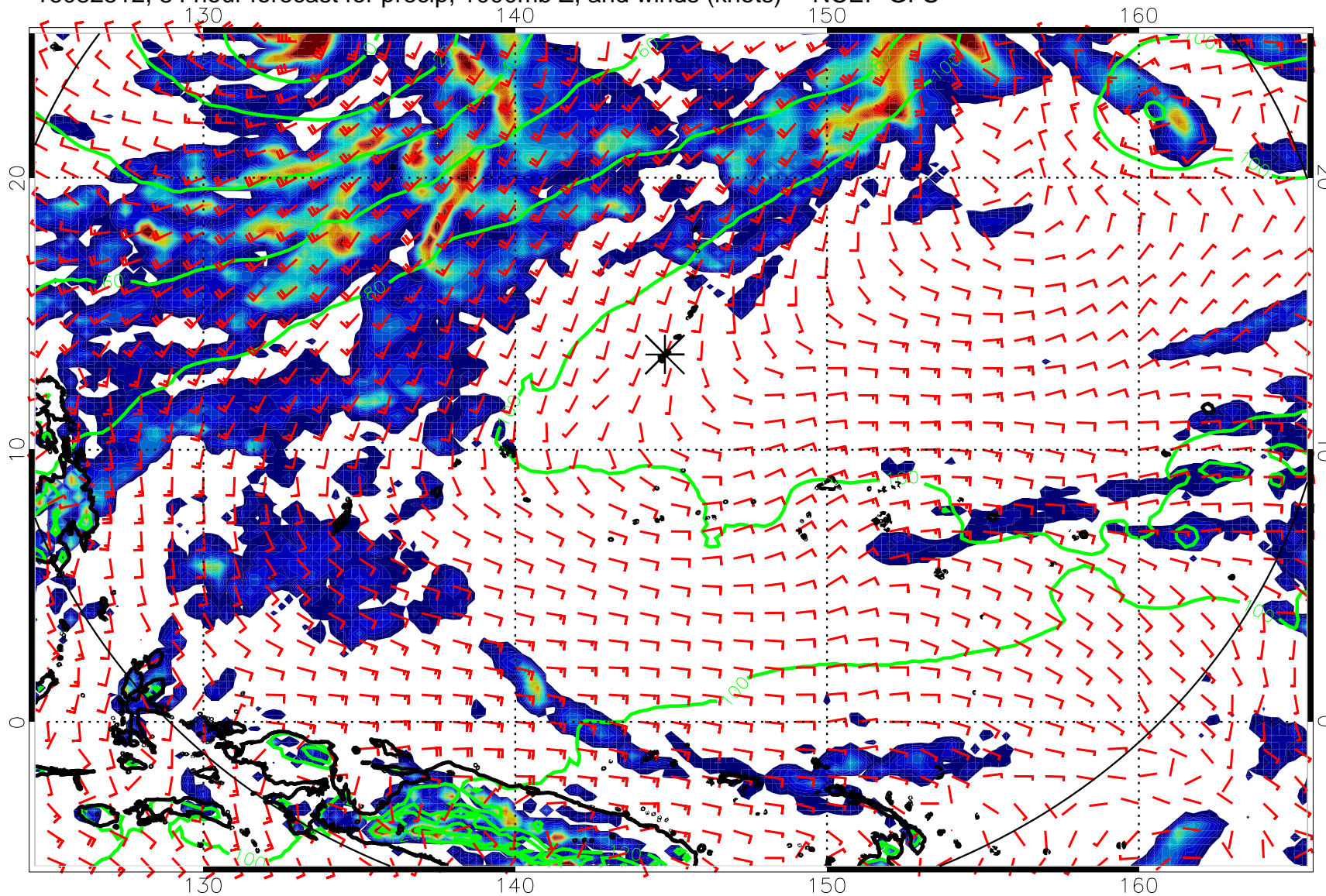
16082512, 84 hour forecast for precip, 1000mb Z, and winds (knots) -- NCEP GFS
