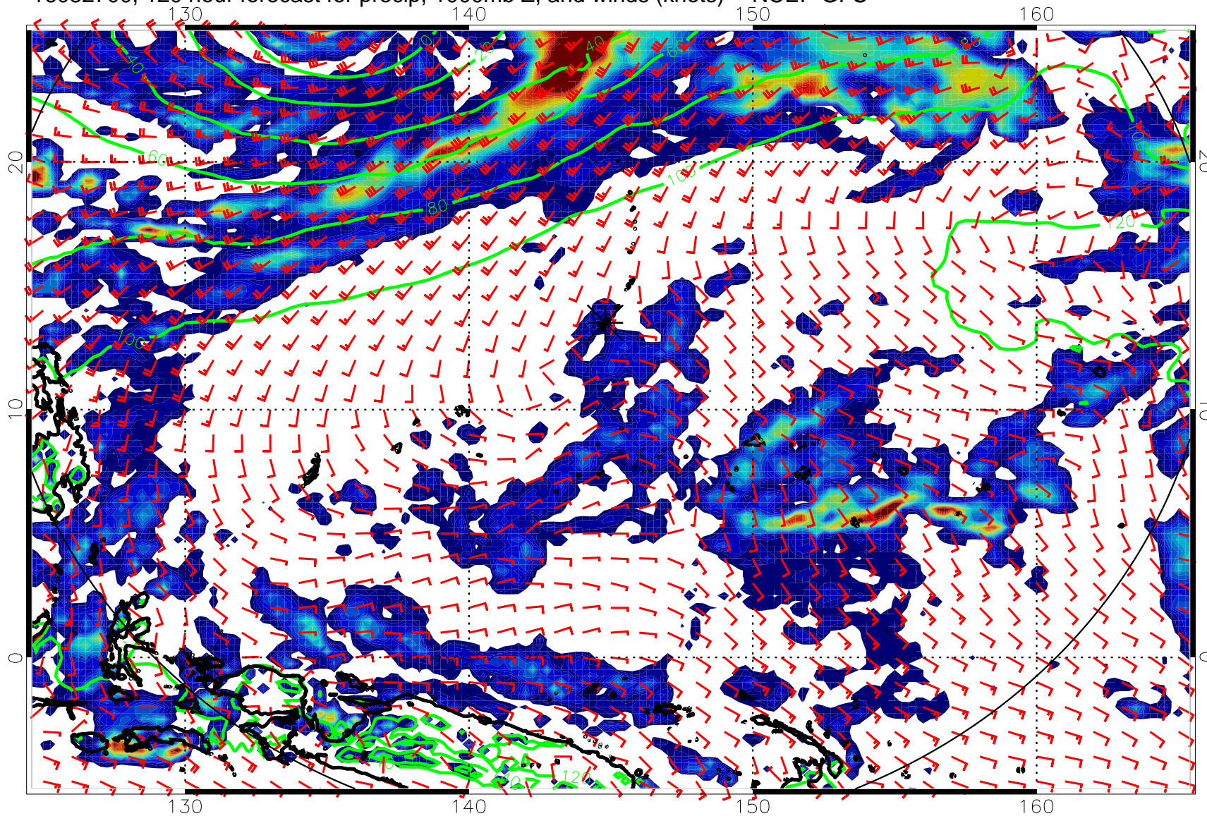
16082700, 120 hour forecast for precip, 1000mb Z, and winds (knots) -- NCEP GFS
