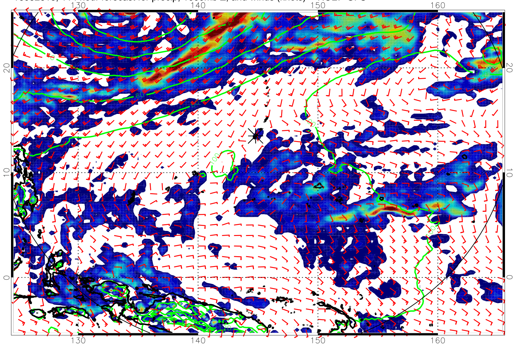
16082618, 114 hour forecast for precip, 1000mb Z, and winds (knots) -- NCEP GFS
