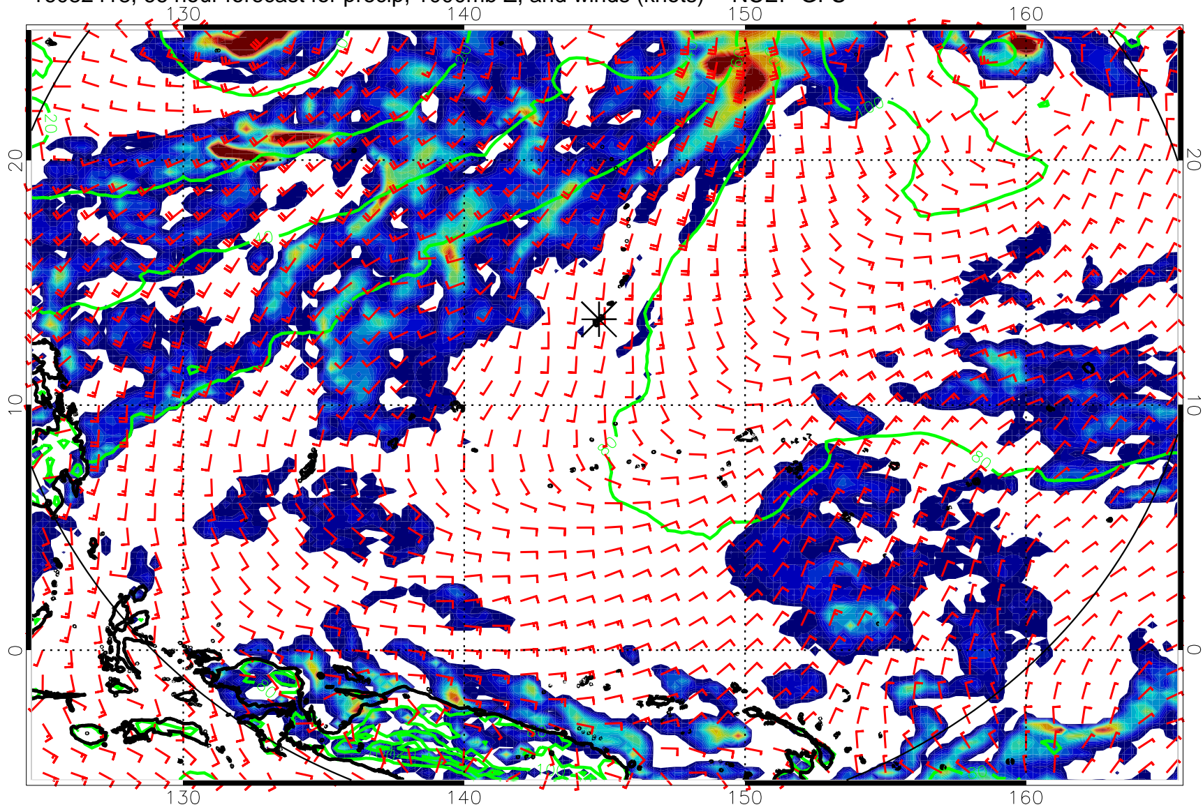
16082418, 66 hour forecast for precip, 1000mb Z, and winds (knots) -- NCEP GFS
