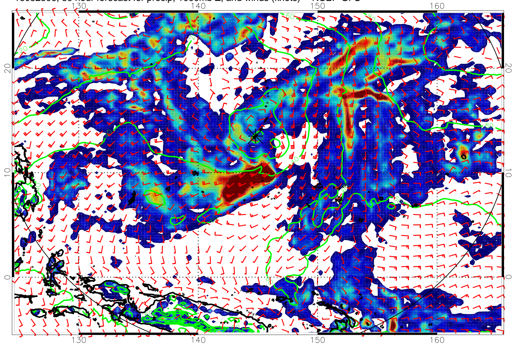
16082306, 30 hour forecast for precip, 1000mb Z, and winds (knots) -- NCEP GFS
