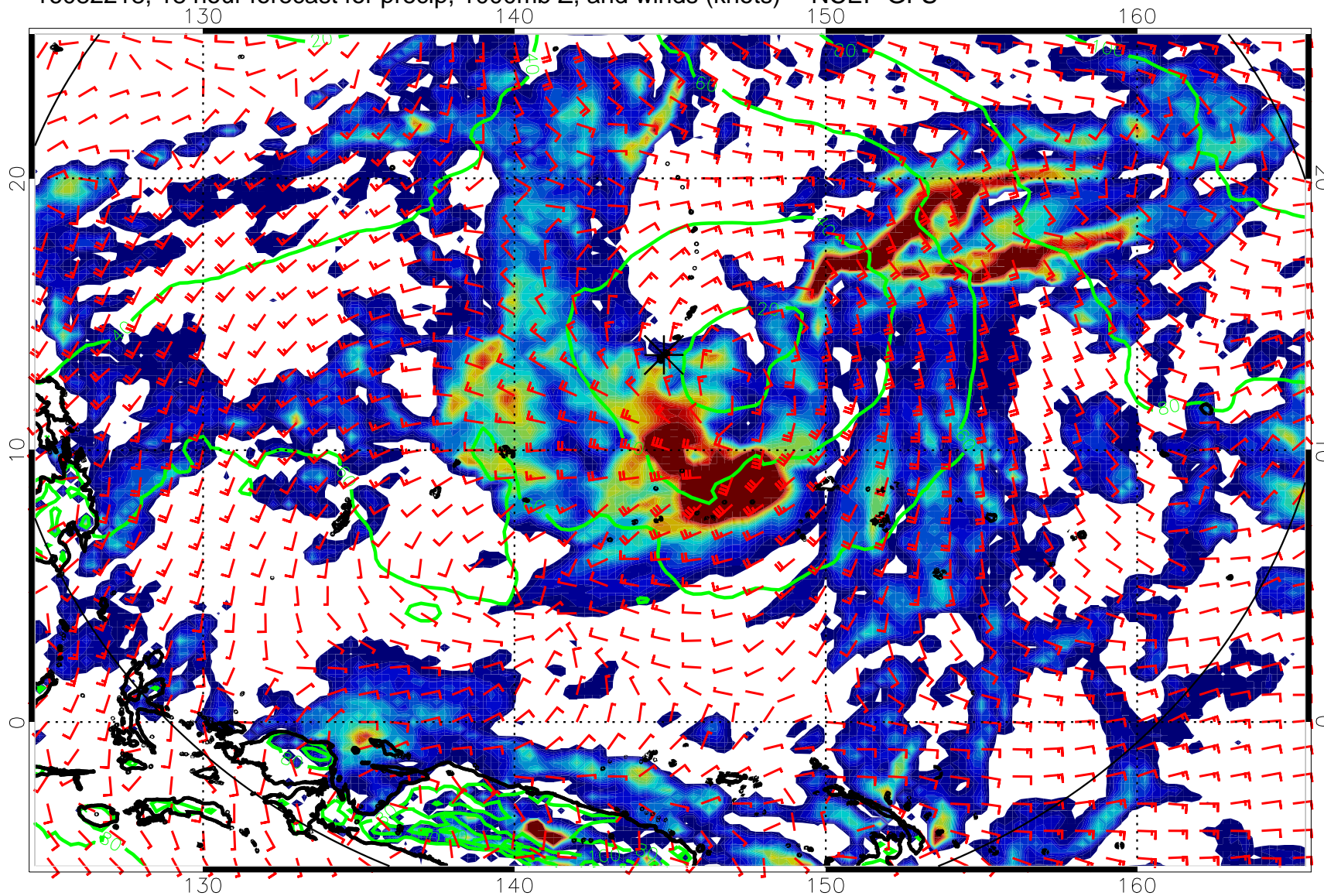
16082218, 18 hour forecast for precip, 1000mb Z, and winds (knots) -- NCEP GFS
