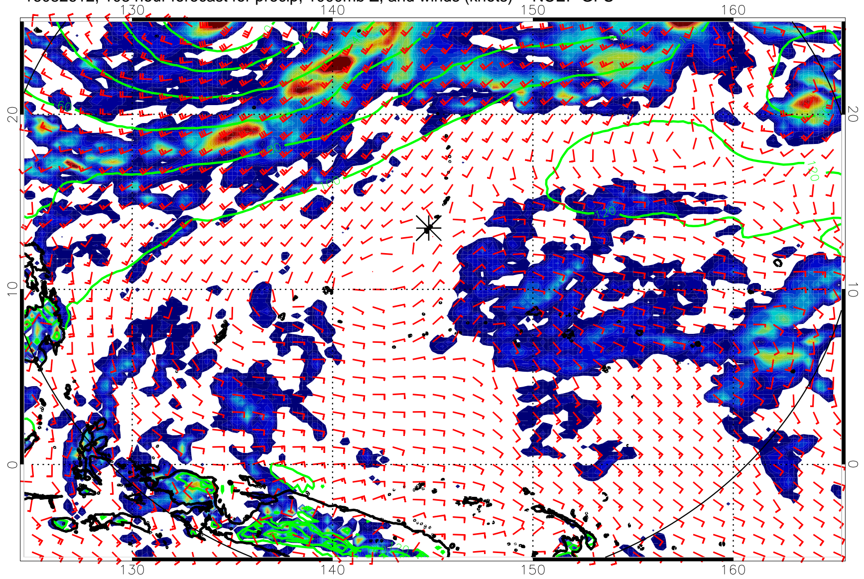
16082612, 108 hour forecast for precip, 1000mb Z, and winds (knots) -- NCEP GFS
