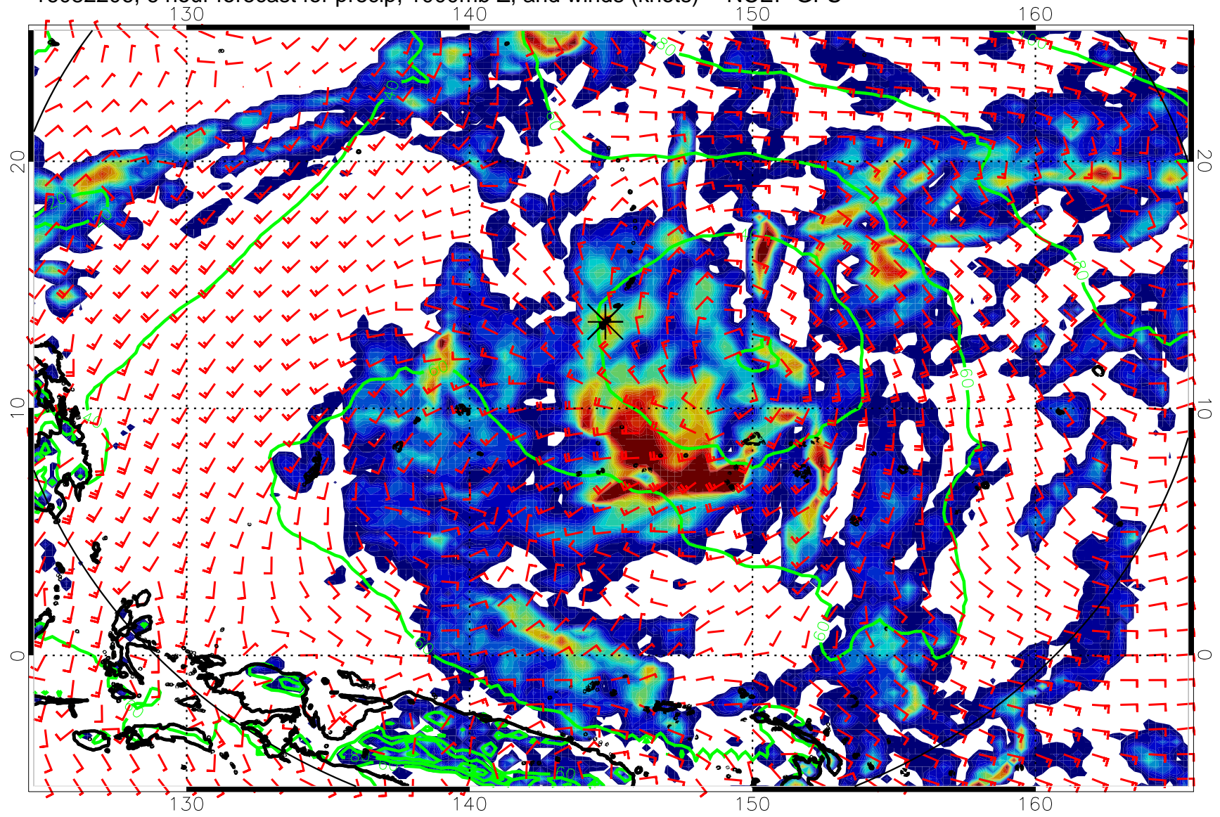
16082206, 6 hour forecast for precip, 1000mb Z, and winds (knots) -- NCEP GFS
