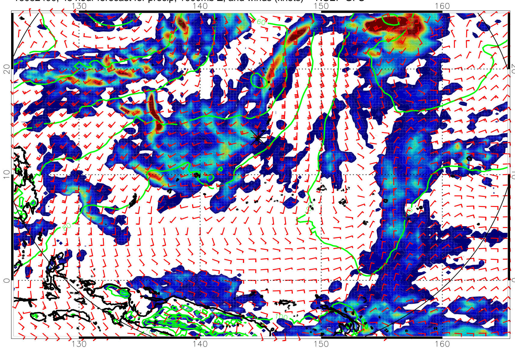
16082400, 48 hour forecast for precip, 1000mb Z, and winds (knots) -- NCEP GFS
