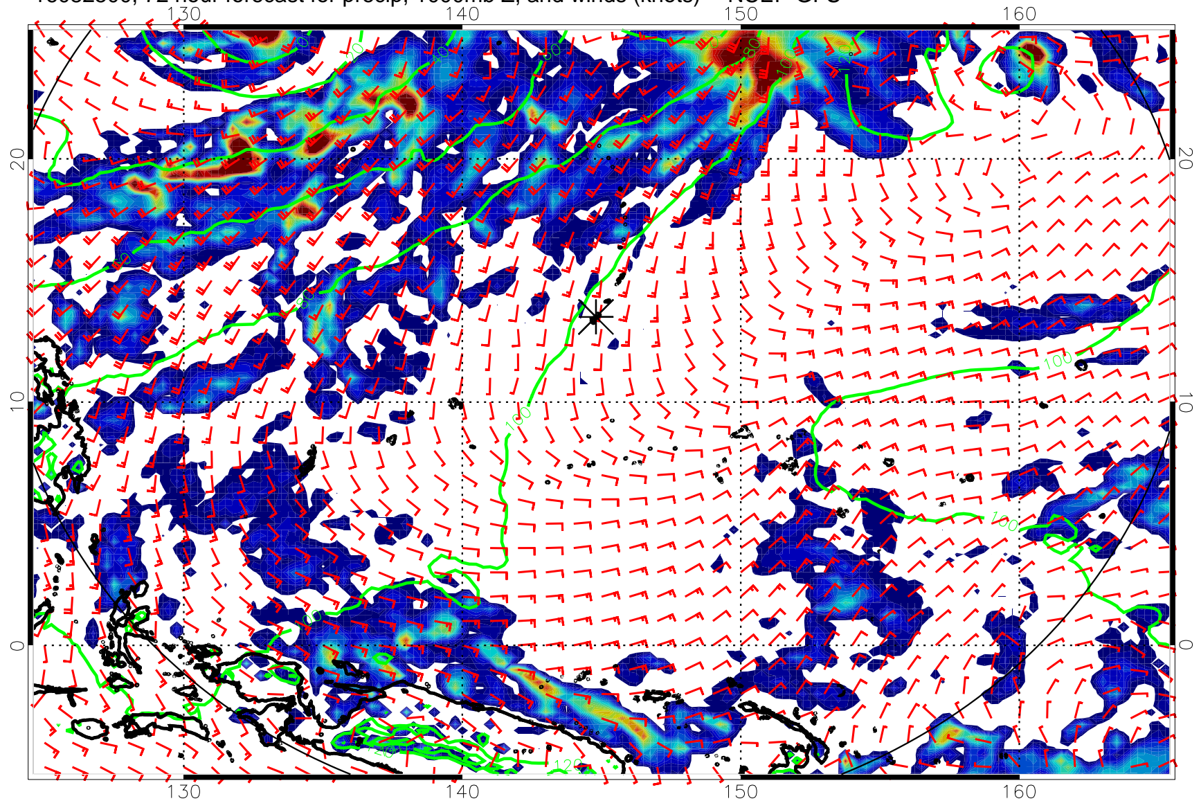
16082500, 72 hour forecast for precip, 1000mb Z, and winds (knots) -- NCEP GFS
