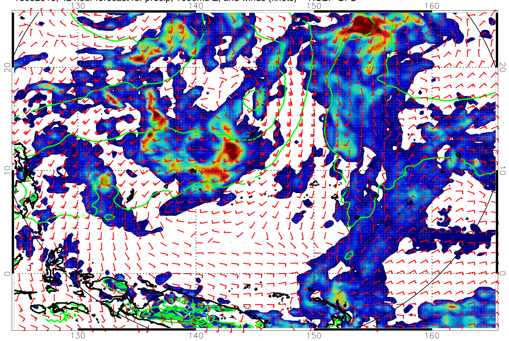
16082318, 42 hour forecast for precip, 1000mb Z, and winds (knots) -- NCEP GFS
