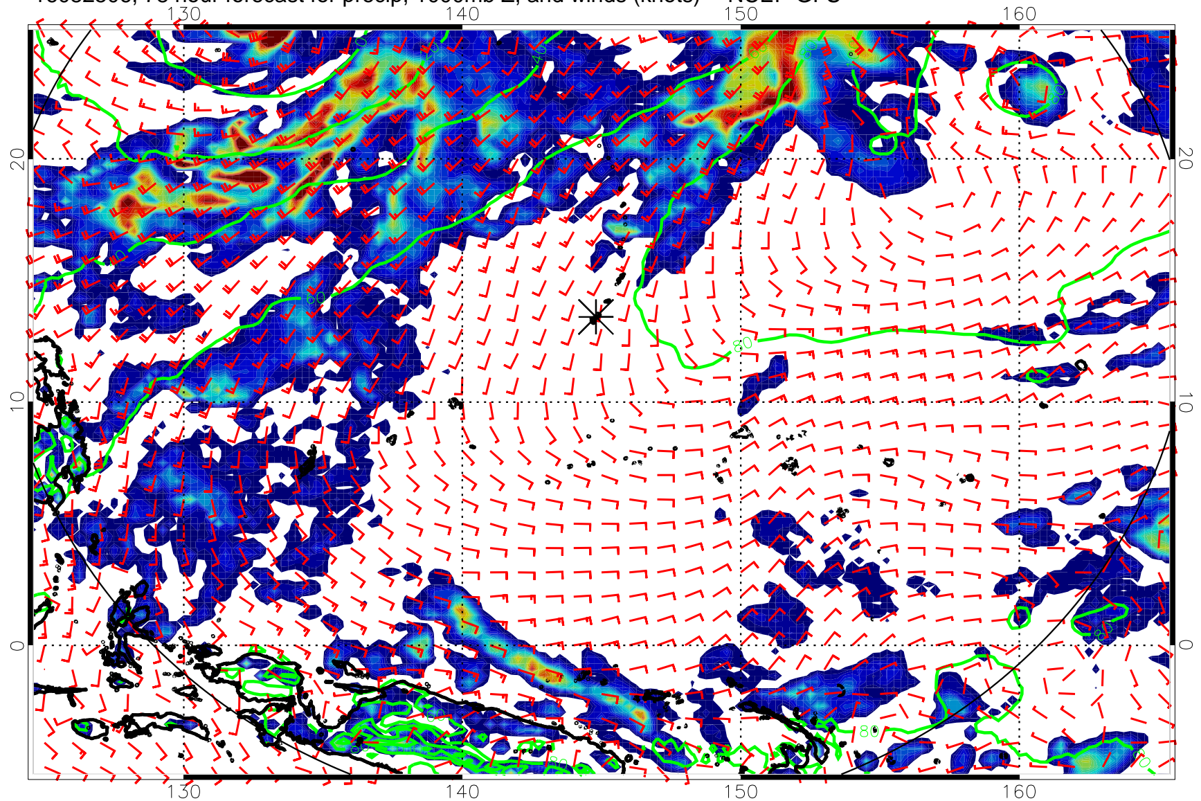
16082506, 78 hour forecast for precip, 1000mb Z, and winds (knots) -- NCEP GFS
