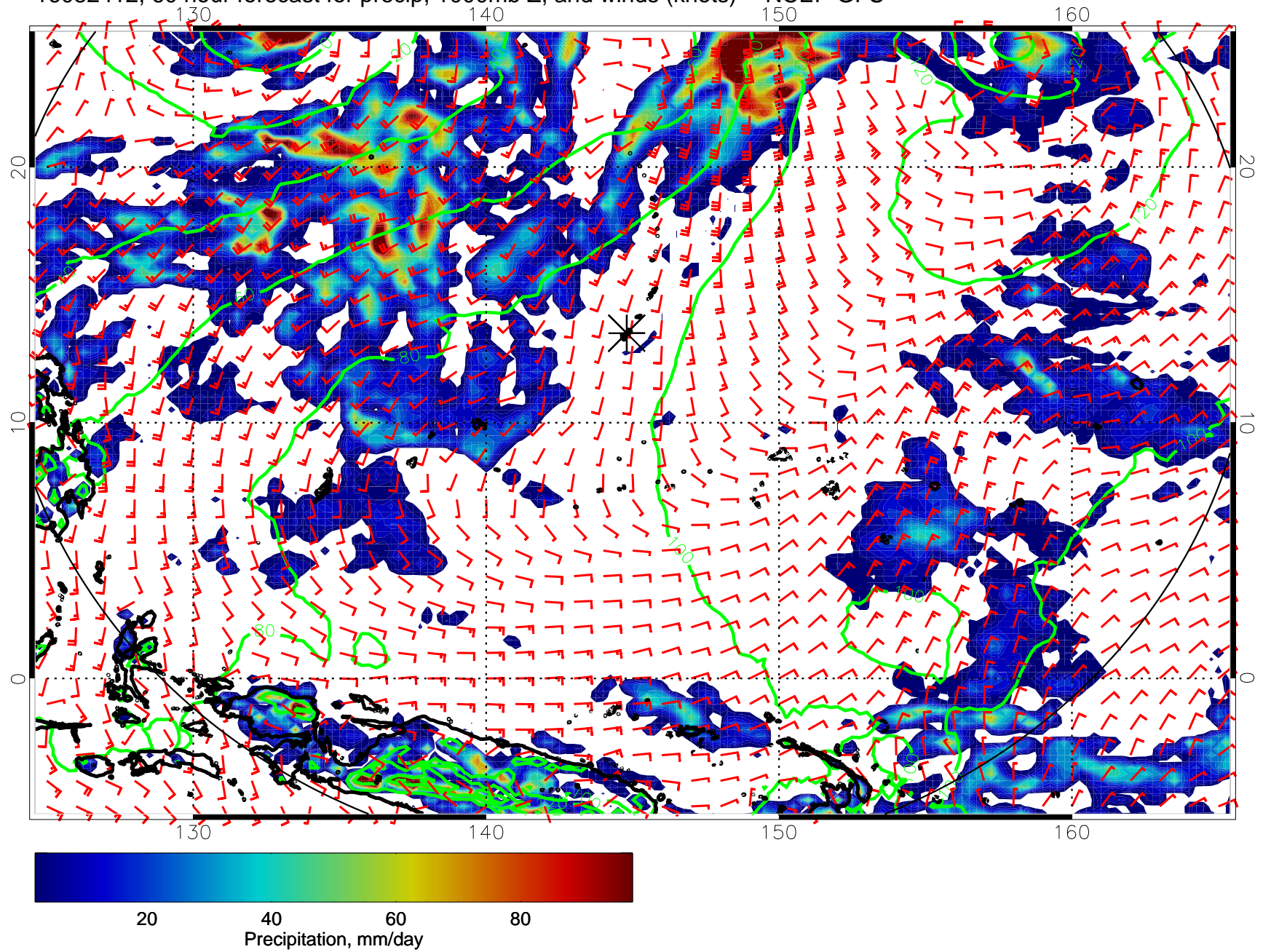
16082412, 60 hour forecast for precip, 1000mb Z, and winds (knots) -- NCEP GFS
