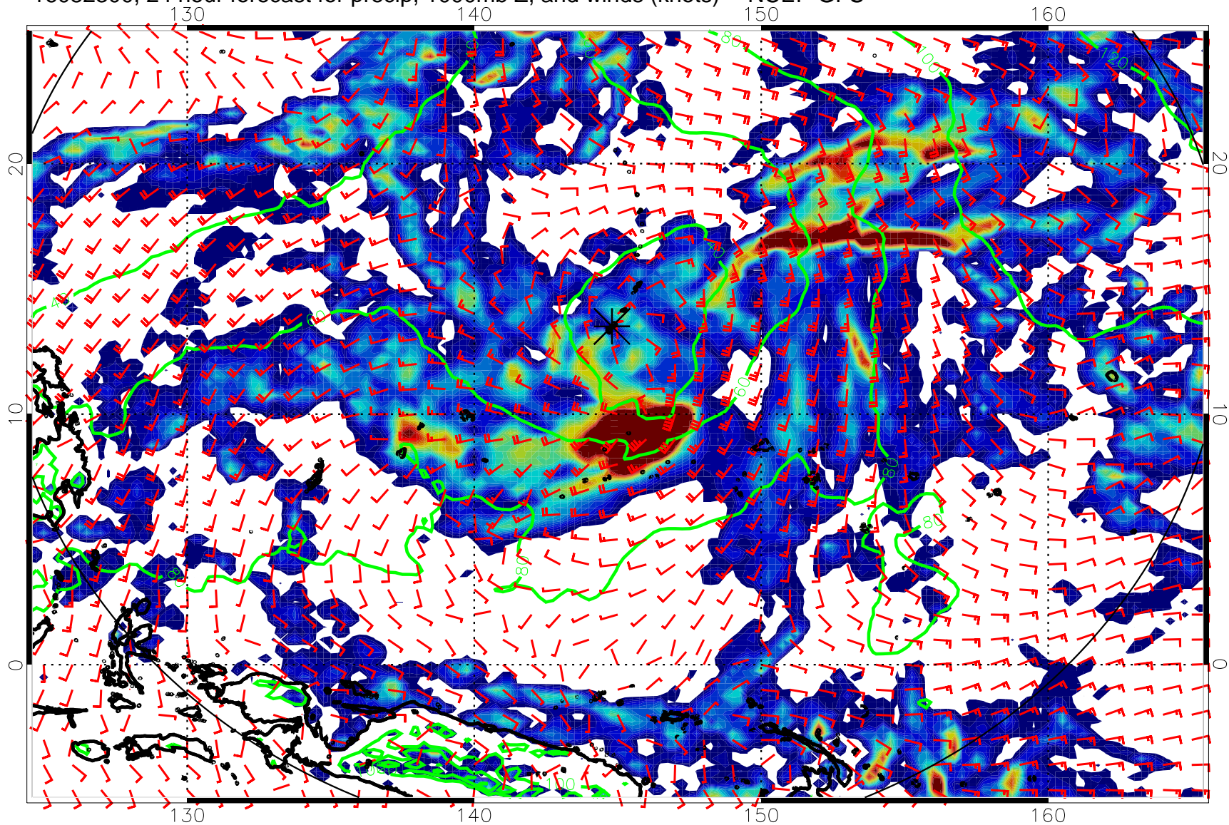
16082300, 24 hour forecast for precip, 1000mb Z, and winds (knots) -- NCEP GFS
