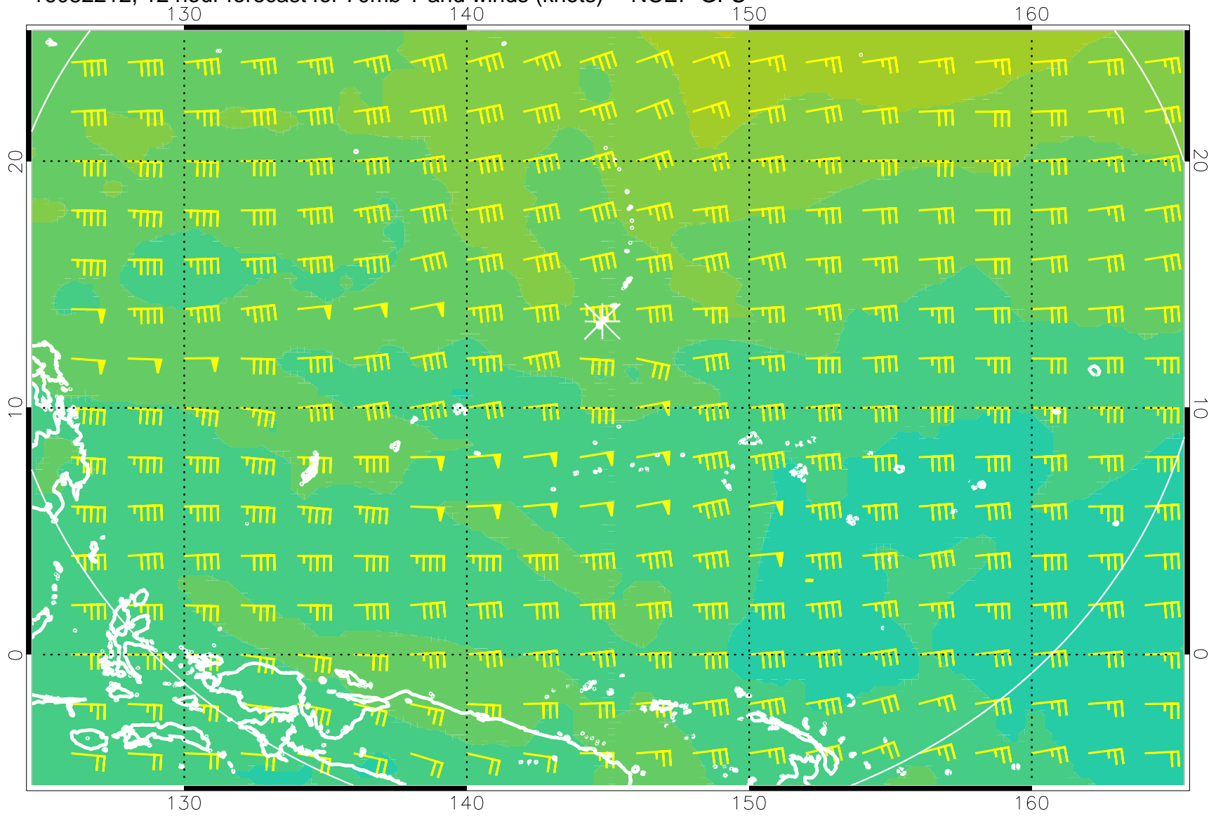
16082212, 12 hour forecast for 70mb T and winds (knots) -- NCEP GFS
