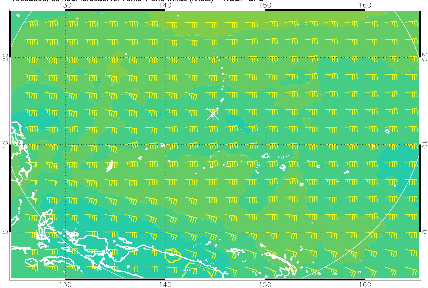
16082306, 30 hour forecast for 70mb T and winds (knots) -- NCEP GFS
