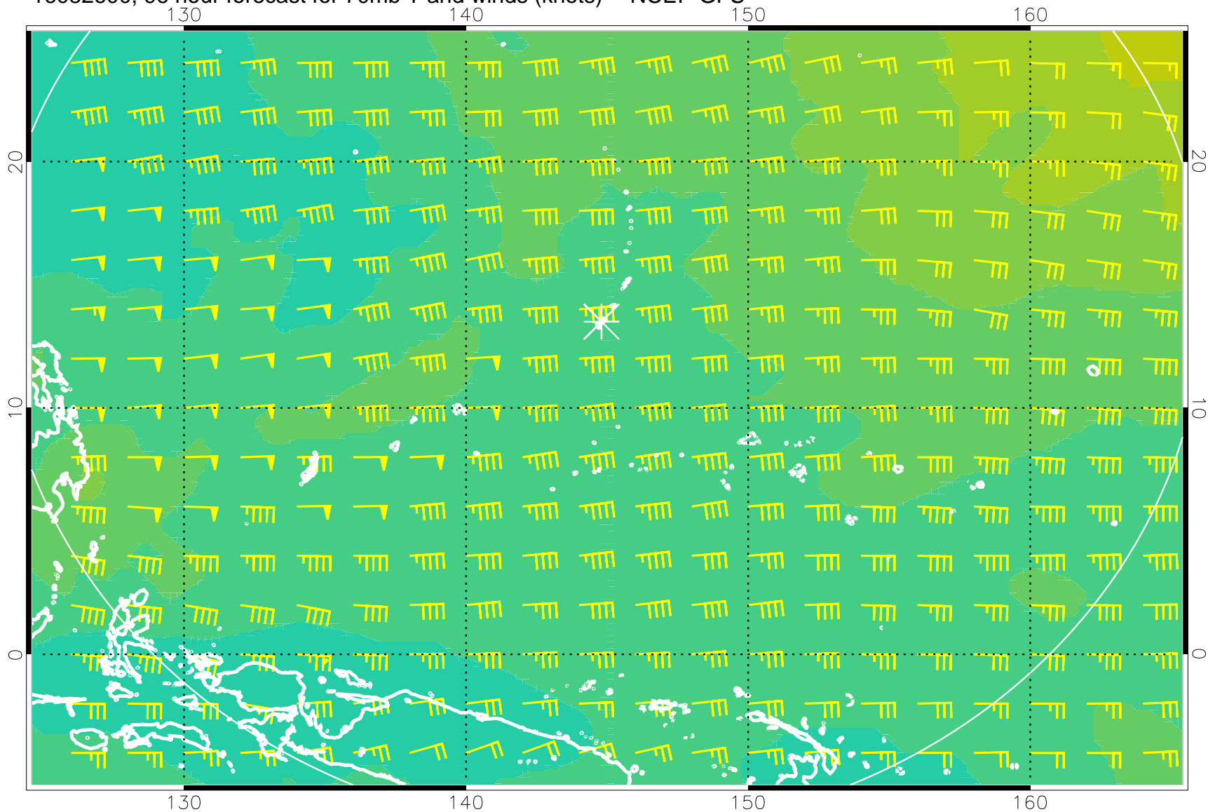
16082600, 96 hour forecast for 70mb T and winds (knots) -- NCEP GFS
