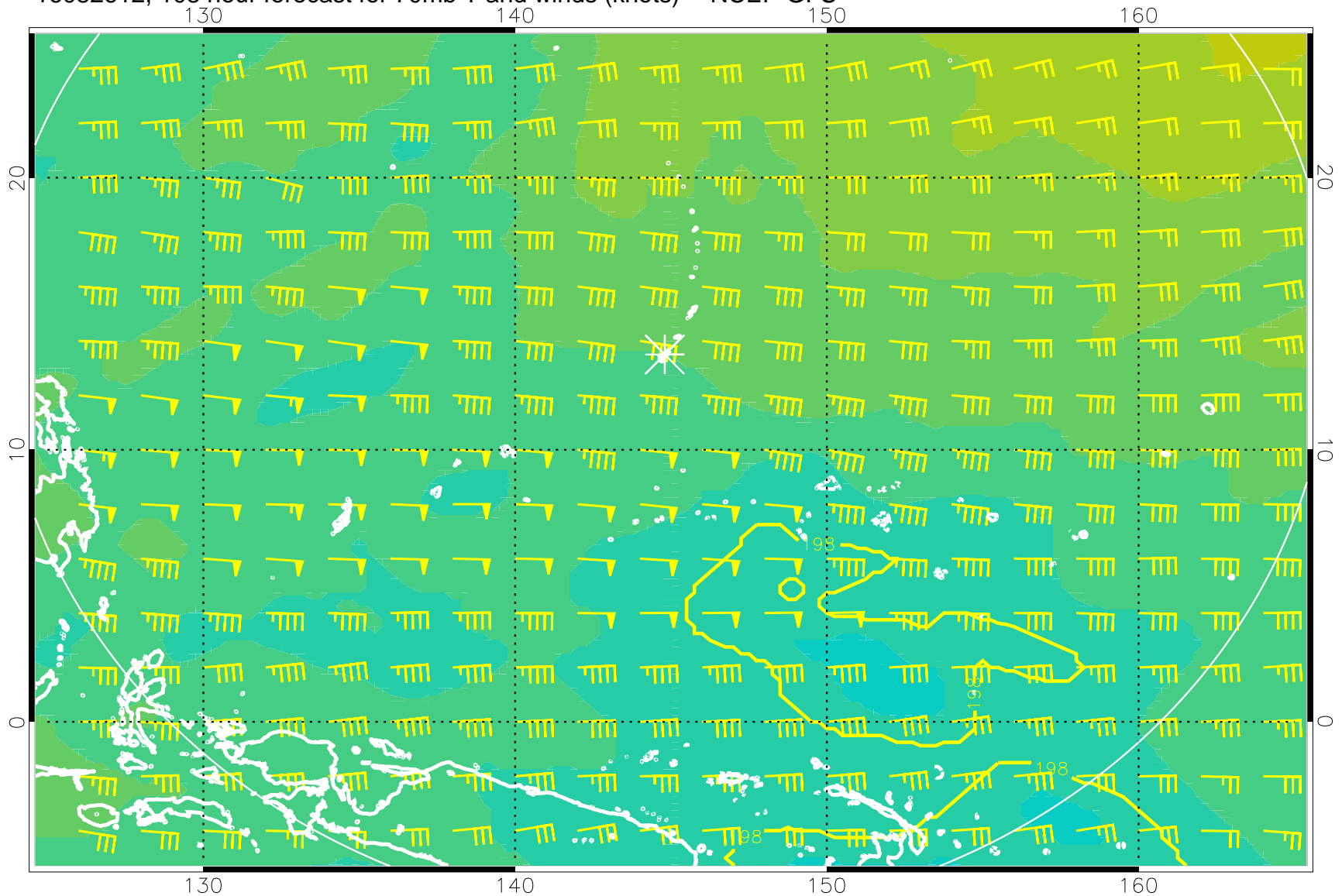
16082612, 108 hour forecast for 70mb T and winds (knots) -- NCEP GFS
