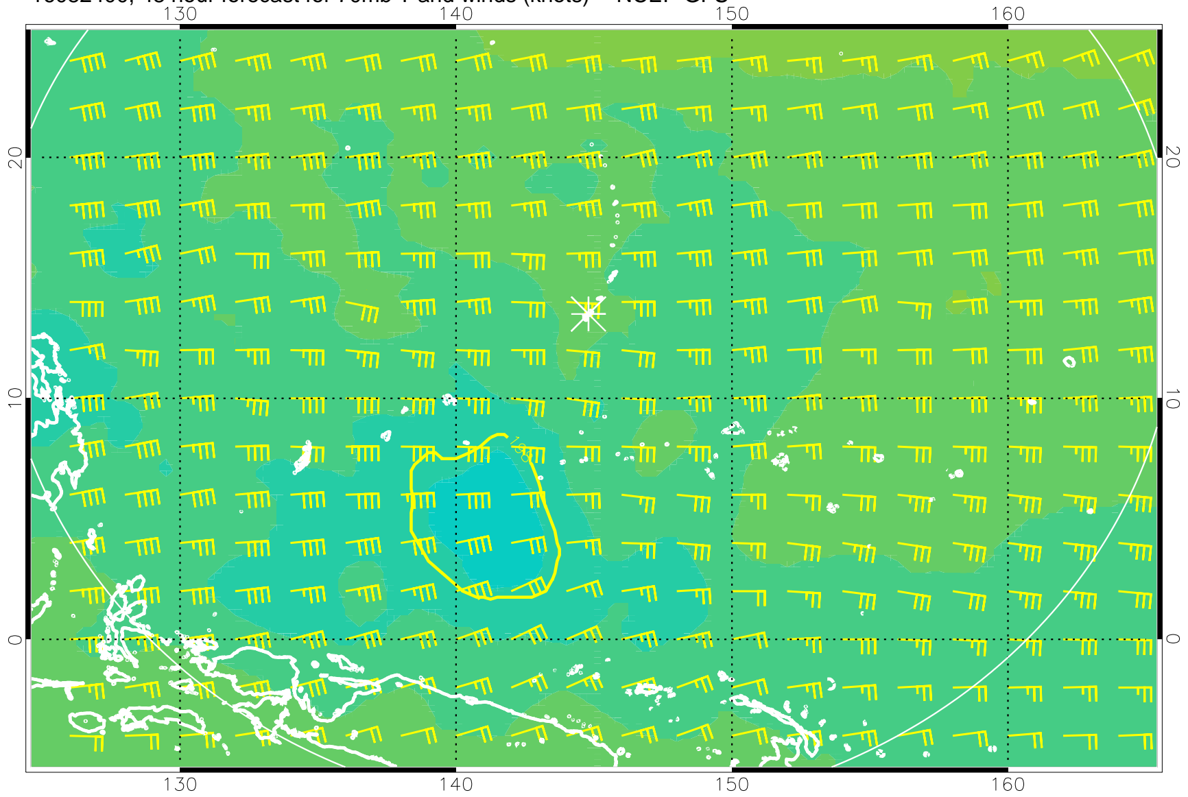
16082400, 48 hour forecast for 70mb T and winds (knots) -- NCEP GFS
