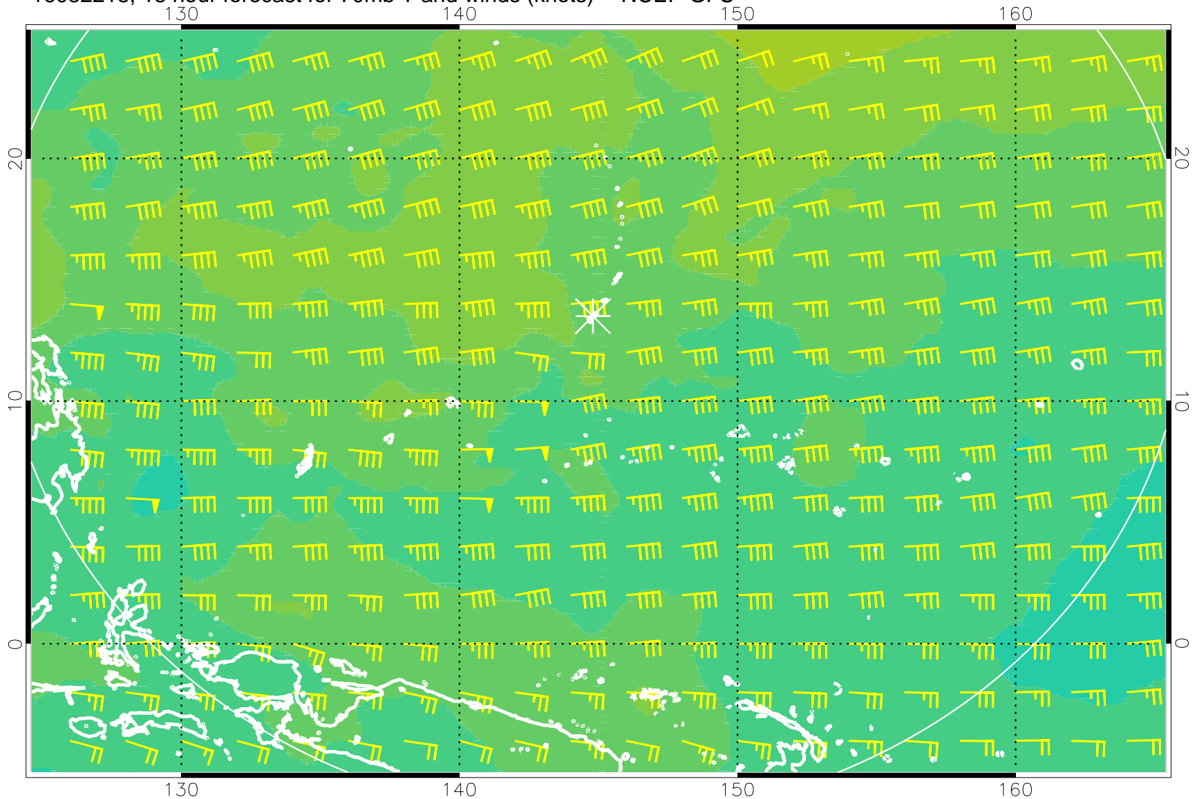
16082218, 18 hour forecast for 70mb T and winds (knots) -- NCEP GFS
