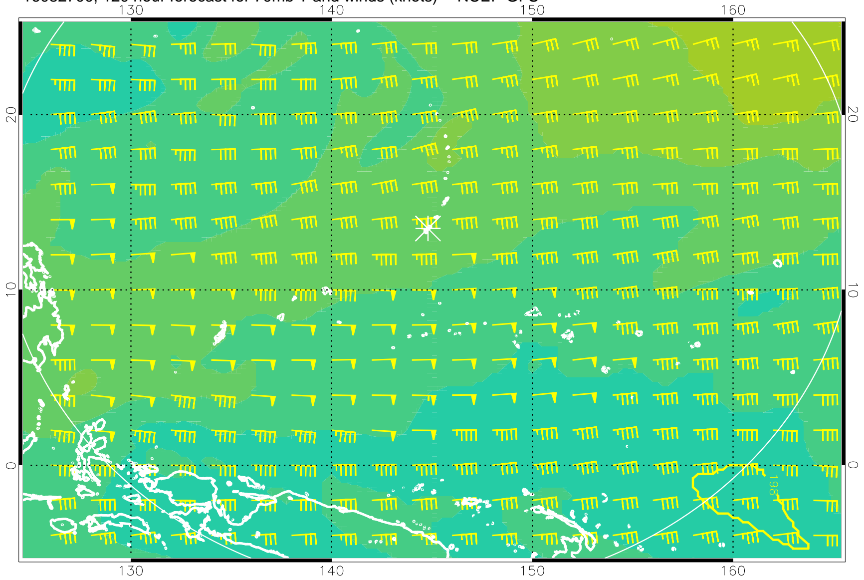
16082700, 120 hour forecast for 70mb T and winds (knots) -- NCEP GFS
