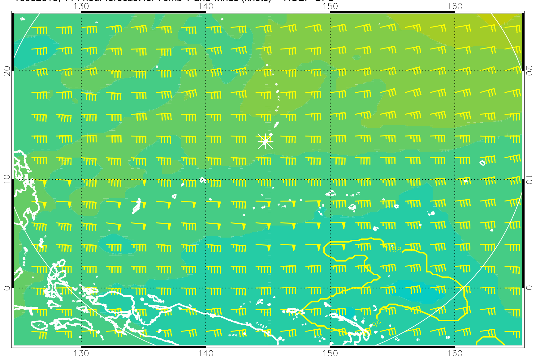
16082618, 114 hour forecast for 70mb T and winds (knots) -- NCEP GFS
