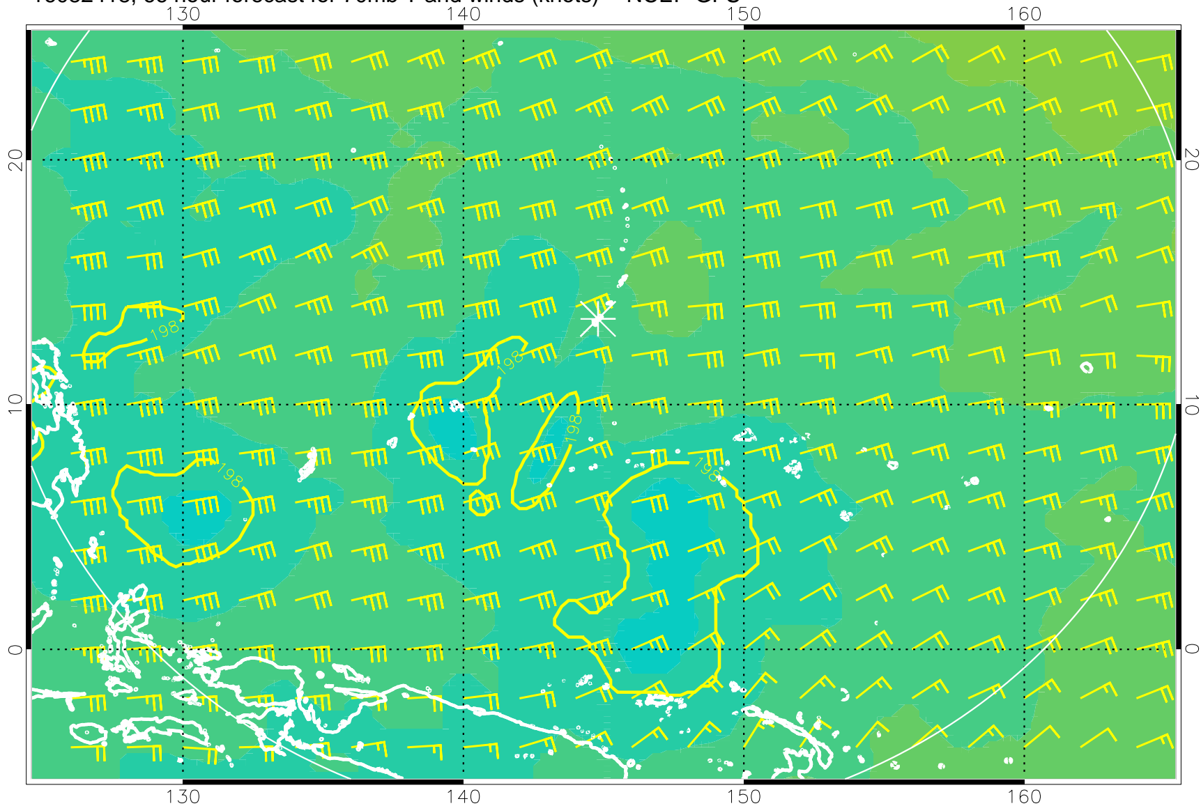
16082418, 66 hour forecast for 70mb T and winds (knots) -- NCEP GFS
