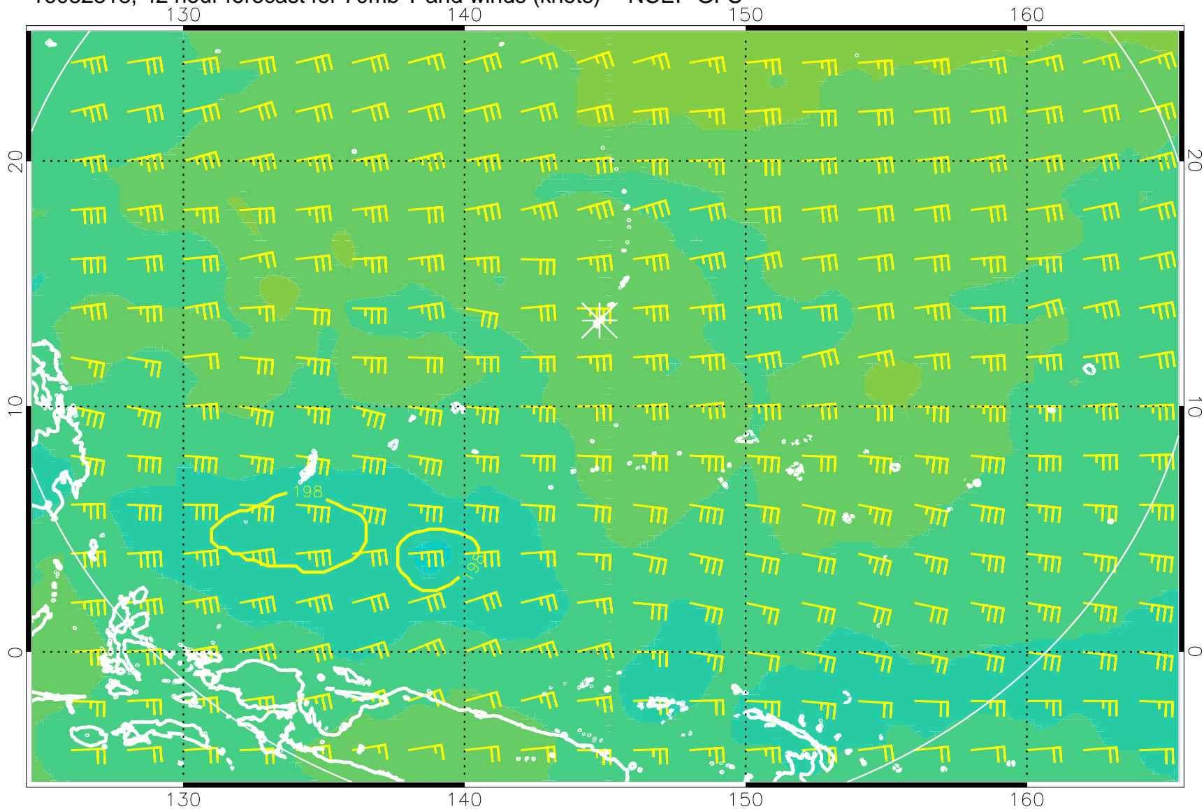
16082318, 42 hour forecast for 70mb T and winds (knots) -- NCEP GFS
