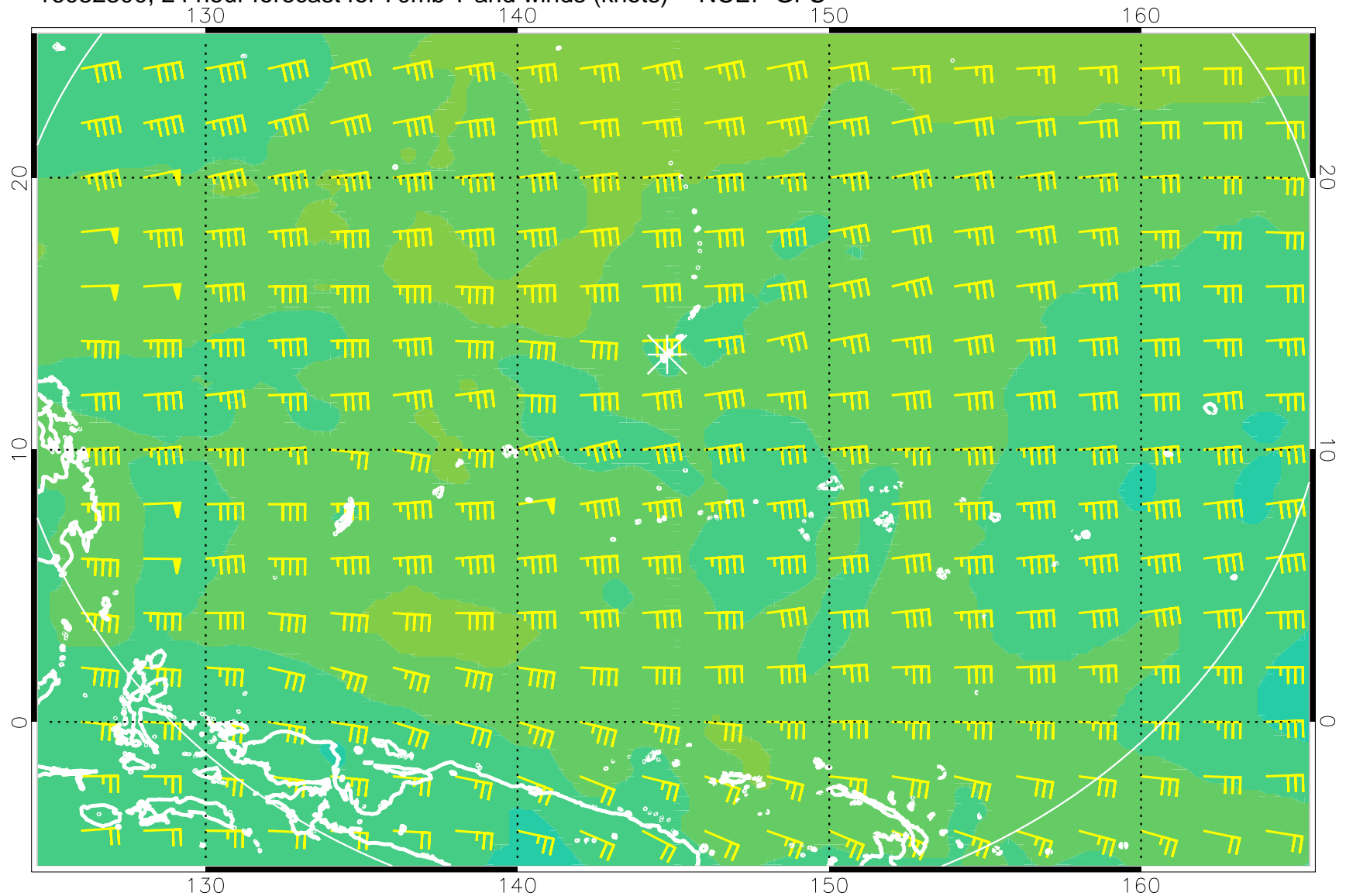
16082300, 24 hour forecast for 70mb T and winds (knots) -- NCEP GFS
