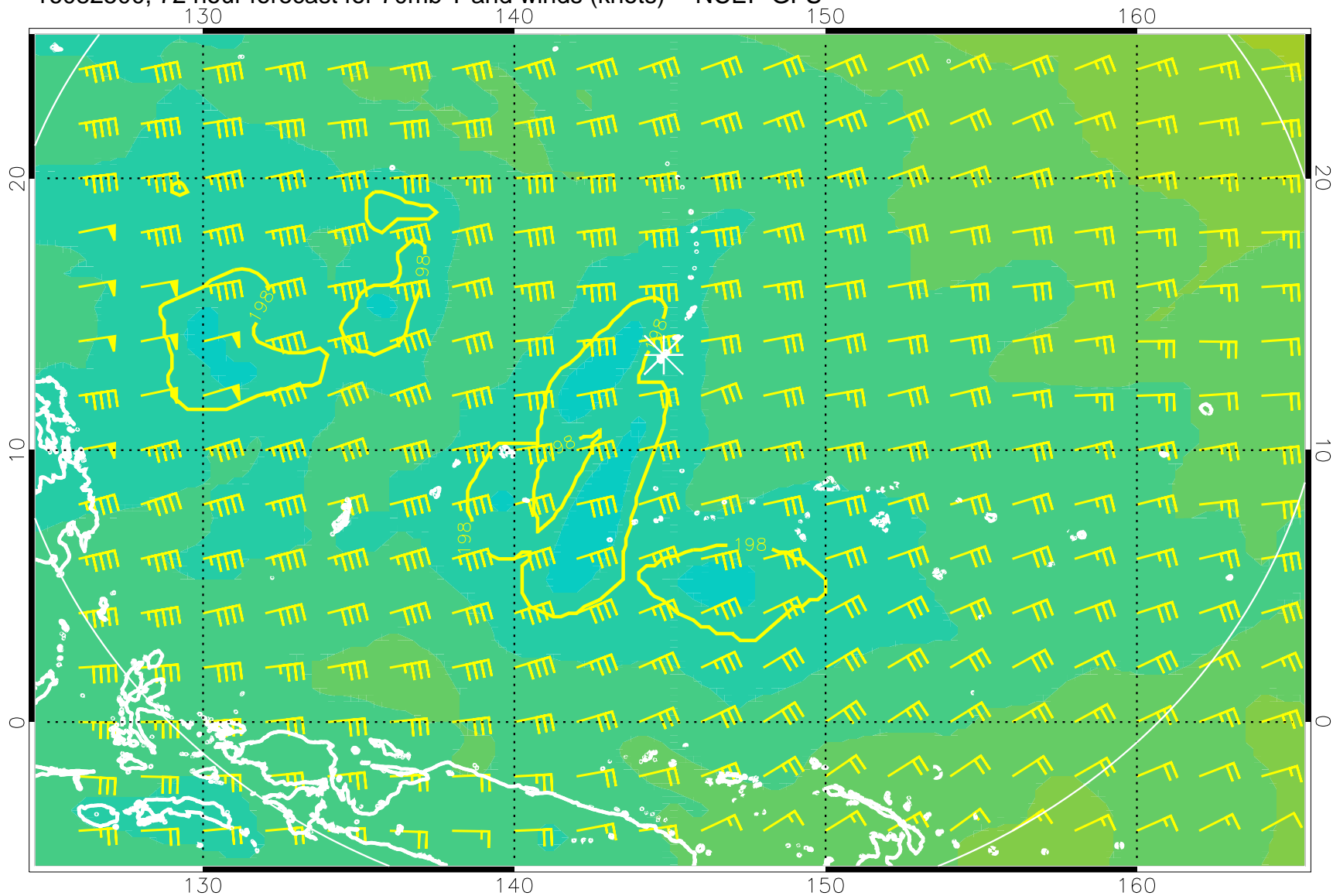
16082500, 72 hour forecast for 70mb T and winds (knots) -- NCEP GFS
