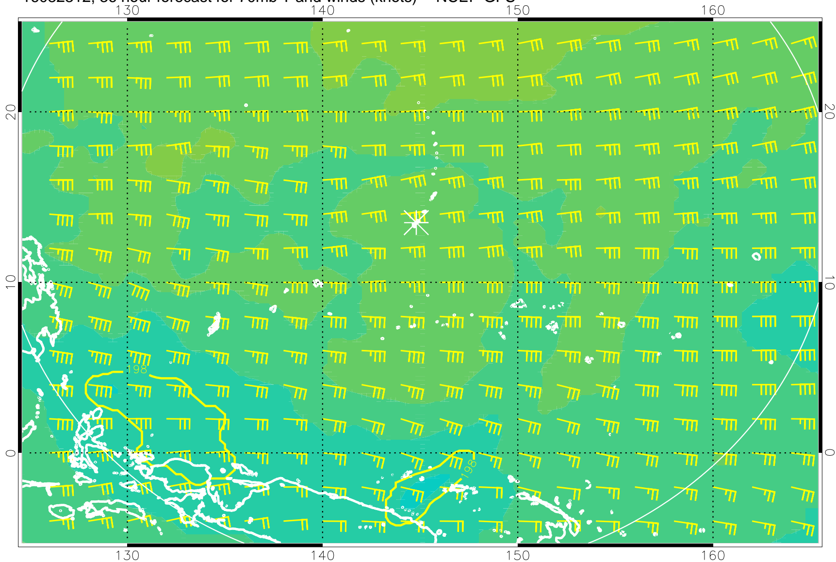
16082312, 36 hour forecast for 70mb T and winds (knots) -- NCEP GFS
