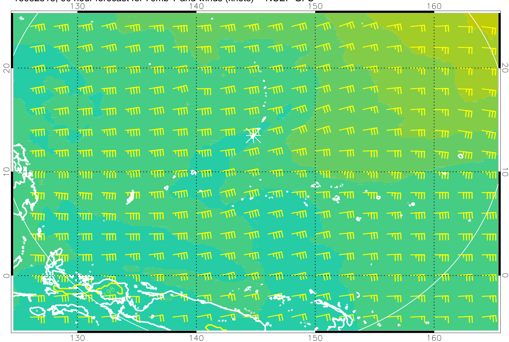
16082518, 90 hour forecast for 70mb T and winds (knots) -- NCEP GFS
