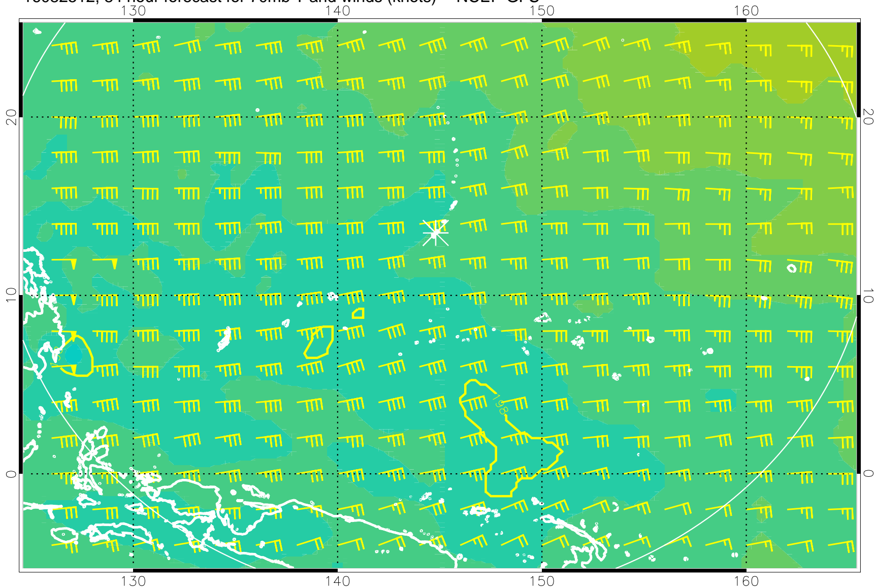
16082512, 84 hour forecast for 70mb T and winds (knots) -- NCEP GFS
