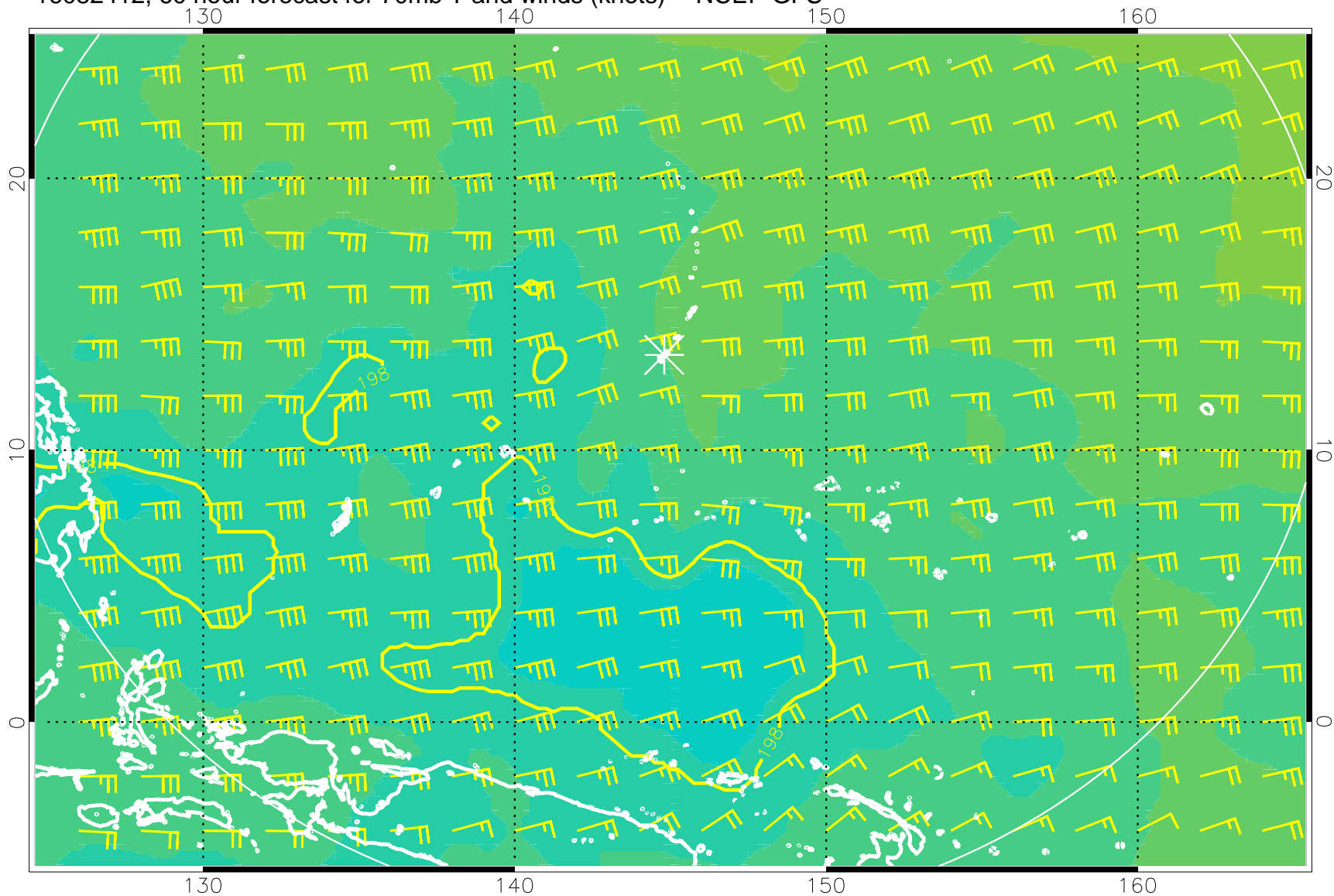
16082412, 60 hour forecast for 70mb T and winds (knots) -- NCEP GFS
