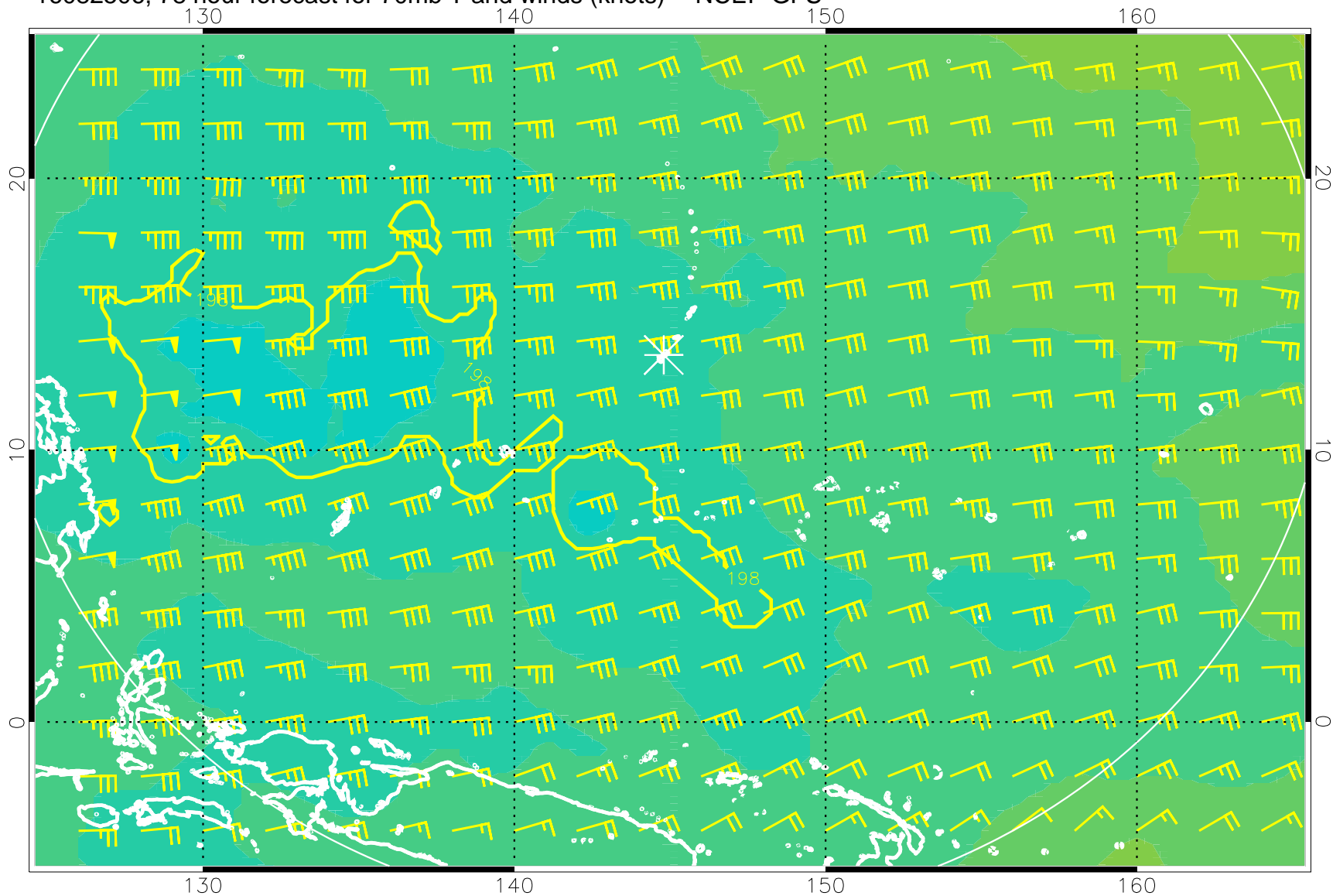
16082506, 78 hour forecast for 70mb T and winds (knots) -- NCEP GFS
