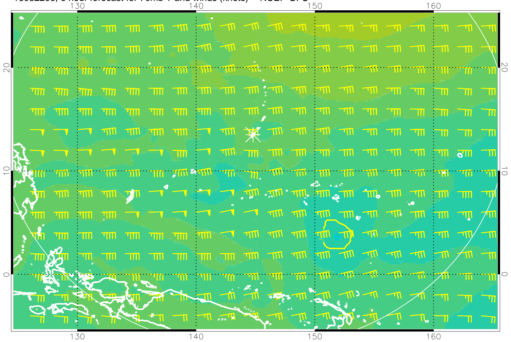
16082206, 6 hour forecast for 70mb T and winds (knots) -- NCEP GFS
