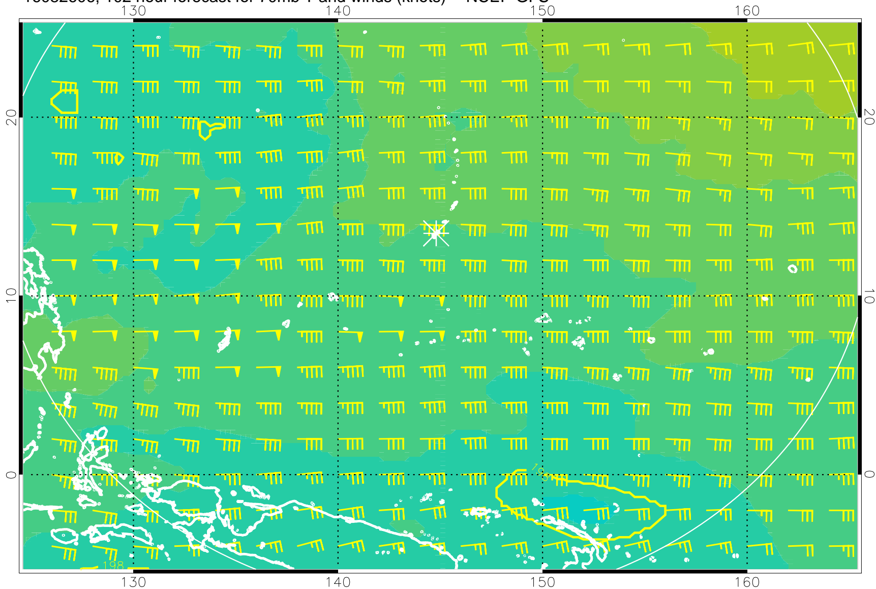
16082606, 102 hour forecast for 70mb T and winds (knots) -- NCEP GFS
