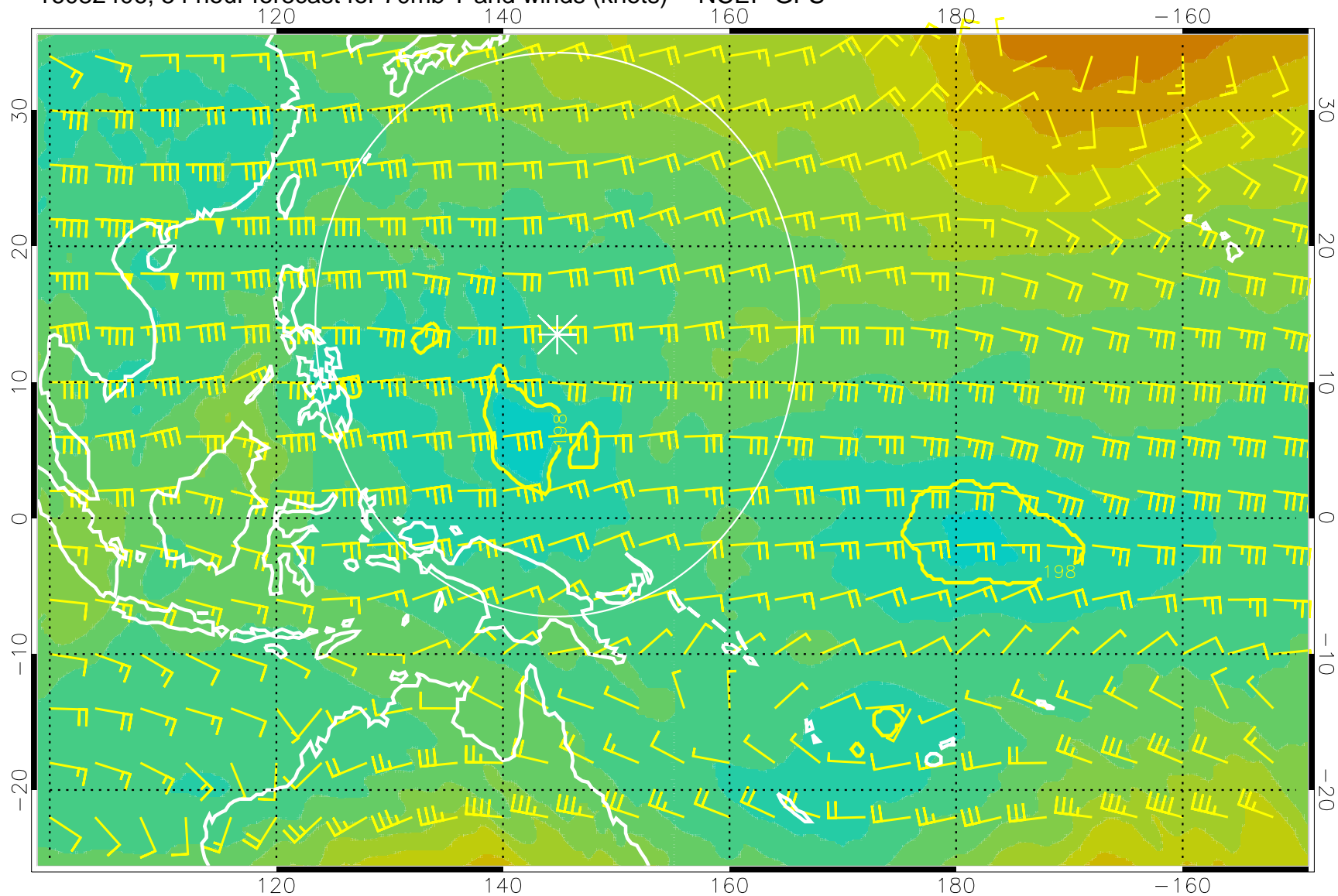
16082406, 54 hour forecast for 70mb T and winds (knots) -- NCEP GFS
