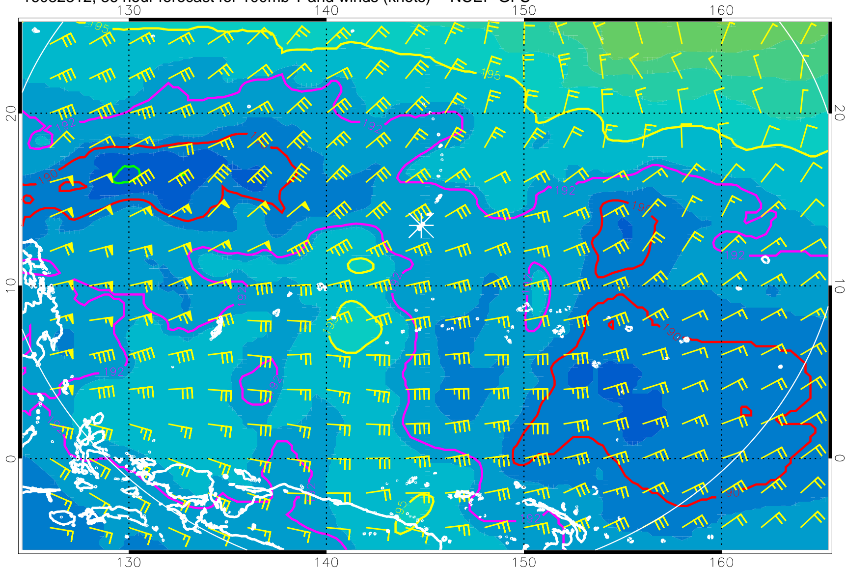
16082312, 36 hour forecast for 100mb T and winds (knots) -- NCEP GFS
