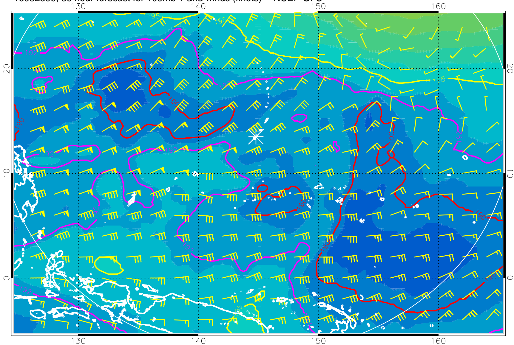
16082306, 30 hour forecast for 100mb T and winds (knots) -- NCEP GFS
