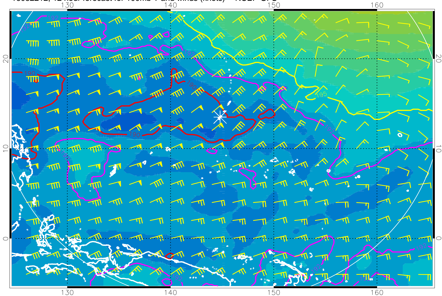
16082212, 12 hour forecast for 100mb T and winds (knots) -- NCEP GFS
