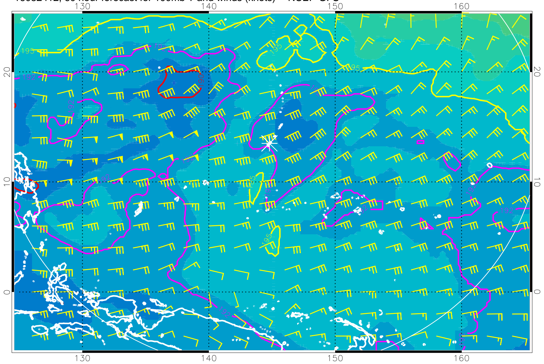
16082412, 60 hour forecast for 100mb T and winds (knots) -- NCEP GFS
