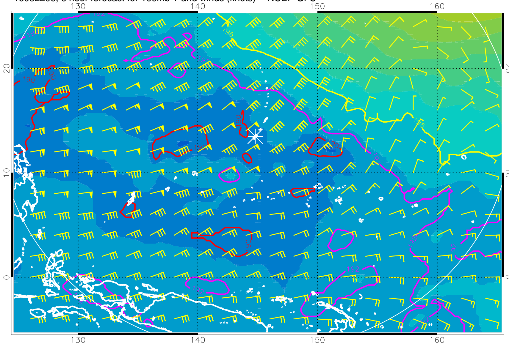
16082206, 6 hour forecast for 100mb T and winds (knots) -- NCEP GFS
