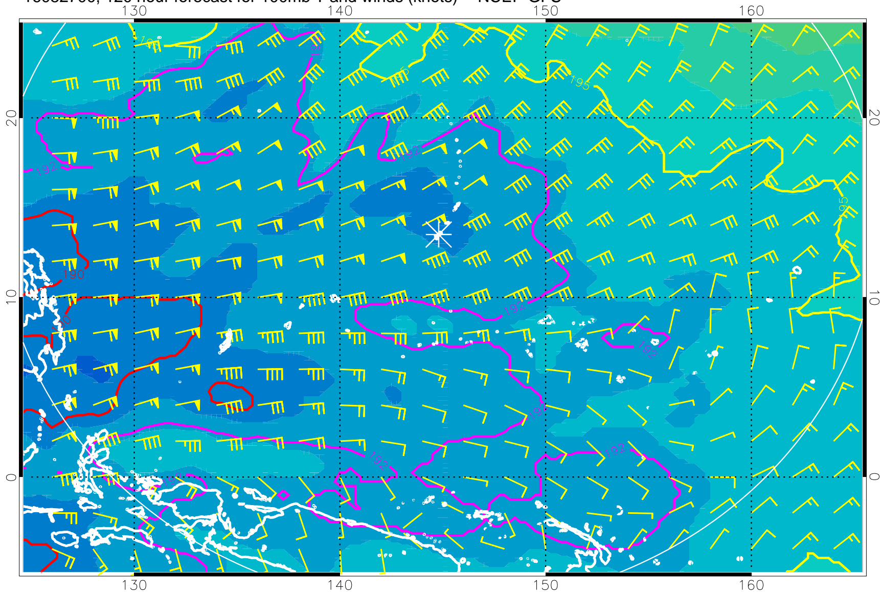
16082700, 120 hour forecast for 100mb T and winds (knots) -- NCEP GFS
