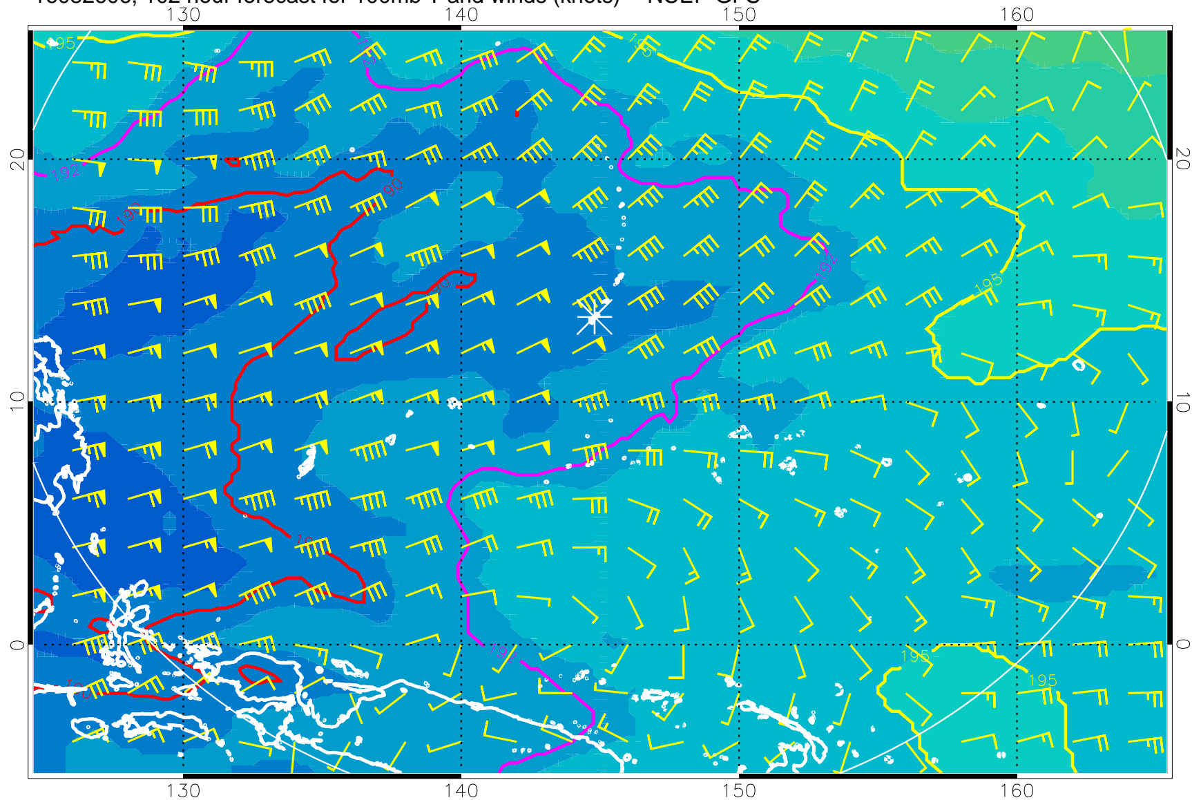
16082606, 102 hour forecast for 100mb T and winds (knots) -- NCEP GFS
