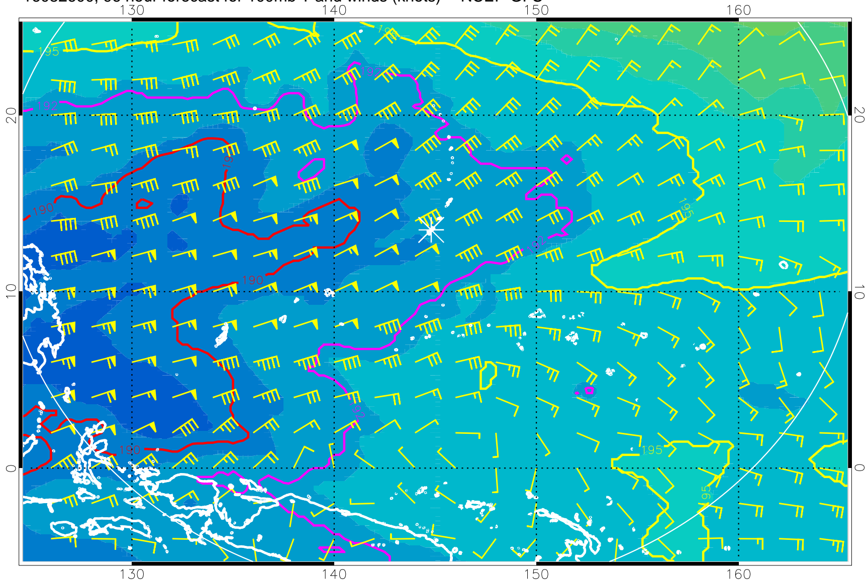
16082600, 96 hour forecast for 100mb T and winds (knots) -- NCEP GFS
