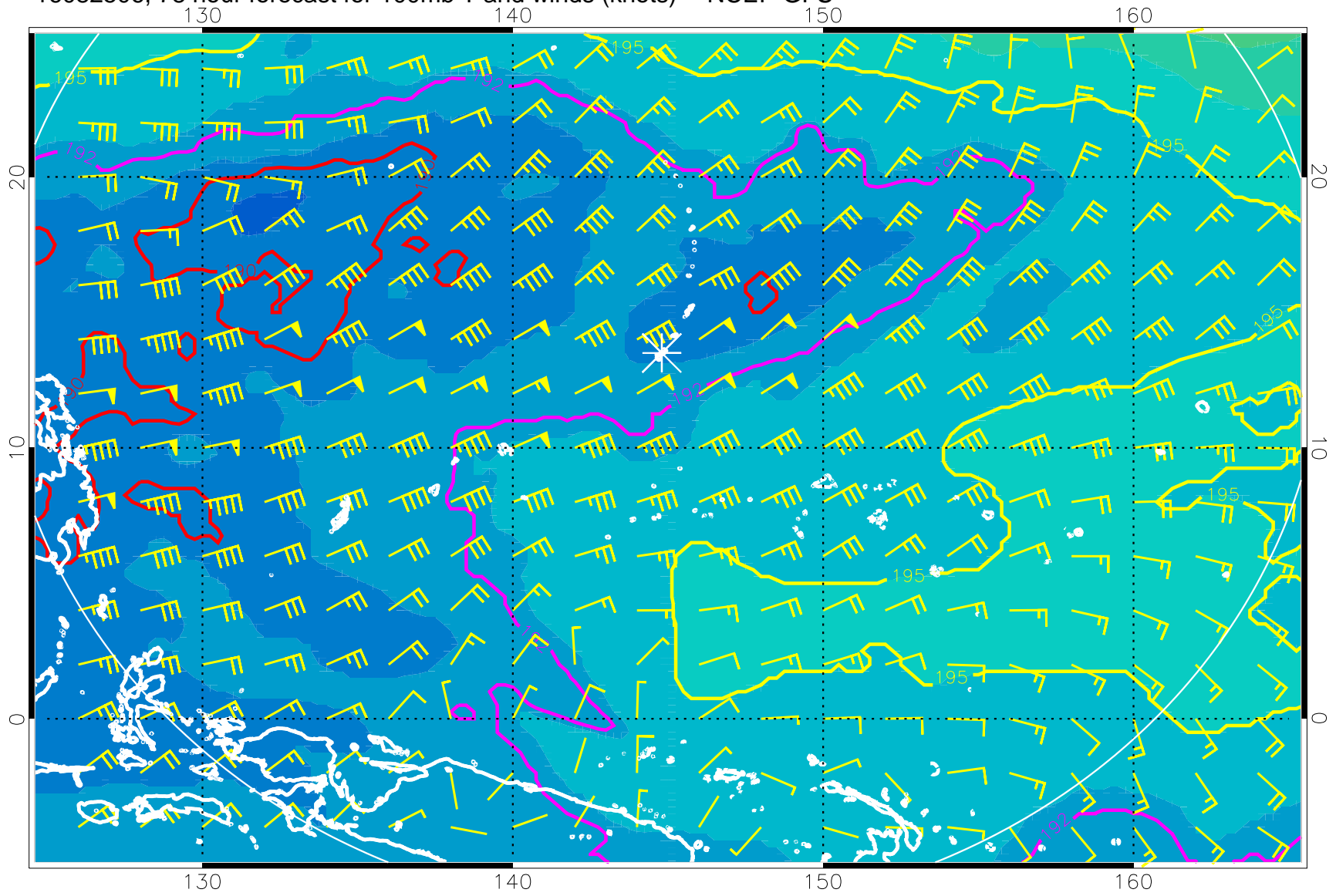
16082506, 78 hour forecast for 100mb T and winds (knots) -- NCEP GFS
