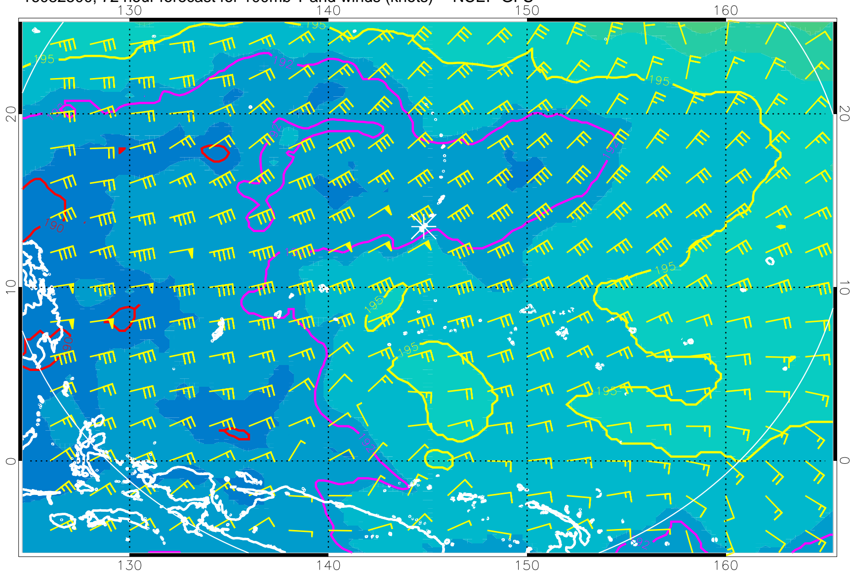
16082500, 72 hour forecast for 100mb T and winds (knots) -- NCEP GFS
