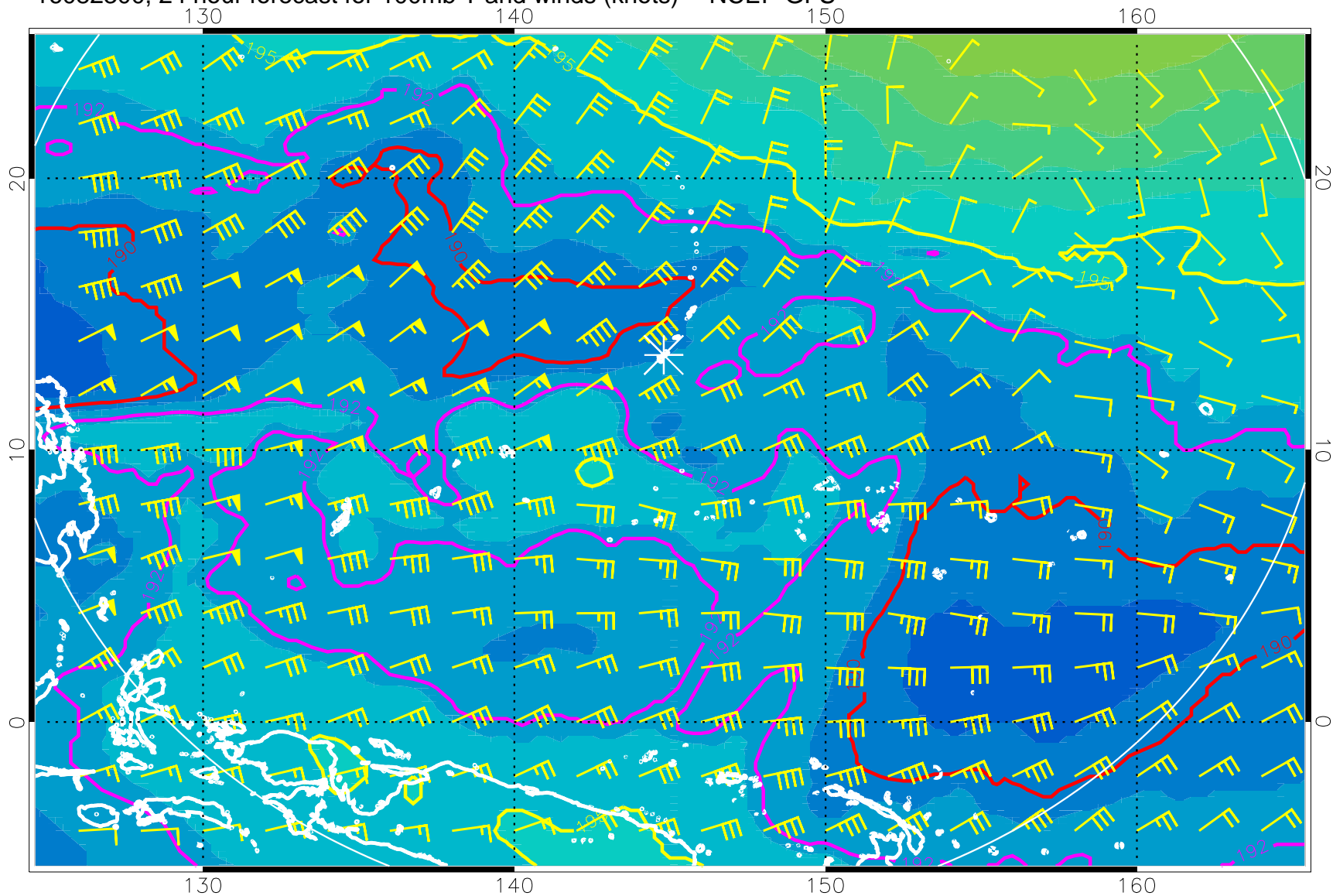
16082300, 24 hour forecast for 100mb T and winds (knots) -- NCEP GFS
