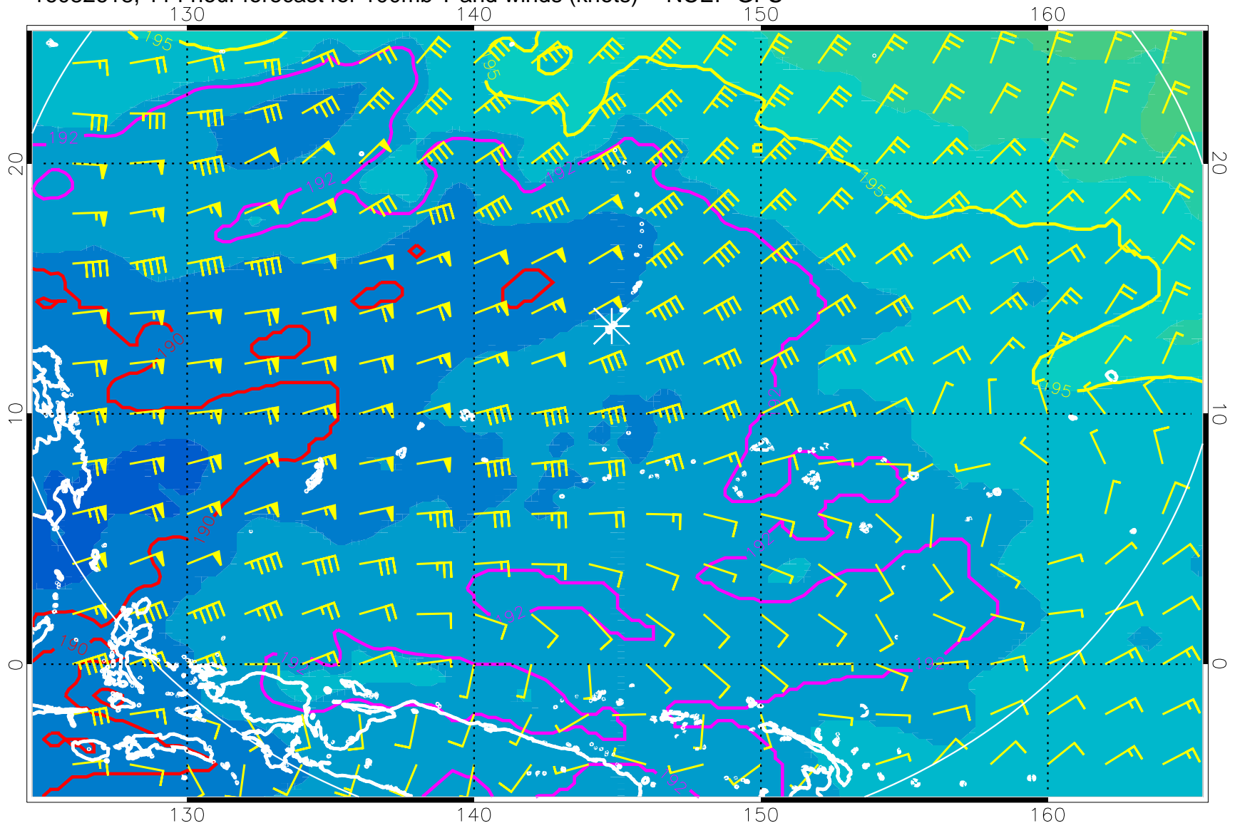
16082618, 114 hour forecast for 100mb T and winds (knots) -- NCEP GFS
