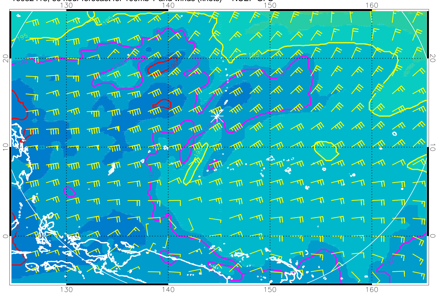
16082418, 66 hour forecast for 100mb T and winds (knots) -- NCEP GFS
