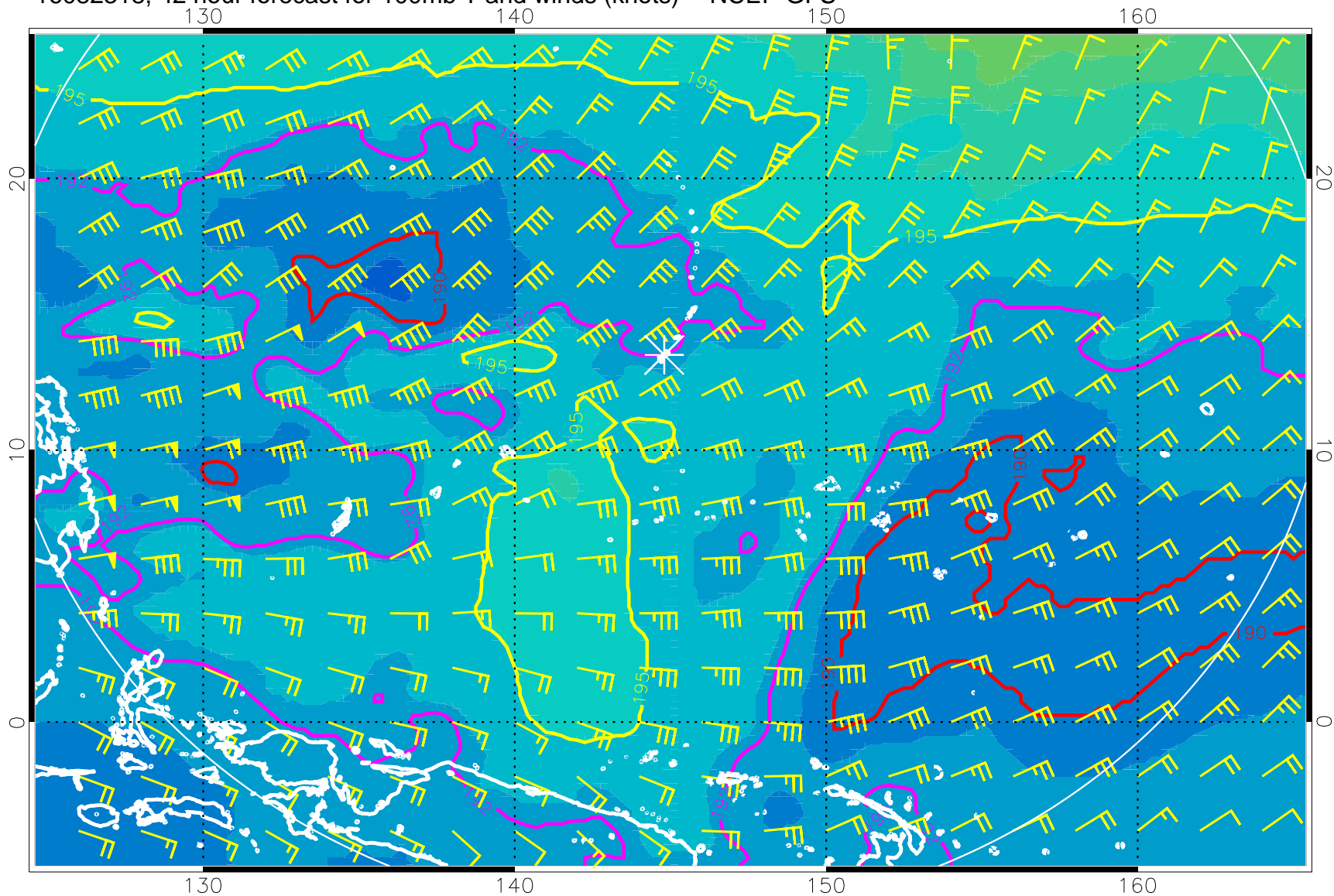
16082318, 42 hour forecast for 100mb T and winds (knots) -- NCEP GFS
