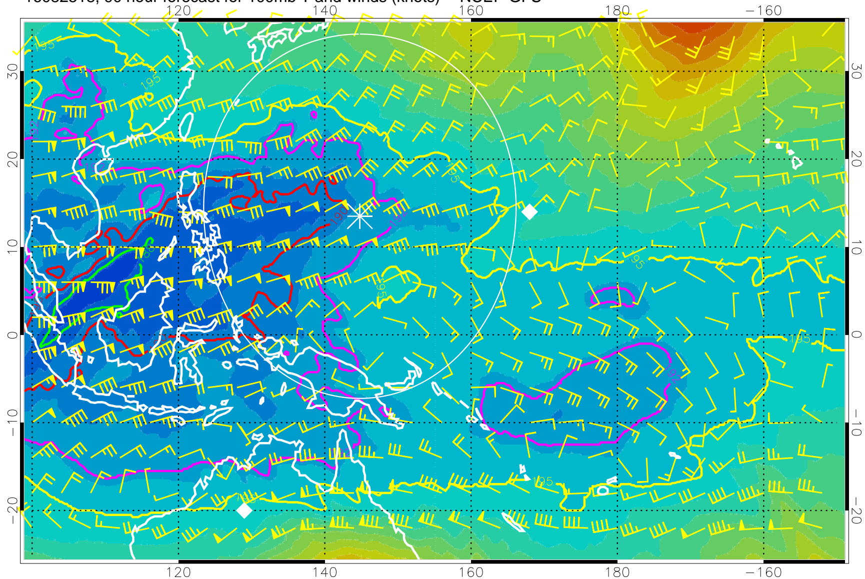
16082518, 90 hour forecast for 100mb T and winds (knots) -- NCEP GFS
