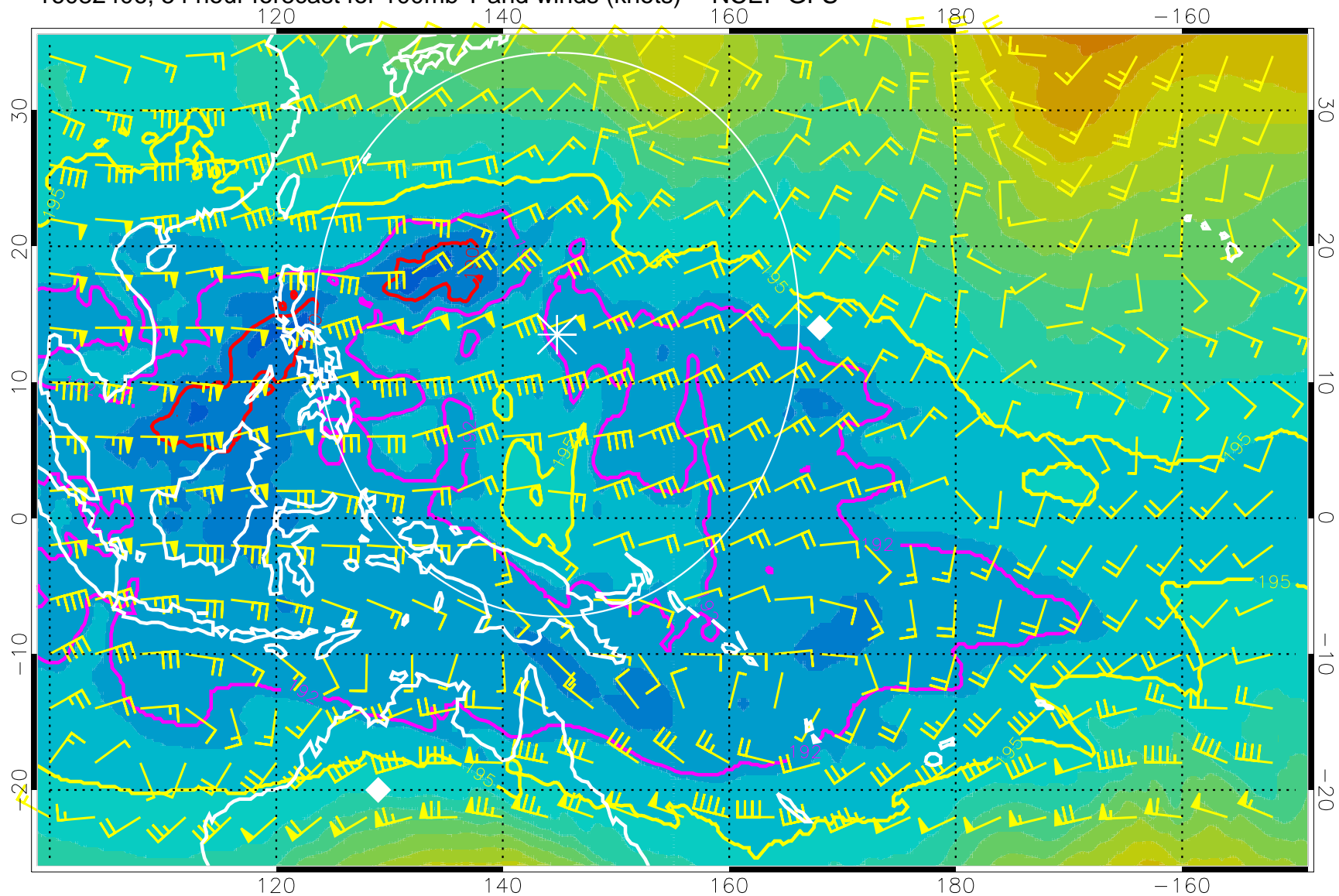
16082406, 54 hour forecast for 100mb T and winds (knots) -- NCEP GFS
