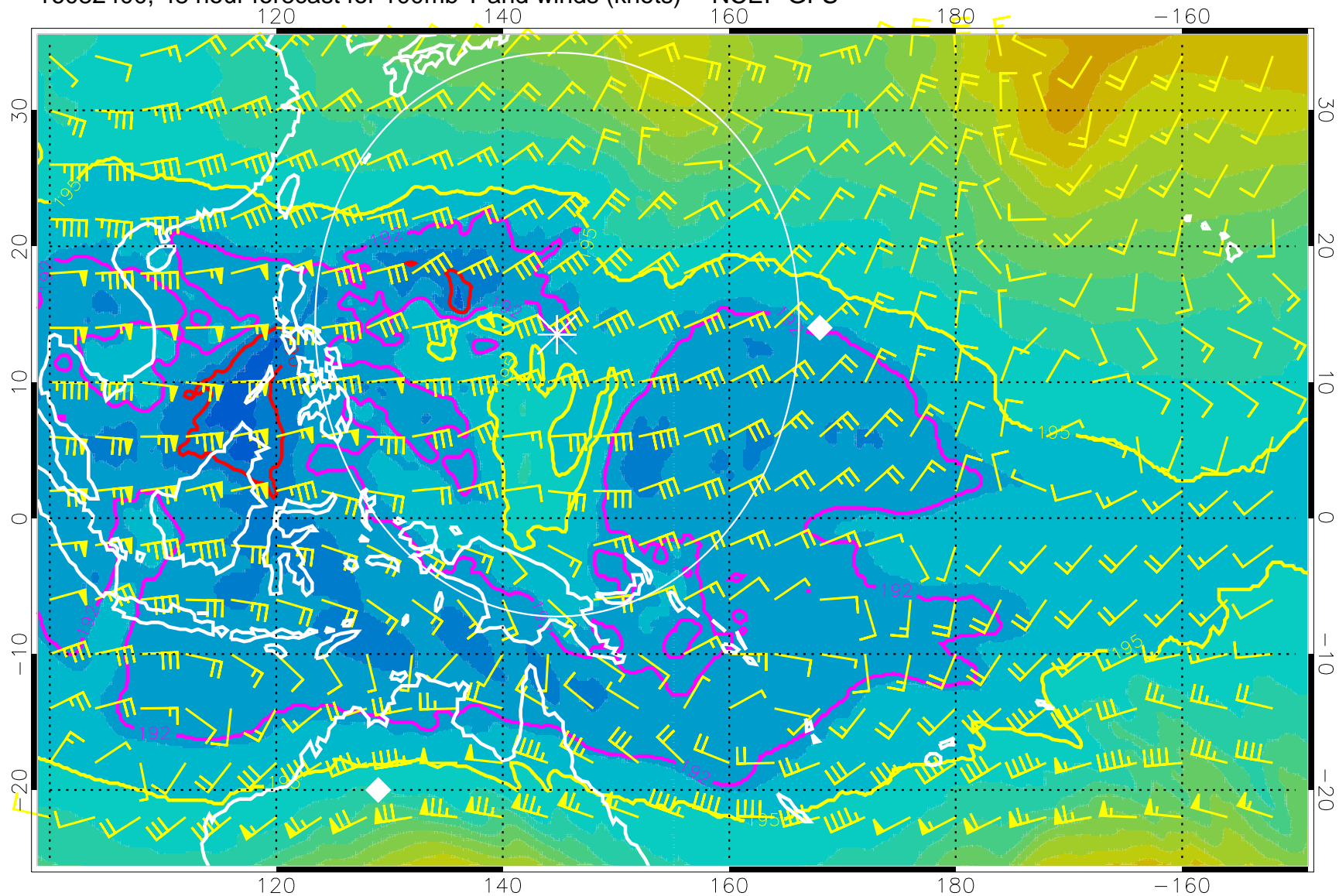
16082400, 48 hour forecast for 100mb T and winds (knots) -- NCEP GFS
