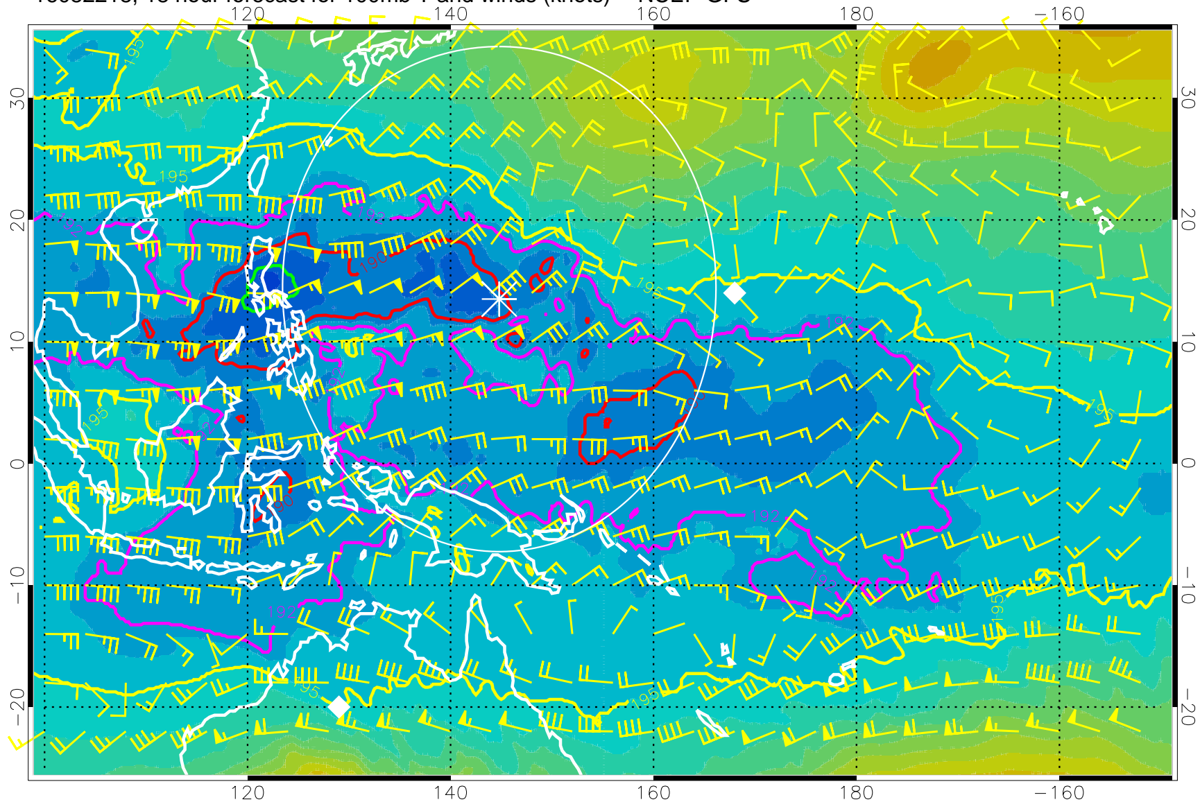
16082218, 18 hour forecast for 100mb T and winds (knots) -- NCEP GFS
