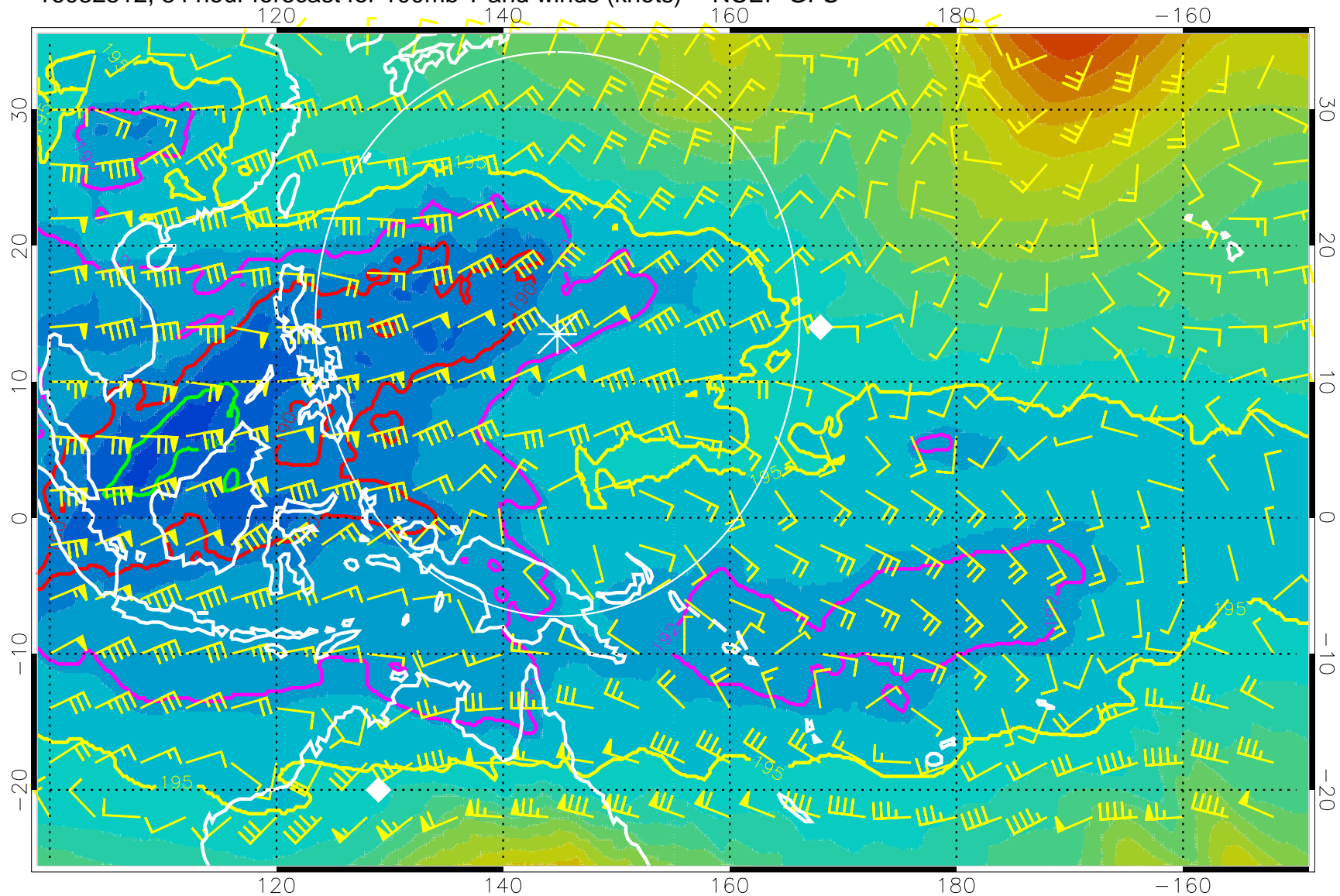
16082512, 84 hour forecast for 100mb T and winds (knots) -- NCEP GFS
