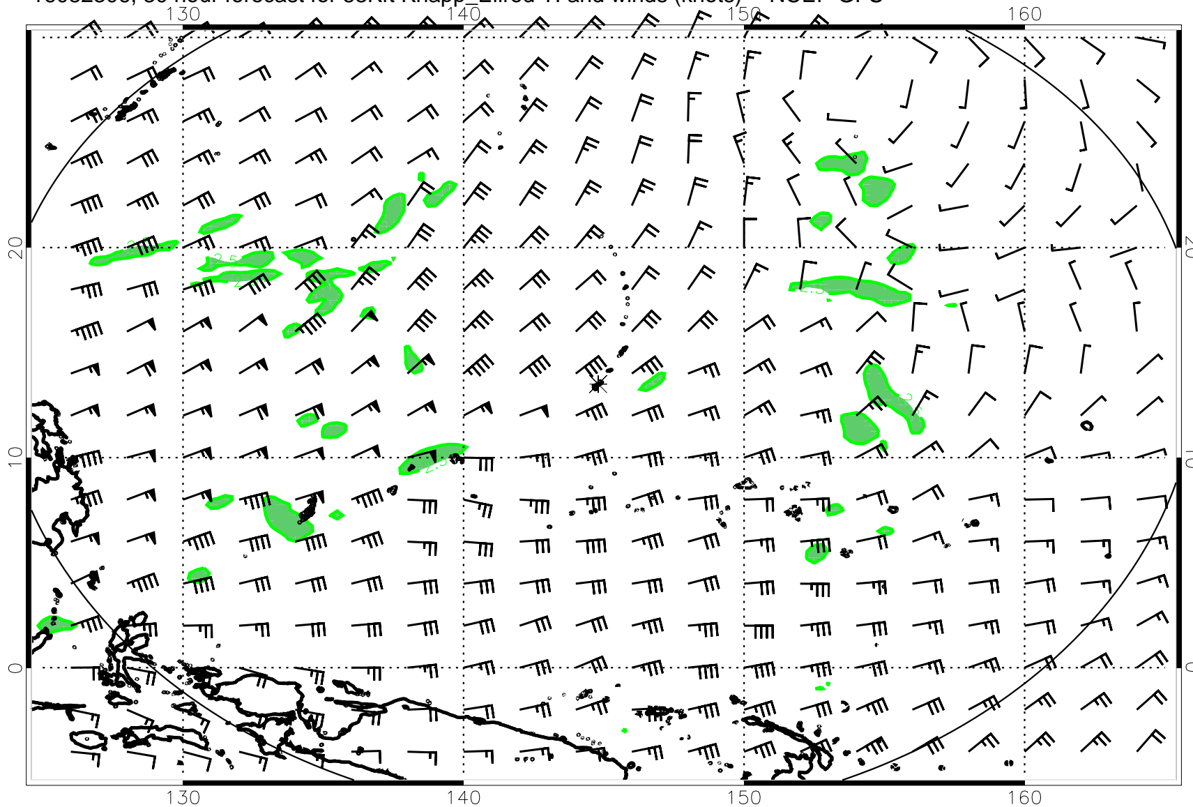
16082306, 30 hour forecast for 53Kft Knapp_Ellrod TI and winds (knots) -- NCEP GFS
