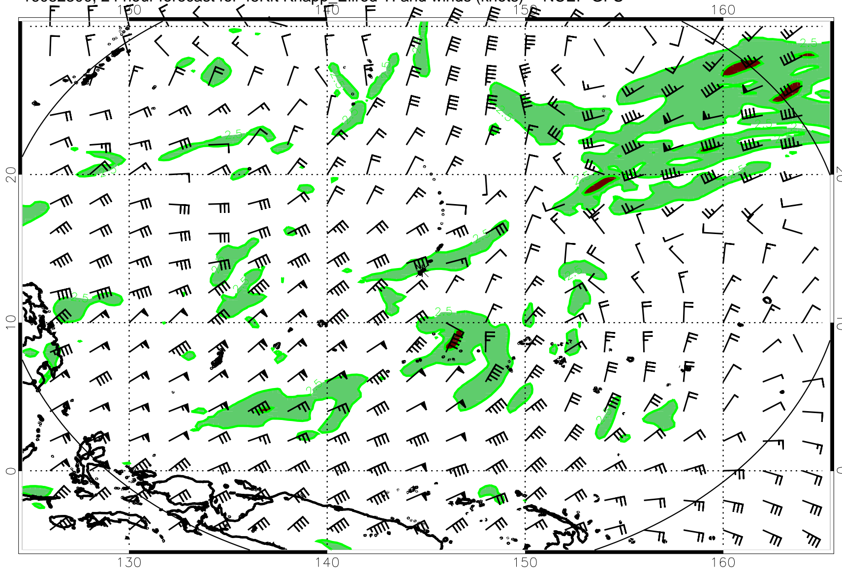
16082300, 24 hour forecast for 45Kft Knapp_Ellrod TI and winds (knots) -- NCEP GFS
