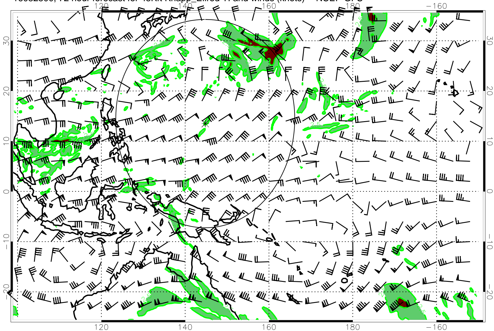
16082500, 72 hour forecast for 45Kft Knapp_Ellrod TI and winds (knots) -- NCEP GFS
