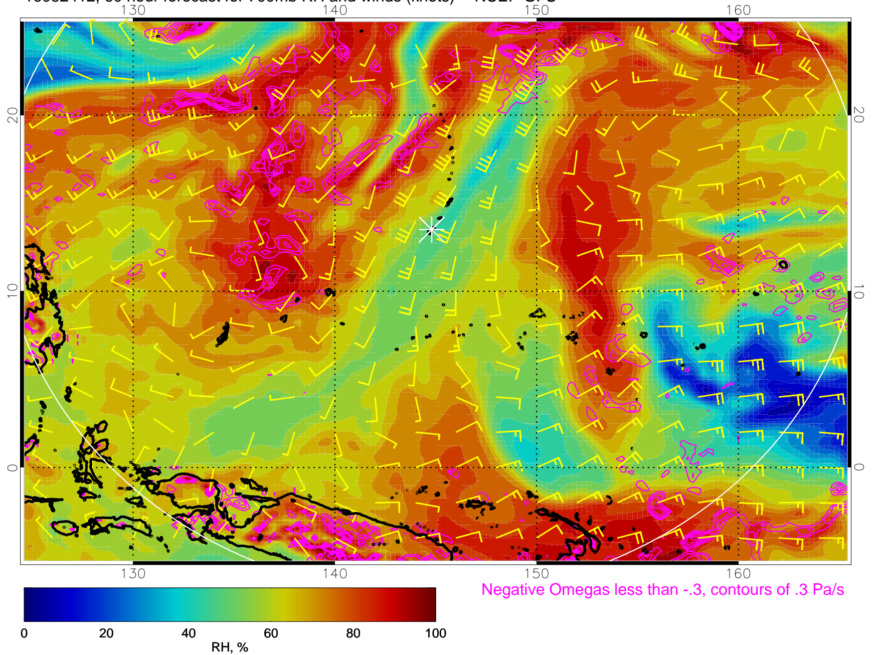
16082412, 60 hour forecast for 700mb RH and winds (knots) -- NCEP GFS
