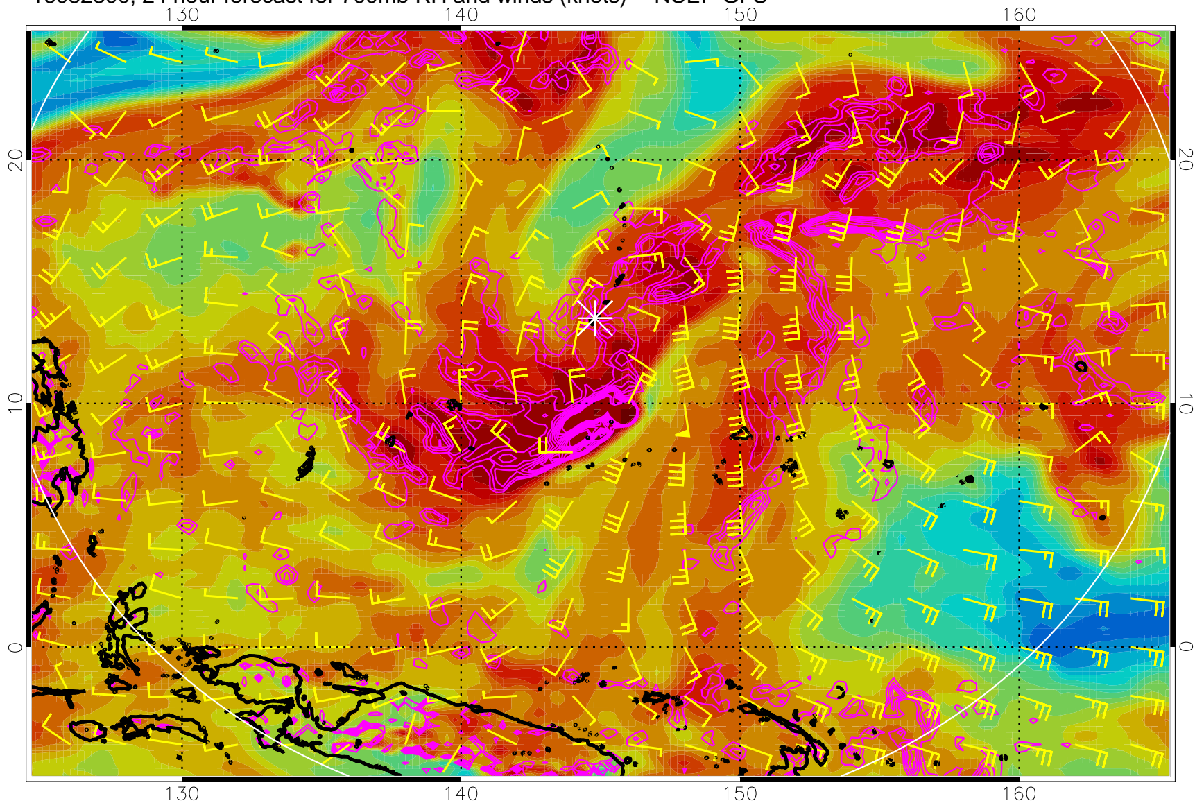
16082300, 24 hour forecast for 700mb RH and winds (knots) -- NCEP GFS
