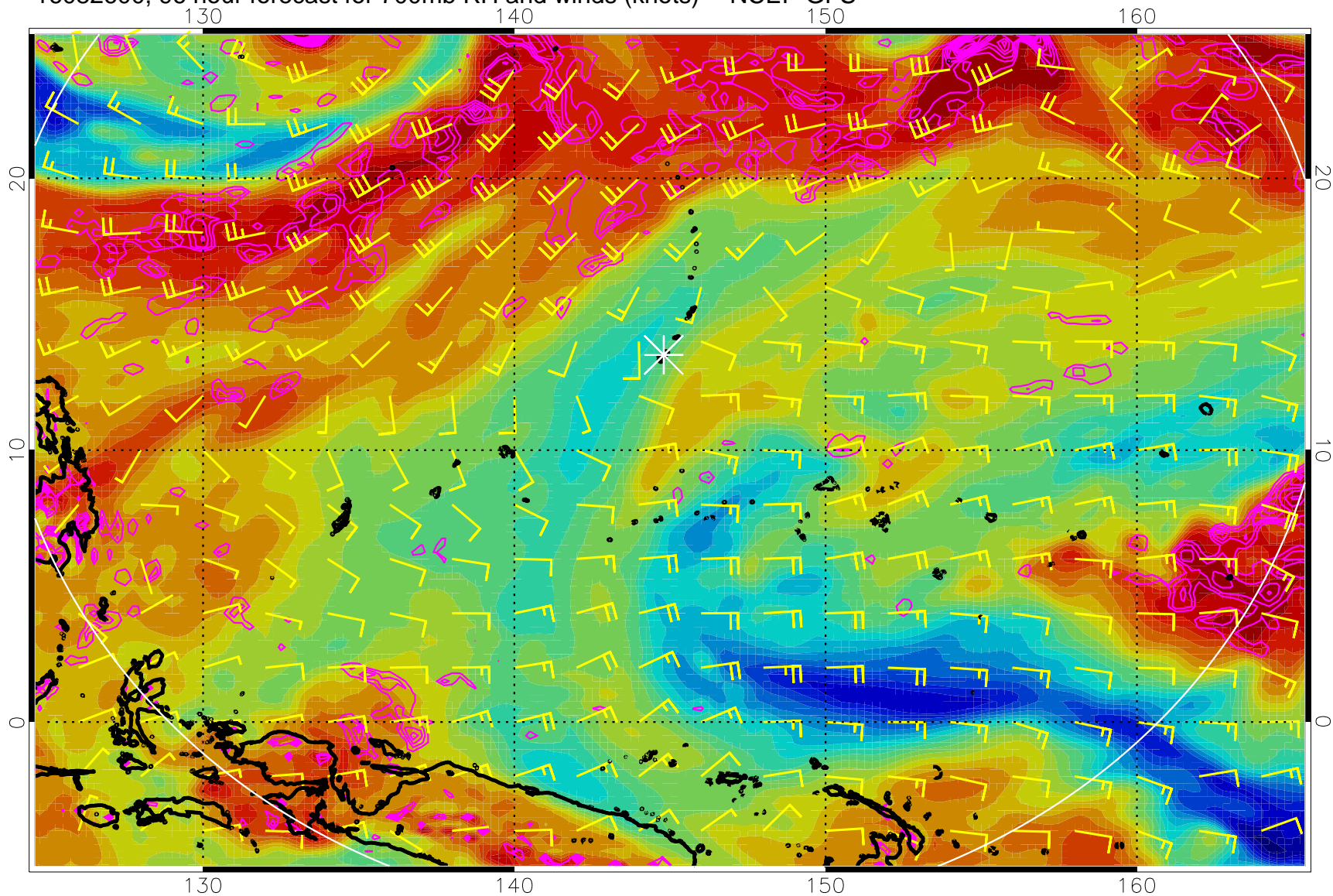
16082600, 96 hour forecast for 700mb RH and winds (knots) -- NCEP GFS
