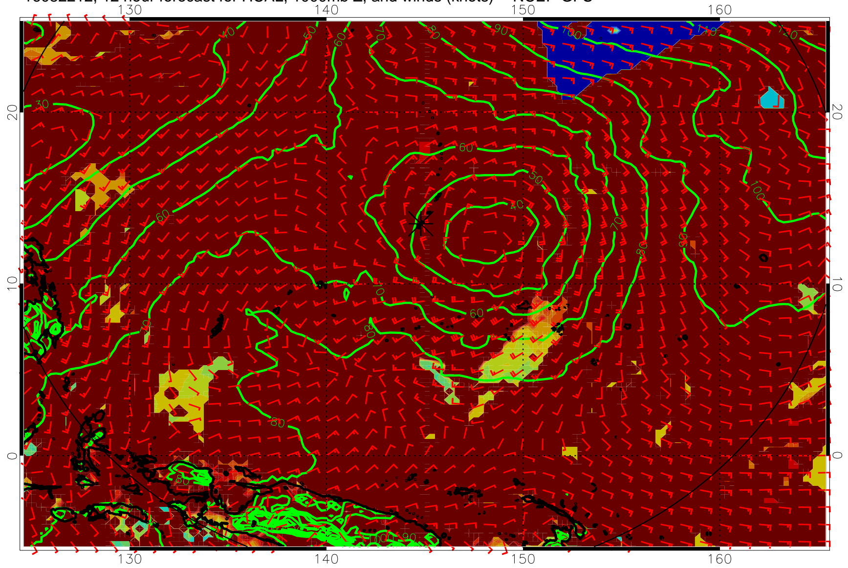
16082212, 12 hour forecast for HCAL, 1000mb Z, and winds (knots) -- NCEP GFS
