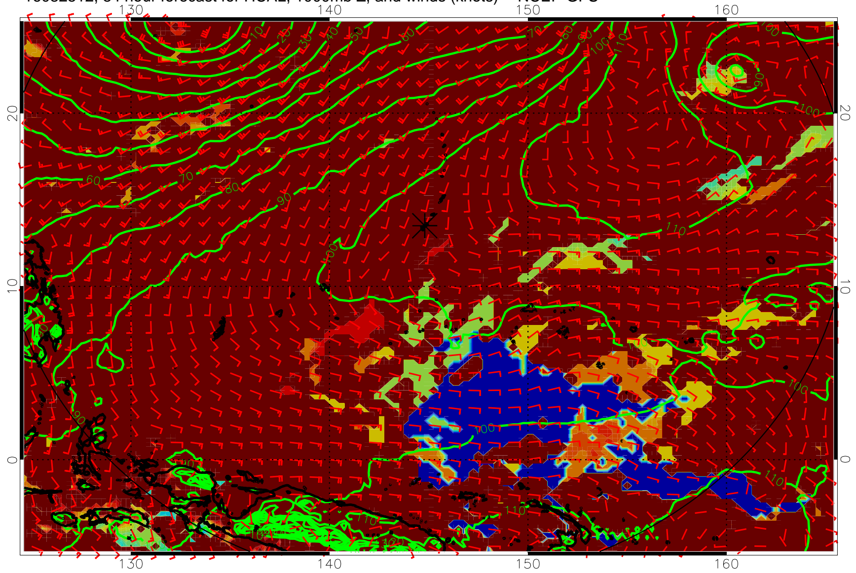
16082512, 84 hour forecast for HCAL, 1000mb Z, and winds (knots) -- NCEP GFS
