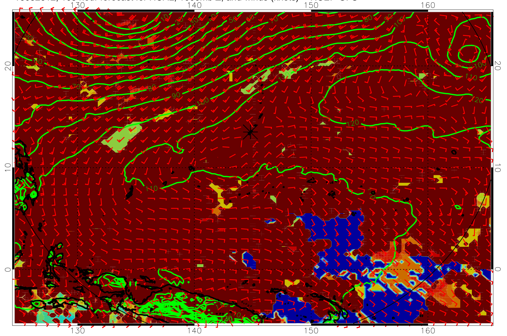
16082612, 108 hour forecast for HCAL, 1000mb Z, and winds (knots) -- NCEP GFS
