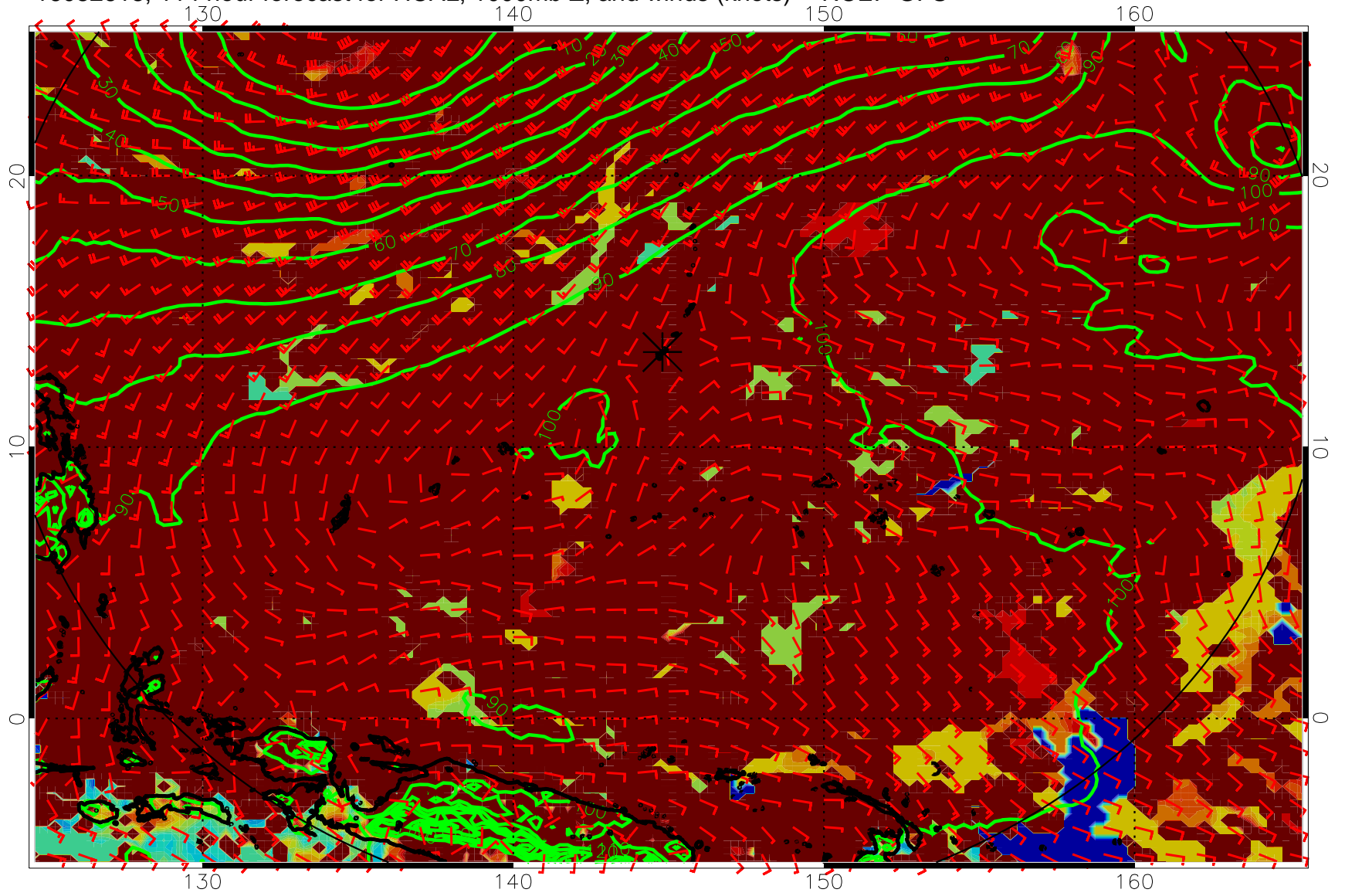
16082618, 114 hour forecast for HCAL, 1000mb Z, and winds (knots) -- NCEP GFS
