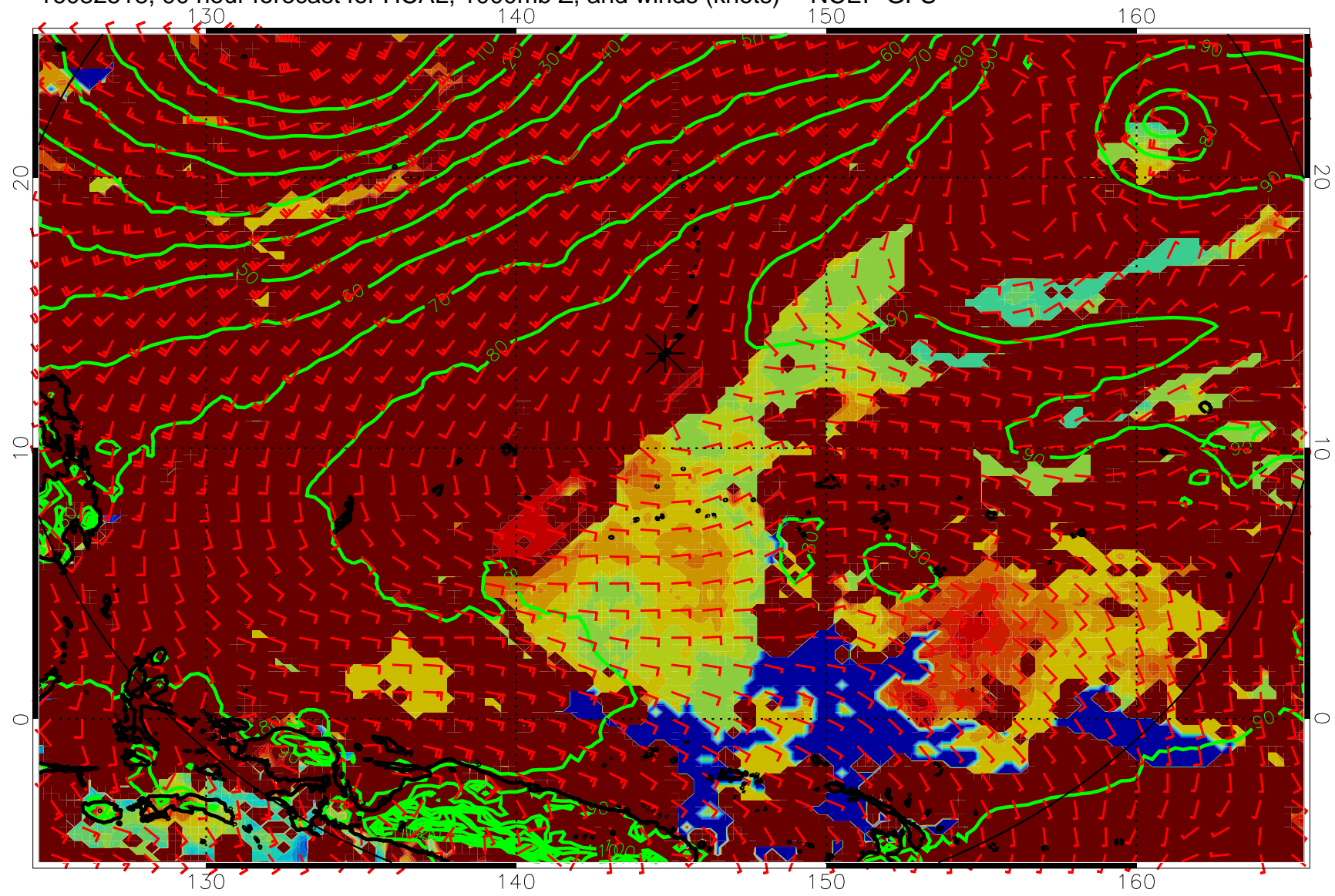
16082518, 90 hour forecast for HCAL, 1000mb Z, and winds (knots) -- NCEP GFS
