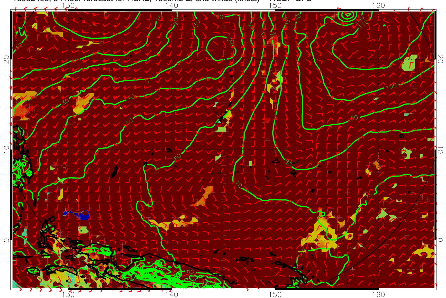
16082406, 54 hour forecast for HCAL, 1000mb Z, and winds (knots) -- NCEP GFS
