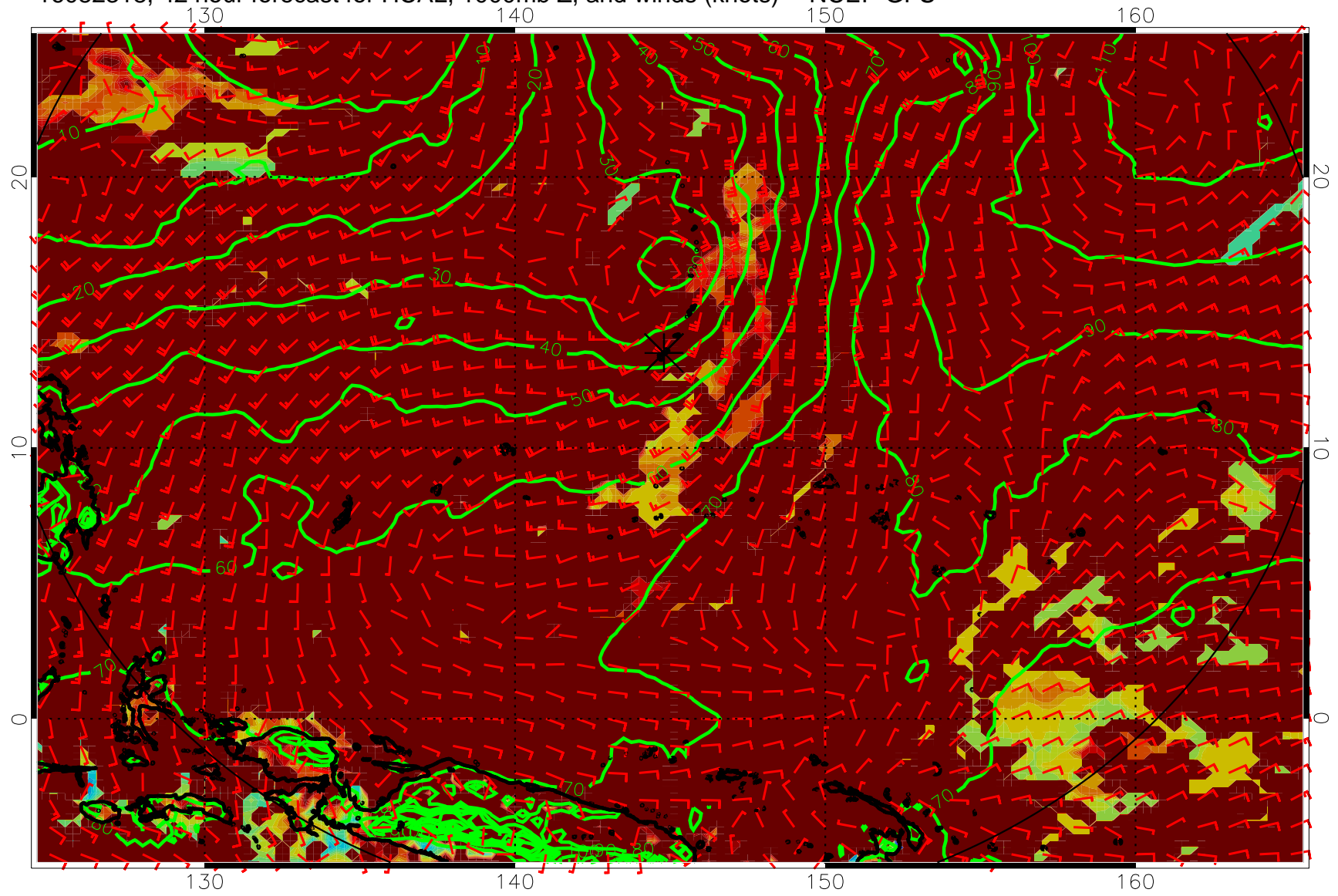
16082318, 42 hour forecast for HCAL, 1000mb Z, and winds (knots) -- NCEP GFS
