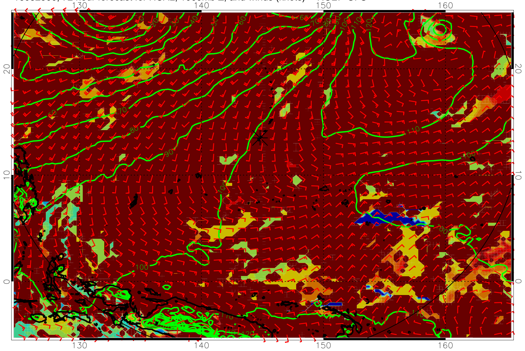
16082500, 72 hour forecast for HCAL, 1000mb Z, and winds (knots) -- NCEP GFS
