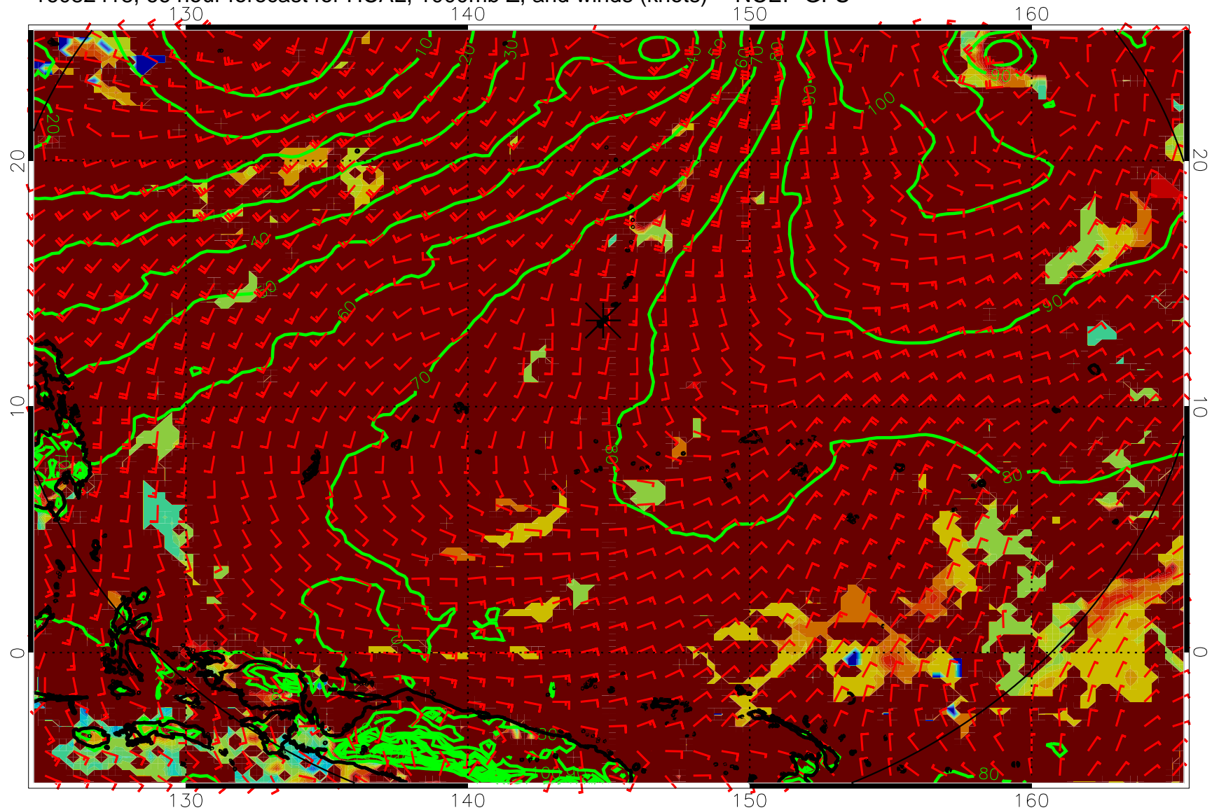
16082418, 66 hour forecast for HCAL, 1000mb Z, and winds (knots) -- NCEP GFS
