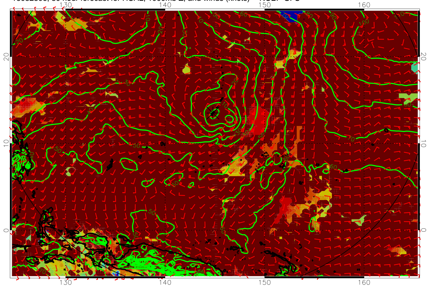
16082306, 30 hour forecast for HCAL, 1000mb Z, and winds (knots) -- NCEP GFS
