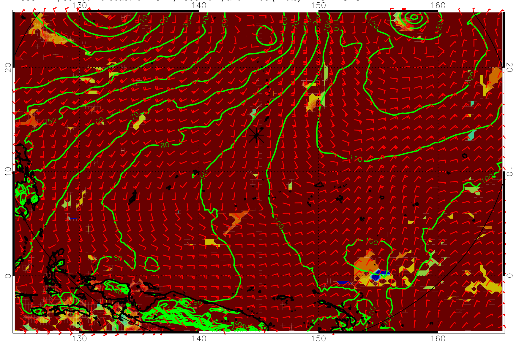
16082412, 60 hour forecast for HCAL, 1000mb Z, and winds (knots) -- NCEP GFS
