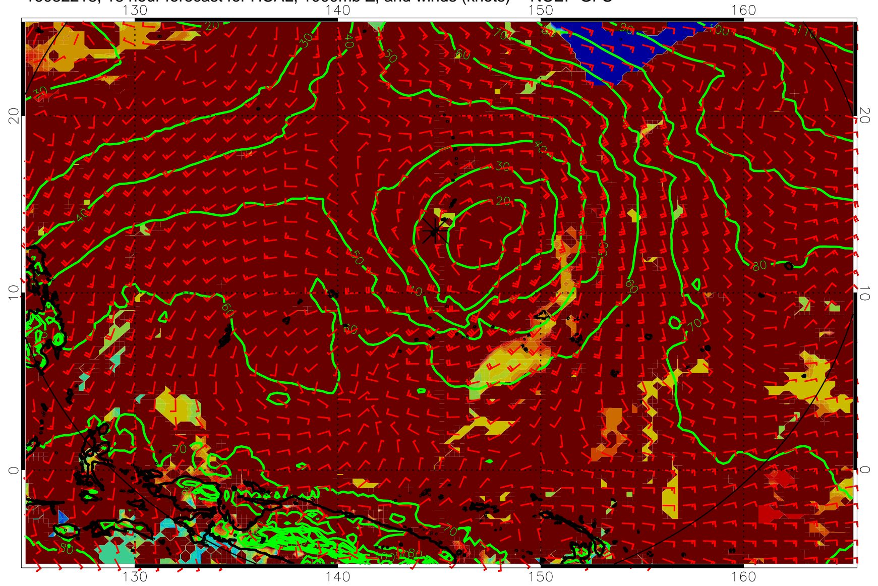
16082218, 18 hour forecast for HCAL, 1000mb Z, and winds (knots) -- NCEP GFS
