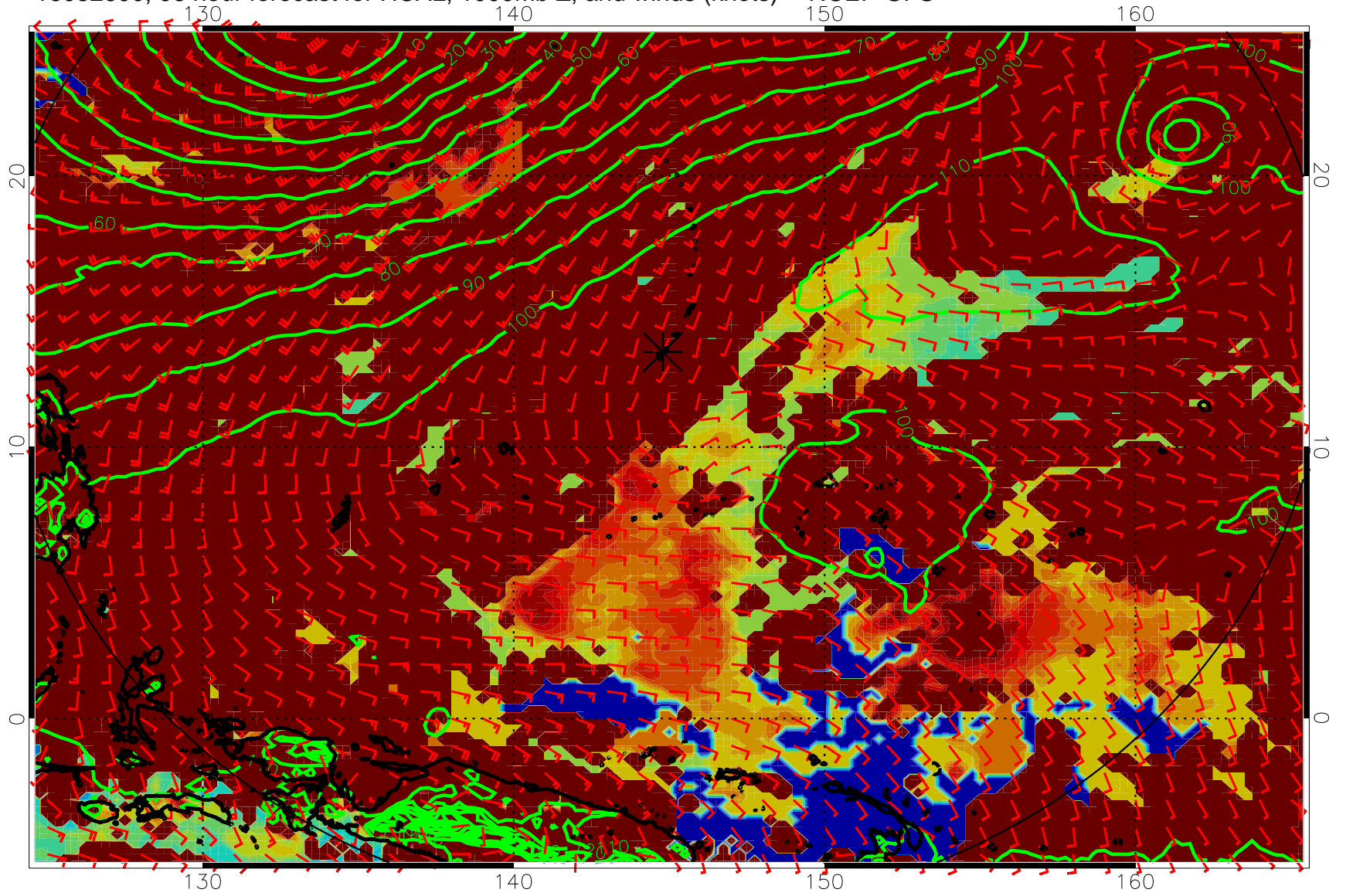
16082600, 96 hour forecast for HCAL, 1000mb Z, and winds (knots) -- NCEP GFS
