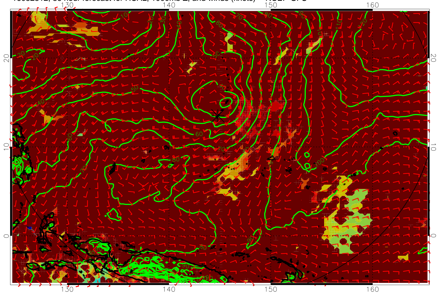
16082312, 36 hour forecast for HCAL, 1000mb Z, and winds (knots) -- NCEP GFS
