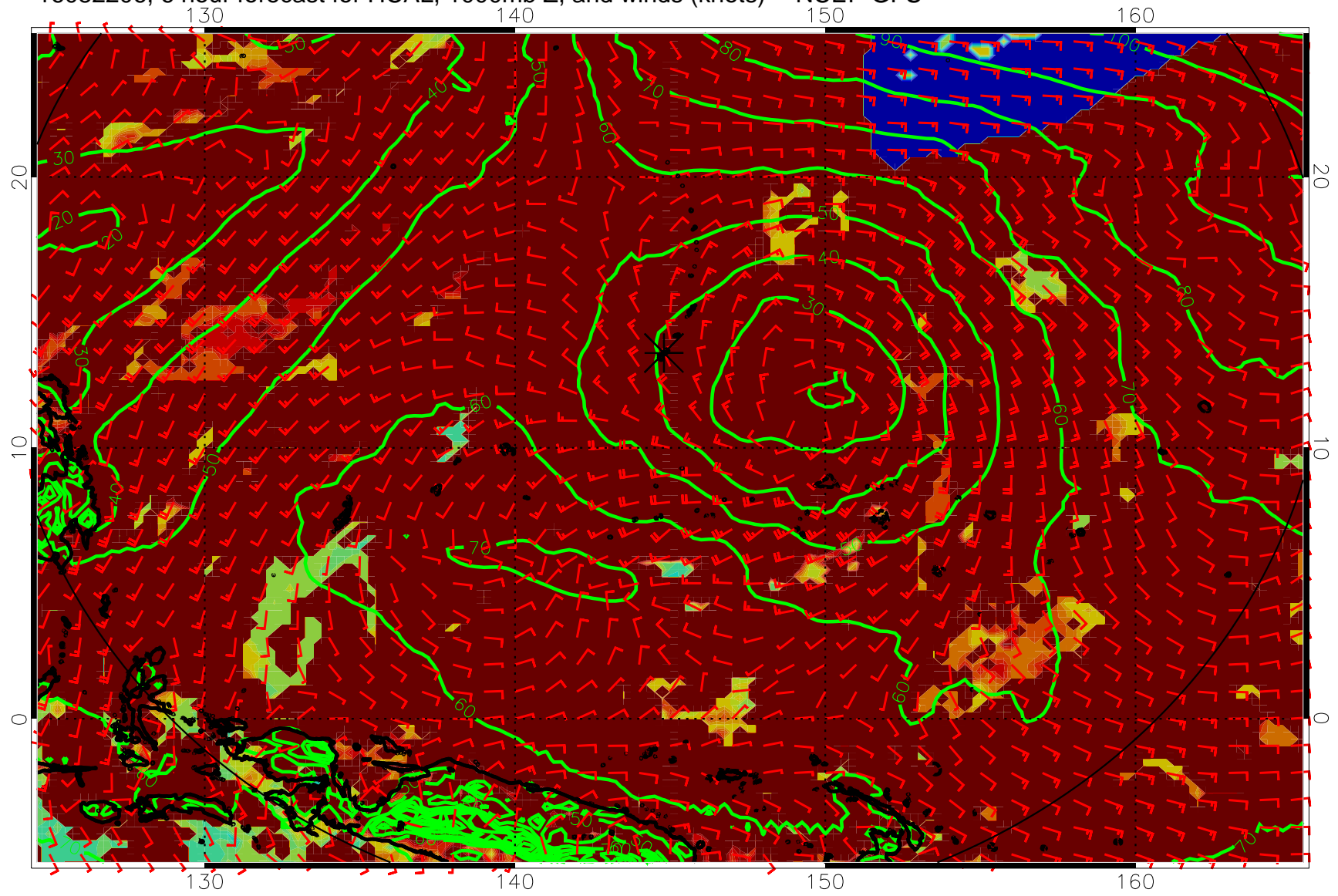
16082206, 6 hour forecast for HCAL, 1000mb Z, and winds (knots) -- NCEP GFS
