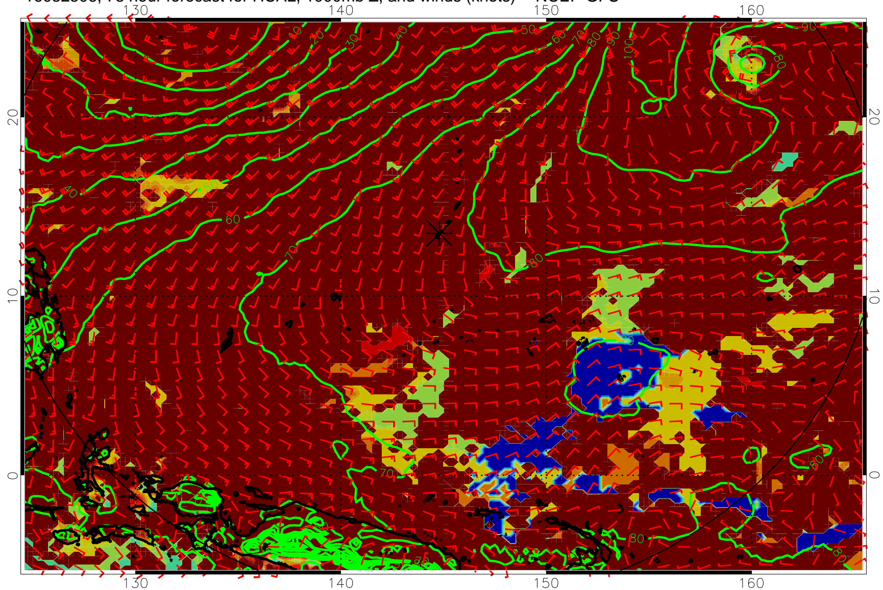
16082506, 78 hour forecast for HCAL, 1000mb Z, and winds (knots) -- NCEP GFS
