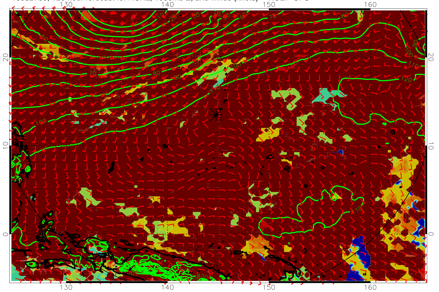
16082700, 120 hour forecast for HCAL, 1000mb Z, and winds (knots) -- NCEP GFS
