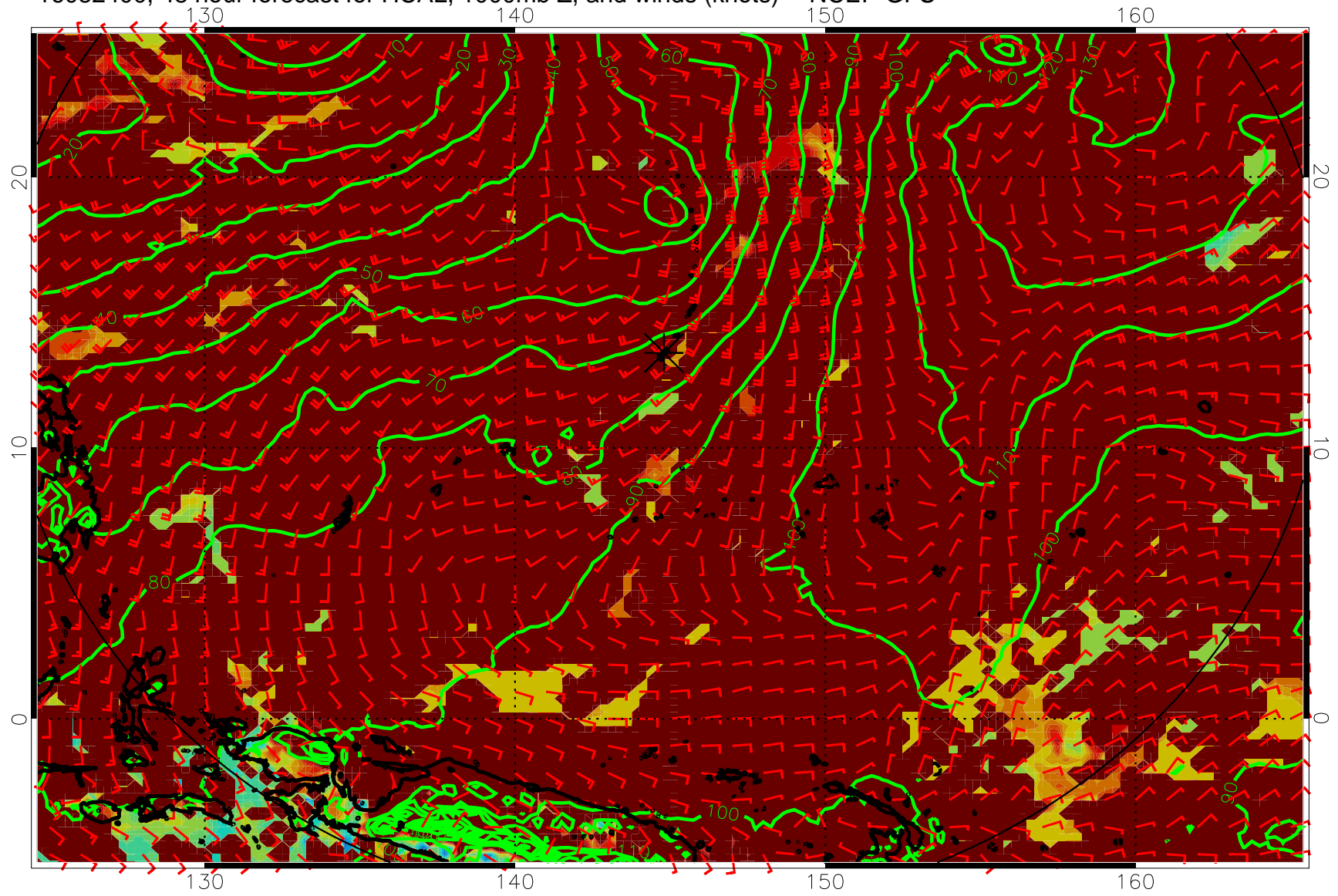
16082400, 48 hour forecast for HCAL, 1000mb Z, and winds (knots) -- NCEP GFS
