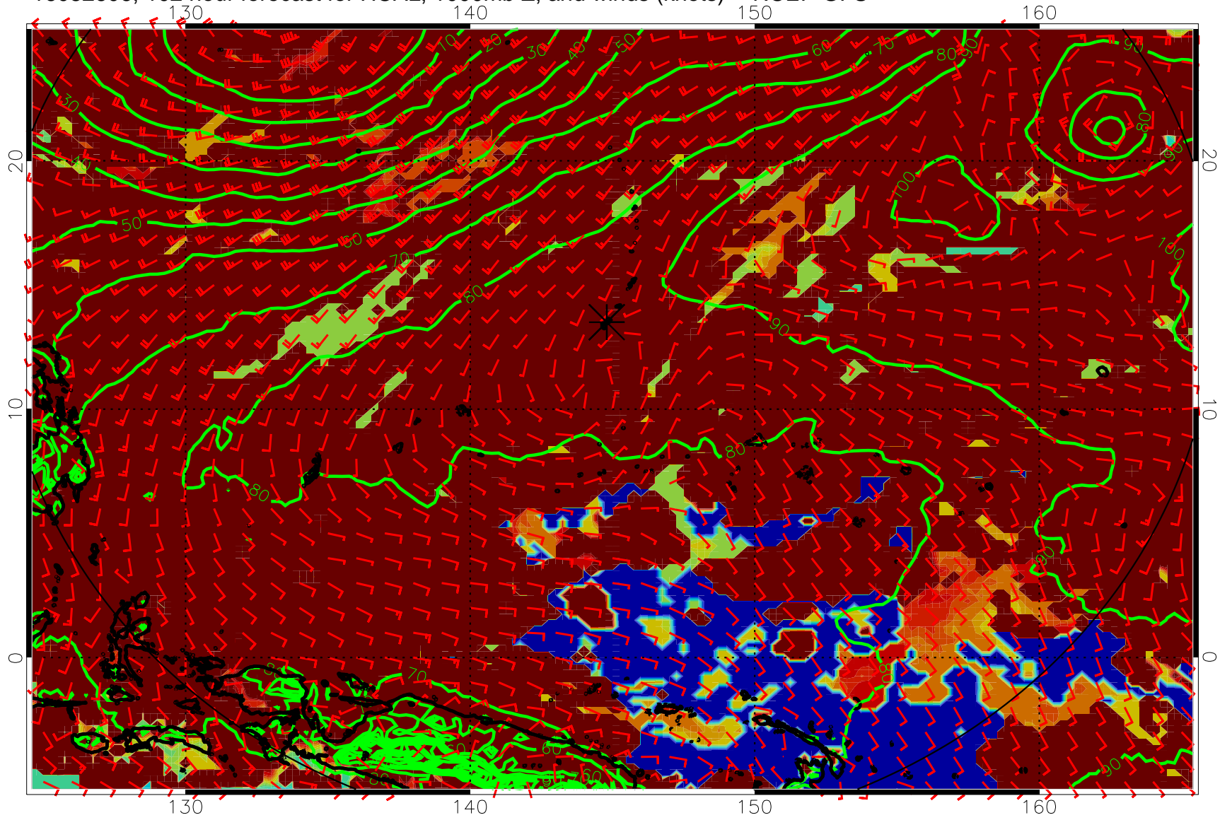
16082606, 102 hour forecast for HCAL, 1000mb Z, and winds (knots) -- NCEP GFS
