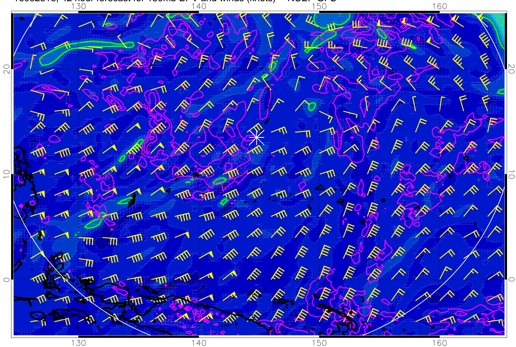
16082318, 42 hour forecast for 150mb EPV and winds (knots) -- NCEP GFS
