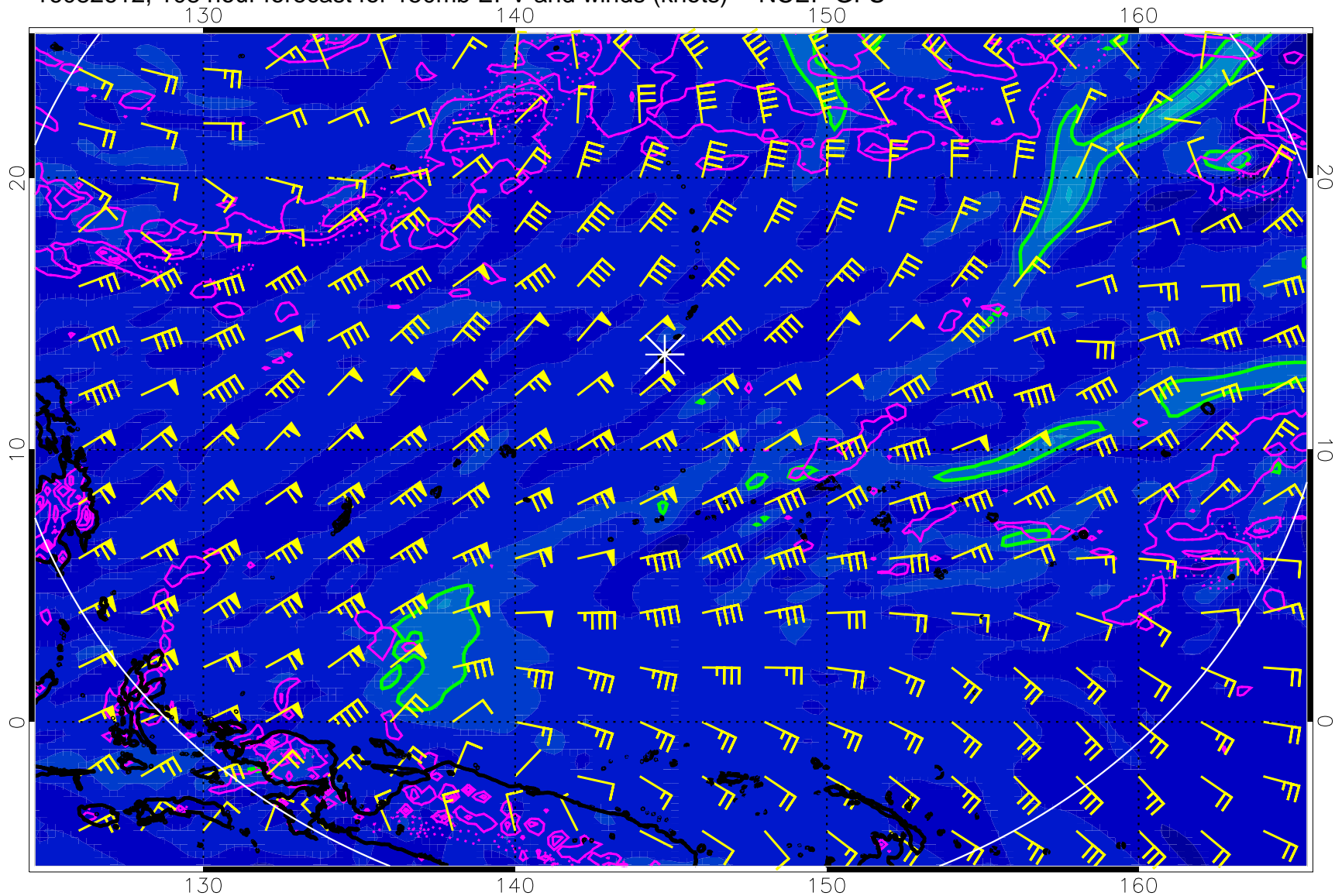
16082612, 108 hour forecast for 150mb EPV and winds (knots) -- NCEP GFS
