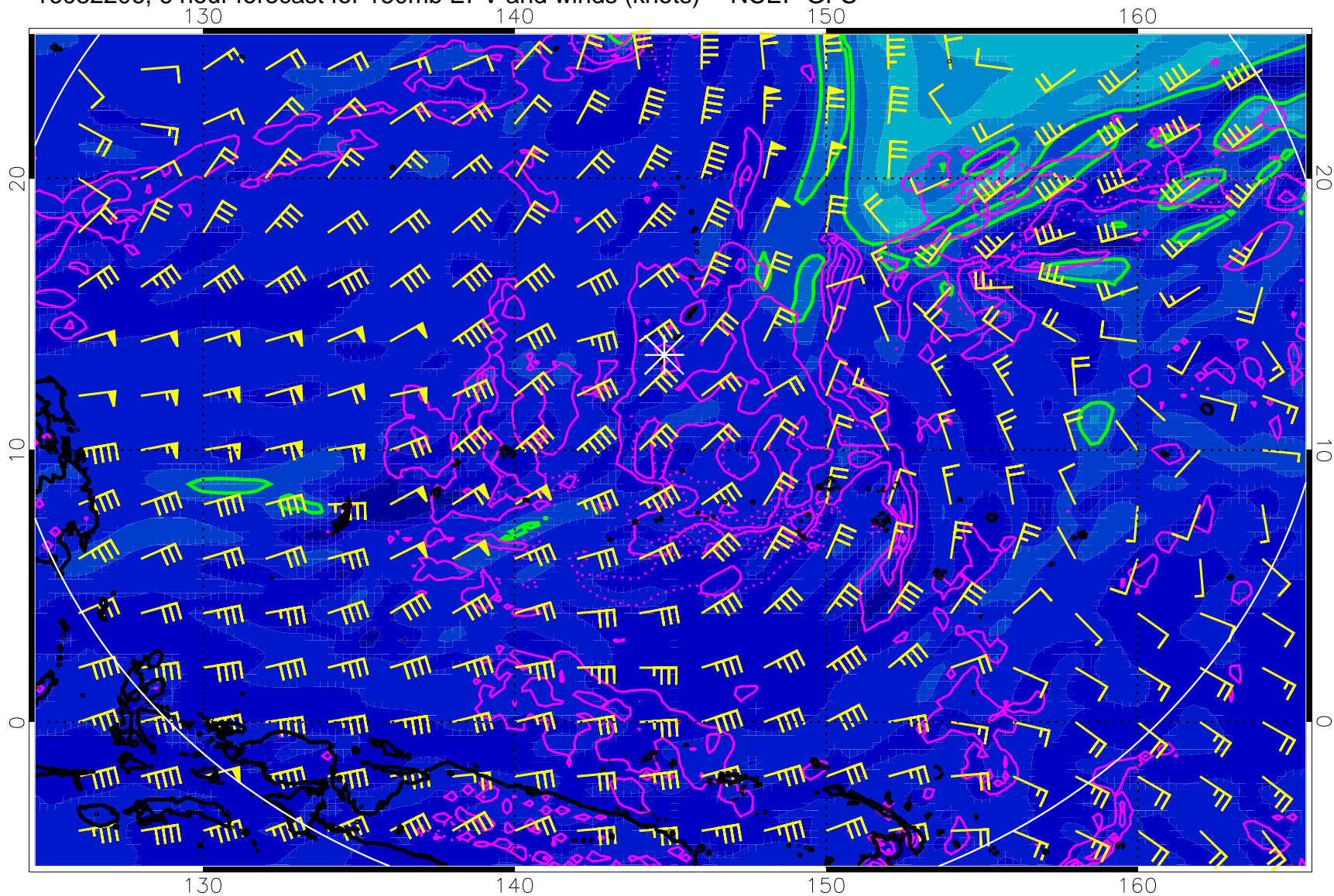
16082206, 6 hour forecast for 150mb EPV and winds (knots) -- NCEP GFS
