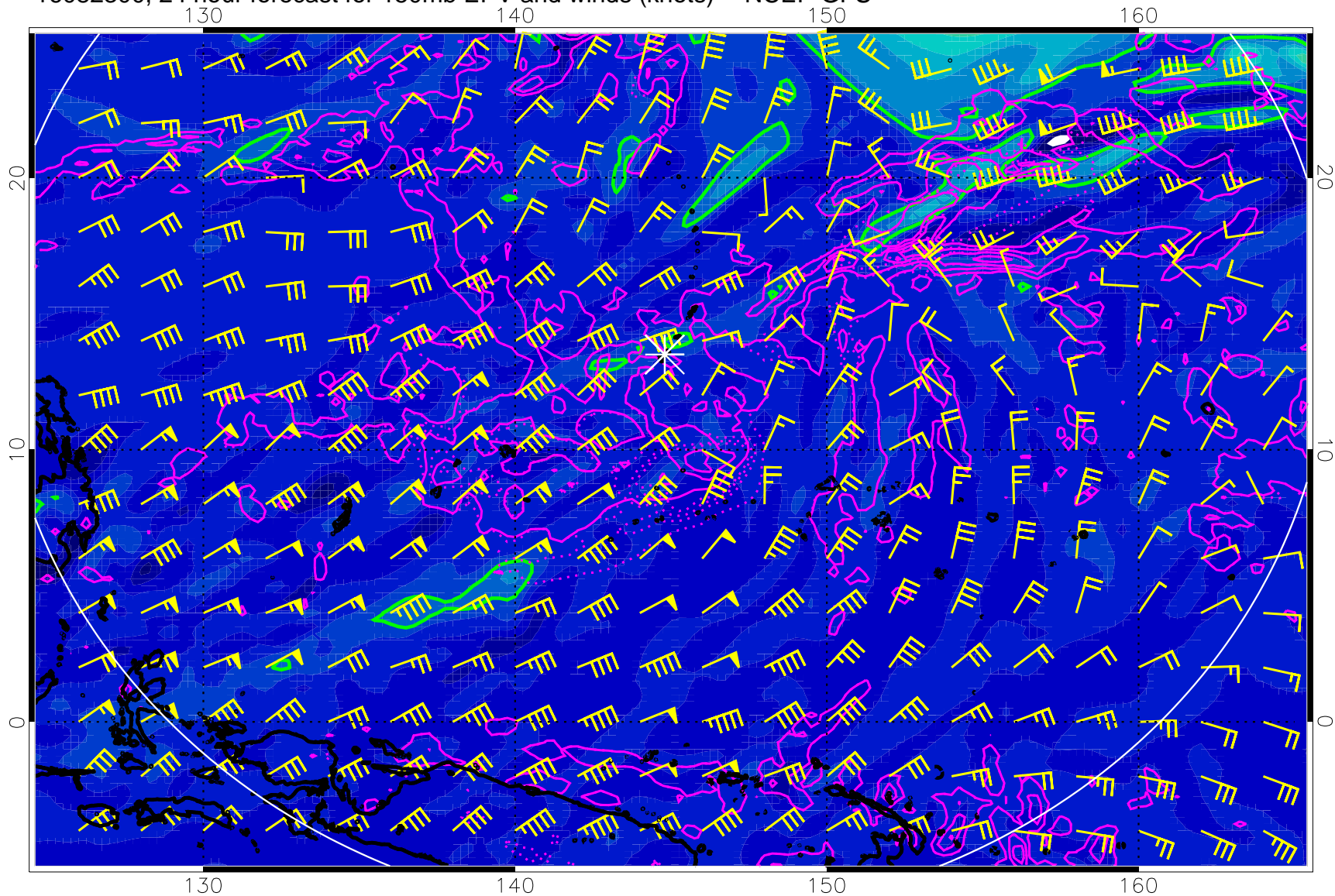
16082300, 24 hour forecast for 150mb EPV and winds (knots) -- NCEP GFS
