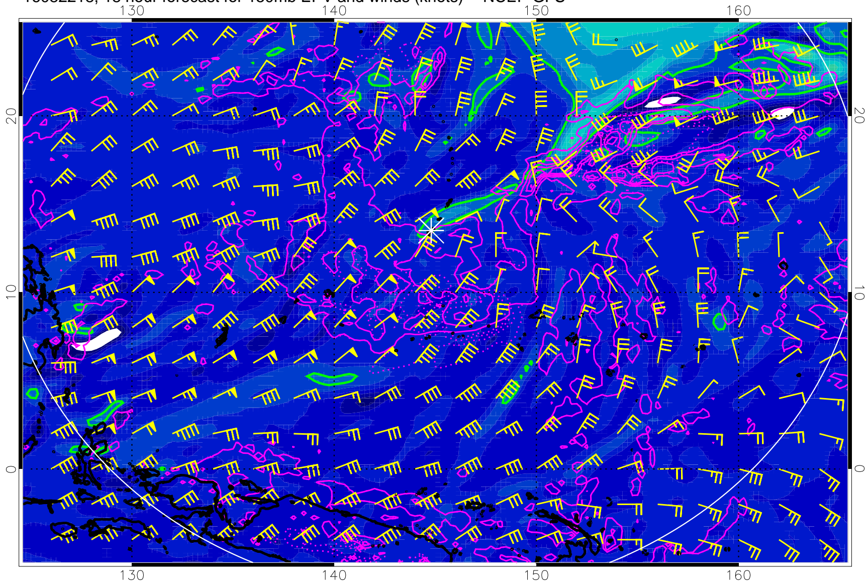
16082218, 18 hour forecast for 150mb EPV and winds (knots) -- NCEP GFS
