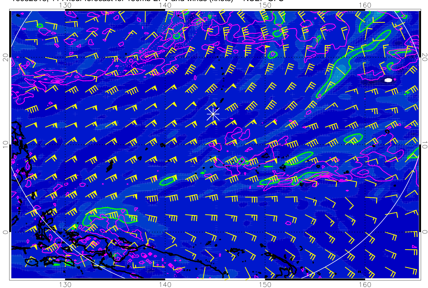
16082618, 114 hour forecast for 150mb EPV and winds (knots) -- NCEP GFS
