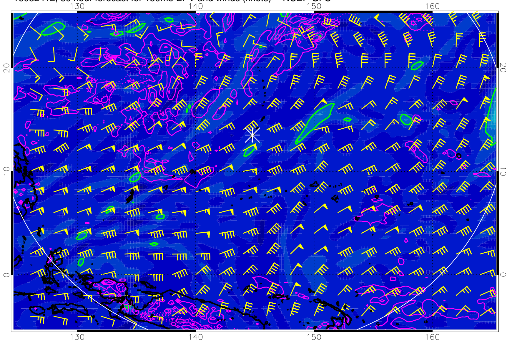
16082412, 60 hour forecast for 150mb EPV and winds (knots) -- NCEP GFS
