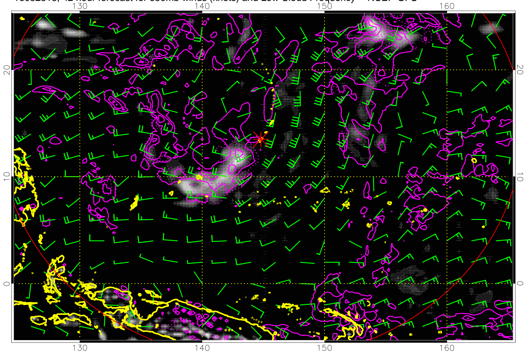
16082318, 42 hour forecast for 850mb winds (knots) and Low Cloud Frequency -- NCEP GFS
