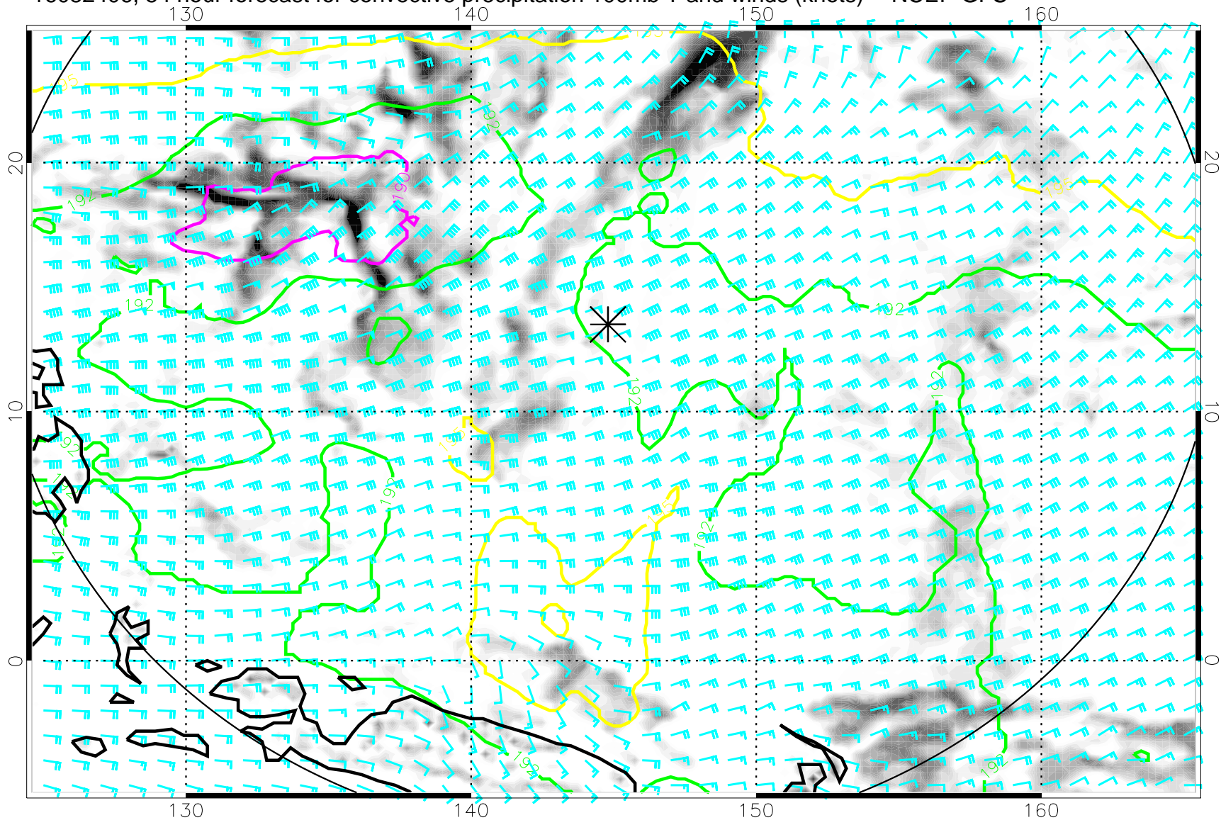
16082406, 54 hour forecast for convective precipitation 100mb T and winds (knots) -- NCEP GFS
