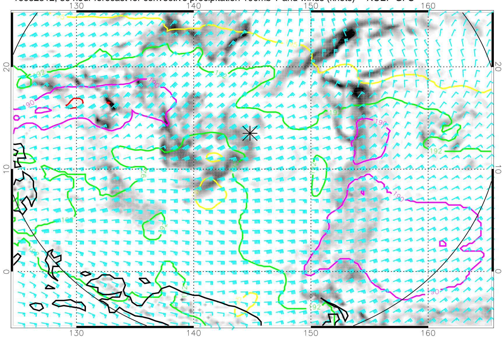
16082312, 36 hour forecast for convective precipitation 100mb T and winds (knots) -- NCEP GFS
