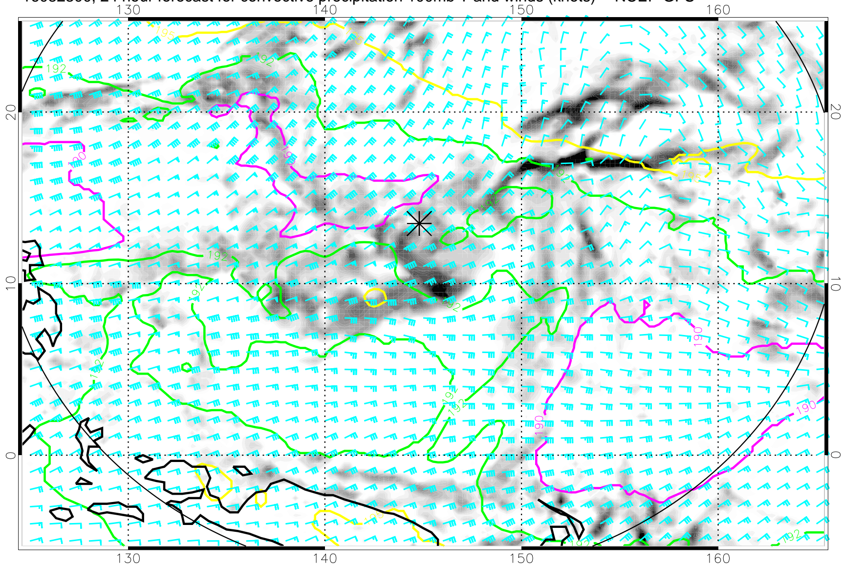
16082300, 24 hour forecast for convective precipitation 100mb T and winds (knots) -- NCEP GFS
