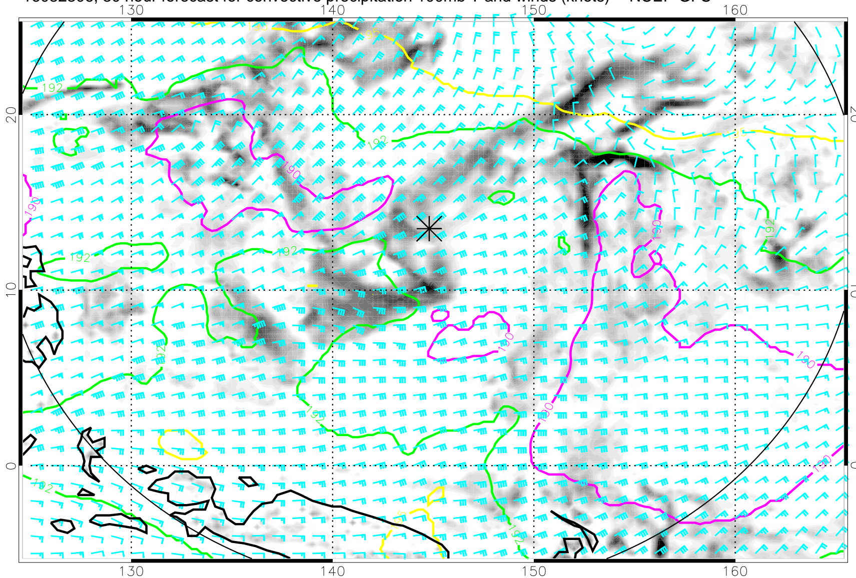
16082306, 30 hour forecast for convective precipitation 100mb T and winds (knots) -- NCEP GFS
