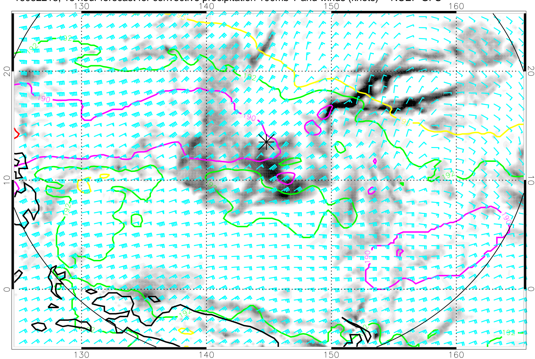
16082218, 18 hour forecast for convective precipitation 100mb T and winds (knots) -- NCEP GFS
