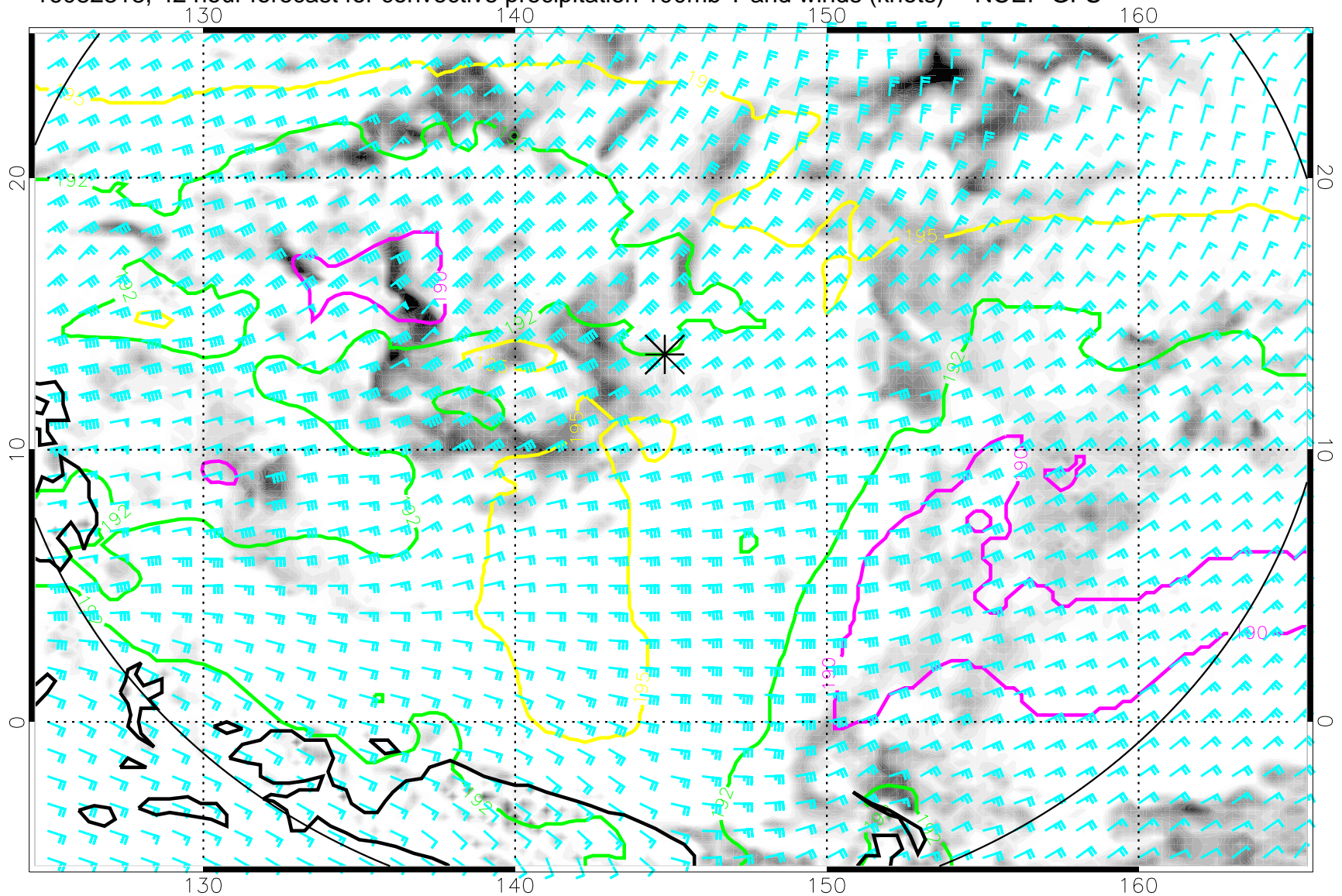
16082318, 42 hour forecast for convective precipitation 100mb T and winds (knots) -- NCEP GFS
