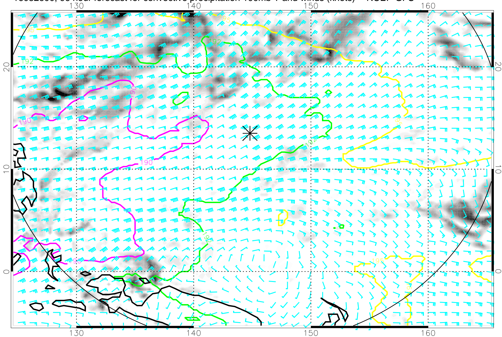
16082600, 96 hour forecast for convective precipitation 100mb T and winds (knots) -- NCEP GFS
