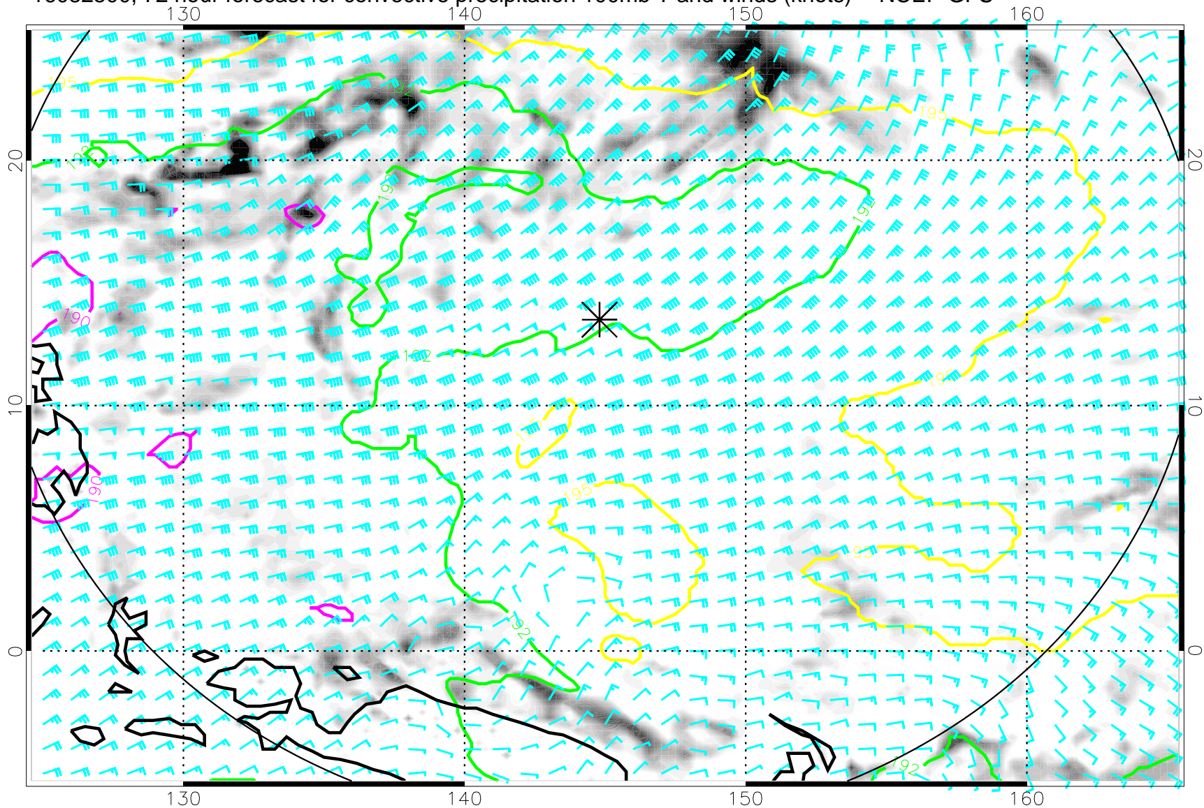
16082500, 72 hour forecast for convective precipitation 100mb T and winds (knots) -- NCEP GFS
