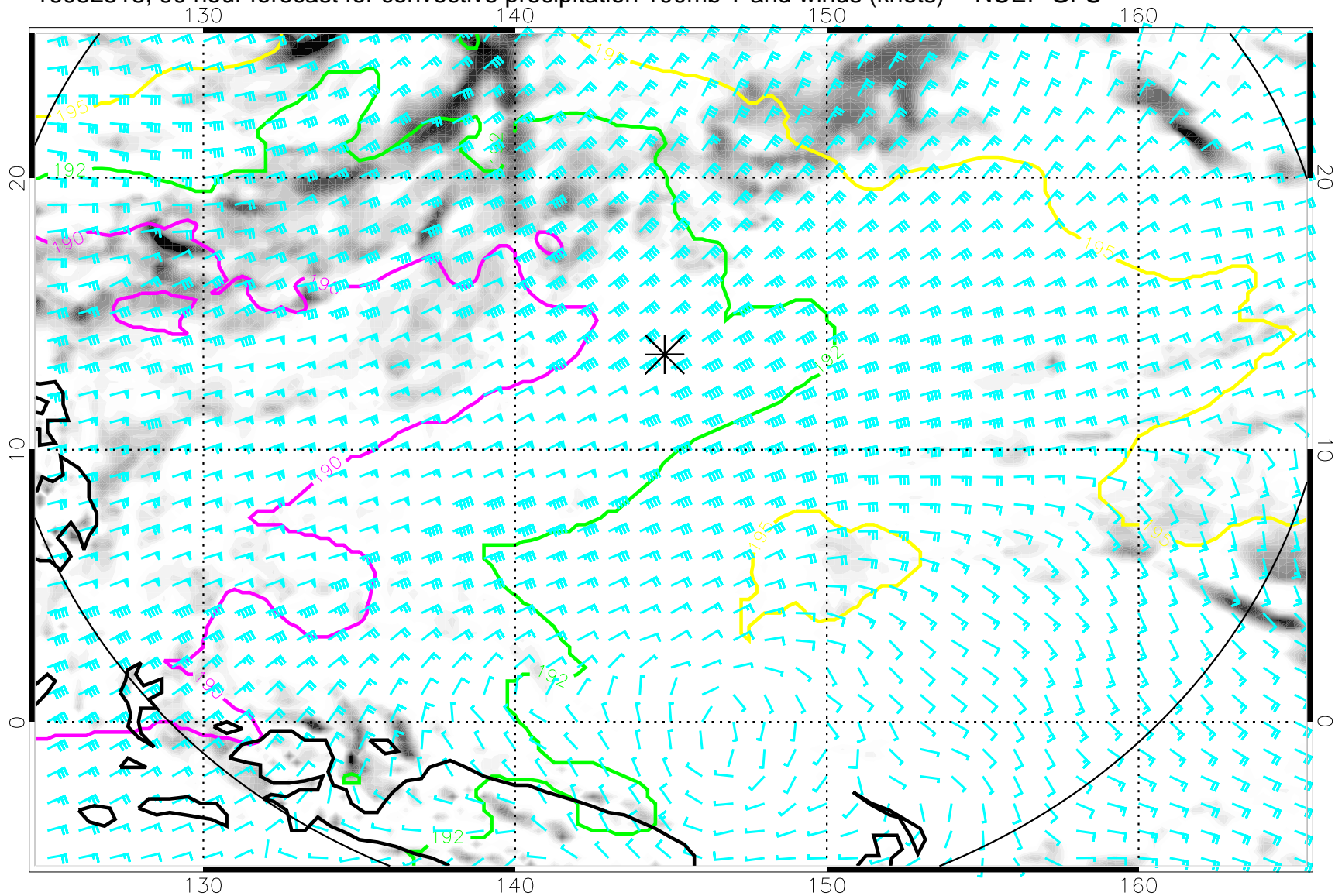
16082518, 90 hour forecast for convective precipitation 100mb T and winds (knots) -- NCEP GFS
