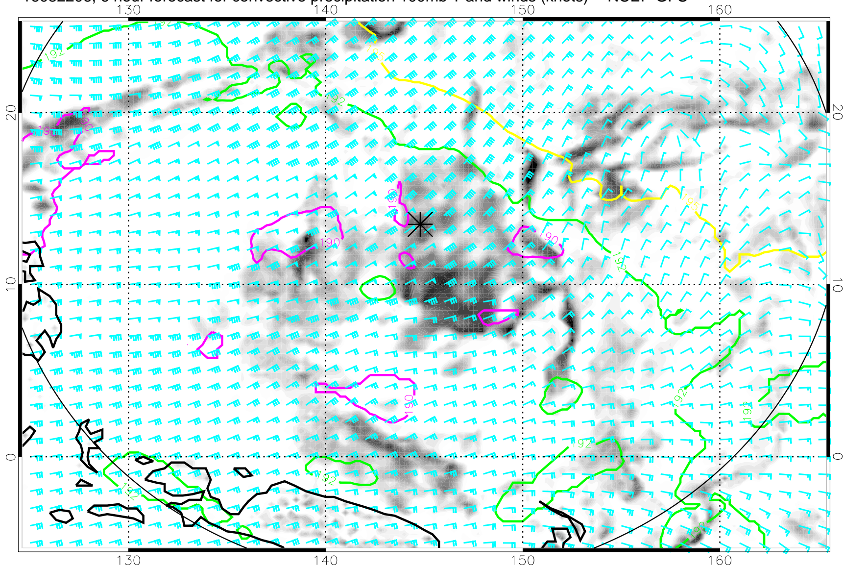
16082206, 6 hour forecast for convective precipitation 100mb T and winds (knots) -- NCEP GFS
