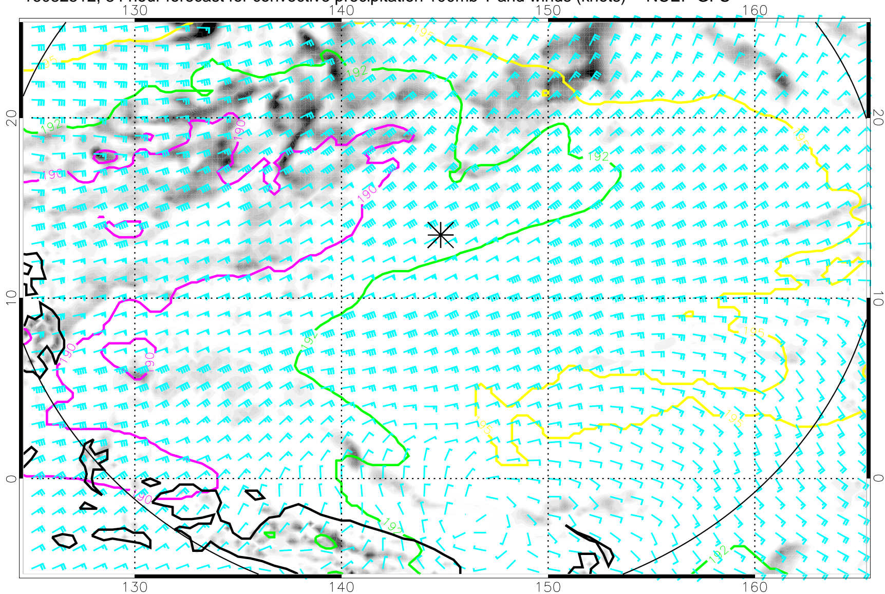
16082512, 84 hour forecast for convective precipitation 100mb T and winds (knots) -- NCEP GFS
