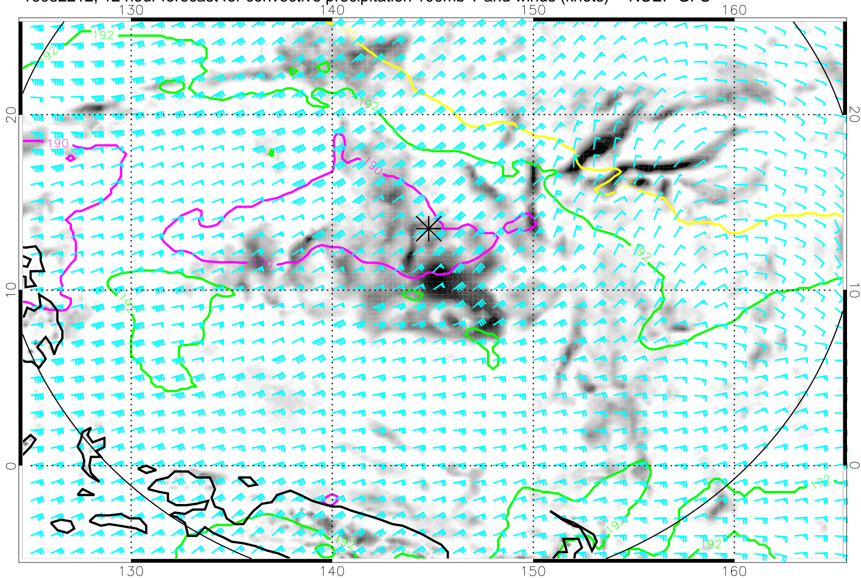
16082212, 12 hour forecast for convective precipitation 100mb T and winds (knots) -- NCEP GFS
