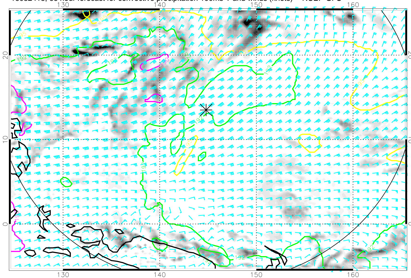
16082418, 66 hour forecast for convective precipitation 100mb T and winds (knots) -- NCEP GFS
