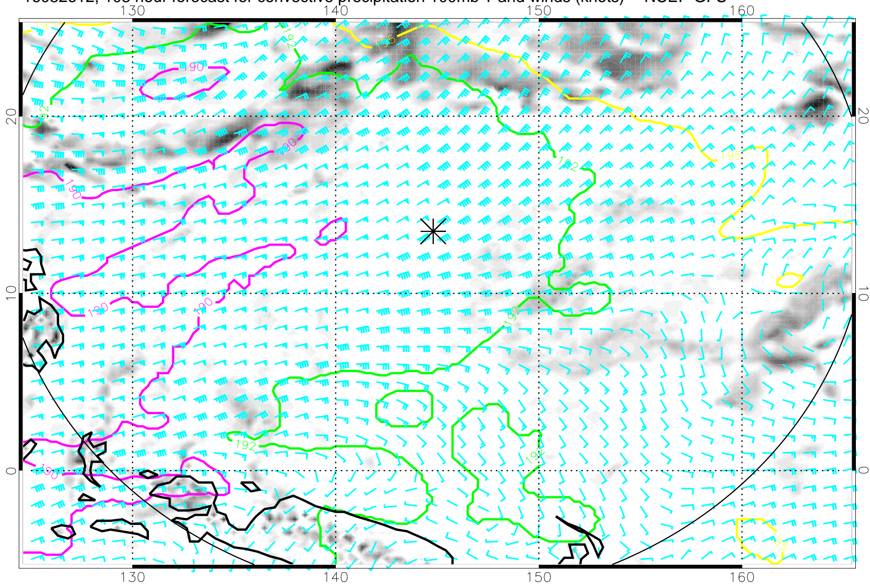
16082612, 108 hour forecast for convective precipitation 100mb T and winds (knots) -- NCEP GFS
