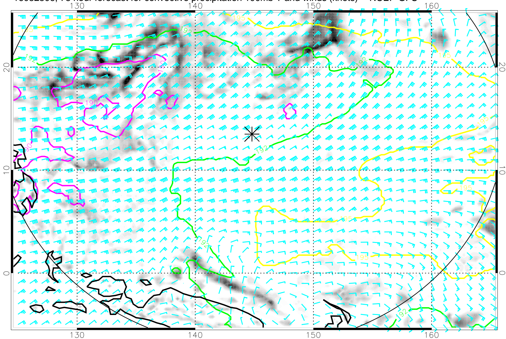
16082506, 78 hour forecast for convective precipitation 100mb T and winds (knots) -- NCEP GFS
