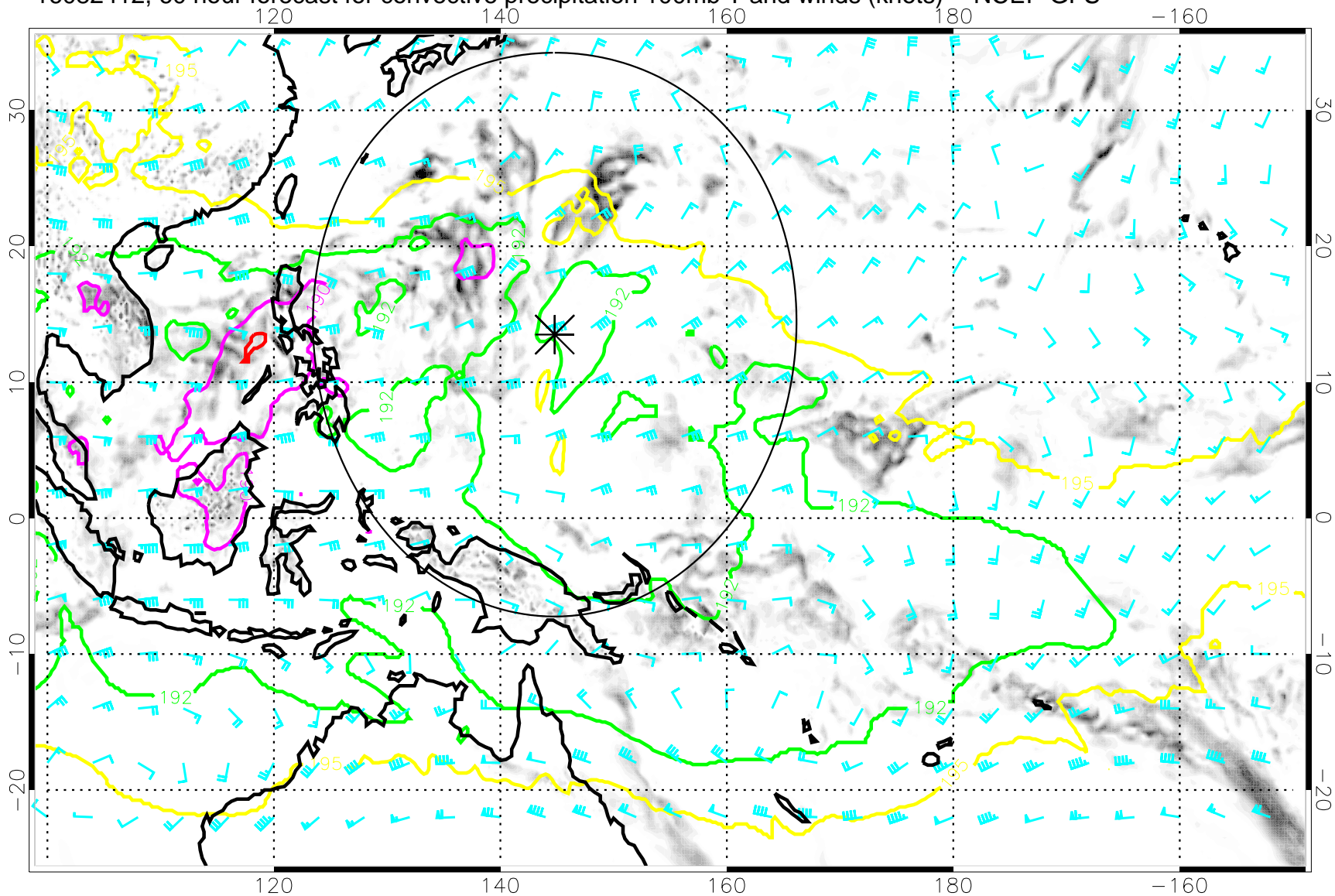
16082412, 60 hour forecast for convective precipitation 100mb T and winds (knots) -- NCEP GFS
