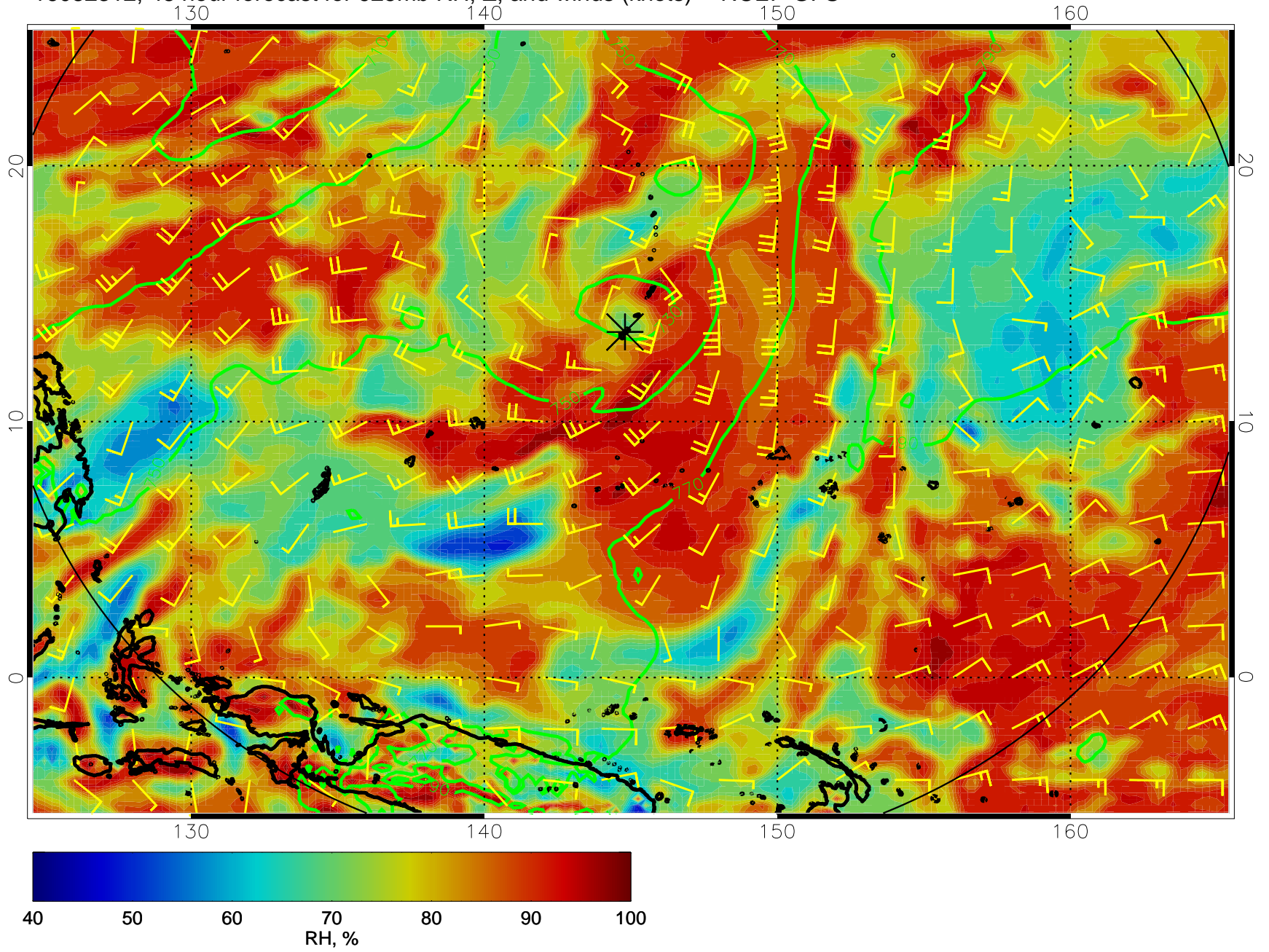
16082312, 48 hour forecast for 925mb RH, Z, and winds (knots) -- NCEP GFS
