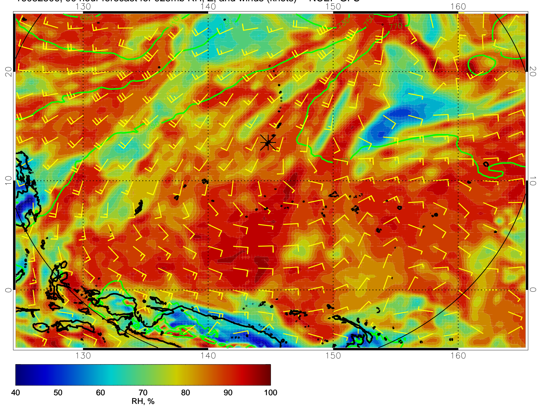
16082506, 90 hour forecast for 925mb RH, Z, and winds (knots) -- NCEP GFS
