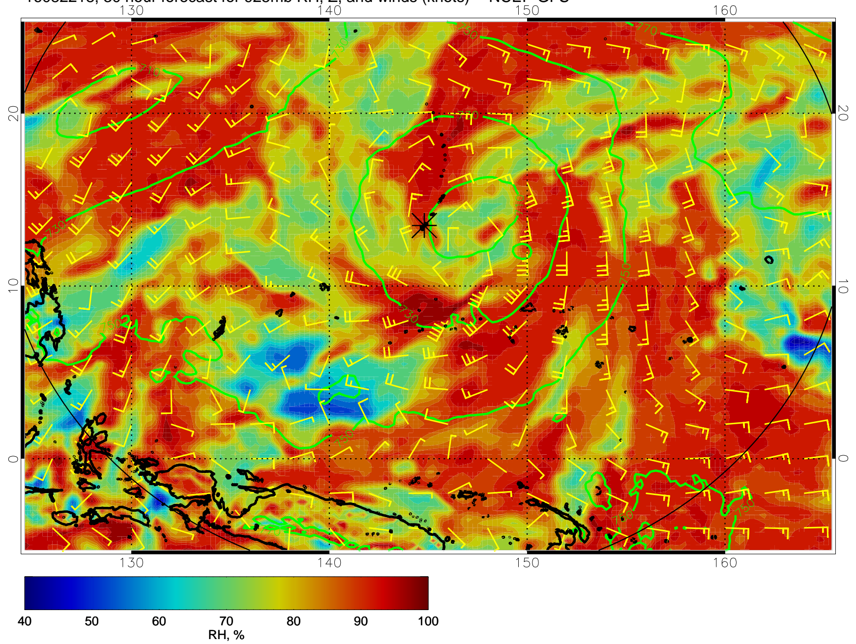
16082218, 30 hour forecast for 925mb RH, Z, and winds (knots) -- NCEP GFS
