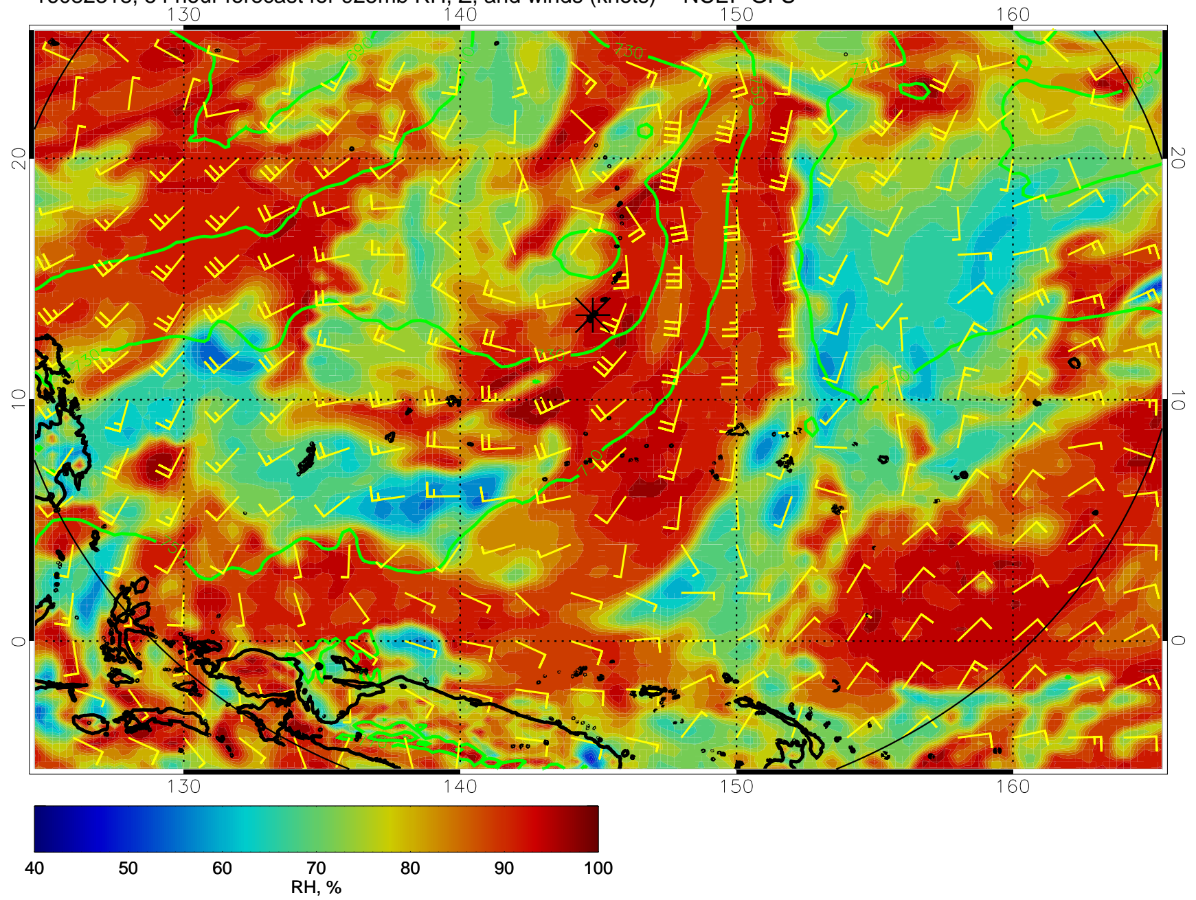
16082318, 54 hour forecast for 925mb RH, Z, and winds (knots) -- NCEP GFS
