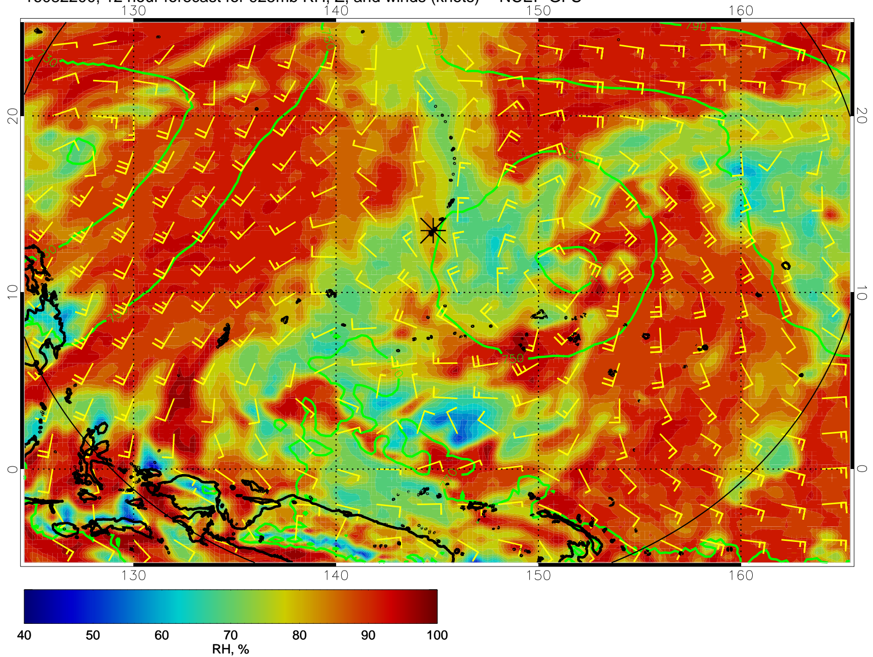
16082200, 12 hour forecast for 925mb RH, Z, and winds (knots) -- NCEP GFS
