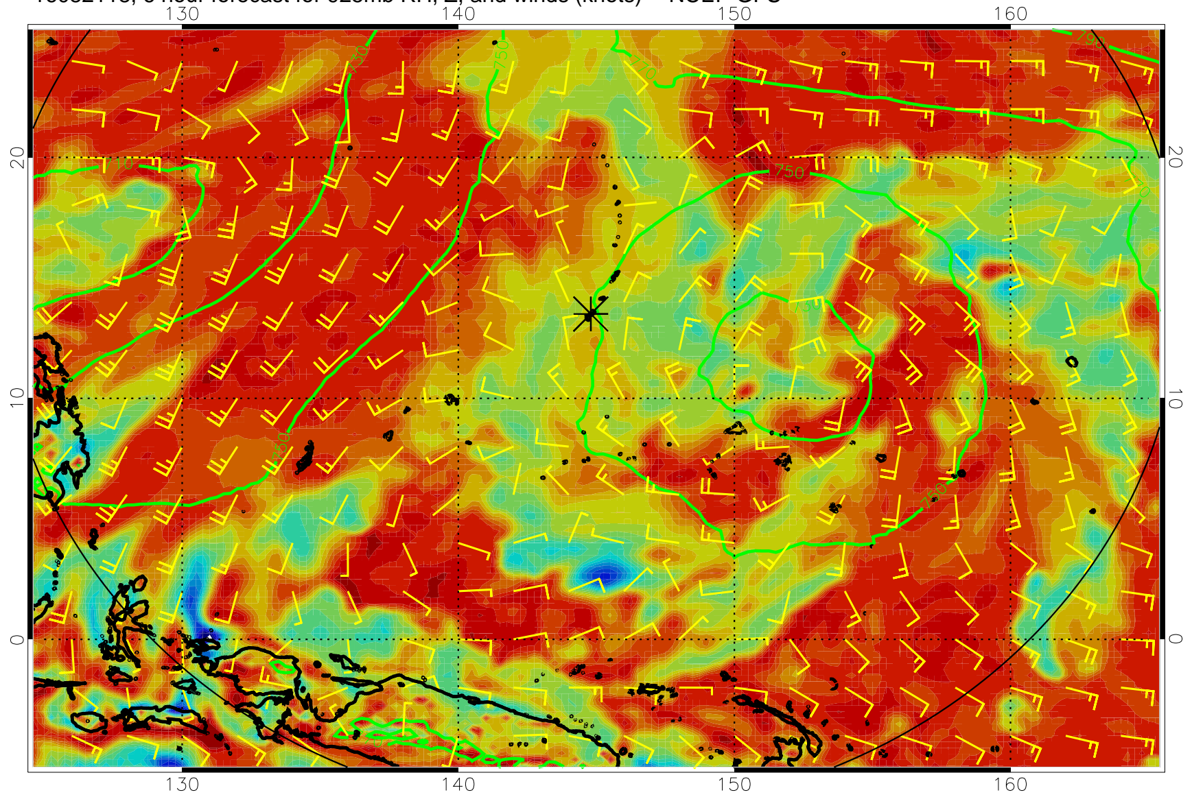
16082118, 6 hour forecast for 925mb RH, Z, and winds (knots) -- NCEP GFS
