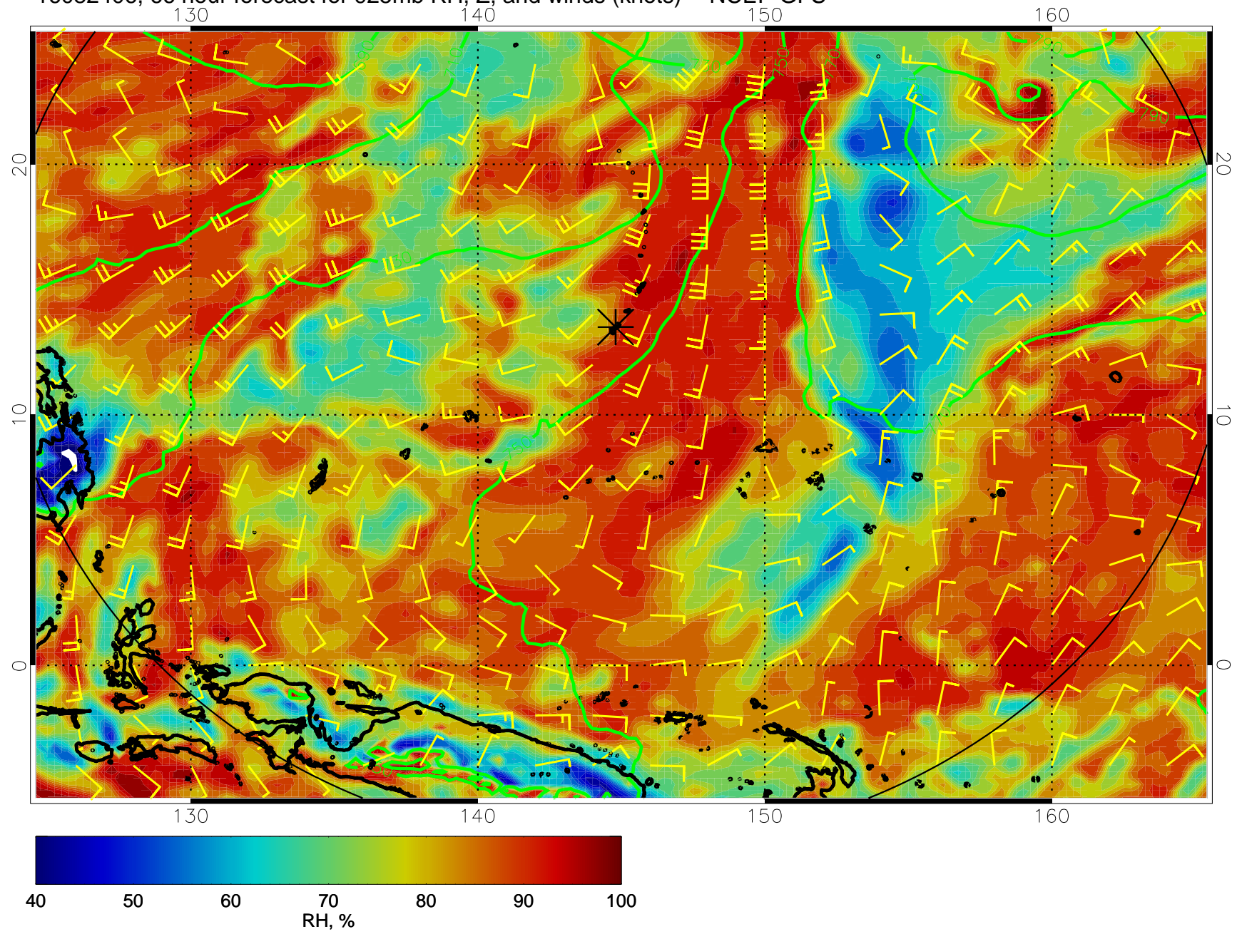
16082406, 66 hour forecast for 925mb RH, Z, and winds (knots) -- NCEP GFS
