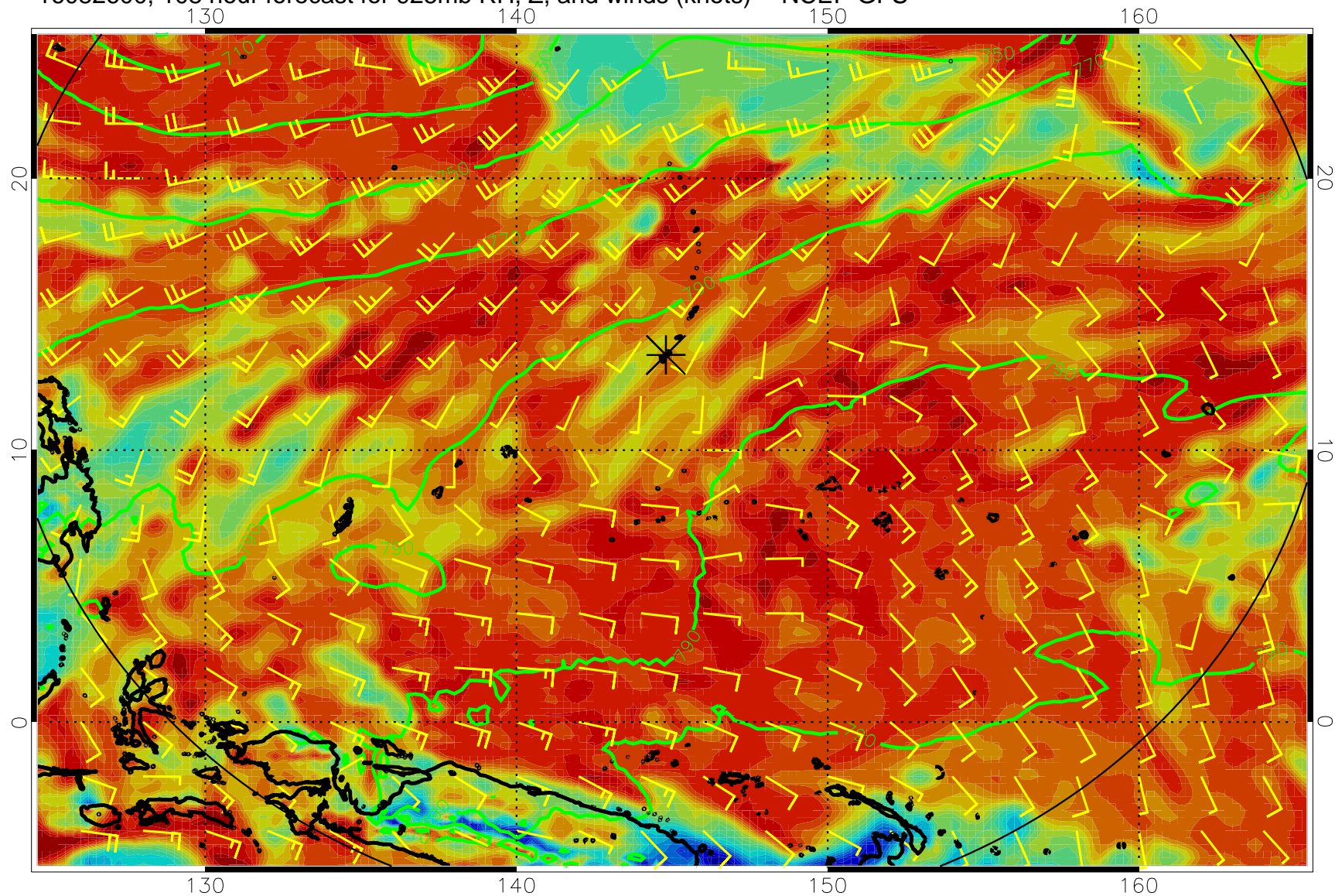
16082600, 108 hour forecast for 925mb RH, Z, and winds (knots) -- NCEP GFS
