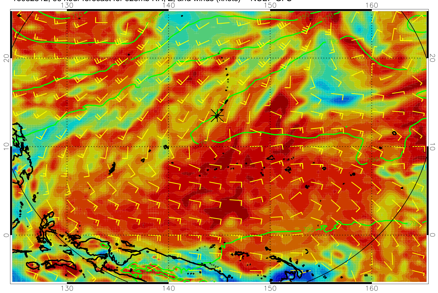
16082512, 96 hour forecast for 925mb RH, Z, and winds (knots) -- NCEP GFS
