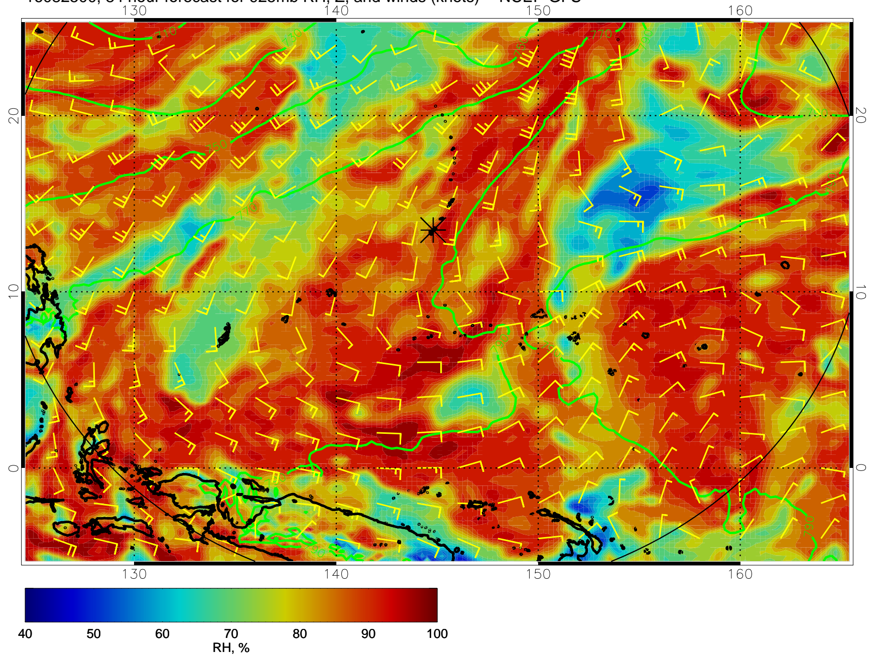
16082500, 84 hour forecast for 925mb RH, Z, and winds (knots) -- NCEP GFS
