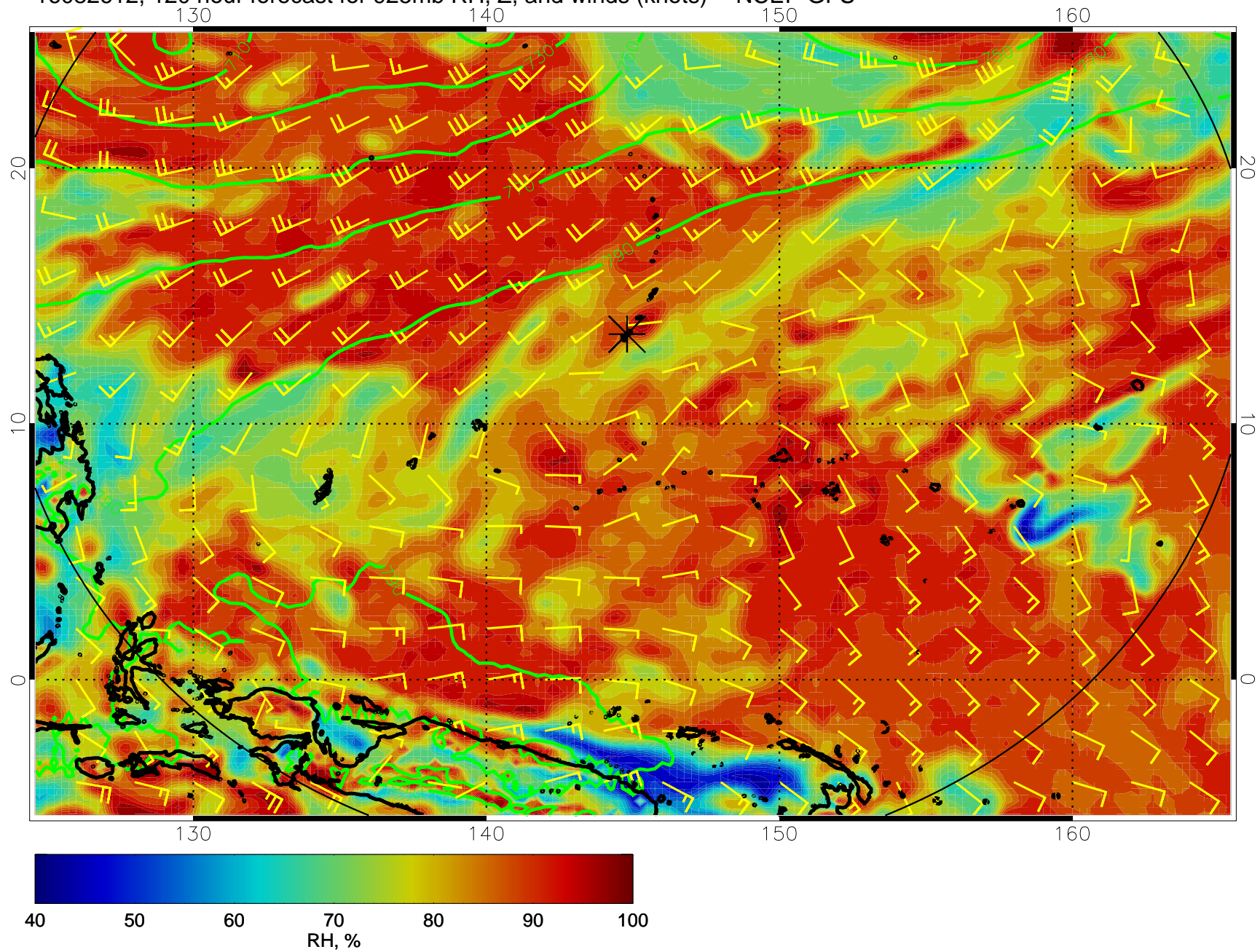
16082612, 120 hour forecast for 925mb RH, Z, and winds (knots) -- NCEP GFS
